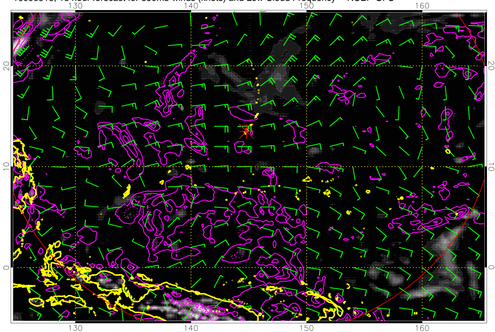
16090518, 18 hour forecast for 850mb winds (knots) and Low Cloud Frequency -- NCEP GFS
