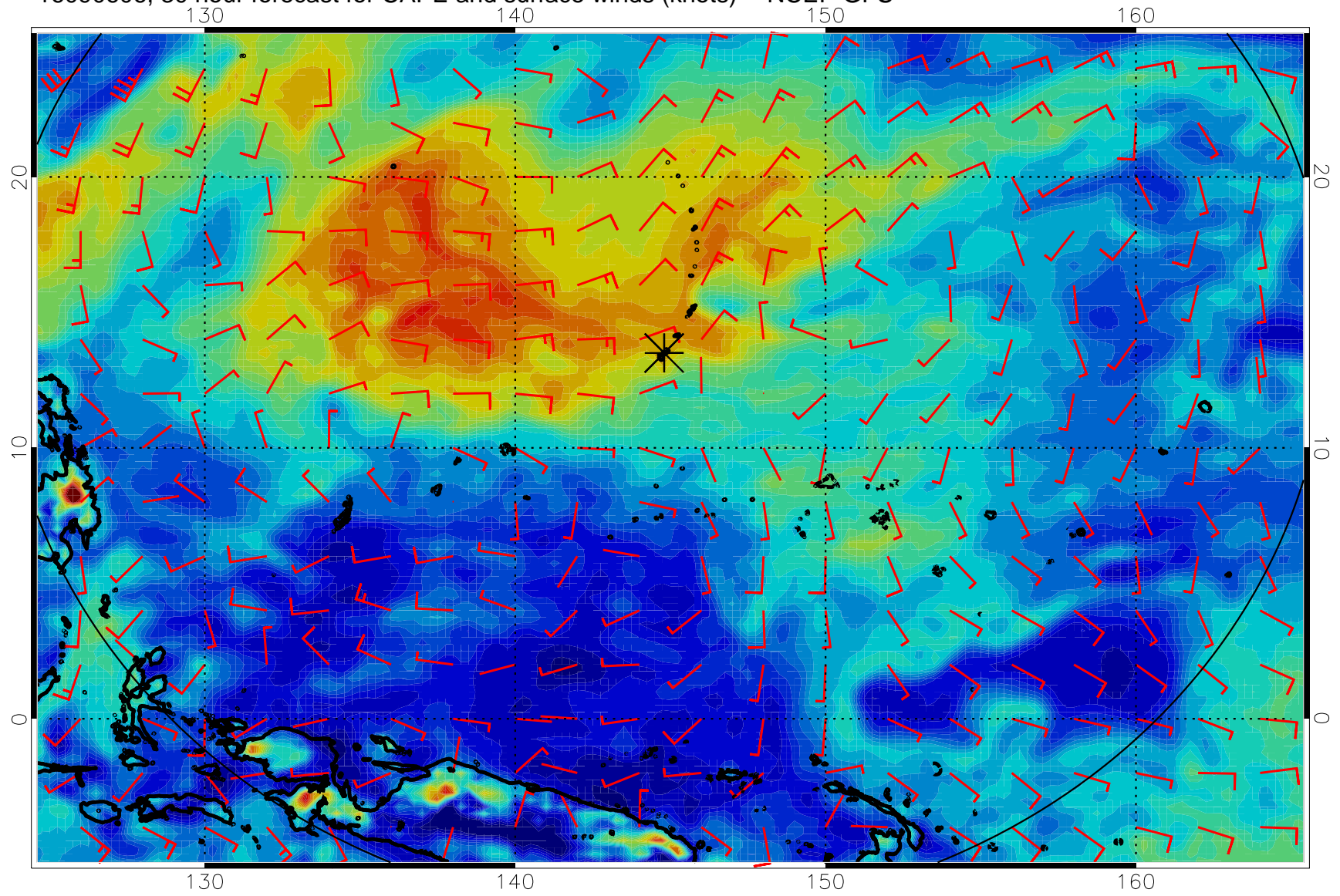
16090606, 30 hour forecast for CAPE and surface winds (knots) -- NCEP GFS
