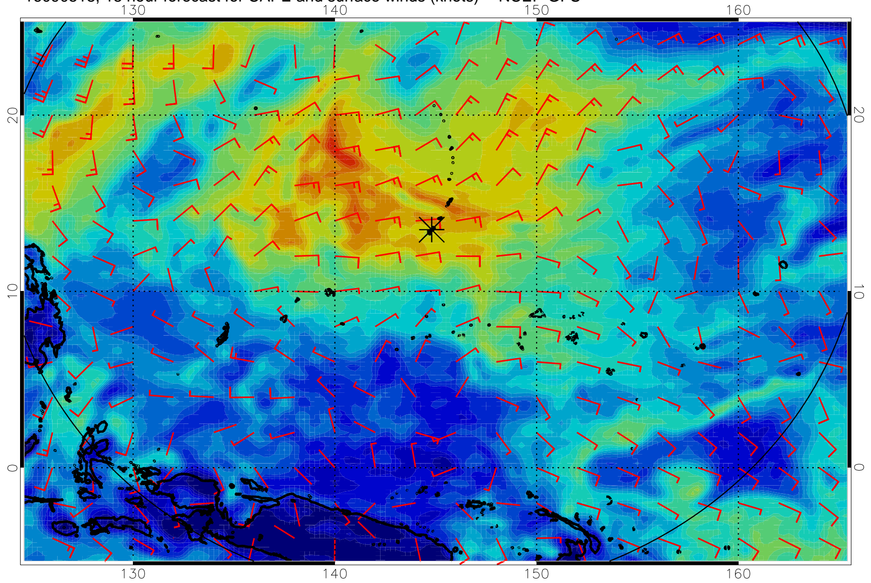
16090518, 18 hour forecast for CAPE and surface winds (knots) -- NCEP GFS
