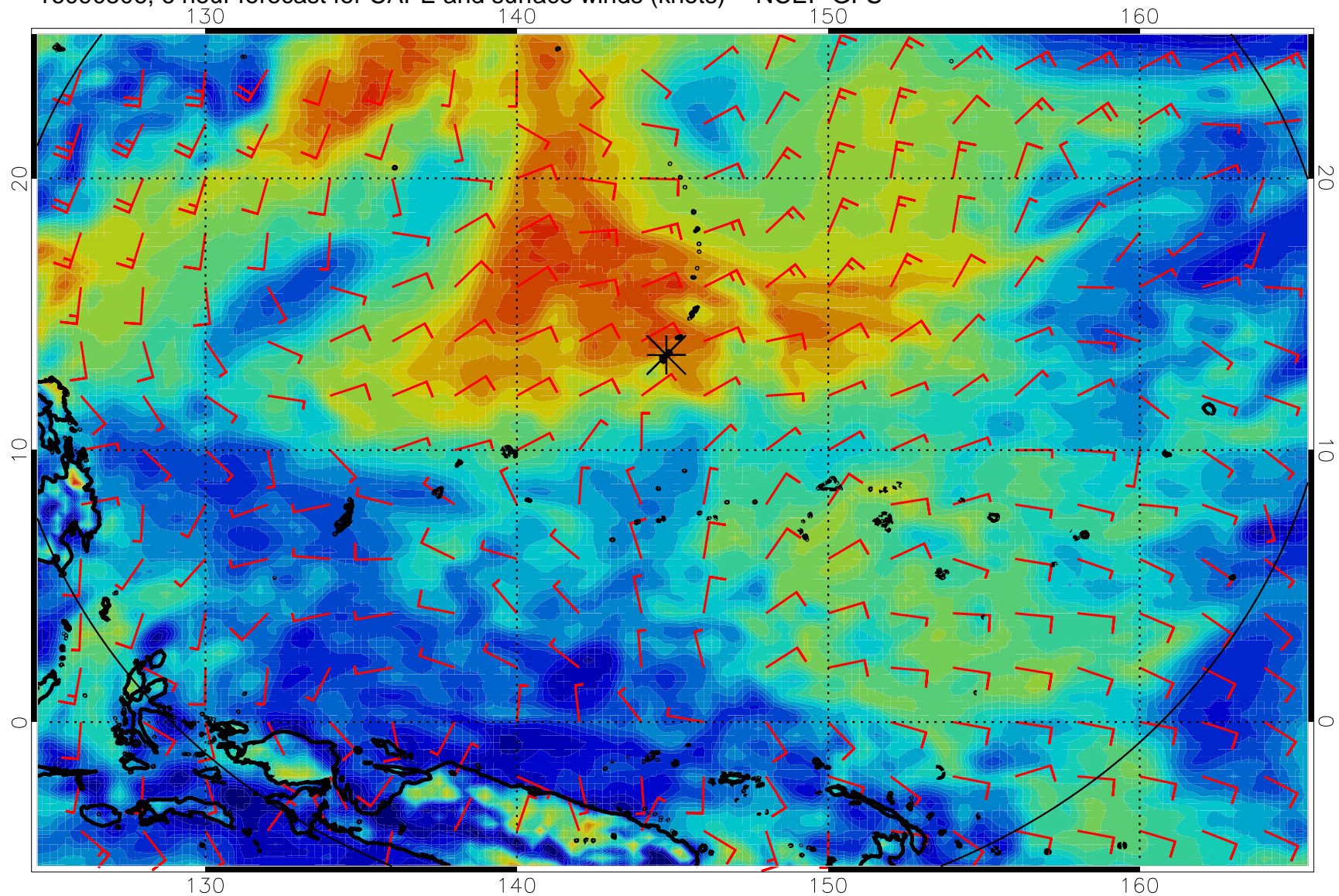
16090506, 6 hour forecast for CAPE and surface winds (knots) -- NCEP GFS
