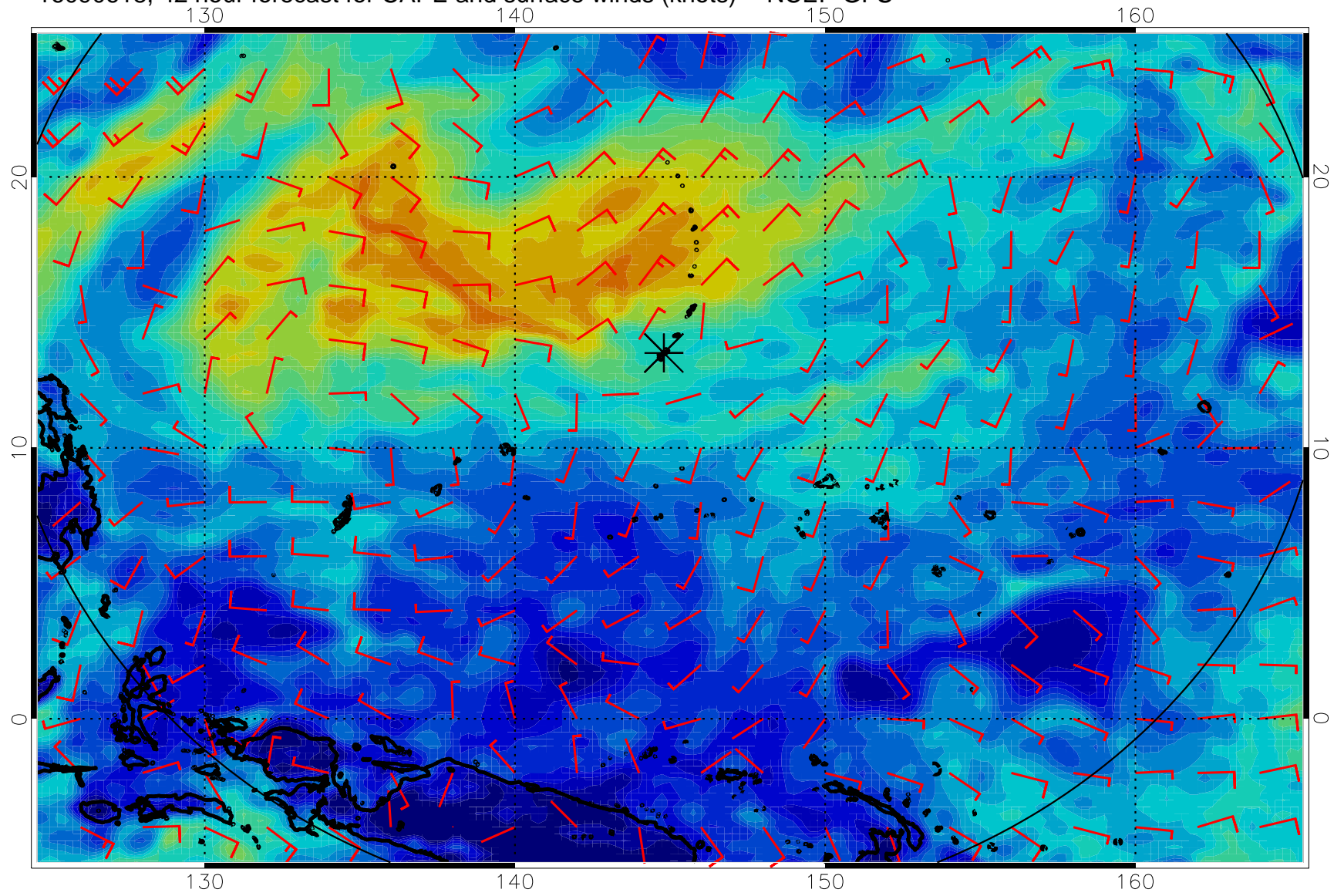
16090618, 42 hour forecast for CAPE and surface winds (knots) -- NCEP GFS
