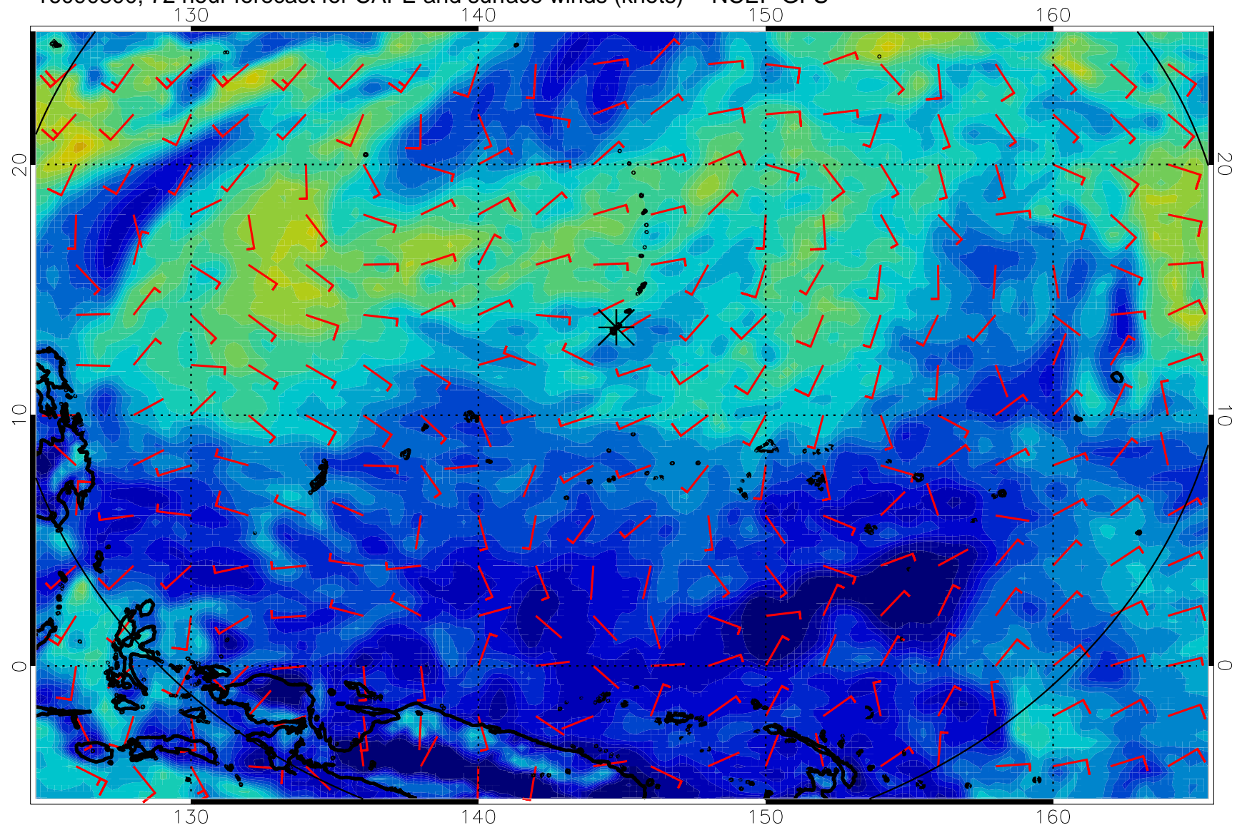
16090800, 72 hour forecast for CAPE and surface winds (knots) -- NCEP GFS
