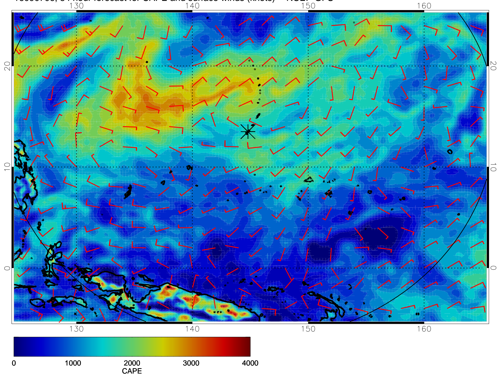
16090706, 54 hour forecast for CAPE and surface winds (knots) -- NCEP GFS
