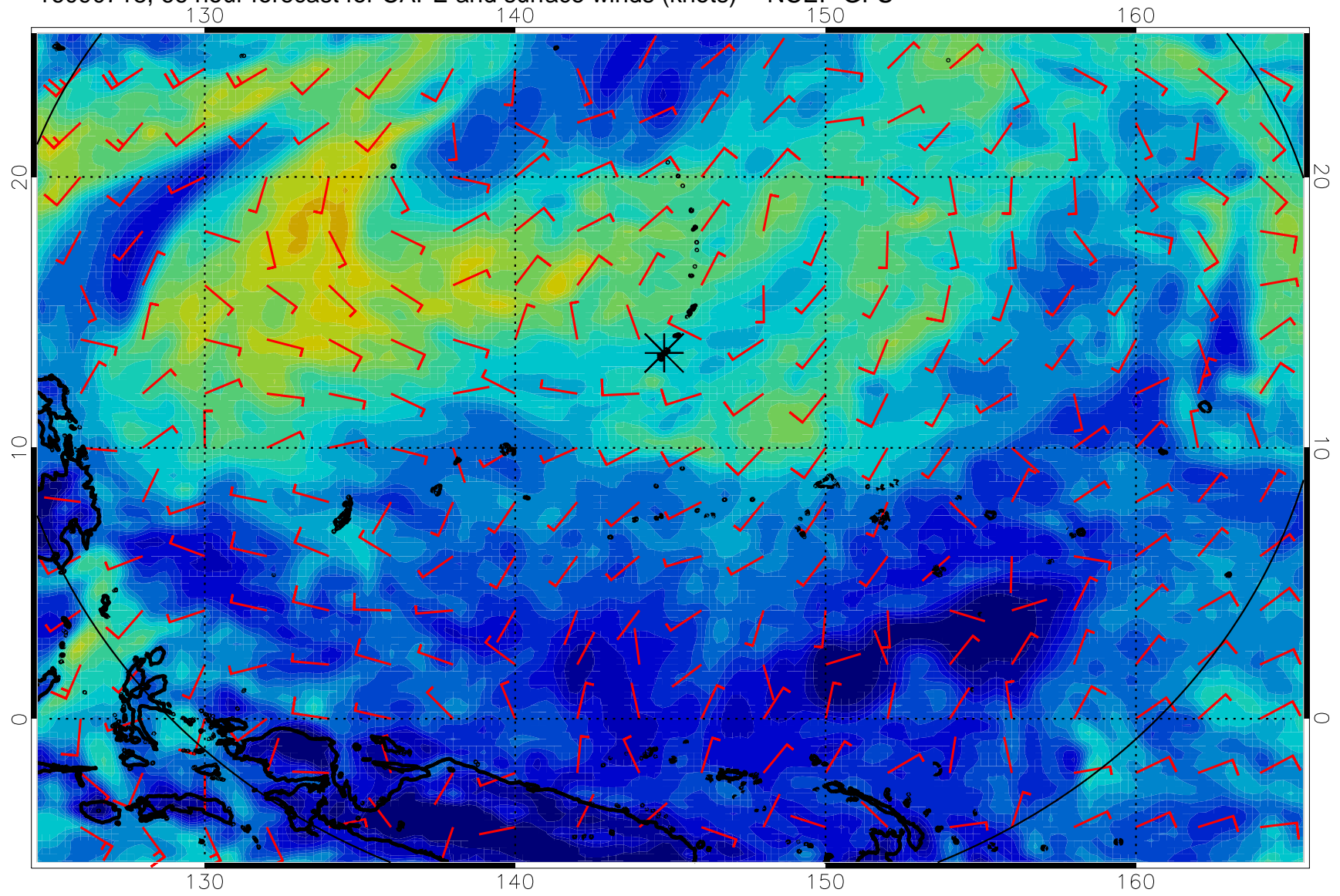
16090718, 66 hour forecast for CAPE and surface winds (knots) -- NCEP GFS
