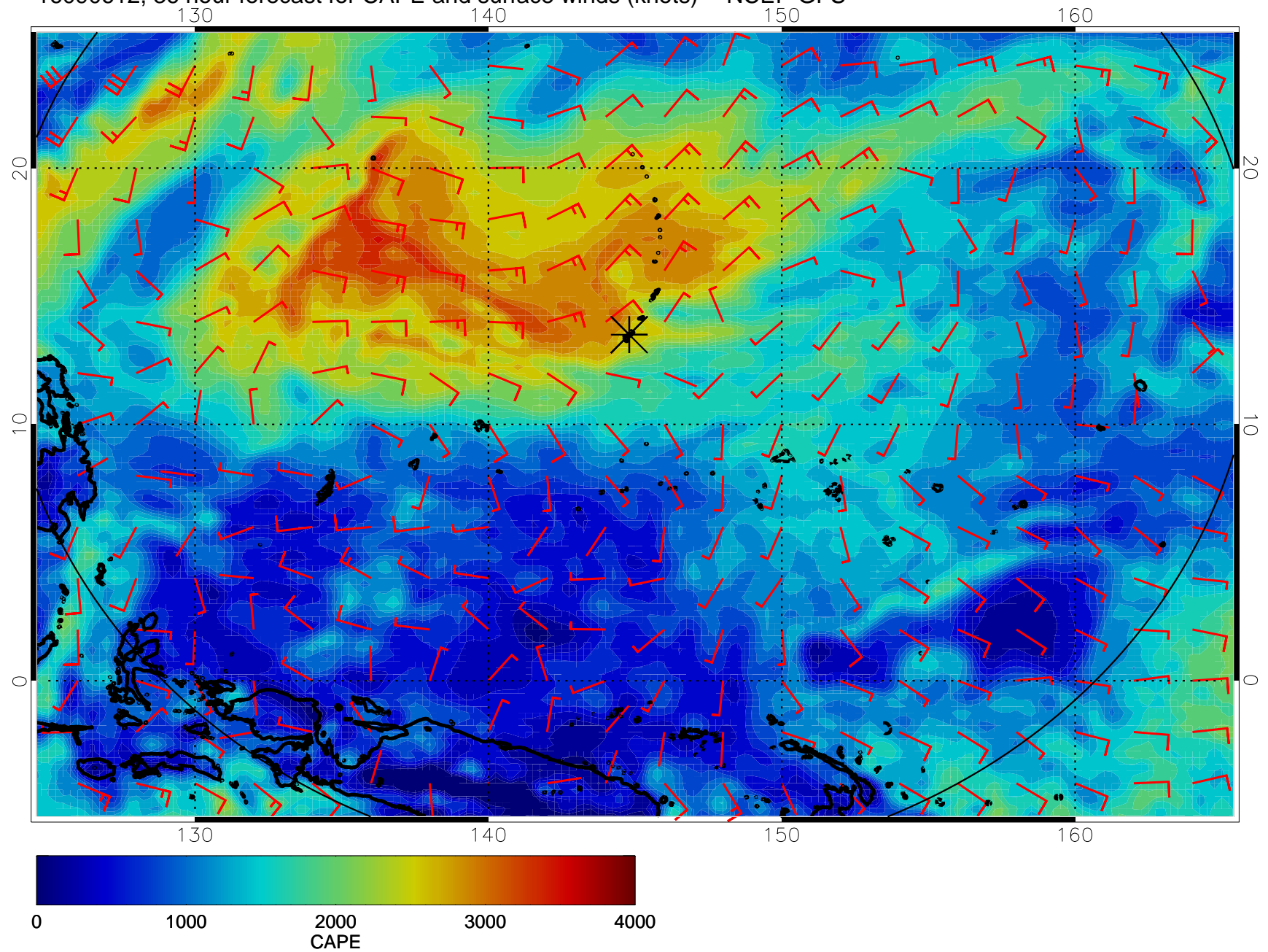
16090612, 36 hour forecast for CAPE and surface winds (knots) -- NCEP GFS
