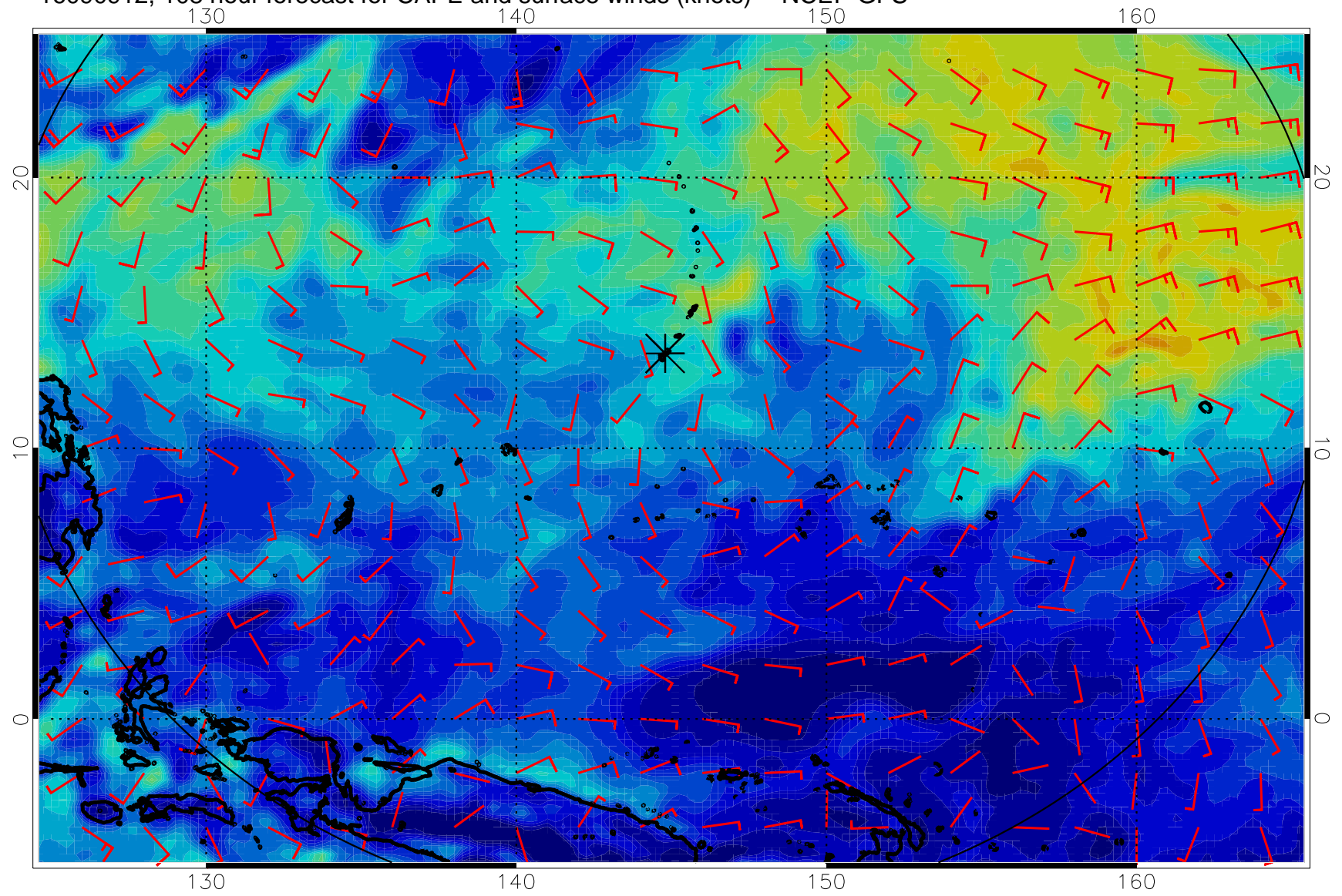
16090912, 108 hour forecast for CAPE and surface winds (knots) -- NCEP GFS
