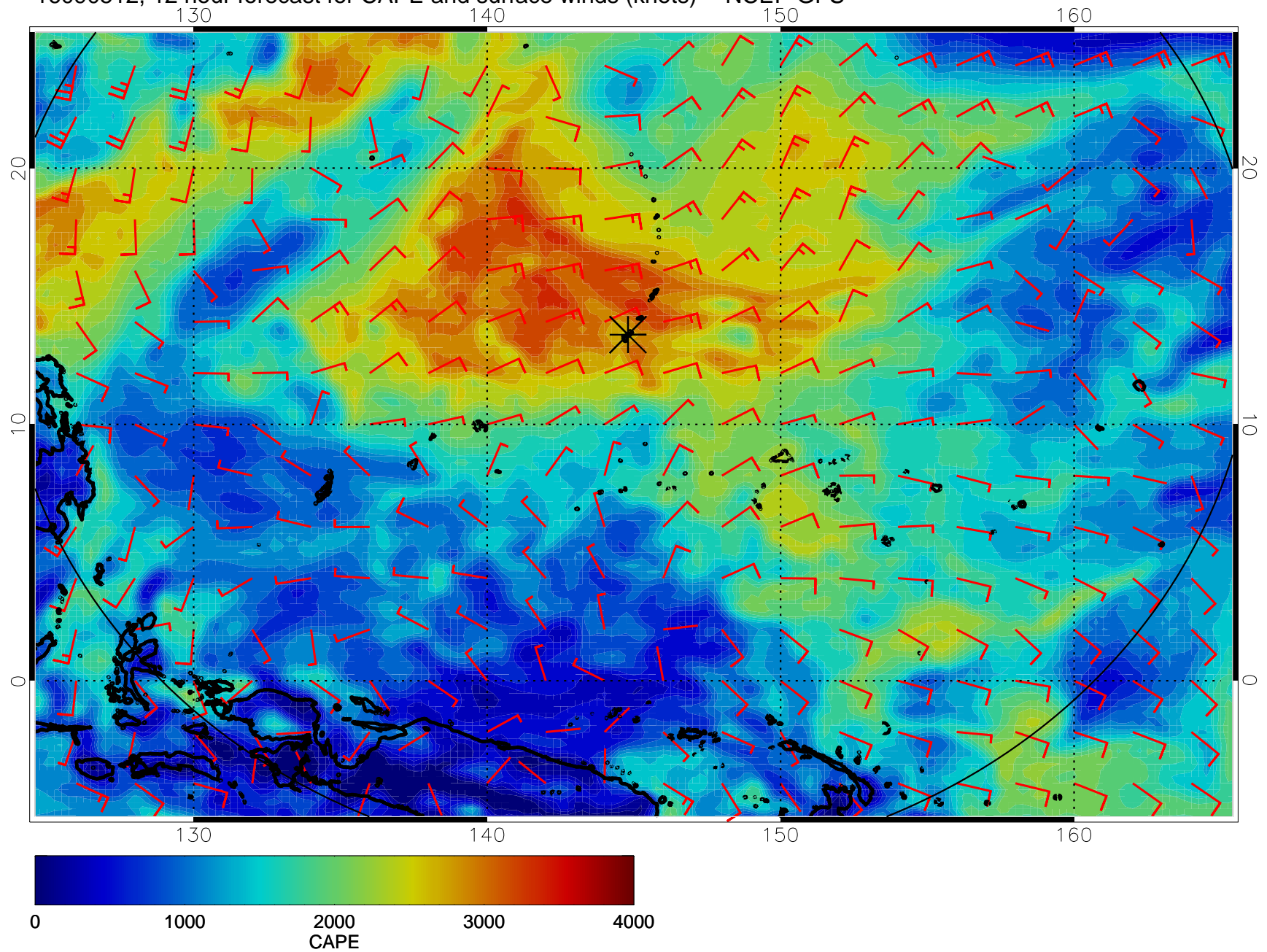
16090512, 12 hour forecast for CAPE and surface winds (knots) -- NCEP GFS
