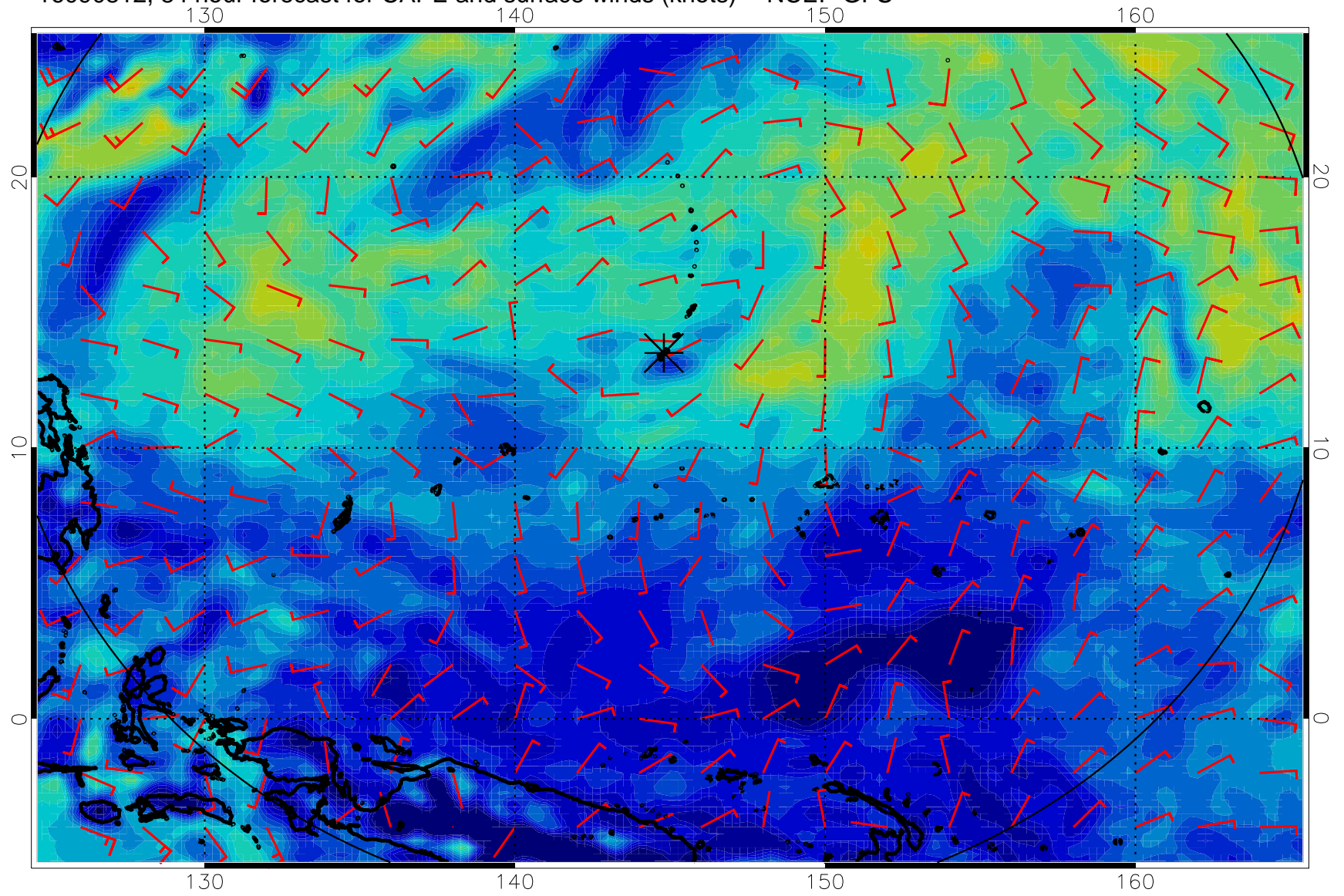
16090812, 84 hour forecast for CAPE and surface winds (knots) -- NCEP GFS
