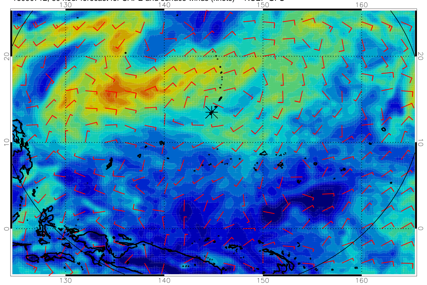
16090712, 60 hour forecast for CAPE and surface winds (knots) -- NCEP GFS
