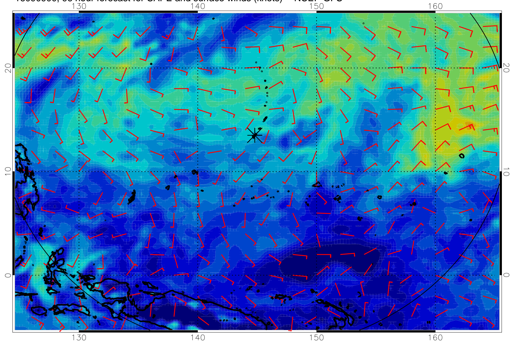
16090900, 96 hour forecast for CAPE and surface winds (knots) -- NCEP GFS
