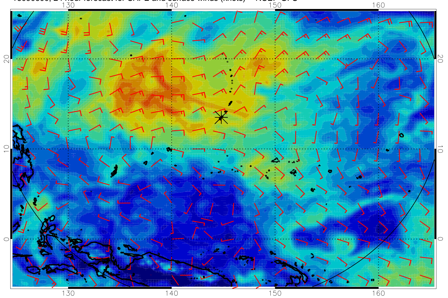
16090600, 24 hour forecast for CAPE and surface winds (knots) -- NCEP GFS
