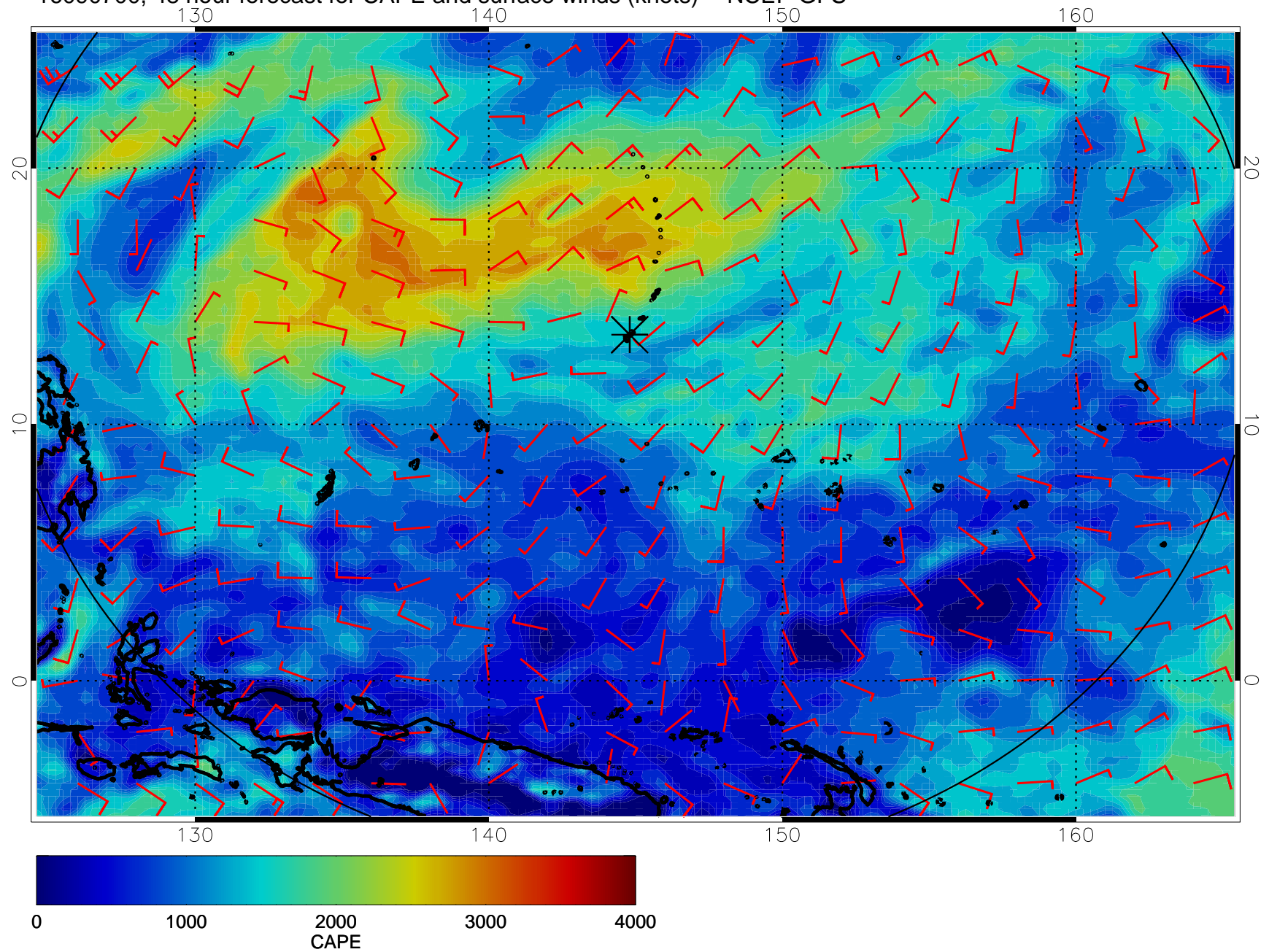
16090700, 48 hour forecast for CAPE and surface winds (knots) -- NCEP GFS
