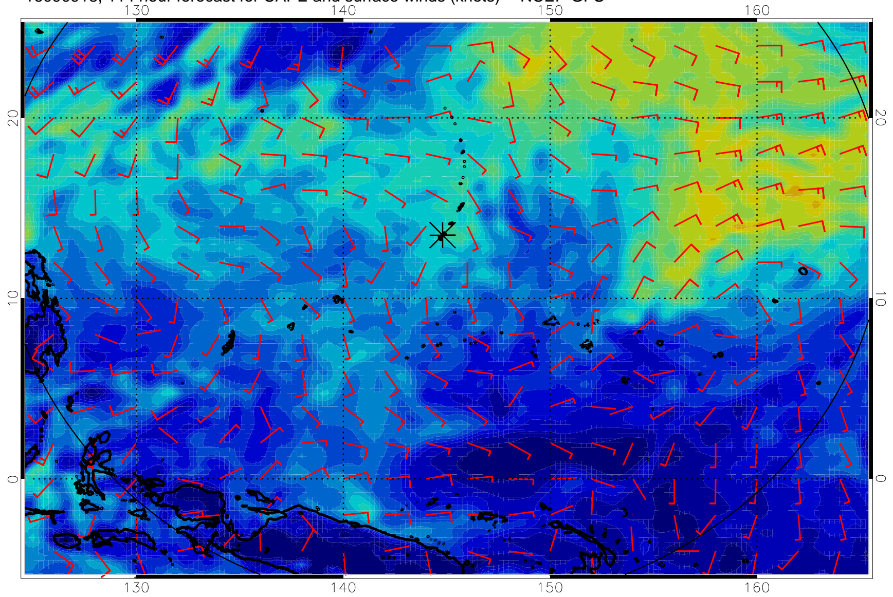
16090918, 114 hour forecast for CAPE and surface winds (knots) -- NCEP GFS
