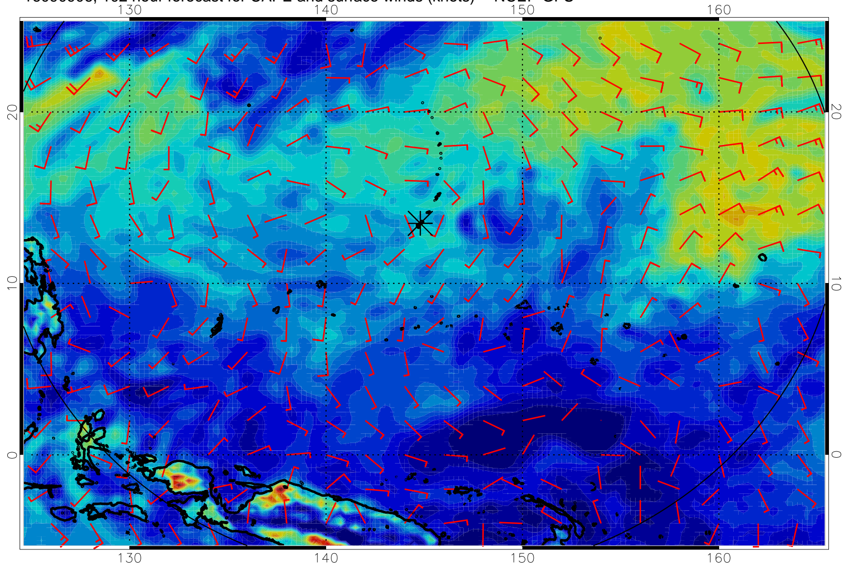
16090906, 102 hour forecast for CAPE and surface winds (knots) -- NCEP GFS
