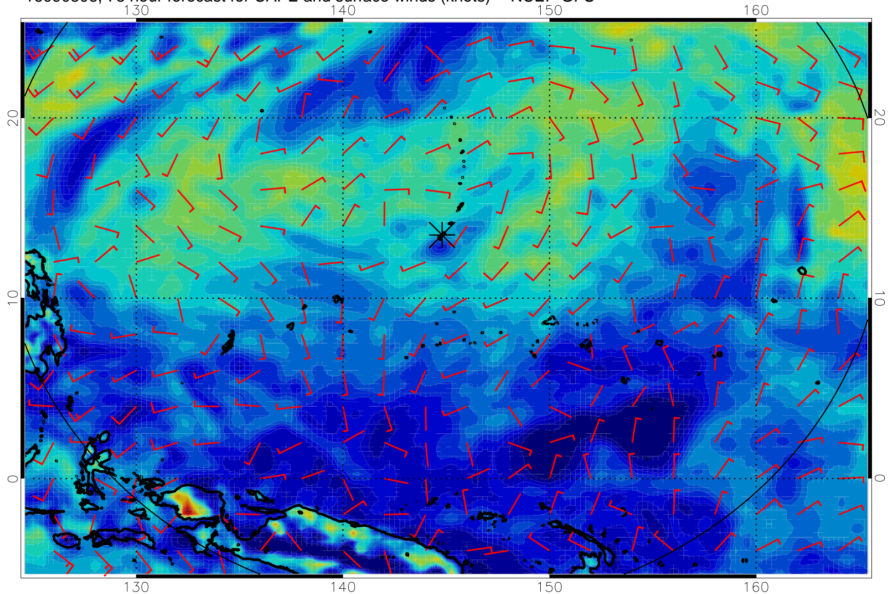
16090806, 78 hour forecast for CAPE and surface winds (knots) -- NCEP GFS
