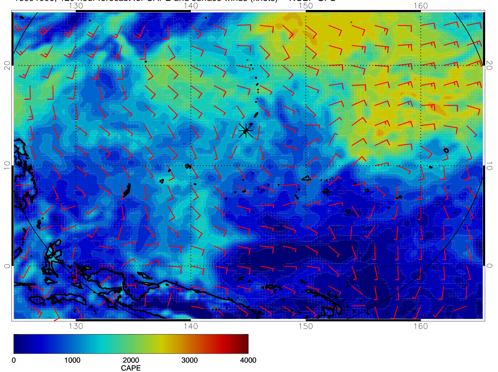
16091000, 120 hour forecast for CAPE and surface winds (knots) -- NCEP GFS
