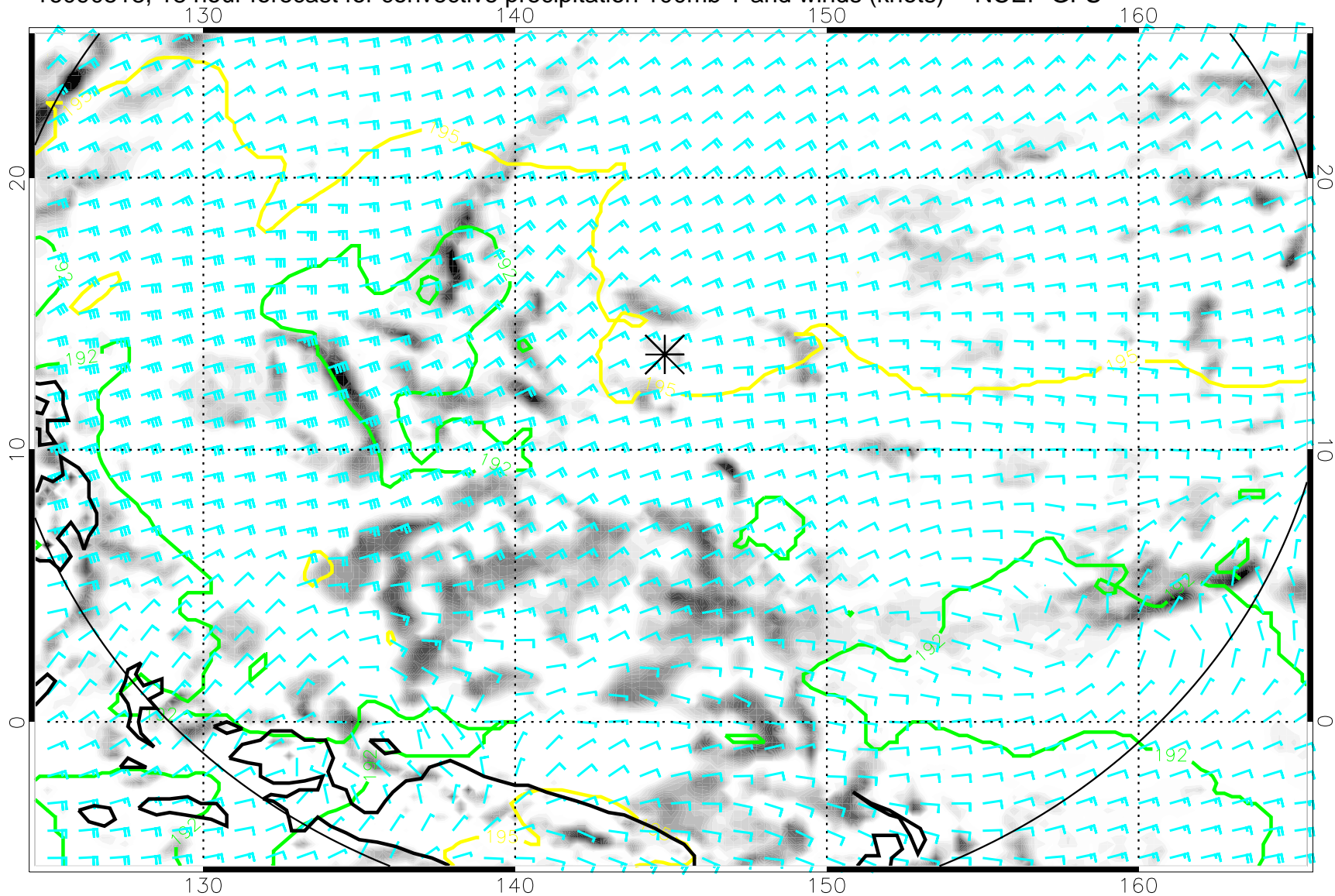
16090518, 18 hour forecast for convective precipitation 100mb T and winds (knots) -- NCEP GFS
