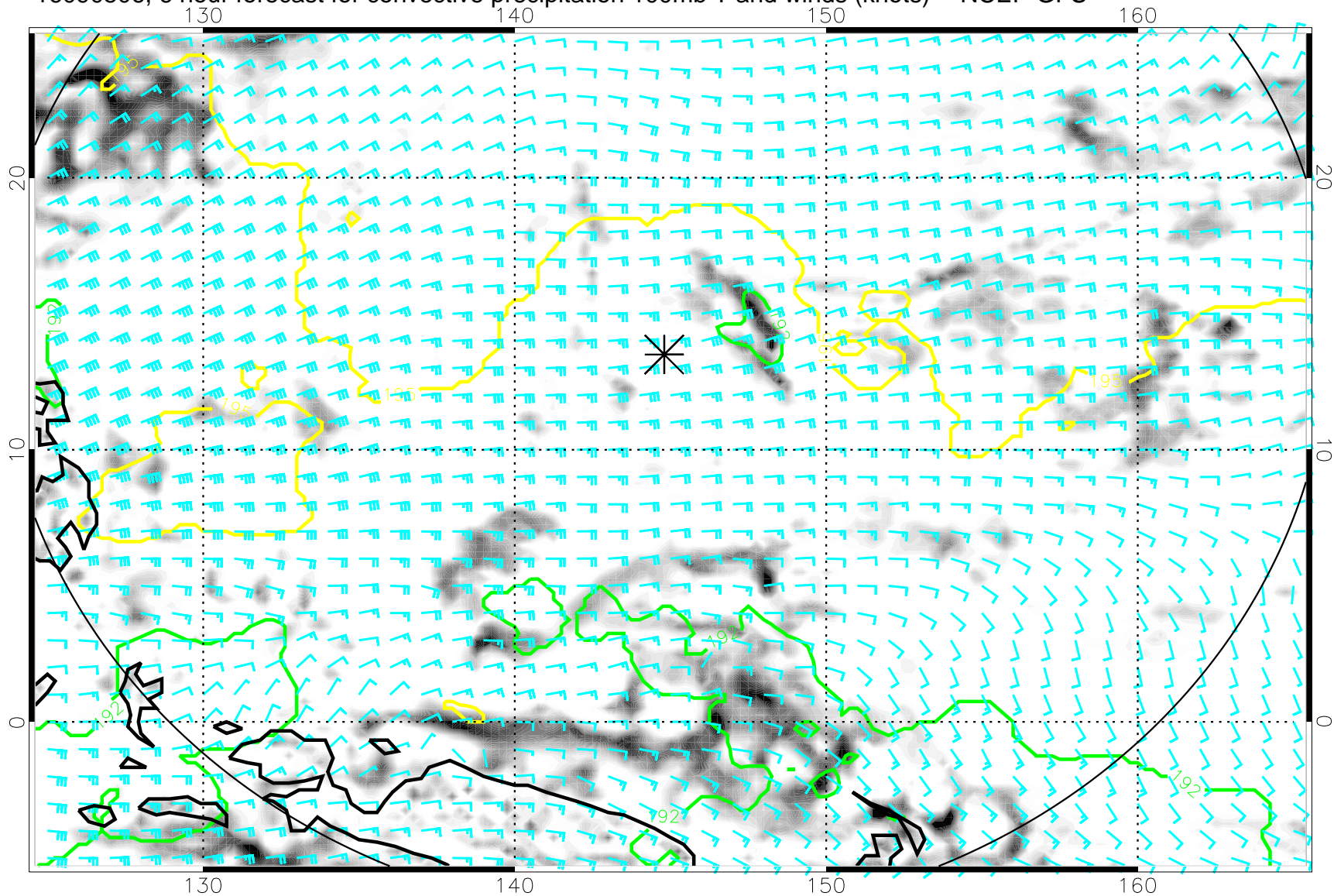
16090506, 6 hour forecast for convective precipitation 100mb T and winds (knots) -- NCEP GFS
