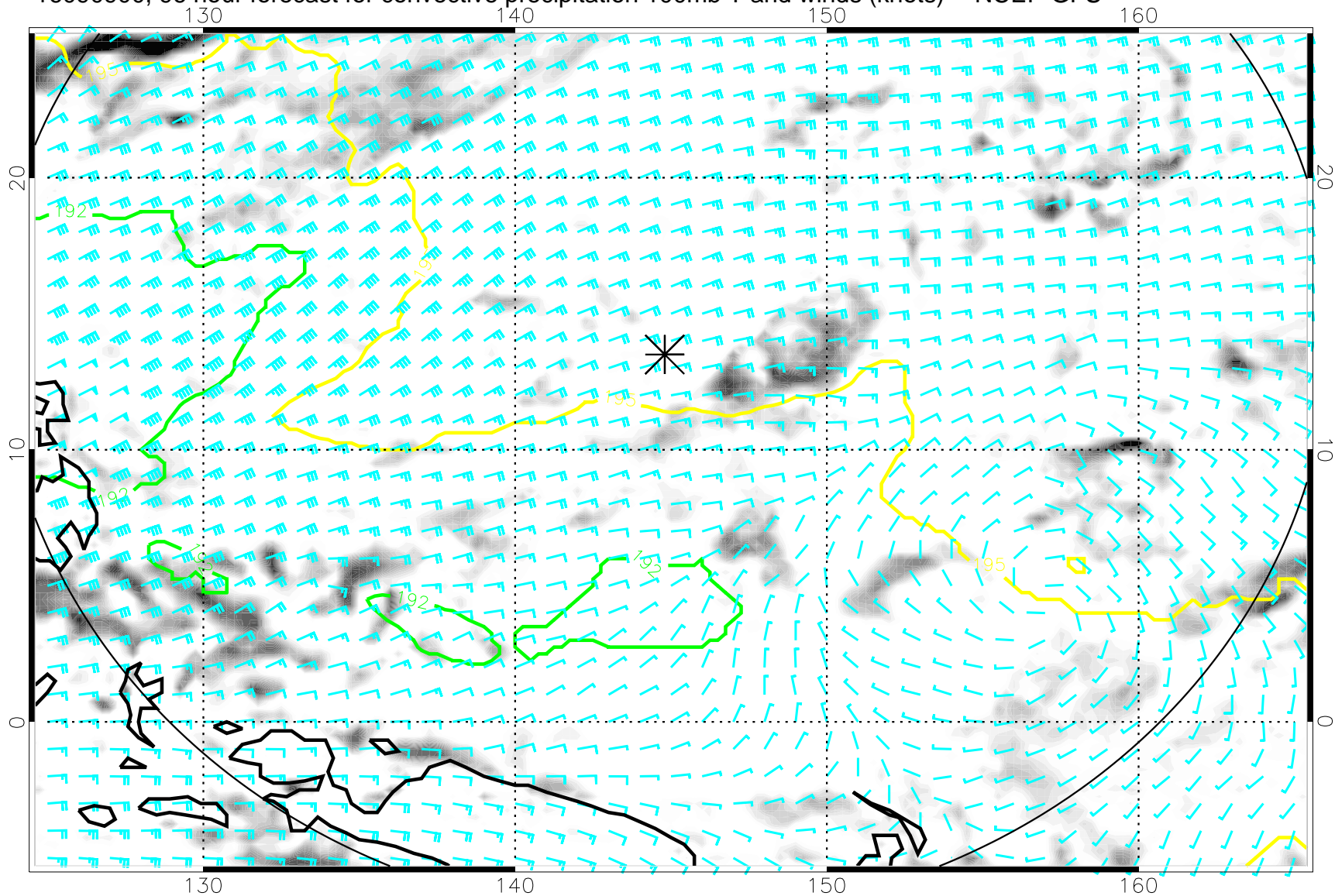
16090900, 96 hour forecast for convective precipitation 100mb T and winds (knots) -- NCEP GFS
