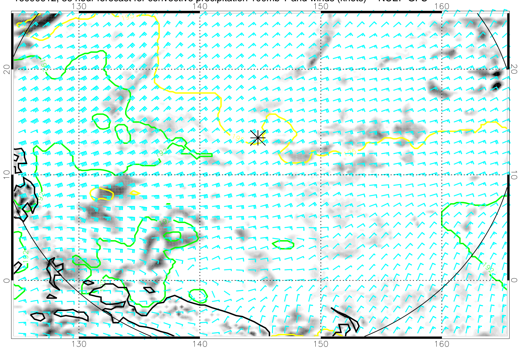
16090612, 36 hour forecast for convective precipitation 100mb T and winds (knots) -- NCEP GFS
