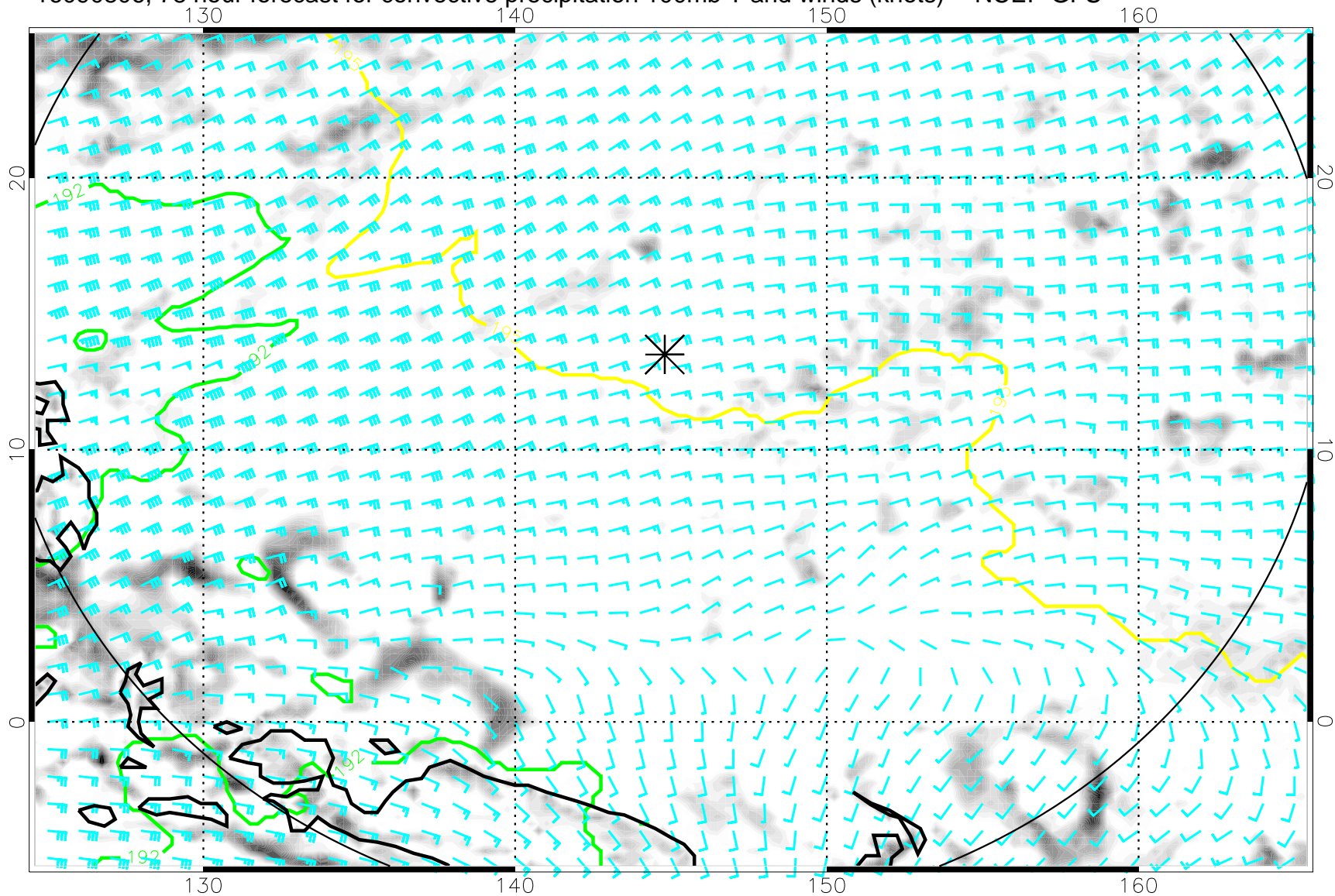
16090806, 78 hour forecast for convective precipitation 100mb T and winds (knots) -- NCEP GFS
