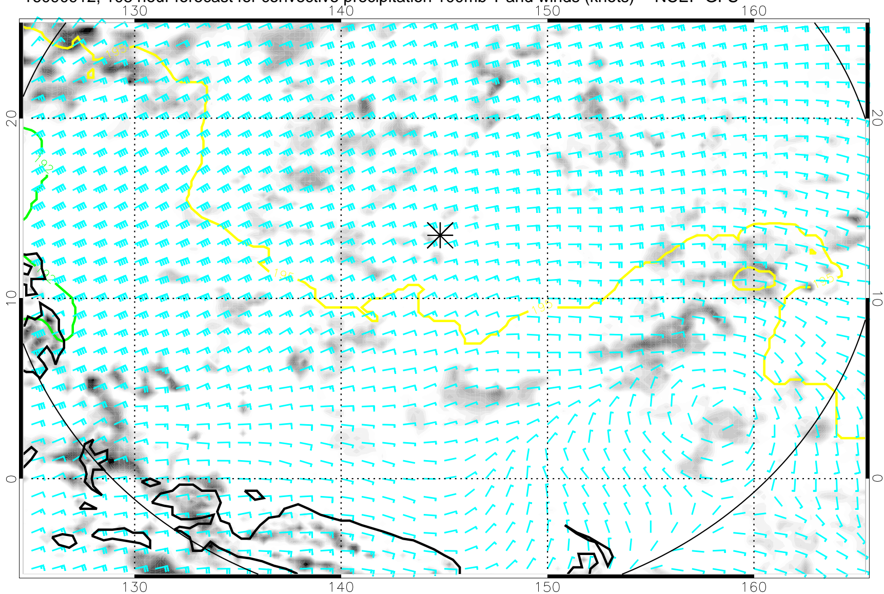
16090912, 108 hour forecast for convective precipitation 100mb T and winds (knots) -- NCEP GFS
