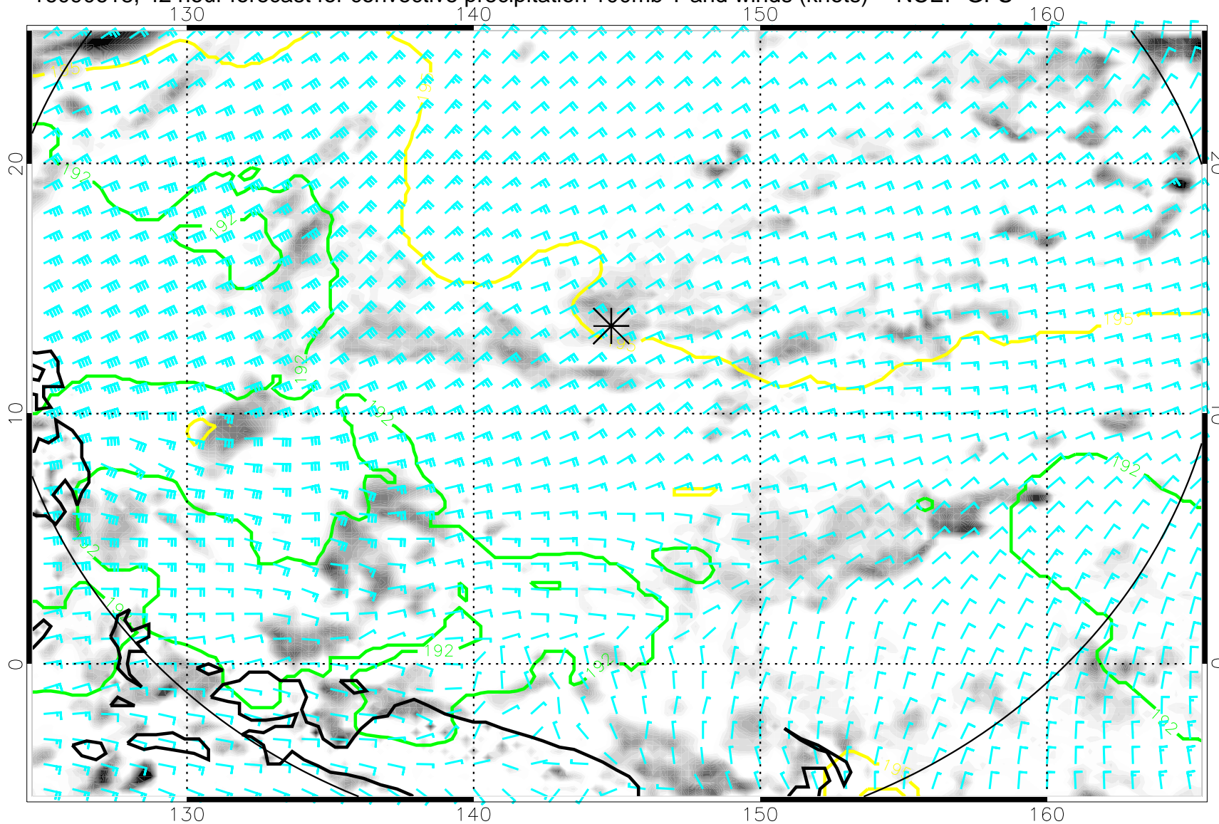
16090618, 42 hour forecast for convective precipitation 100mb T and winds (knots) -- NCEP GFS
