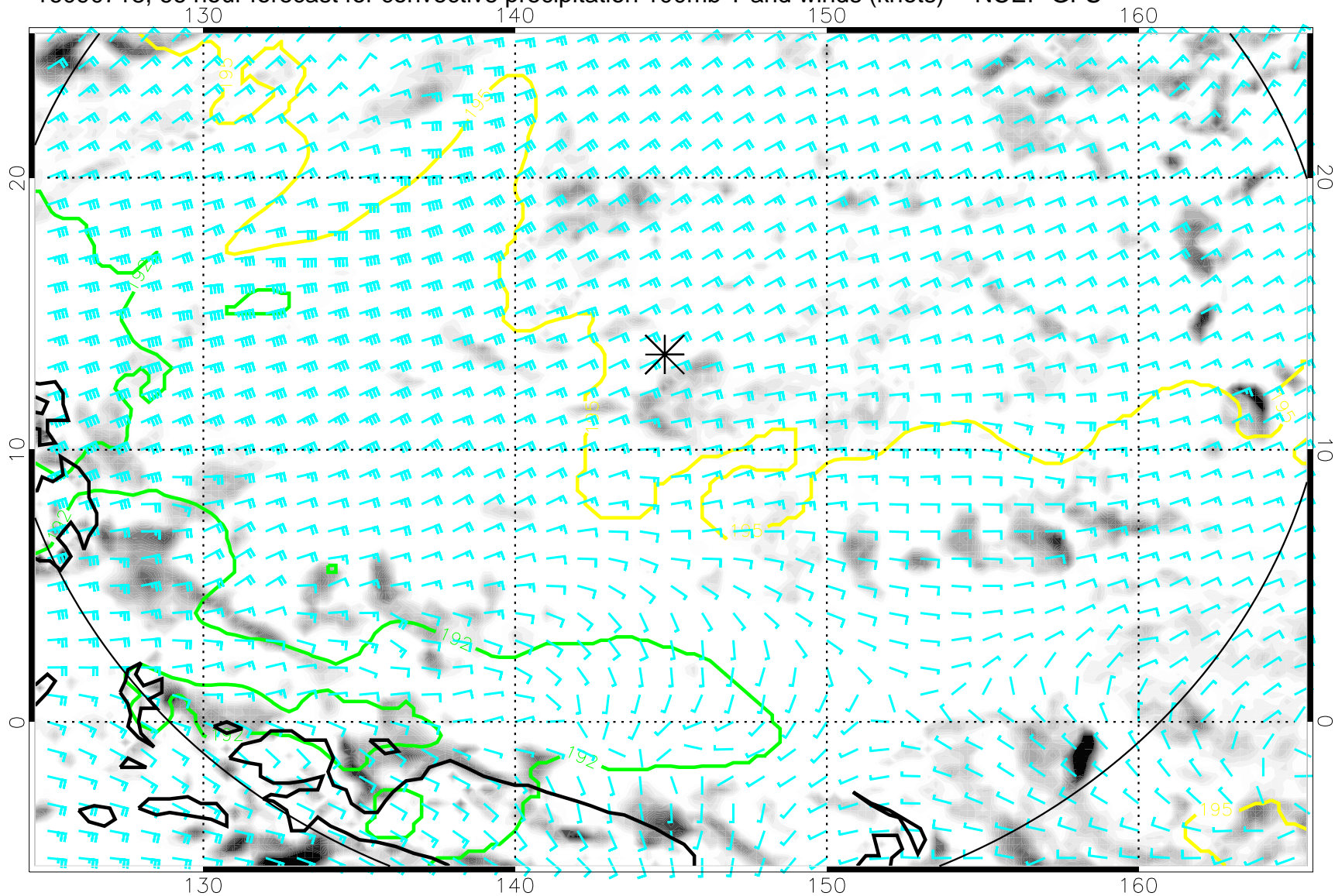
16090718, 66 hour forecast for convective precipitation 100mb T and winds (knots) -- NCEP GFS
