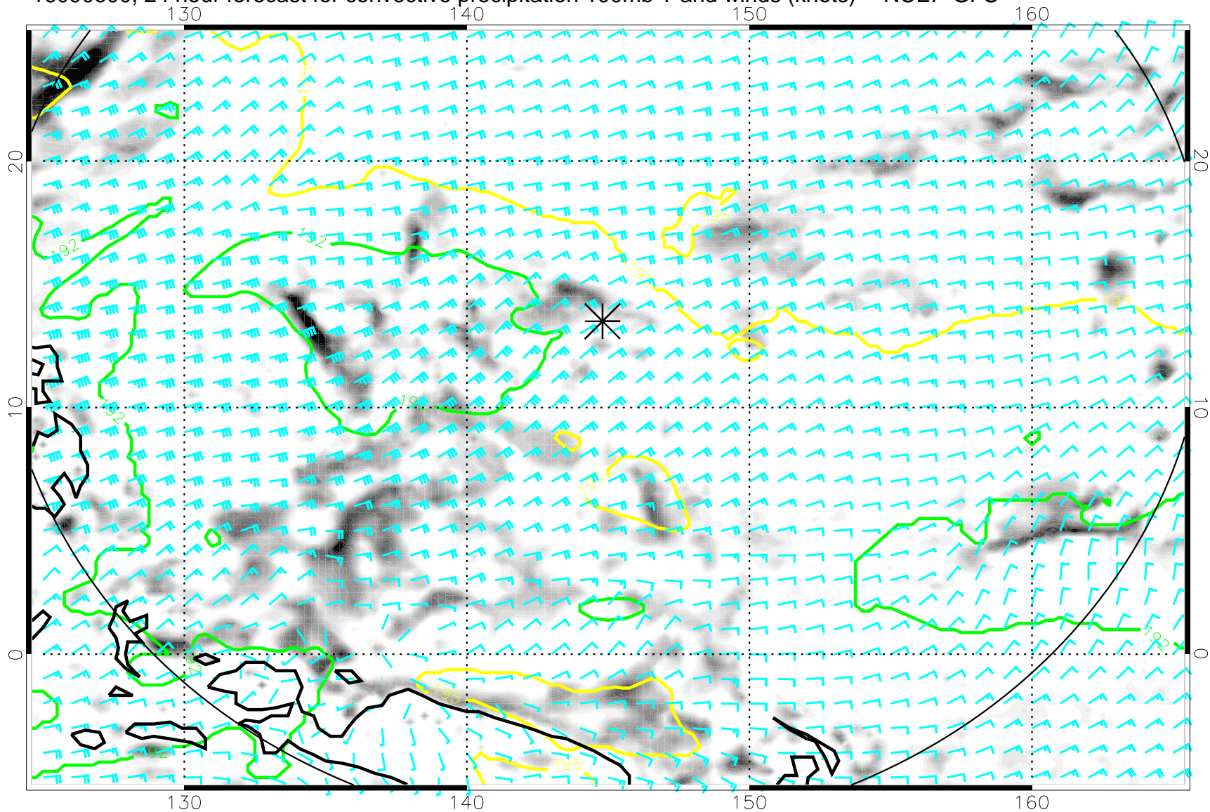
16090600, 24 hour forecast for convective precipitation 100mb T and winds (knots) -- NCEP GFS
