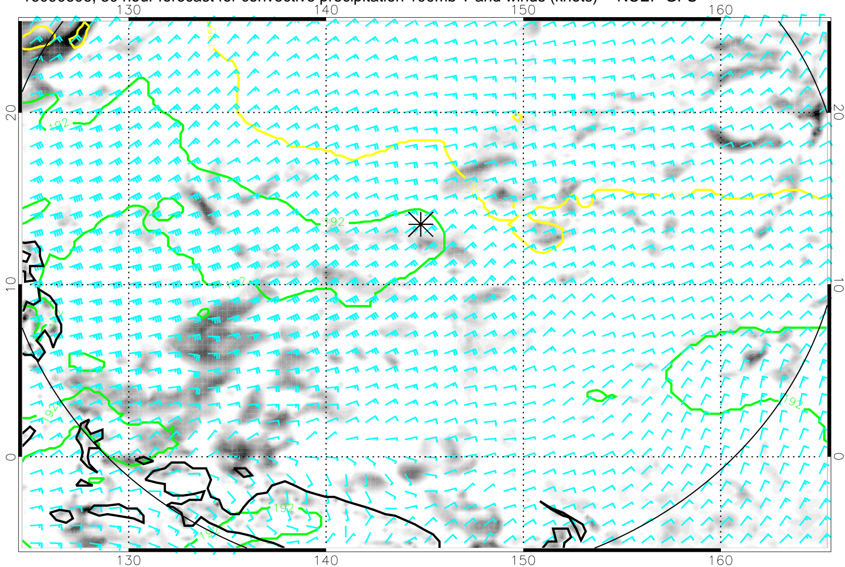
16090606, 30 hour forecast for convective precipitation 100mb T and winds (knots) -- NCEP GFS
