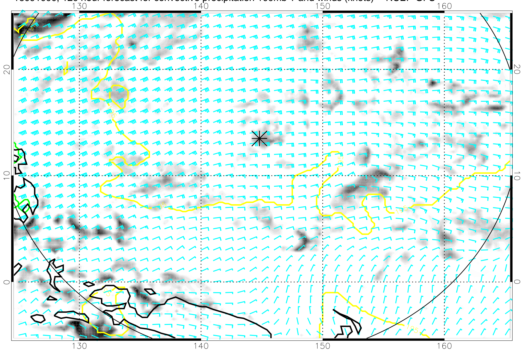
16091000, 120 hour forecast for convective precipitation 100mb T and winds (knots) -- NCEP GFS
