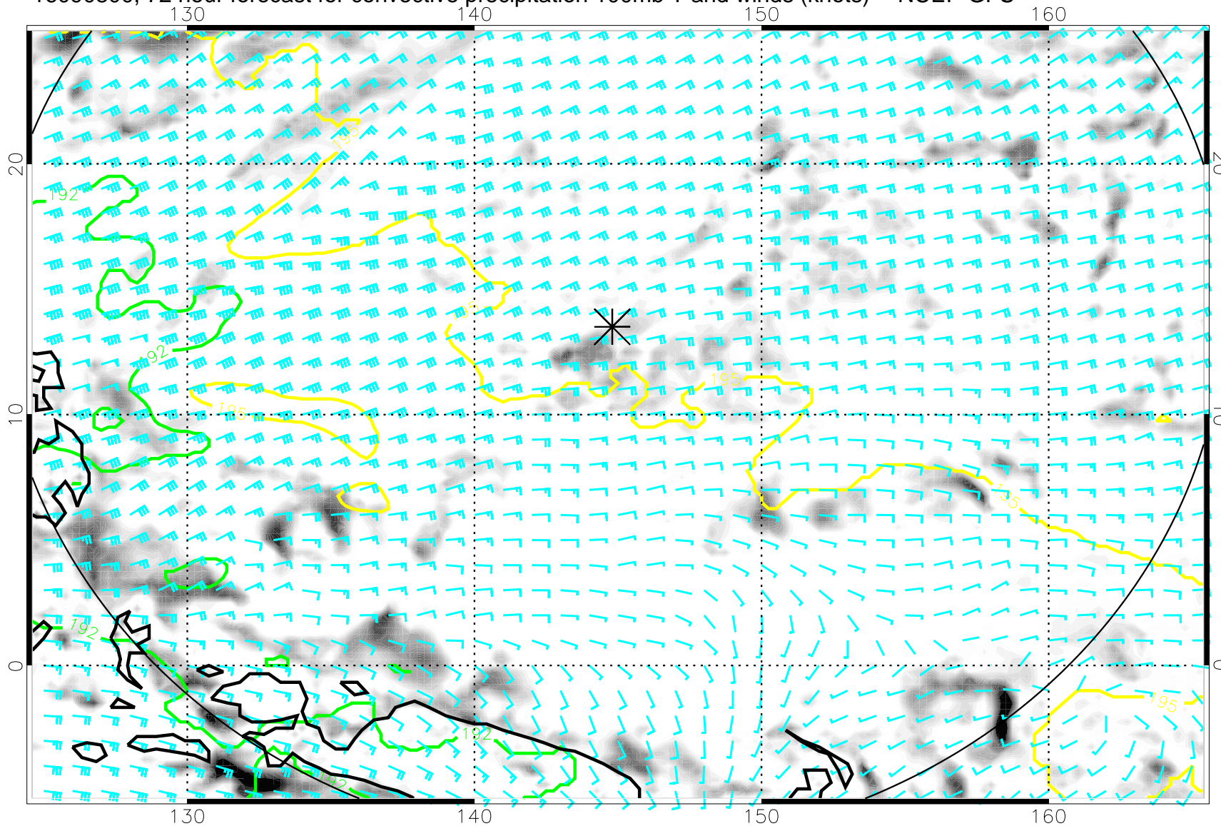
16090800, 72 hour forecast for convective precipitation 100mb T and winds (knots) -- NCEP GFS
