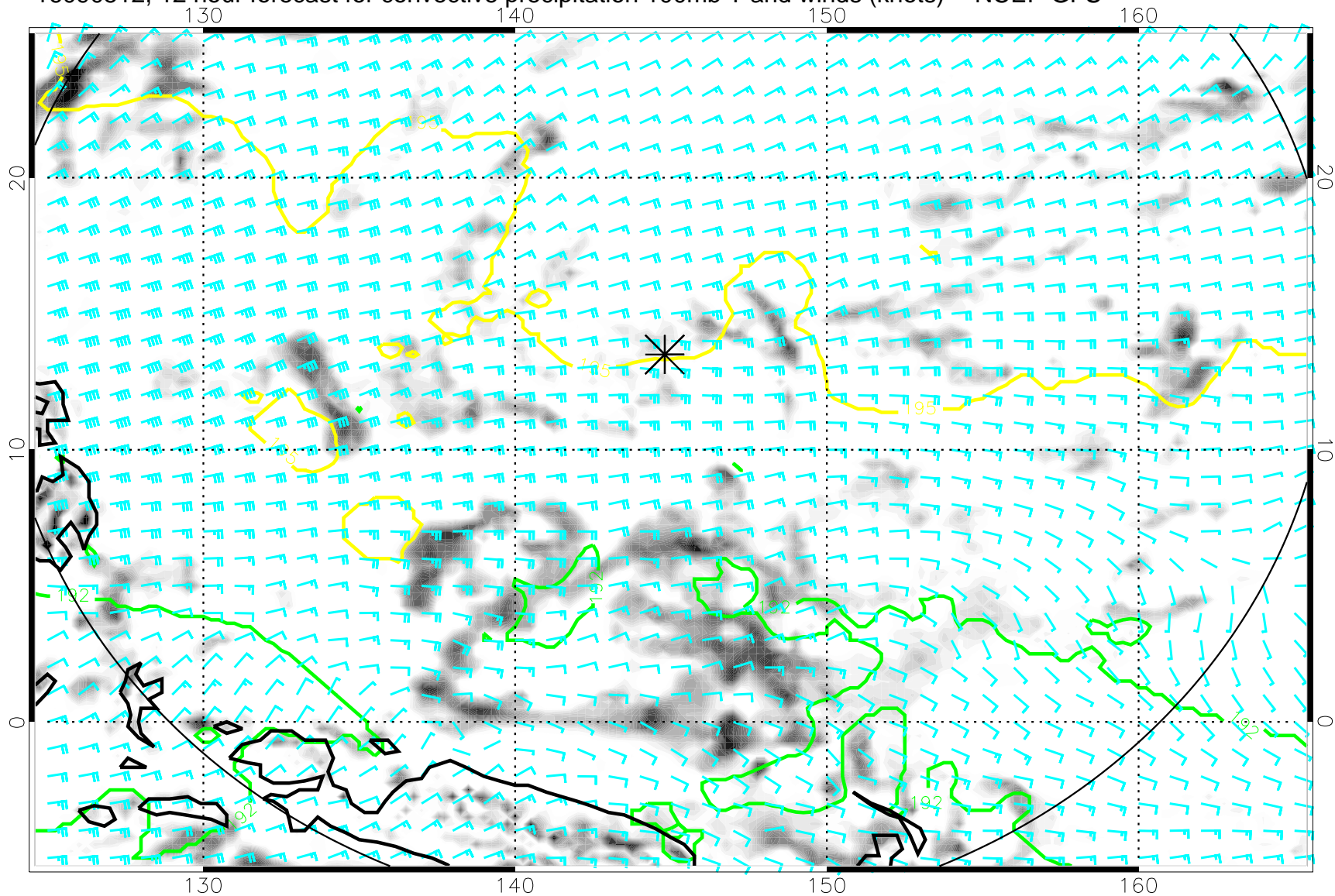
16090512, 12 hour forecast for convective precipitation 100mb T and winds (knots) -- NCEP GFS
