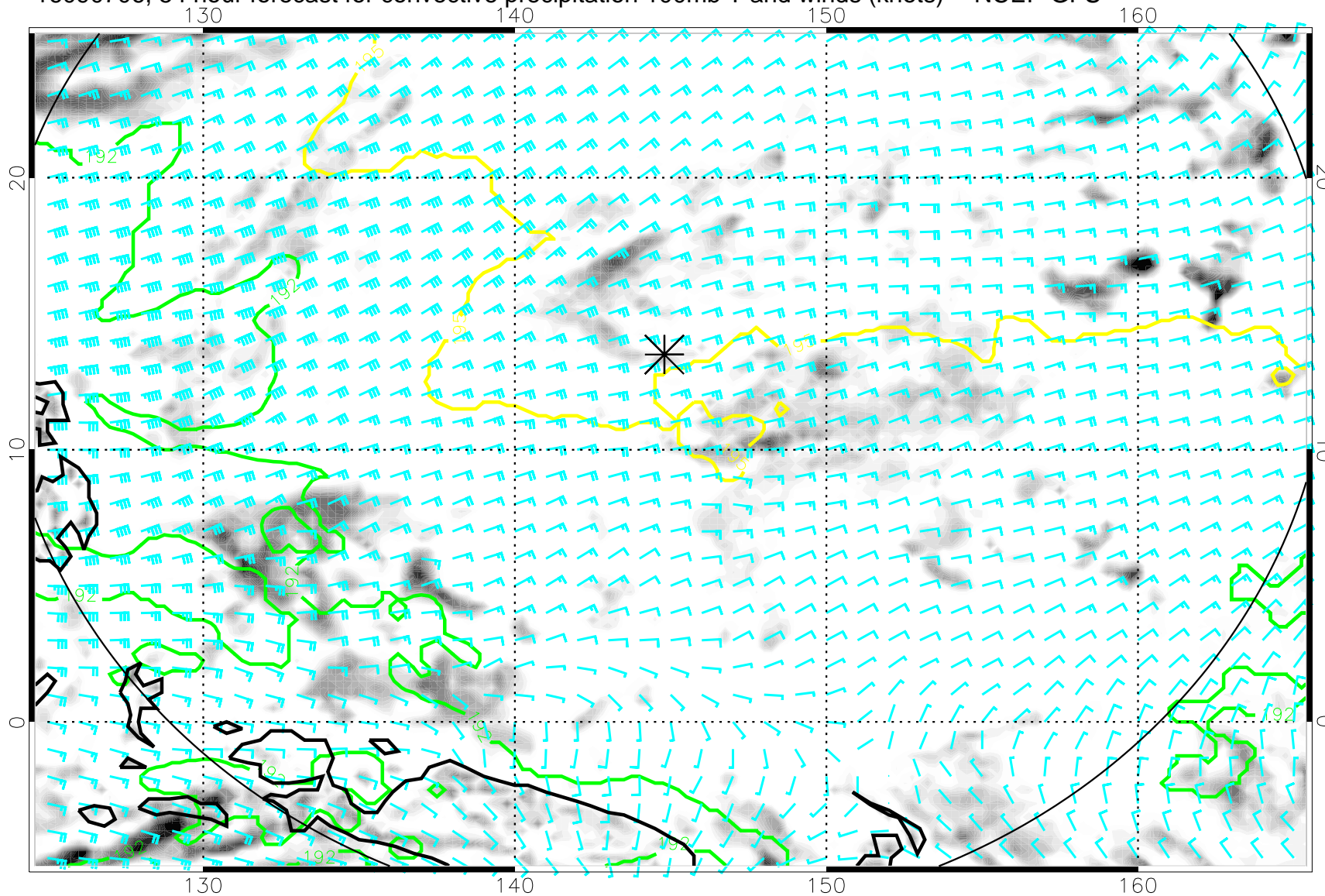
16090706, 54 hour forecast for convective precipitation 100mb T and winds (knots) -- NCEP GFS
