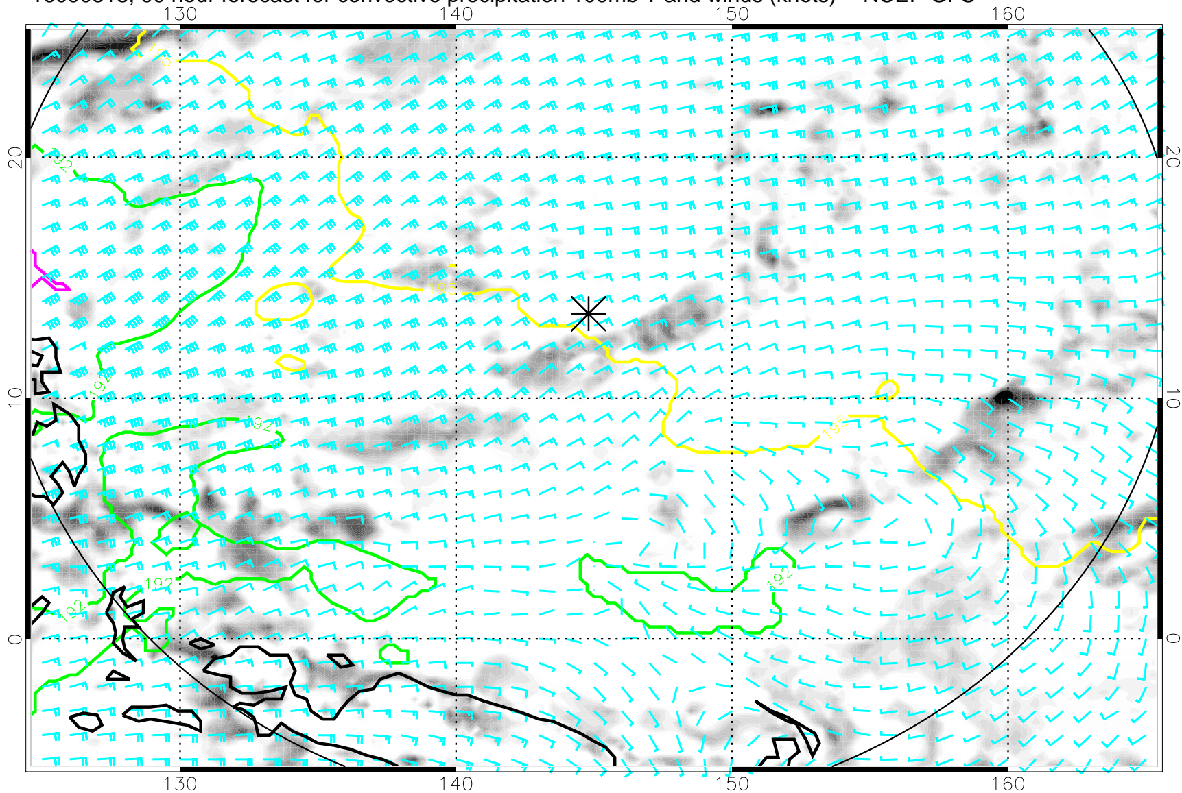
16090818, 90 hour forecast for convective precipitation 100mb T and winds (knots) -- NCEP GFS
