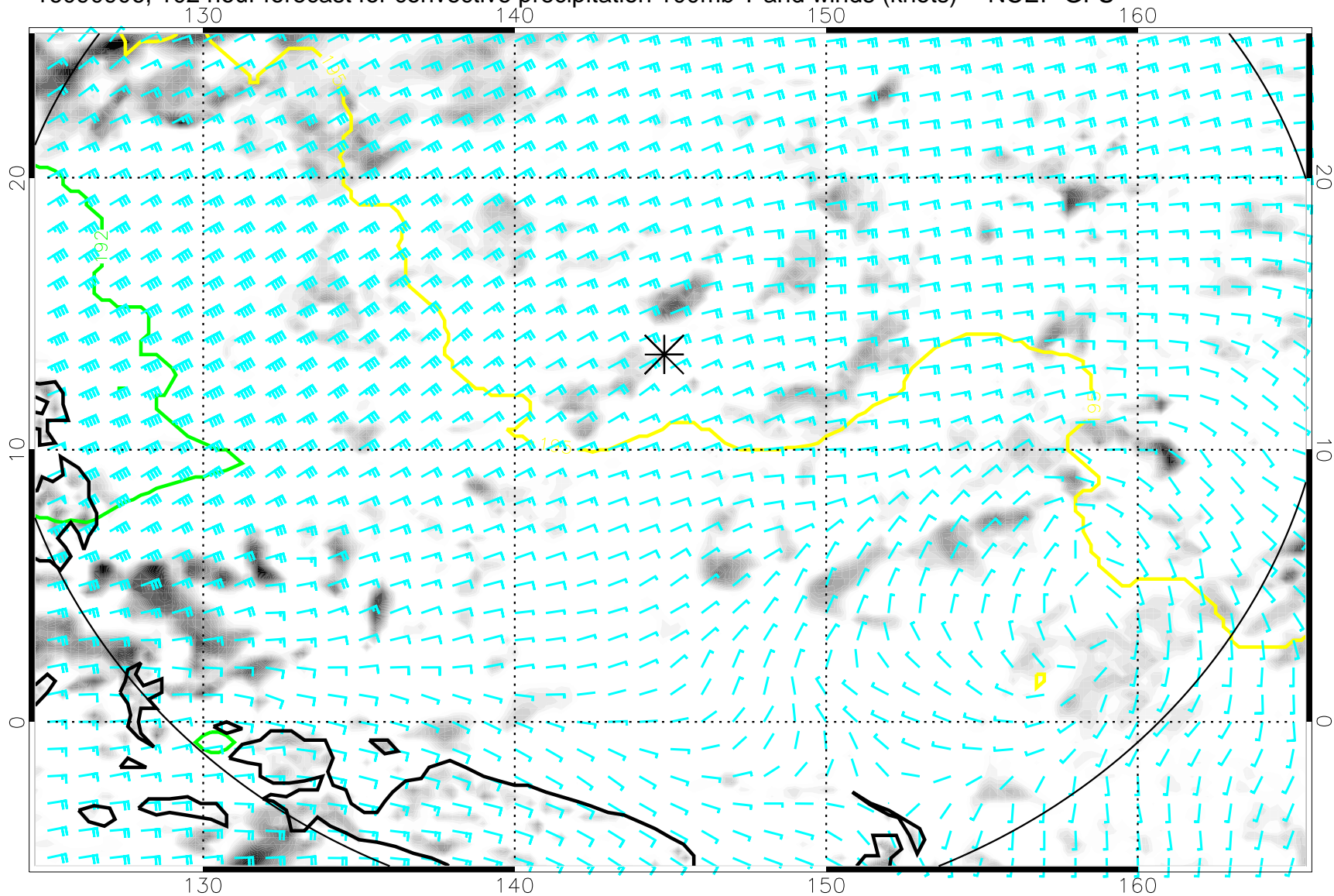
16090906, 102 hour forecast for convective precipitation 100mb T and winds (knots) -- NCEP GFS
