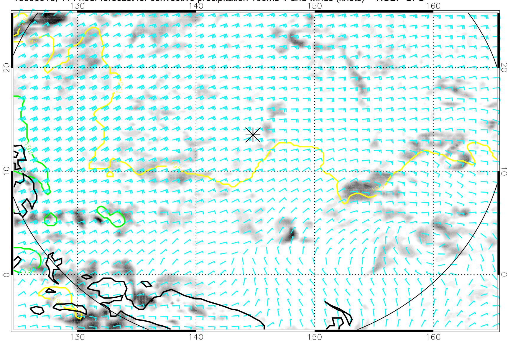
16090918, 114 hour forecast for convective precipitation 100mb T and winds (knots) -- NCEP GFS
