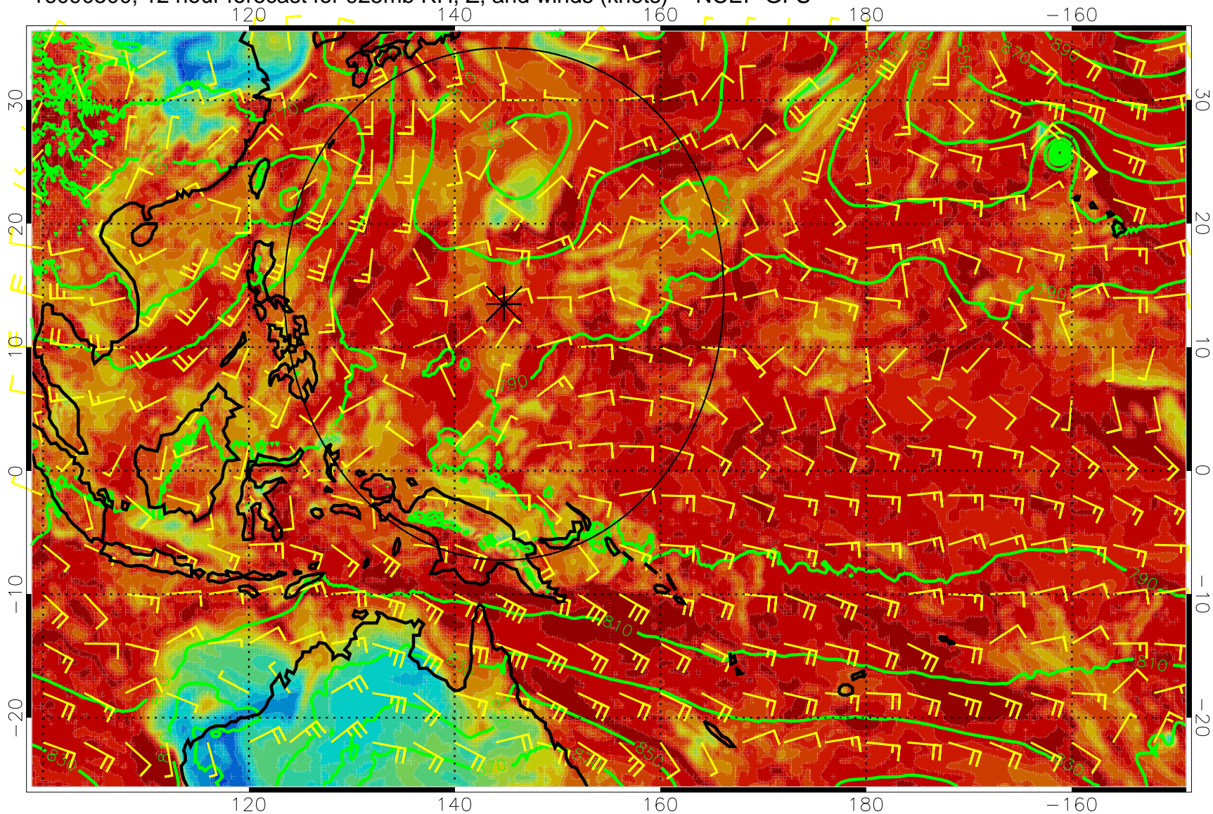
16090500, 12 hour forecast for 925mb RH, Z, and winds (knots) -- NCEP GFS
