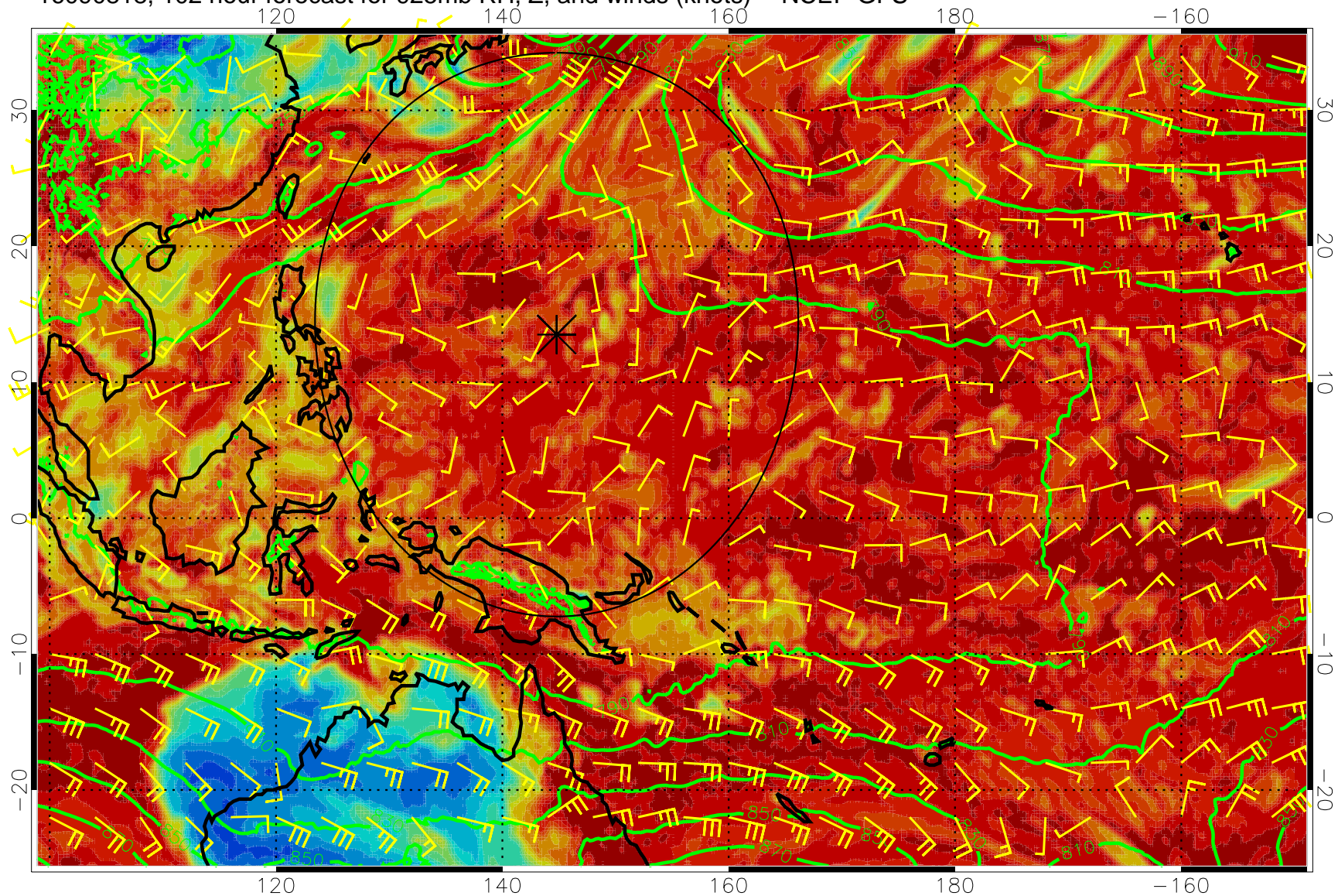
16090818, 102 hour forecast for 925mb RH, Z, and winds (knots) -- NCEP GFS
