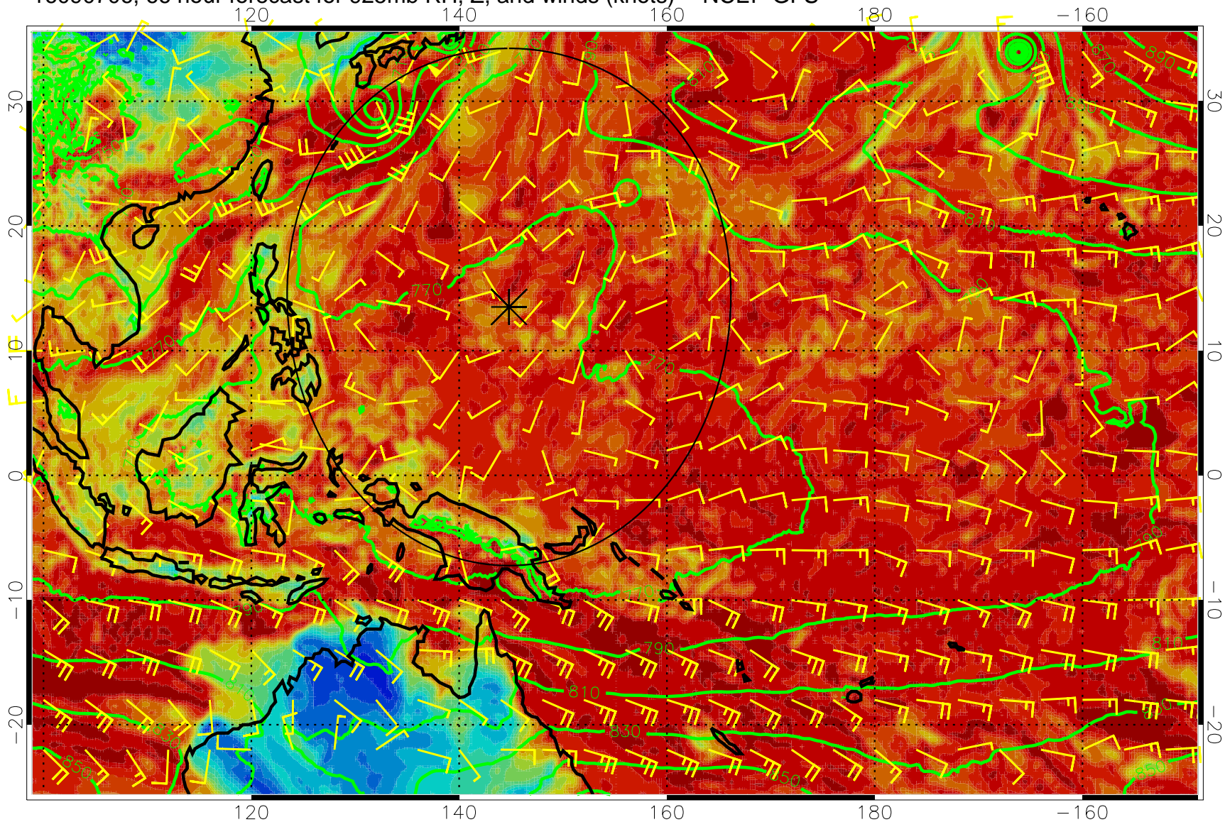
16090706, 66 hour forecast for 925mb RH, Z, and winds (knots) -- NCEP GFS
