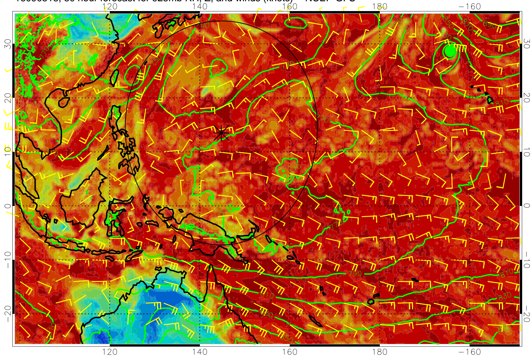
16090518, 30 hour forecast for 925mb RH, Z, and winds (knots) -- NCEP GFS
