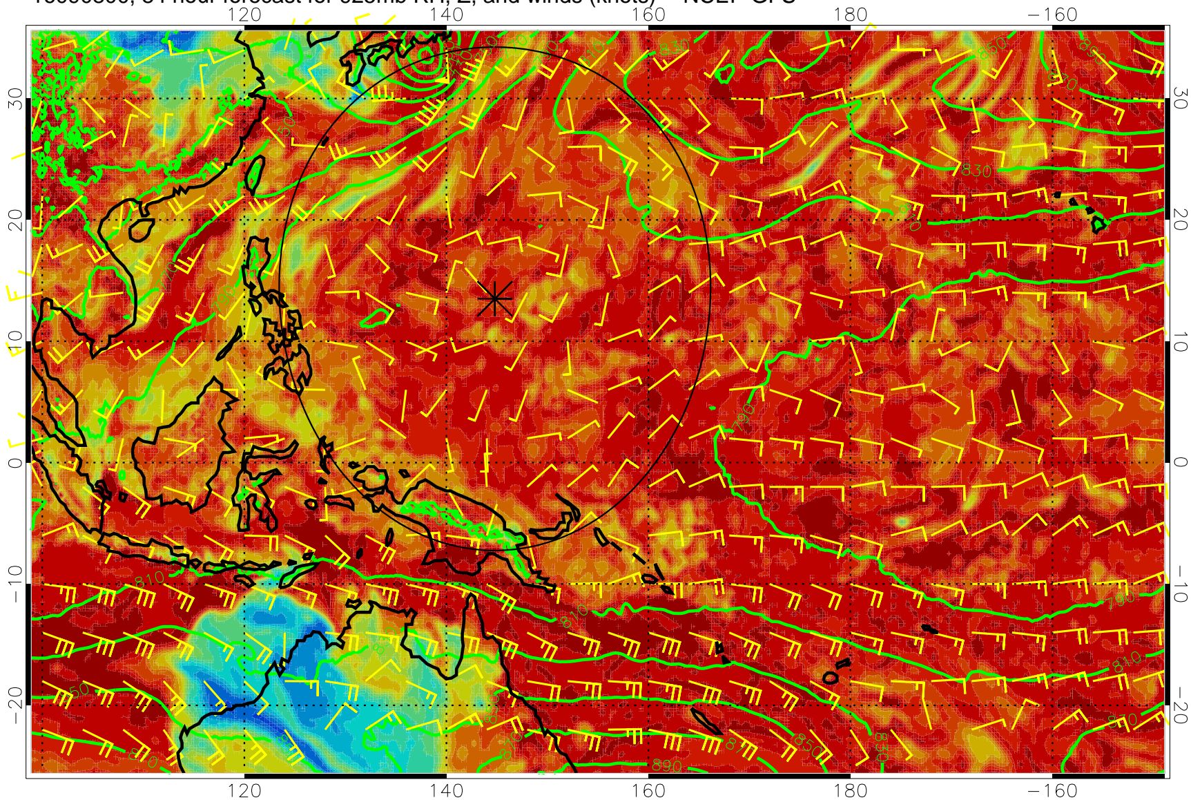
16090800, 84 hour forecast for 925mb RH, Z, and winds (knots) -- NCEP GFS
