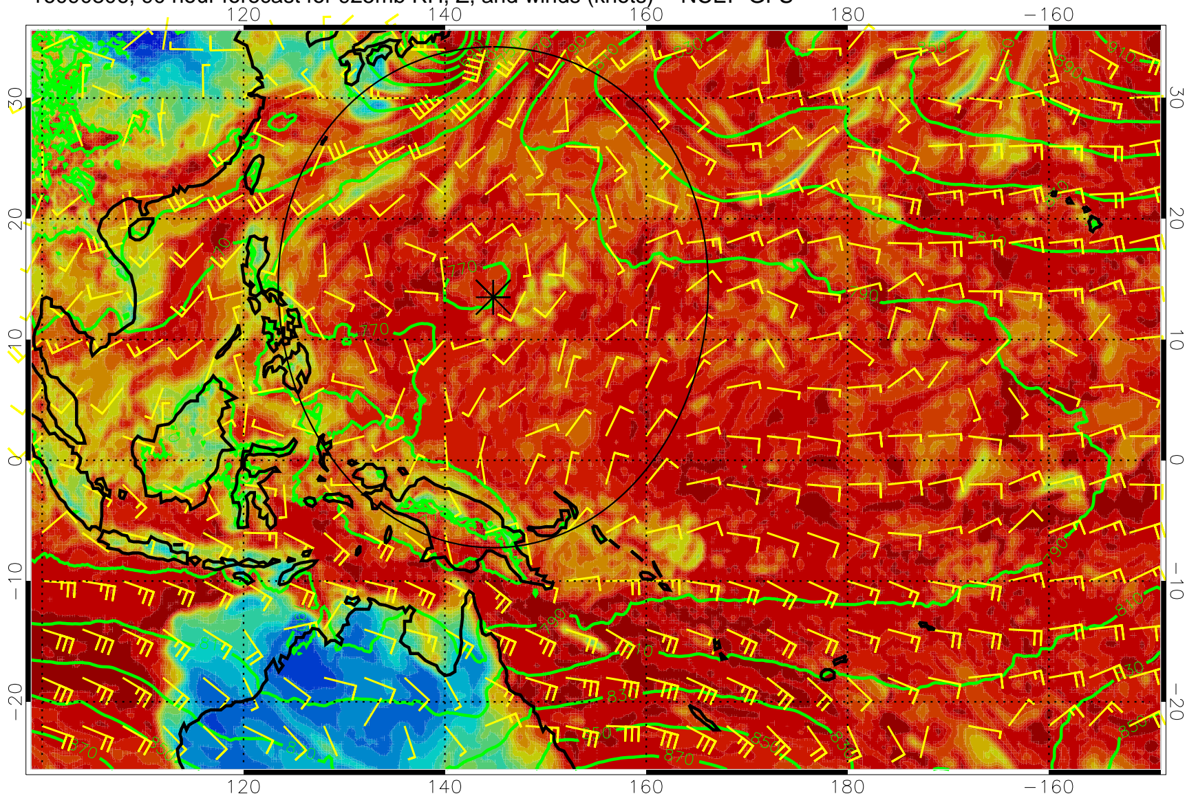
16090806, 90 hour forecast for 925mb RH, Z, and winds (knots) -- NCEP GFS
