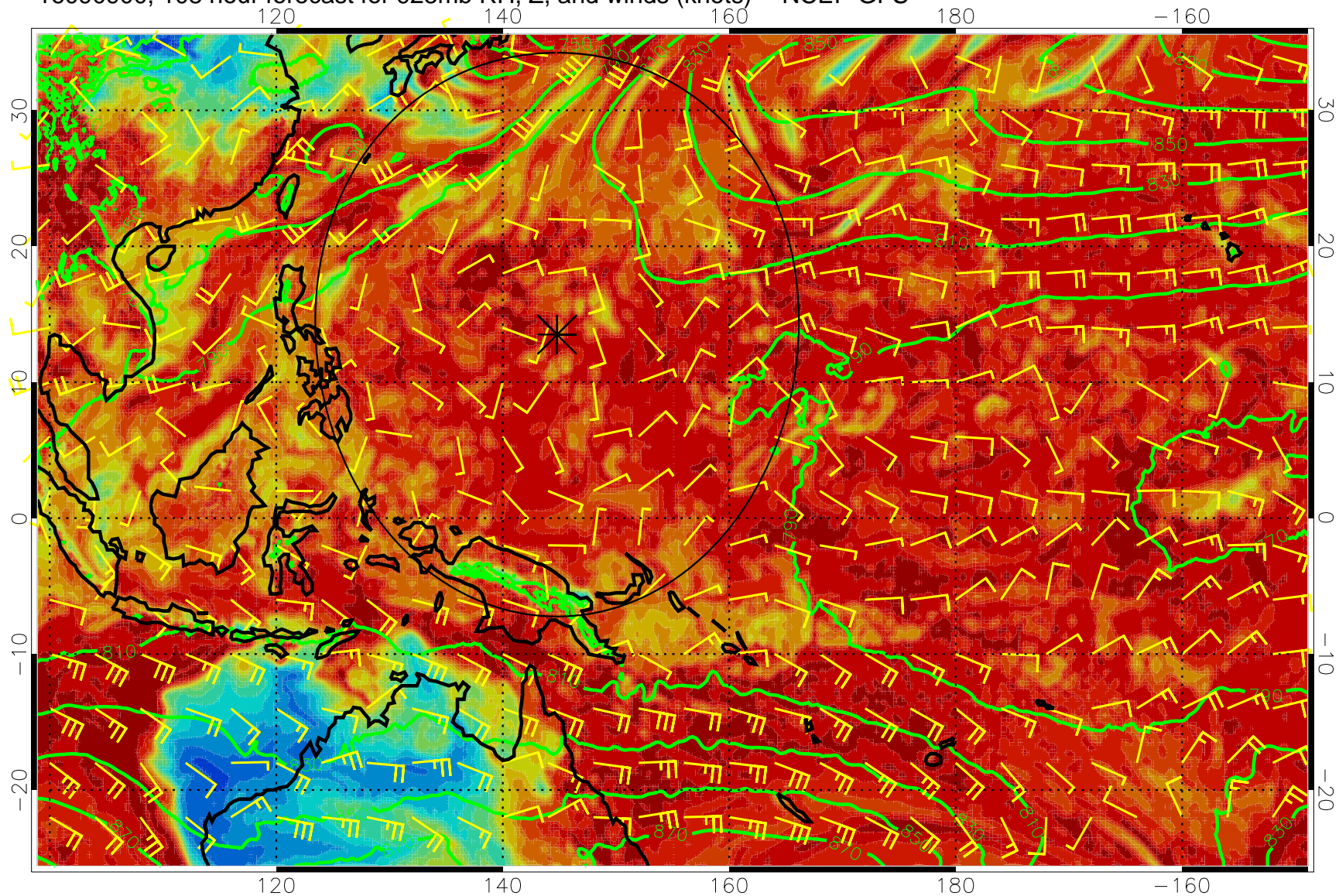
16090900, 108 hour forecast for 925mb RH, Z, and winds (knots) -- NCEP GFS
