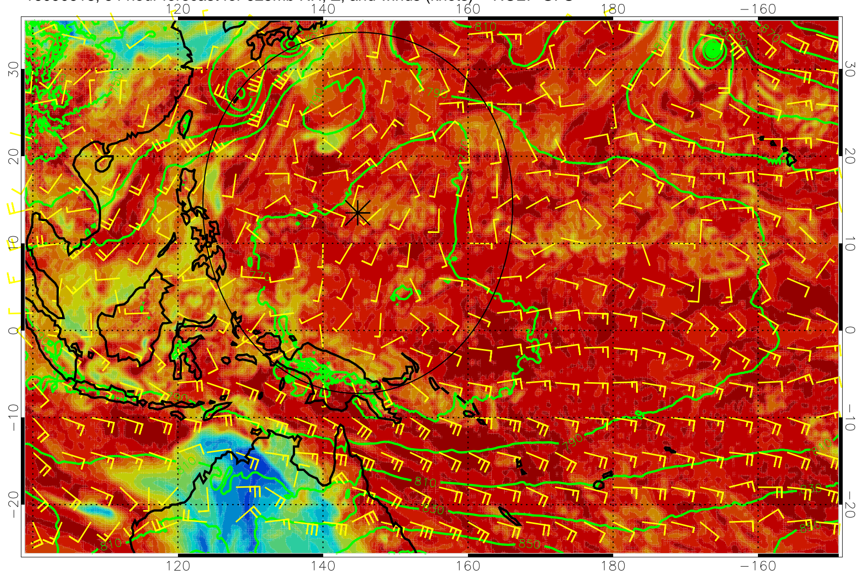
16090618, 54 hour forecast for 925mb RH, Z, and winds (knots) -- NCEP GFS
