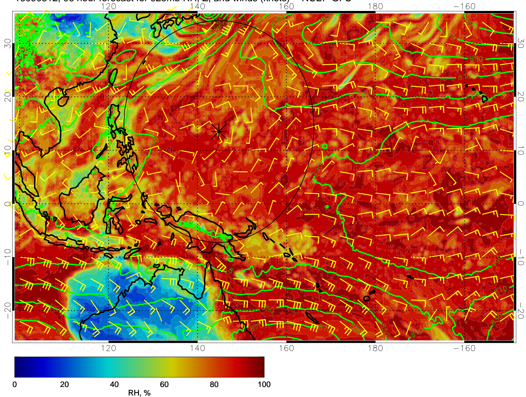
16090812, 96 hour forecast for 925mb RH, Z, and winds (knots) -- NCEP GFS
