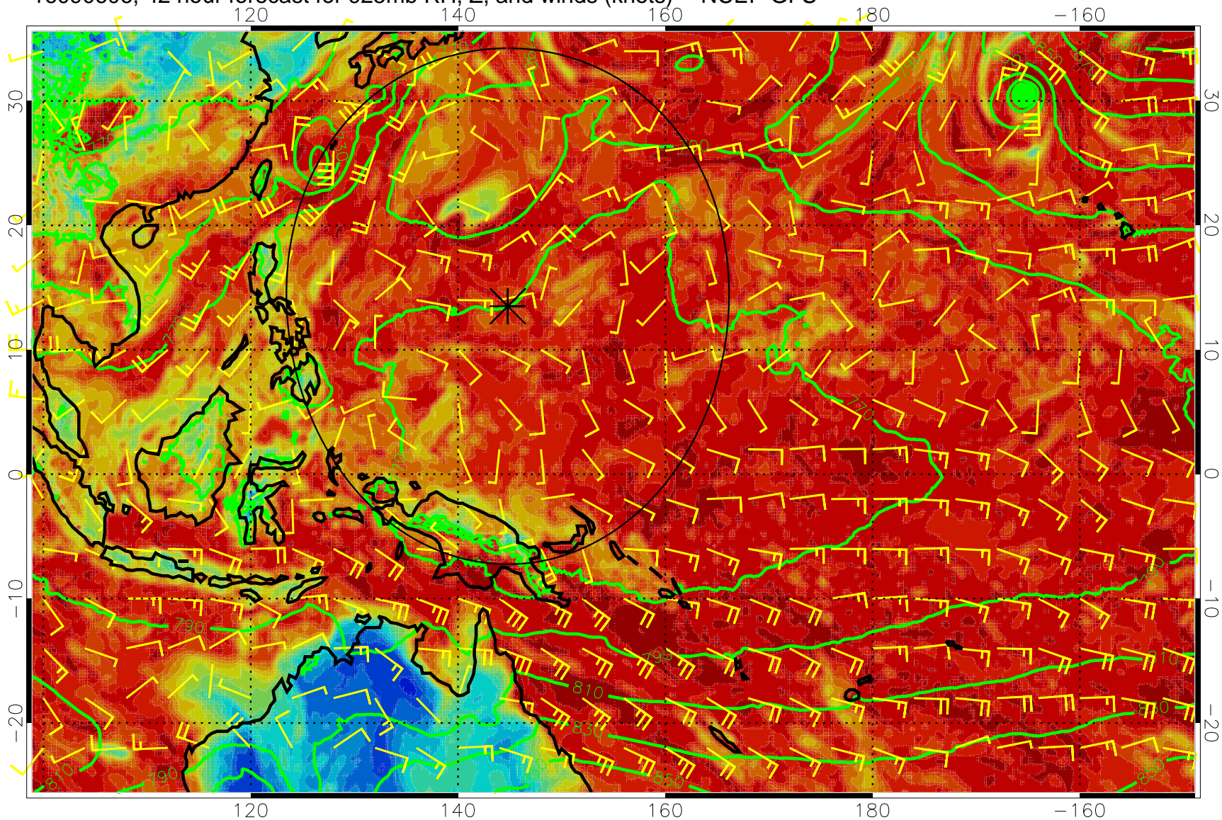
16090606, 42 hour forecast for 925mb RH, Z, and winds (knots) -- NCEP GFS
