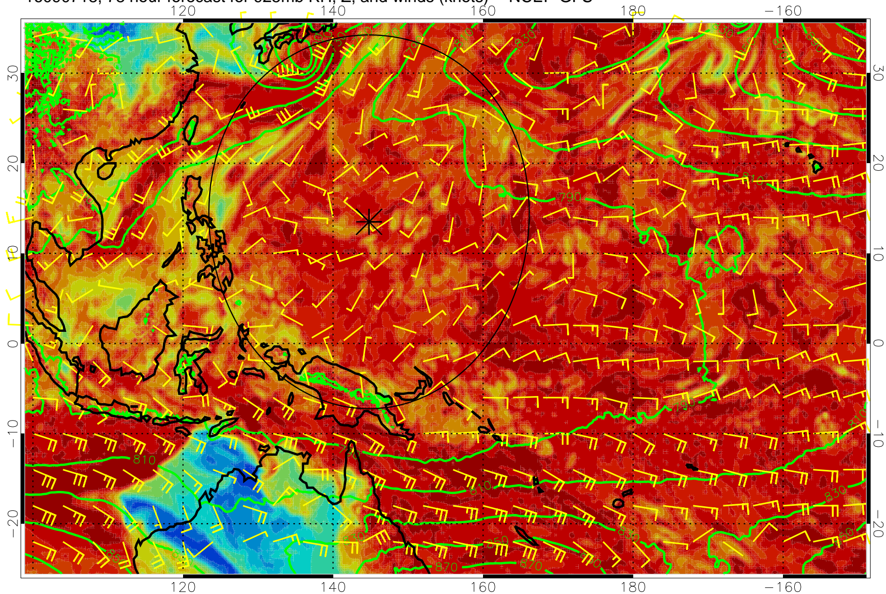
16090718, 78 hour forecast for 925mb RH, Z, and winds (knots) -- NCEP GFS
