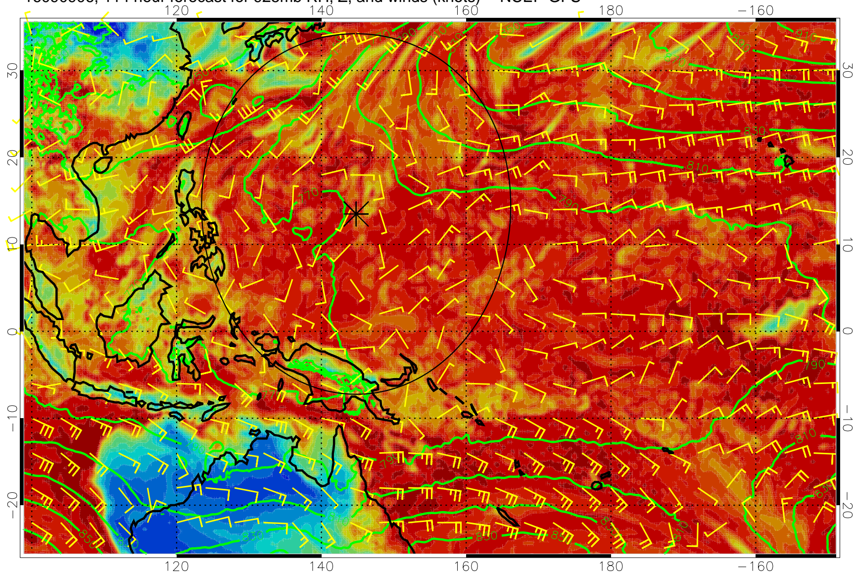
16090906, 114 hour forecast for 925mb RH, Z, and winds (knots) -- NCEP GFS
