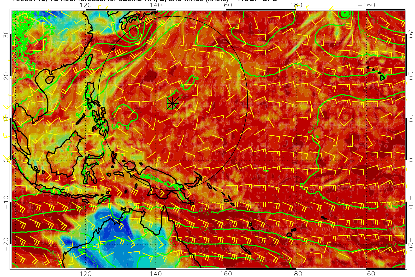
16090712, 72 hour forecast for 925mb RH, Z, and winds (knots) -- NCEP GFS
