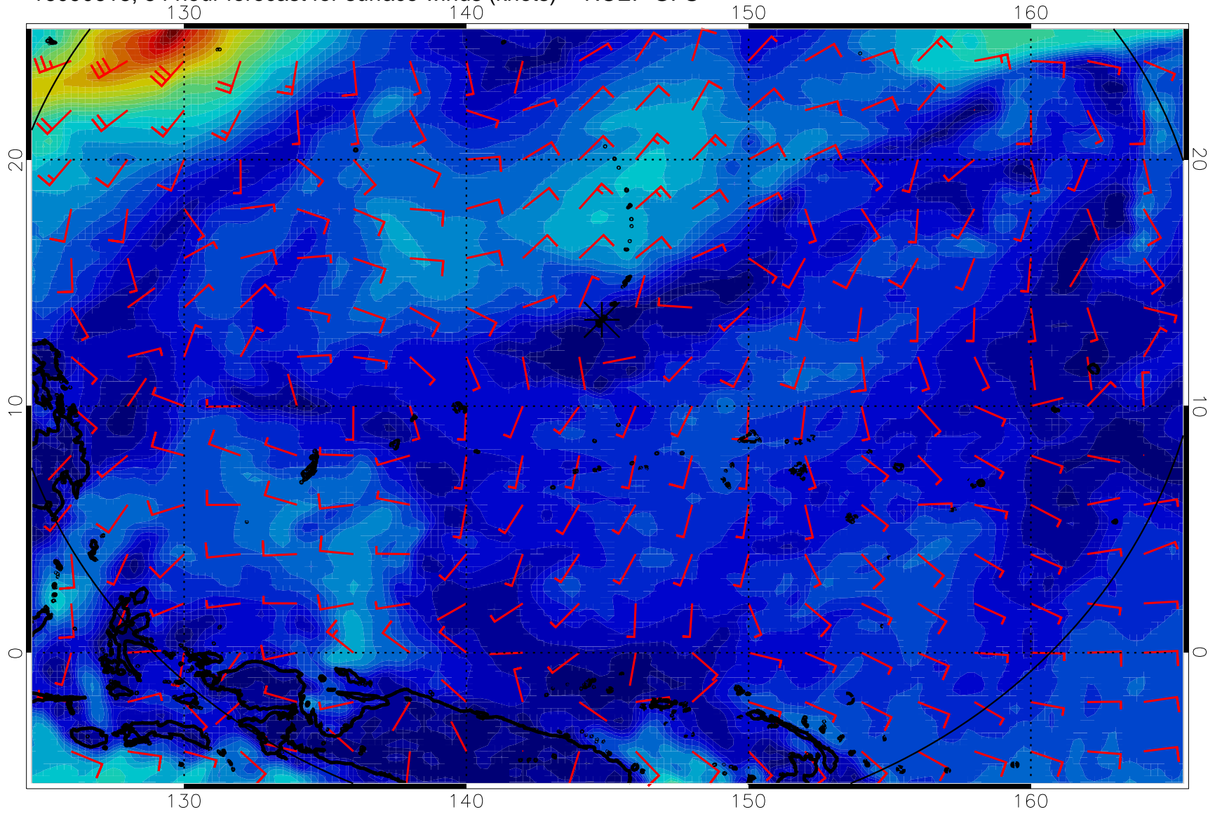
16090618, 54 hour forecast for surface winds (knots) -- NCEP GFS
