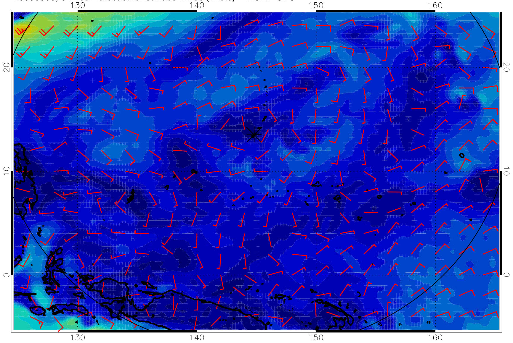
16090800, 84 hour forecast for surface winds (knots) -- NCEP GFS
