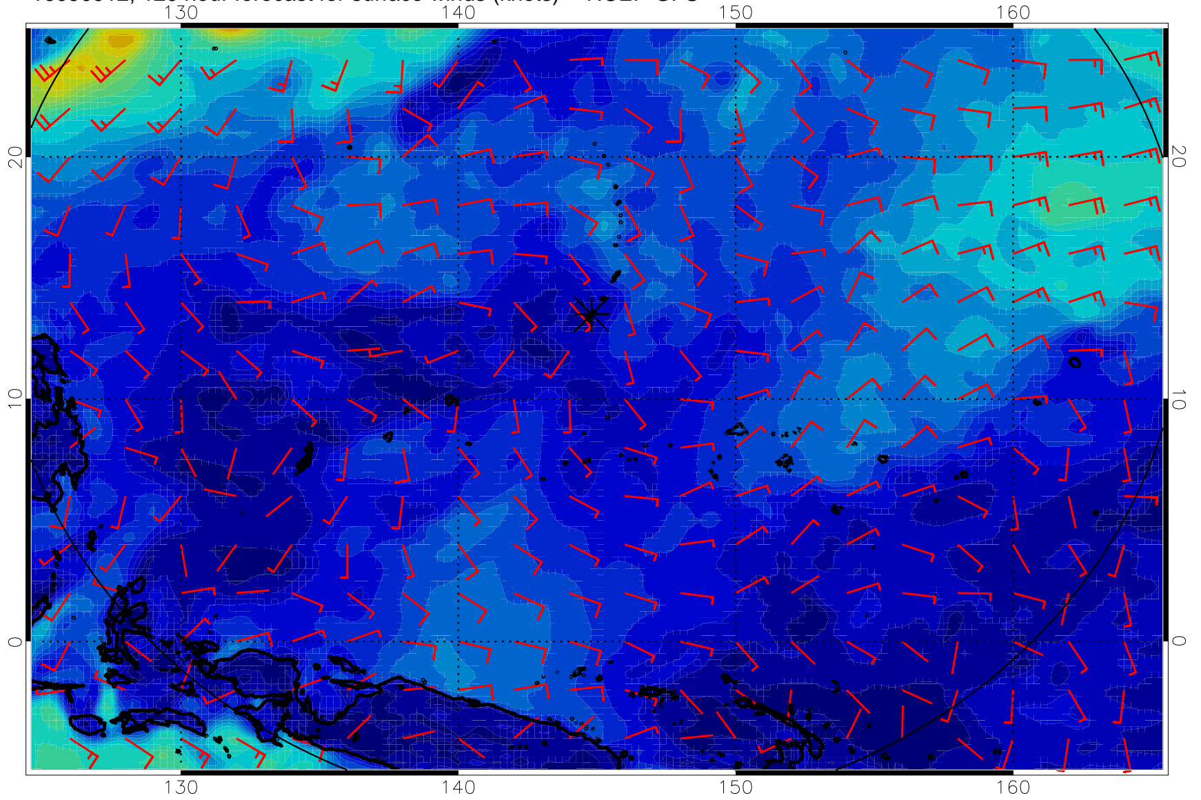
16090912, 120 hour forecast for surface winds (knots) -- NCEP GFS
