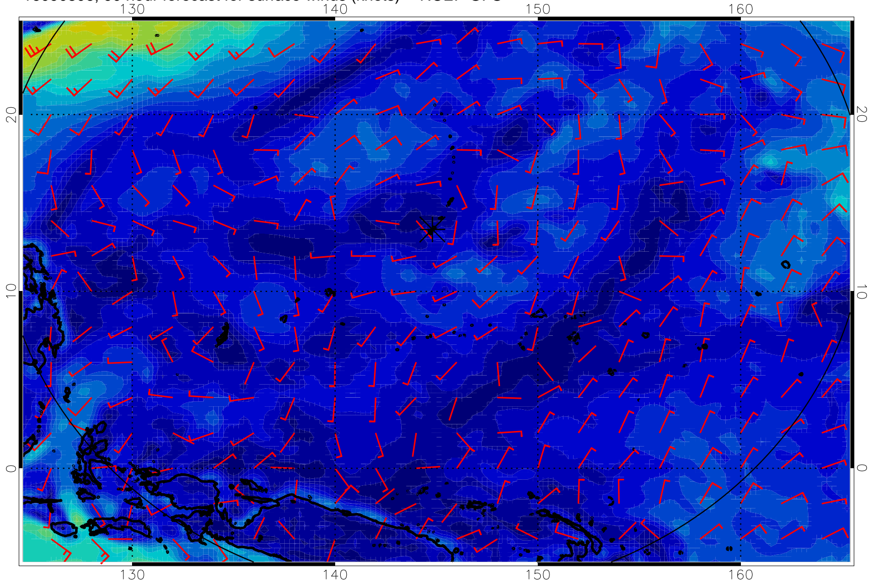
16090806, 90 hour forecast for surface winds (knots) -- NCEP GFS
