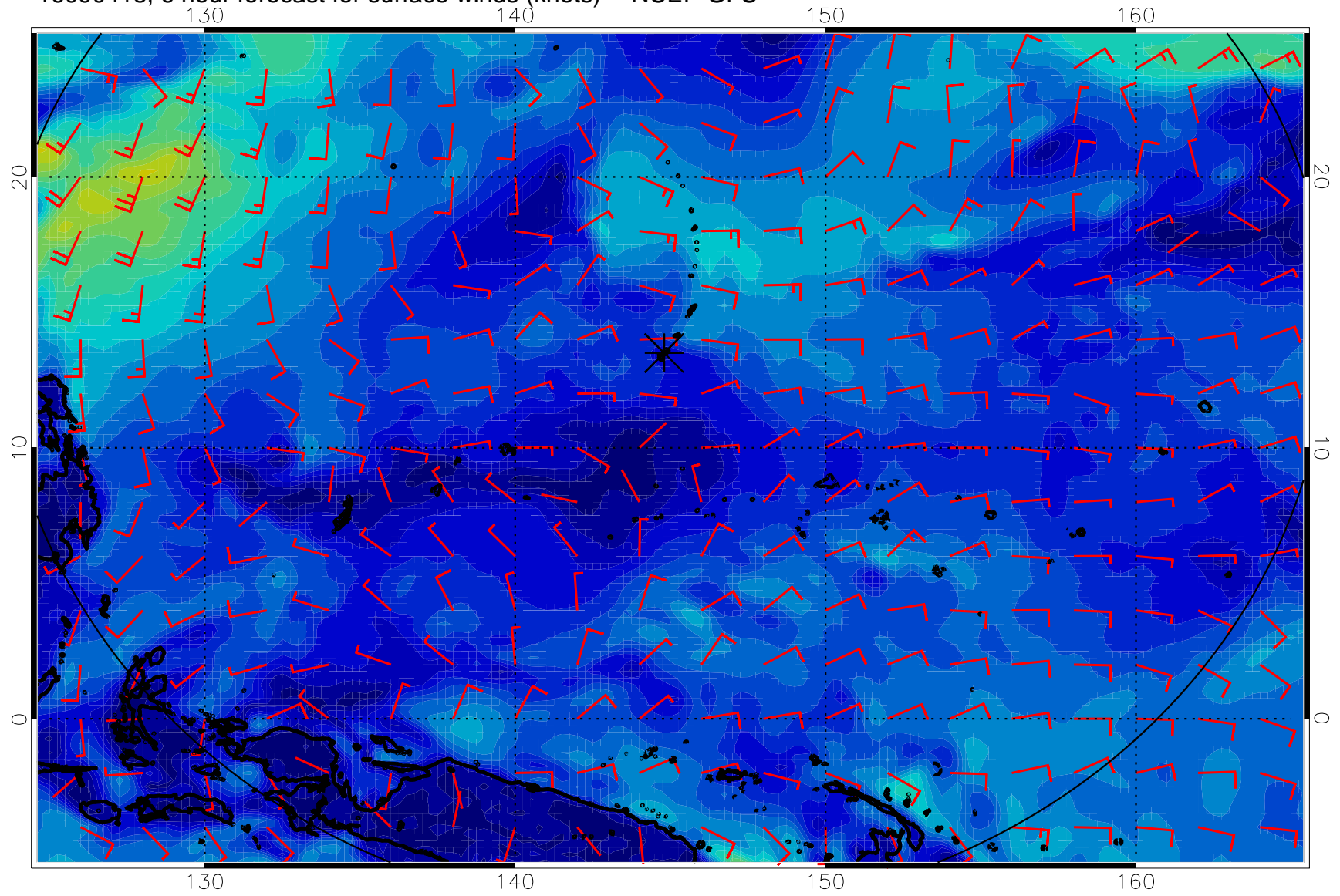
16090418, 6 hour forecast for surface winds (knots) -- NCEP GFS
