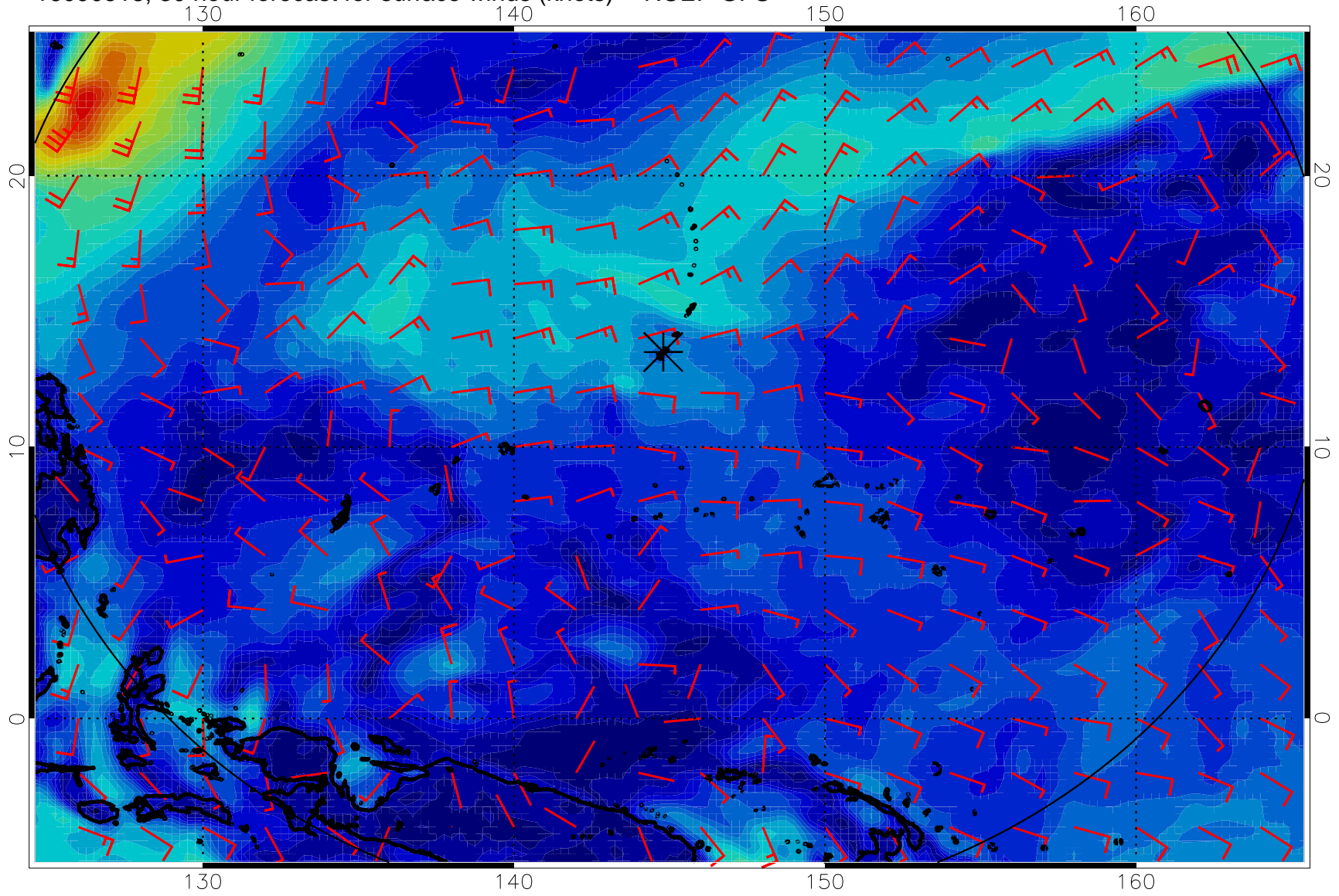
16090518, 30 hour forecast for surface winds (knots) -- NCEP GFS
