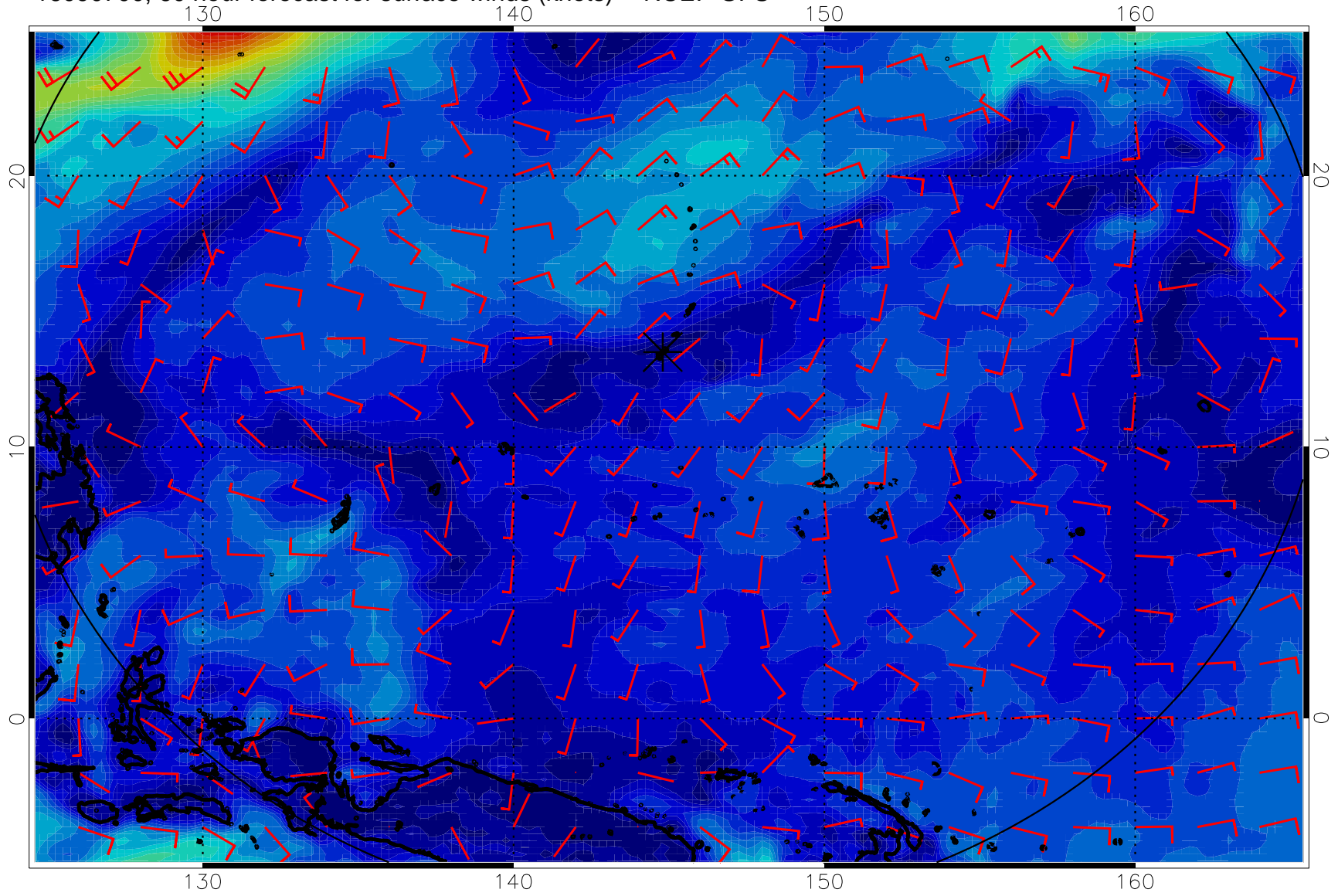
16090700, 60 hour forecast for surface winds (knots) -- NCEP GFS
