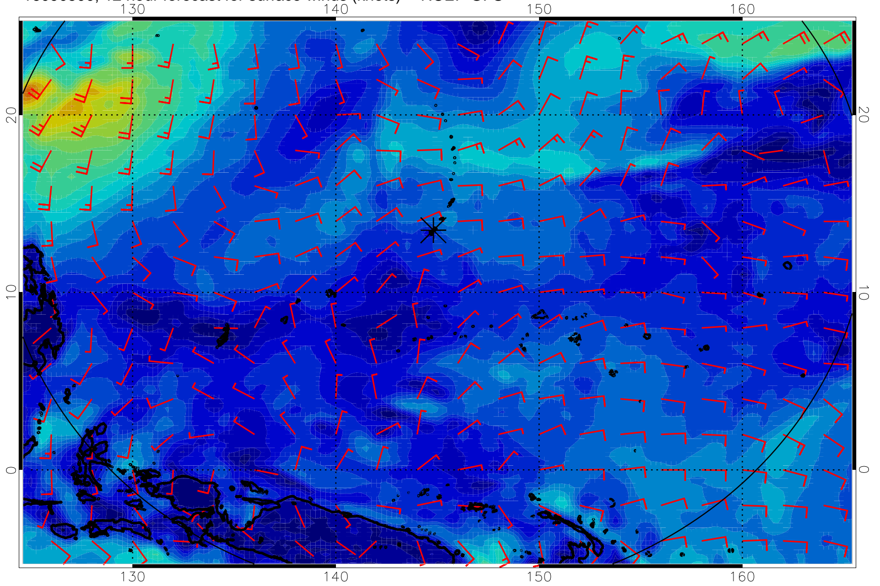
16090500, 12 hour forecast for surface winds (knots) -- NCEP GFS
