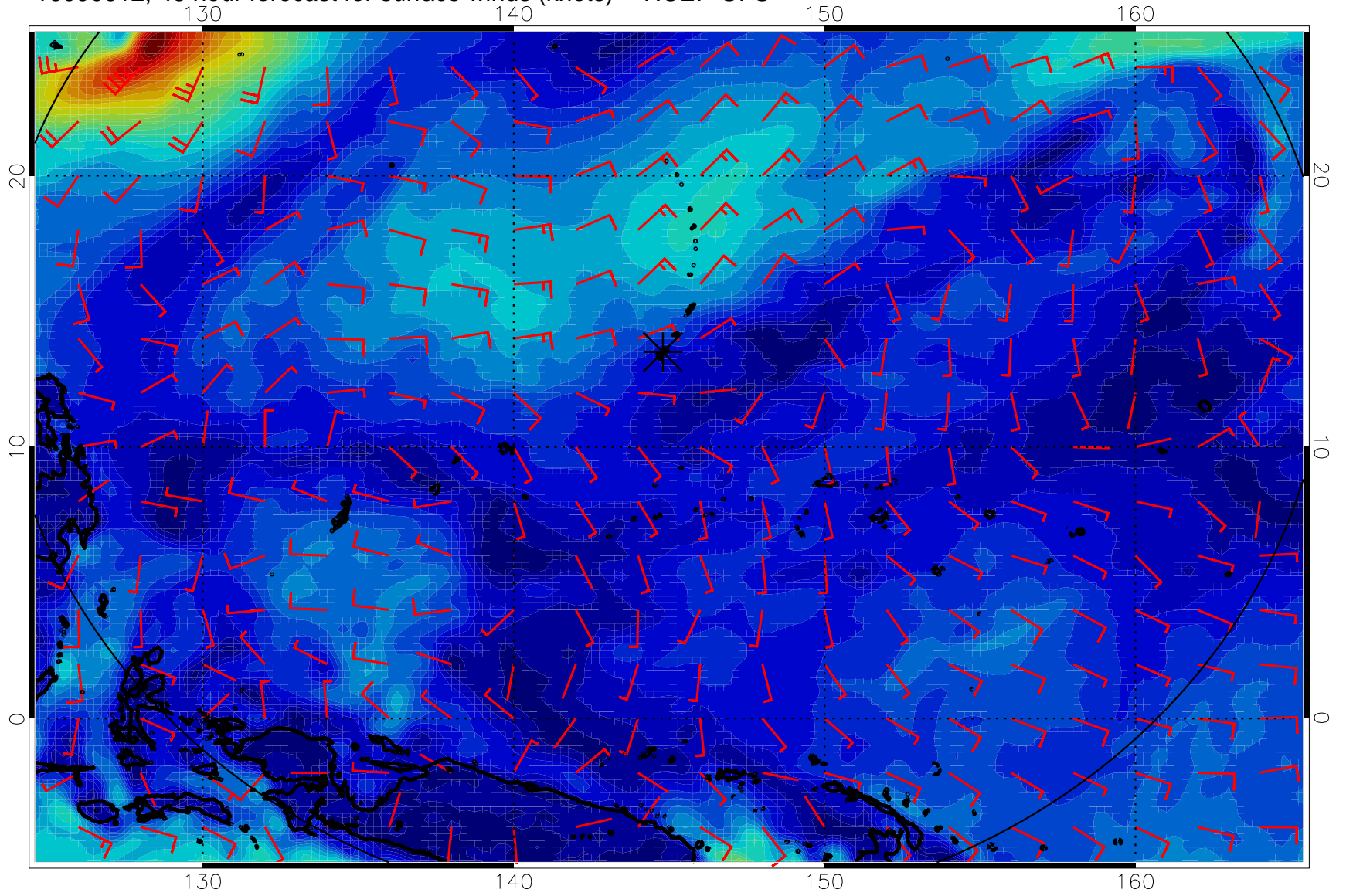
16090612, 48 hour forecast for surface winds (knots) -- NCEP GFS
