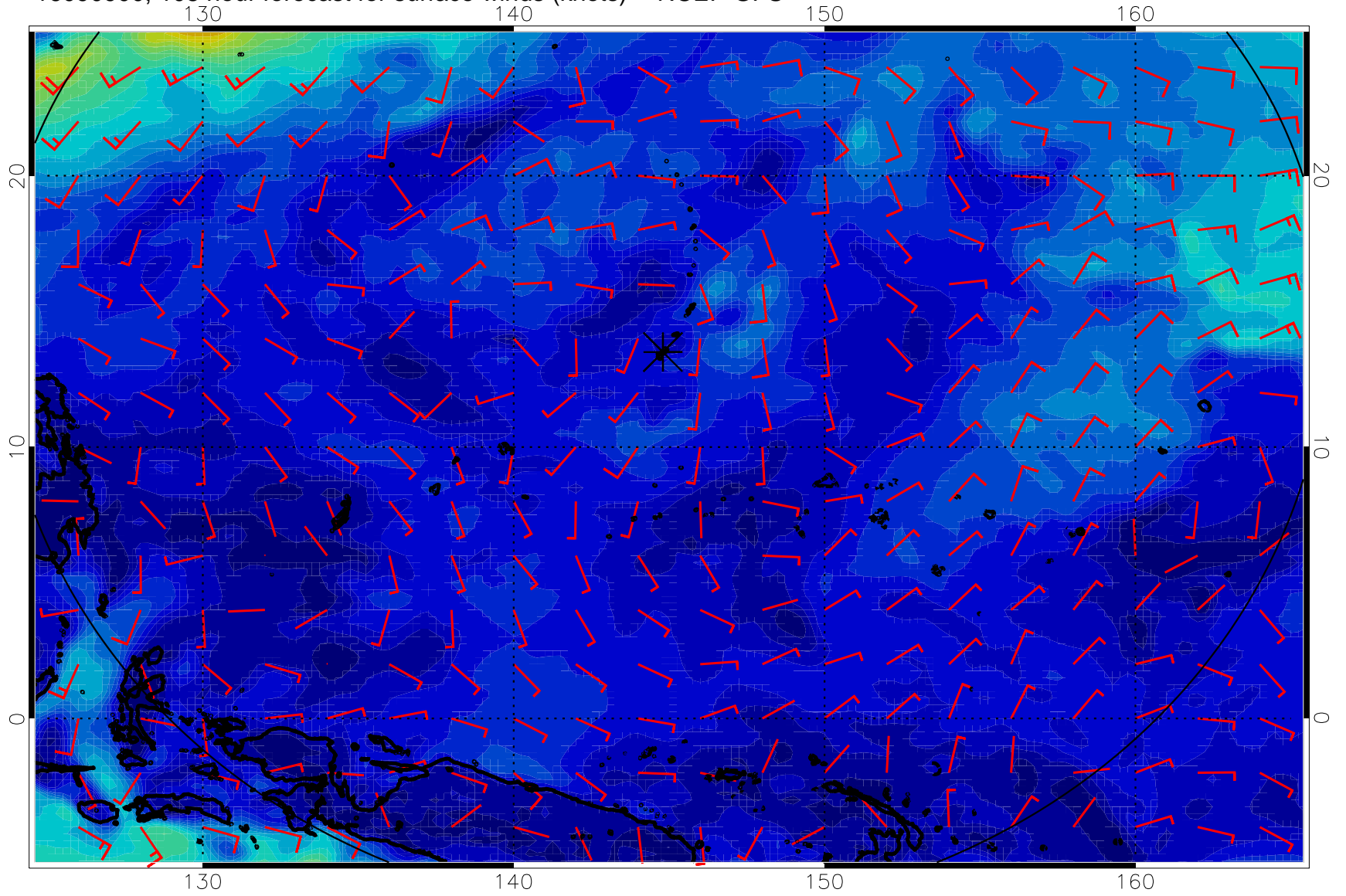
16090900, 108 hour forecast for surface winds (knots) -- NCEP GFS
