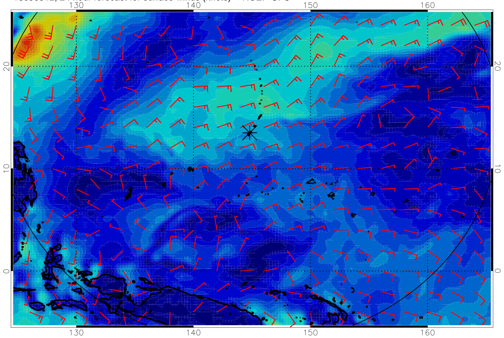
16090512, 24 hour forecast for surface winds (knots) -- NCEP GFS
