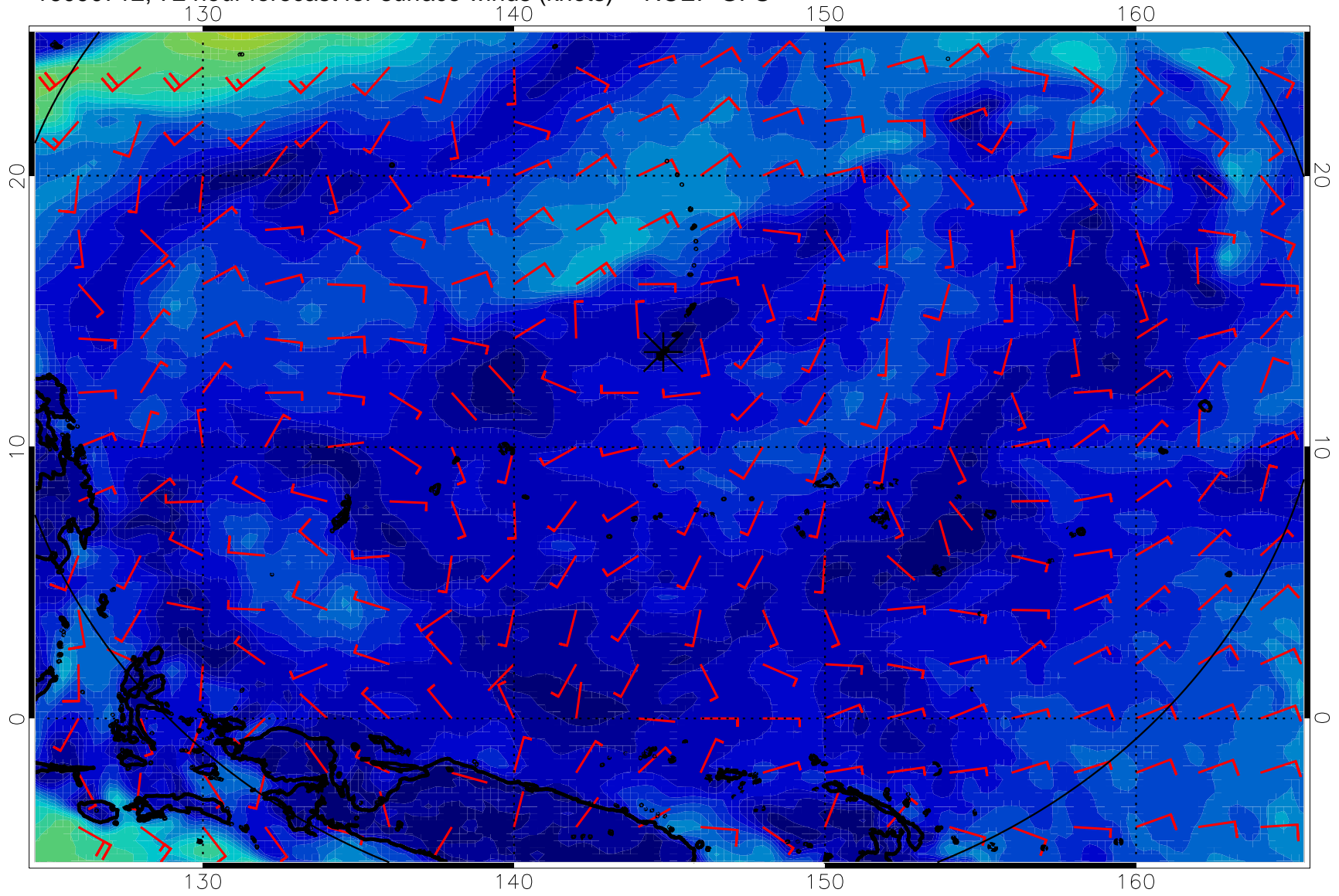
16090712, 72 hour forecast for surface winds (knots) -- NCEP GFS
