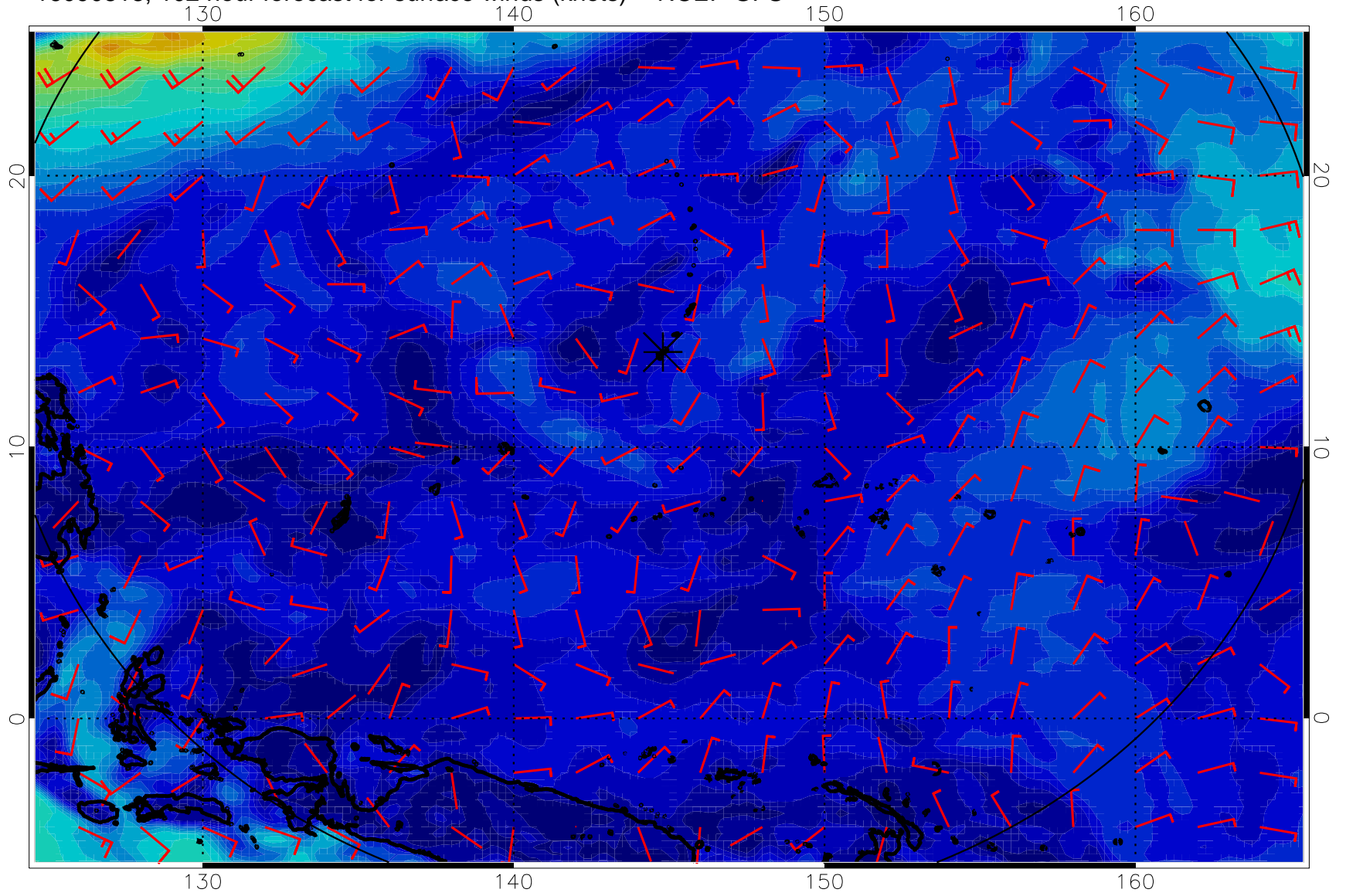
16090818, 102 hour forecast for surface winds (knots) -- NCEP GFS
