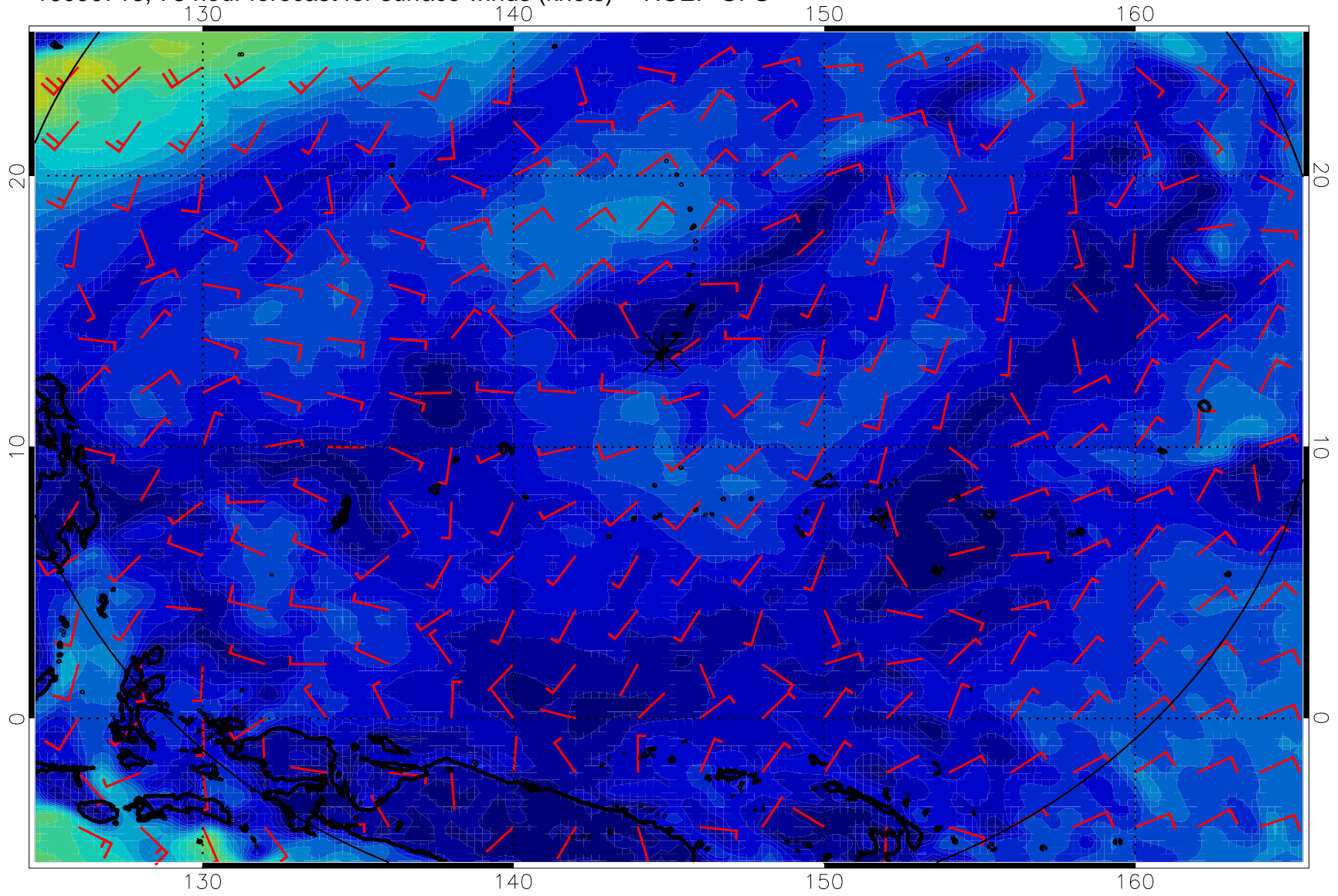
16090718, 78 hour forecast for surface winds (knots) -- NCEP GFS
