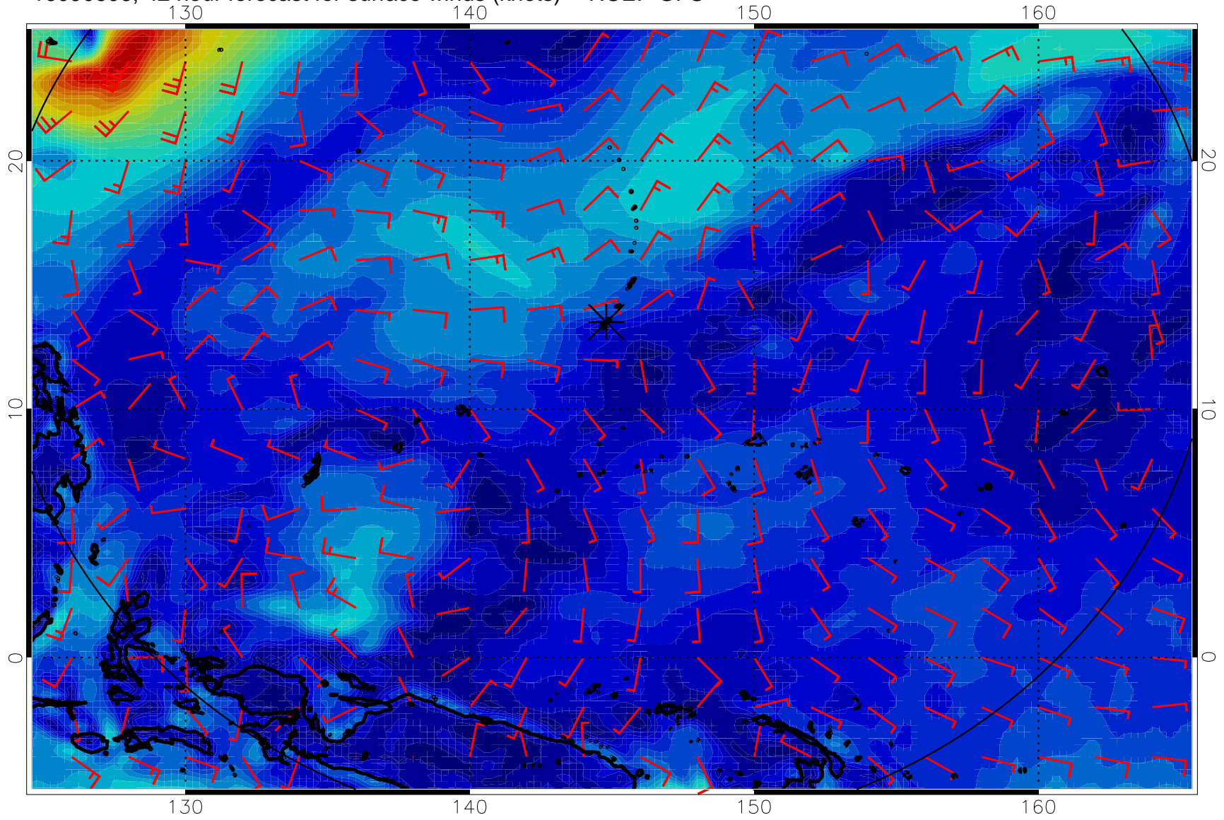
16090606, 42 hour forecast for surface winds (knots) -- NCEP GFS
