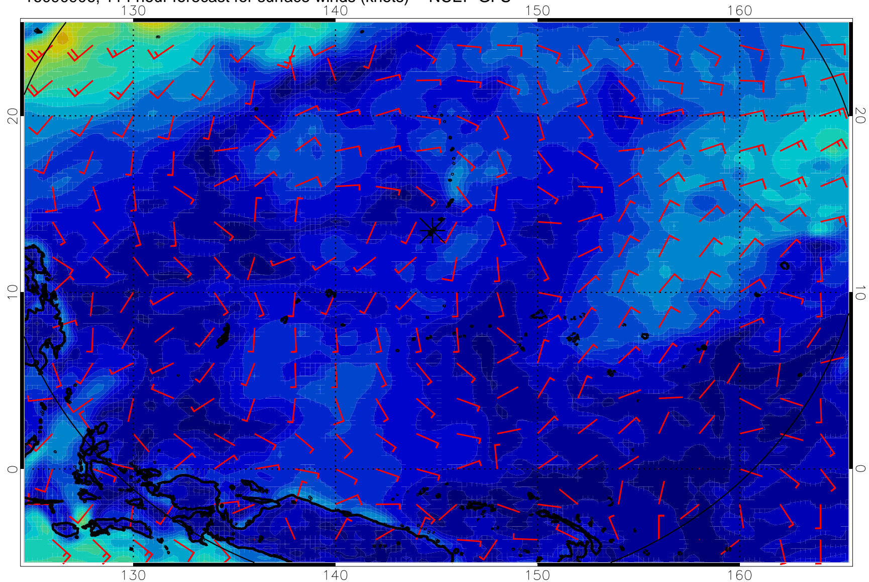
16090906, 114 hour forecast for surface winds (knots) -- NCEP GFS
