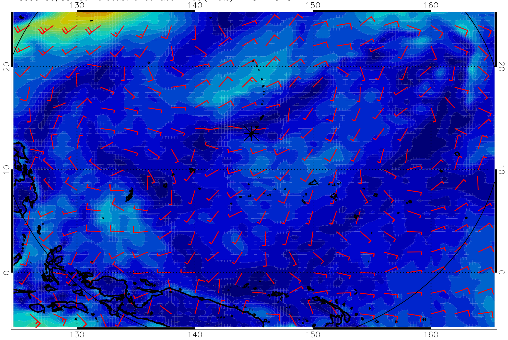
16090706, 66 hour forecast for surface winds (knots) -- NCEP GFS
