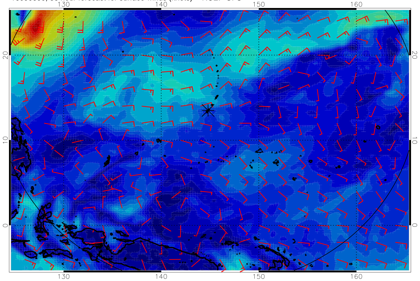
16090600, 36 hour forecast for surface winds (knots) -- NCEP GFS
