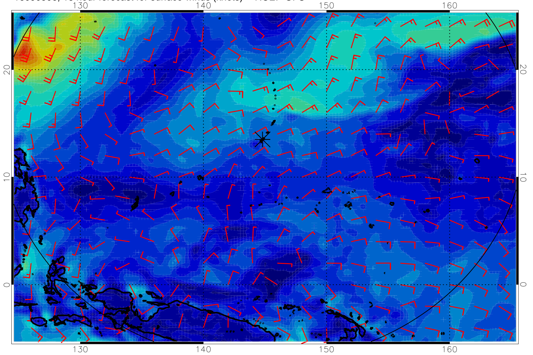
16090506, 18 hour forecast for surface winds (knots) -- NCEP GFS
