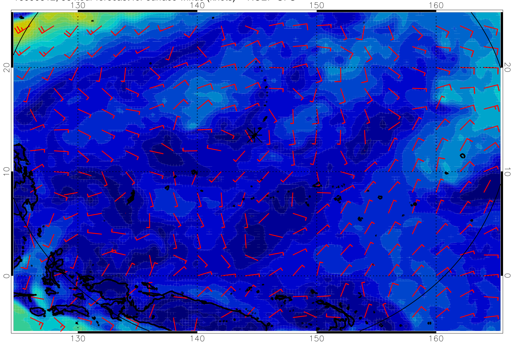
16090812, 96 hour forecast for surface winds (knots) -- NCEP GFS
