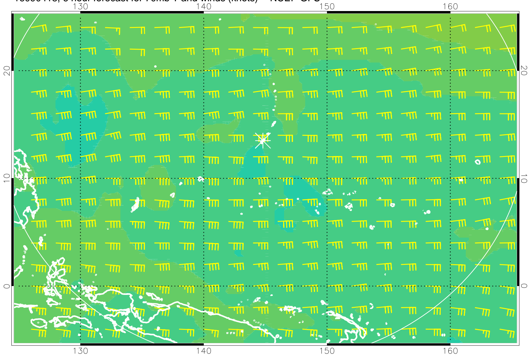
16090418, 6 hour forecast for 70mb T and winds (knots) -- NCEP GFS
