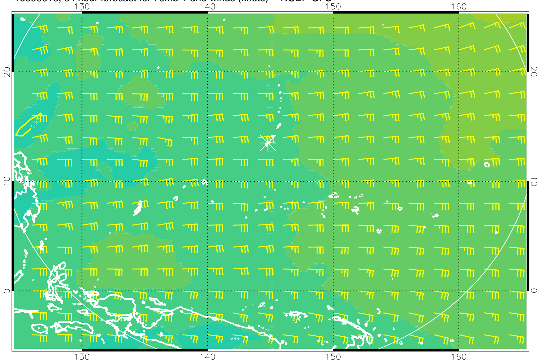
16090618, 54 hour forecast for 70mb T and winds (knots) -- NCEP GFS
