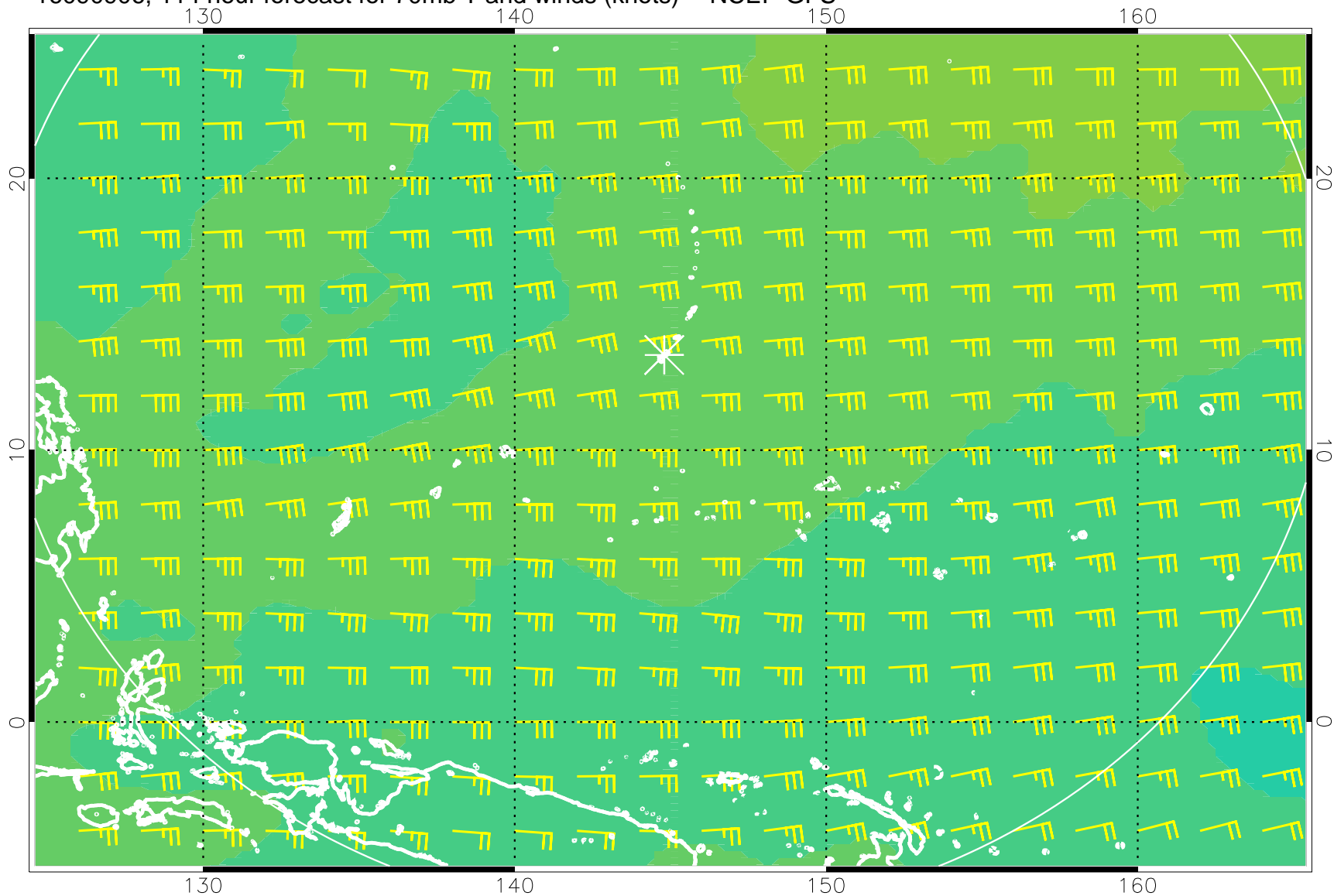
16090906, 114 hour forecast for 70mb T and winds (knots) -- NCEP GFS
