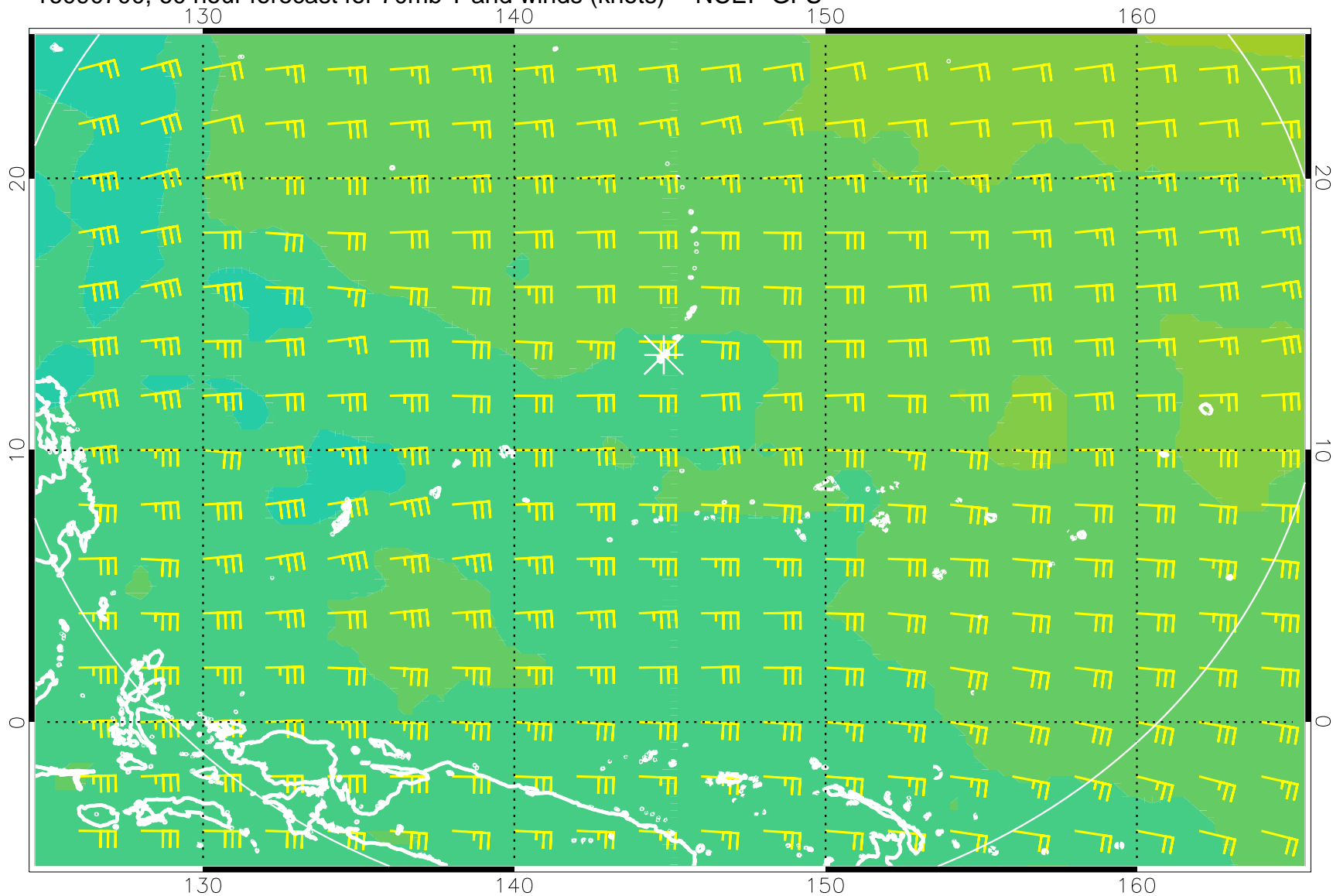
16090700, 60 hour forecast for 70mb T and winds (knots) -- NCEP GFS
