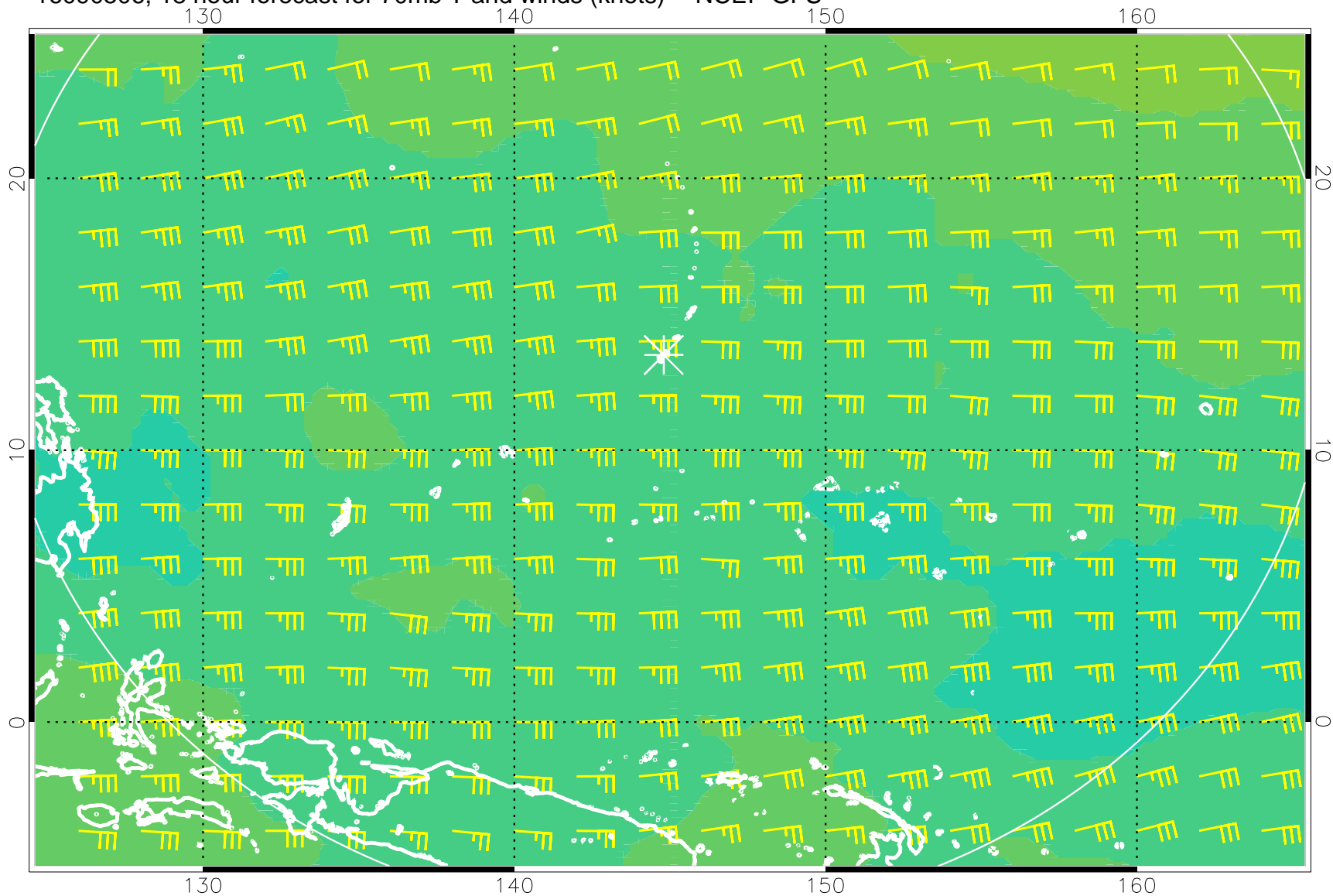
16090506, 18 hour forecast for 70mb T and winds (knots) -- NCEP GFS
