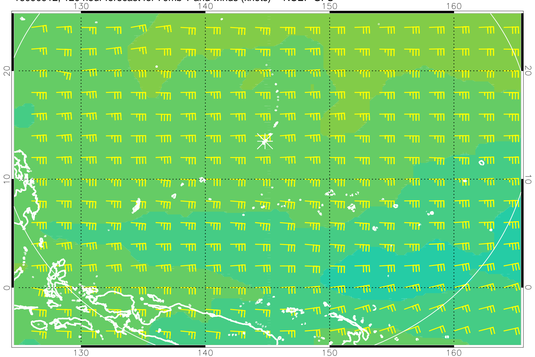
16090912, 120 hour forecast for 70mb T and winds (knots) -- NCEP GFS
