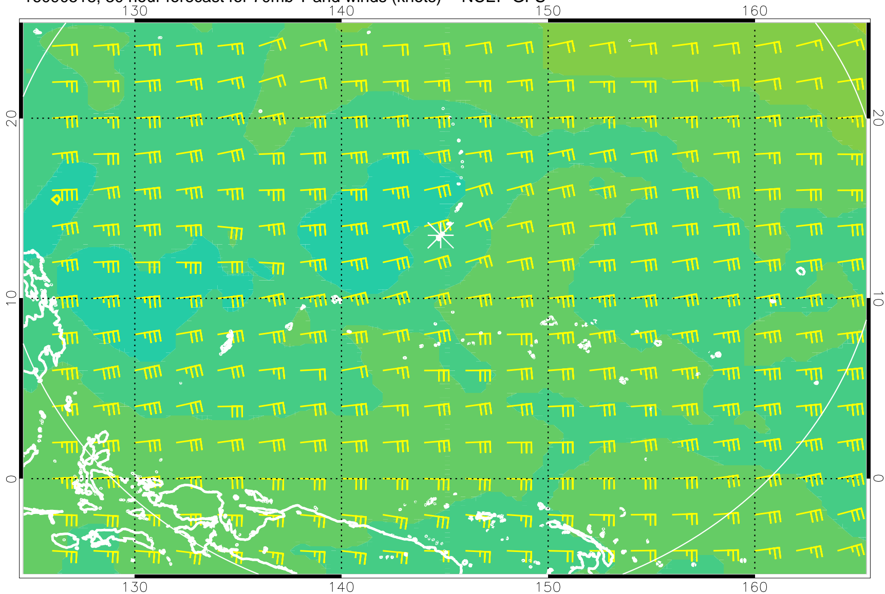
16090518, 30 hour forecast for 70mb T and winds (knots) -- NCEP GFS
