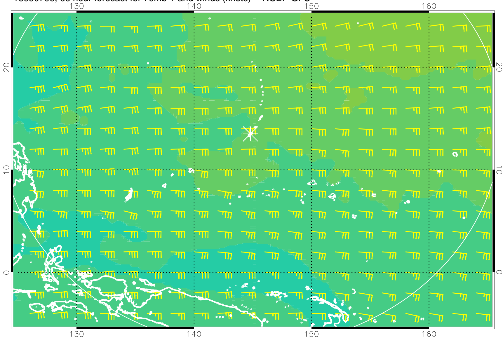
16090706, 66 hour forecast for 70mb T and winds (knots) -- NCEP GFS
