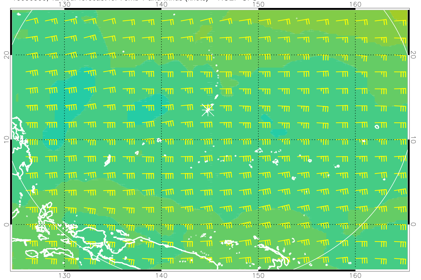
16090500, 12 hour forecast for 70mb T and winds (knots) -- NCEP GFS
