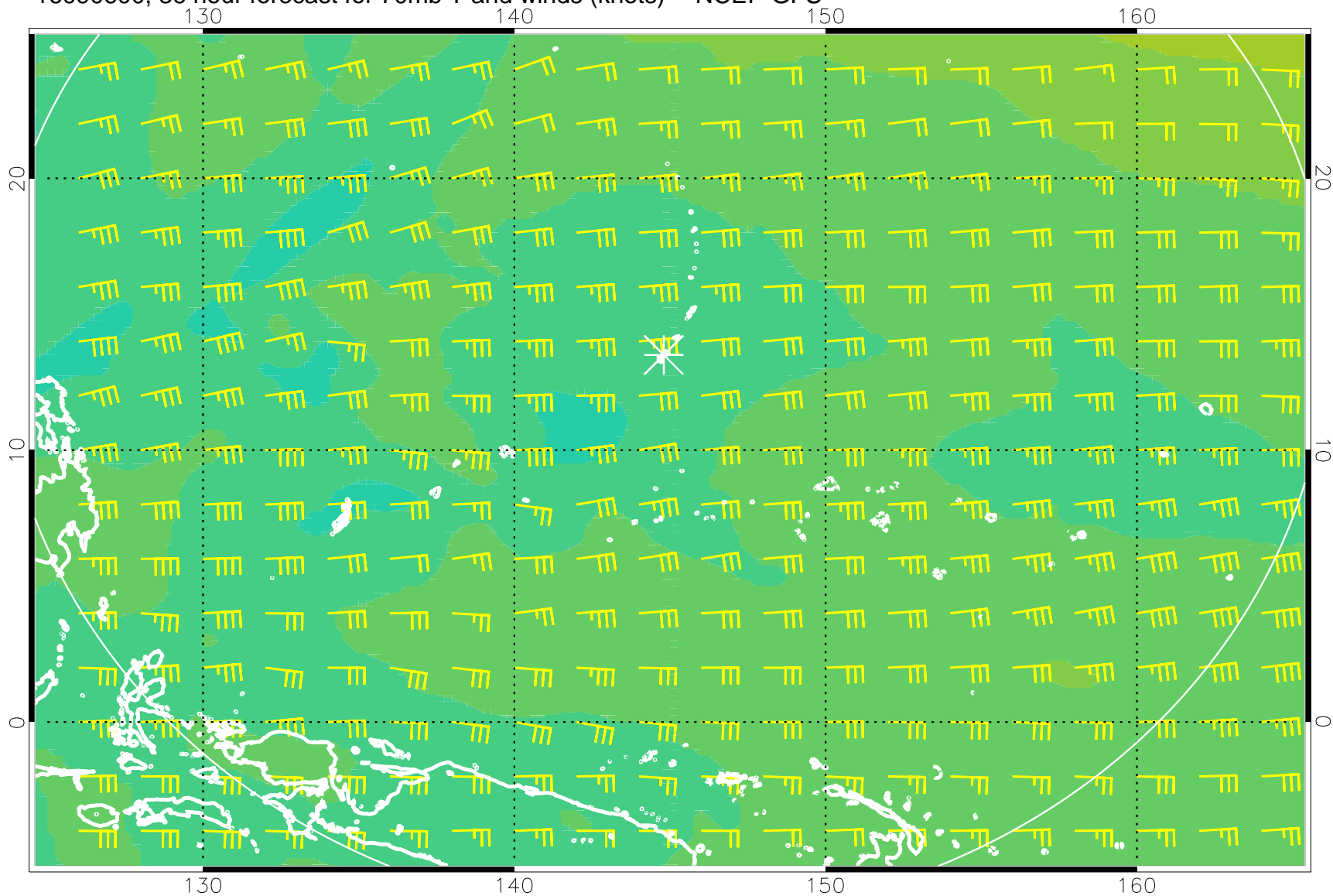
16090600, 36 hour forecast for 70mb T and winds (knots) -- NCEP GFS
