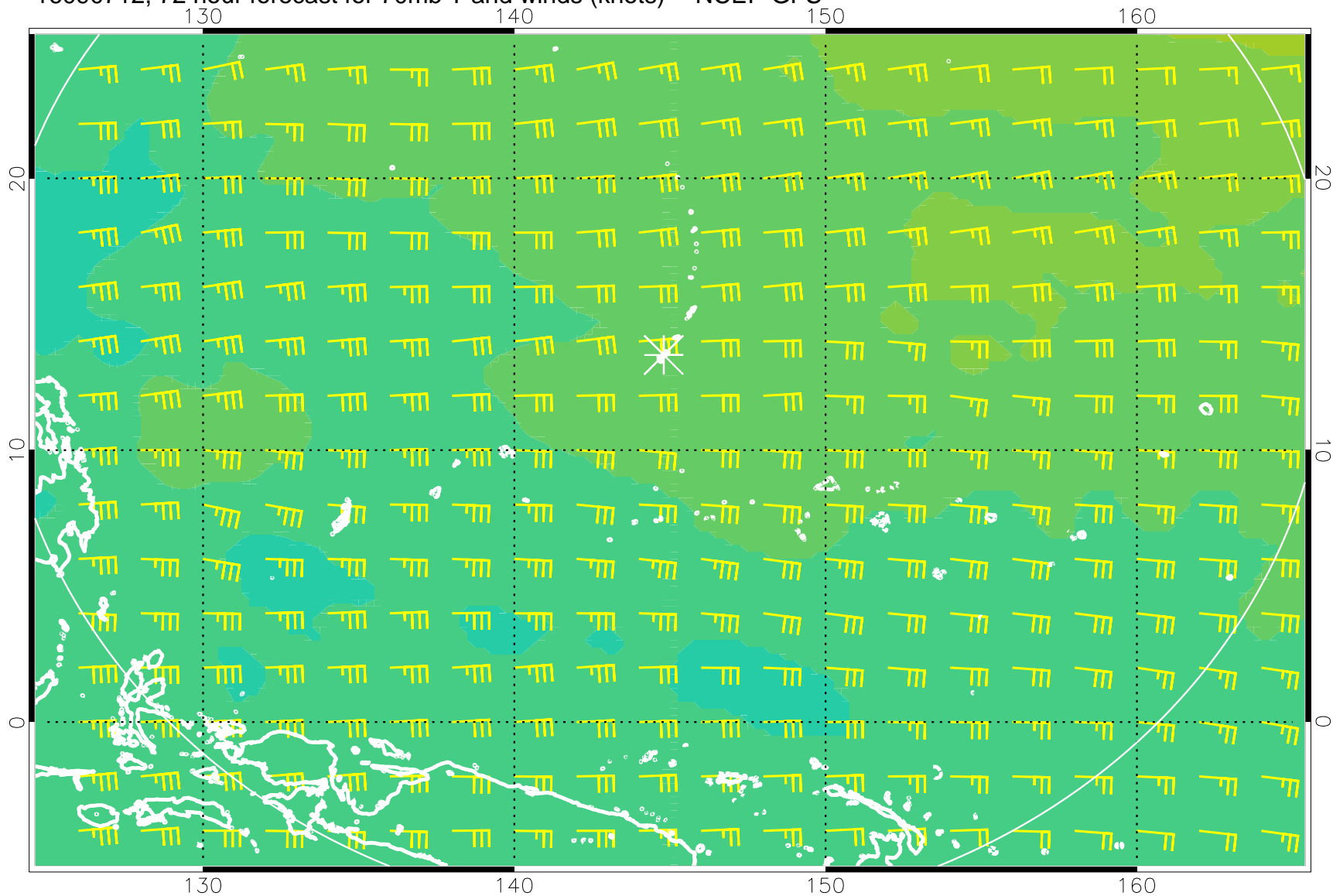
16090712, 72 hour forecast for 70mb T and winds (knots) -- NCEP GFS
