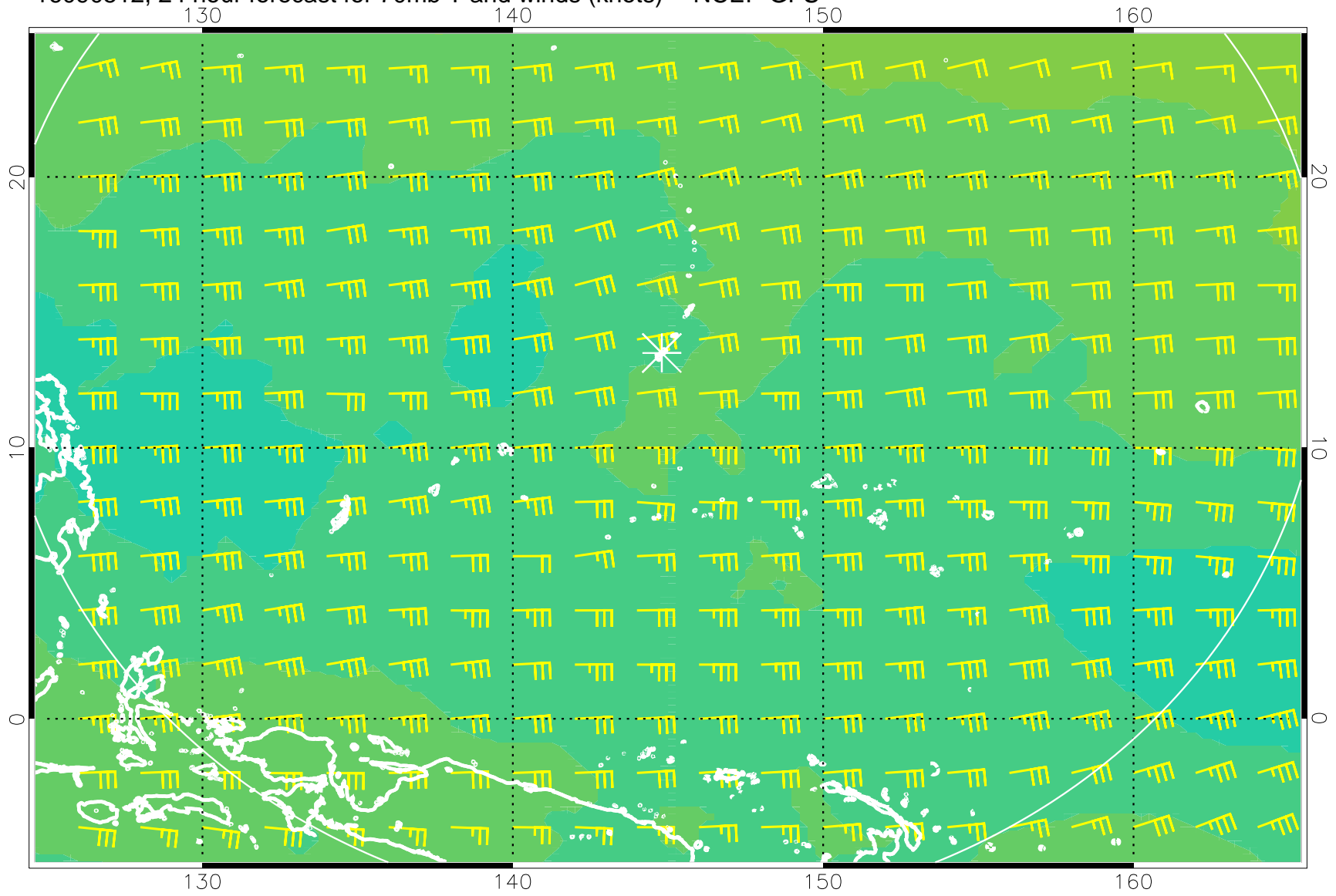
16090512, 24 hour forecast for 70mb T and winds (knots) -- NCEP GFS
