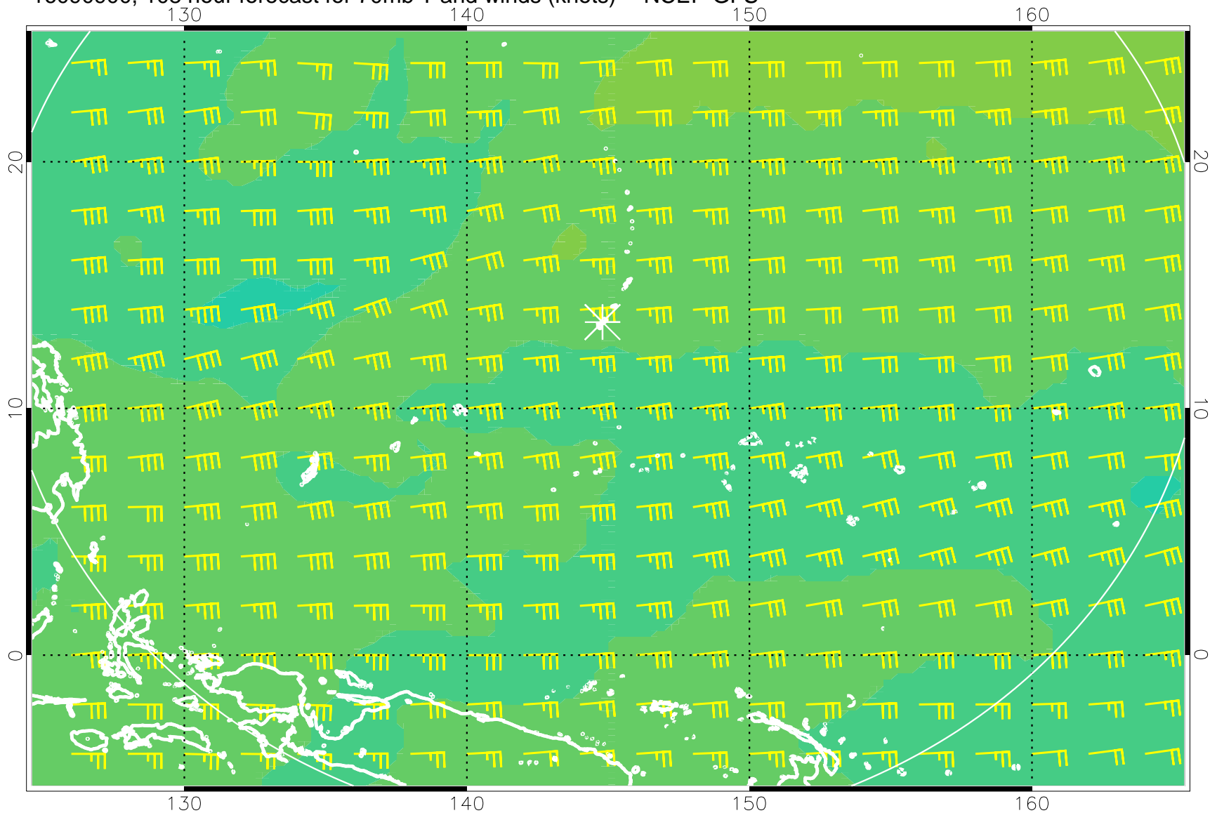
16090900, 108 hour forecast for 70mb T and winds (knots) -- NCEP GFS
