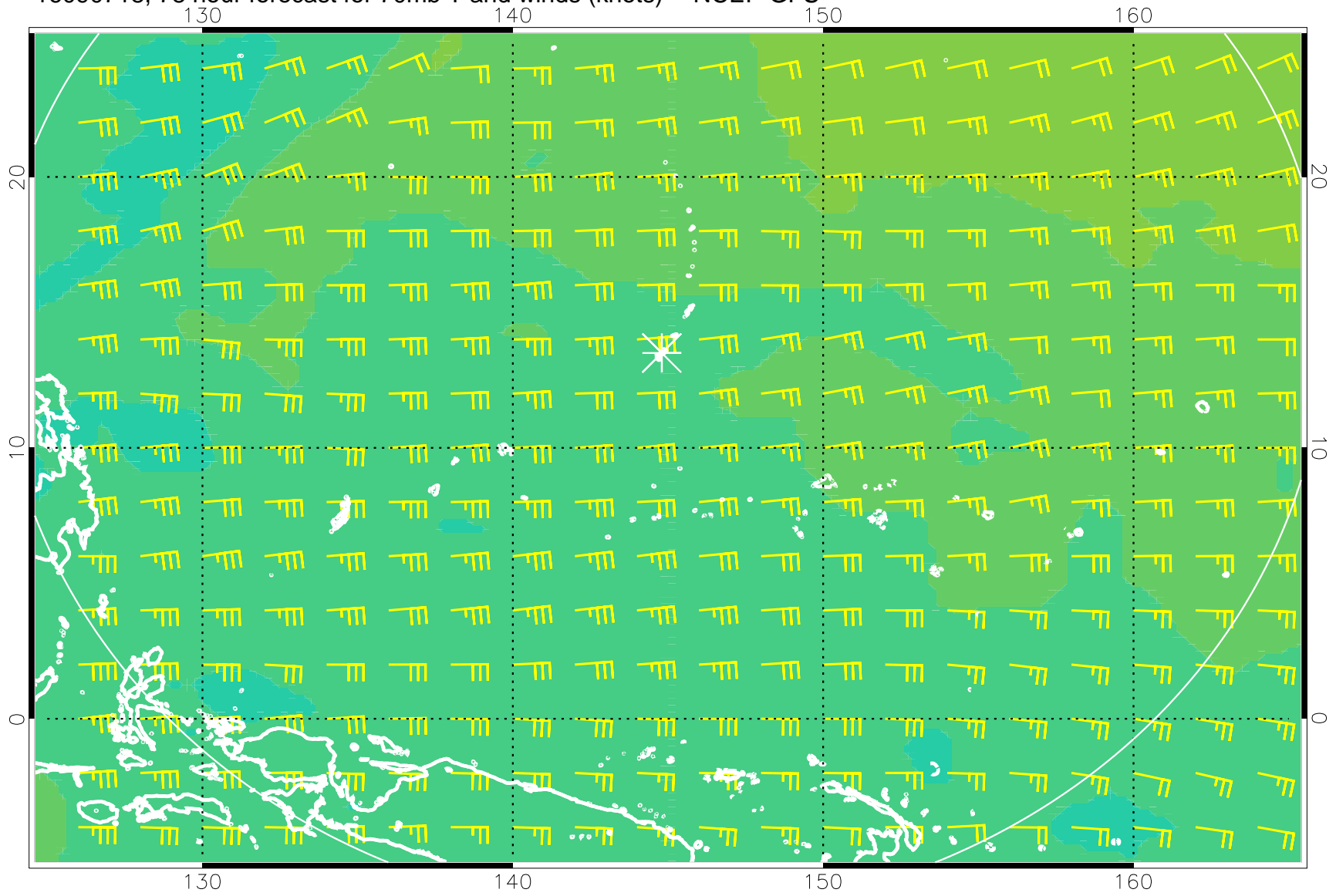
16090718, 78 hour forecast for 70mb T and winds (knots) -- NCEP GFS
