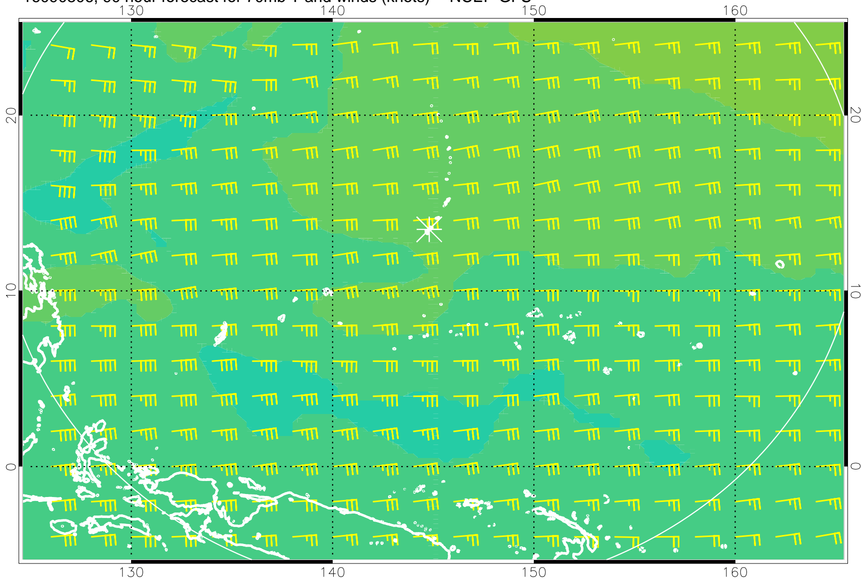
16090806, 90 hour forecast for 70mb T and winds (knots) -- NCEP GFS
