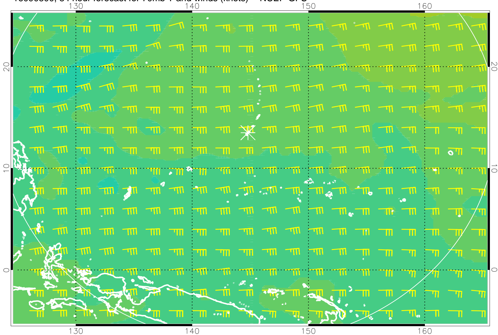
16090800, 84 hour forecast for 70mb T and winds (knots) -- NCEP GFS
