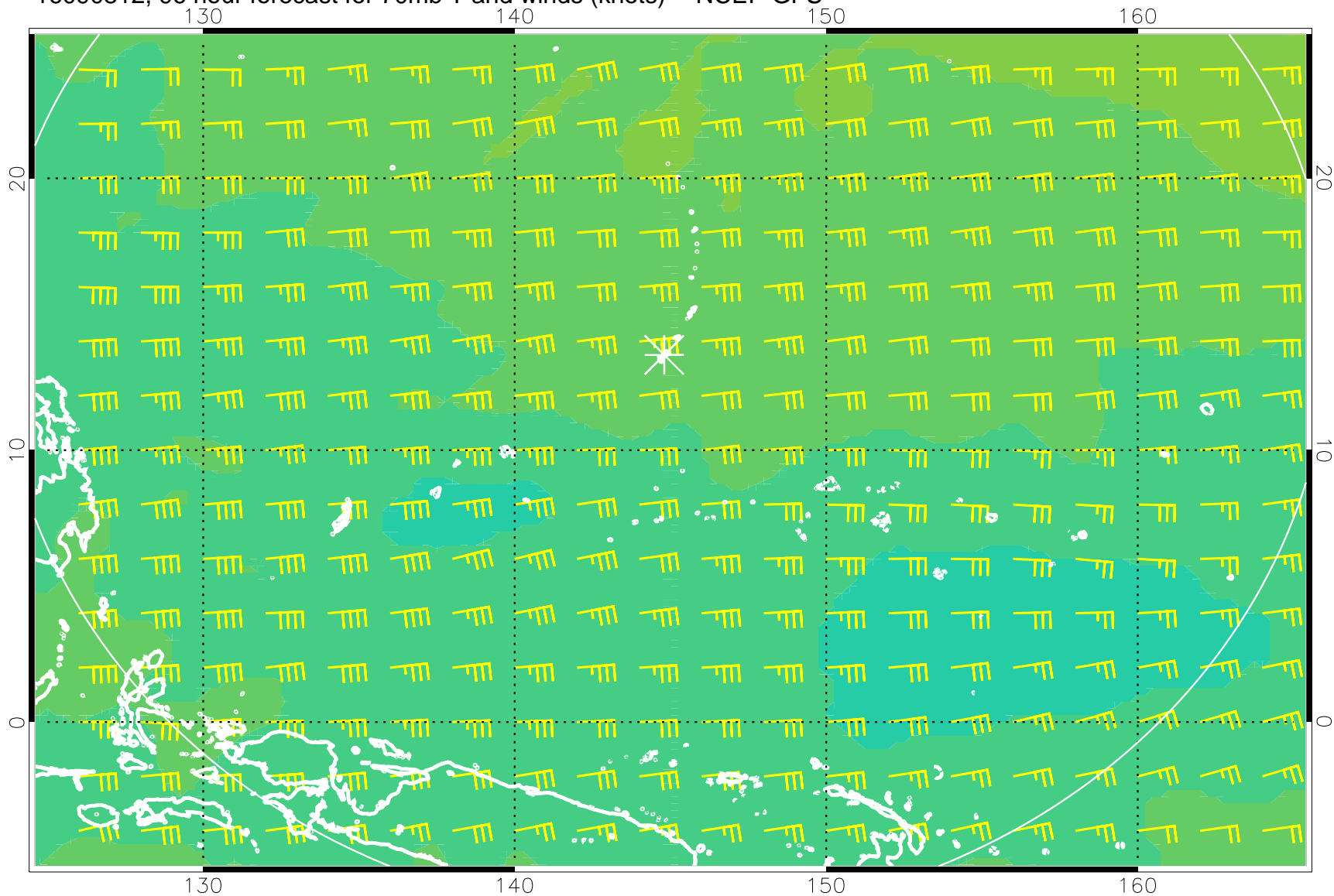
16090812, 96 hour forecast for 70mb T and winds (knots) -- NCEP GFS
