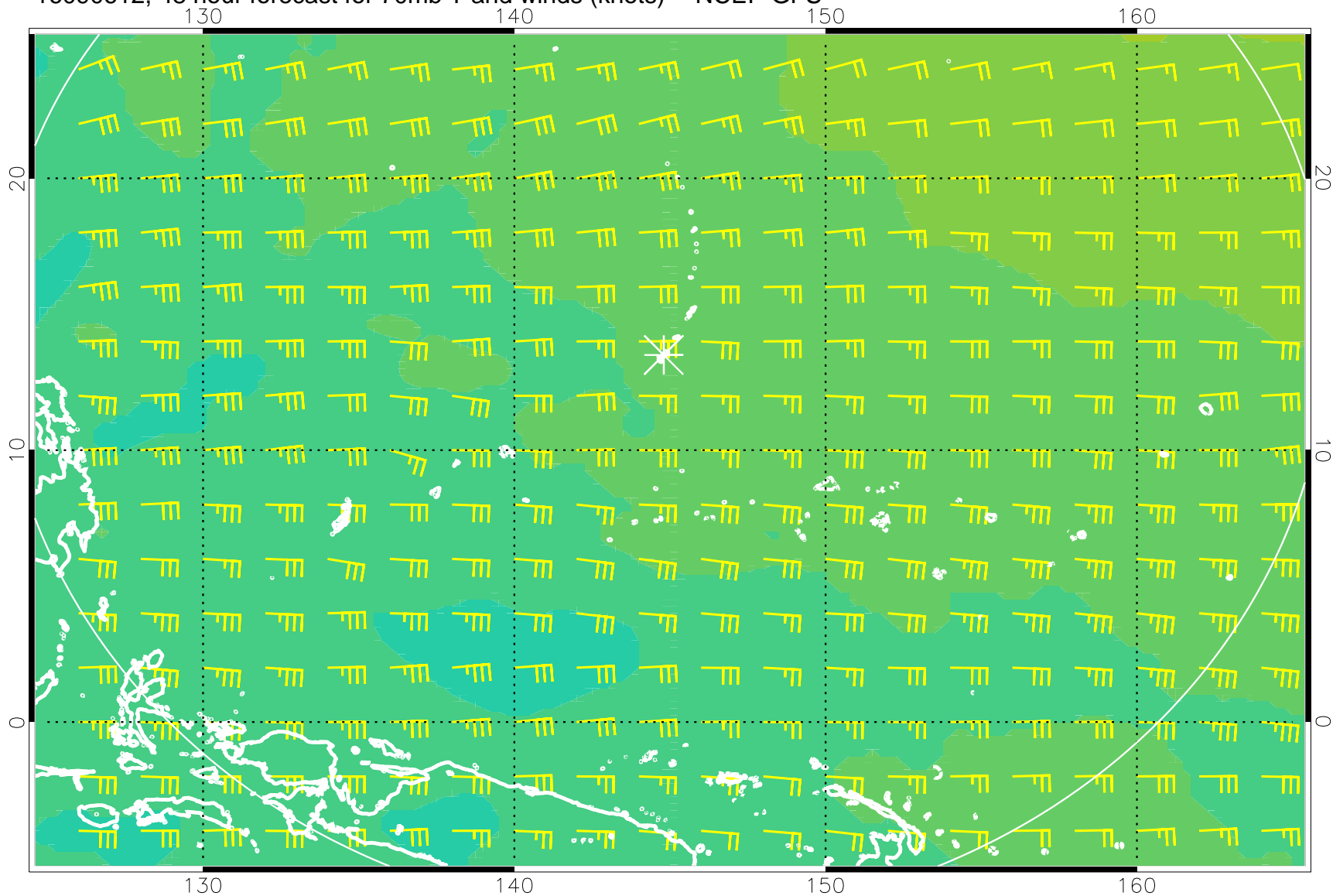
16090612, 48 hour forecast for 70mb T and winds (knots) -- NCEP GFS
