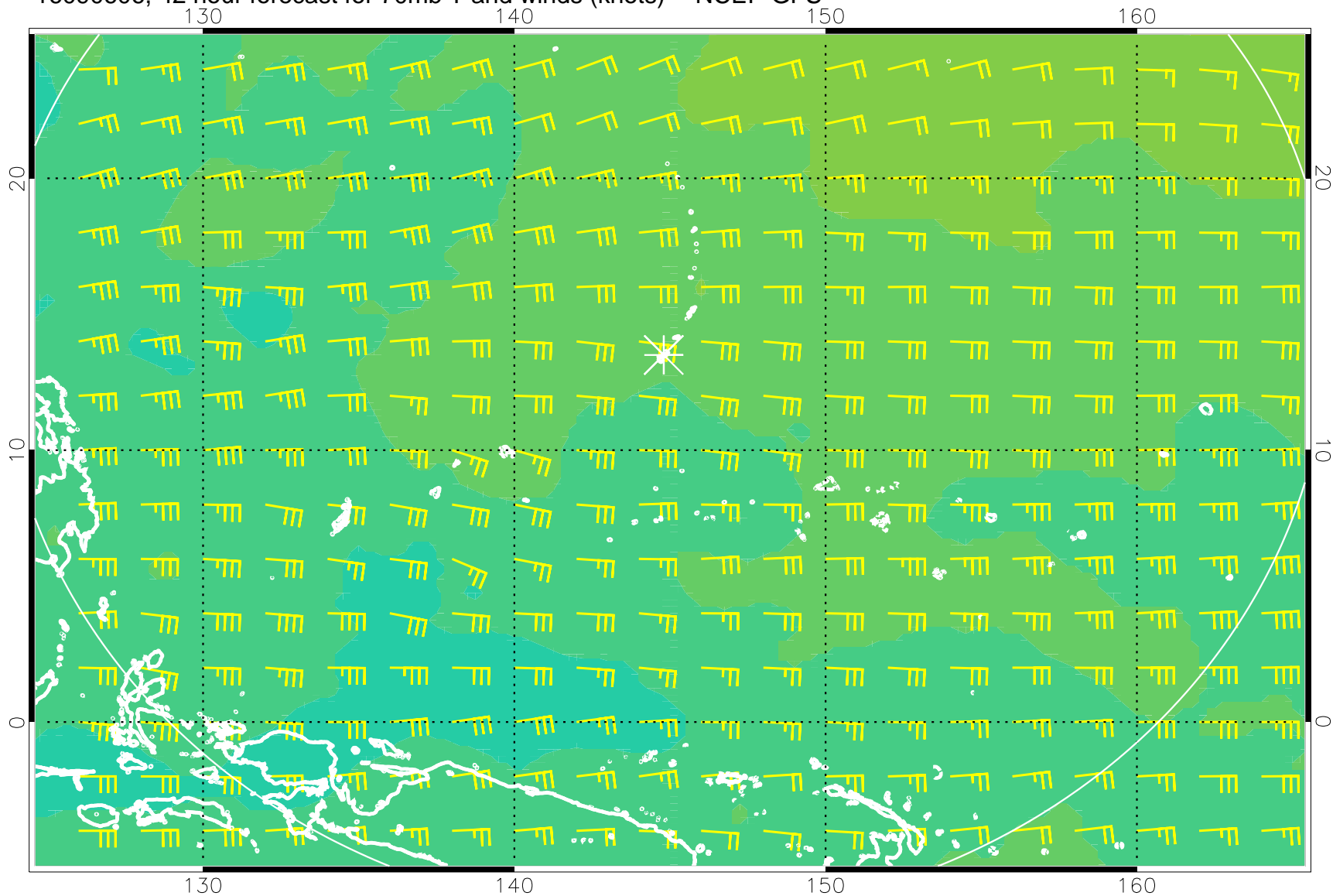
16090606, 42 hour forecast for 70mb T and winds (knots) -- NCEP GFS
