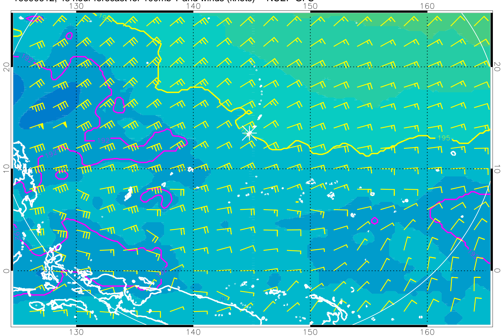
16090612, 48 hour forecast for 100mb T and winds (knots) -- NCEP GFS
