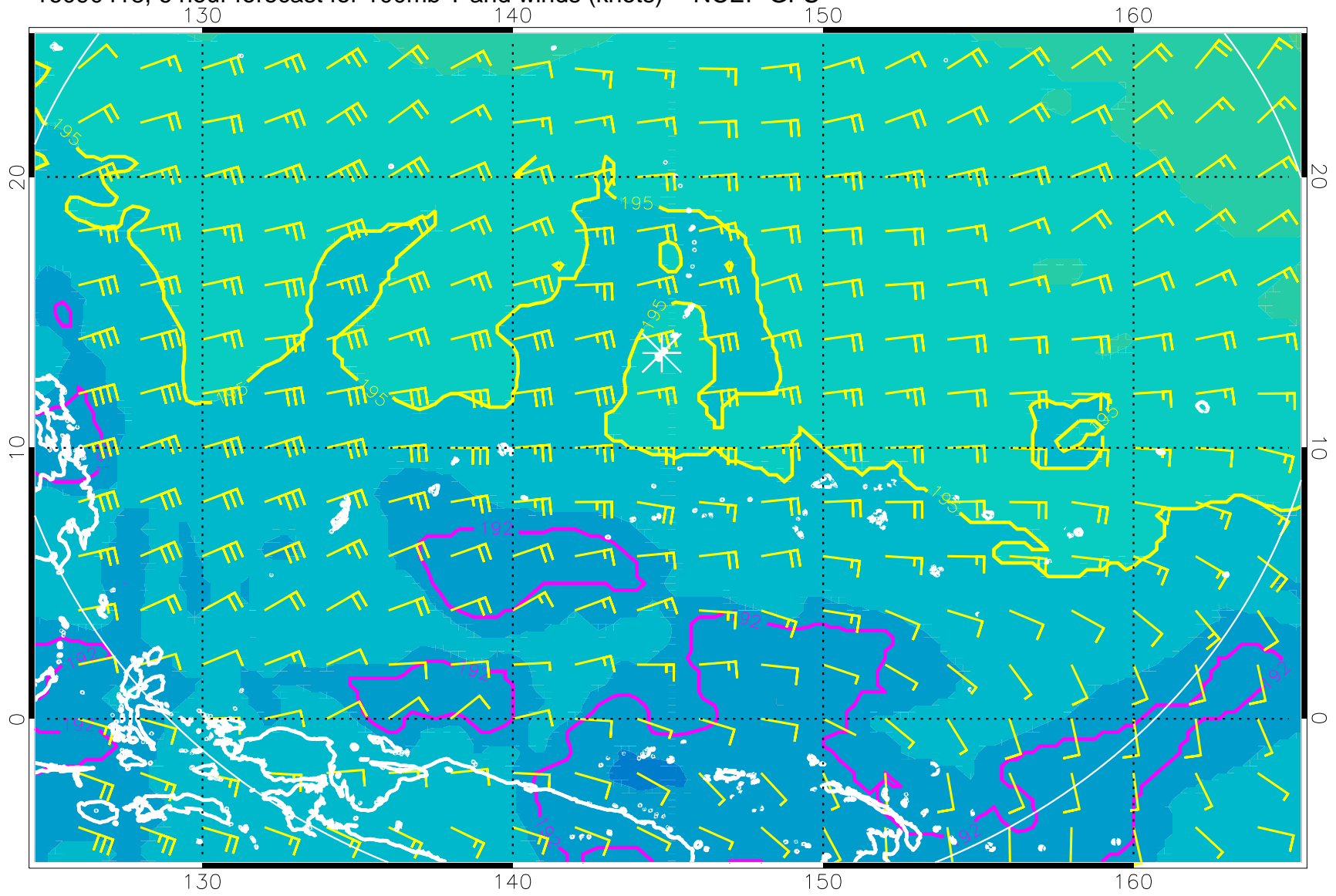
16090418, 6 hour forecast for 100mb T and winds (knots) -- NCEP GFS
