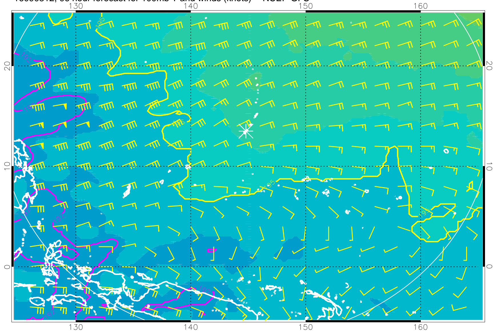
16090812, 96 hour forecast for 100mb T and winds (knots) -- NCEP GFS
