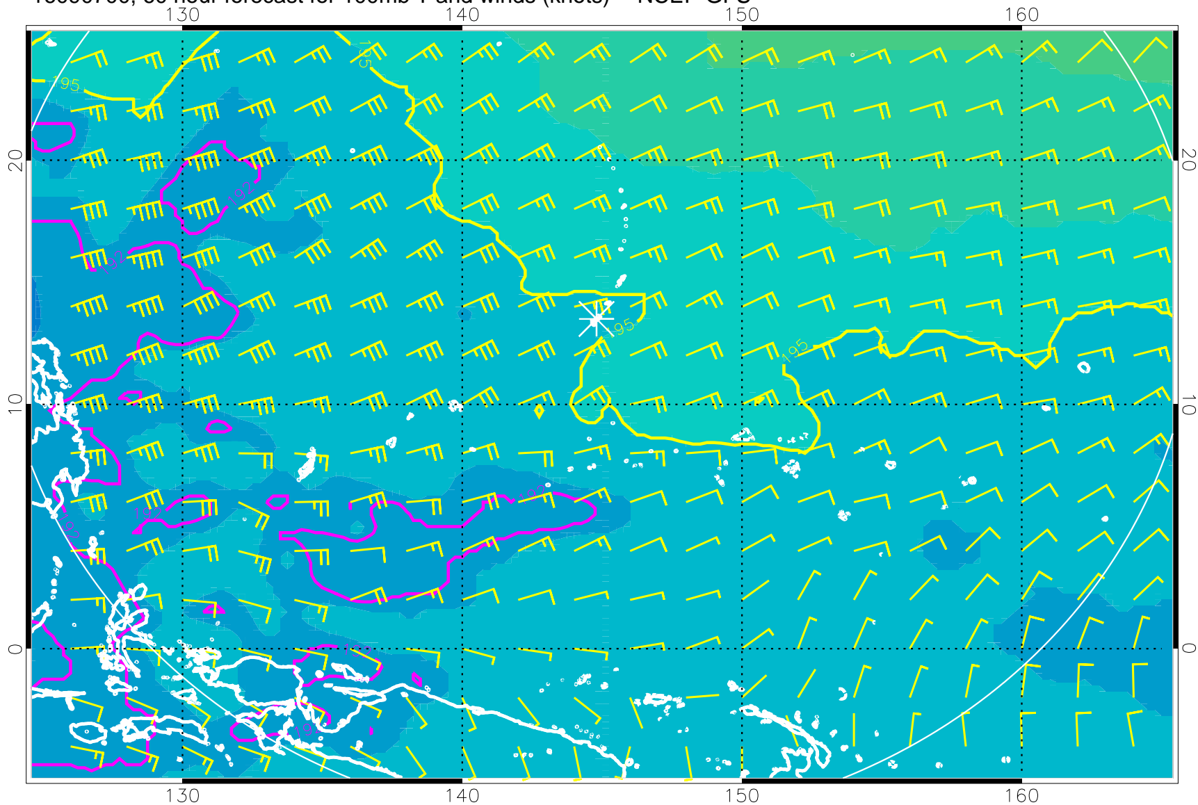
16090700, 60 hour forecast for 100mb T and winds (knots) -- NCEP GFS
