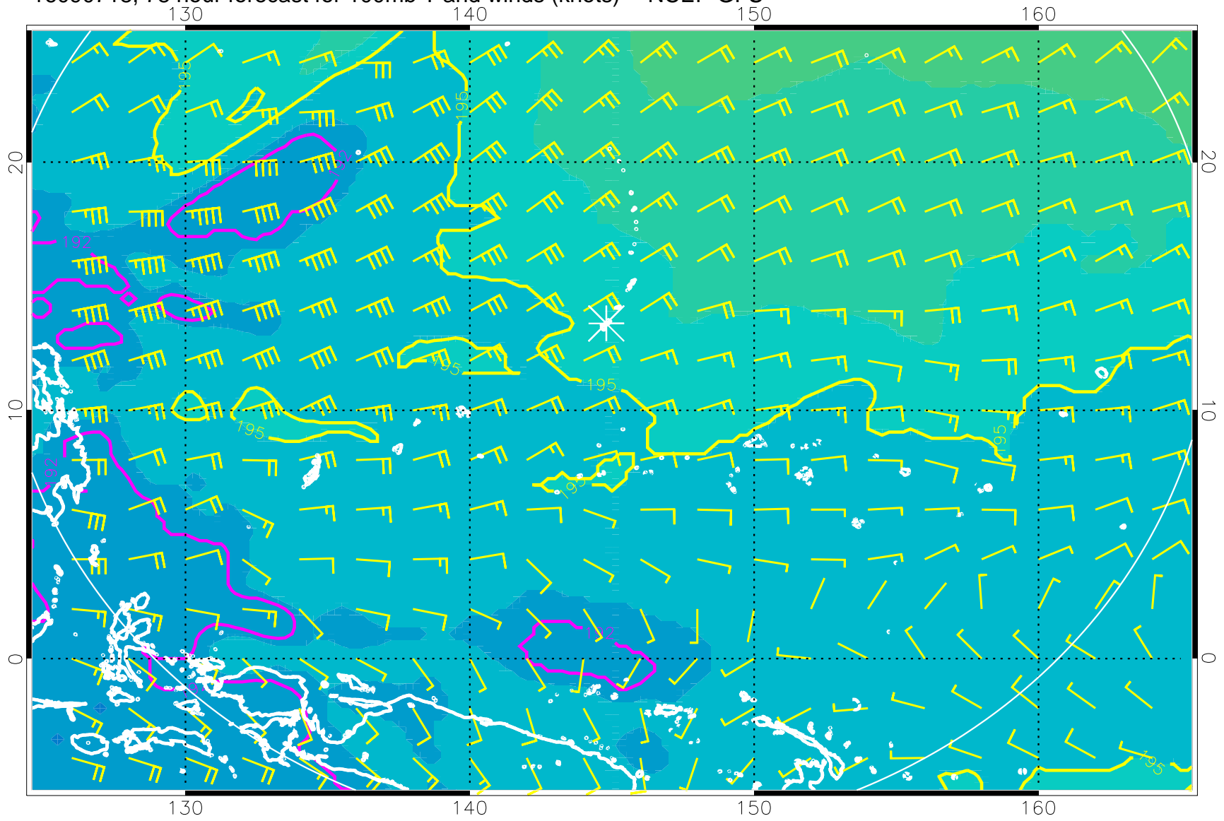
16090718, 78 hour forecast for 100mb T and winds (knots) -- NCEP GFS
