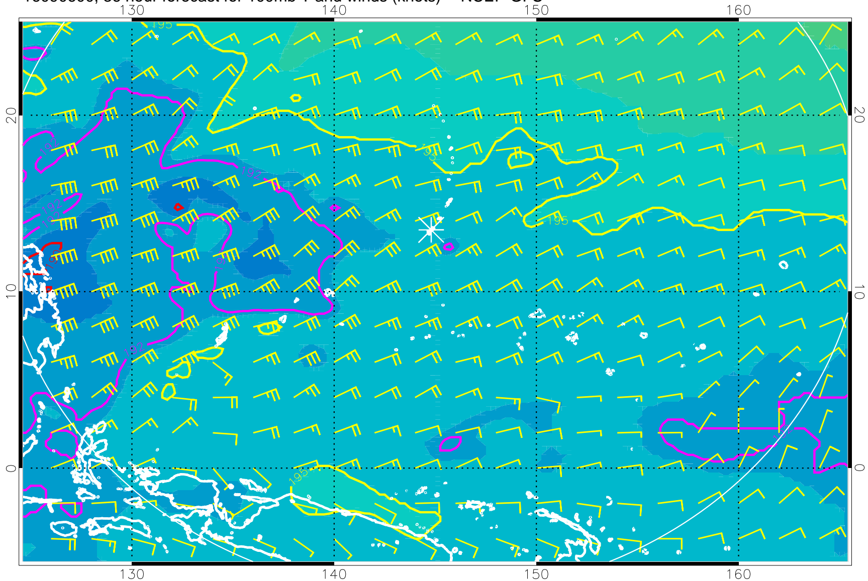
16090600, 36 hour forecast for 100mb T and winds (knots) -- NCEP GFS
