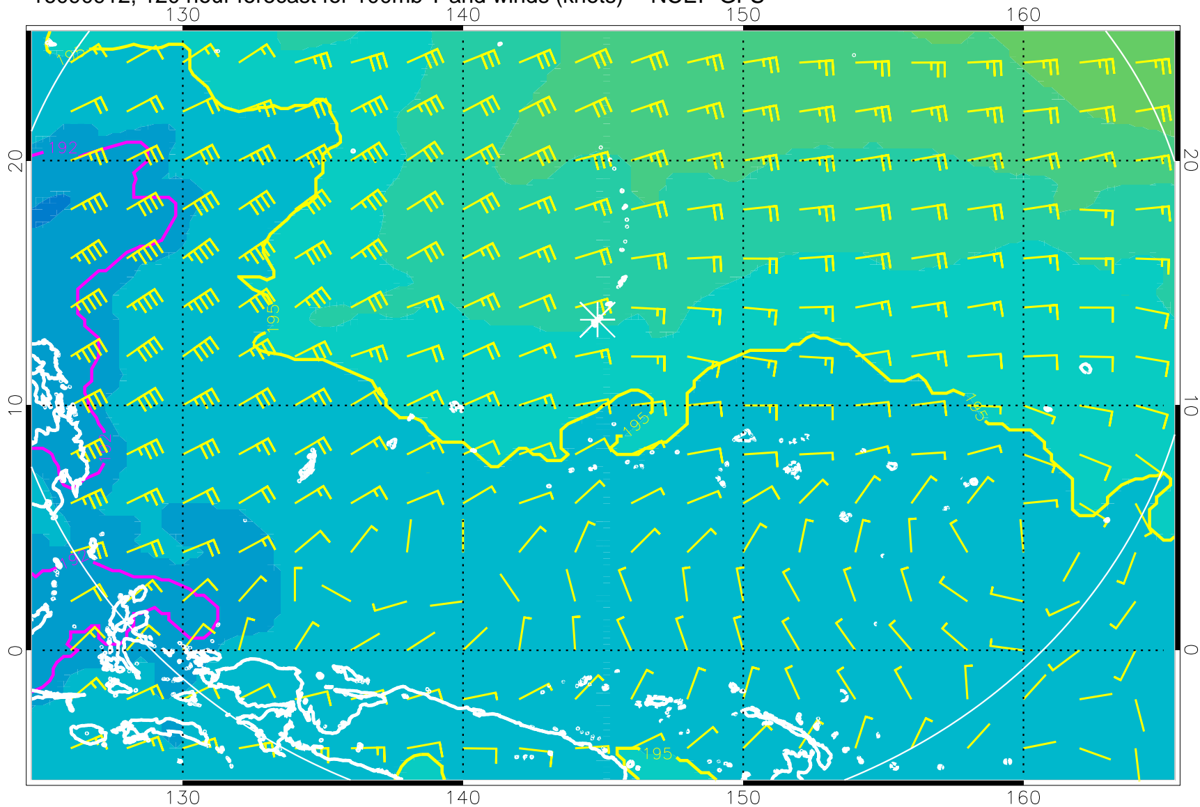
16090912, 120 hour forecast for 100mb T and winds (knots) -- NCEP GFS
