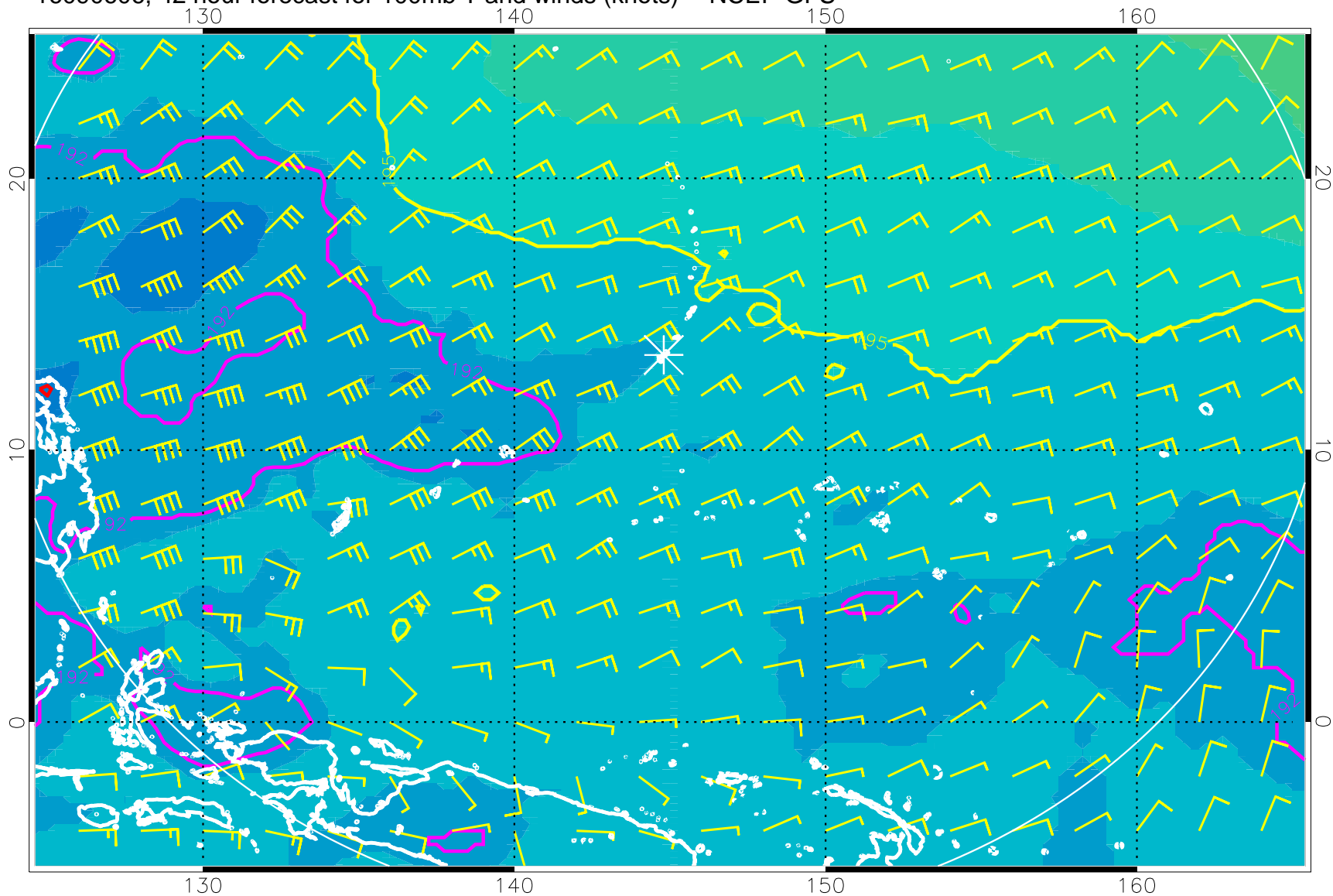
16090606, 42 hour forecast for 100mb T and winds (knots) -- NCEP GFS
