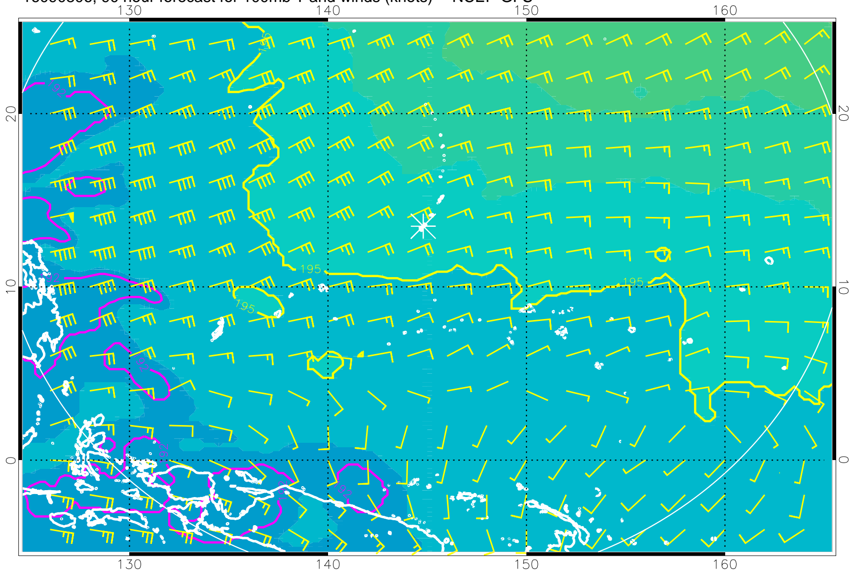
16090806, 90 hour forecast for 100mb T and winds (knots) -- NCEP GFS
