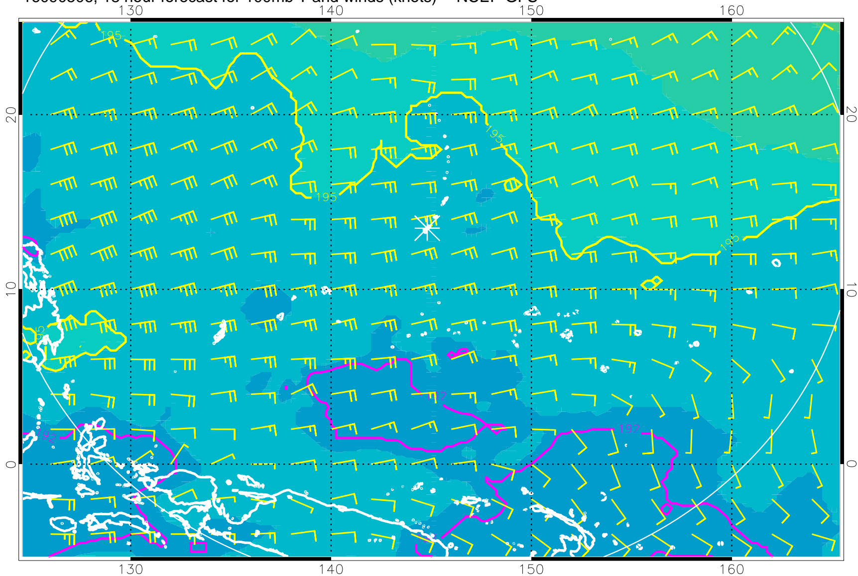
16090506, 18 hour forecast for 100mb T and winds (knots) -- NCEP GFS
