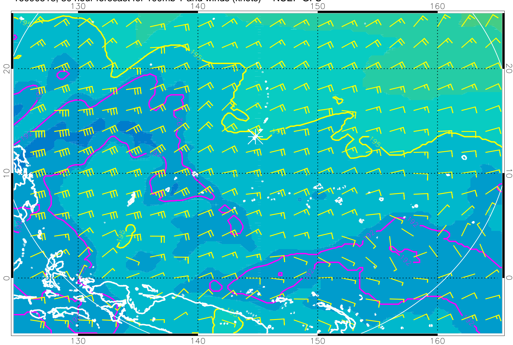
16090518, 30 hour forecast for 100mb T and winds (knots) -- NCEP GFS
