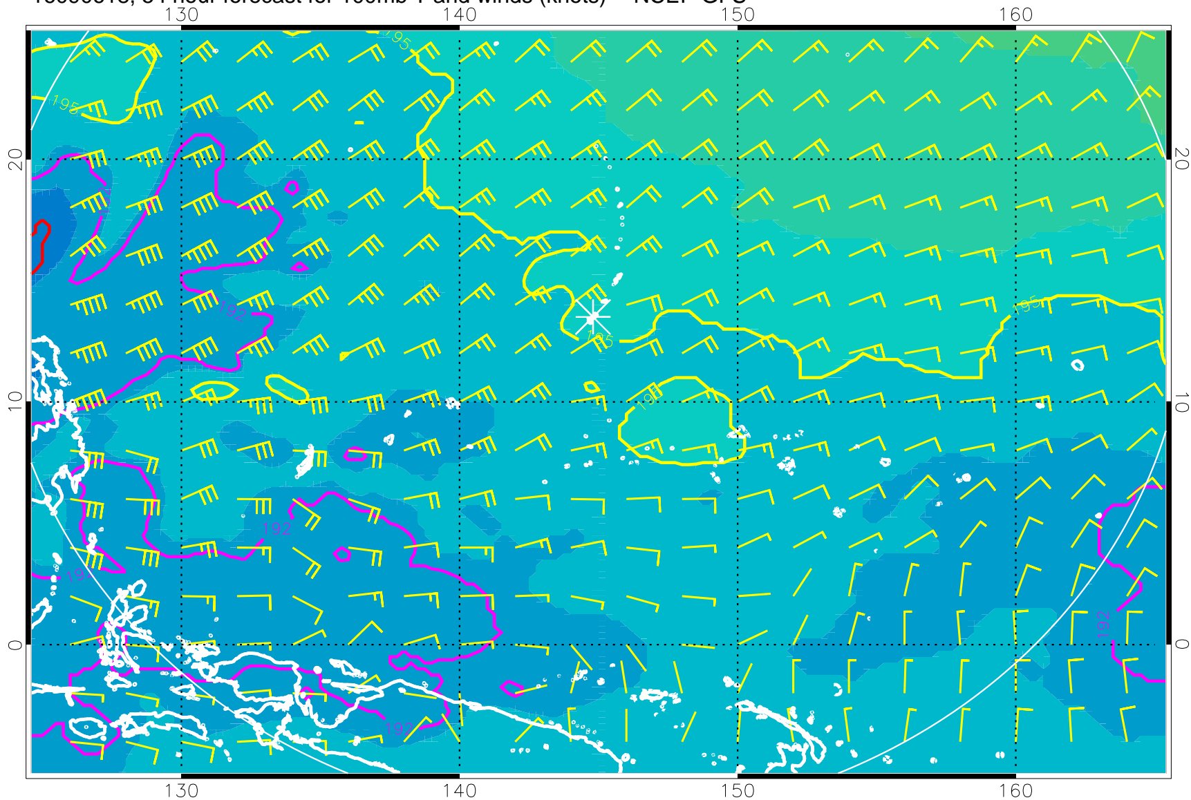
16090618, 54 hour forecast for 100mb T and winds (knots) -- NCEP GFS
