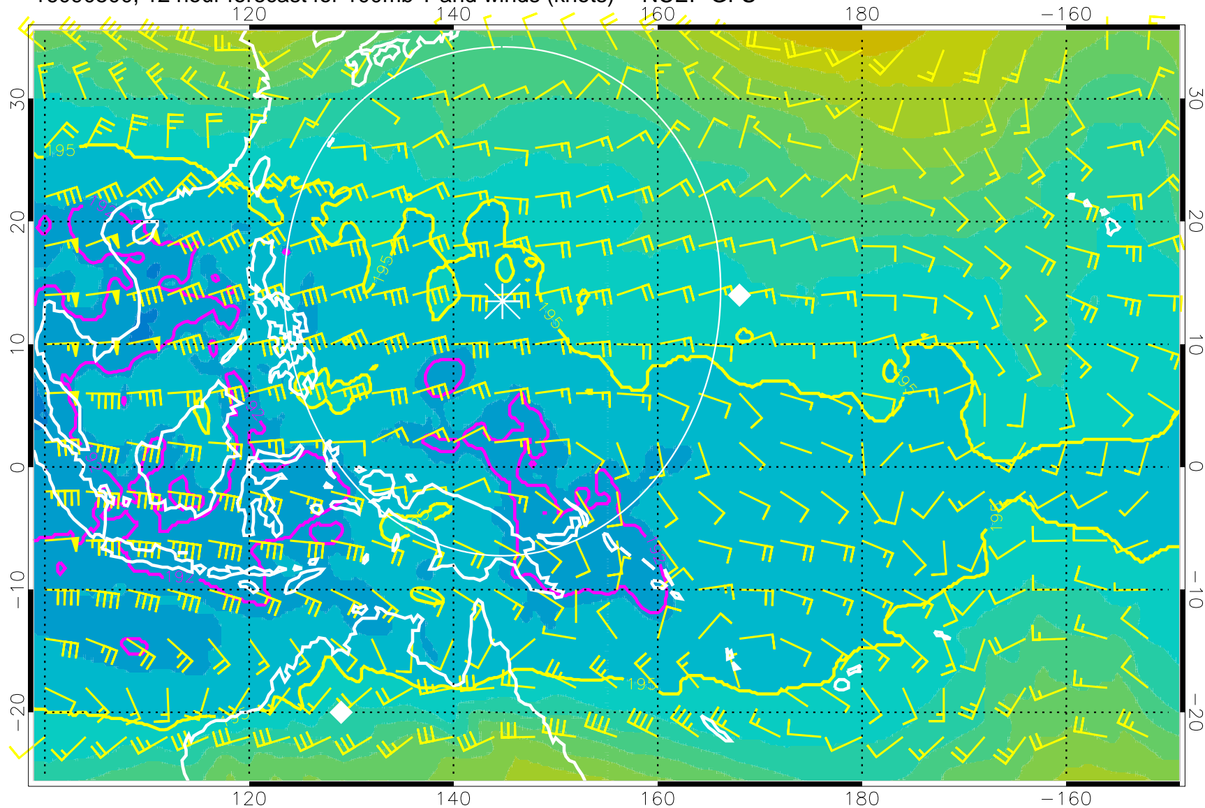
16090500, 12 hour forecast for 100mb T and winds (knots) -- NCEP GFS
