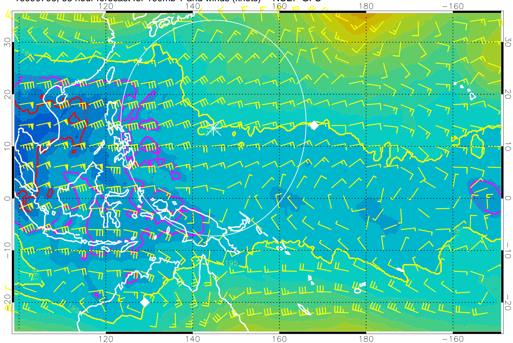
16090706, 66 hour forecast for 100mb T and winds (knots) -- NCEP GFS
