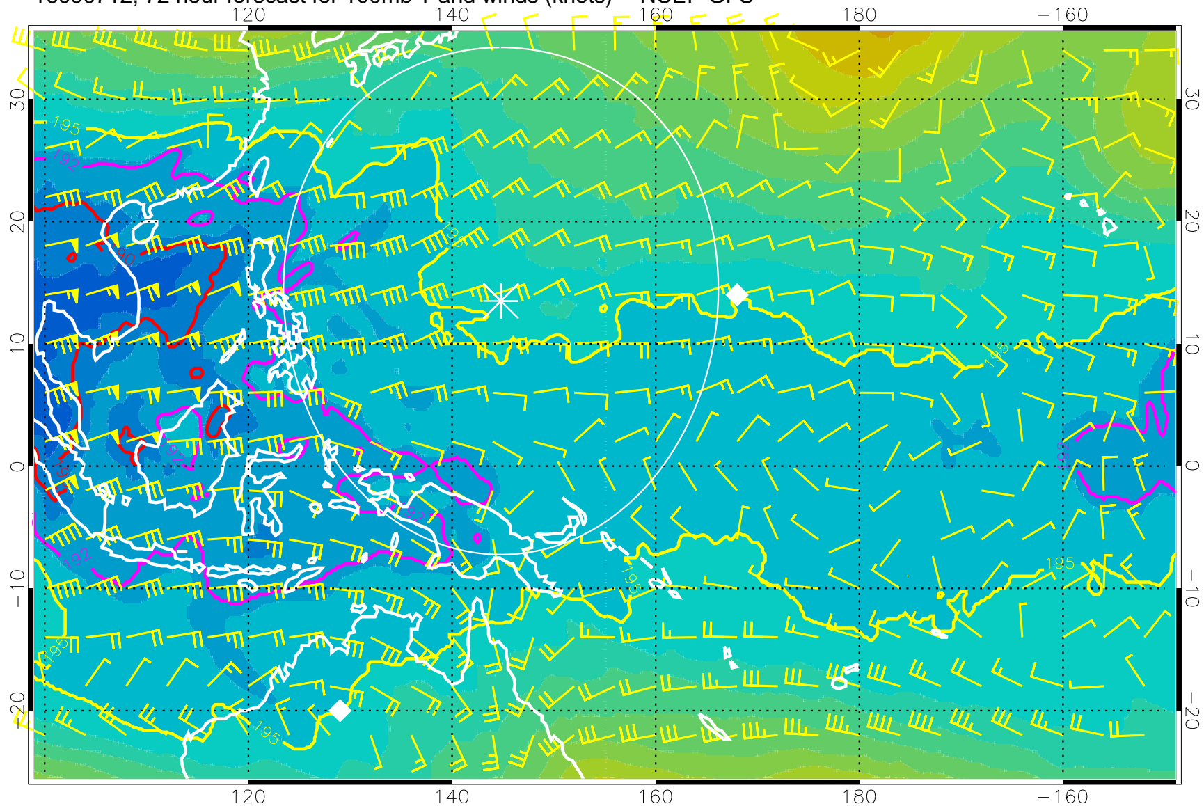
16090712, 72 hour forecast for 100mb T and winds (knots) -- NCEP GFS
