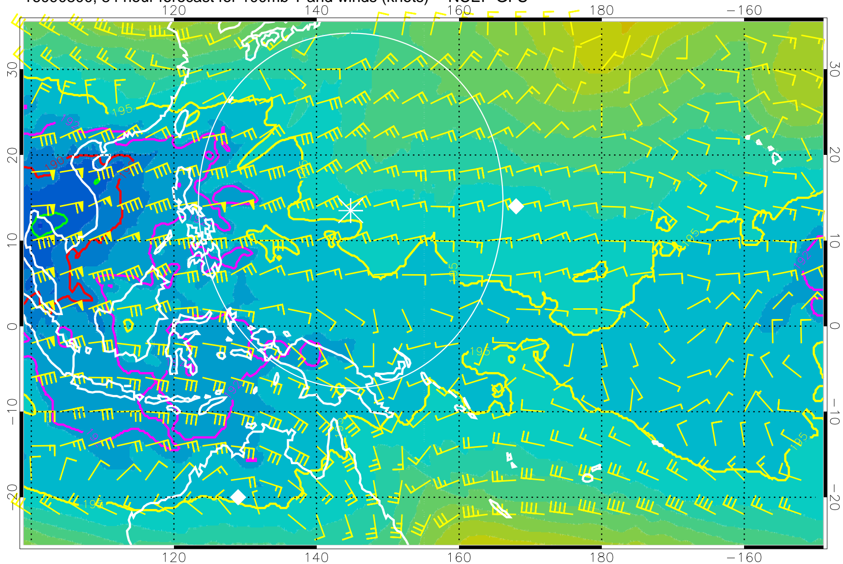
16090800, 84 hour forecast for 100mb T and winds (knots) -- NCEP GFS
