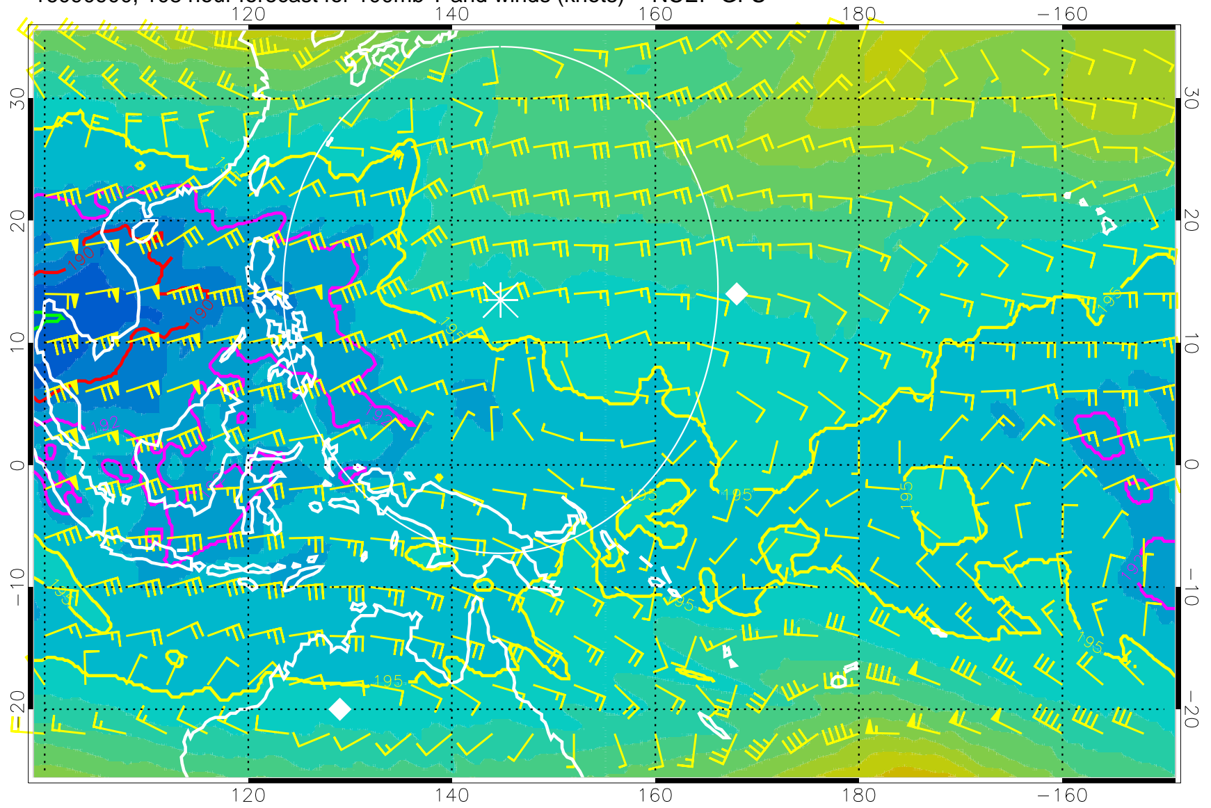
16090900, 108 hour forecast for 100mb T and winds (knots) -- NCEP GFS
