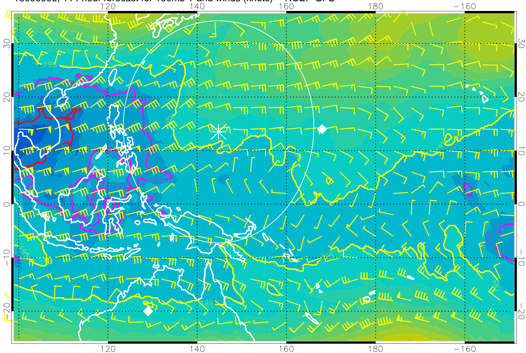
16090906, 114 hour forecast for 100mb T and winds (knots) -- NCEP GFS
