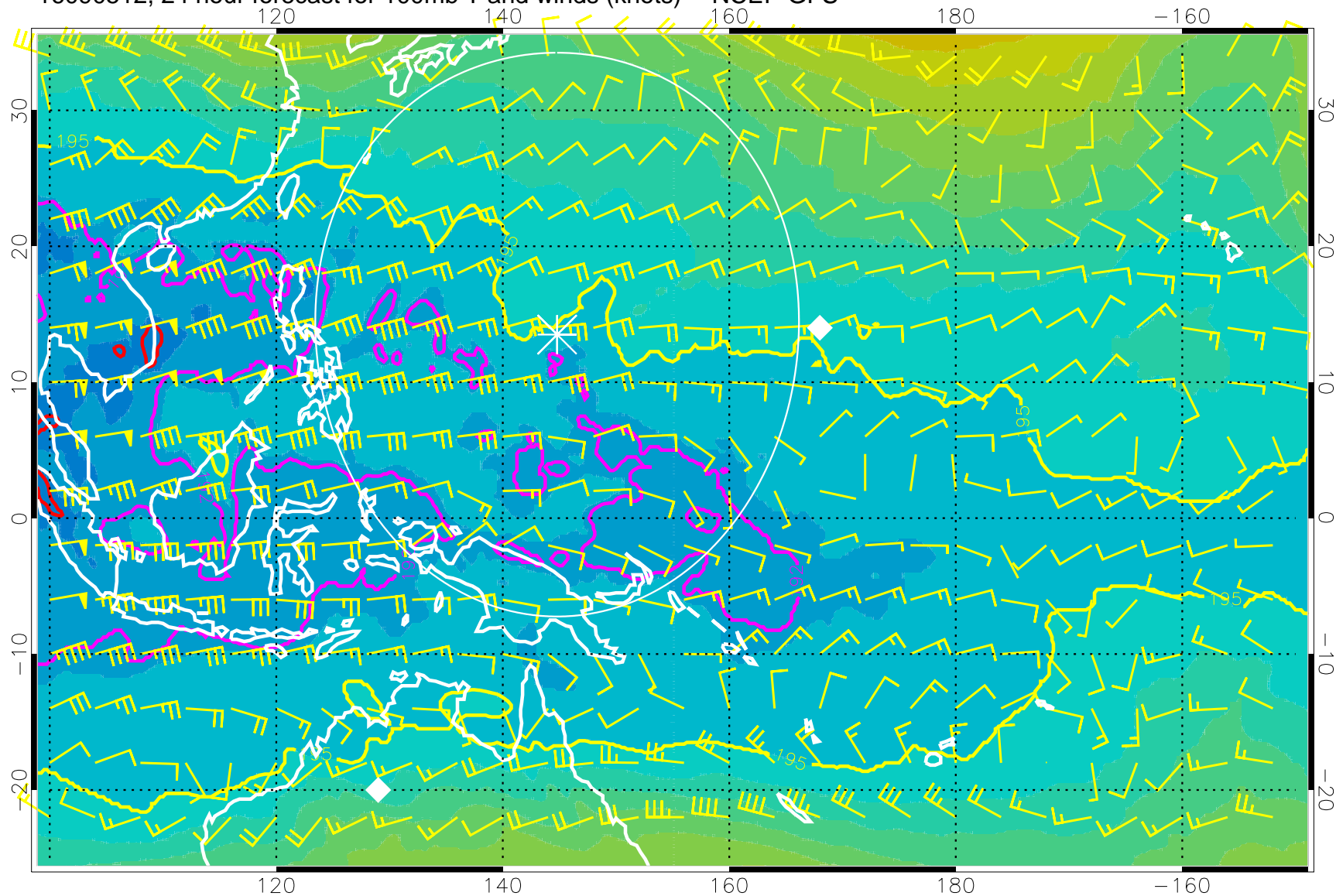
16090512, 24 hour forecast for 100mb T and winds (knots) -- NCEP GFS
