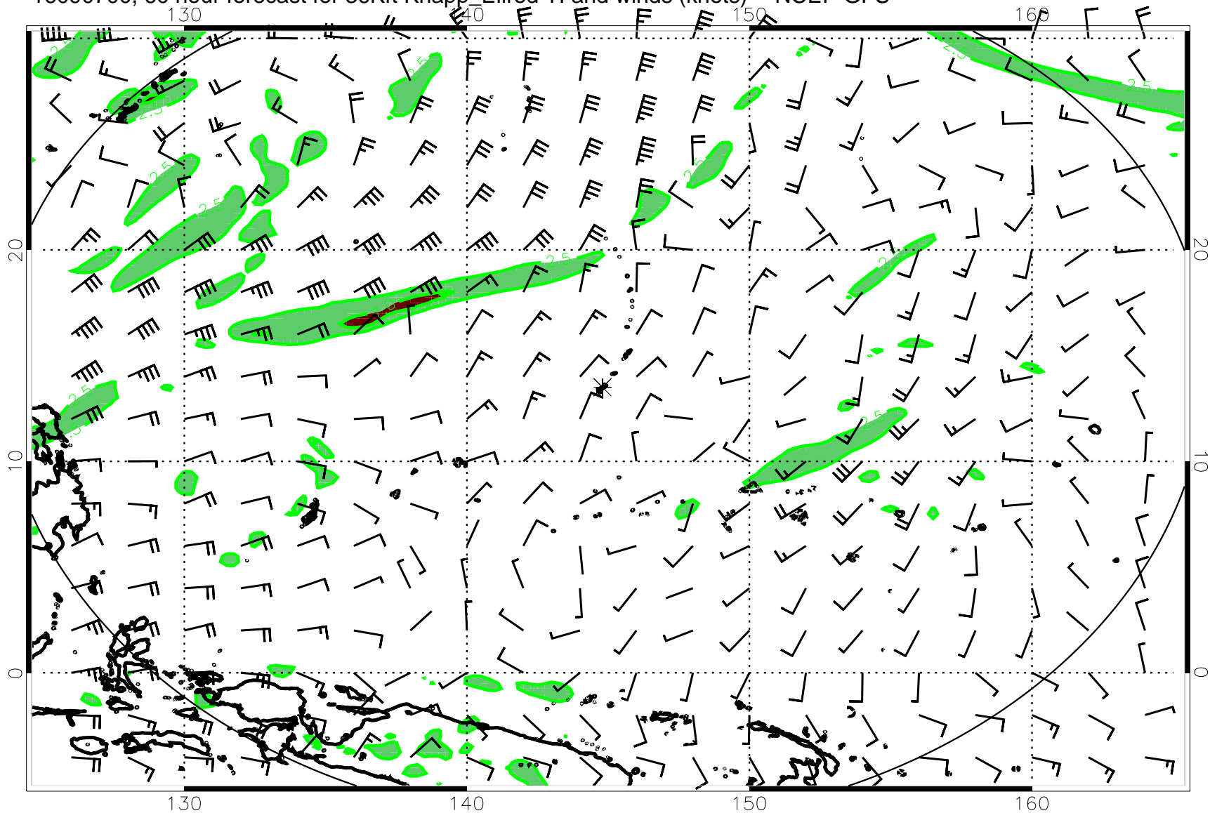
16090700, 60 hour forecast for 36Kft Knapp_Ellrod TI and winds (knots) -- NCEP GFS
