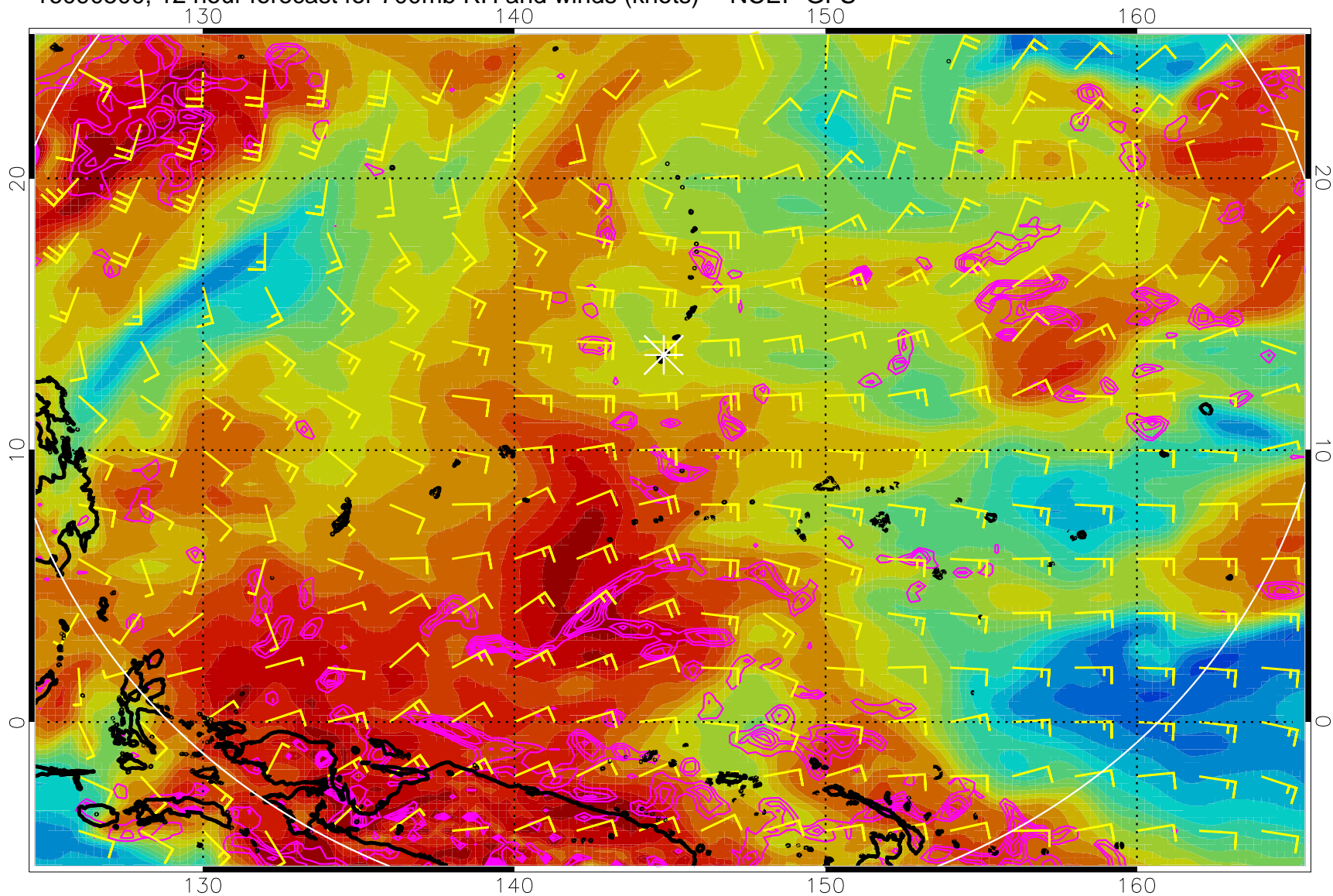
16090500, 12 hour forecast for 700mb RH and winds (knots) -- NCEP GFS
