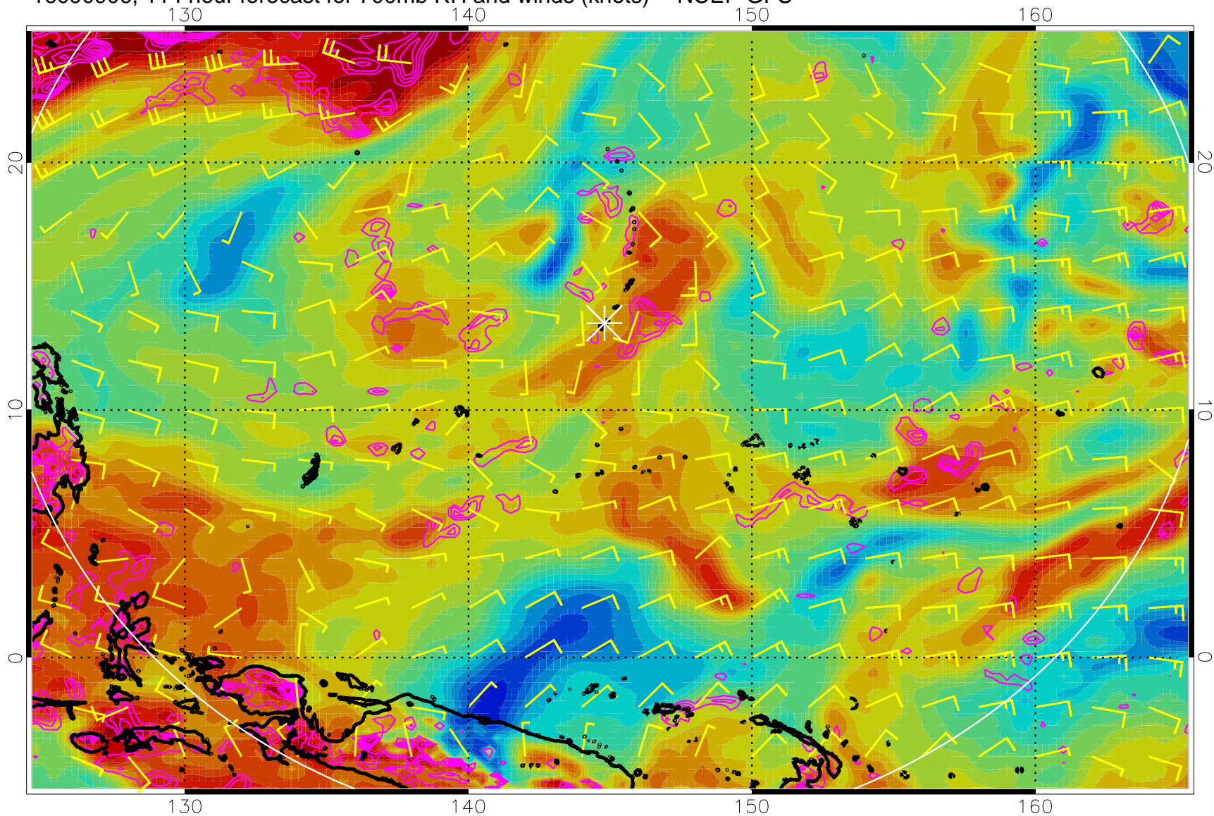
16090906, 114 hour forecast for 700mb RH and winds (knots) -- NCEP GFS
