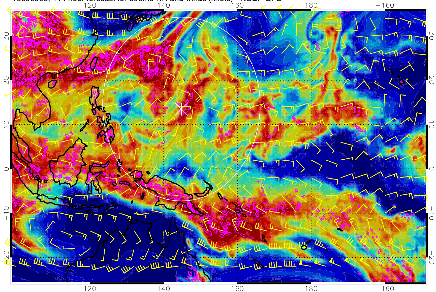
16090906, 114 hour forecast for 500mb RH and winds (knots) - NCEP GFS
