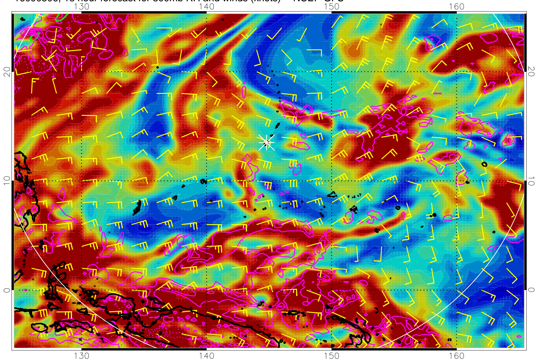
16090506, 18 hour forecast for 300mb RH and winds (knots) -- NCEP GFS
