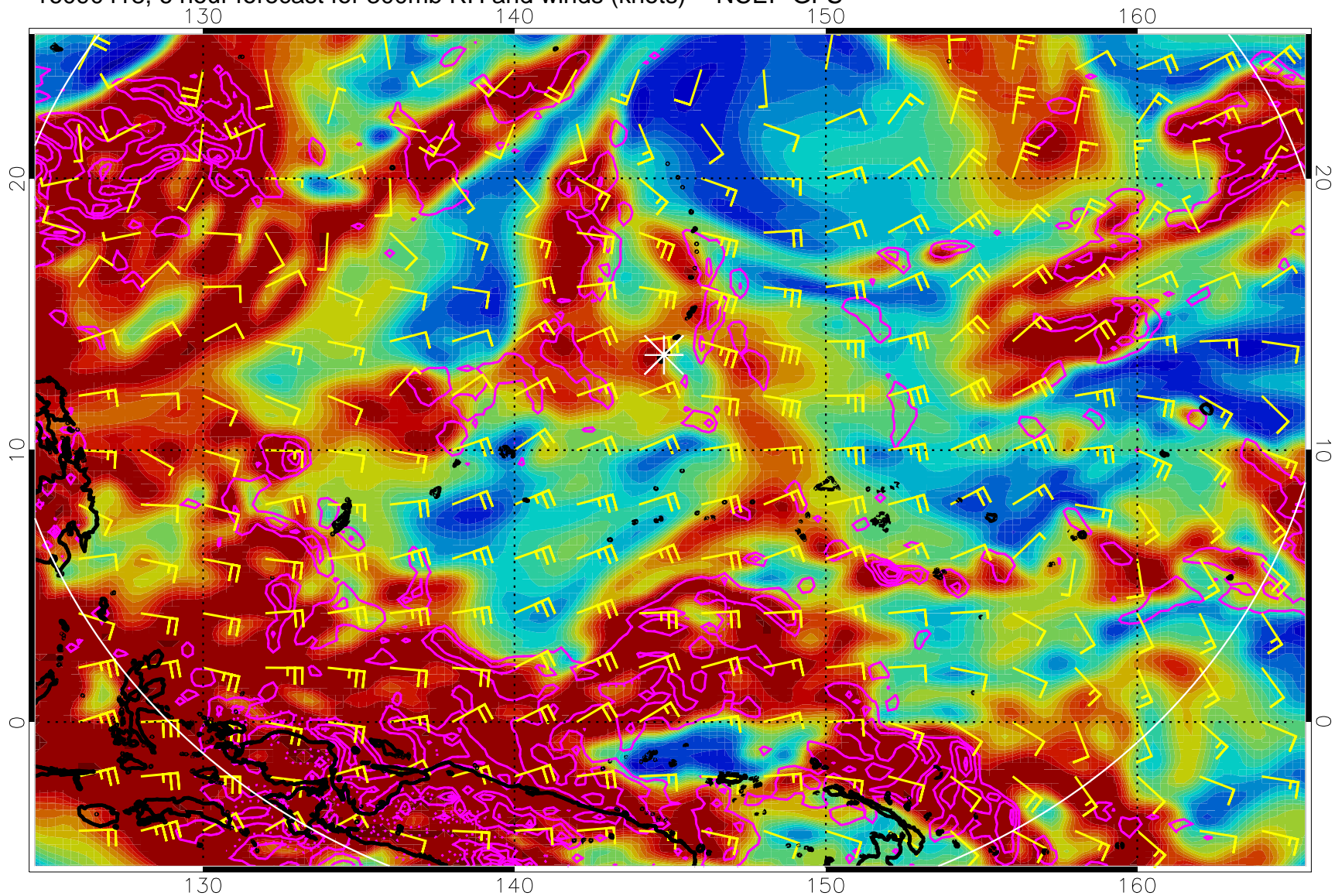
16090418, 6 hour forecast for 300mb RH and winds (knots) -- NCEP GFS
