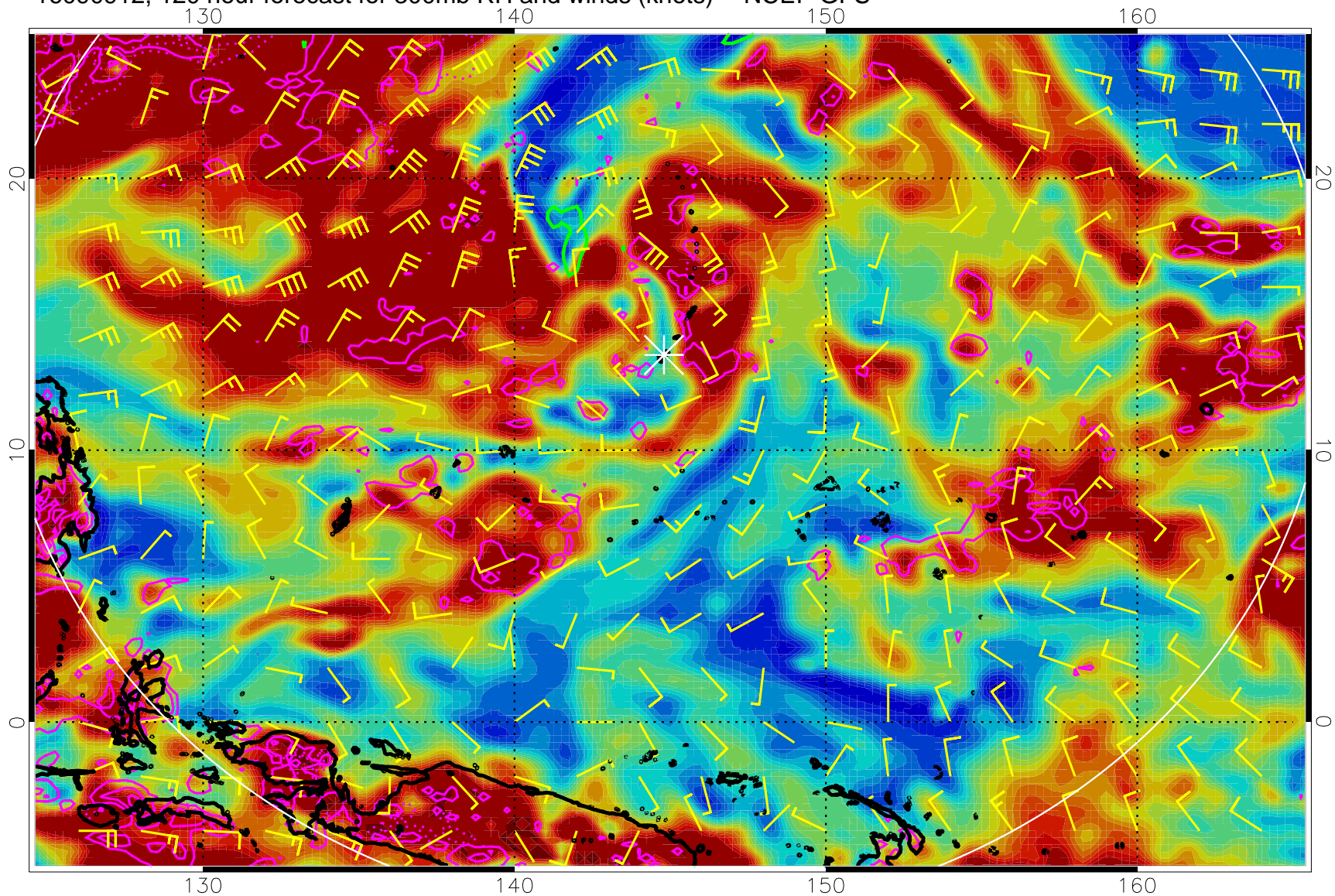
16090912, 120 hour forecast for 300mb RH and winds (knots) -- NCEP GFS
