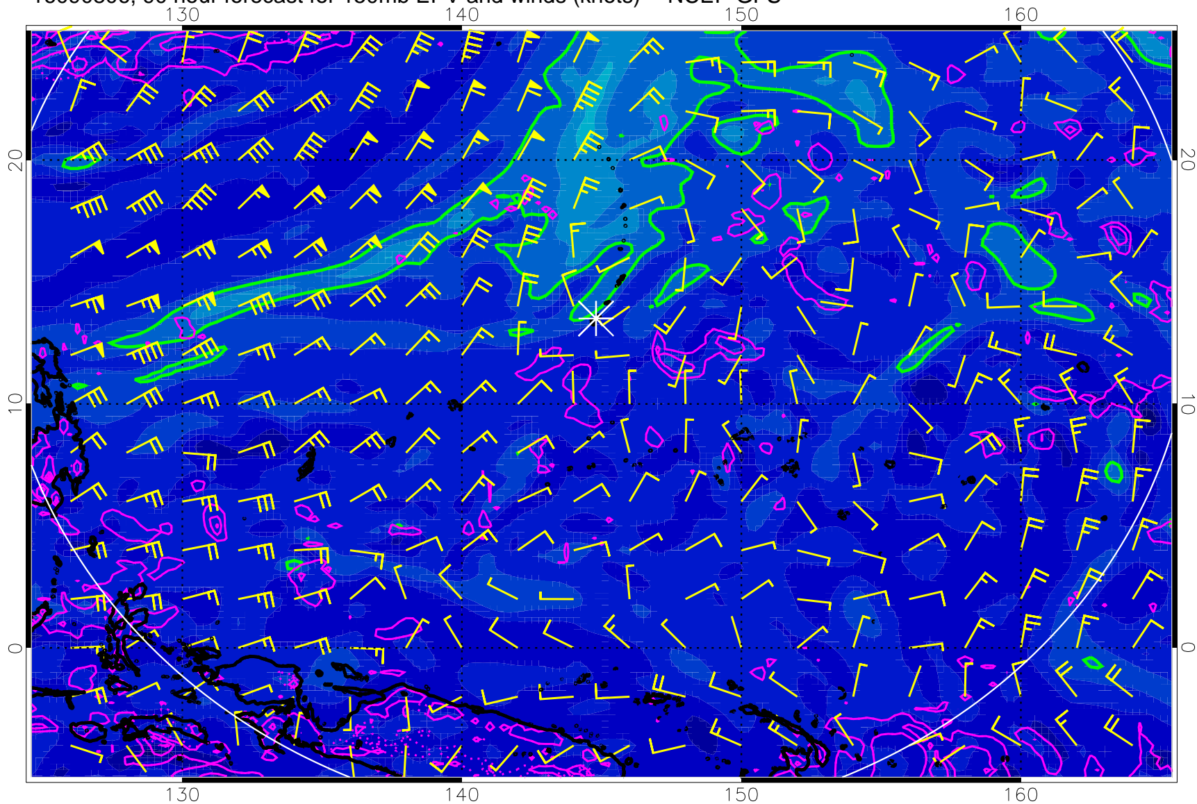
16090806, 90 hour forecast for 150mb EPV and winds (knots) -- NCEP GFS
