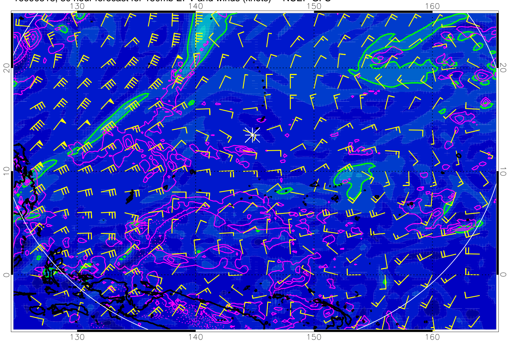
16090518, 30 hour forecast for 150mb EPV and winds (knots) -- NCEP GFS
