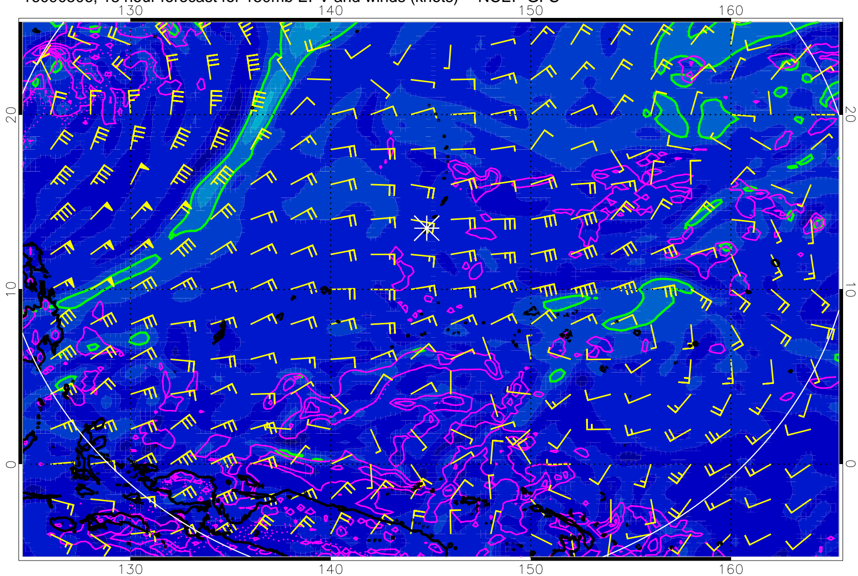
16090506, 18 hour forecast for 150mb EPV and winds (knots) -- NCEP GFS
