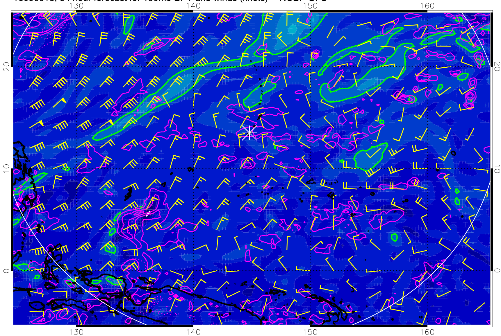
16090618, 54 hour forecast for 150mb EPV and winds (knots) -- NCEP GFS
