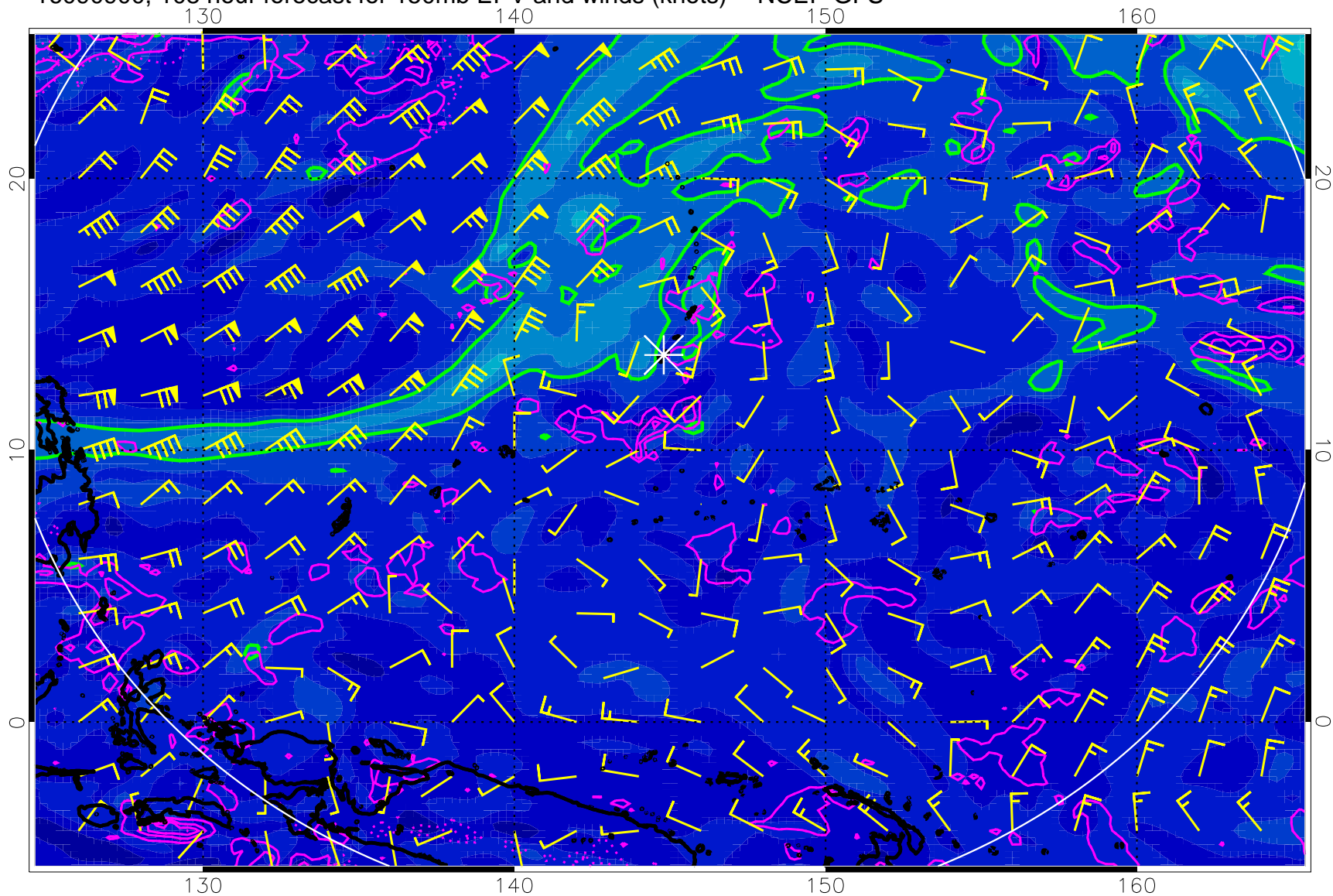
16090900, 108 hour forecast for 150mb EPV and winds (knots) -- NCEP GFS
