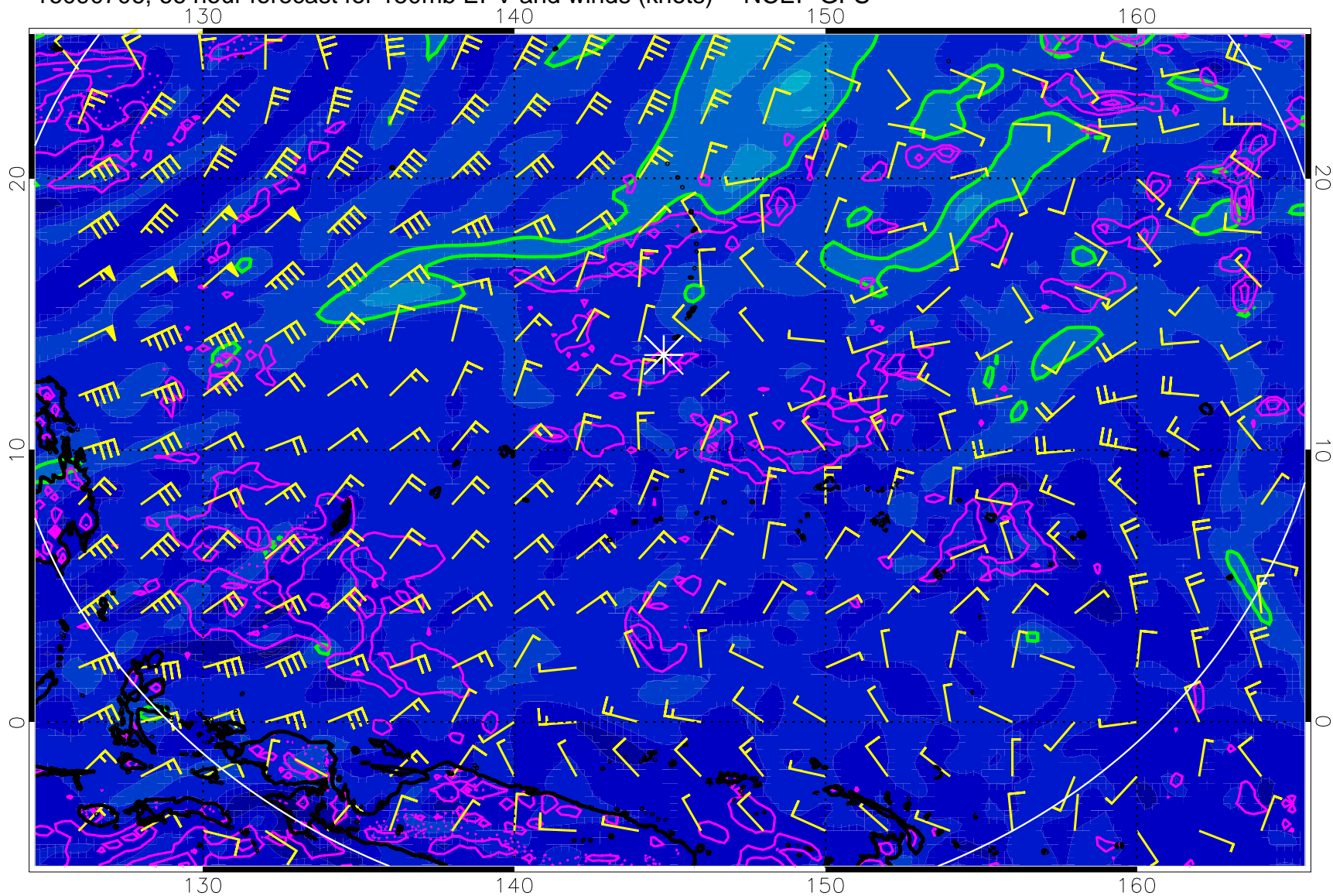
16090706, 66 hour forecast for 150mb EPV and winds (knots) -- NCEP GFS
