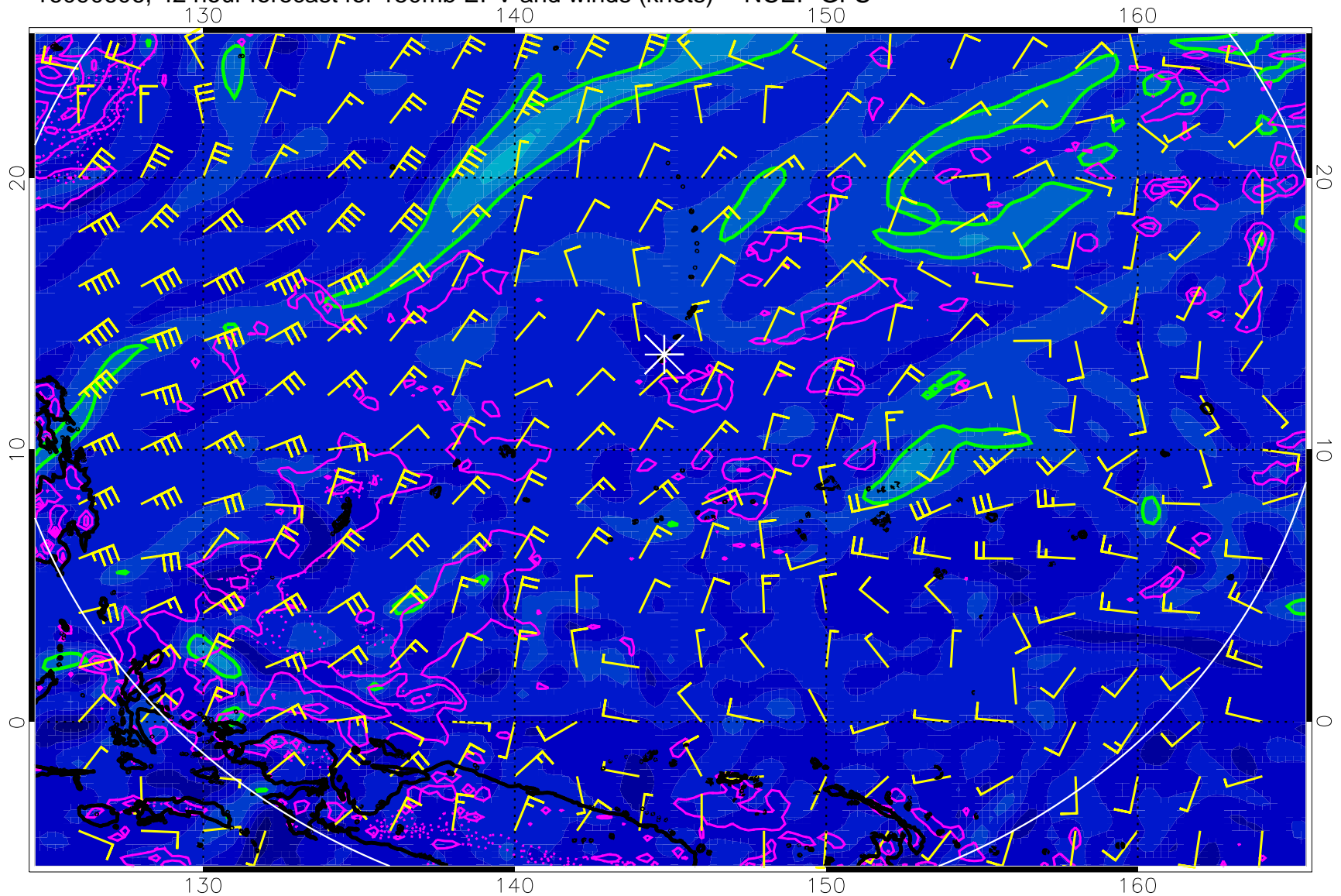
16090606, 42 hour forecast for 150mb EPV and winds (knots) -- NCEP GFS
