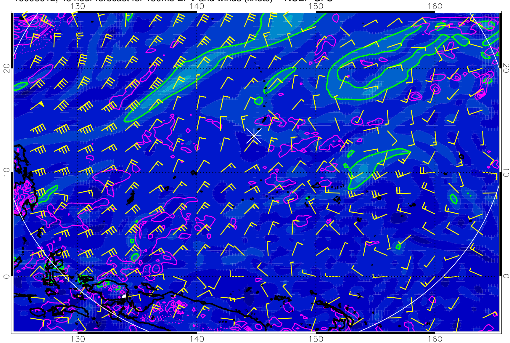
16090612, 48 hour forecast for 150mb EPV and winds (knots) -- NCEP GFS
