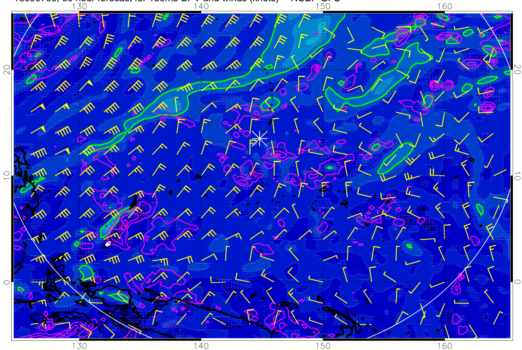
16090700, 60 hour forecast for 150mb EPV and winds (knots) -- NCEP GFS
