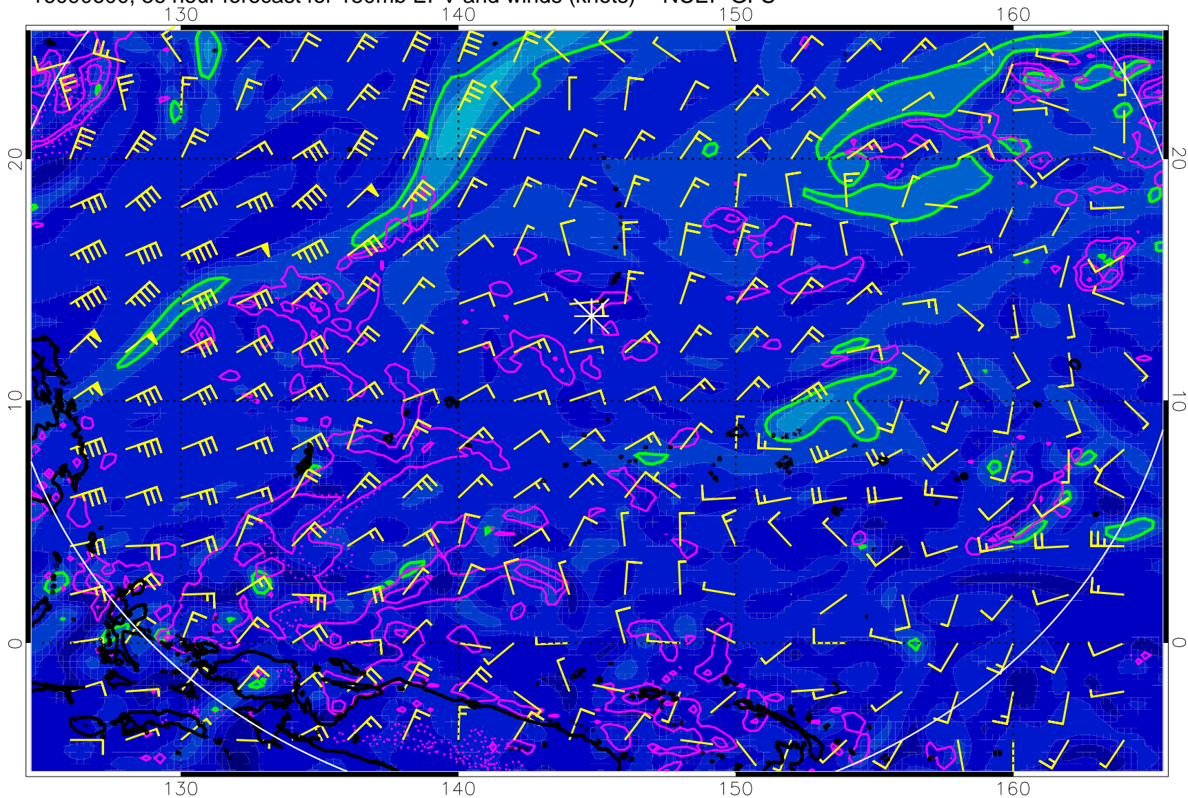
16090600, 36 hour forecast for 150mb EPV and winds (knots) -- NCEP GFS
