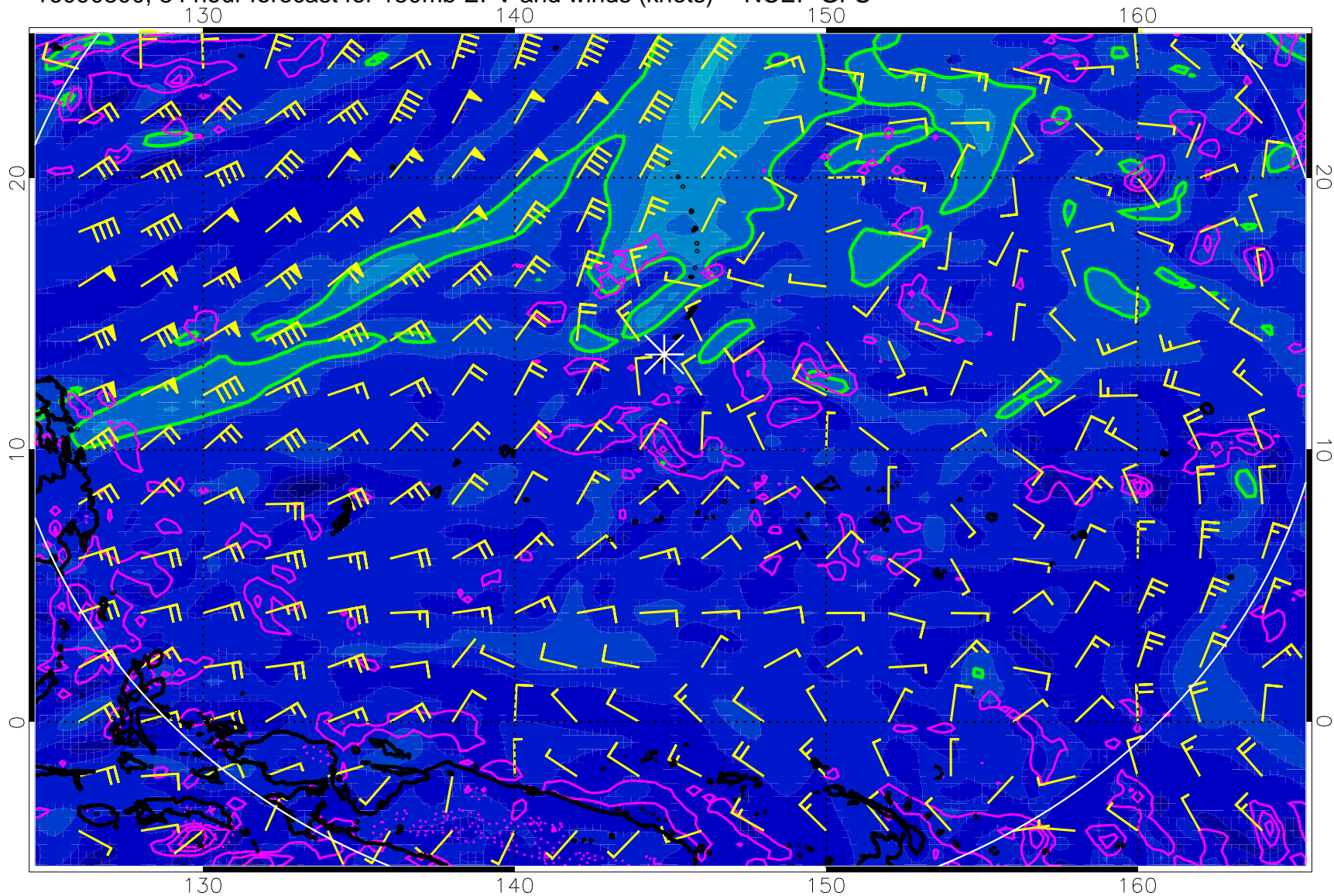
16090800, 84 hour forecast for 150mb EPV and winds (knots) -- NCEP GFS
