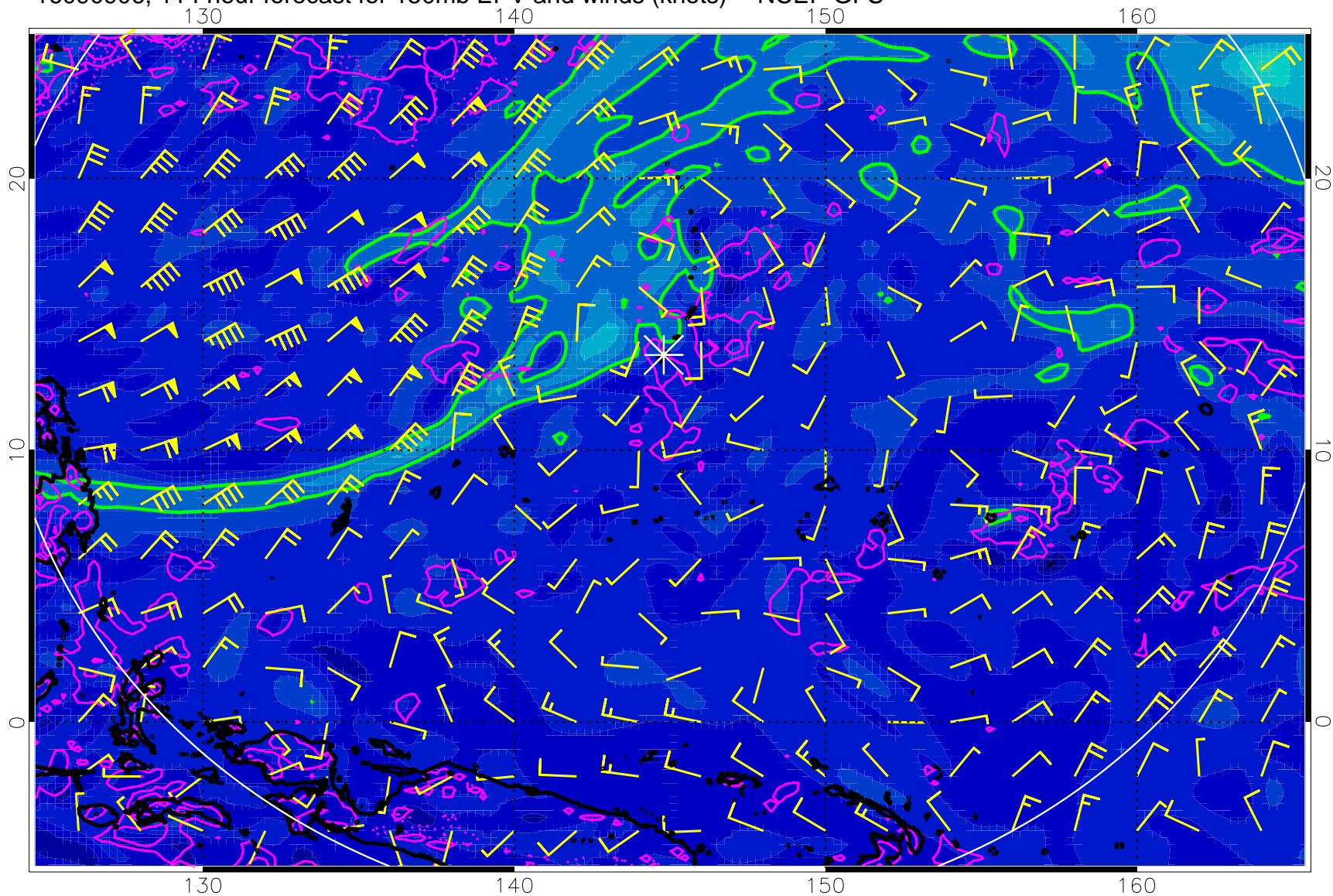
16090906, 114 hour forecast for 150mb EPV and winds (knots) -- NCEP GFS
