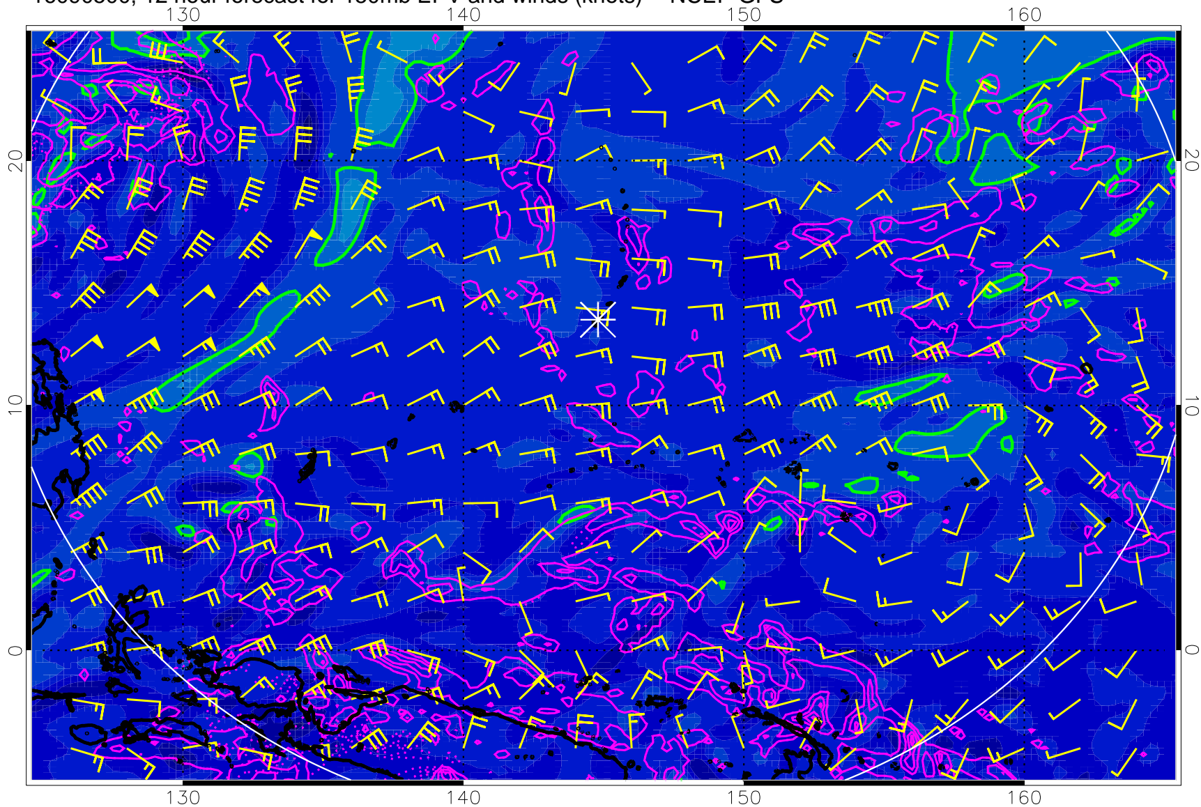
16090500, 12 hour forecast for 150mb EPV and winds (knots) -- NCEP GFS
