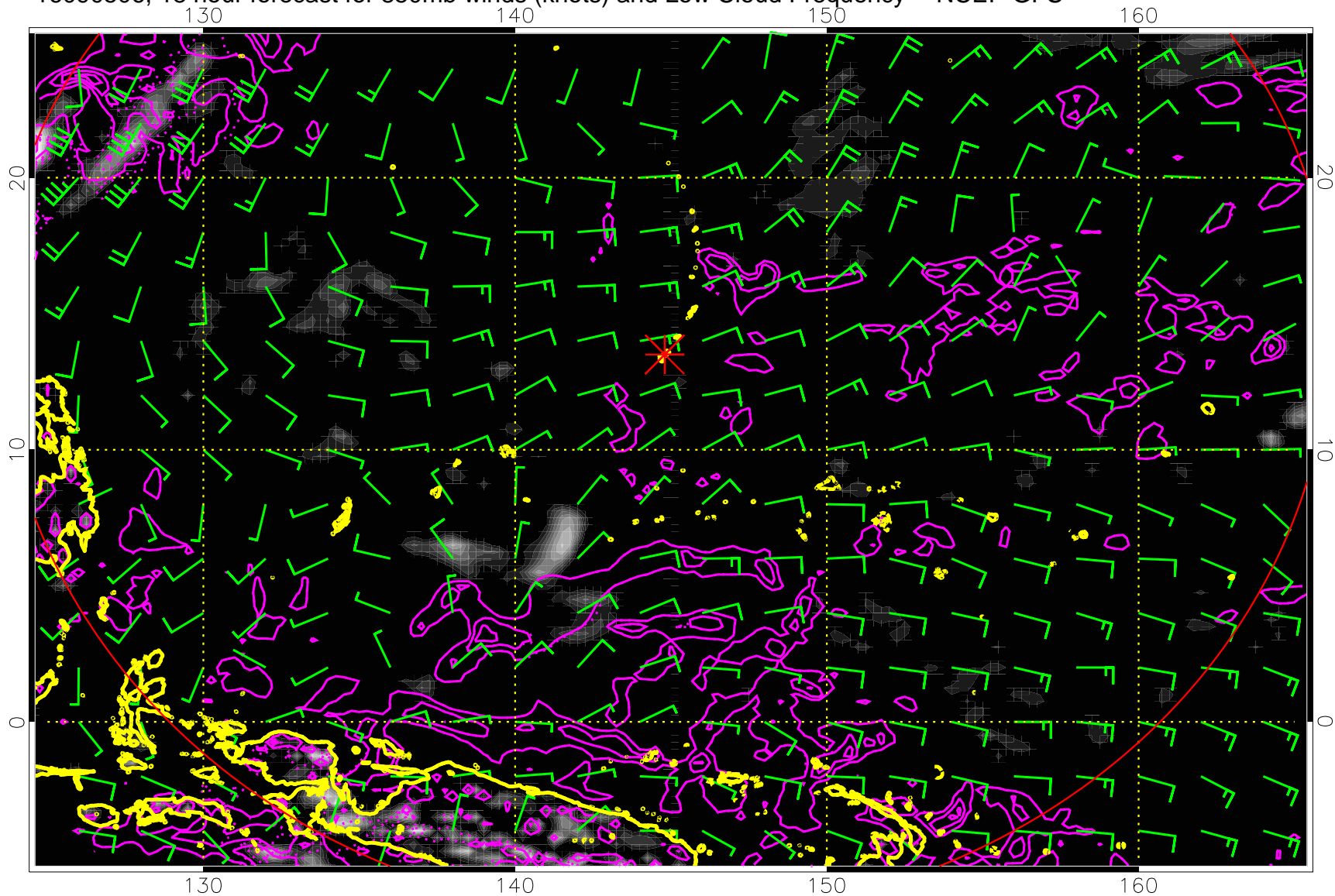
16090506, 18 hour forecast for 850mb winds (knots) and Low Cloud Frequency -- NCEP GFS
