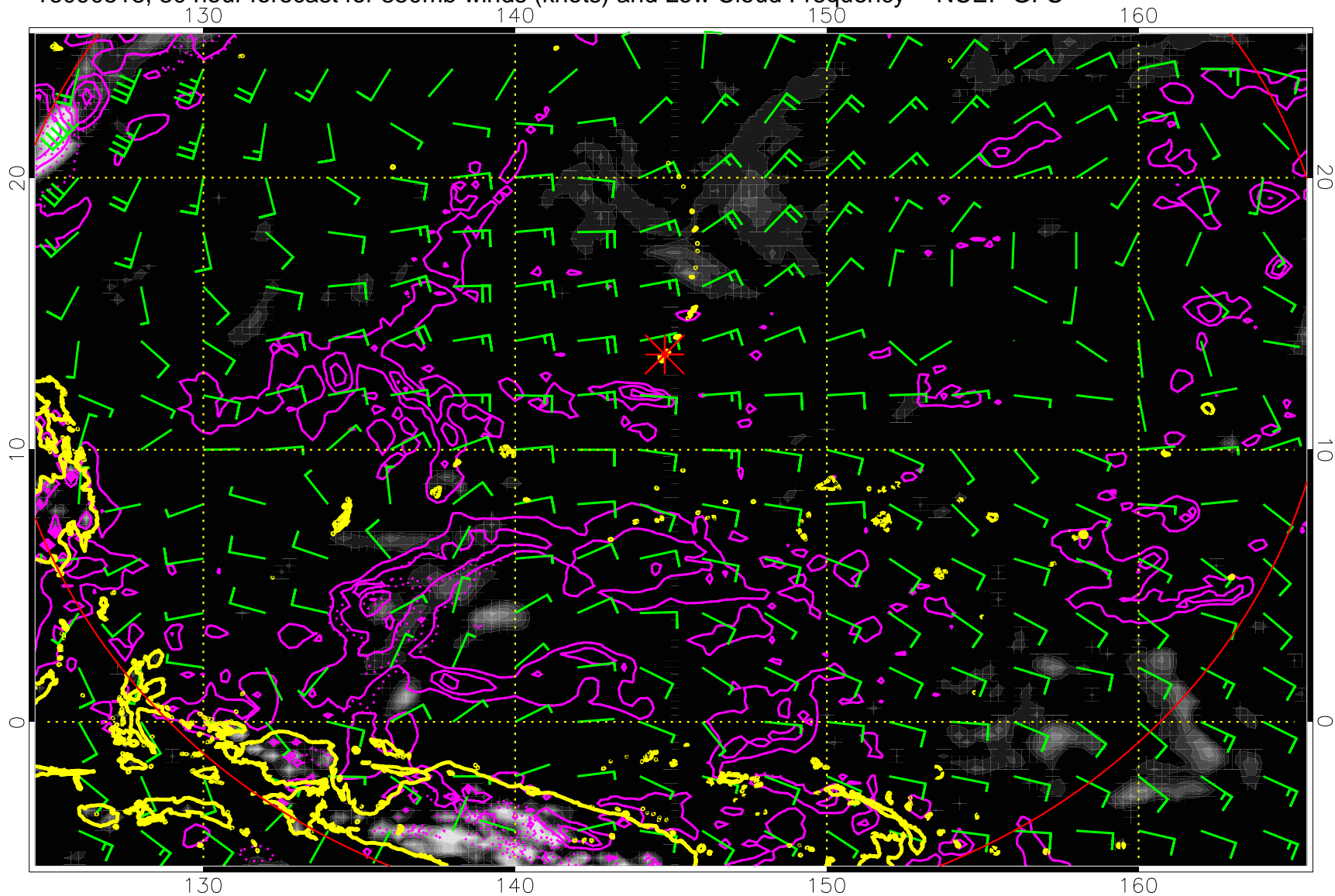
16090518, 30 hour forecast for 850mb winds (knots) and Low Cloud Frequency -- NCEP GFS
