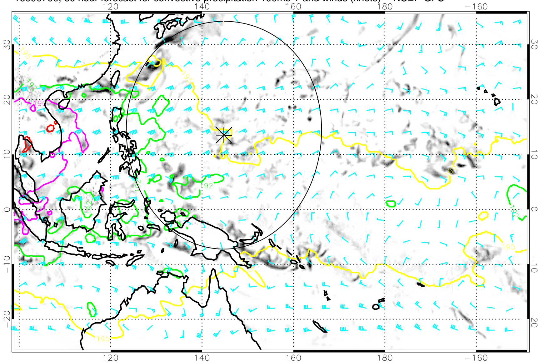
16090700, 60 hour forecast for convective precipitation 100mb T and winds (knots) -- NCEP GFS
