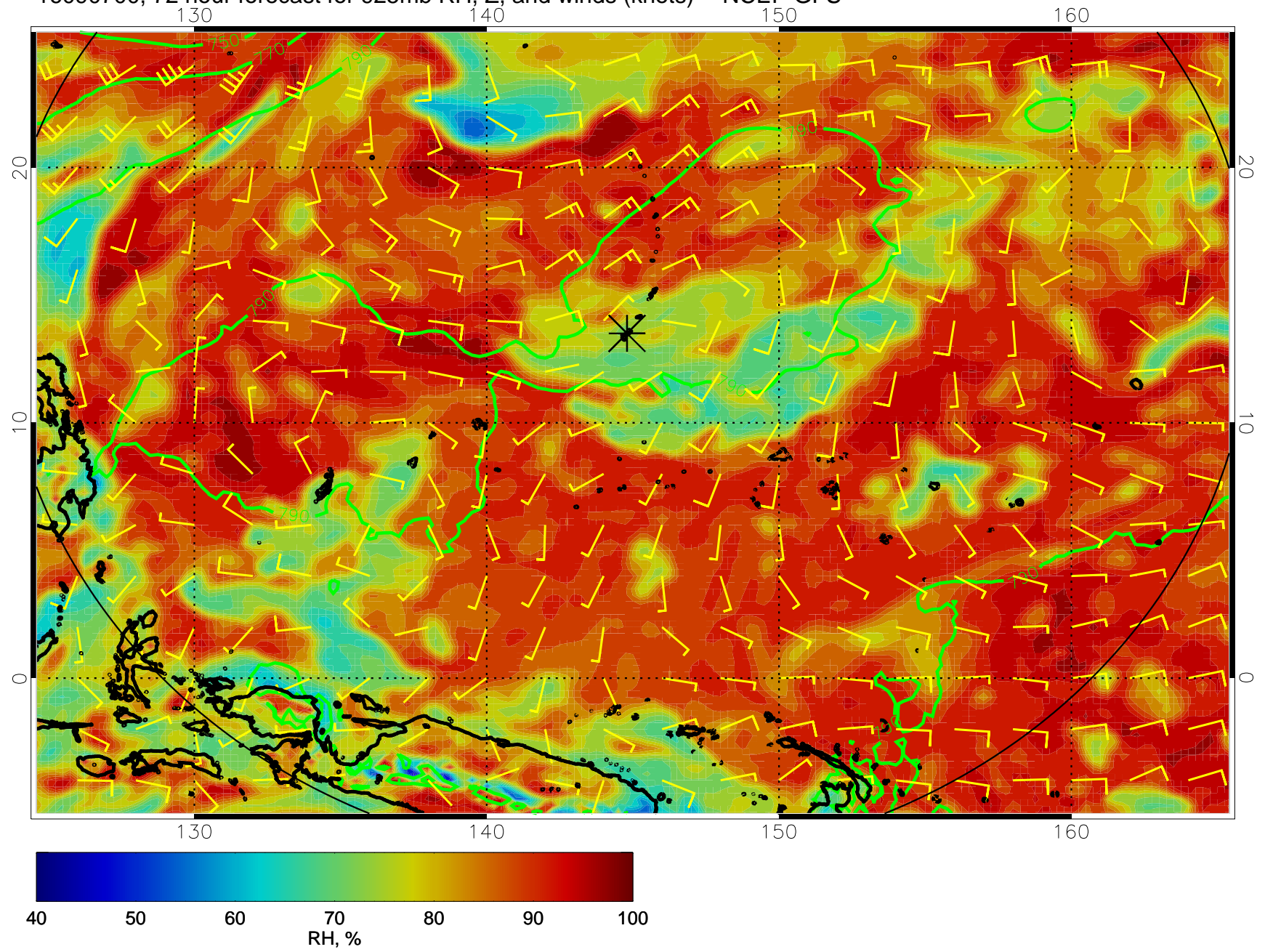
16090700, 72 hour forecast for 925mb RH, Z, and winds (knots) -- NCEP GFS
