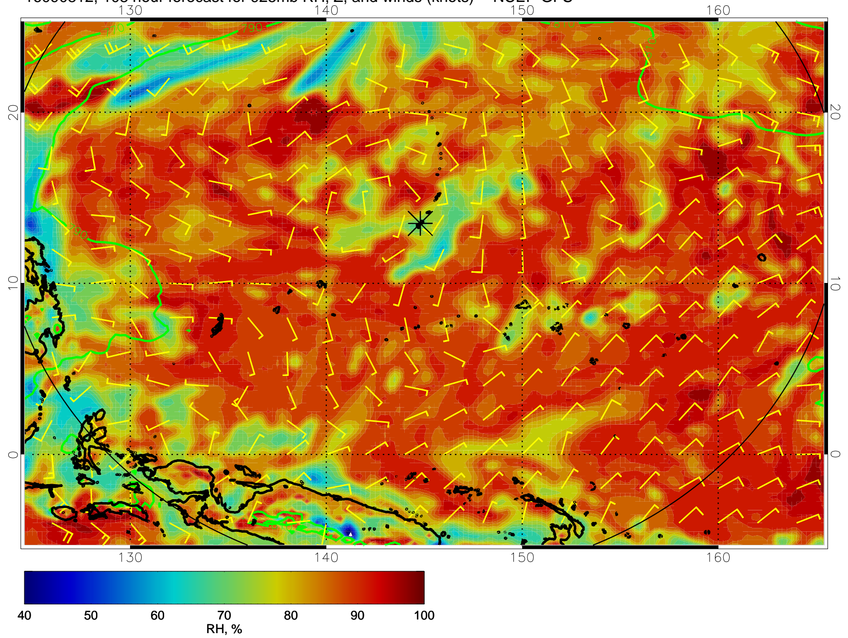
16090812, 108 hour forecast for 925mb RH, Z, and winds (knots) -- NCEP GFS
