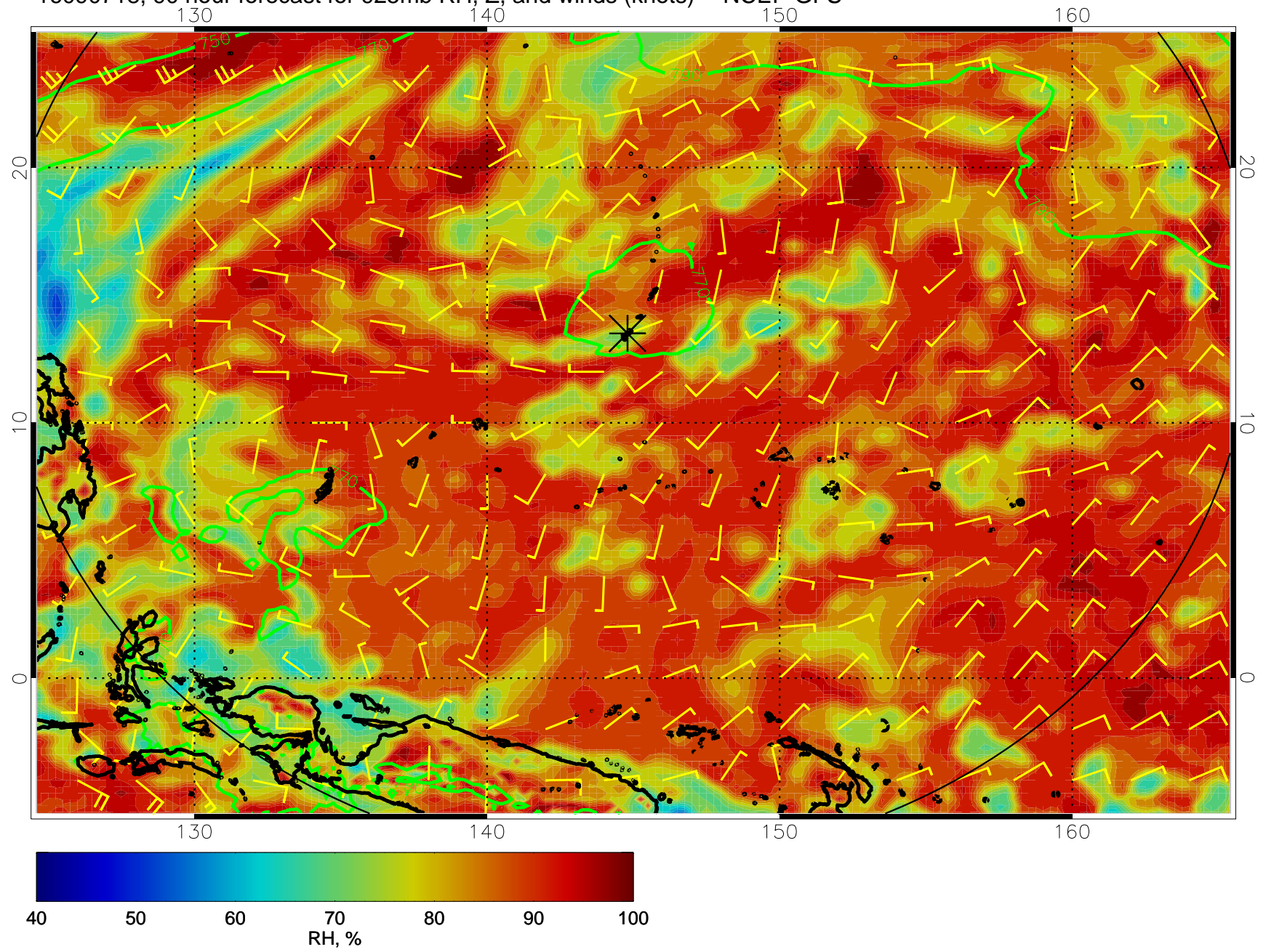
16090718, 90 hour forecast for 925mb RH, Z, and winds (knots) -- NCEP GFS
