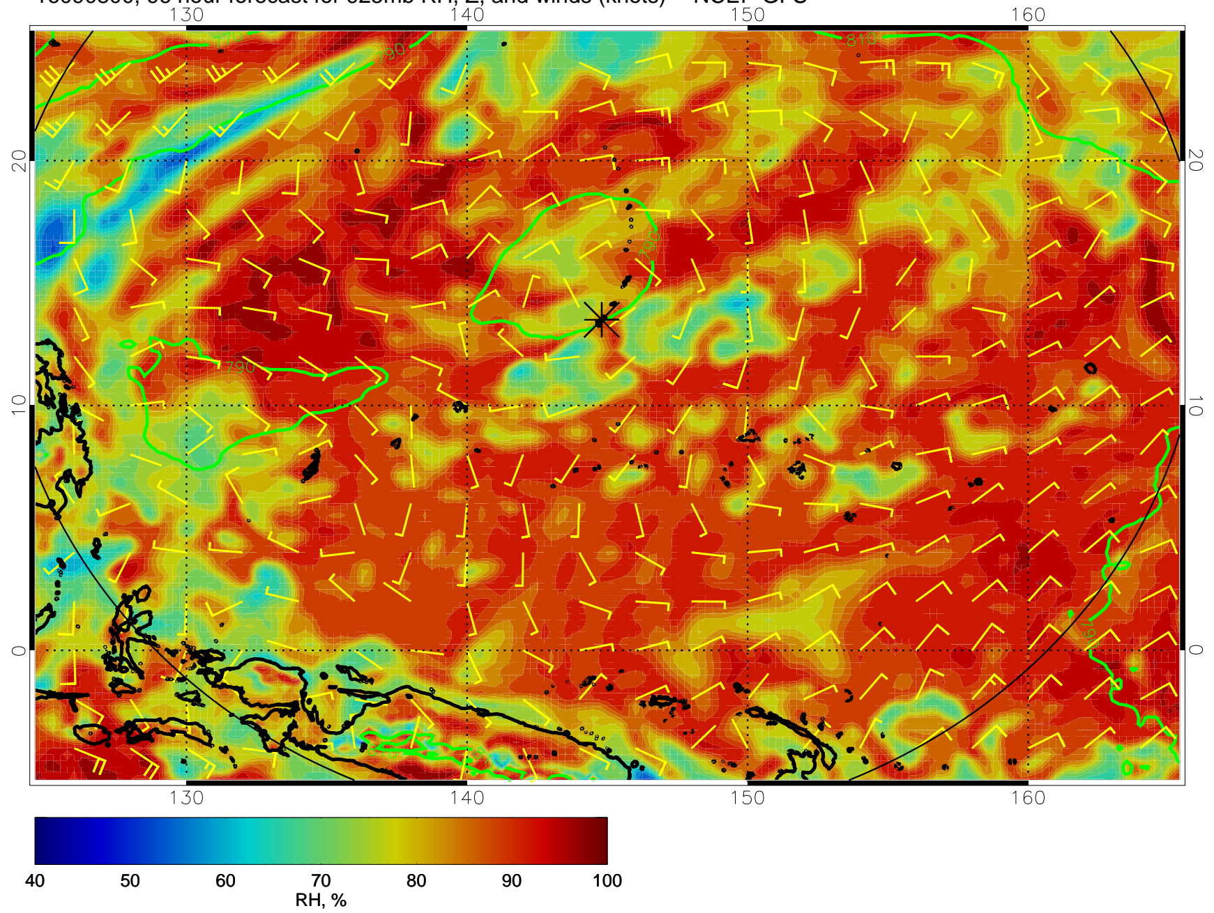
16090800, 96 hour forecast for 925mb RH, Z, and winds (knots) -- NCEP GFS
