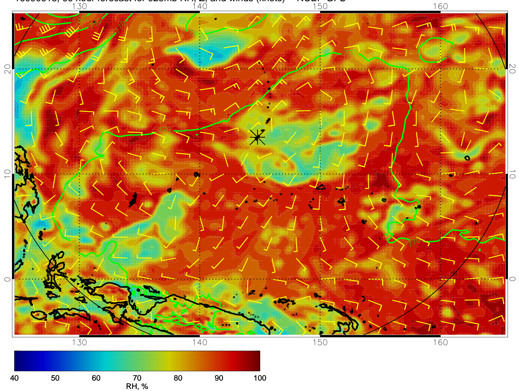
16090618, 66 hour forecast for 925mb RH, Z, and winds (knots) -- NCEP GFS
