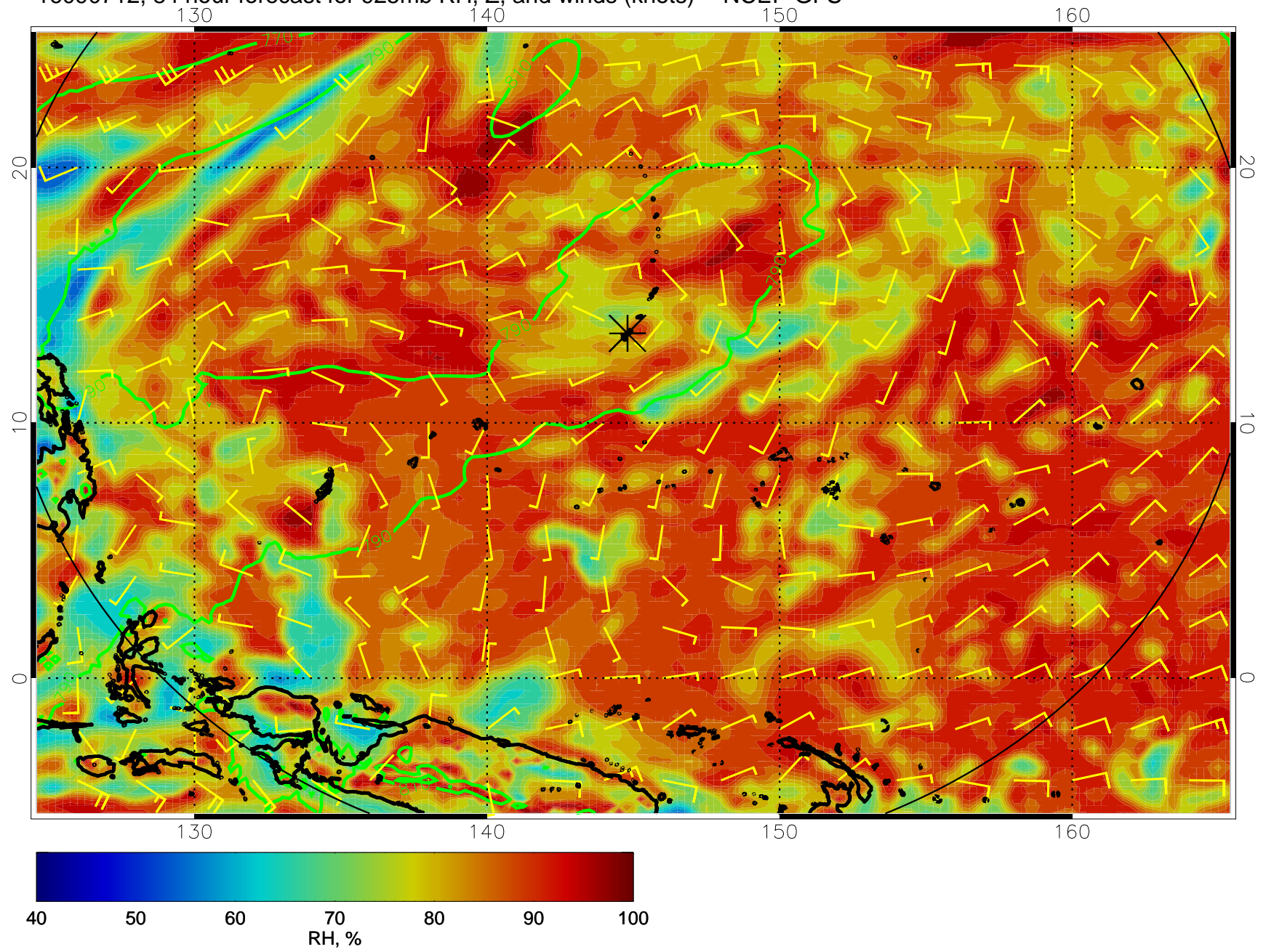
16090712, 84 hour forecast for 925mb RH, Z, and winds (knots) -- NCEP GFS
