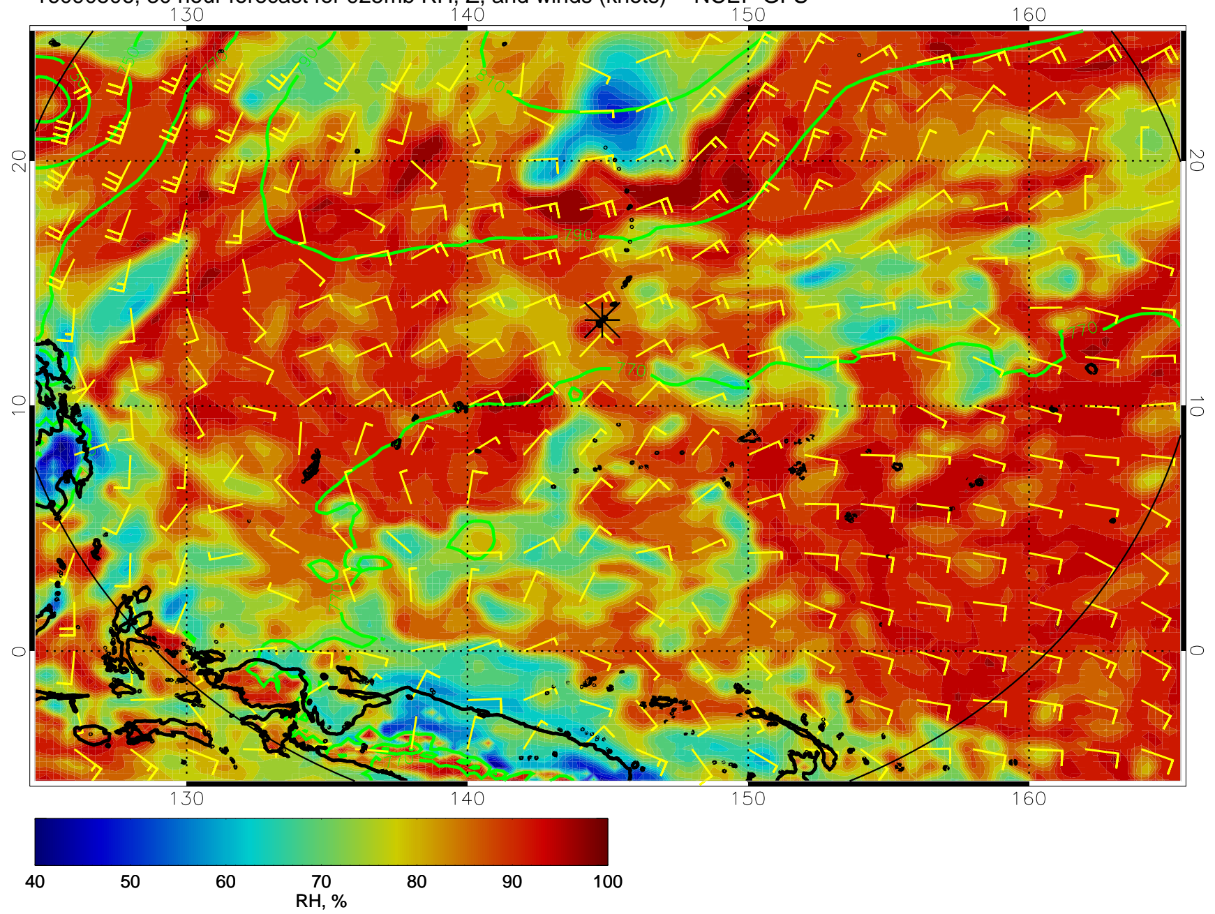
16090506, 30 hour forecast for 925mb RH, Z, and winds (knots) -- NCEP GFS
