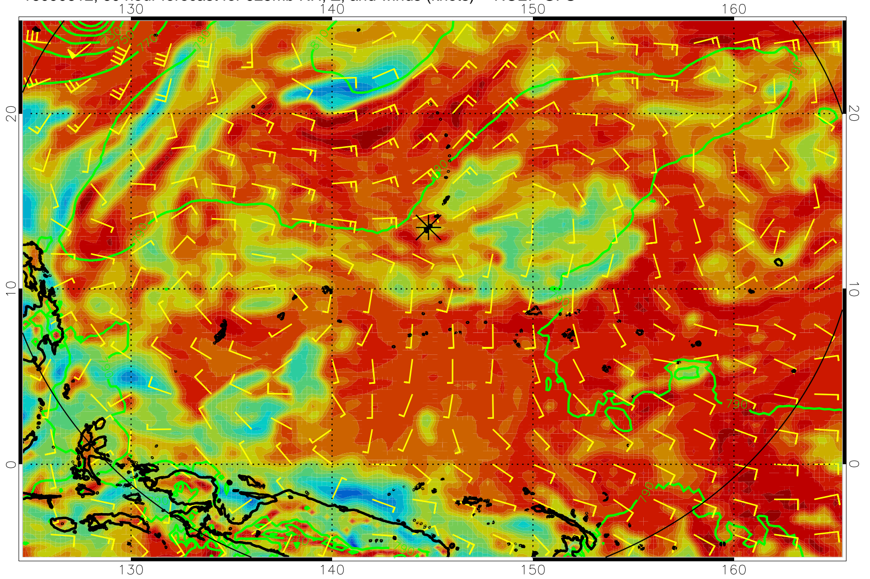
16090612, 60 hour forecast for 925mb RH, Z, and winds (knots) -- NCEP GFS
