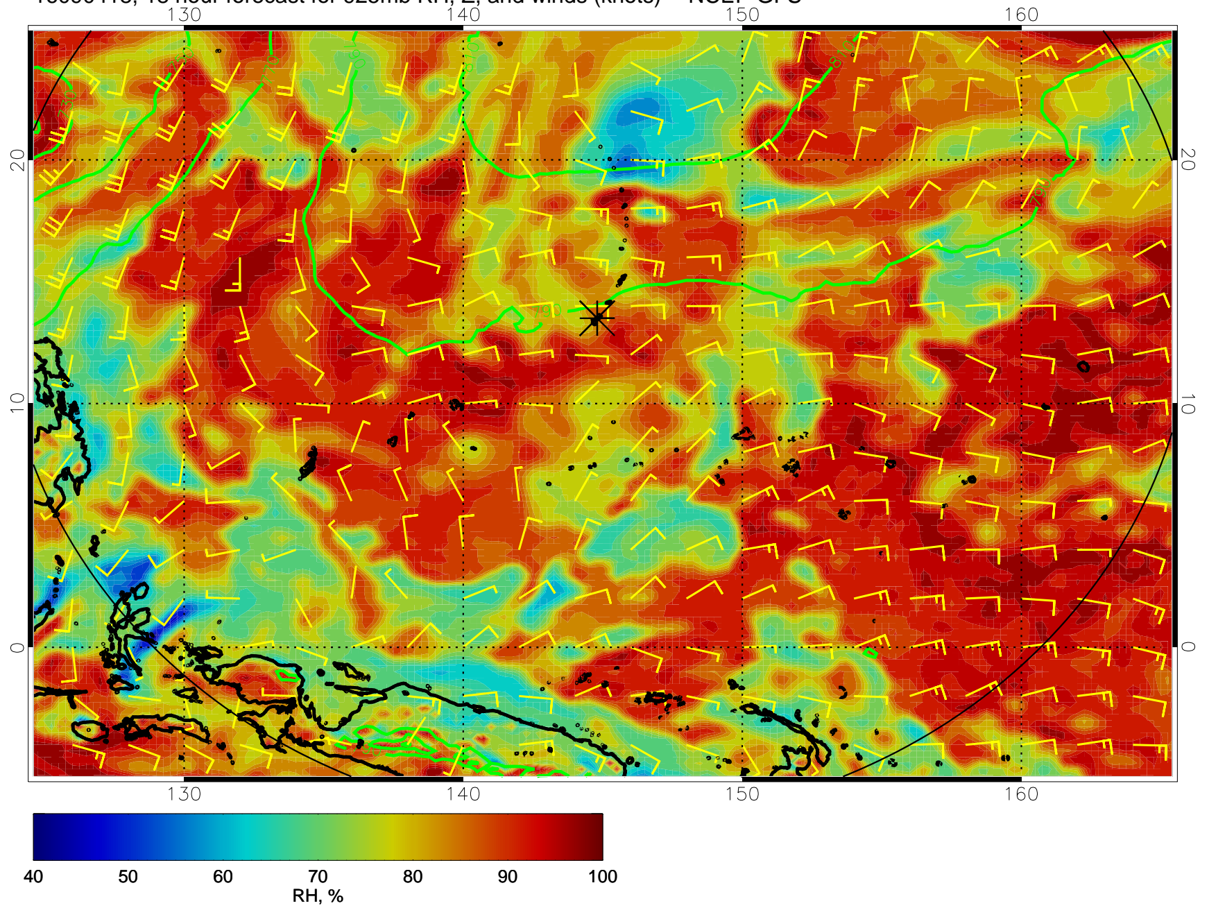
16090418, 18 hour forecast for 925mb RH, Z, and winds (knots) -- NCEP GFS
