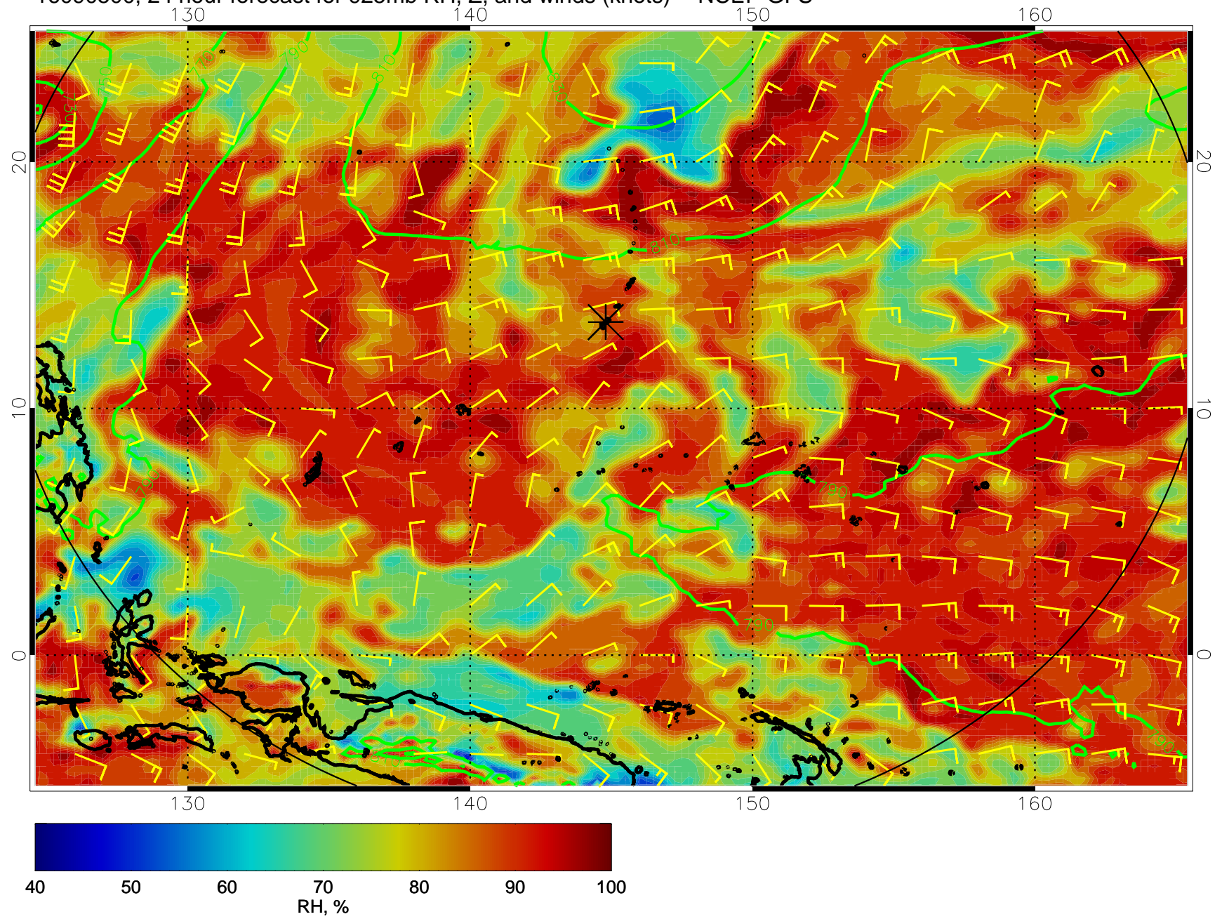
16090500, 24 hour forecast for 925mb RH, Z, and winds (knots) -- NCEP GFS
