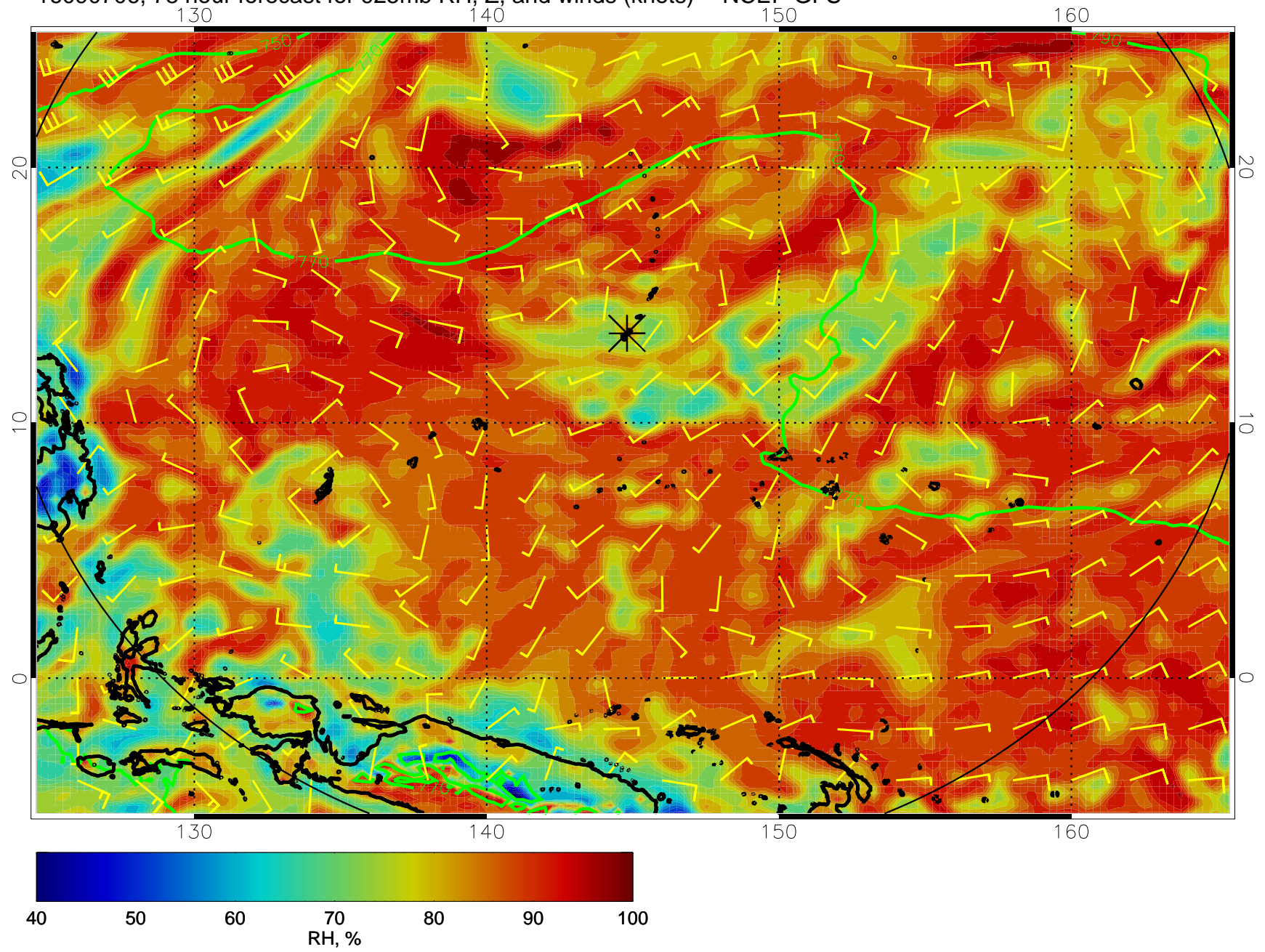
16090706, 78 hour forecast for 925mb RH, Z, and winds (knots) -- NCEP GFS
