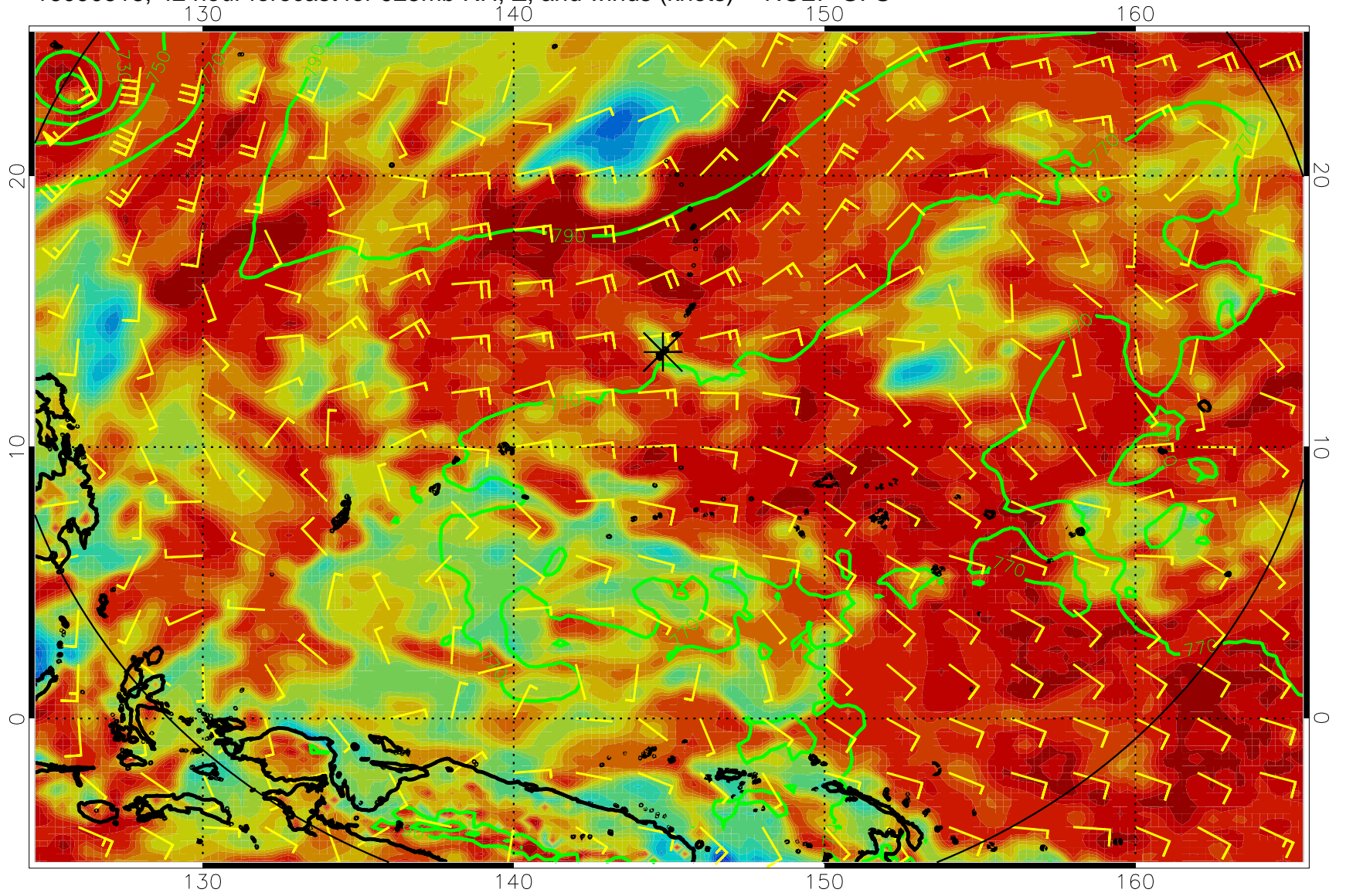
16090518, 42 hour forecast for 925mb RH, Z, and winds (knots) -- NCEP GFS
