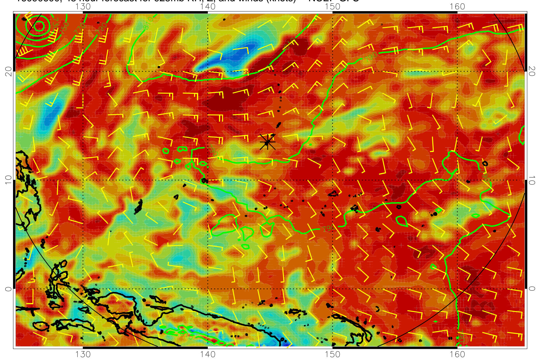
16090600, 48 hour forecast for 925mb RH, Z, and winds (knots) -- NCEP GFS
