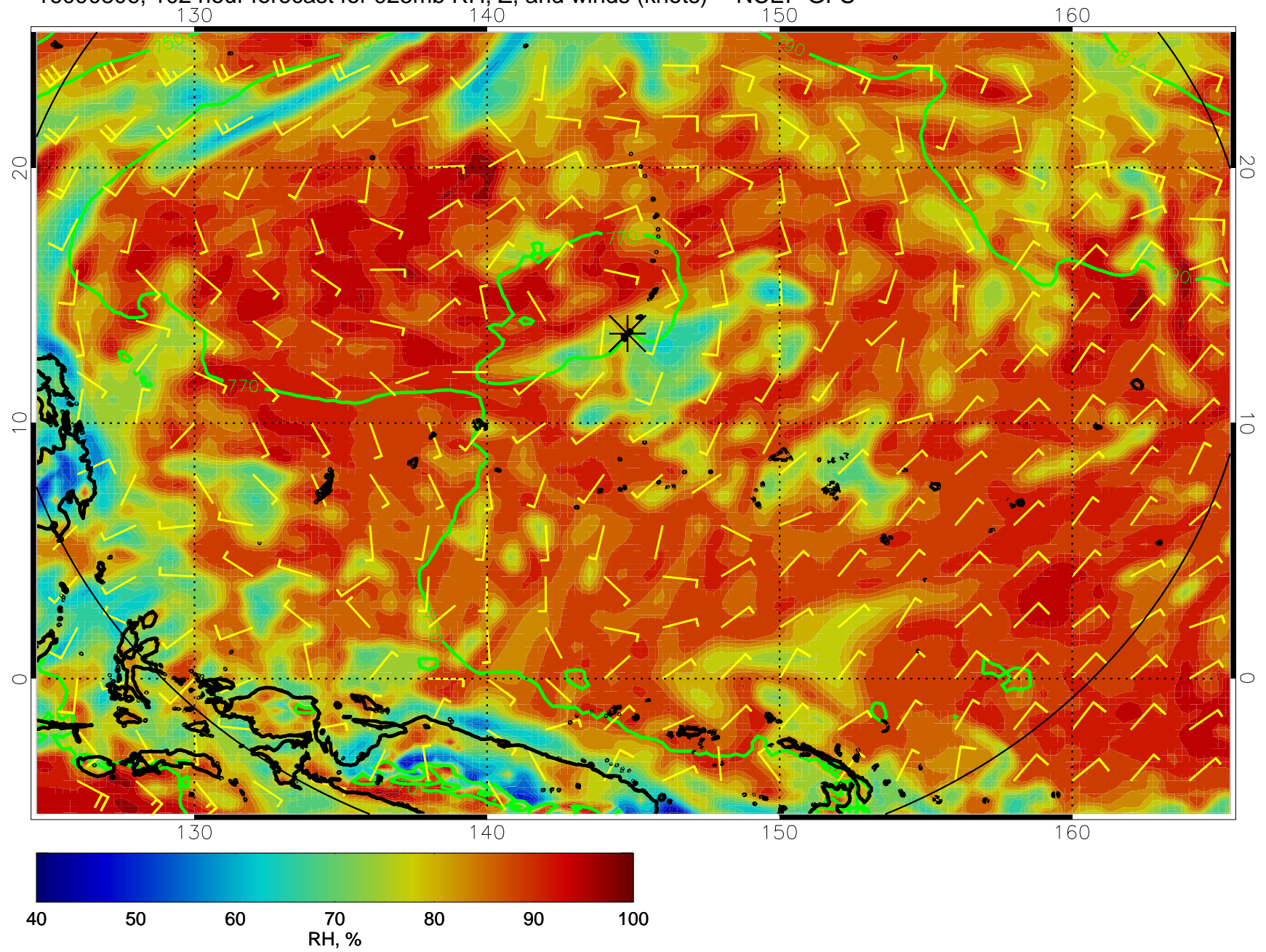
16090806, 102 hour forecast for 925mb RH, Z, and winds (knots) -- NCEP GFS
