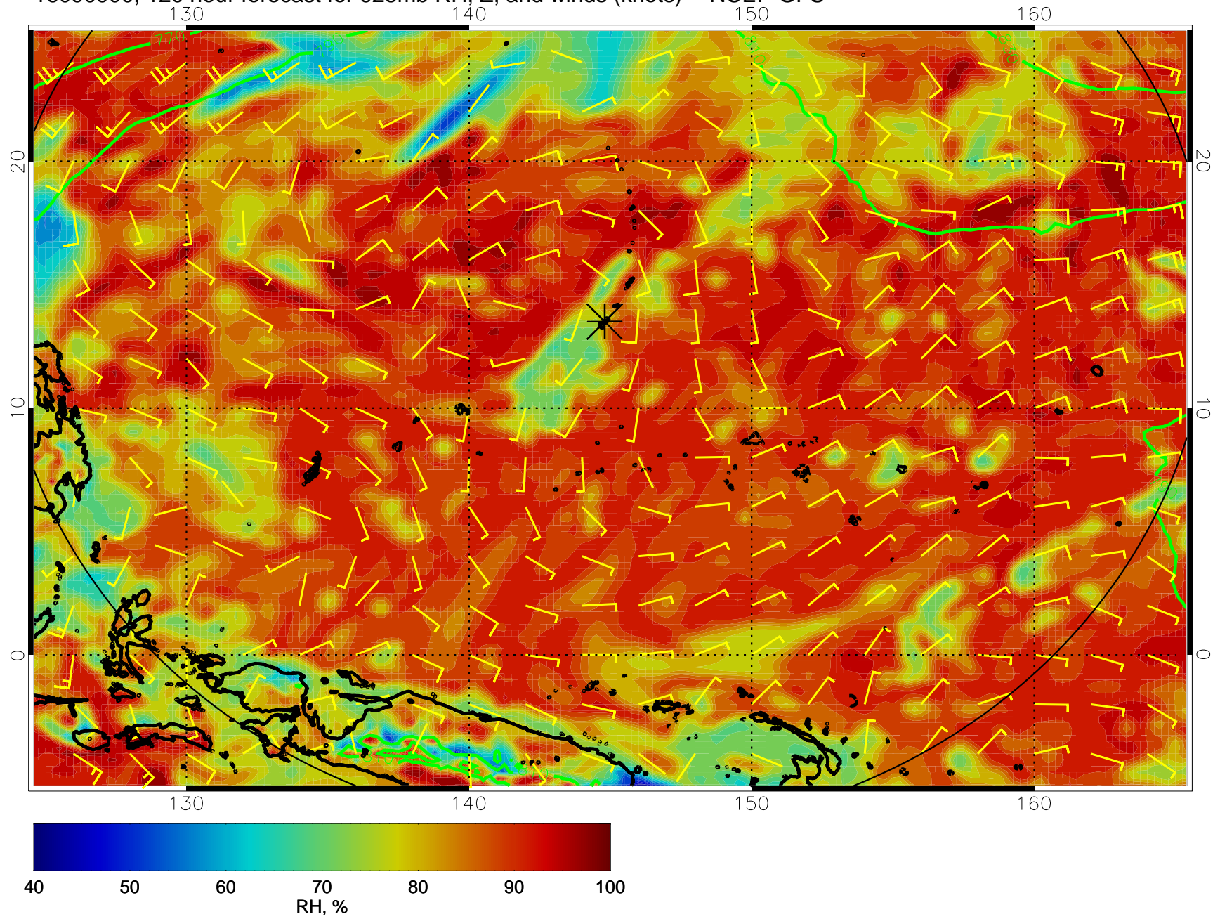
16090900, 120 hour forecast for 925mb RH, Z, and winds (knots) -- NCEP GFS
