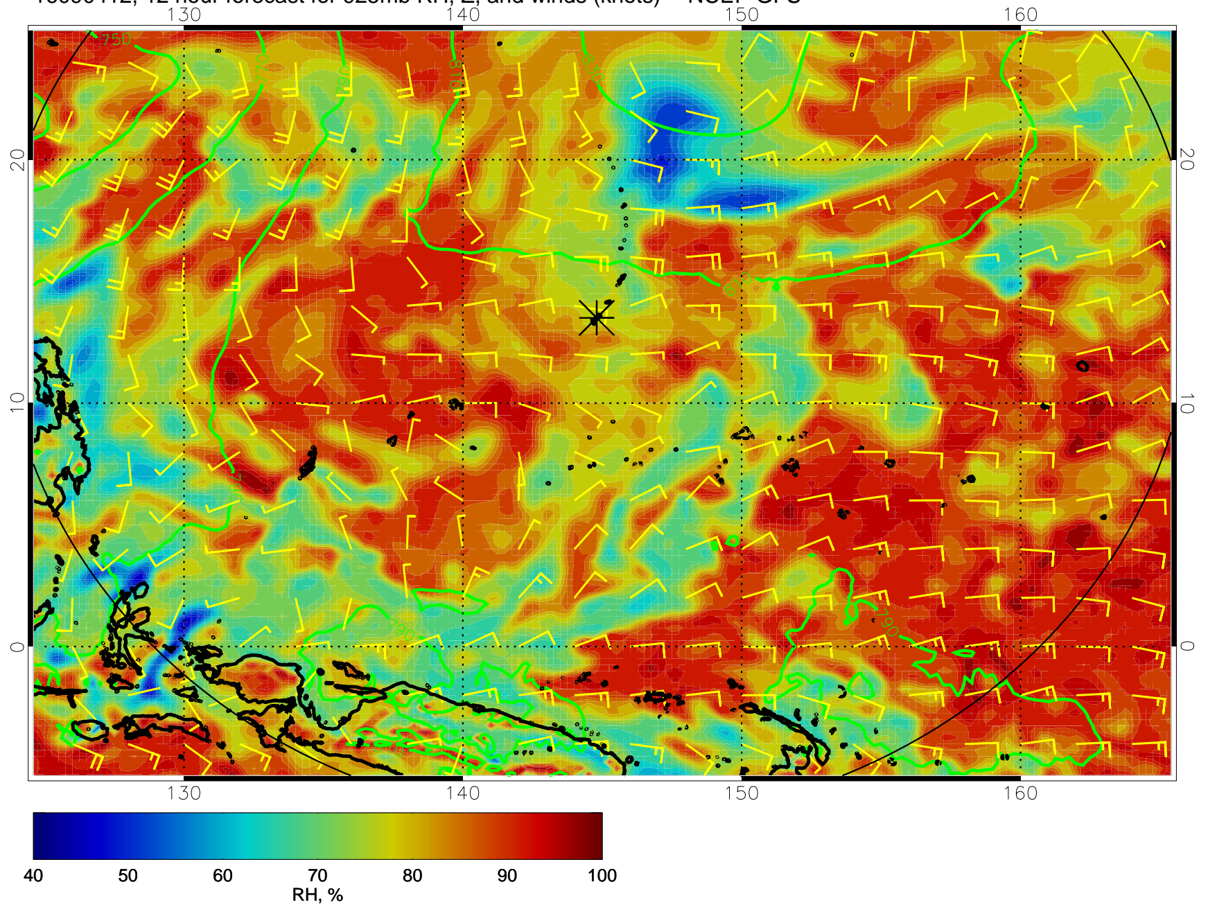
16090412, 12 hour forecast for 925mb RH, Z, and winds (knots) -- NCEP GFS
