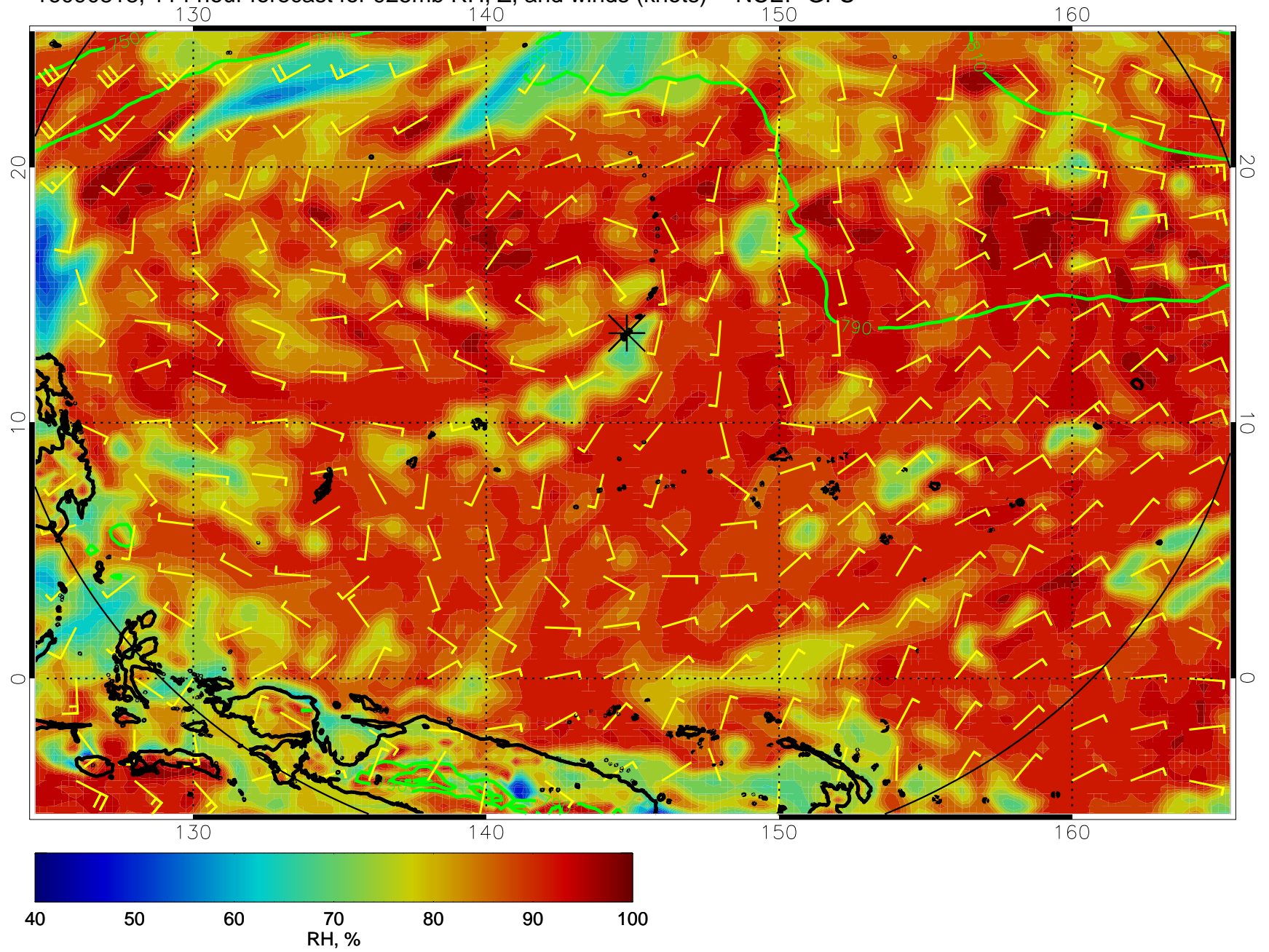
16090818, 114 hour forecast for 925mb RH, Z, and winds (knots) -- NCEP GFS
