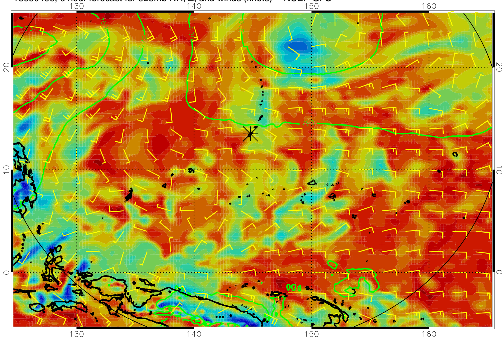
16090406, 6 hour forecast for 925mb RH, Z, and winds (knots) -- NCEP GFS
