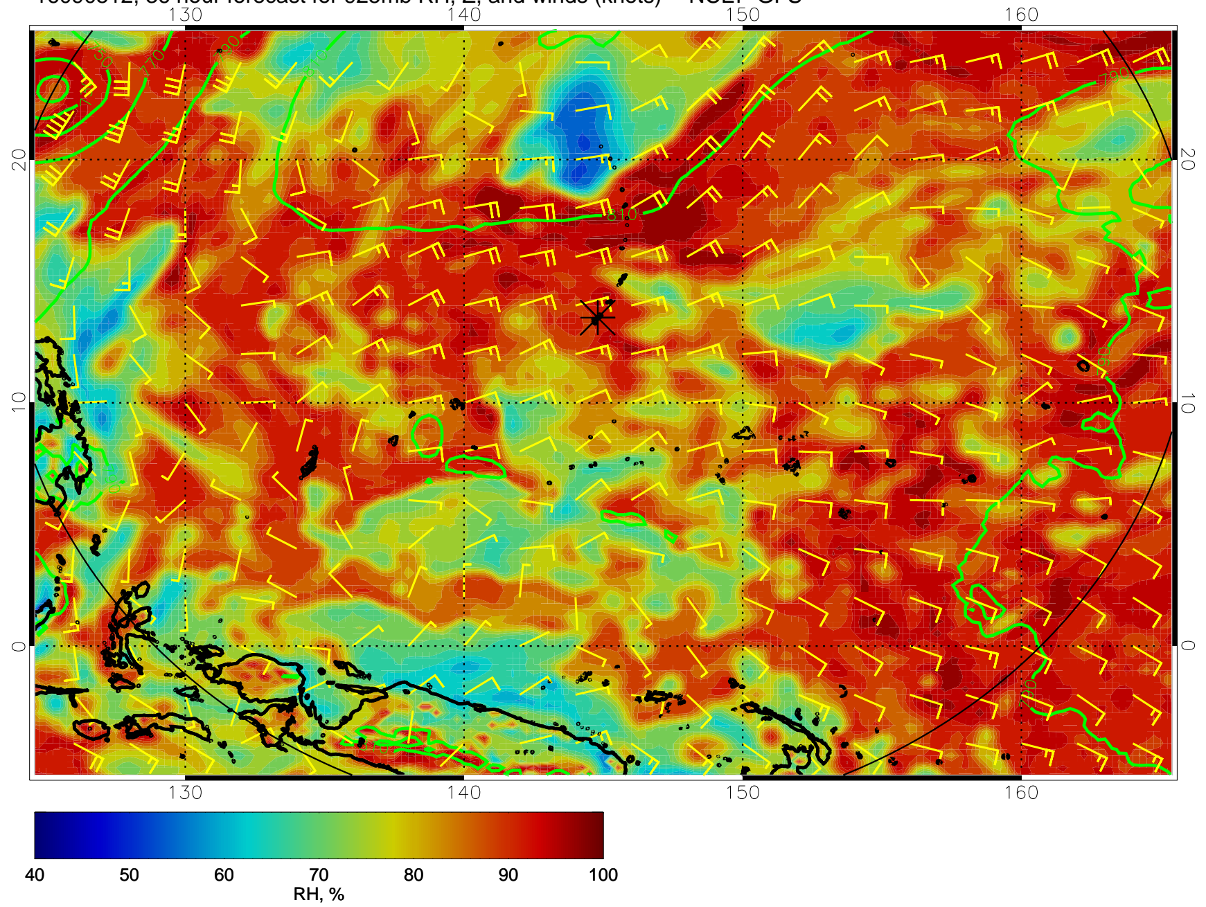
16090512, 36 hour forecast for 925mb RH, Z, and winds (knots) -- NCEP GFS
