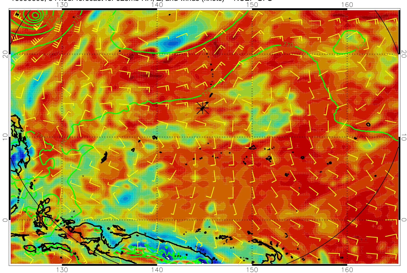
16090606, 54 hour forecast for 925mb RH, Z, and winds (knots) -- NCEP GFS
