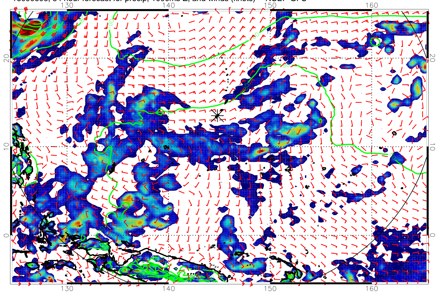
16090606, 54 hour forecast for precip, 1000mb Z, and winds (knots) -- NCEP GFS
