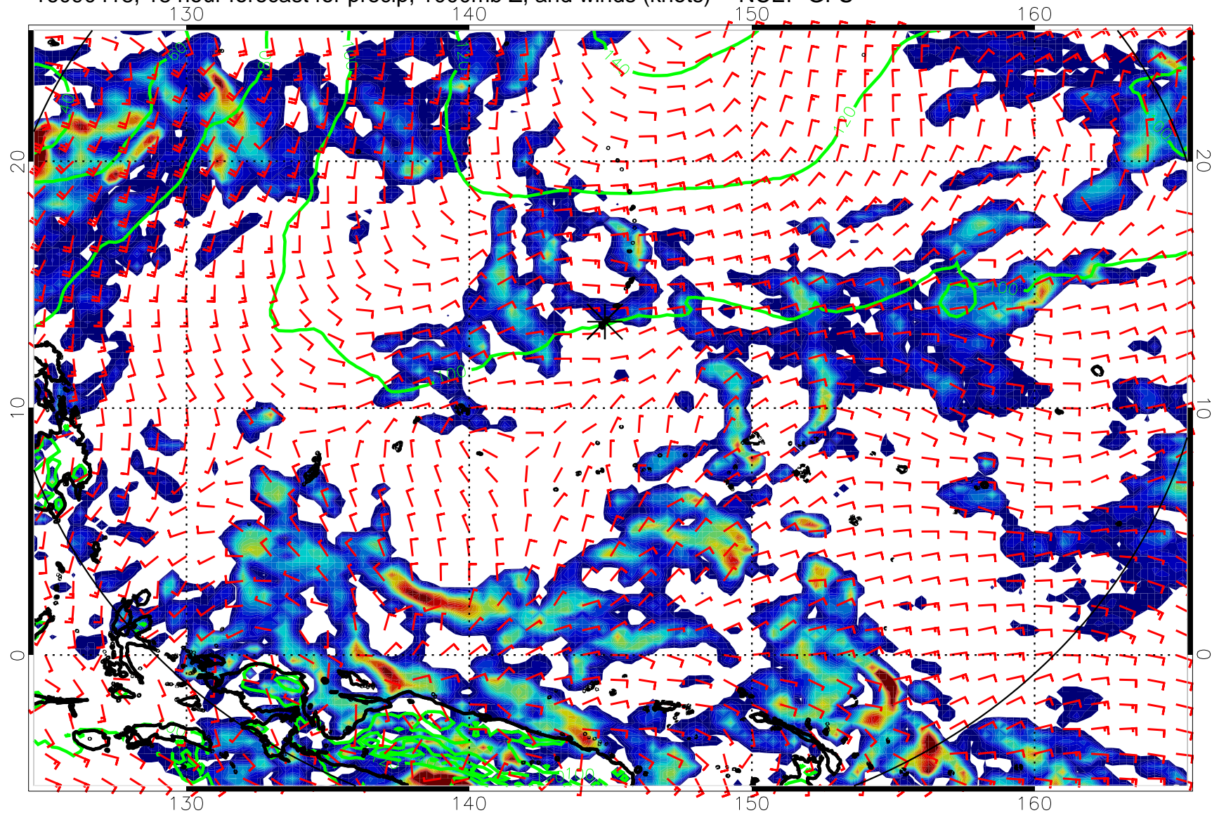
16090418, 18 hour forecast for precip, 1000mb Z, and winds (knots) -- NCEP GFS
