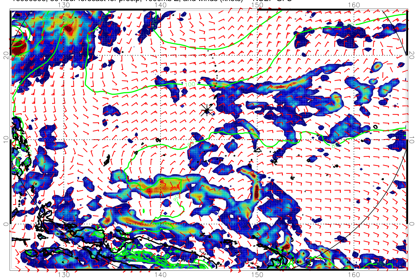
16090506, 30 hour forecast for precip, 1000mb Z, and winds (knots) -- NCEP GFS
