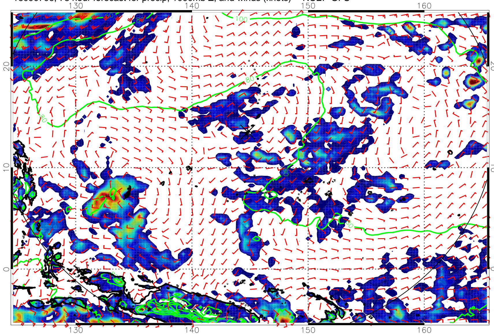
16090706, 78 hour forecast for precip, 1000mb Z, and winds (knots) -- NCEP GFS
