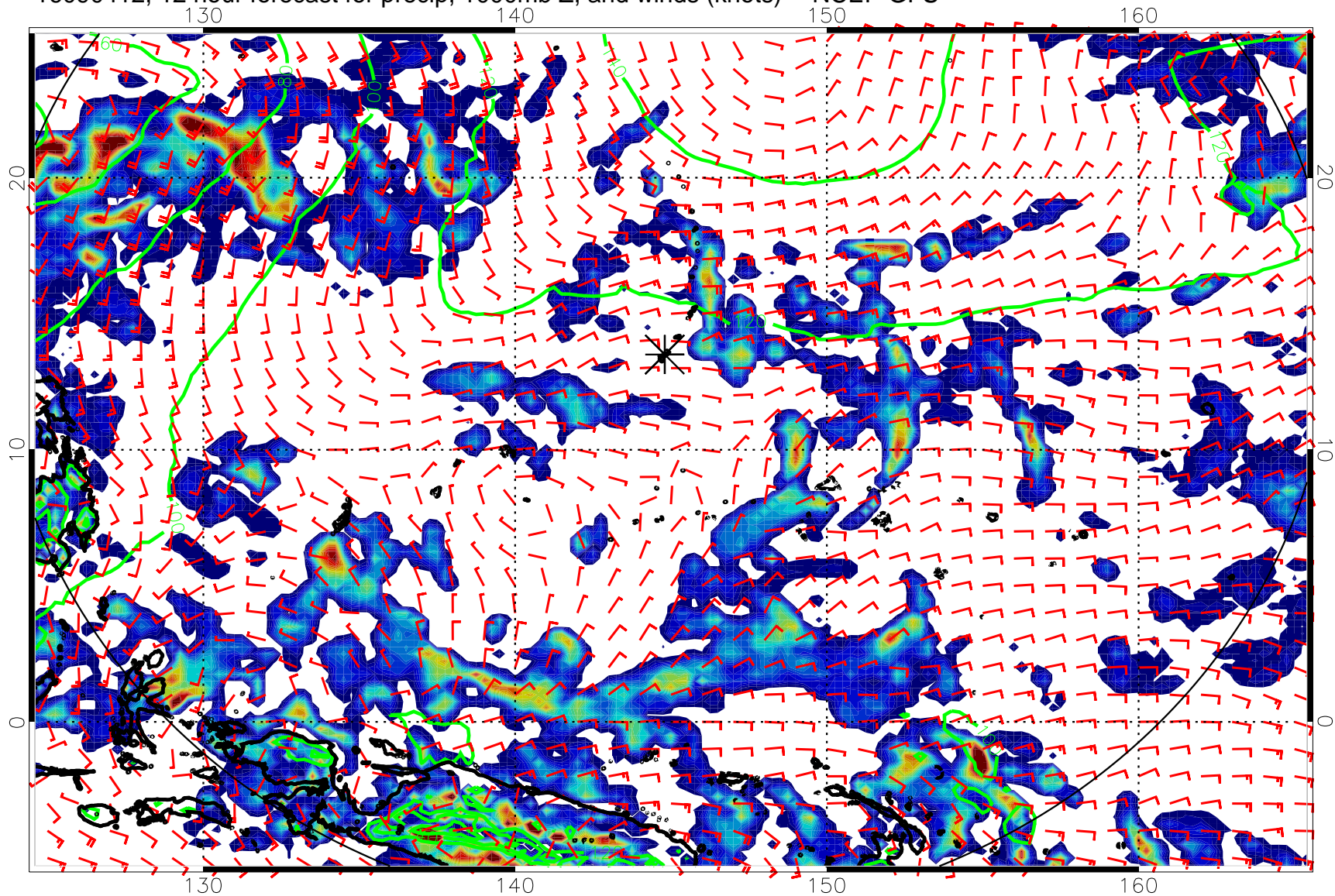
16090412, 12 hour forecast for precip, 1000mb Z, and winds (knots) -- NCEP GFS
