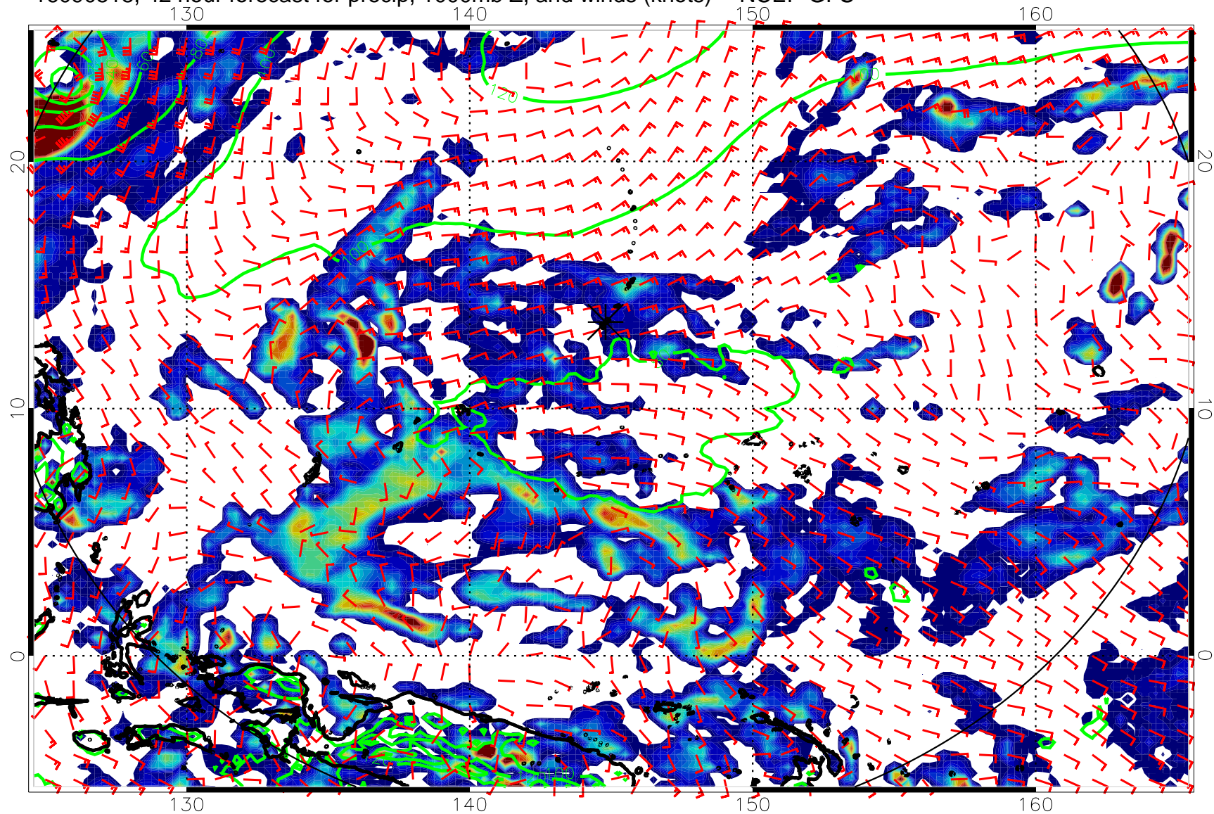
16090518, 42 hour forecast for precip, 1000mb Z, and winds (knots) -- NCEP GFS
