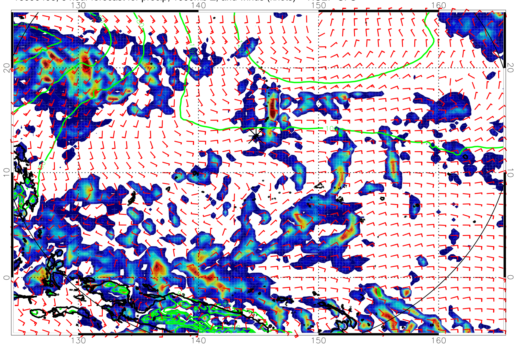
16090406, 6 hour forecast for precip, 1000mb Z, and winds (knots) -- NCEP GFS
