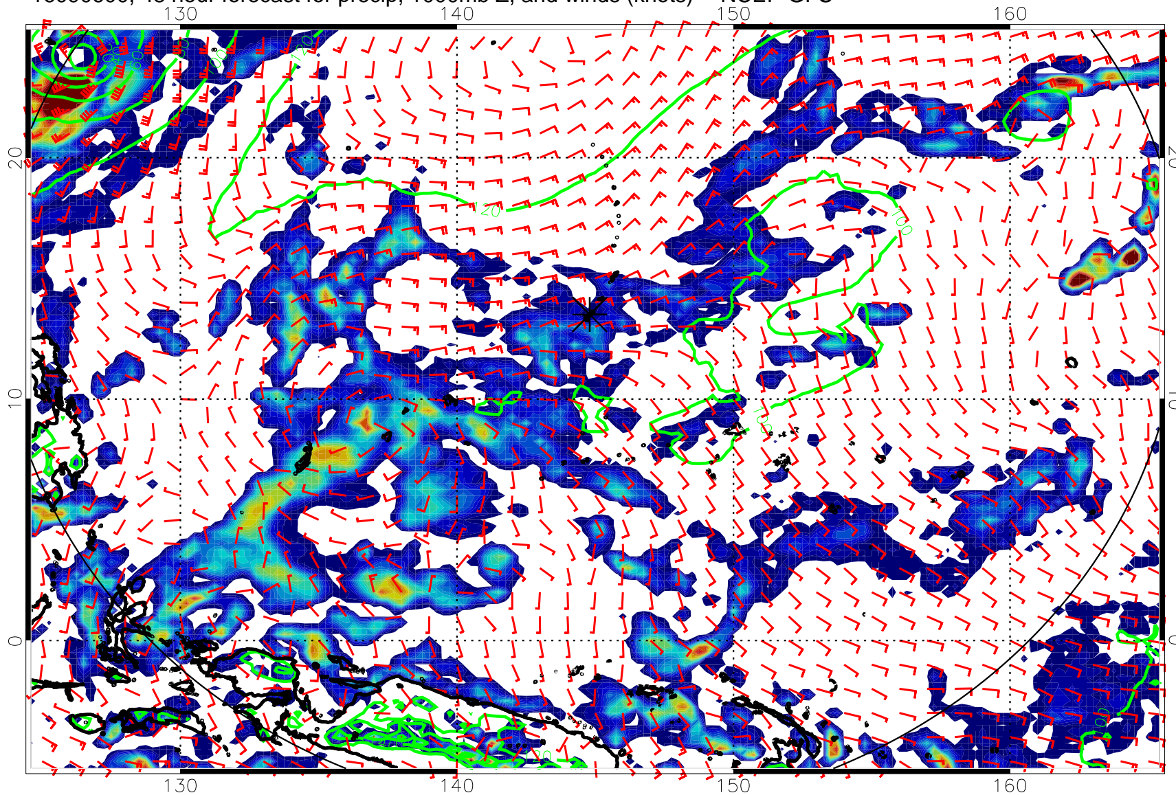
16090600, 48 hour forecast for precip, 1000mb Z, and winds (knots) -- NCEP GFS
