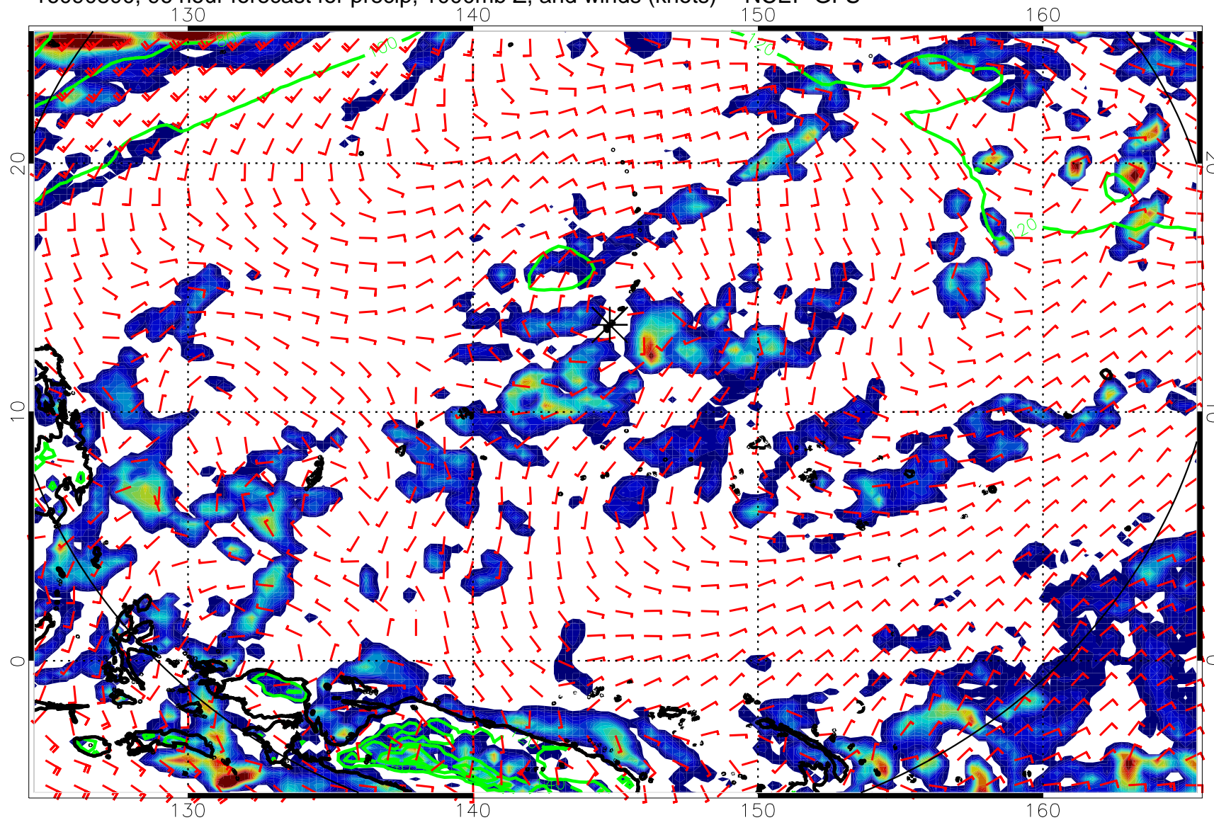
16090800, 96 hour forecast for precip, 1000mb Z, and winds (knots) -- NCEP GFS
