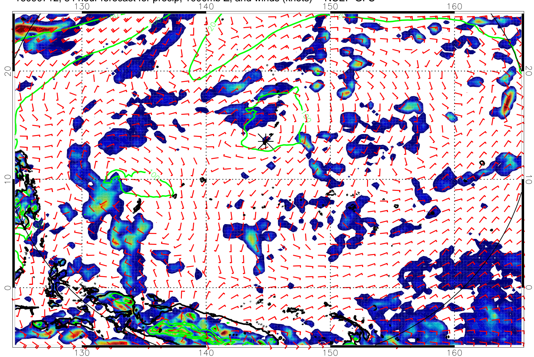
16090712, 84 hour forecast for precip, 1000mb Z, and winds (knots) -- NCEP GFS
