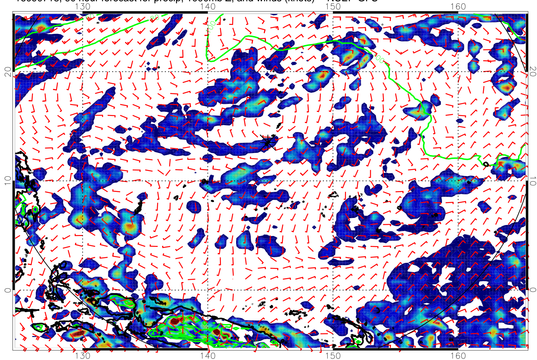
16090718, 90 hour forecast for precip, 1000mb Z, and winds (knots) -- NCEP GFS
