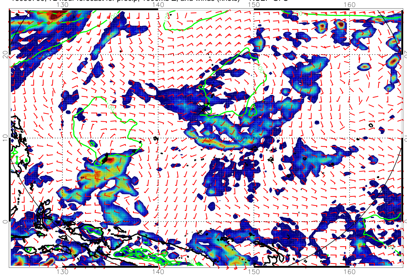
16090700, 72 hour forecast for precip, 1000mb Z, and winds (knots) -- NCEP GFS
