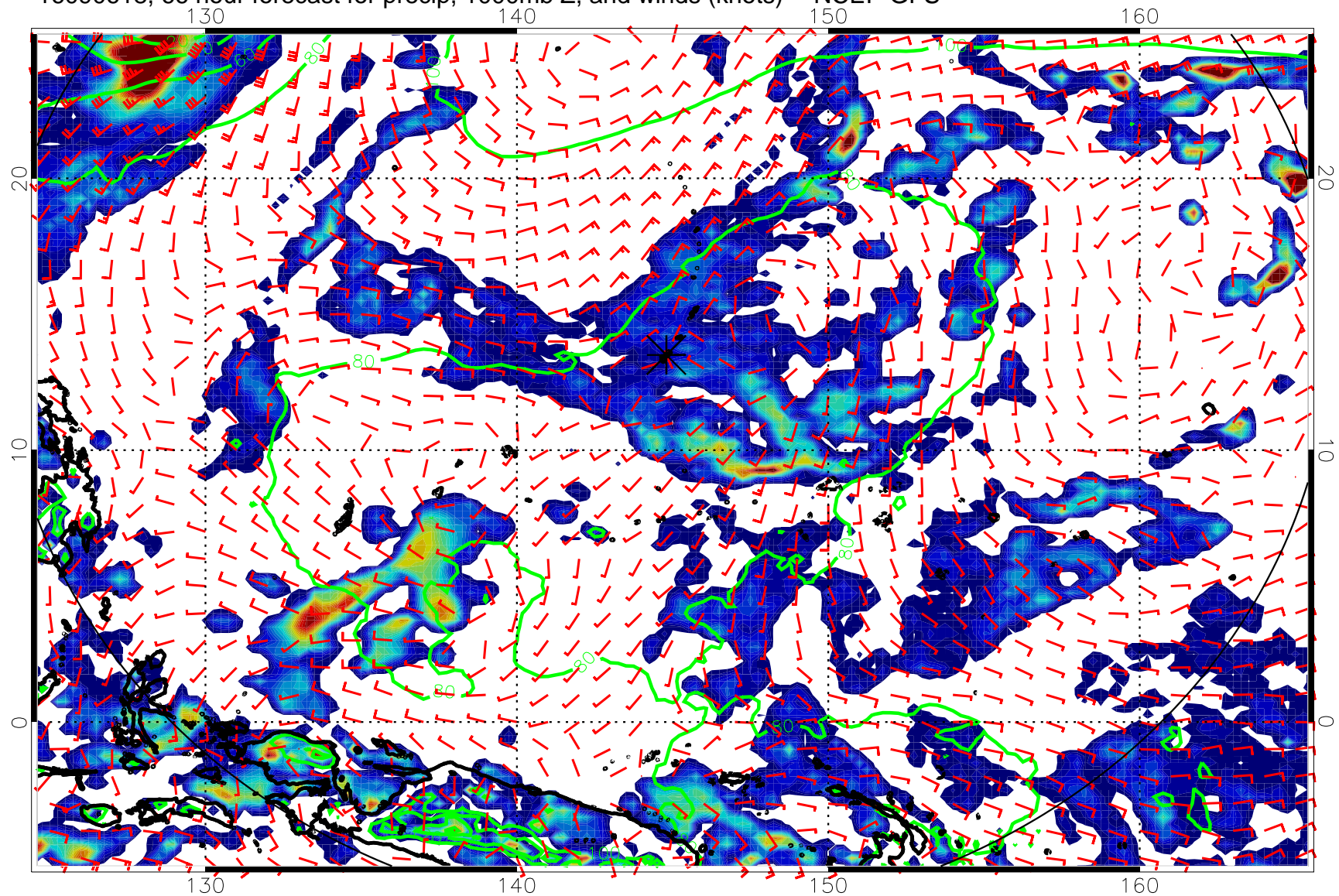
16090618, 66 hour forecast for precip, 1000mb Z, and winds (knots) -- NCEP GFS
