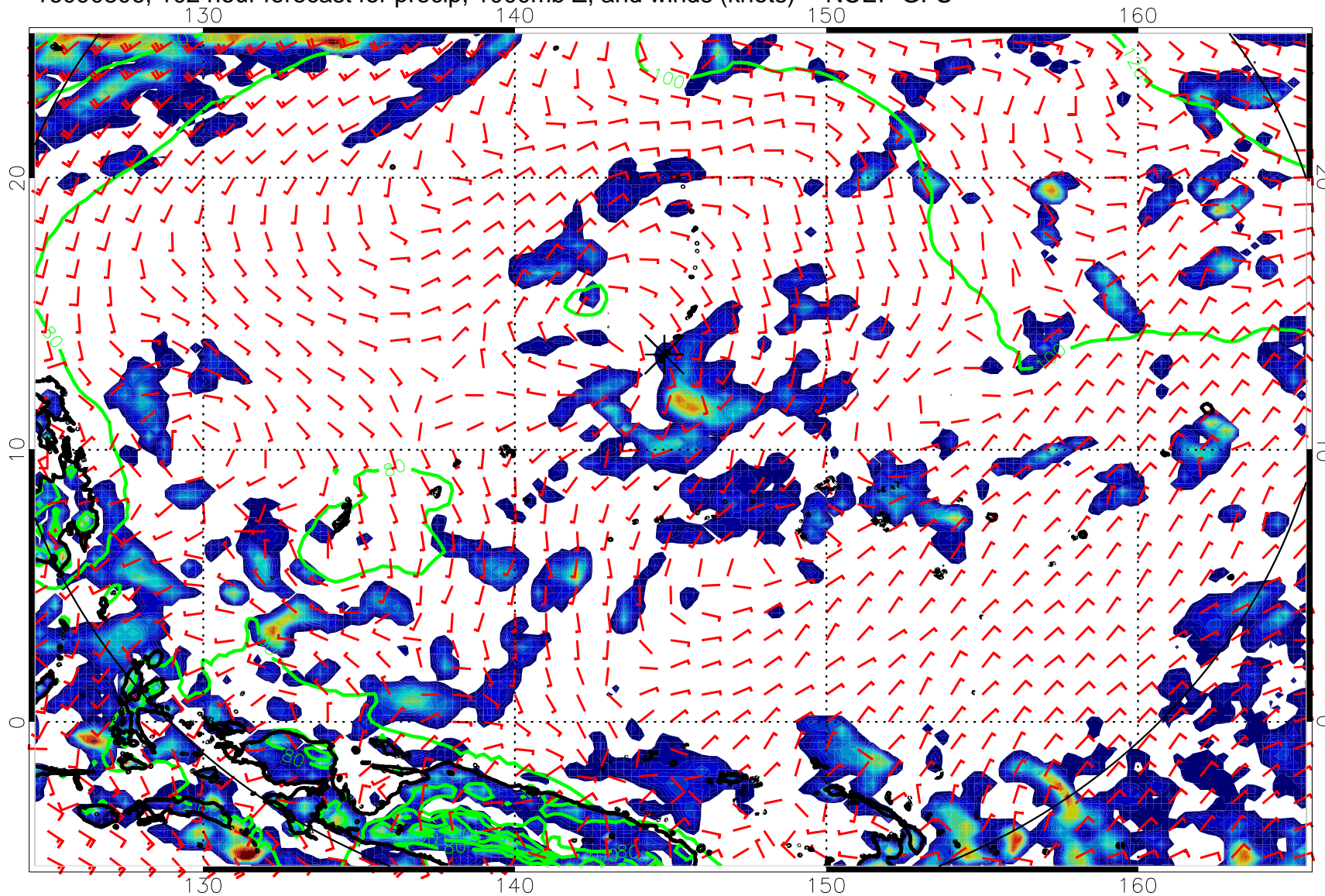
16090806, 102 hour forecast for precip, 1000mb Z, and winds (knots) -- NCEP GFS
