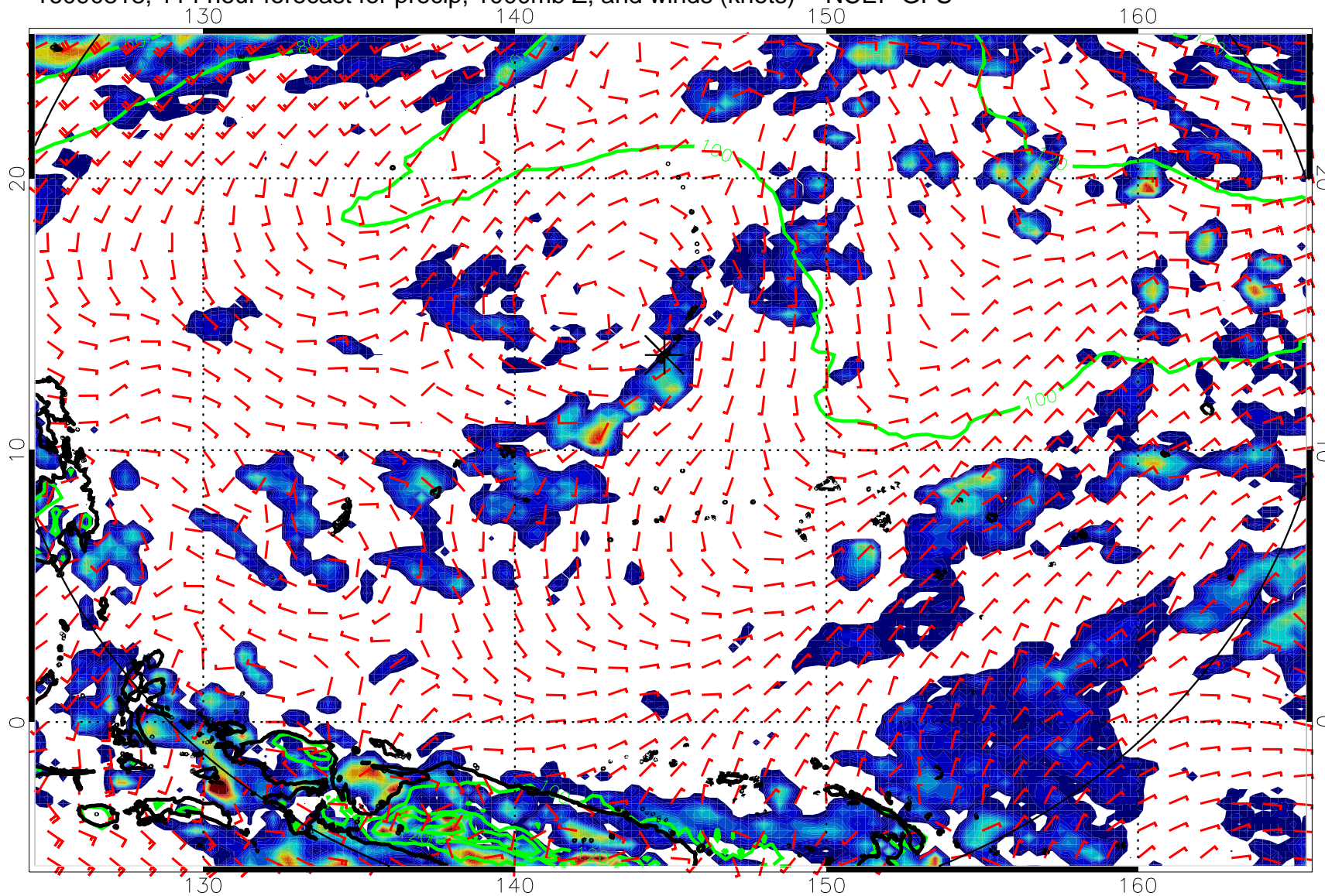
16090818, 114 hour forecast for precip, 1000mb Z, and winds (knots) -- NCEP GFS
