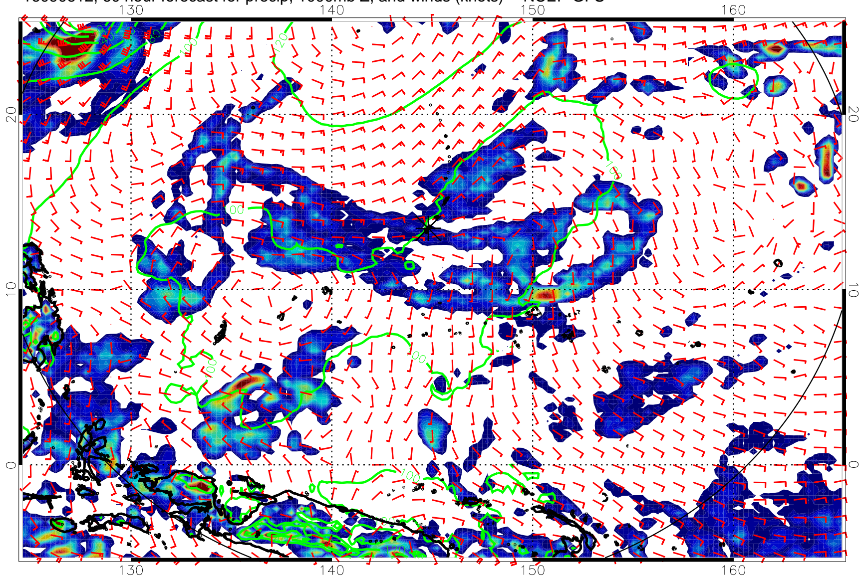
16090612, 60 hour forecast for precip, 1000mb Z, and winds (knots) -- NCEP GFS
