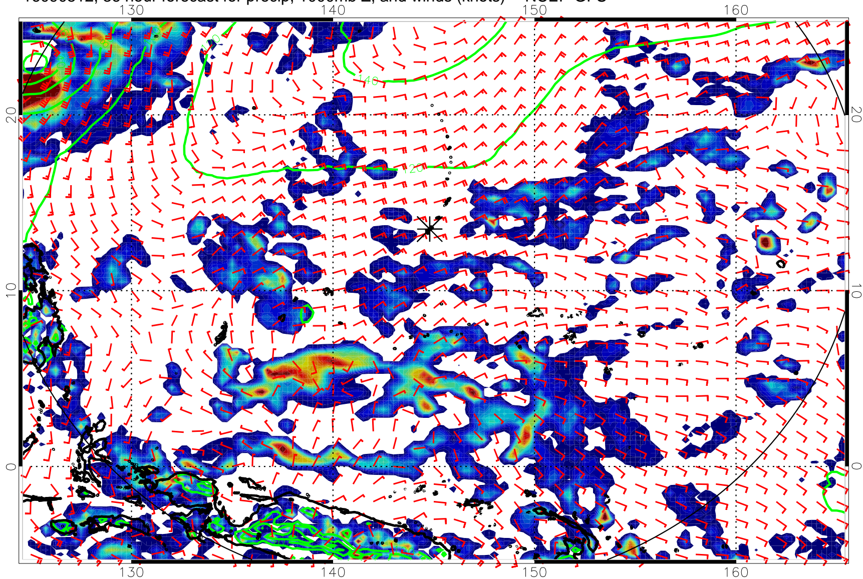
16090512, 36 hour forecast for precip, 1000mb Z, and winds (knots) -- NCEP GFS
