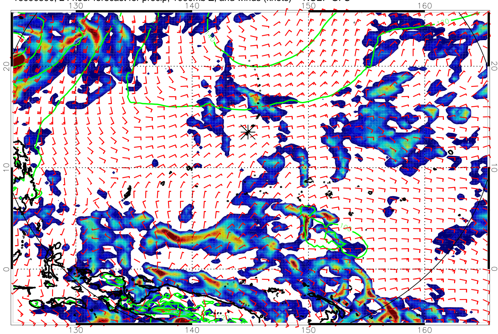
16090500, 24 hour forecast for precip, 1000mb Z, and winds (knots) -- NCEP GFS
