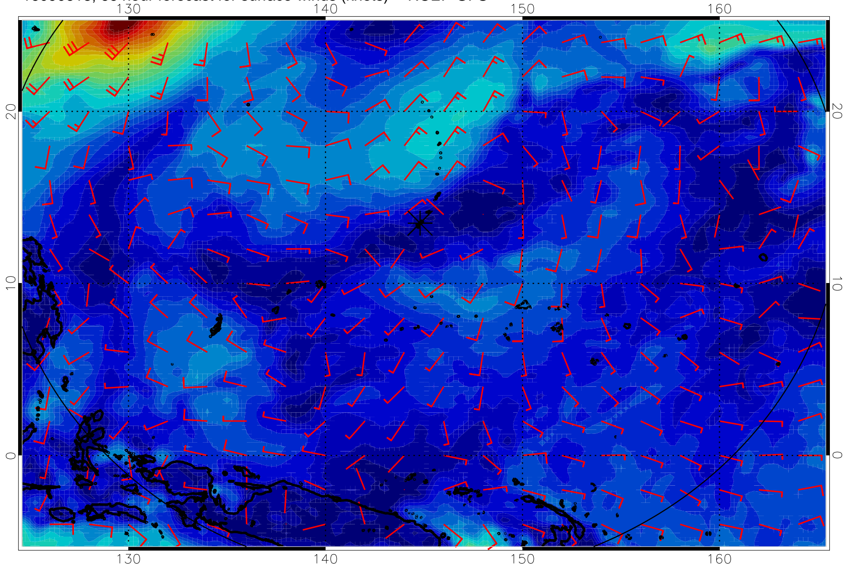
16090618, 66 hour forecast for surface winds (knots) -- NCEP GFS
