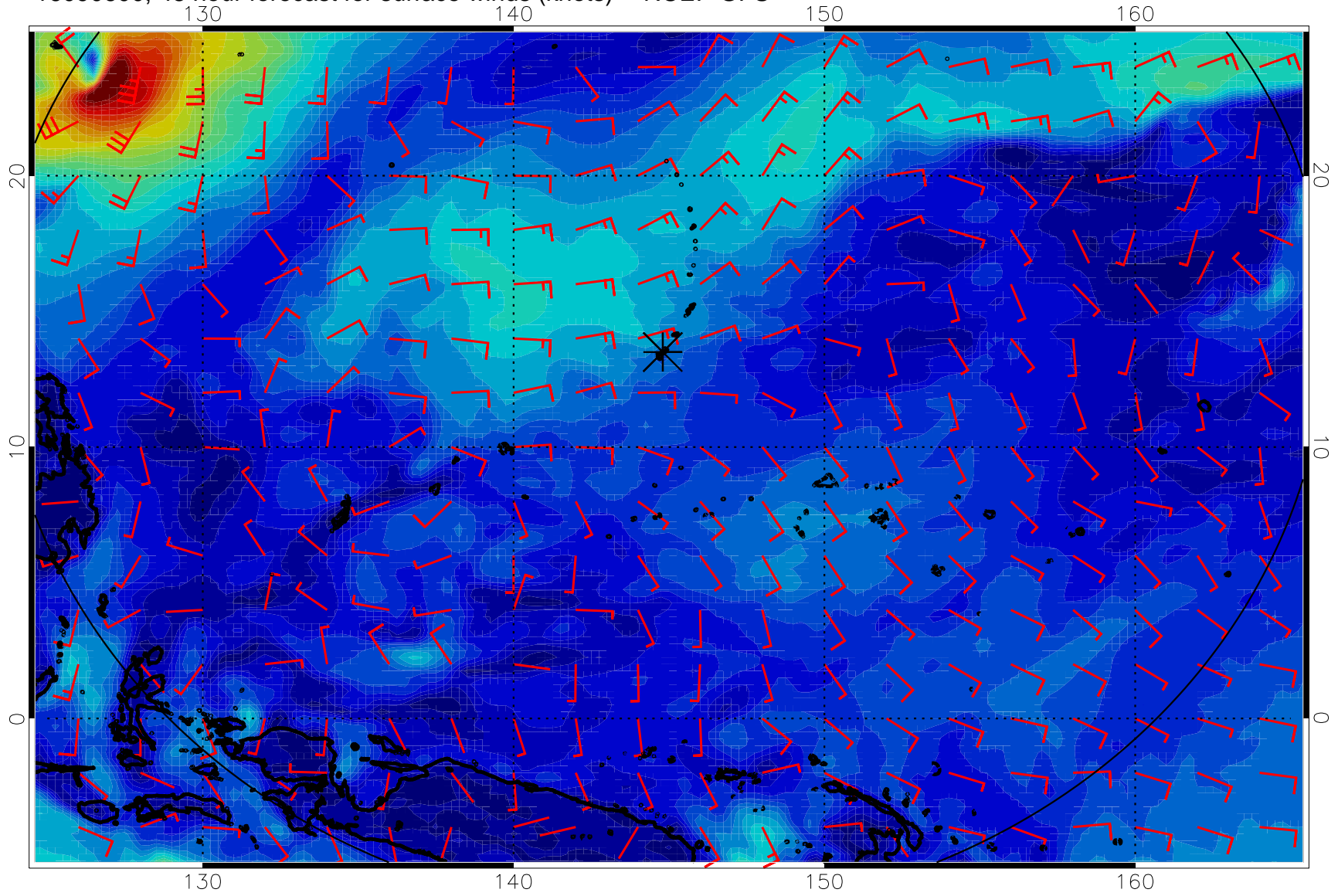
16090600, 48 hour forecast for surface winds (knots) -- NCEP GFS
