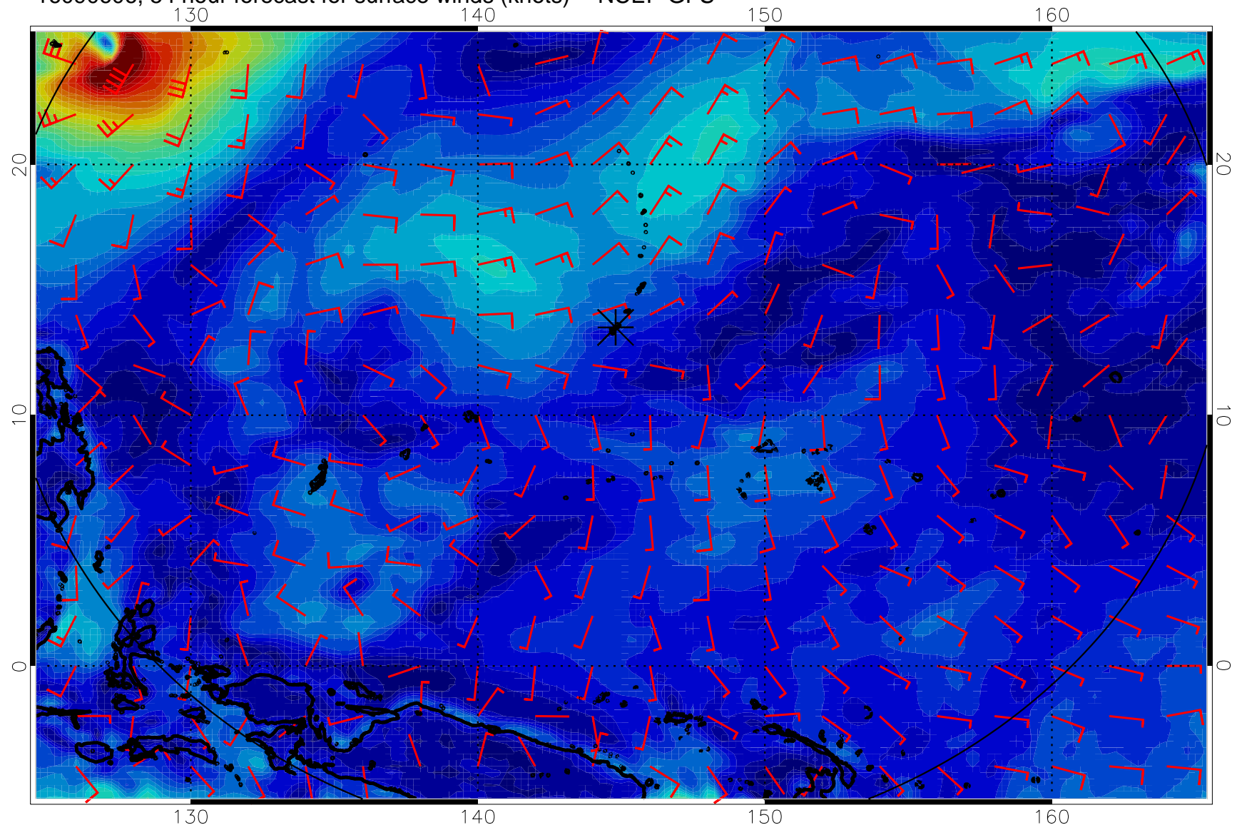
16090606, 54 hour forecast for surface winds (knots) -- NCEP GFS
