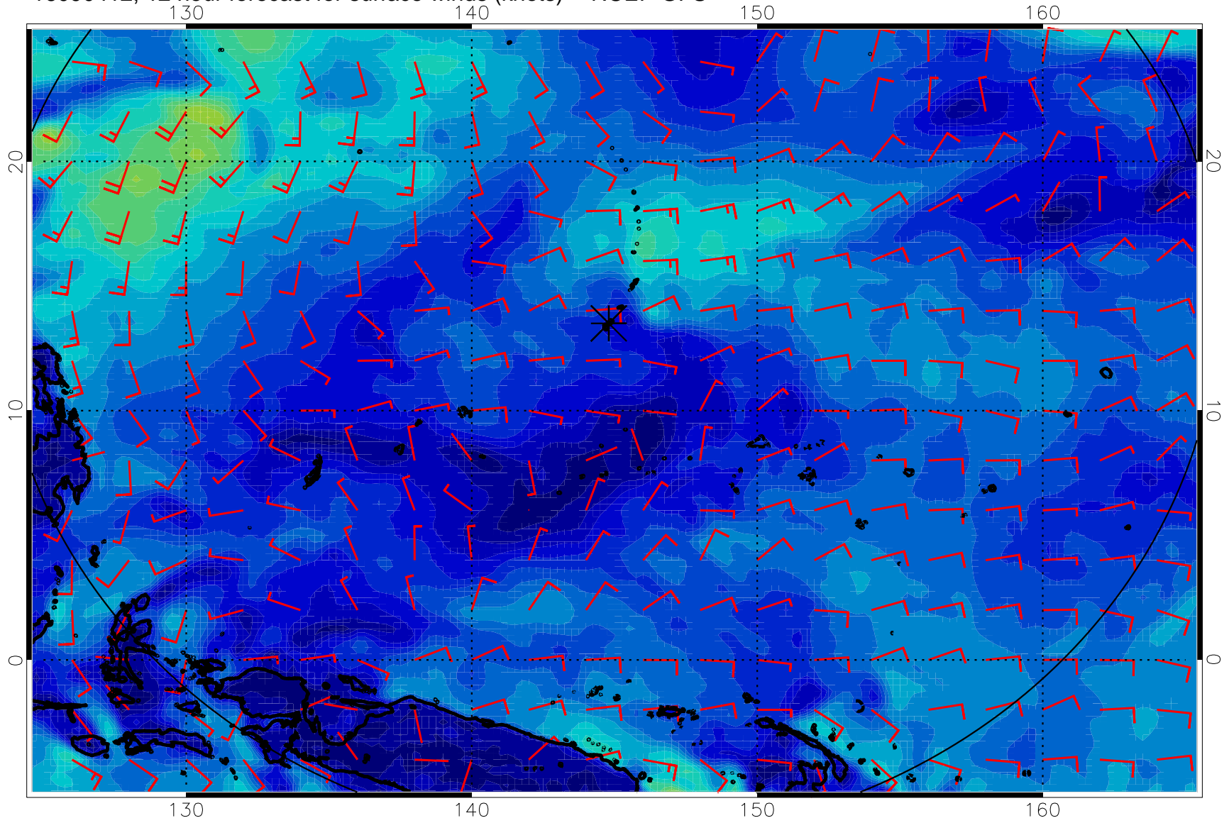
16090412, 12 hour forecast for surface winds (knots) -- NCEP GFS
