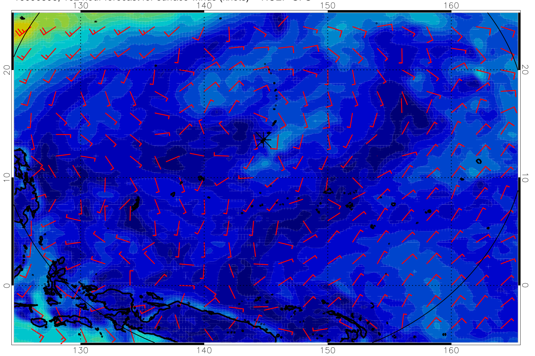
16090806, 102 hour forecast for surface winds (knots) -- NCEP GFS
