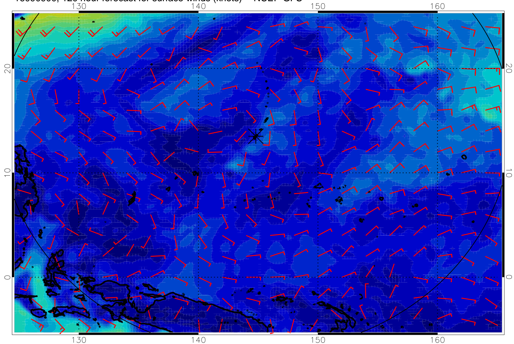
16090900, 120 hour forecast for surface winds (knots) -- NCEP GFS
