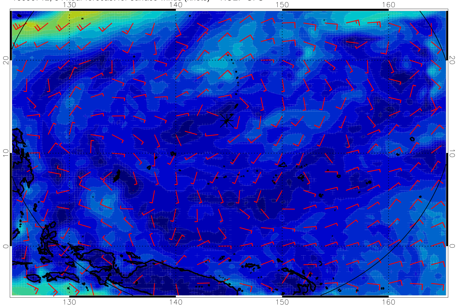
16090712, 84 hour forecast for surface winds (knots) -- NCEP GFS
