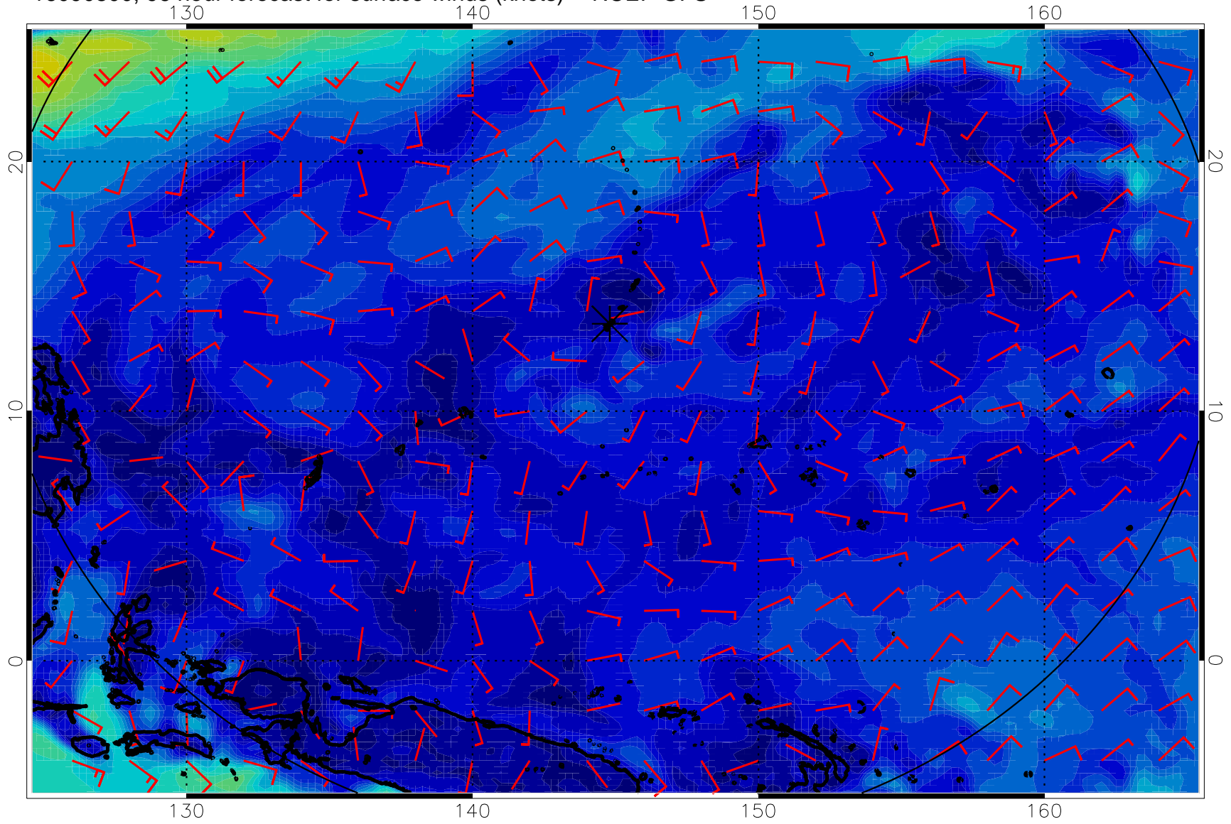
16090800, 96 hour forecast for surface winds (knots) -- NCEP GFS
