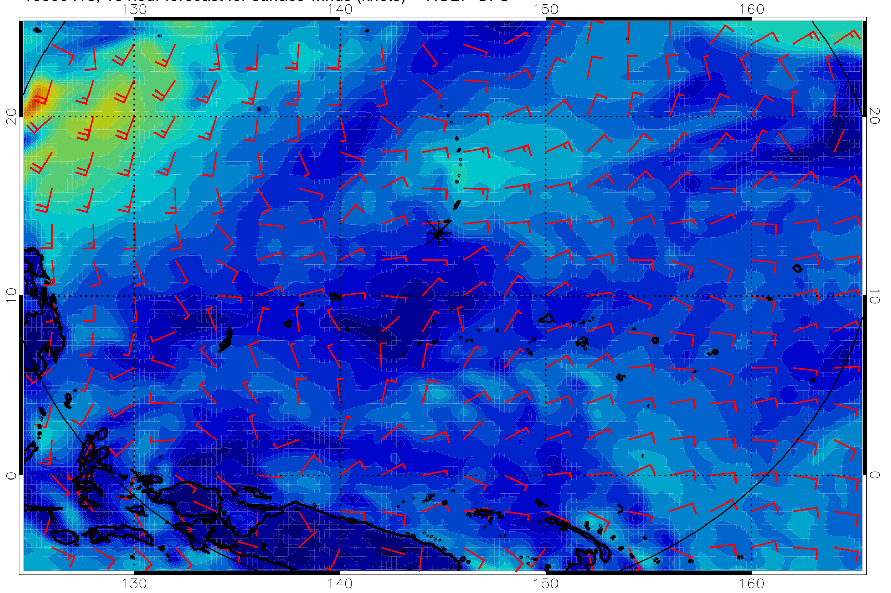
16090418, 18 hour forecast for surface winds (knots) -- NCEP GFS
