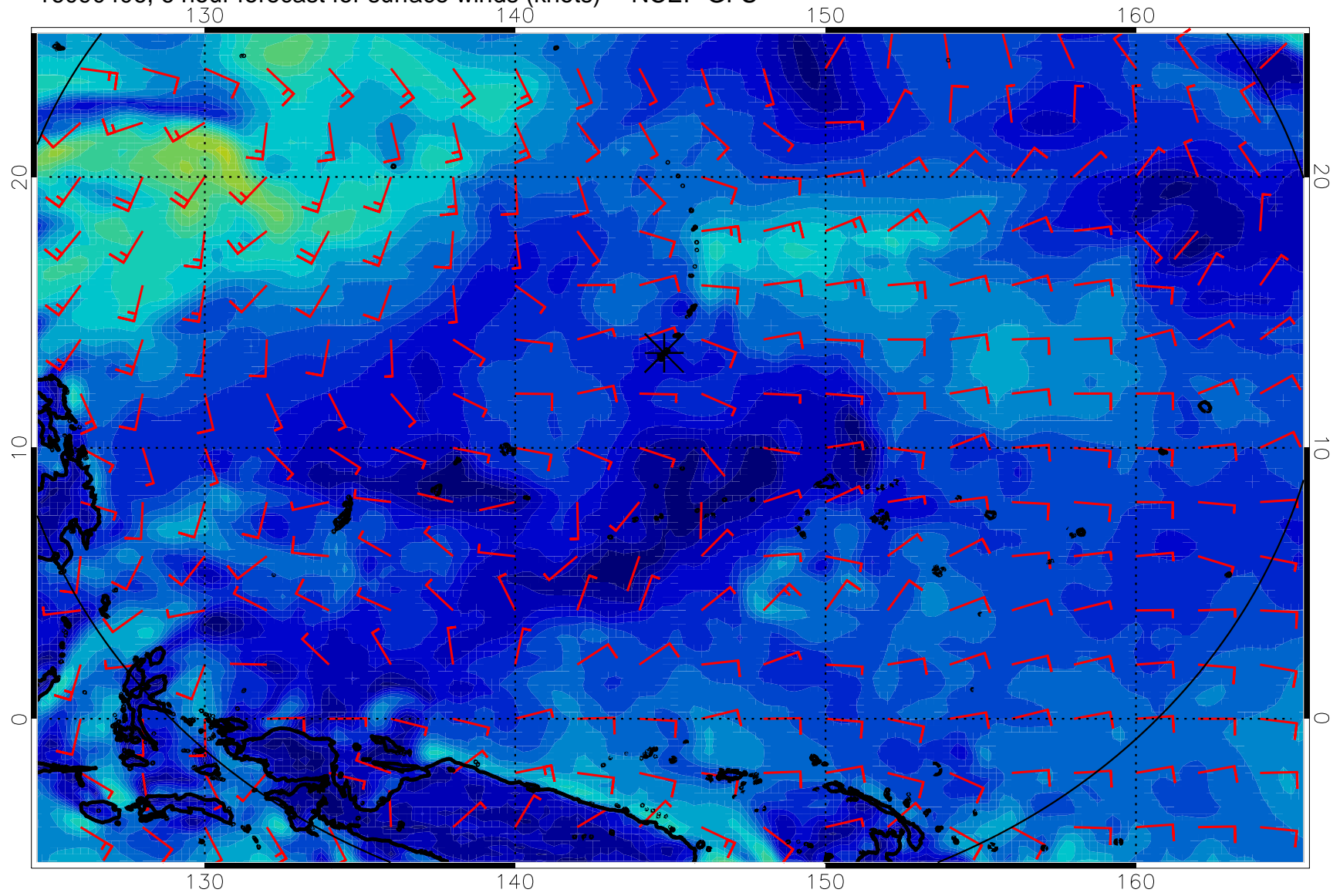
16090406, 6 hour forecast for surface winds (knots) -- NCEP GFS
