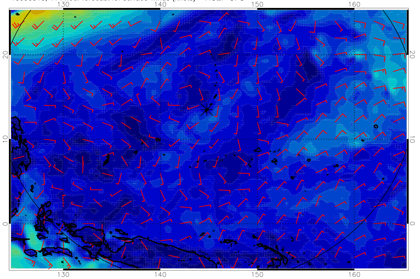
16090818, 114 hour forecast for surface winds (knots) -- NCEP GFS
