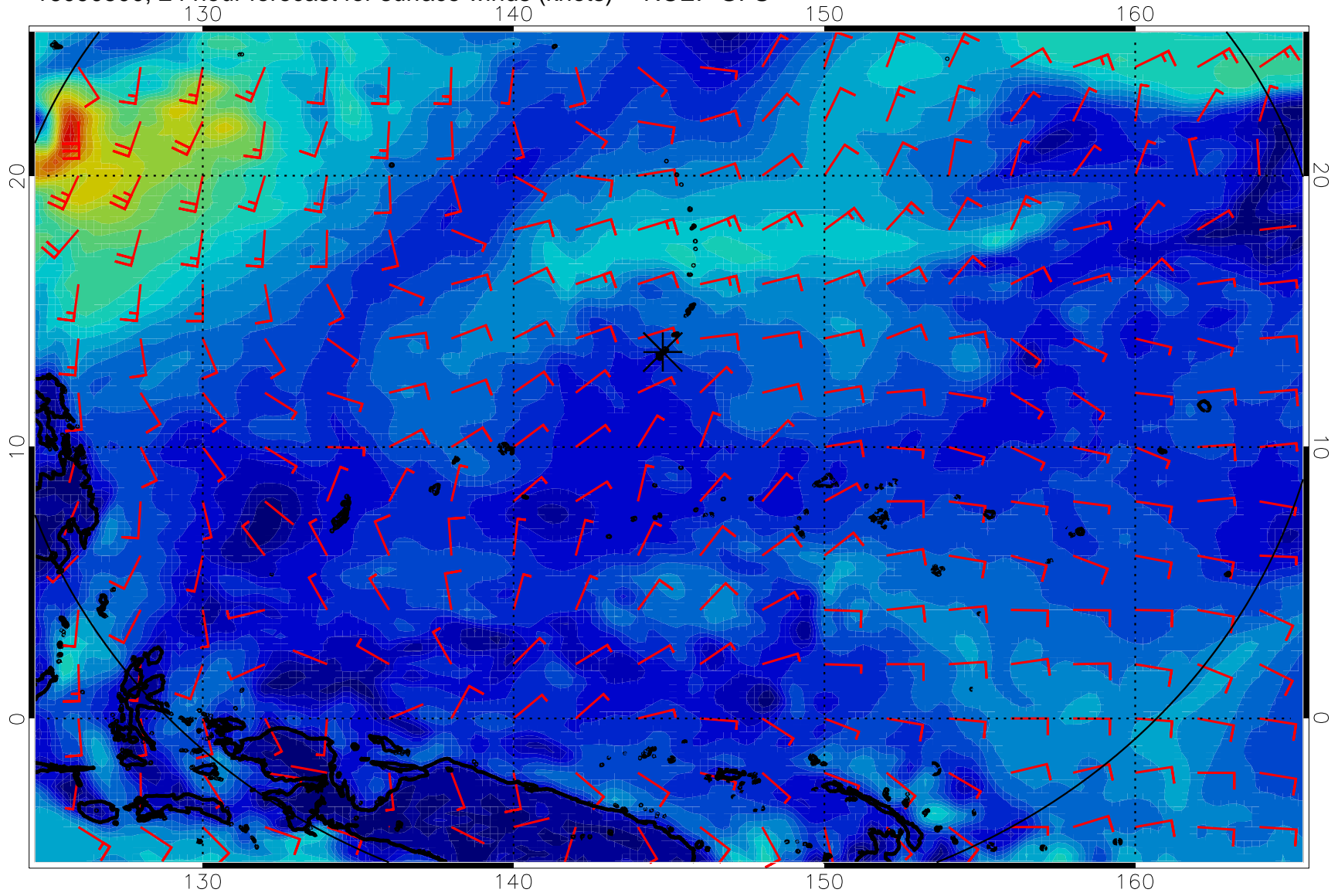
16090500, 24 hour forecast for surface winds (knots) -- NCEP GFS
