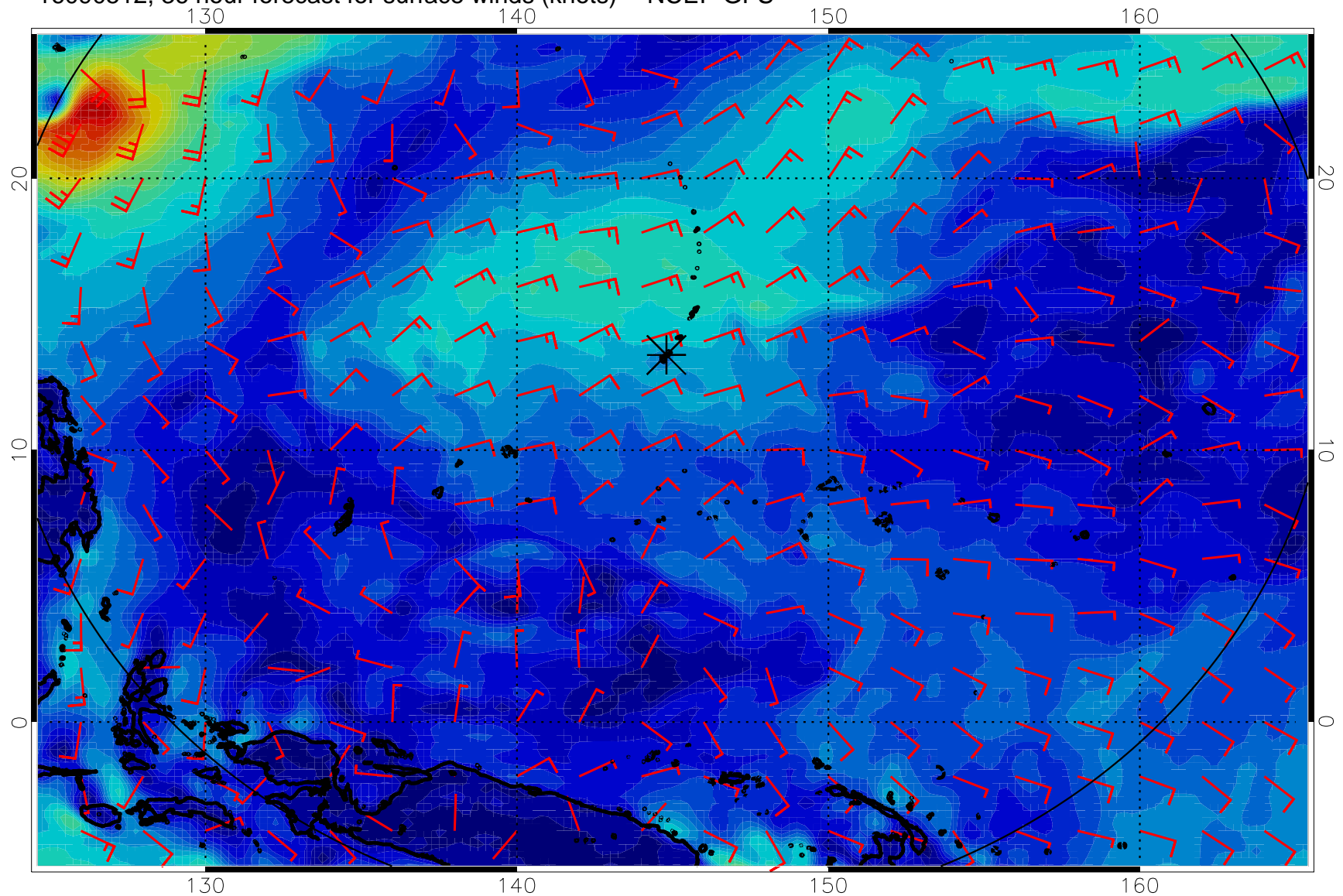
16090512, 36 hour forecast for surface winds (knots) -- NCEP GFS
