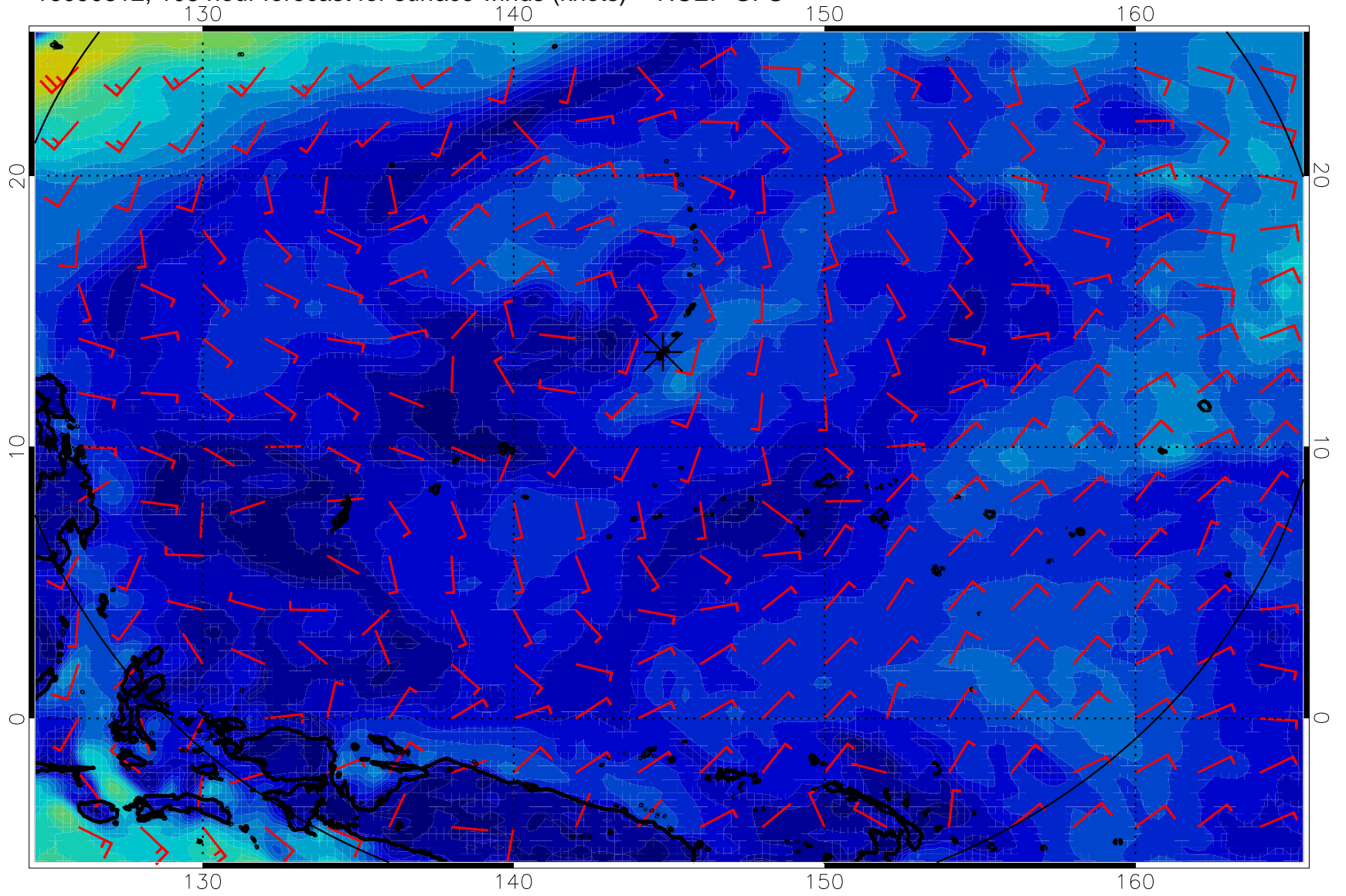
16090812, 108 hour forecast for surface winds (knots) -- NCEP GFS
