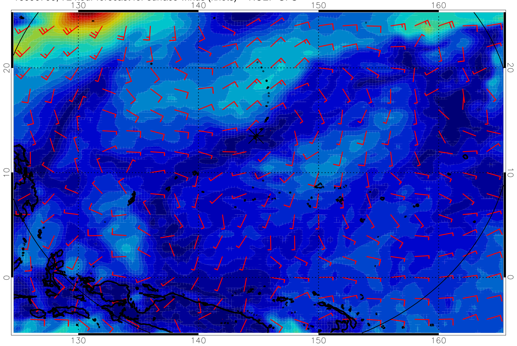
16090700, 72 hour forecast for surface winds (knots) -- NCEP GFS
