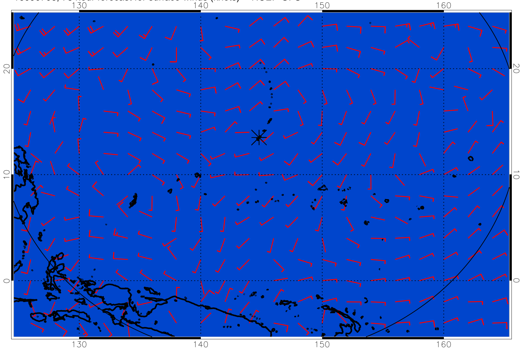
16090706, 78 hour forecast for surface winds (knots) -- NCEP GFS
