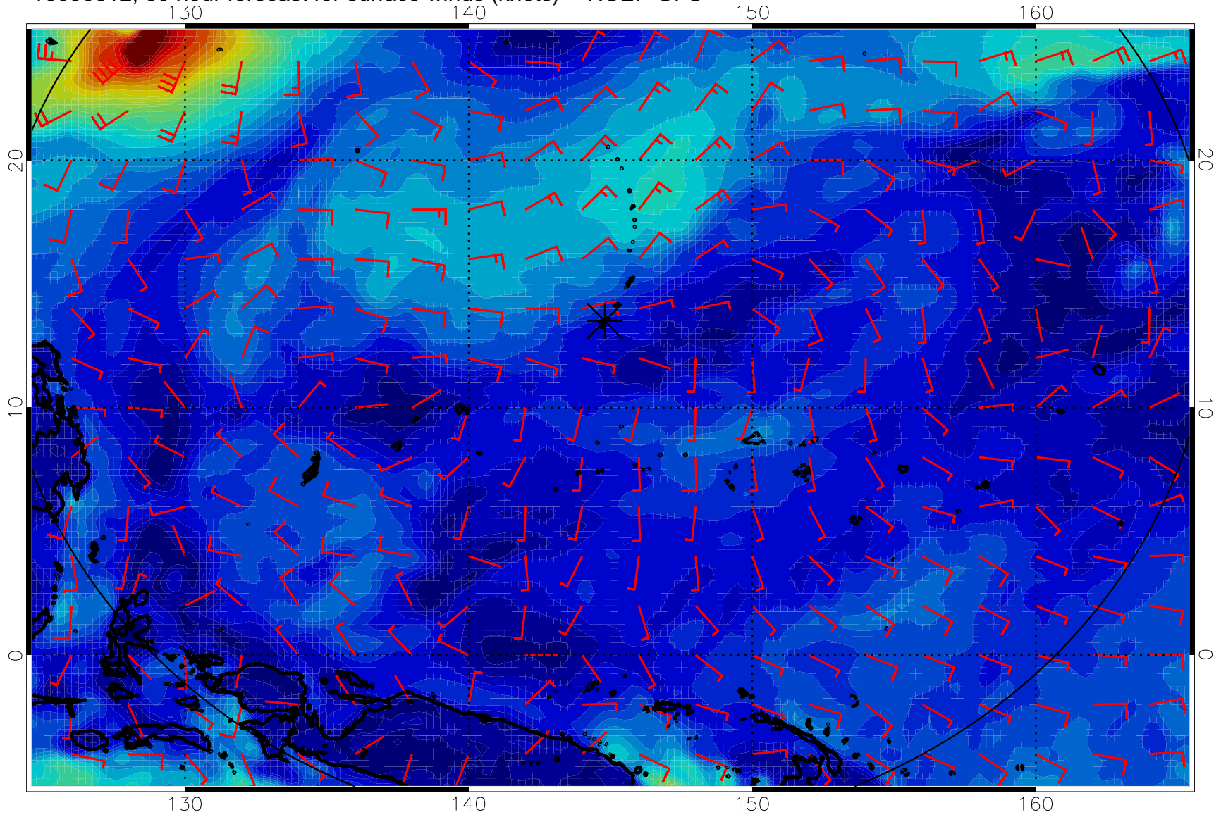
16090612, 60 hour forecast for surface winds (knots) -- NCEP GFS
