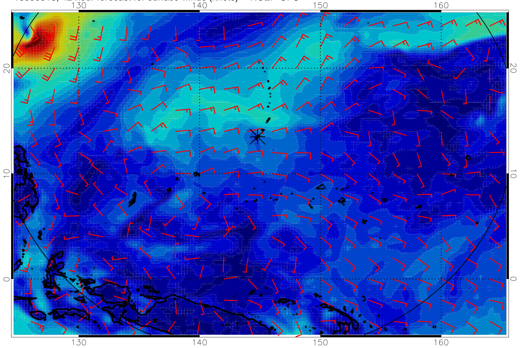
16090518, 42 hour forecast for surface winds (knots) -- NCEP GFS
