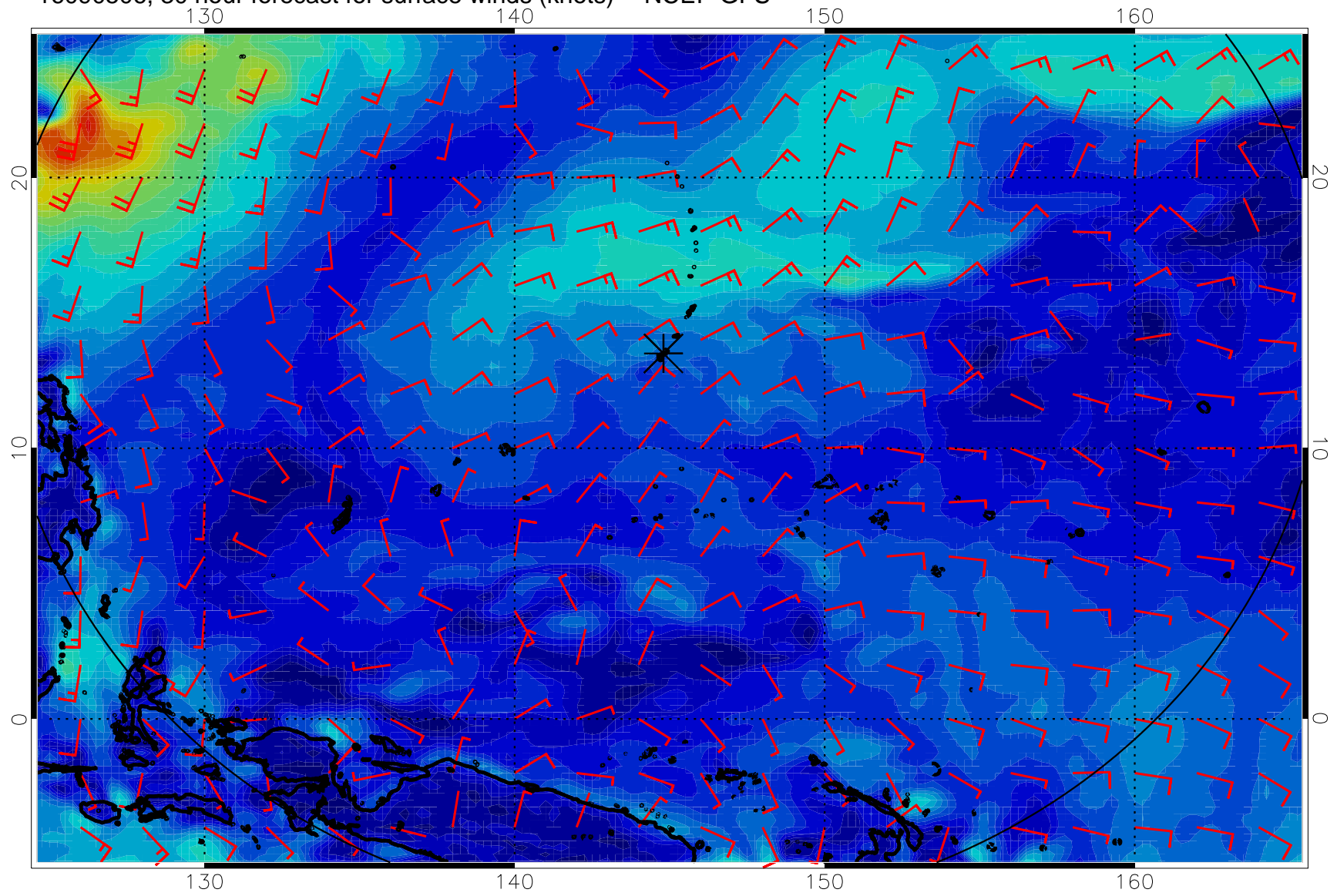
16090506, 30 hour forecast for surface winds (knots) -- NCEP GFS
