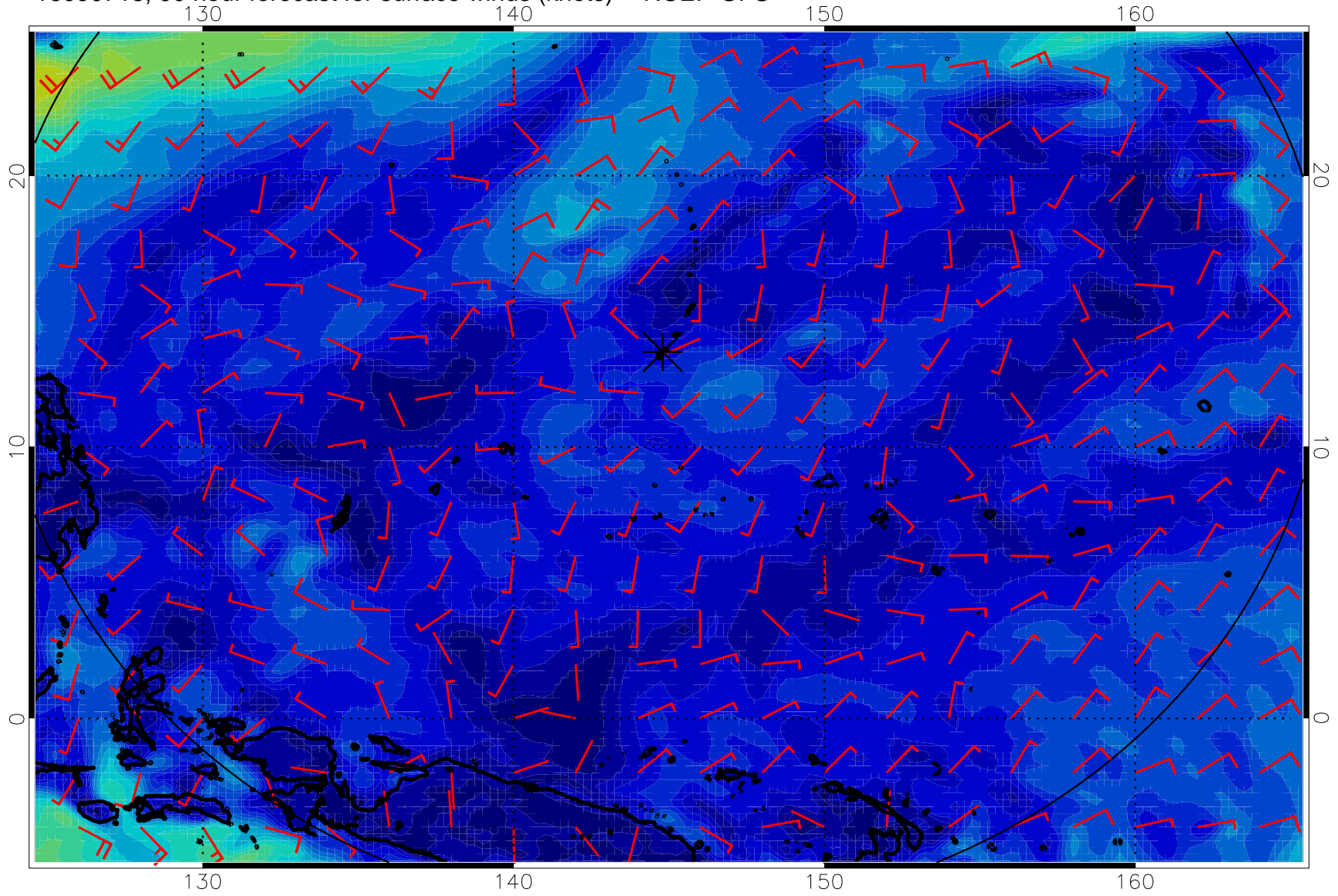
16090718, 90 hour forecast for surface winds (knots) -- NCEP GFS
