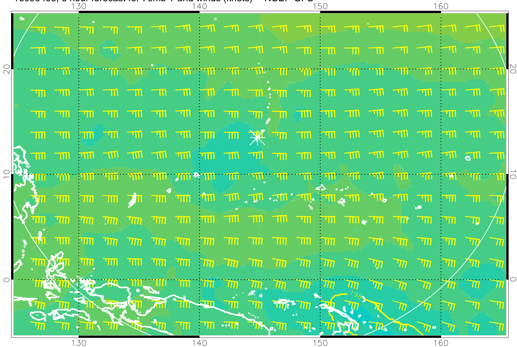
16090406, 6 hour forecast for 70mb T and winds (knots) -- NCEP GFS
