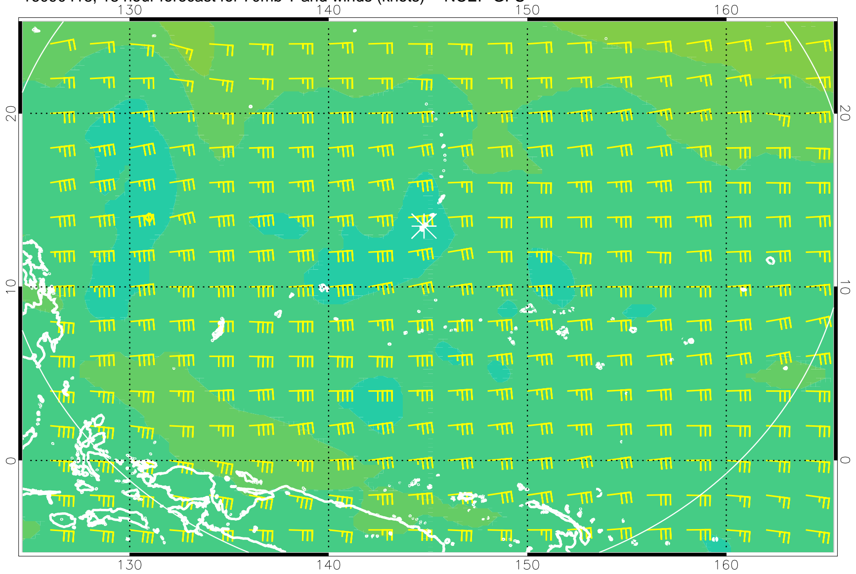
16090418, 18 hour forecast for 70mb T and winds (knots) -- NCEP GFS
