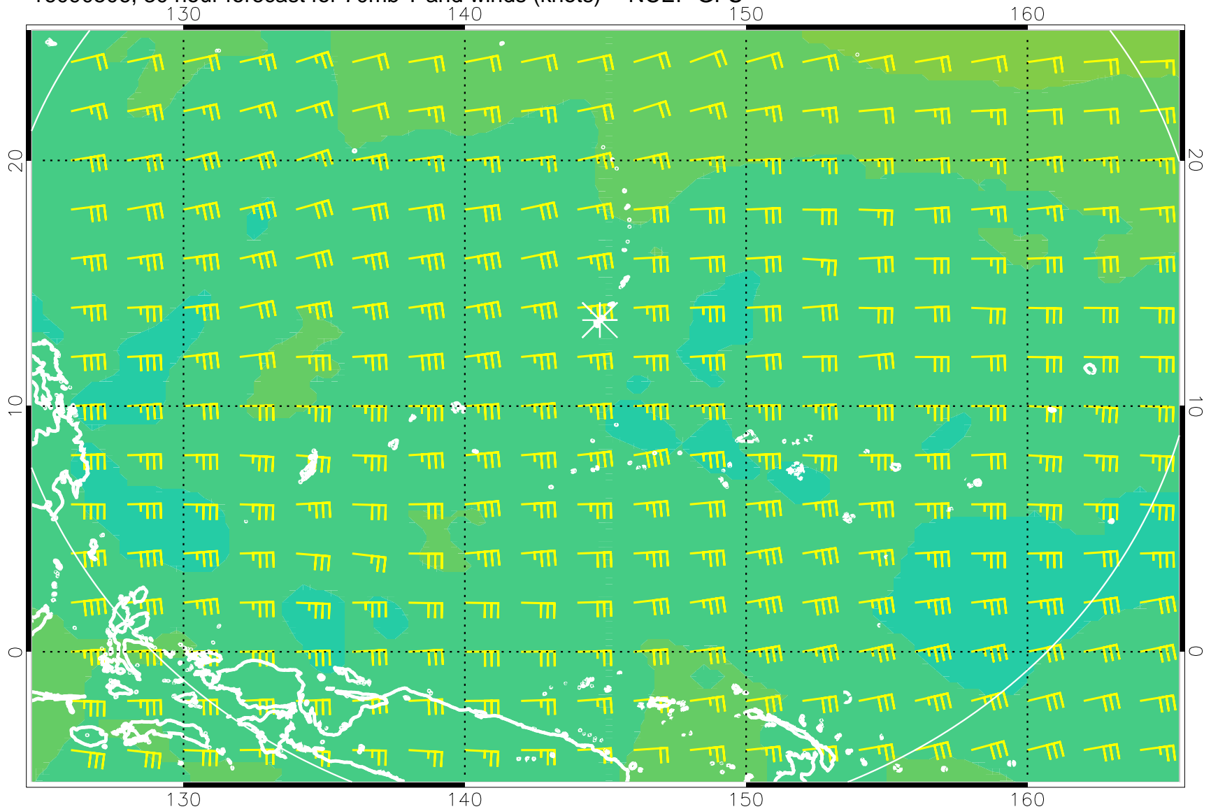
16090506, 30 hour forecast for 70mb T and winds (knots) -- NCEP GFS
