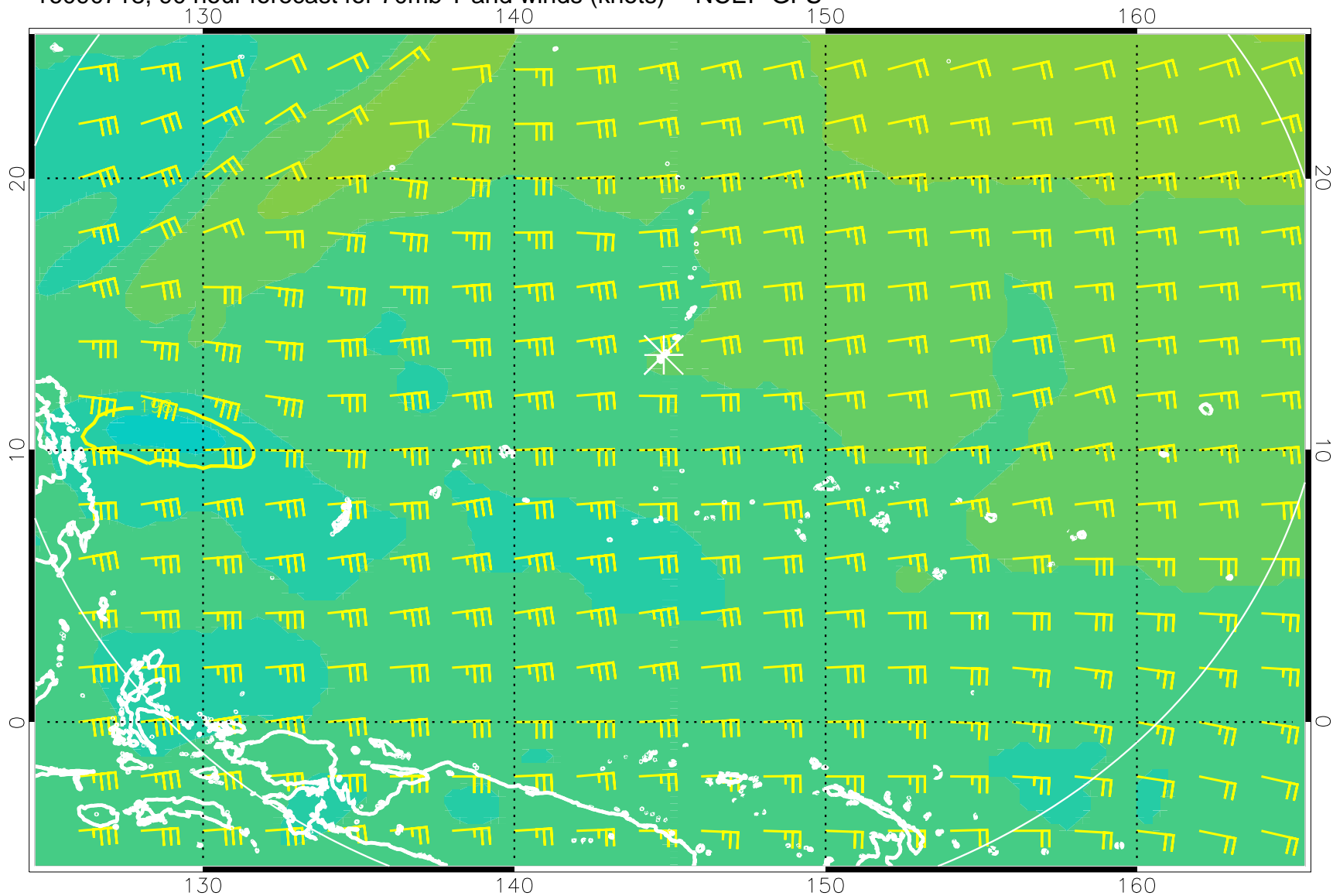
16090718, 90 hour forecast for 70mb T and winds (knots) -- NCEP GFS
