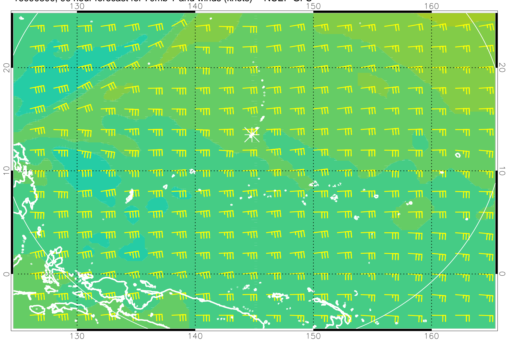
16090800, 96 hour forecast for 70mb T and winds (knots) -- NCEP GFS
