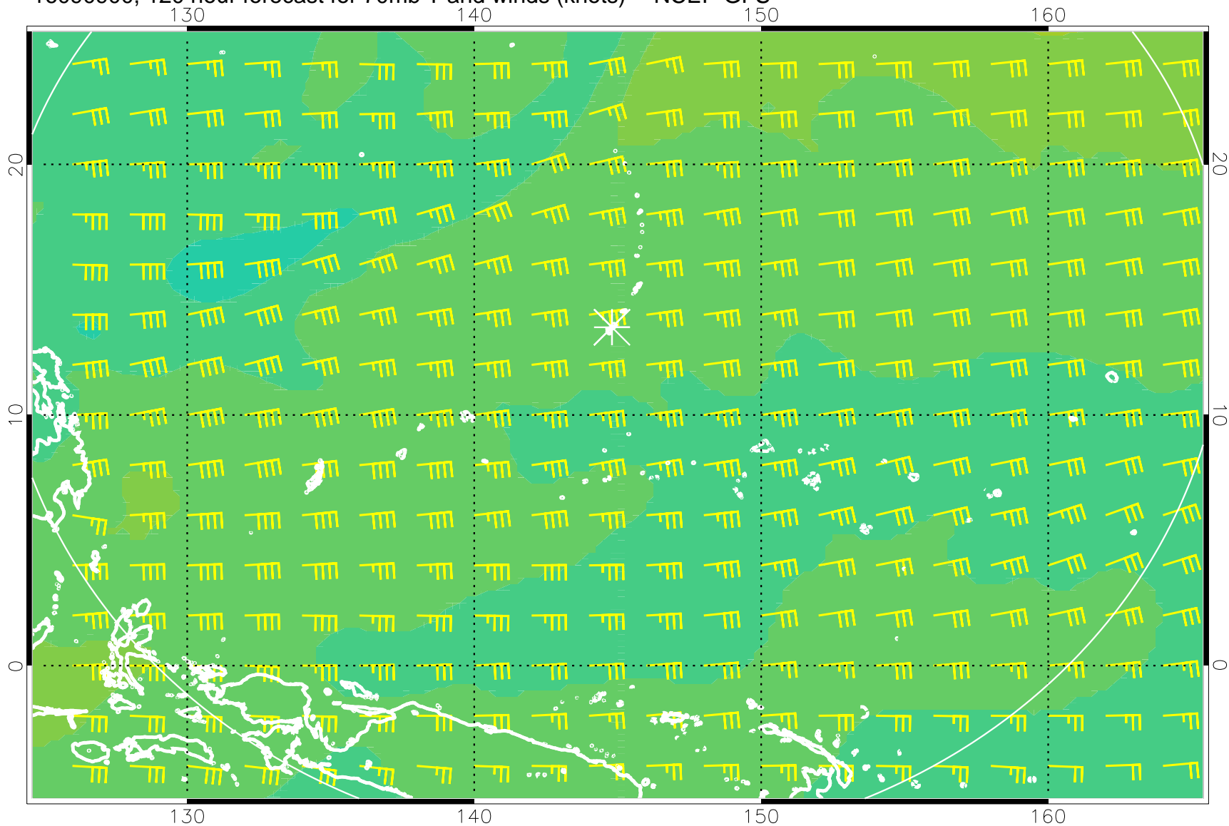
16090900, 120 hour forecast for 70mb T and winds (knots) -- NCEP GFS
