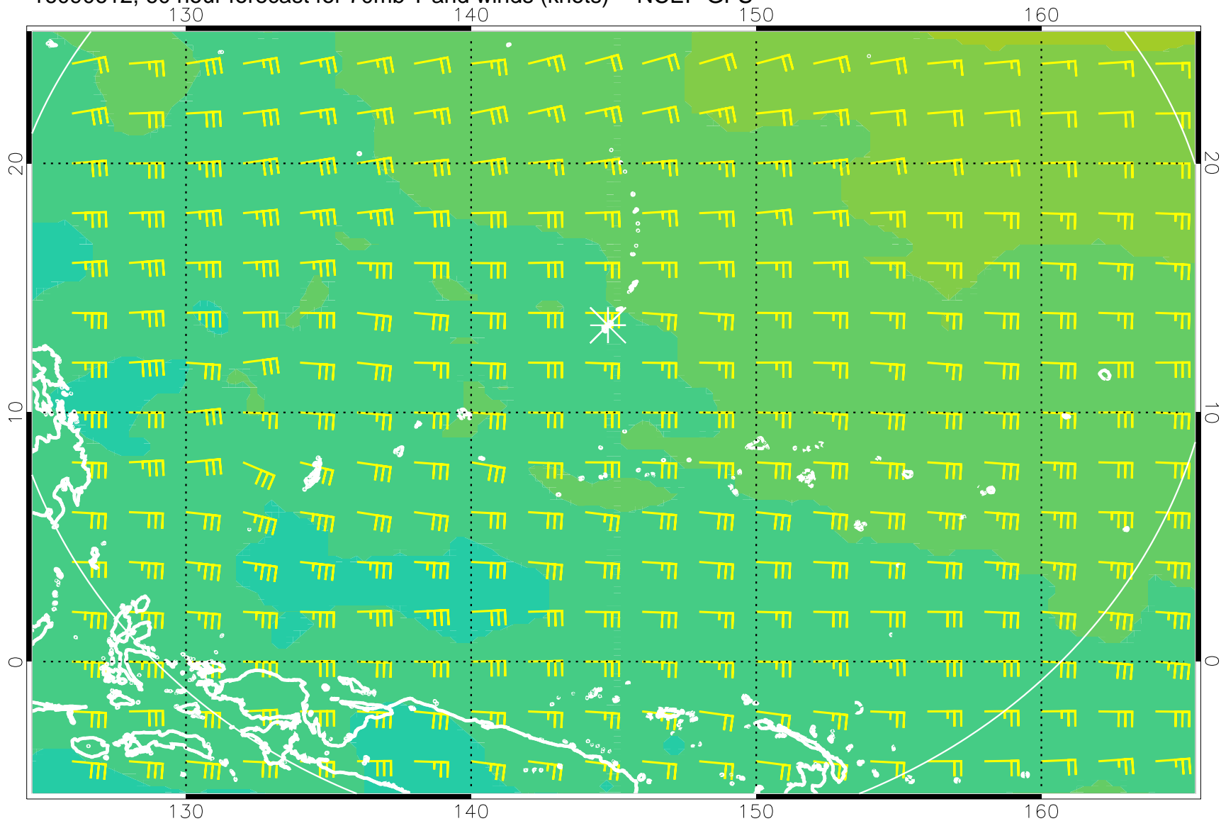
16090612, 60 hour forecast for 70mb T and winds (knots) -- NCEP GFS
