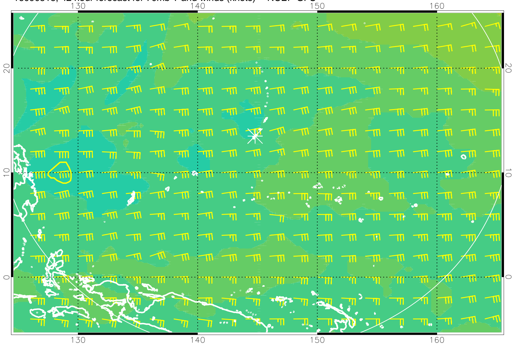
16090518, 42 hour forecast for 70mb T and winds (knots) -- NCEP GFS
