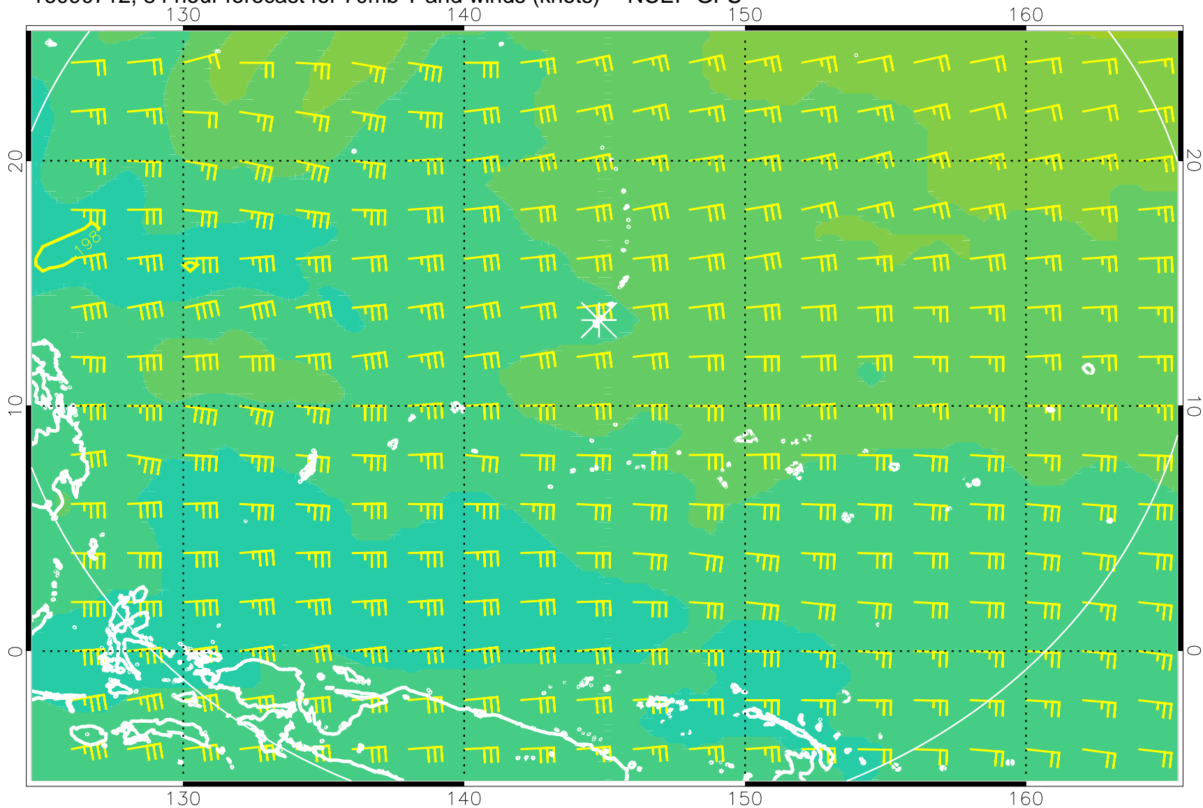
16090712, 84 hour forecast for 70mb T and winds (knots) -- NCEP GFS
