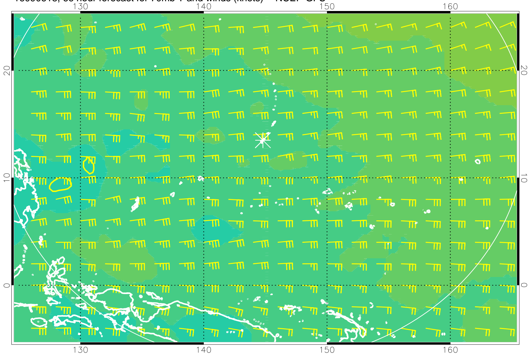
16090618, 66 hour forecast for 70mb T and winds (knots) -- NCEP GFS
