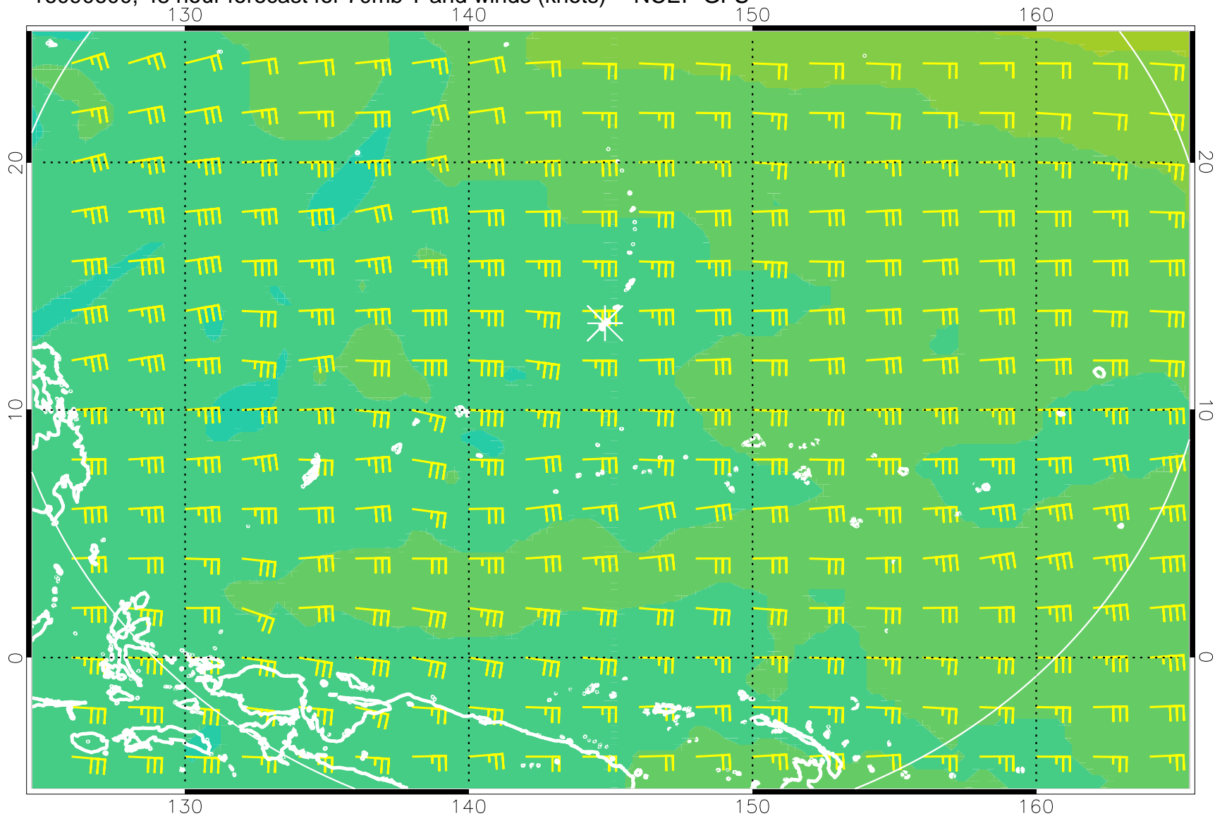
16090600, 48 hour forecast for 70mb T and winds (knots) -- NCEP GFS
