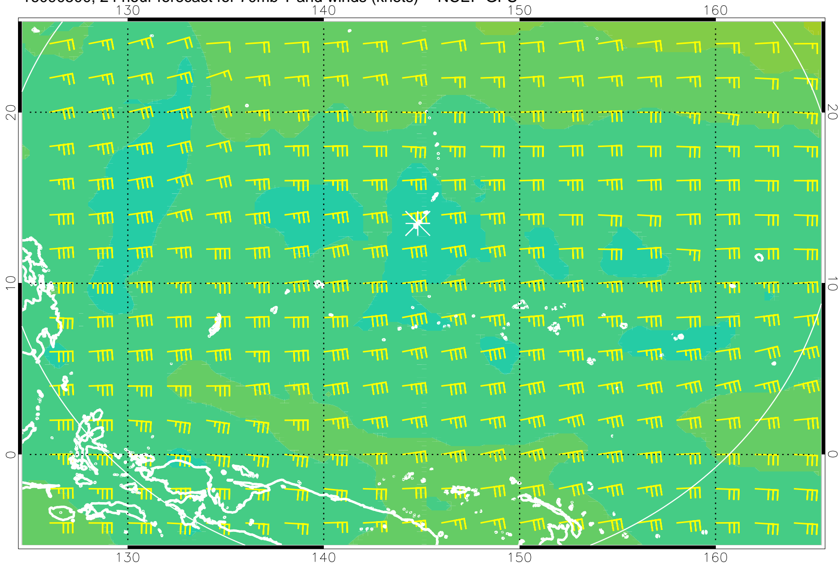
16090500, 24 hour forecast for 70mb T and winds (knots) -- NCEP GFS
