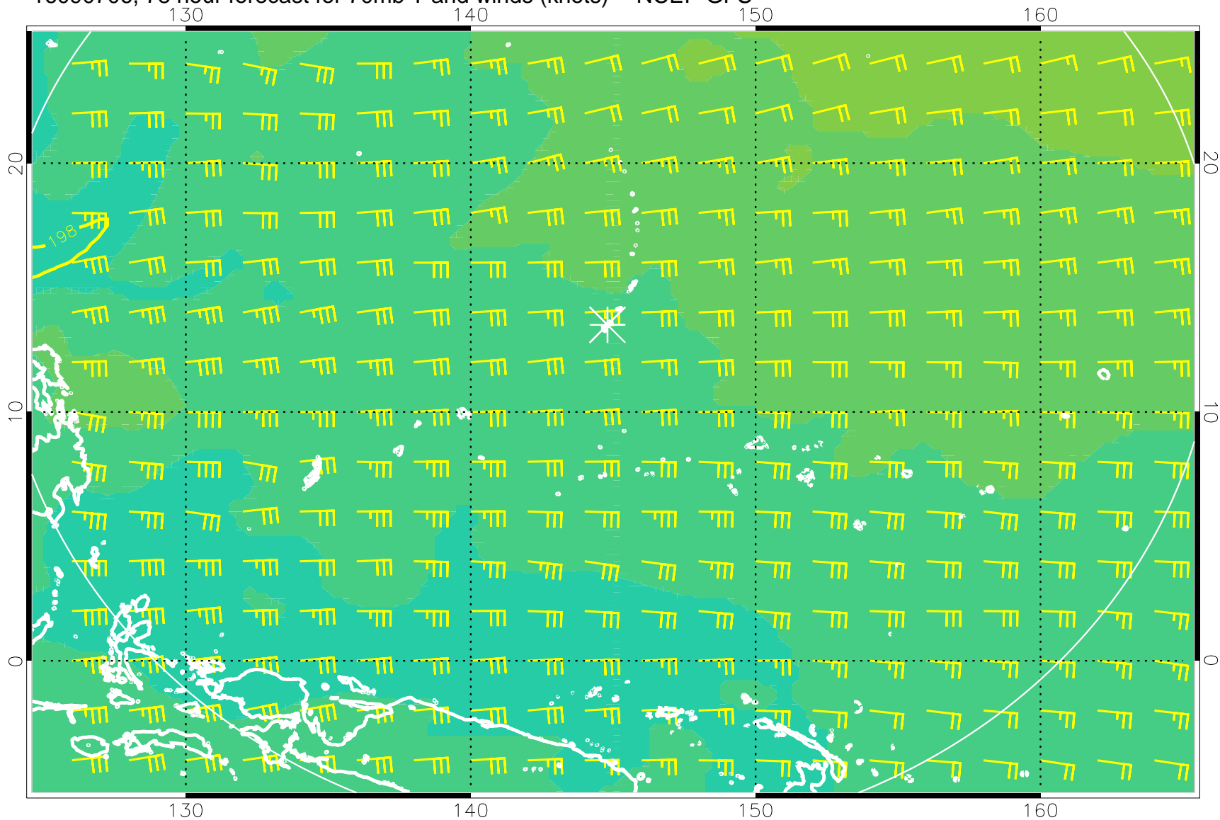
16090706, 78 hour forecast for 70mb T and winds (knots) -- NCEP GFS
