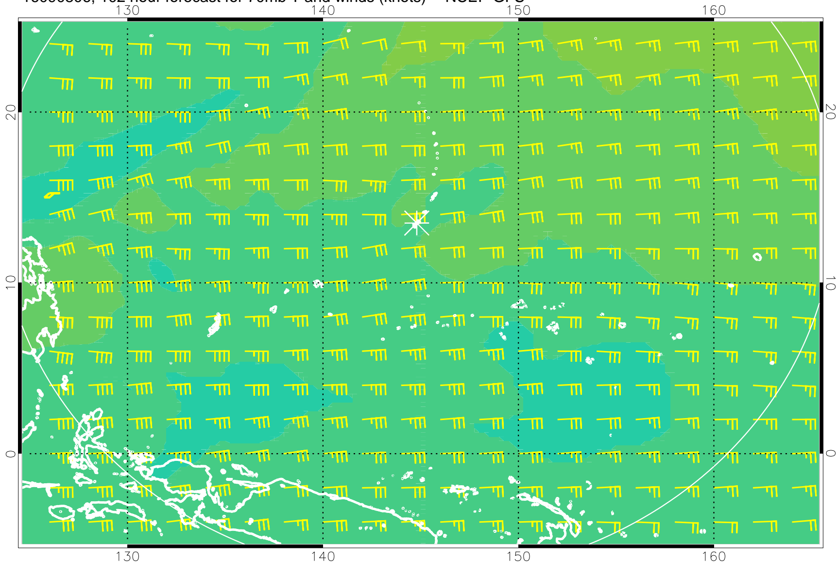
16090806, 102 hour forecast for 70mb T and winds (knots) -- NCEP GFS
