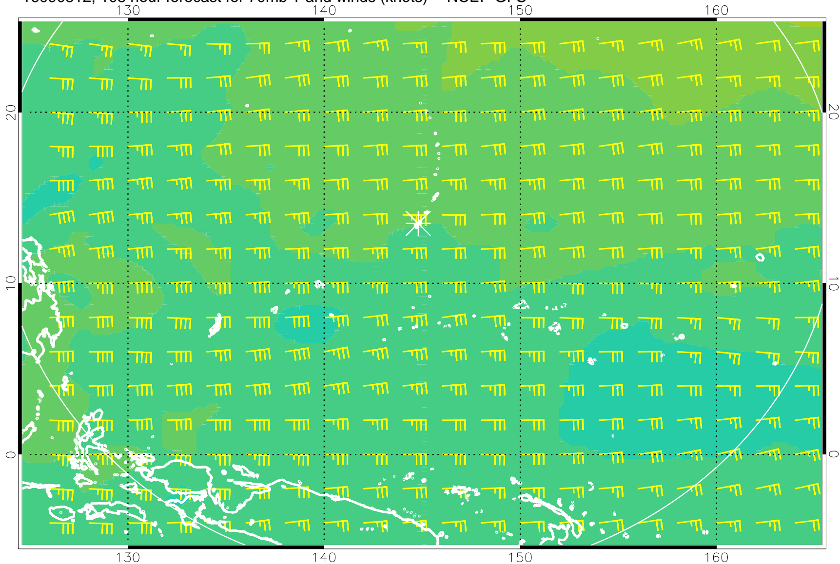
16090812, 108 hour forecast for 70mb T and winds (knots) -- NCEP GFS
