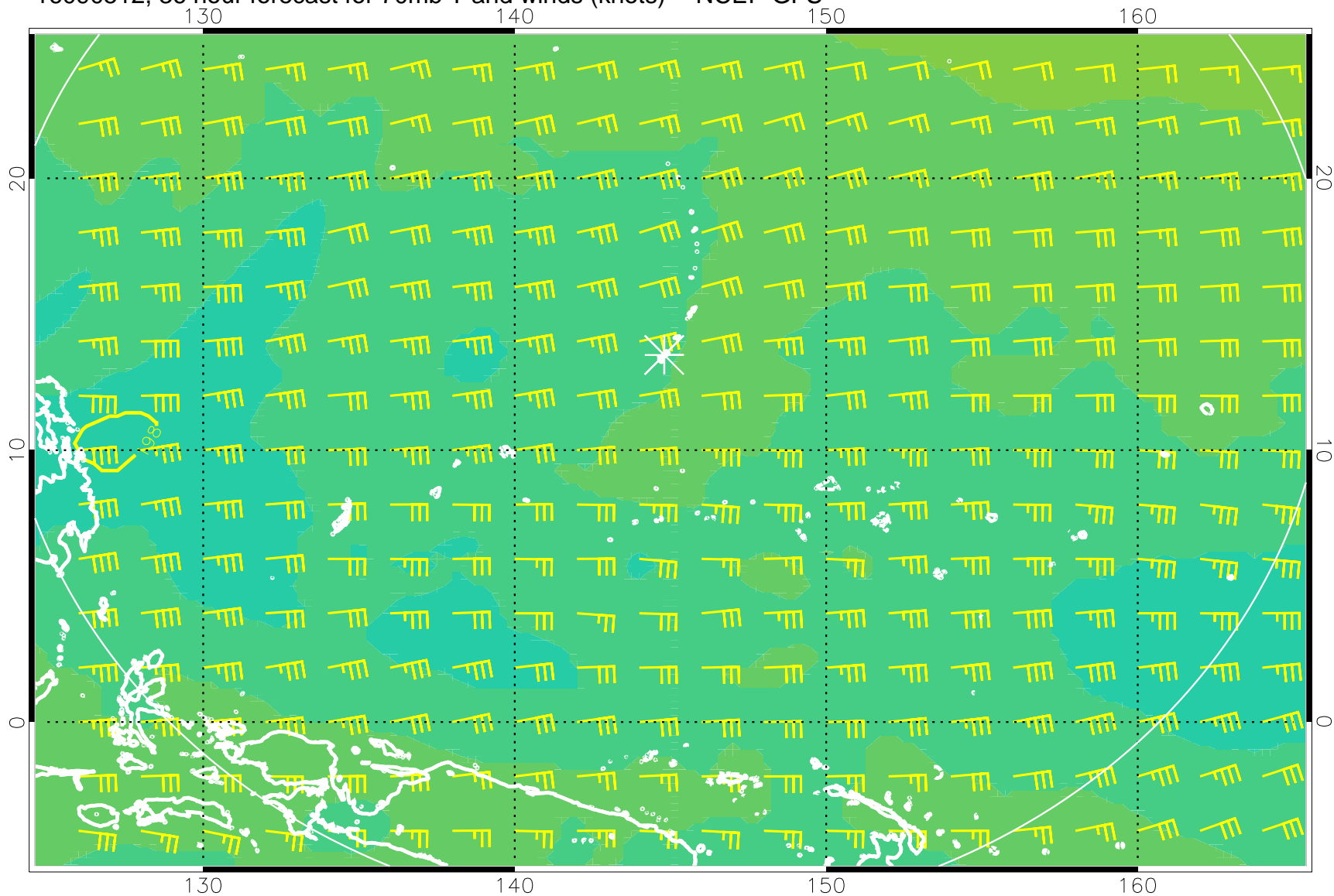
16090512, 36 hour forecast for 70mb T and winds (knots) -- NCEP GFS
