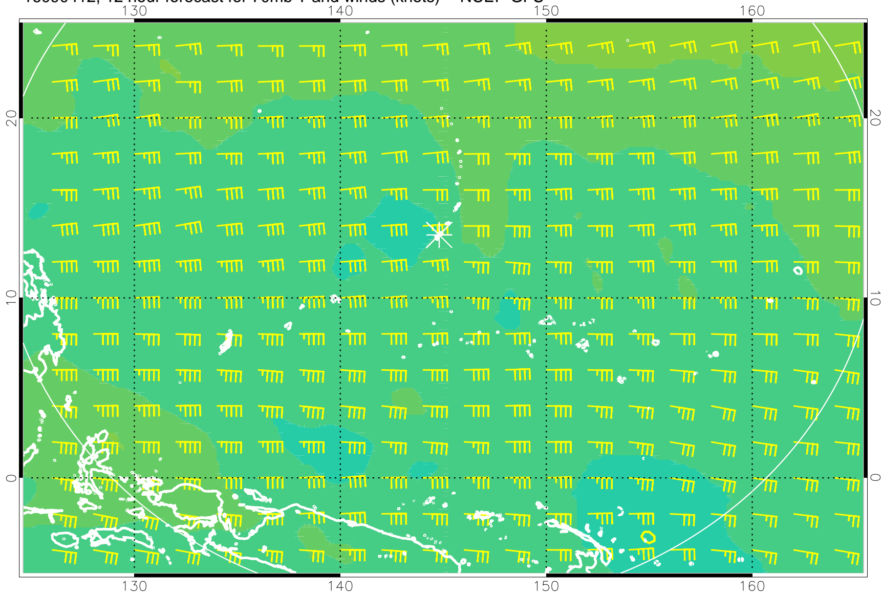
16090412, 12 hour forecast for 70mb T and winds (knots) -- NCEP GFS
