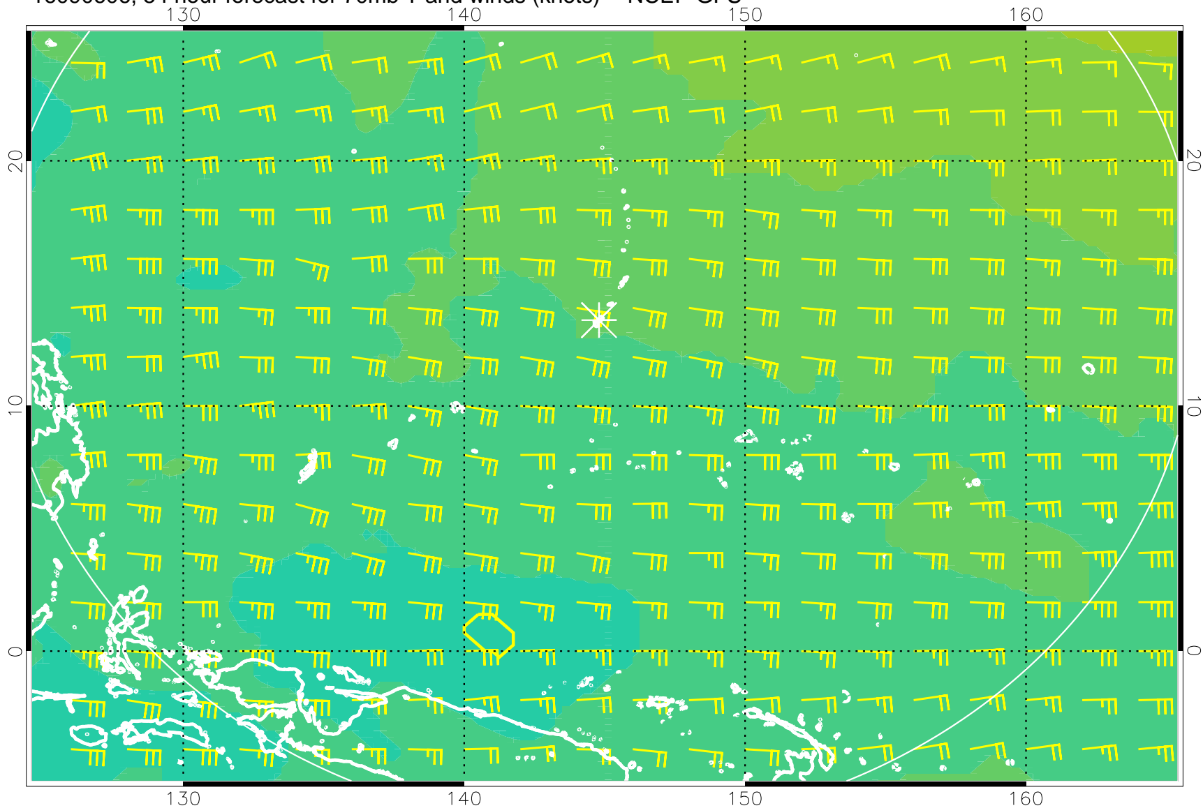
16090606, 54 hour forecast for 70mb T and winds (knots) -- NCEP GFS
