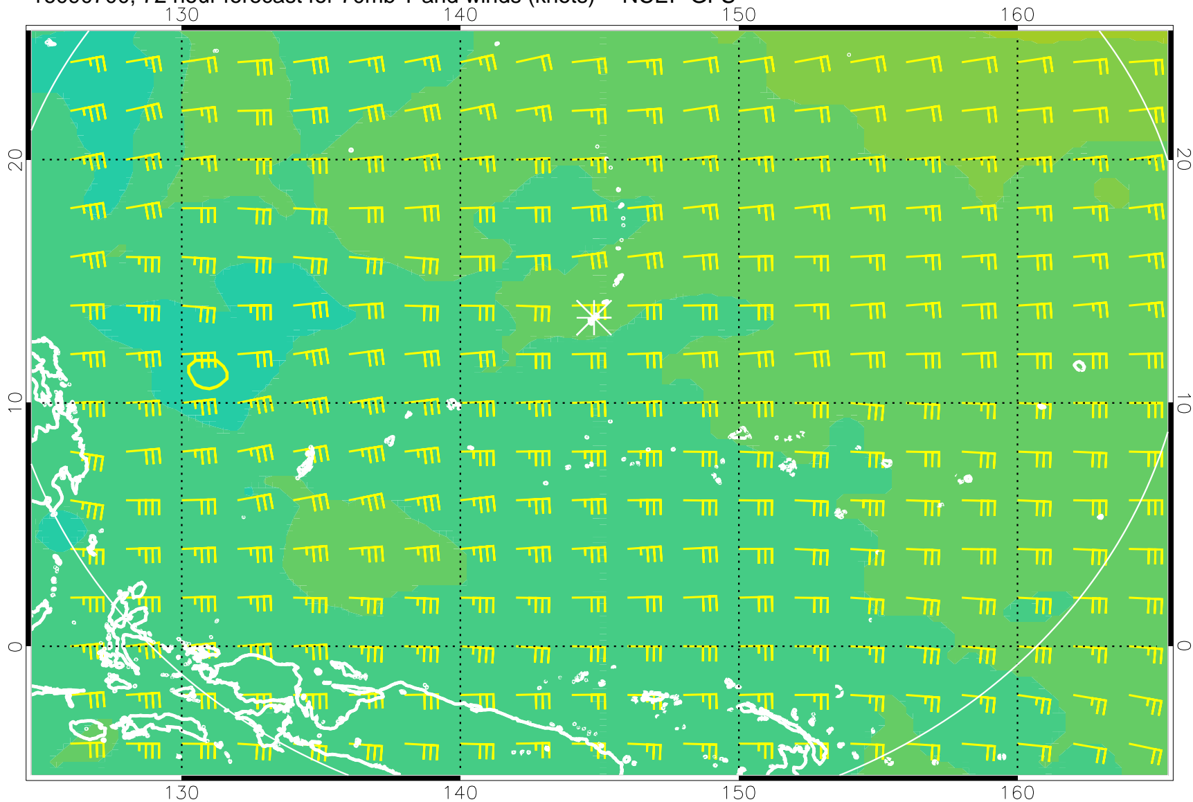
16090700, 72 hour forecast for 70mb T and winds (knots) -- NCEP GFS
