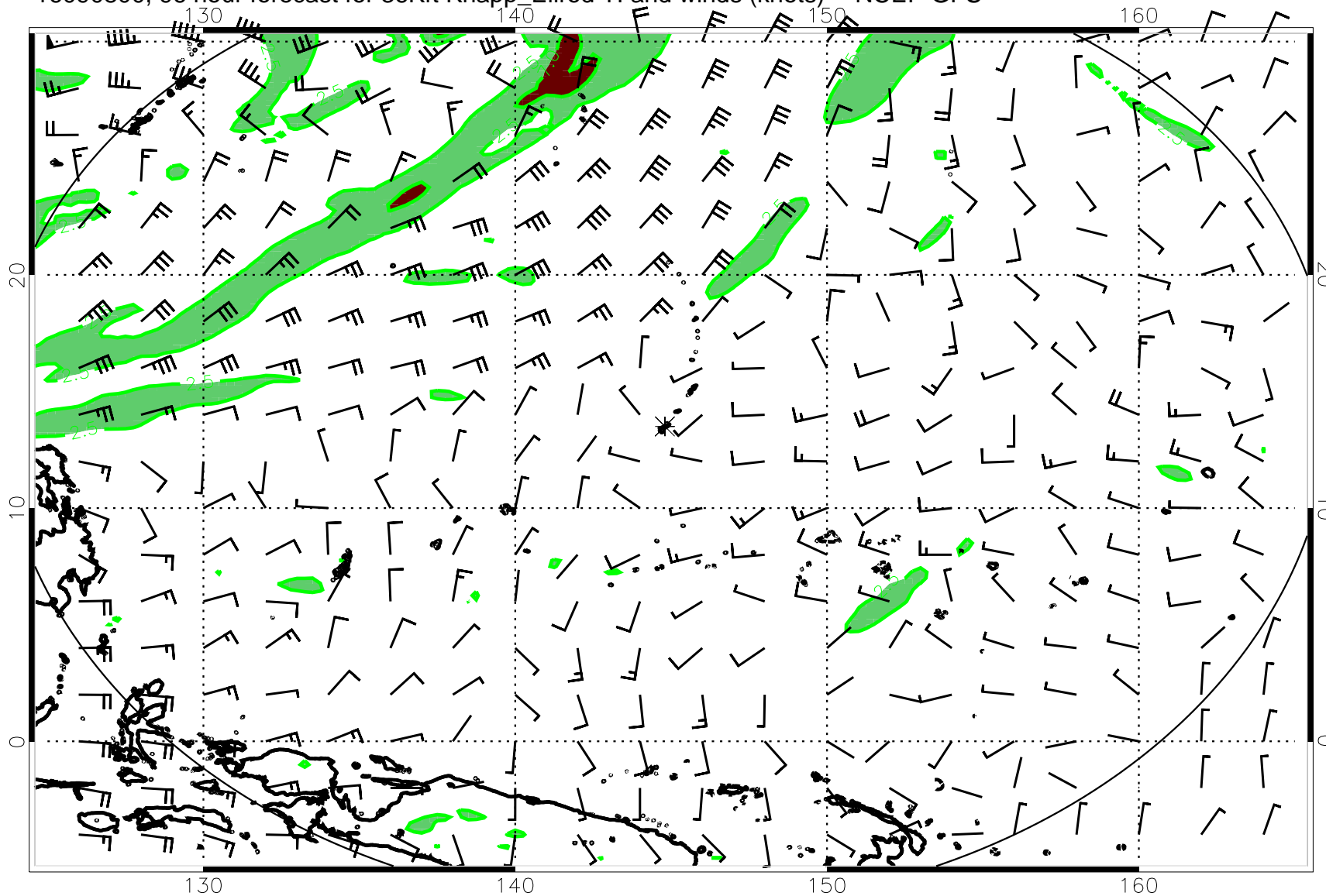
16090800, 96 hour forecast for 36Kft Knapp_Ellrod TI and winds (knots) -- NCEP GFS
