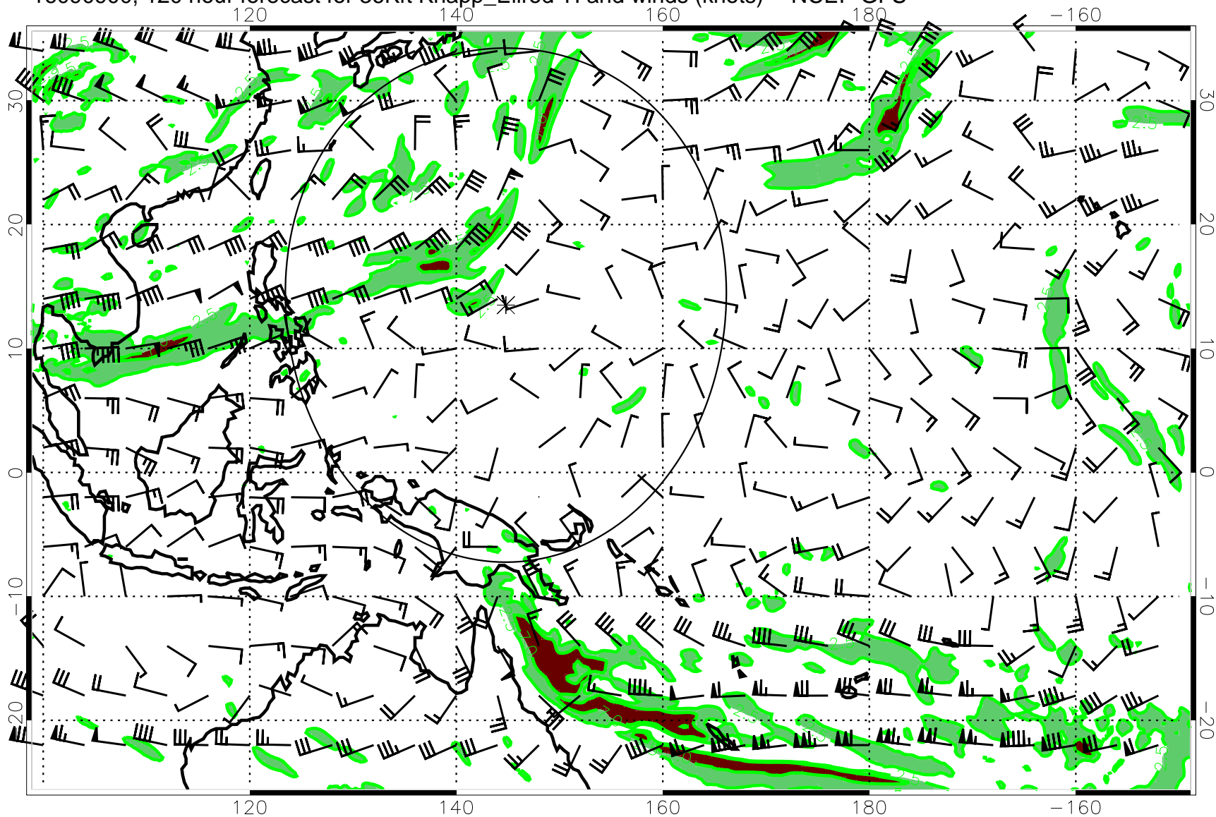
16090900, 120 hour forecast for 36Kft Knapp_Ellrod TI and winds (knots) -- NCEP GFS
