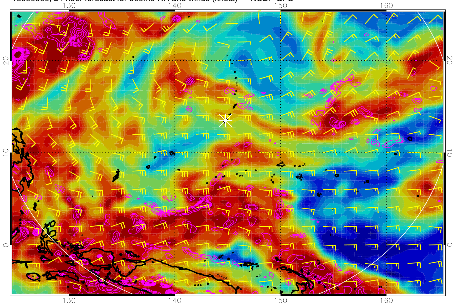
16090500, 24 hour forecast for 500mb RH and winds (knots) -- NCEP GFS
