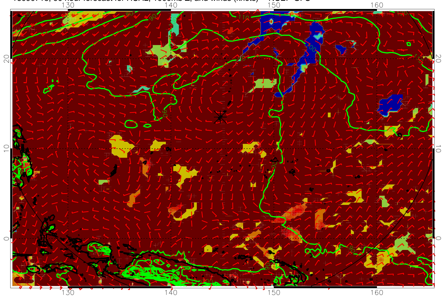
16090718, 90 hour forecast for HCAL, 1000mb Z, and winds (knots) -- NCEP GFS
