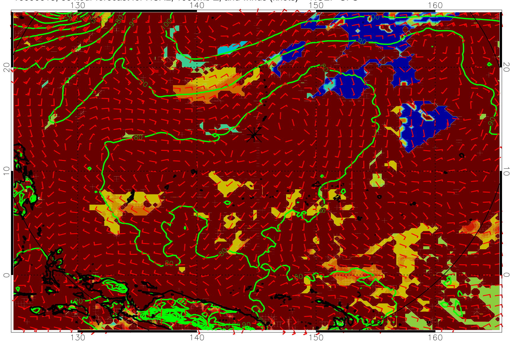
16090618, 66 hour forecast for HCAL, 1000mb Z, and winds (knots) -- NCEP GFS
