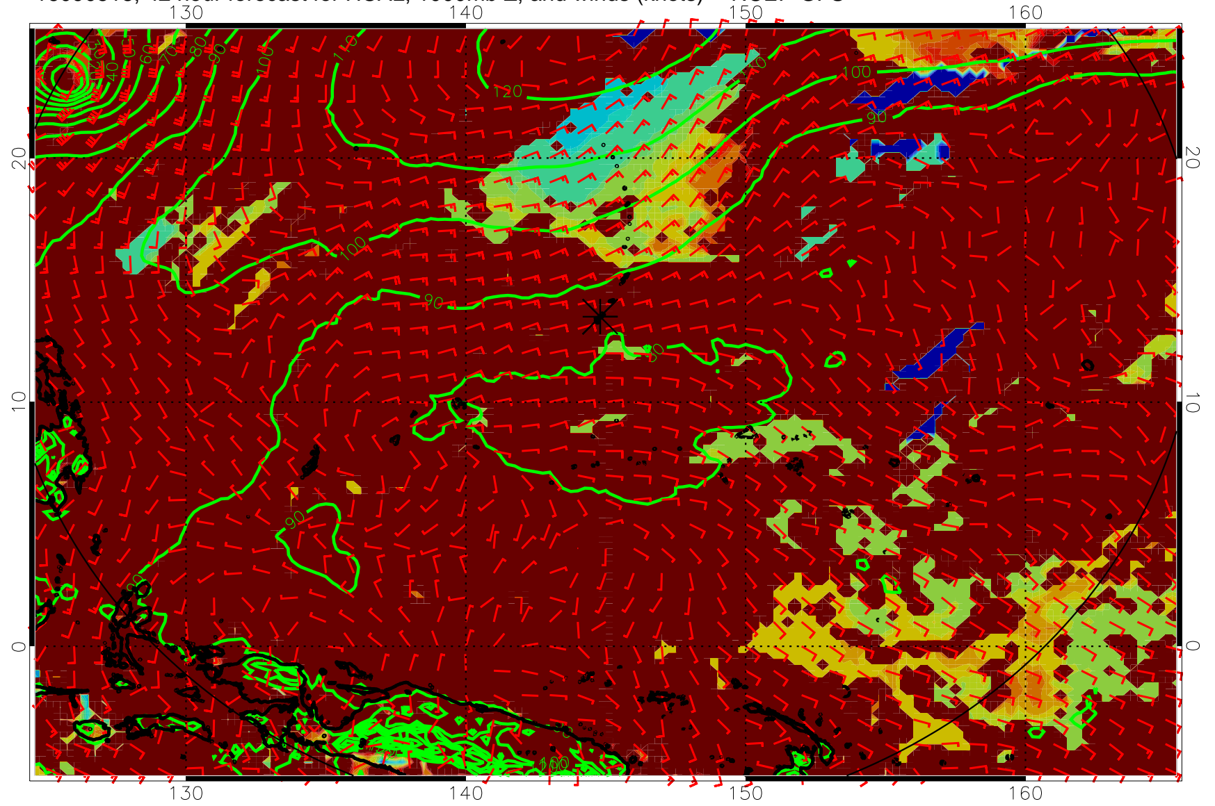
16090518, 42 hour forecast for HCAL, 1000mb Z, and winds (knots) -- NCEP GFS
