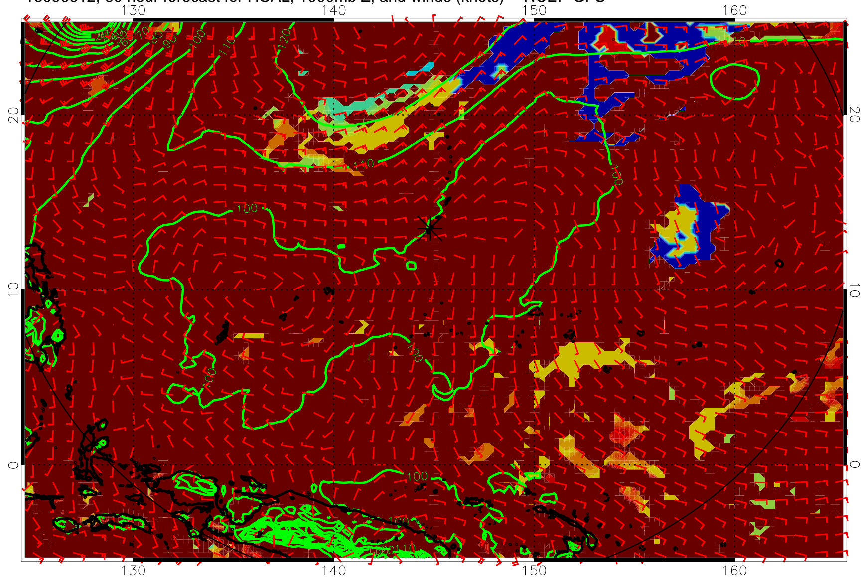
16090612, 60 hour forecast for HCAL, 1000mb Z, and winds (knots) -- NCEP GFS
