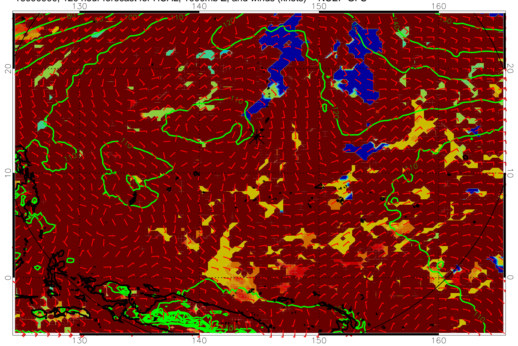
16090900, 120 hour forecast for HCAL, 1000mb Z, and winds (knots) -- NCEP GFS
