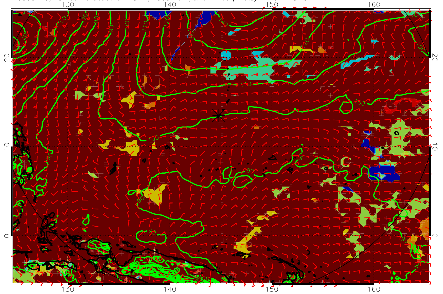
16090418, 18 hour forecast for HCAL, 1000mb Z, and winds (knots) -- NCEP GFS
