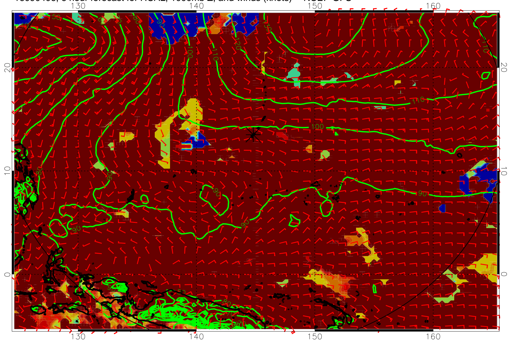
16090406, 6 hour forecast for HCAL, 1000mb Z, and winds (knots) -- NCEP GFS
