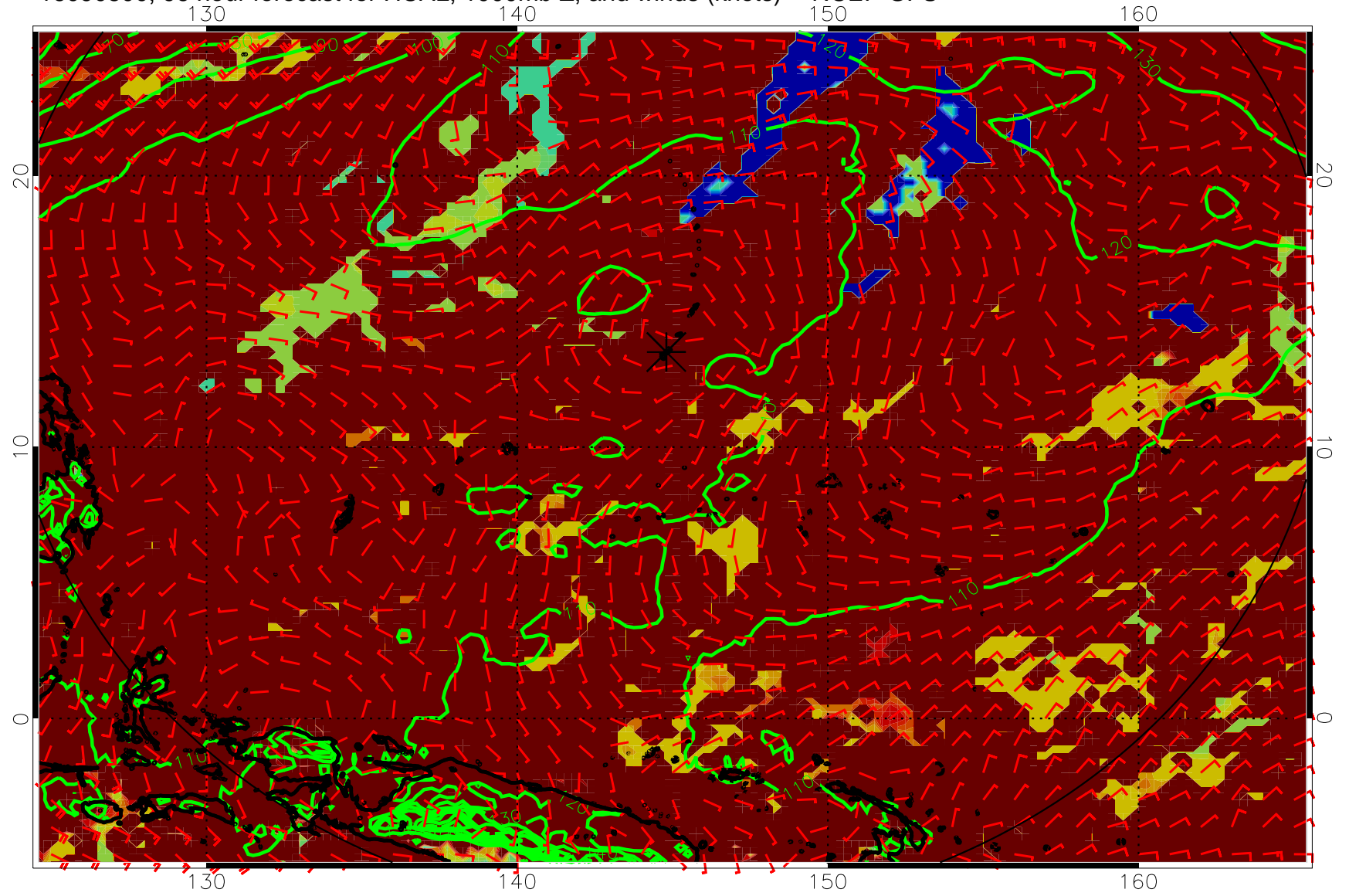
16090800, 96 hour forecast for HCAL, 1000mb Z, and winds (knots) -- NCEP GFS
