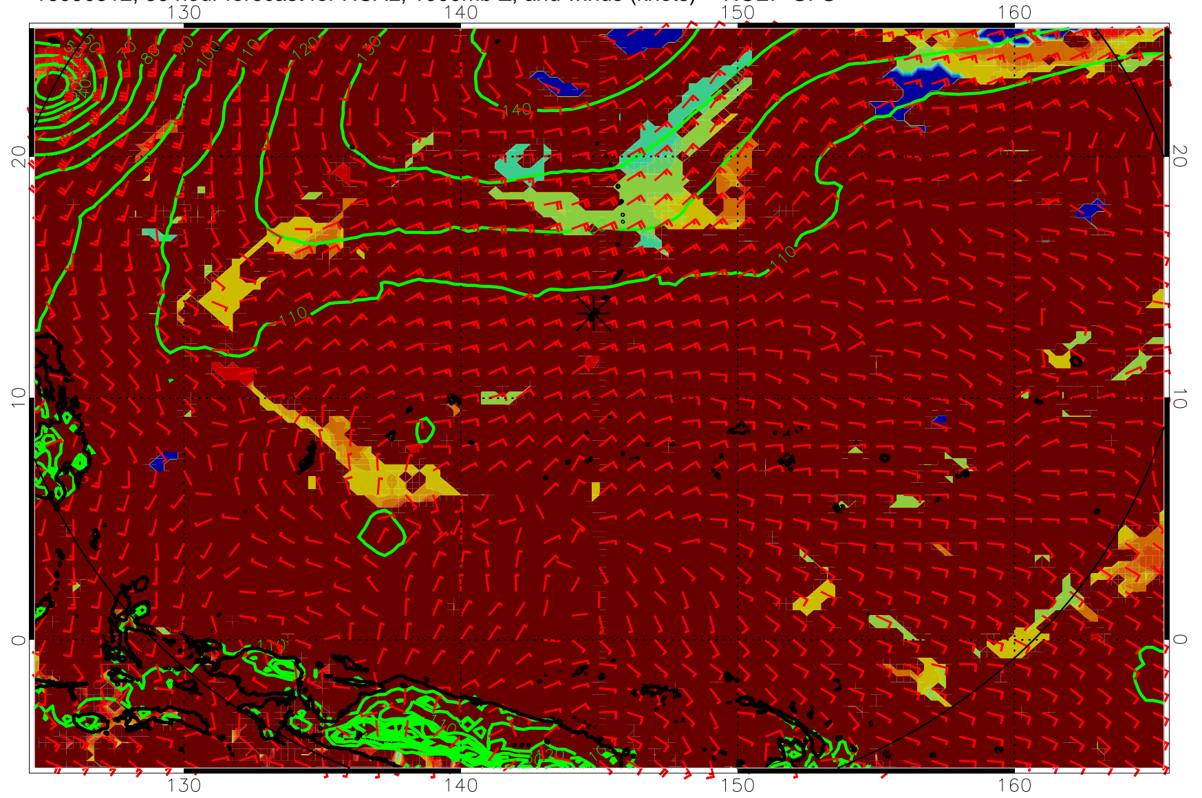
16090512, 36 hour forecast for HCAL, 1000mb Z, and winds (knots) -- NCEP GFS
