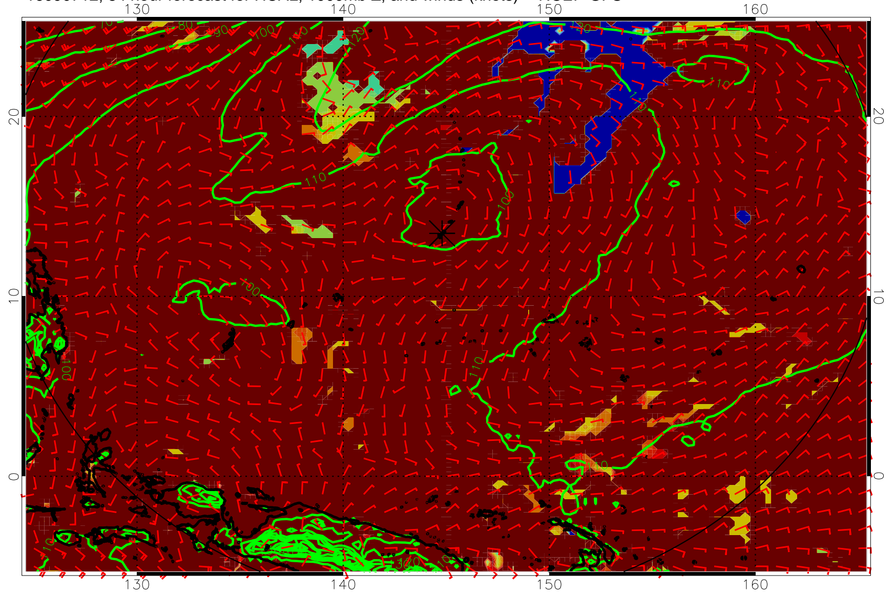
16090712, 84 hour forecast for HCAL, 1000mb Z, and winds (knots) -- NCEP GFS
