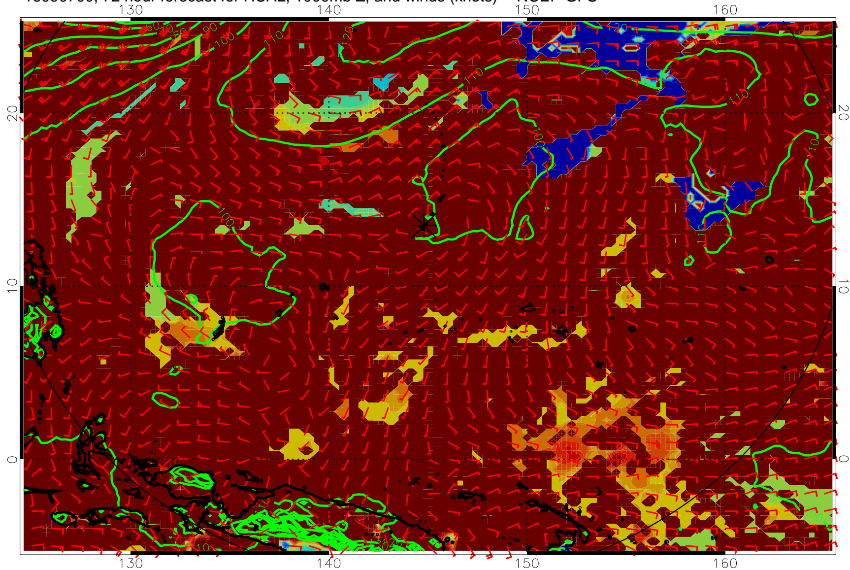
16090700, 72 hour forecast for HCAL, 1000mb Z, and winds (knots) -- NCEP GFS
