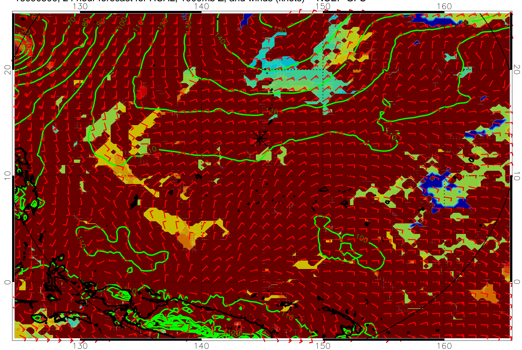
16090500, 24 hour forecast for HCAL, 1000mb Z, and winds (knots) -- NCEP GFS
