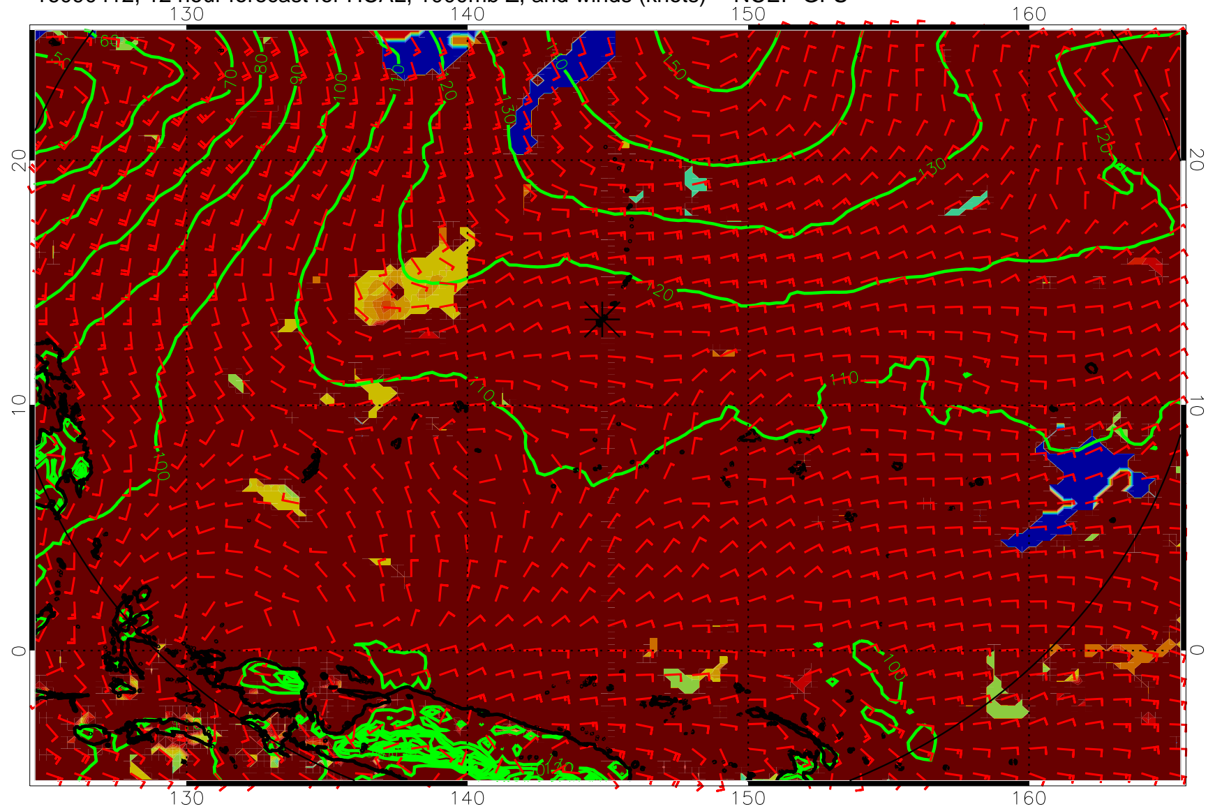
16090412, 12 hour forecast for HCAL, 1000mb Z, and winds (knots) -- NCEP GFS
