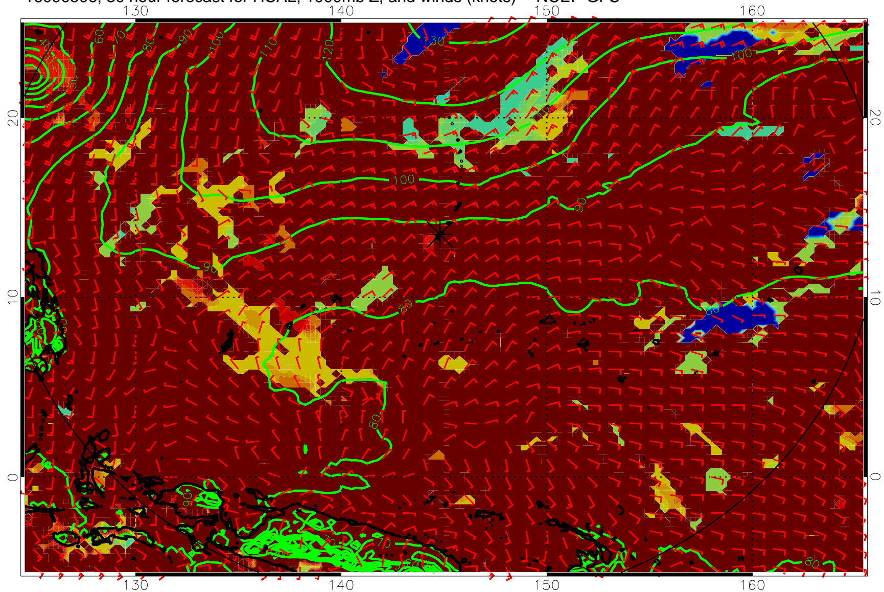
16090506, 30 hour forecast for HCAL, 1000mb Z, and winds (knots) -- NCEP GFS
