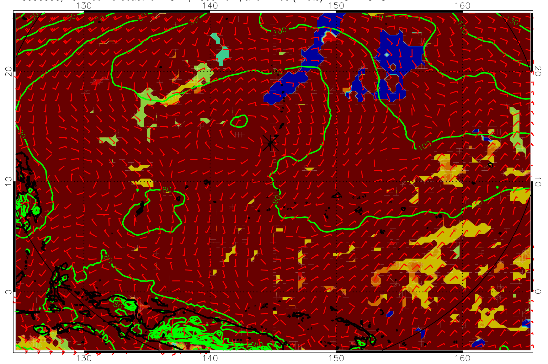
16090806, 102 hour forecast for HCAL, 1000mb Z, and winds (knots) -- NCEP GFS
