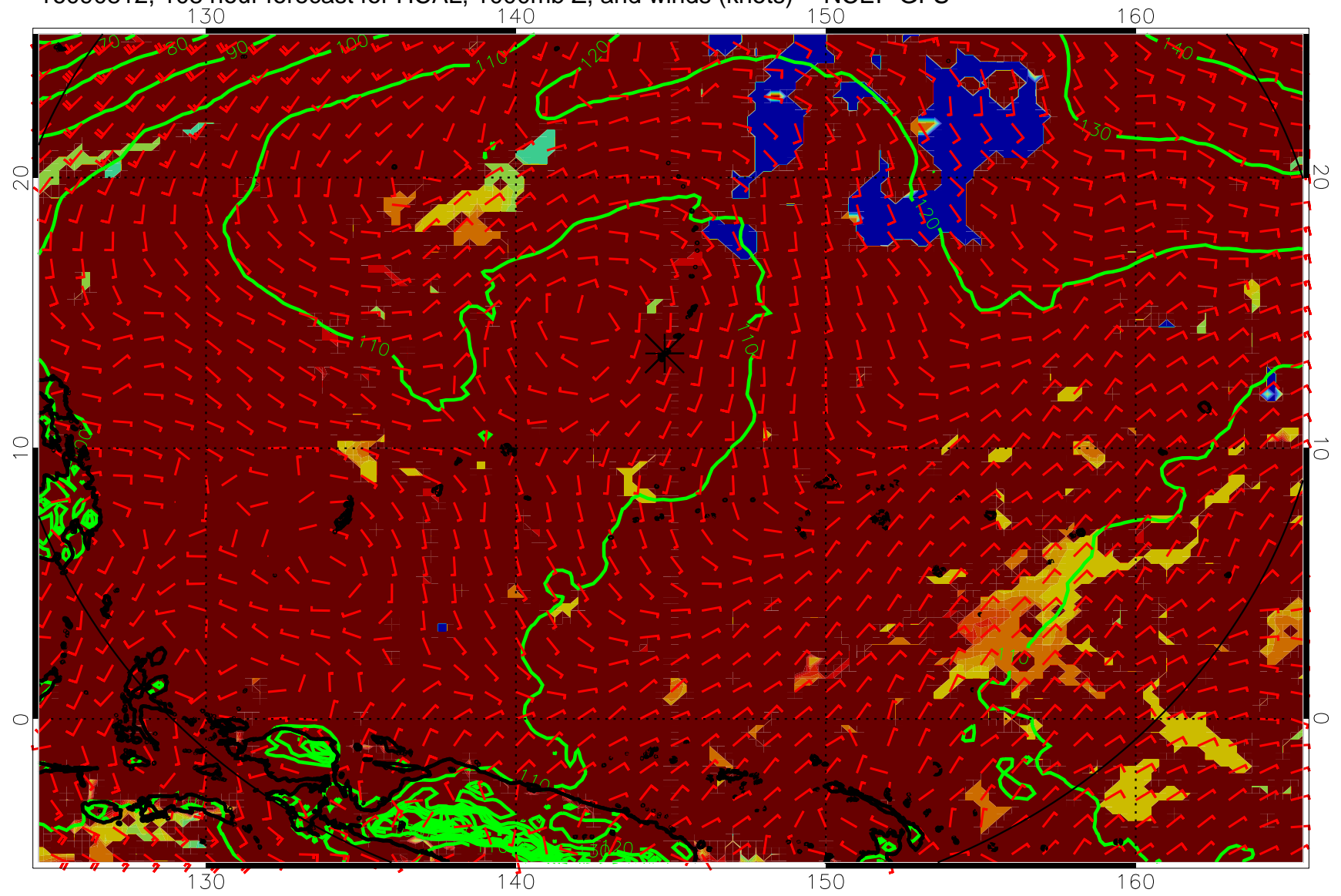
16090812, 108 hour forecast for HCAL, 1000mb Z, and winds (knots) -- NCEP GFS
