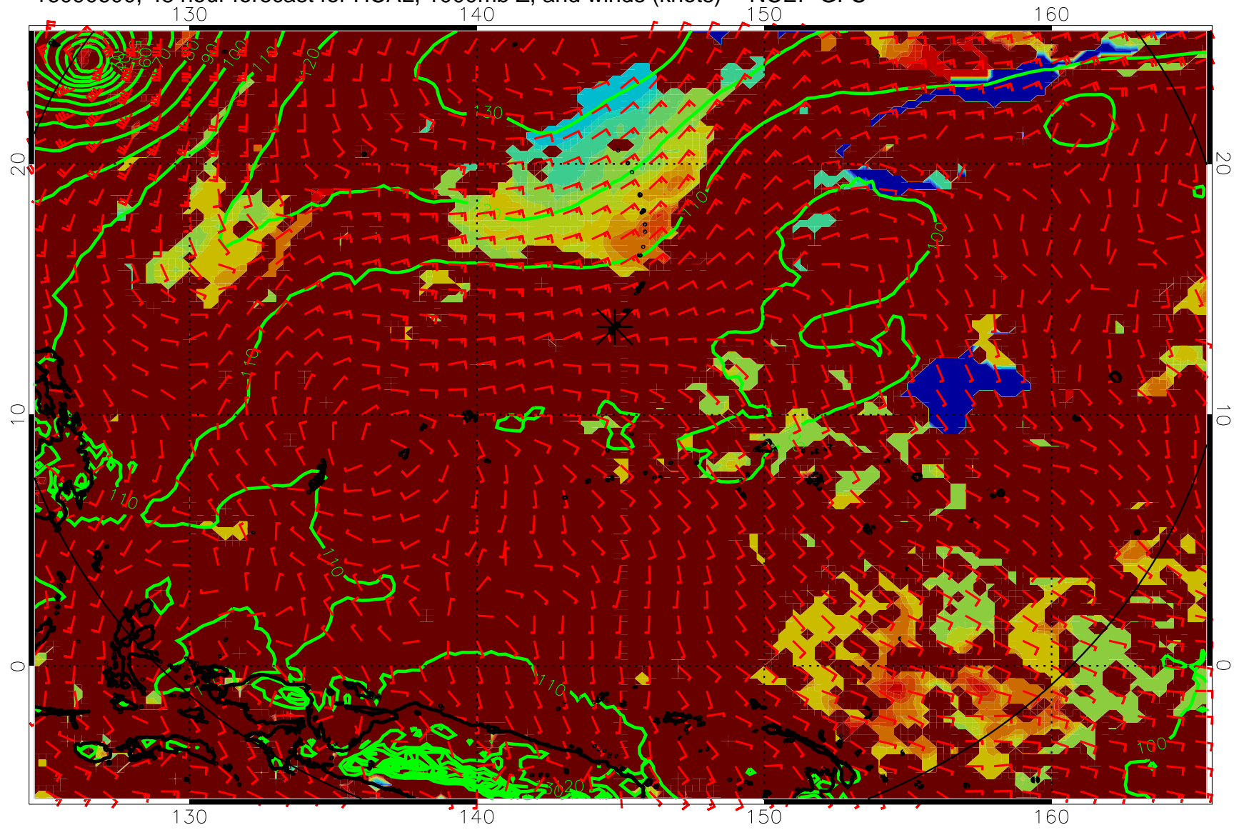
16090600, 48 hour forecast for HCAL, 1000mb Z, and winds (knots) -- NCEP GFS
