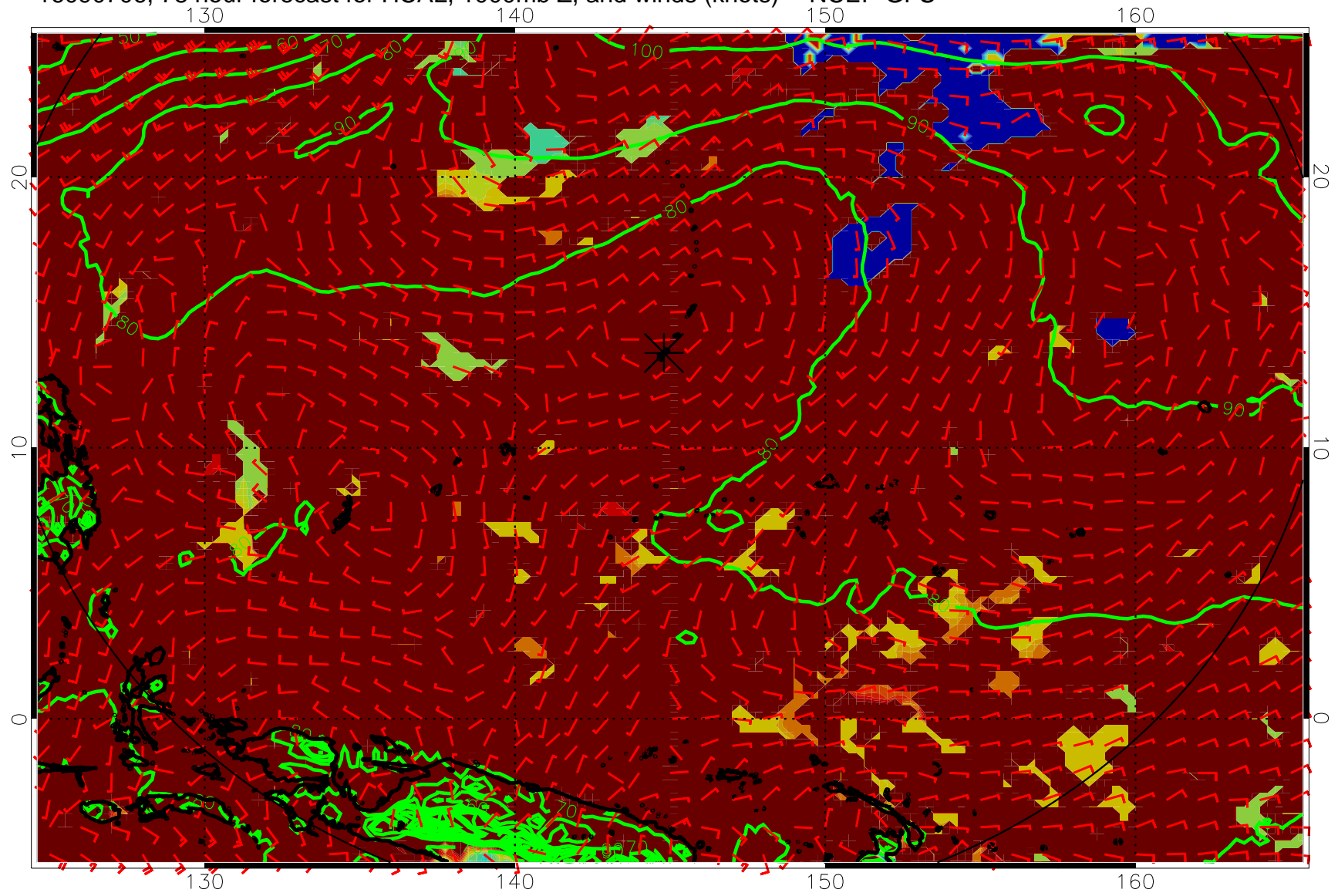
16090706, 78 hour forecast for HCAL, 1000mb Z, and winds (knots) -- NCEP GFS
