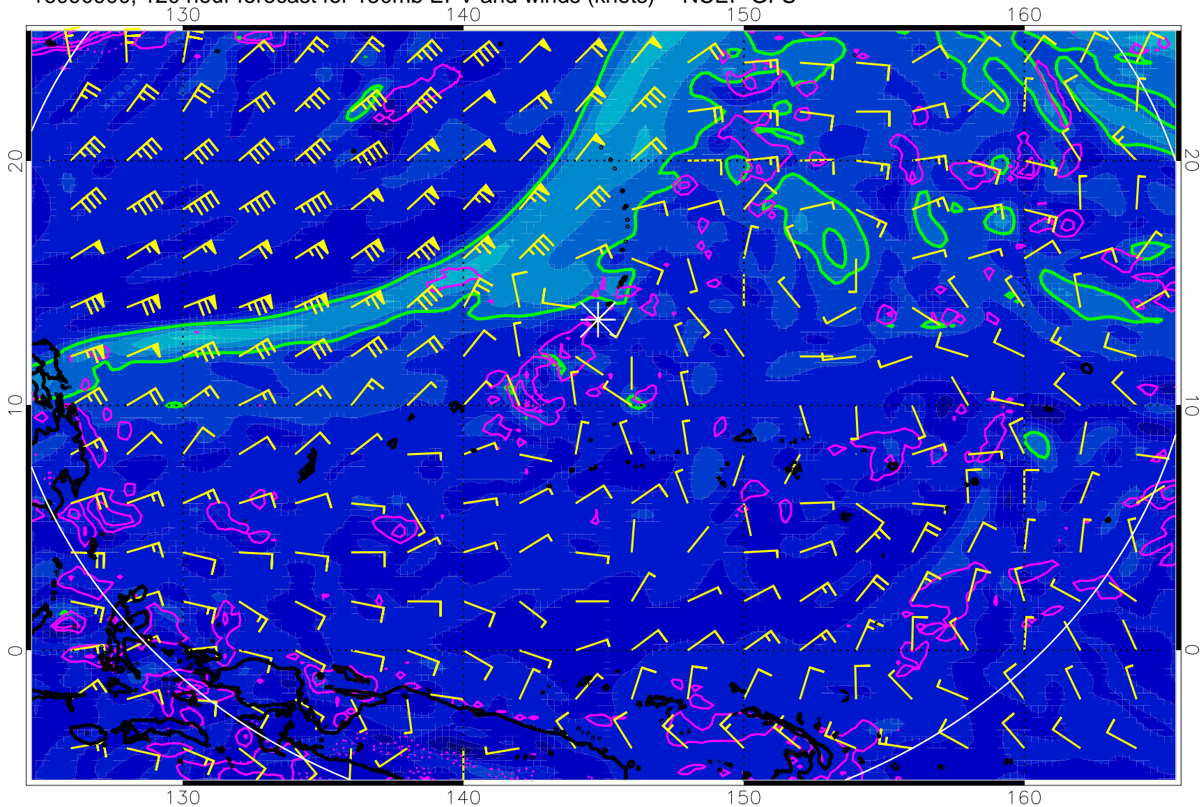
16090900, 120 hour forecast for 150mb EPV and winds (knots) -- NCEP GFS
