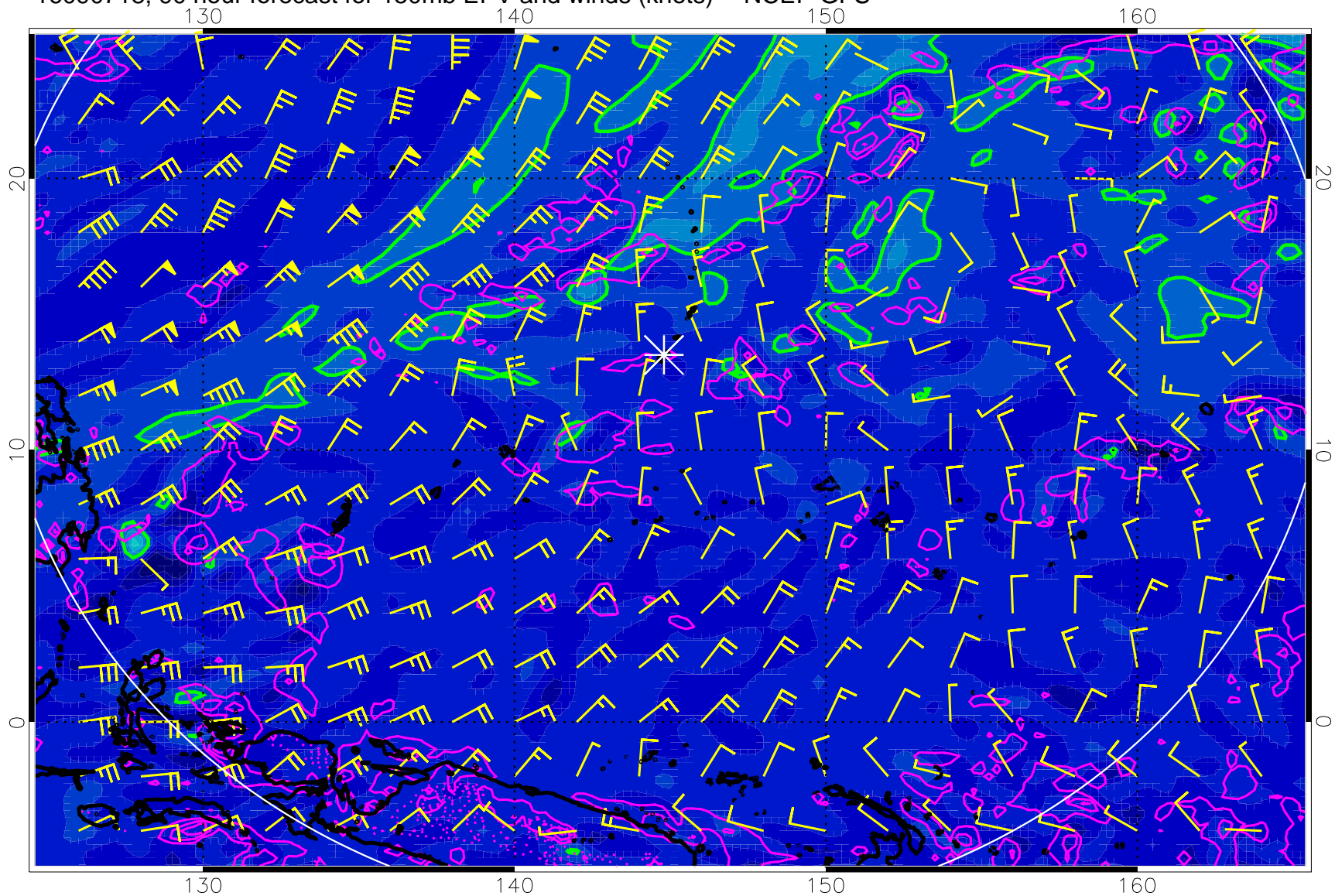
16090718, 90 hour forecast for 150mb EPV and winds (knots) -- NCEP GFS
