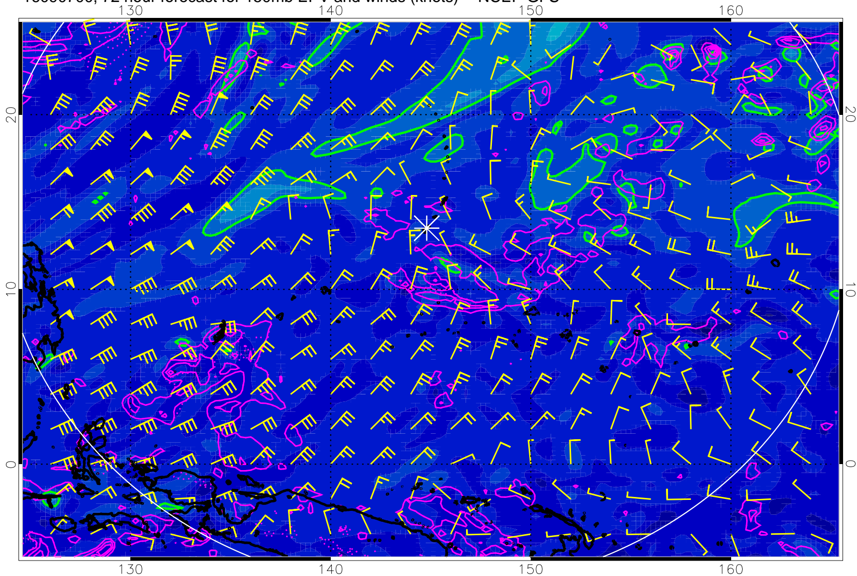
16090700, 72 hour forecast for 150mb EPV and winds (knots) -- NCEP GFS
