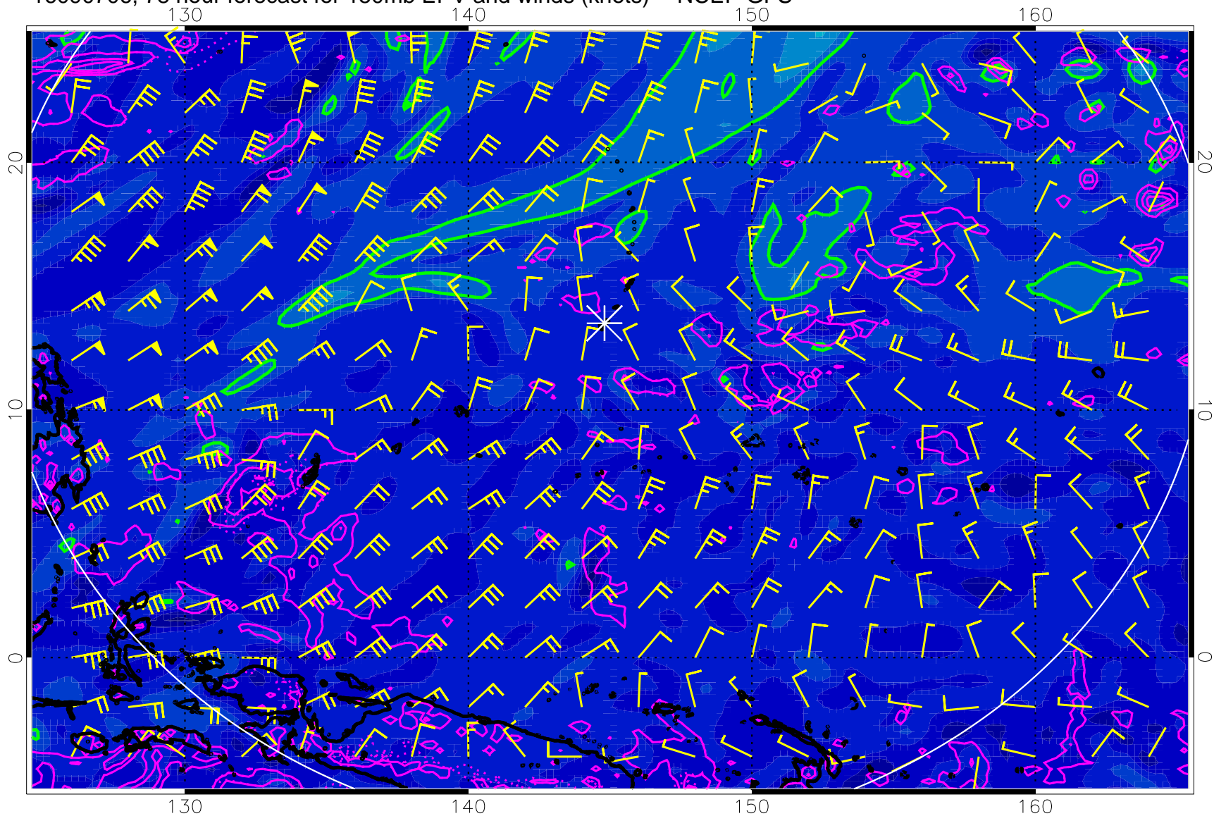
16090706, 78 hour forecast for 150mb EPV and winds (knots) -- NCEP GFS
