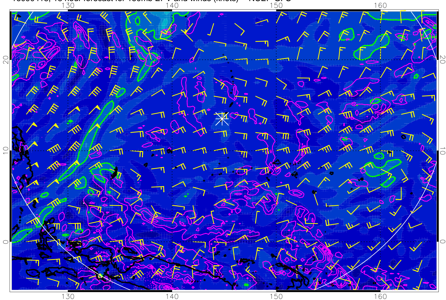
16090418, 18 hour forecast for 150mb EPV and winds (knots) -- NCEP GFS
