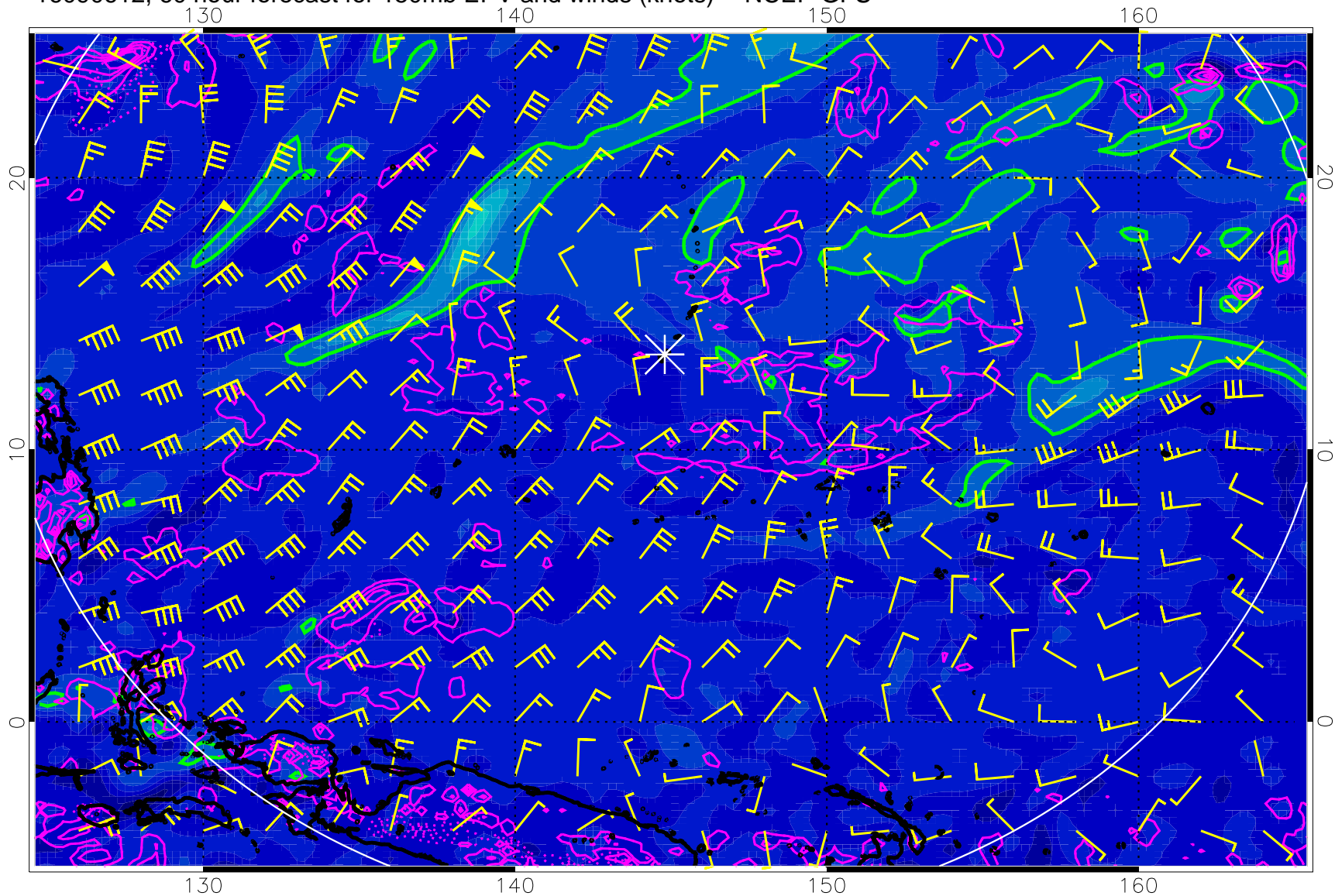
16090612, 60 hour forecast for 150mb EPV and winds (knots) -- NCEP GFS
