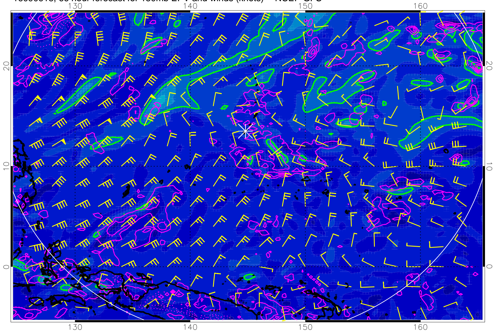
16090618, 66 hour forecast for 150mb EPV and winds (knots) -- NCEP GFS
