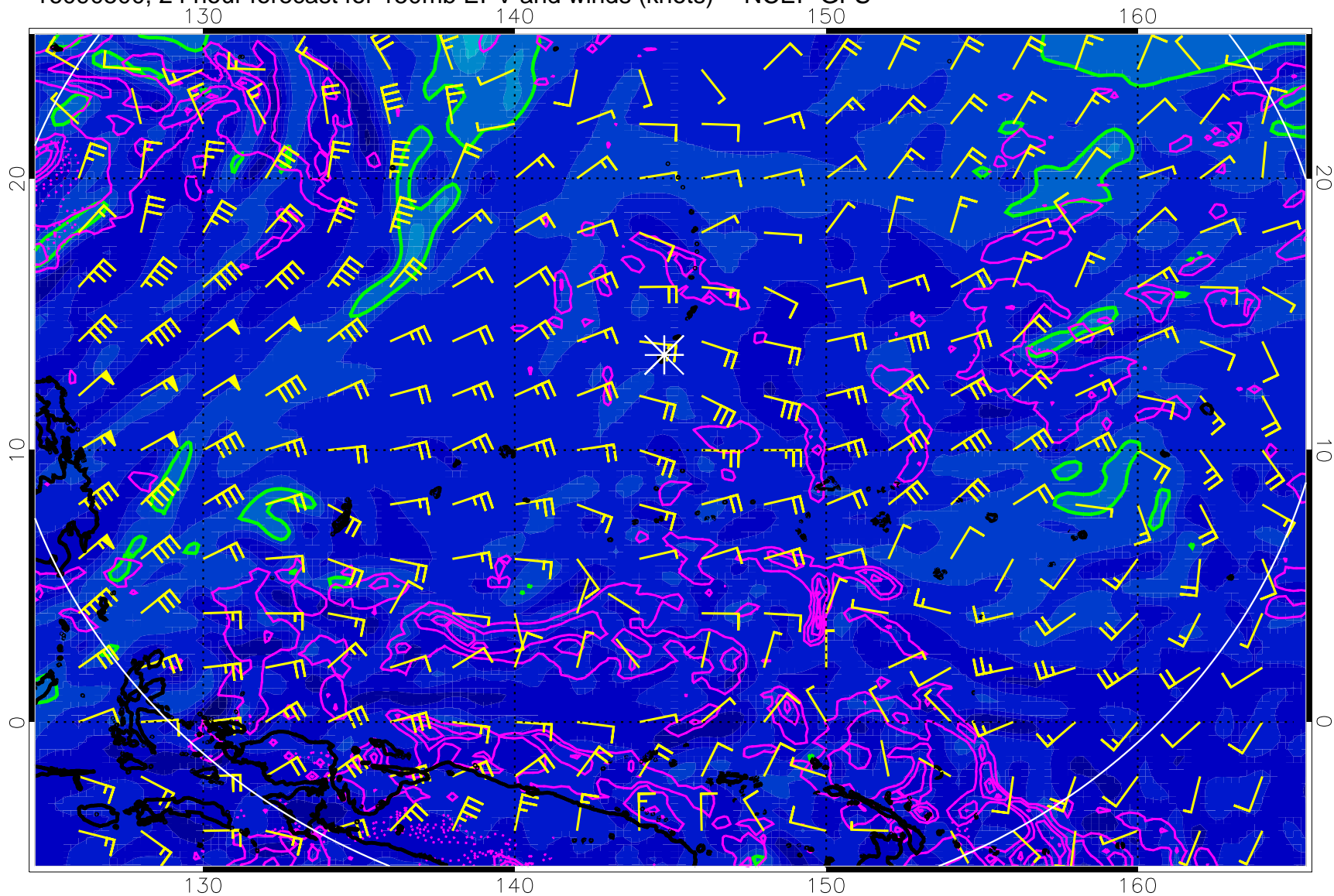
16090500, 24 hour forecast for 150mb EPV and winds (knots) -- NCEP GFS
