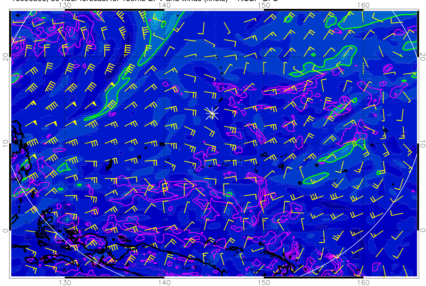
16090506, 30 hour forecast for 150mb EPV and winds (knots) -- NCEP GFS
