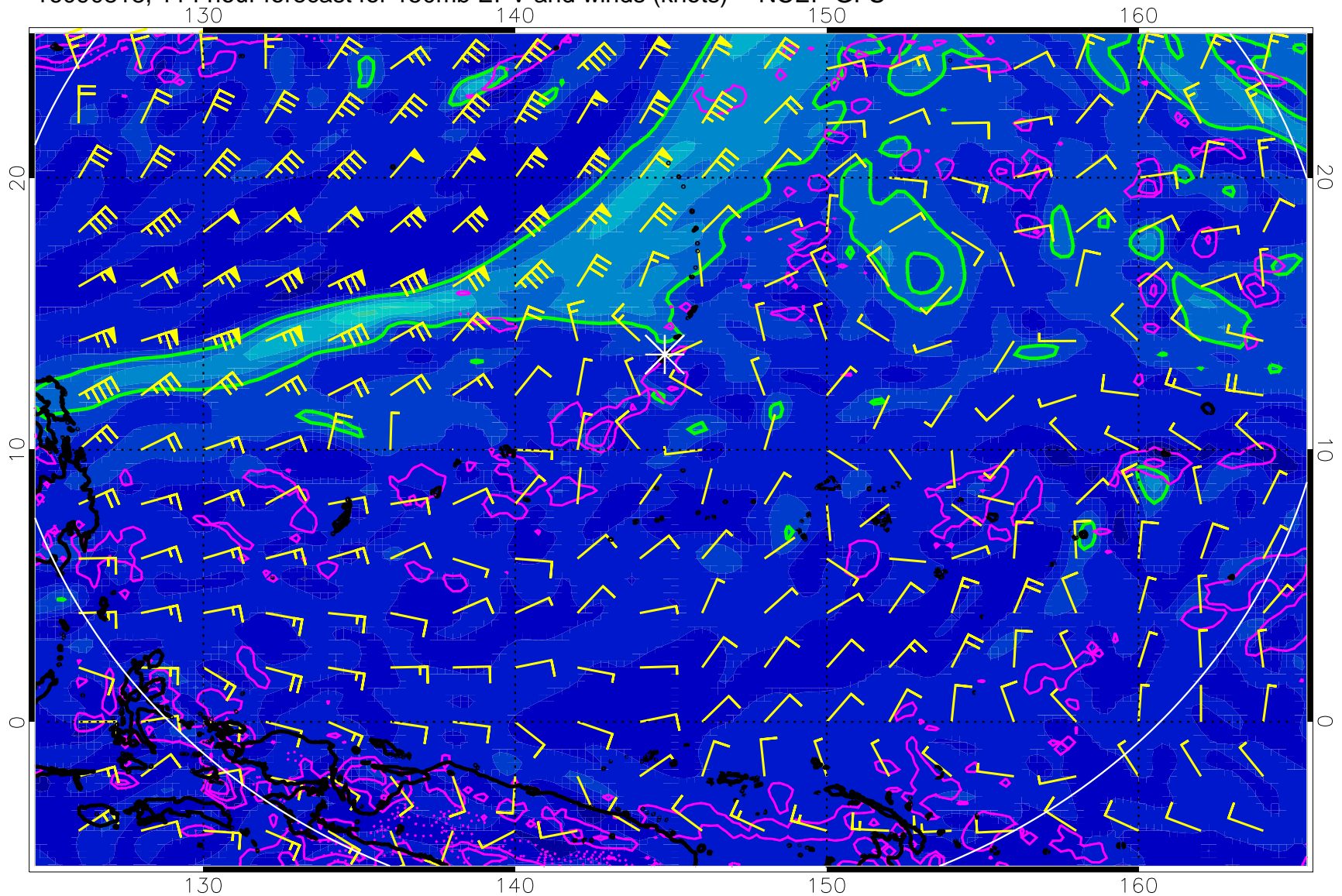
16090818, 114 hour forecast for 150mb EPV and winds (knots) -- NCEP GFS
