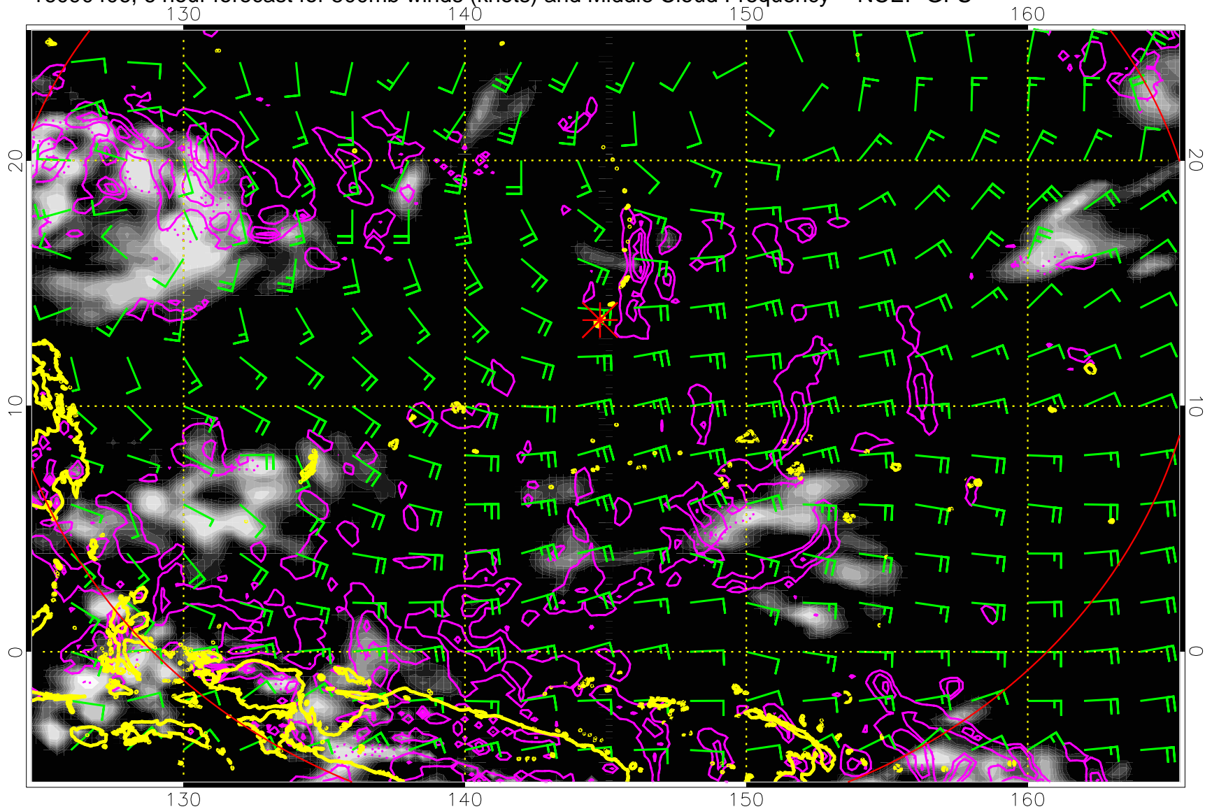
16090406, 6 hour forecast for 500mb winds (knots) and Middle Cloud Frequency -- NCEP GFS
