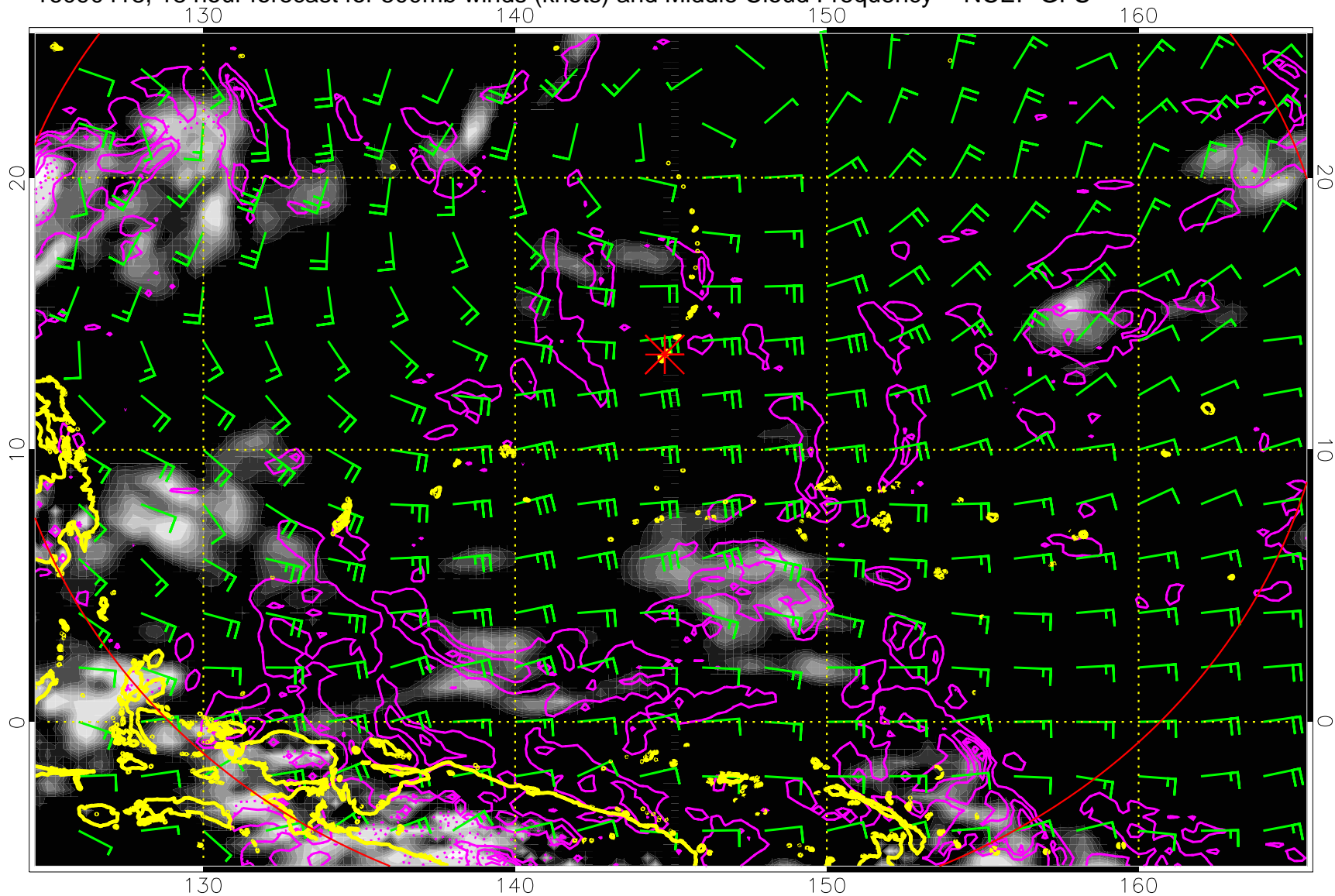
16090418, 18 hour forecast for 500mb winds (knots) and Middle Cloud Frequency -- NCEP GFS
