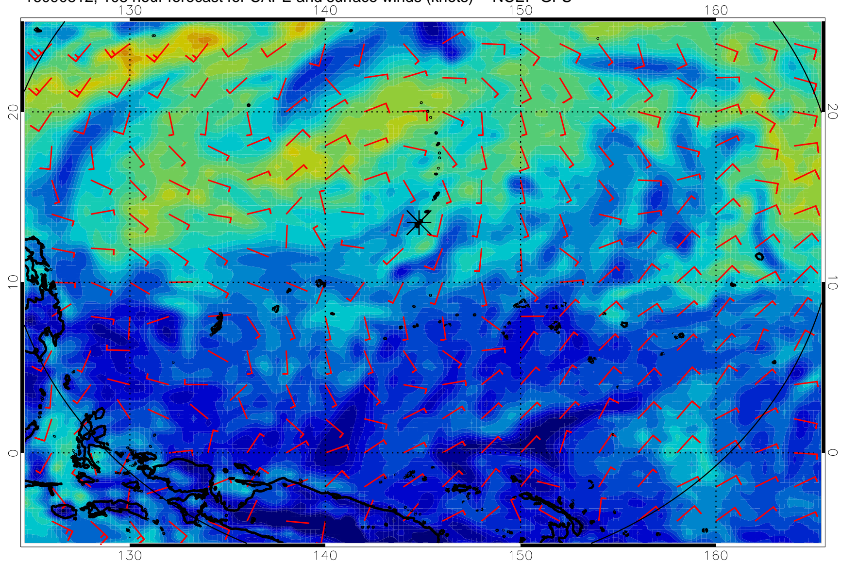
16090812, 108 hour forecast for CAPE and surface winds (knots) -- NCEP GFS
