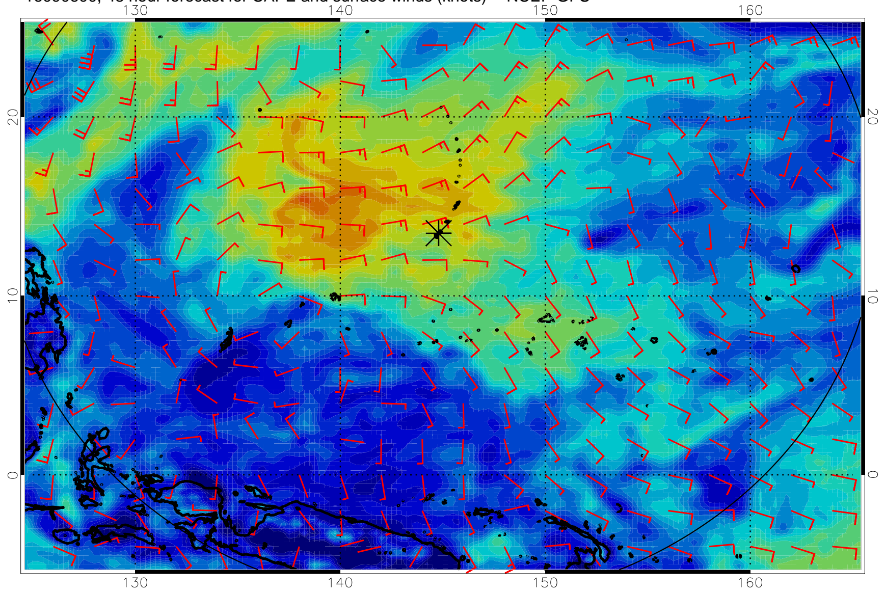
16090600, 48 hour forecast for CAPE and surface winds (knots) -- NCEP GFS
