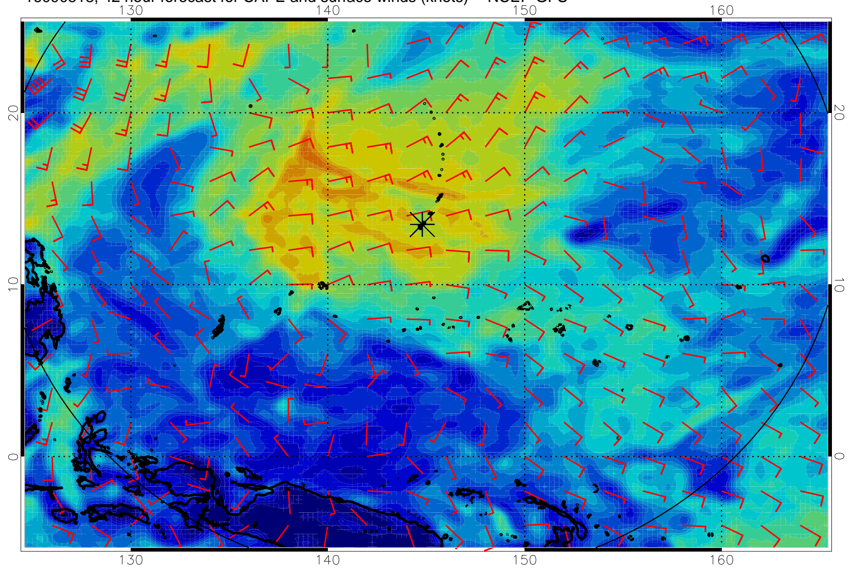
16090518, 42 hour forecast for CAPE and surface winds (knots) -- NCEP GFS
