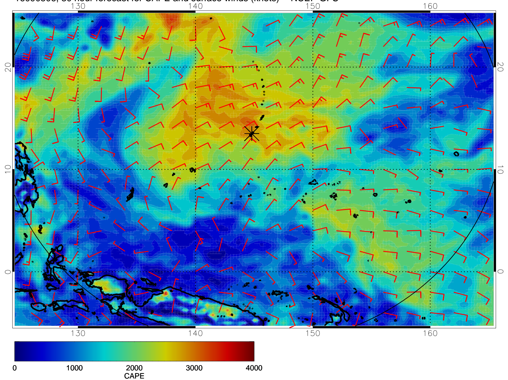
16090506, 30 hour forecast for CAPE and surface winds (knots) -- NCEP GFS
