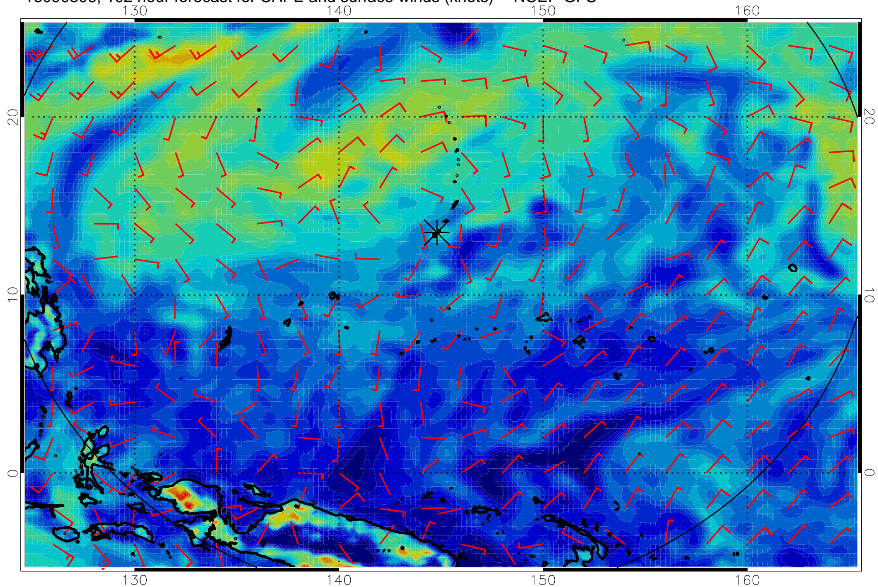
16090806, 102 hour forecast for CAPE and surface winds (knots) -- NCEP GFS
