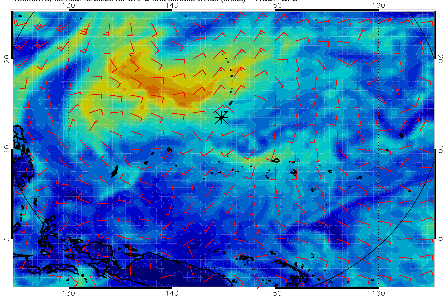
16090618, 66 hour forecast for CAPE and surface winds (knots) -- NCEP GFS
