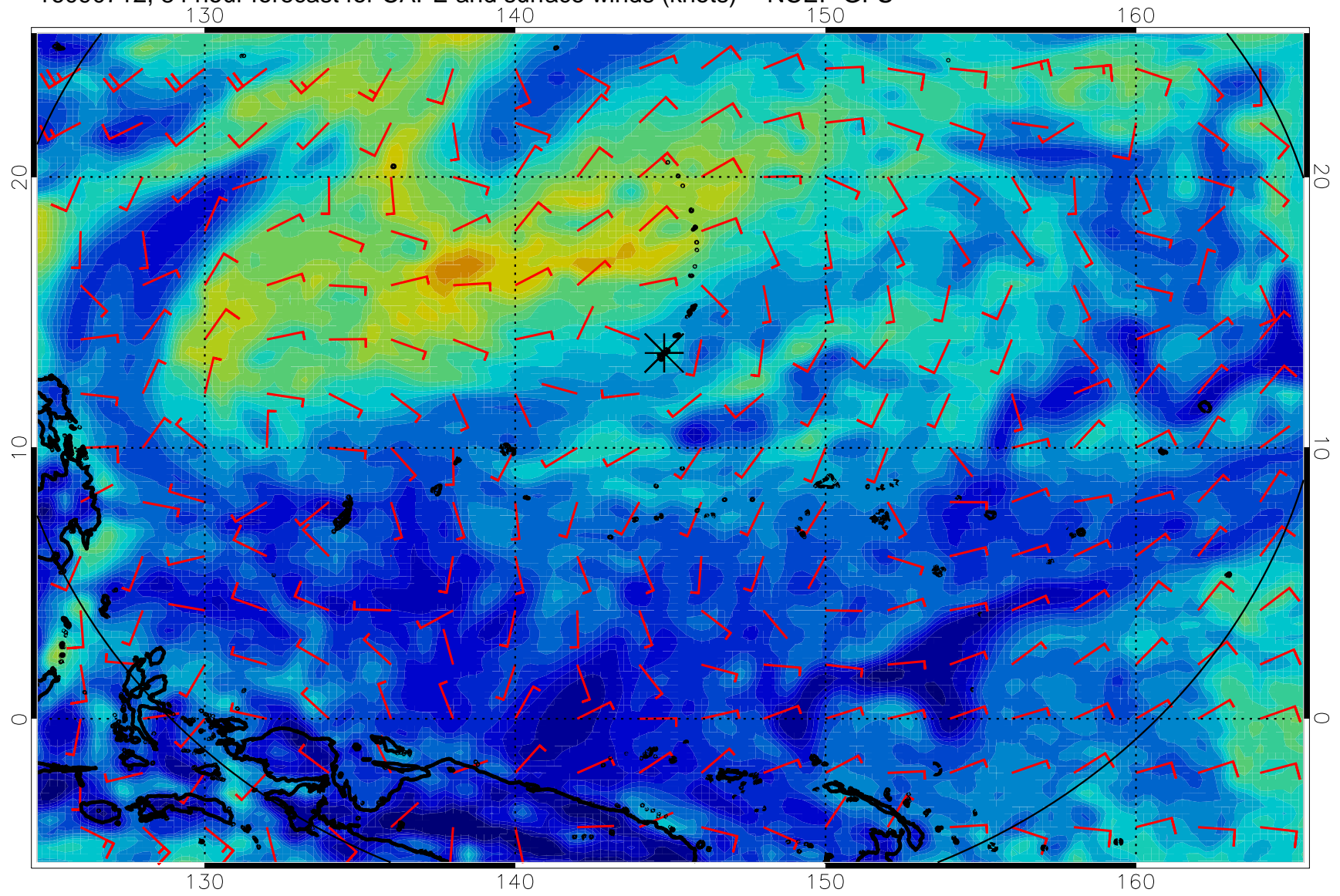
16090712, 84 hour forecast for CAPE and surface winds (knots) -- NCEP GFS
