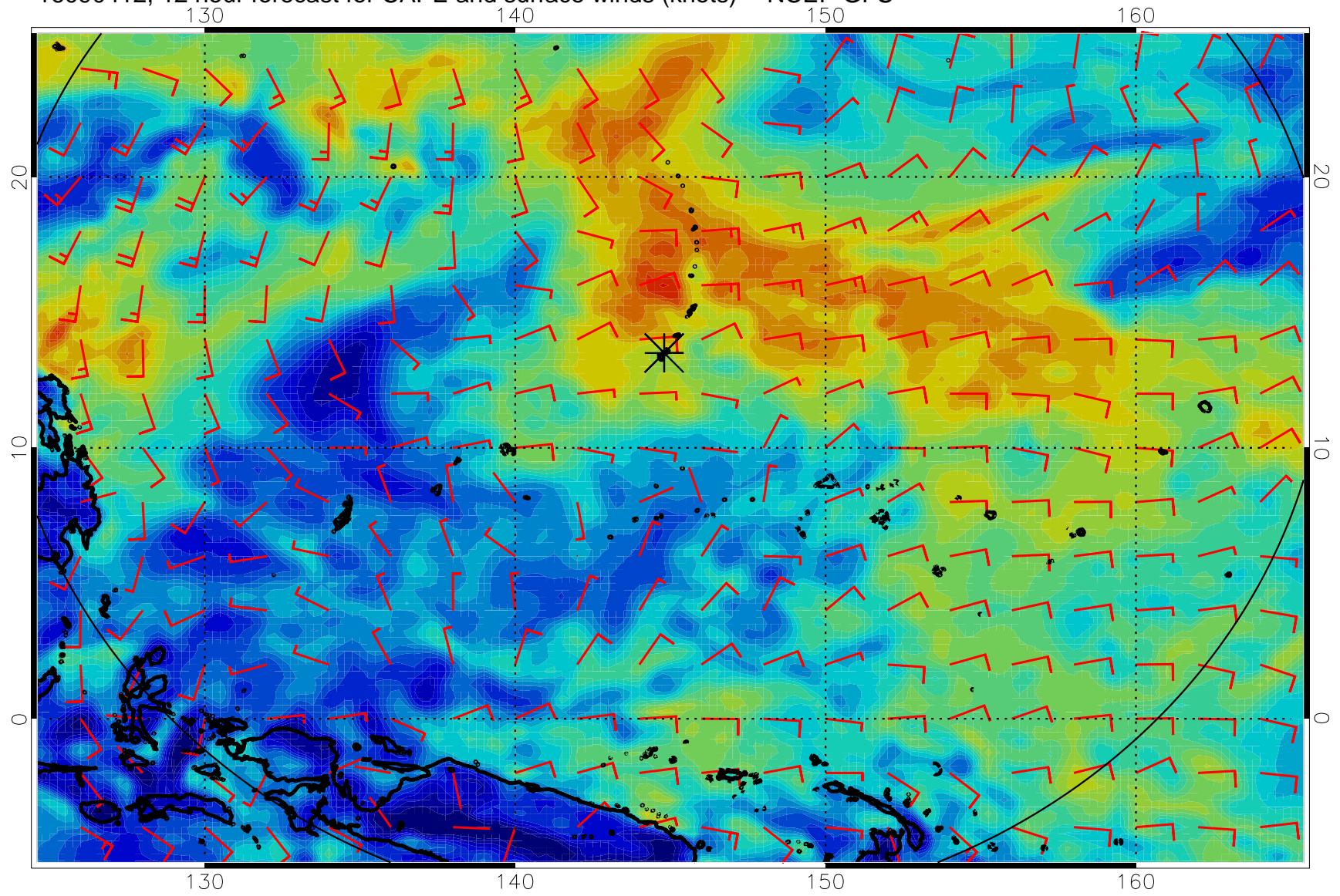
16090412, 12 hour forecast for CAPE and surface winds (knots) -- NCEP GFS
