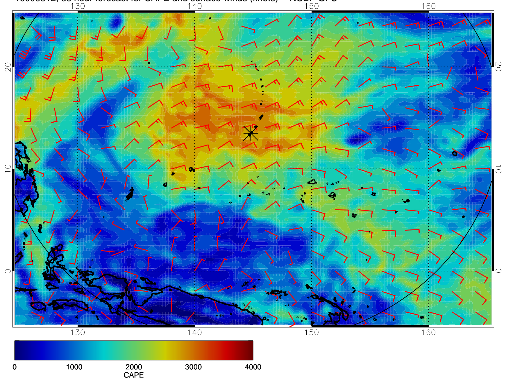
16090512, 36 hour forecast for CAPE and surface winds (knots) -- NCEP GFS
