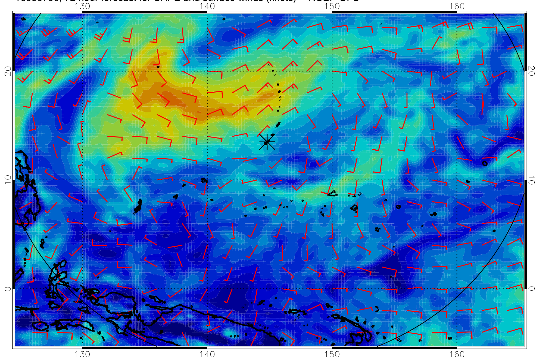
16090700, 72 hour forecast for CAPE and surface winds (knots) -- NCEP GFS
