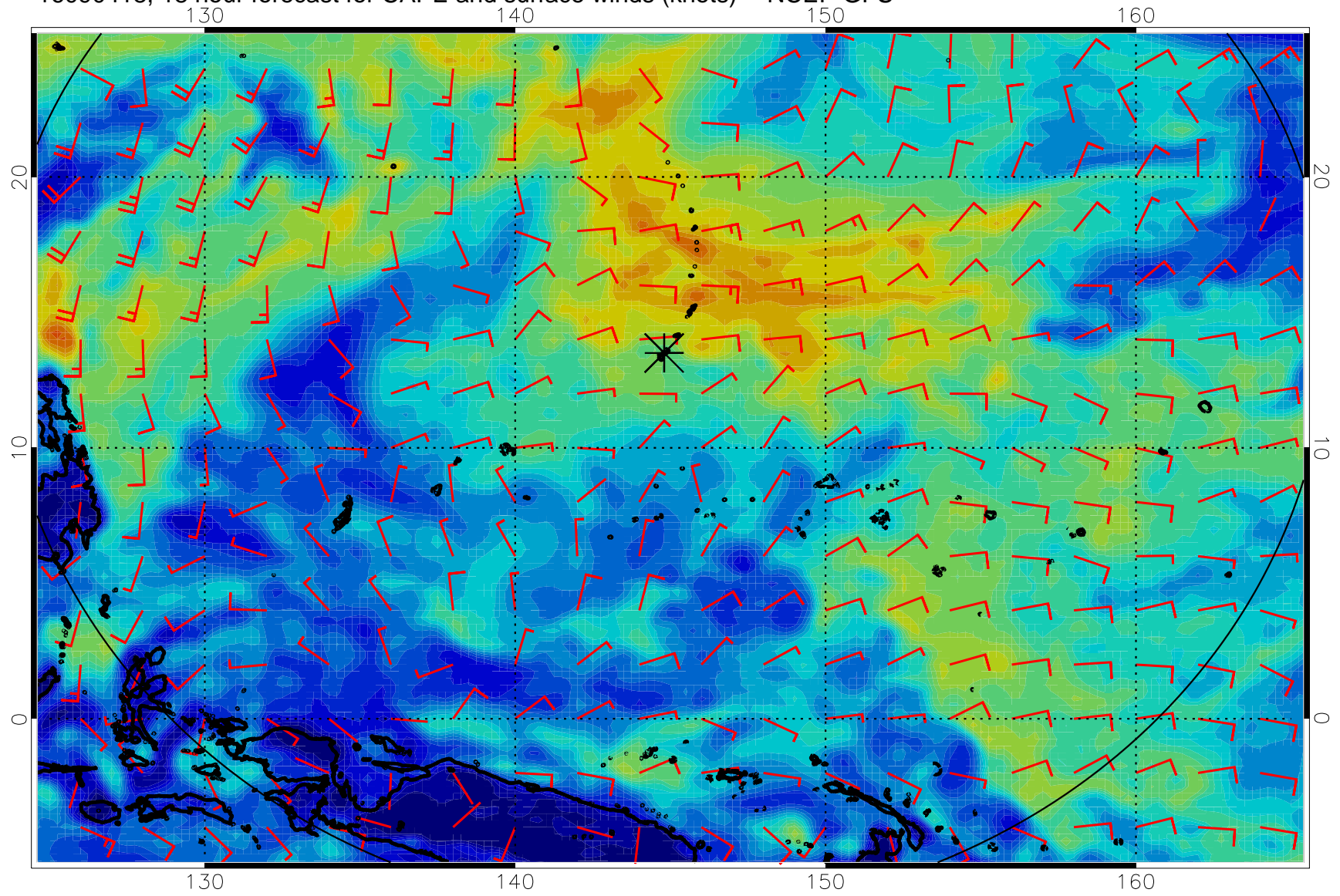
16090418, 18 hour forecast for CAPE and surface winds (knots) -- NCEP GFS
