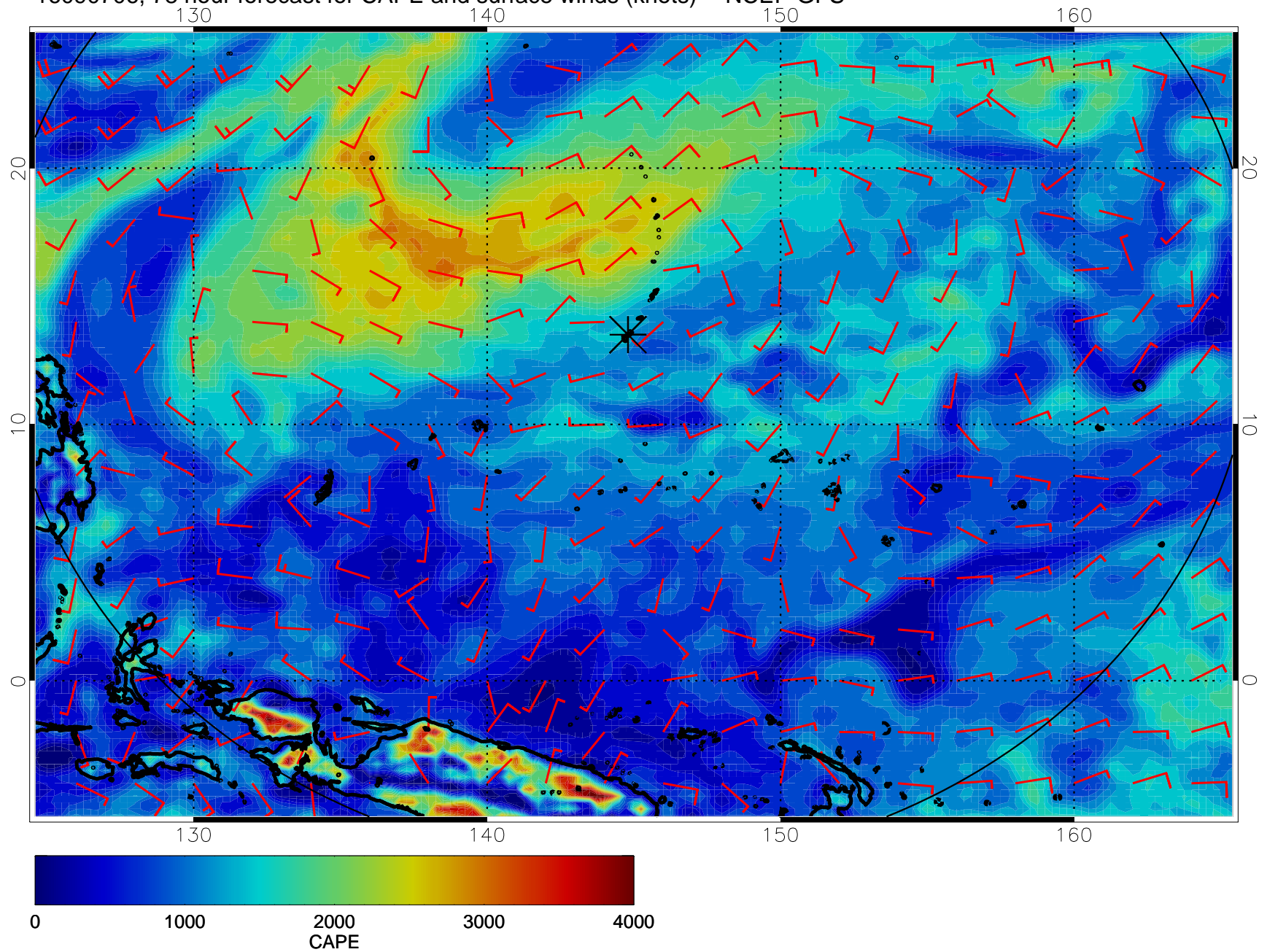
16090706, 78 hour forecast for CAPE and surface winds (knots) -- NCEP GFS
