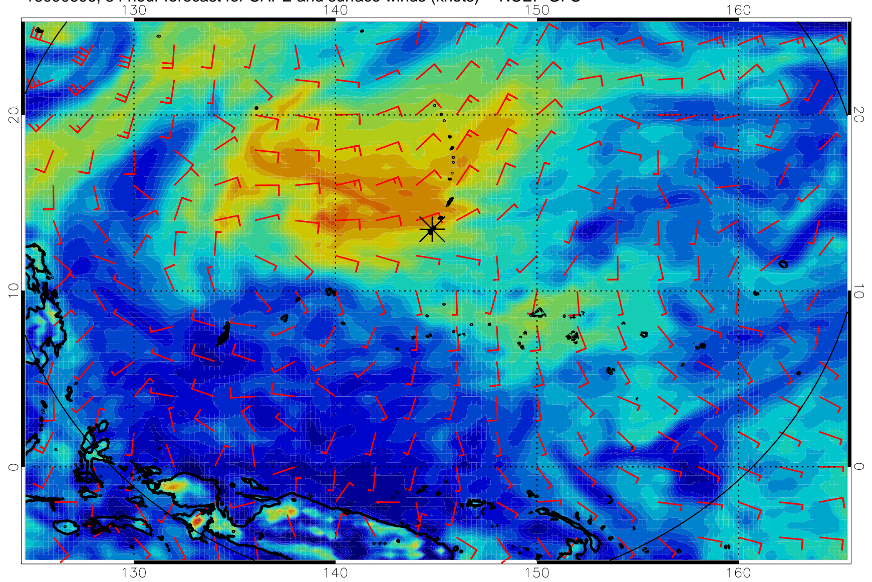
16090606, 54 hour forecast for CAPE and surface winds (knots) -- NCEP GFS
