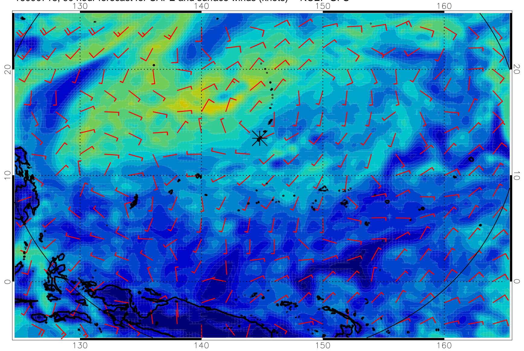
16090718, 90 hour forecast for CAPE and surface winds (knots) -- NCEP GFS
