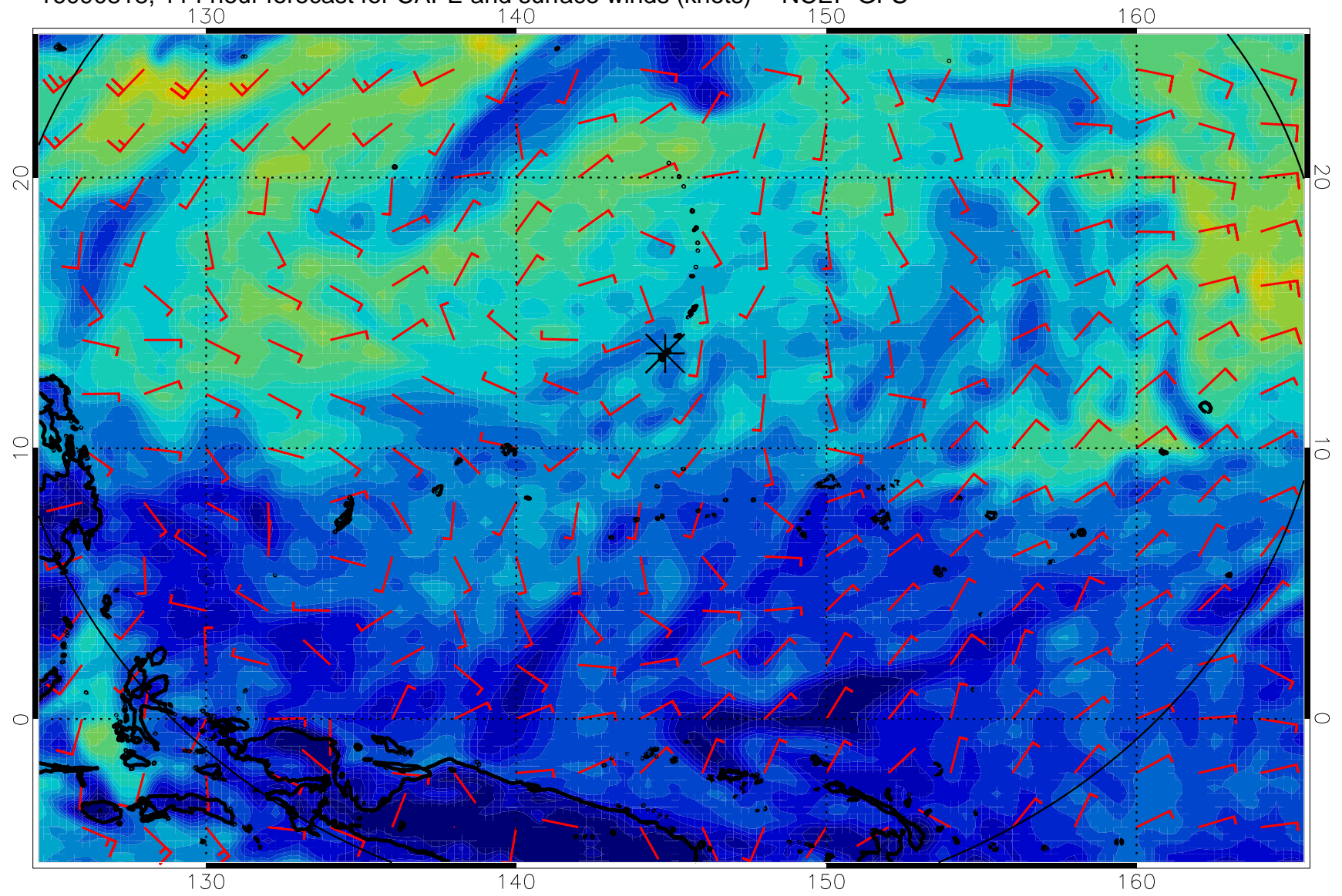
16090818, 114 hour forecast for CAPE and surface winds (knots) -- NCEP GFS
