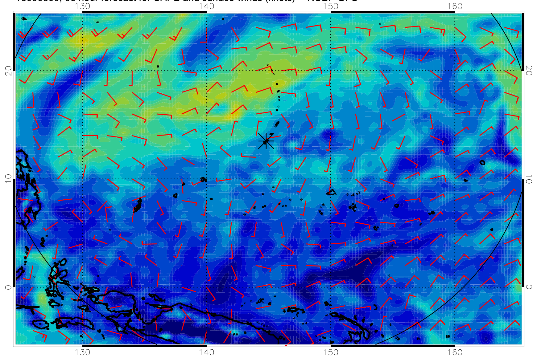
16090800, 96 hour forecast for CAPE and surface winds (knots) -- NCEP GFS
