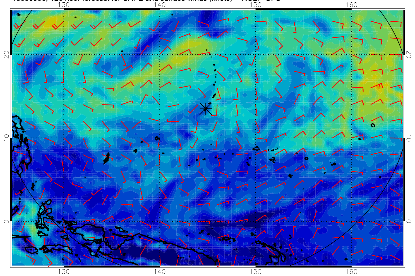
16090900, 120 hour forecast for CAPE and surface winds (knots) -- NCEP GFS
