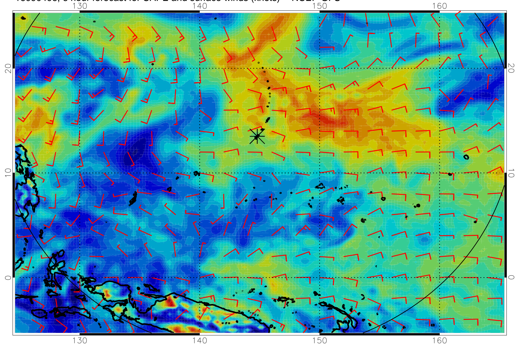
16090406, 6 hour forecast for CAPE and surface winds (knots) -- NCEP GFS
