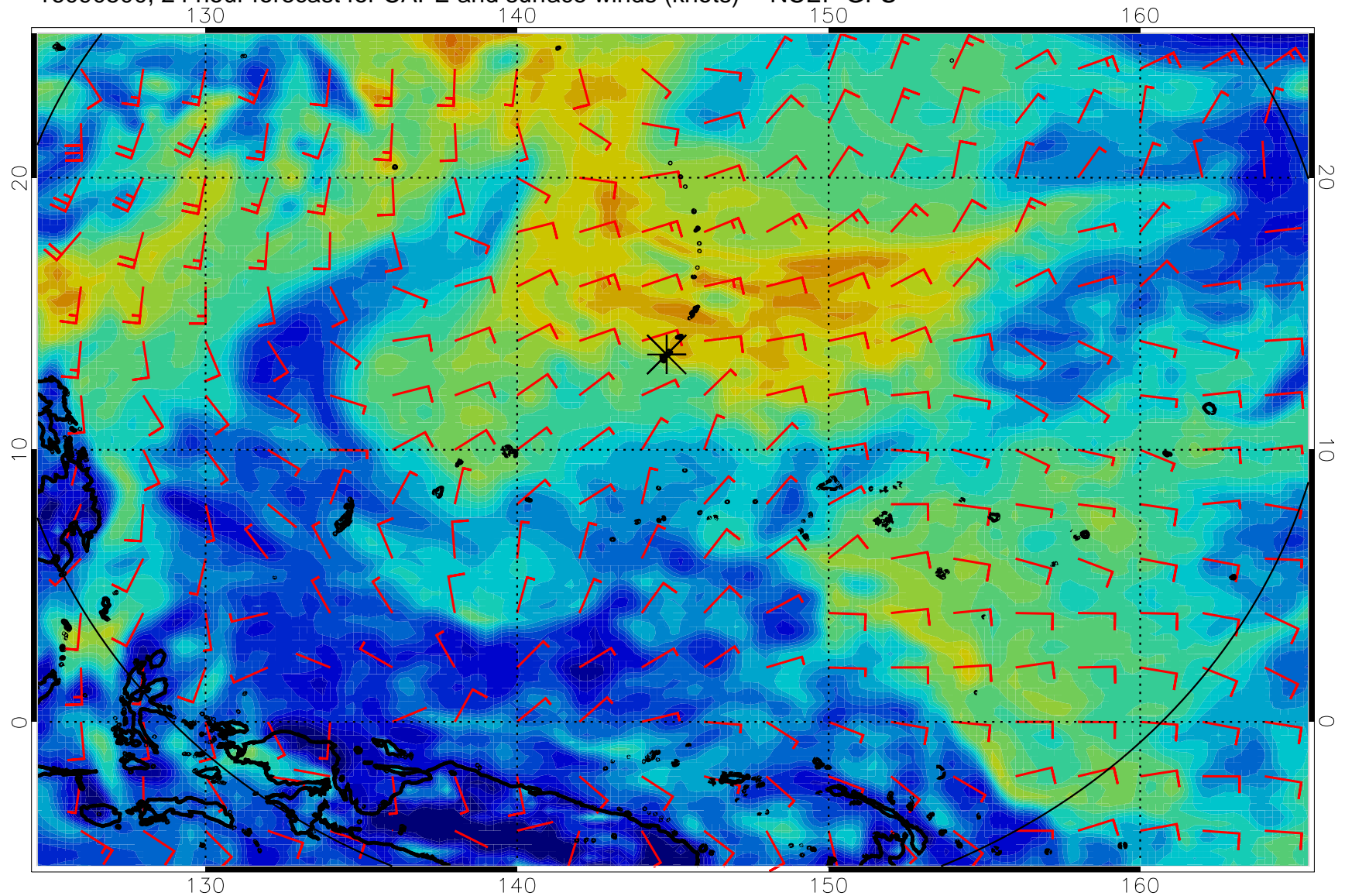
16090500, 24 hour forecast for CAPE and surface winds (knots) -- NCEP GFS
