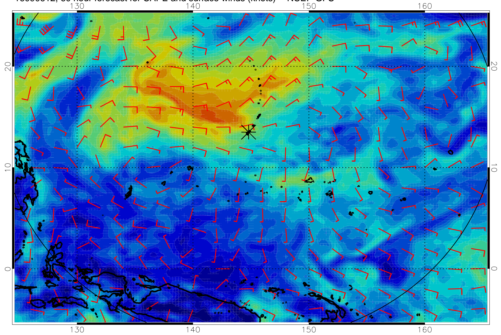
16090612, 60 hour forecast for CAPE and surface winds (knots) -- NCEP GFS
