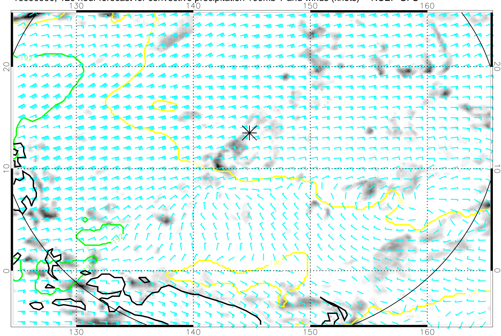
16090900, 120 hour forecast for convective precipitation 100mb T and winds (knots) -- NCEP GFS
