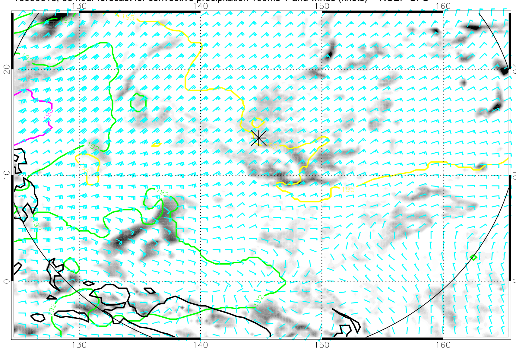
16090618, 66 hour forecast for convective precipitation 100mb T and winds (knots) -- NCEP GFS
