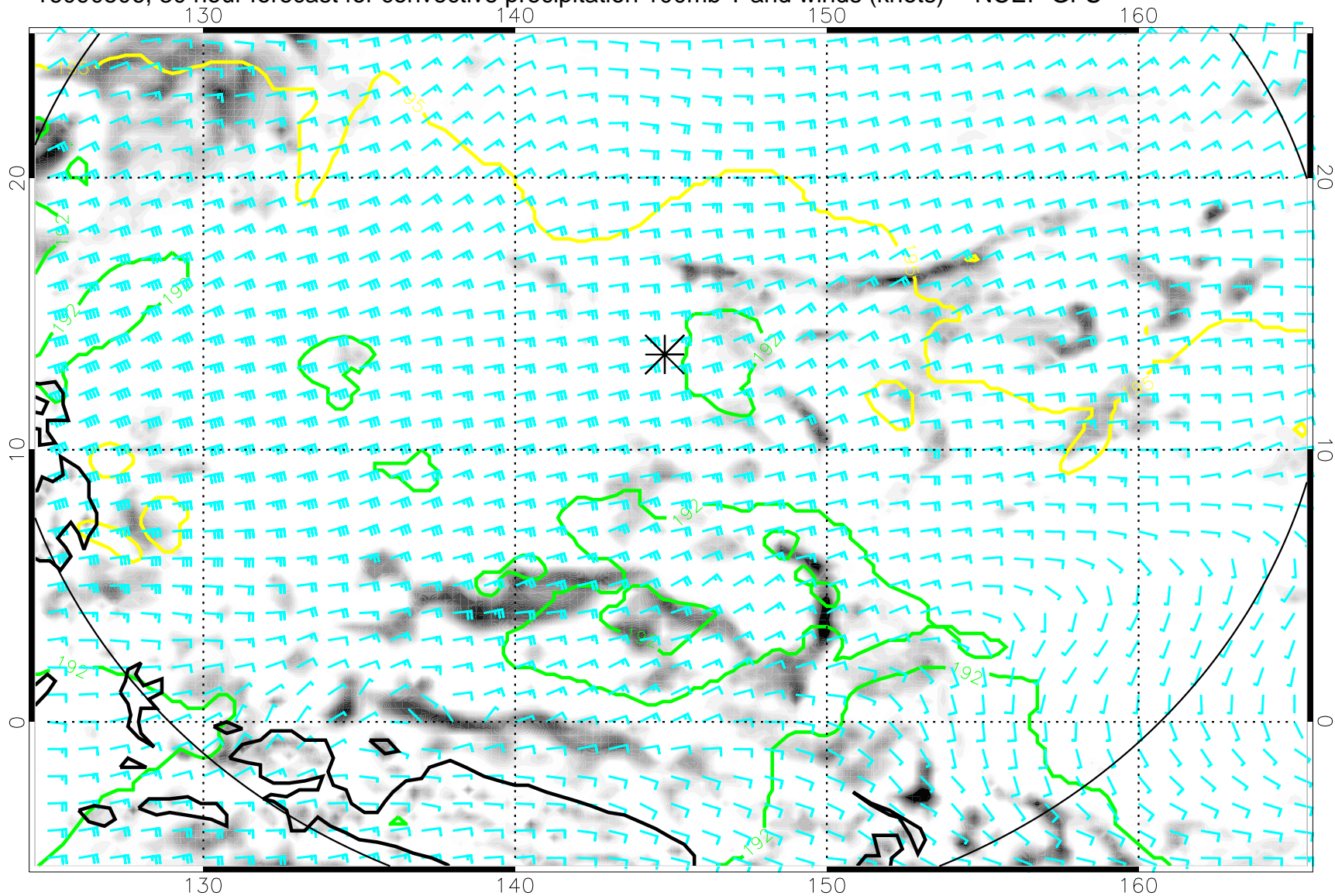
16090506, 30 hour forecast for convective precipitation 100mb T and winds (knots) -- NCEP GFS
