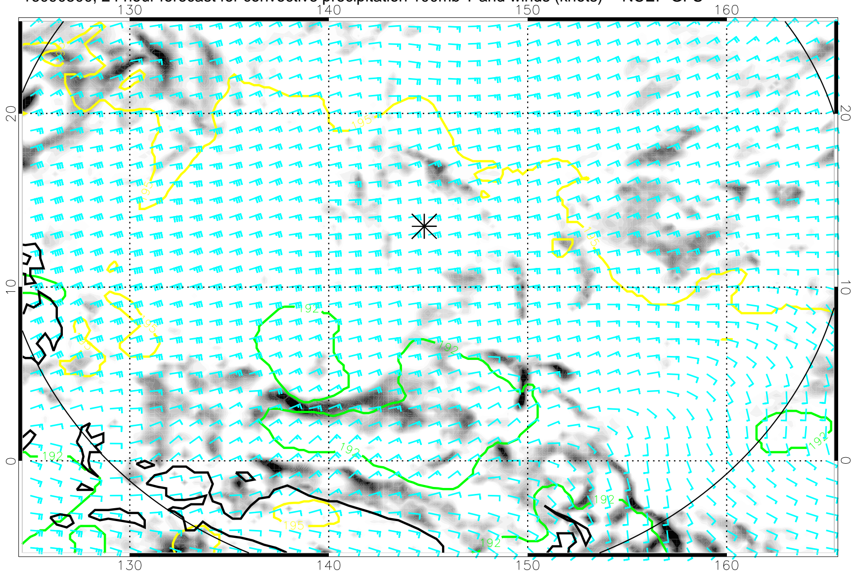
16090500, 24 hour forecast for convective precipitation 100mb T and winds (knots) -- NCEP GFS
