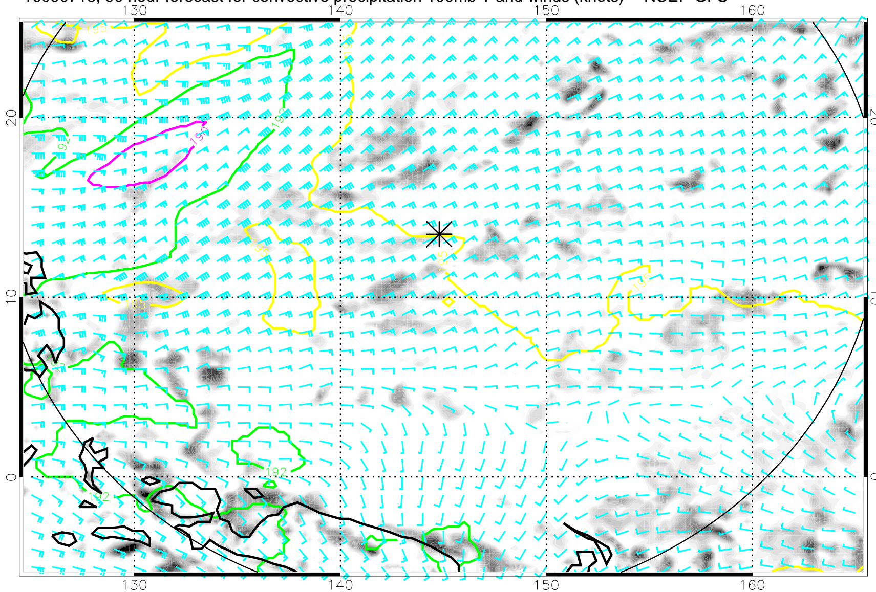
16090718, 90 hour forecast for convective precipitation 100mb T and winds (knots) -- NCEP GFS
