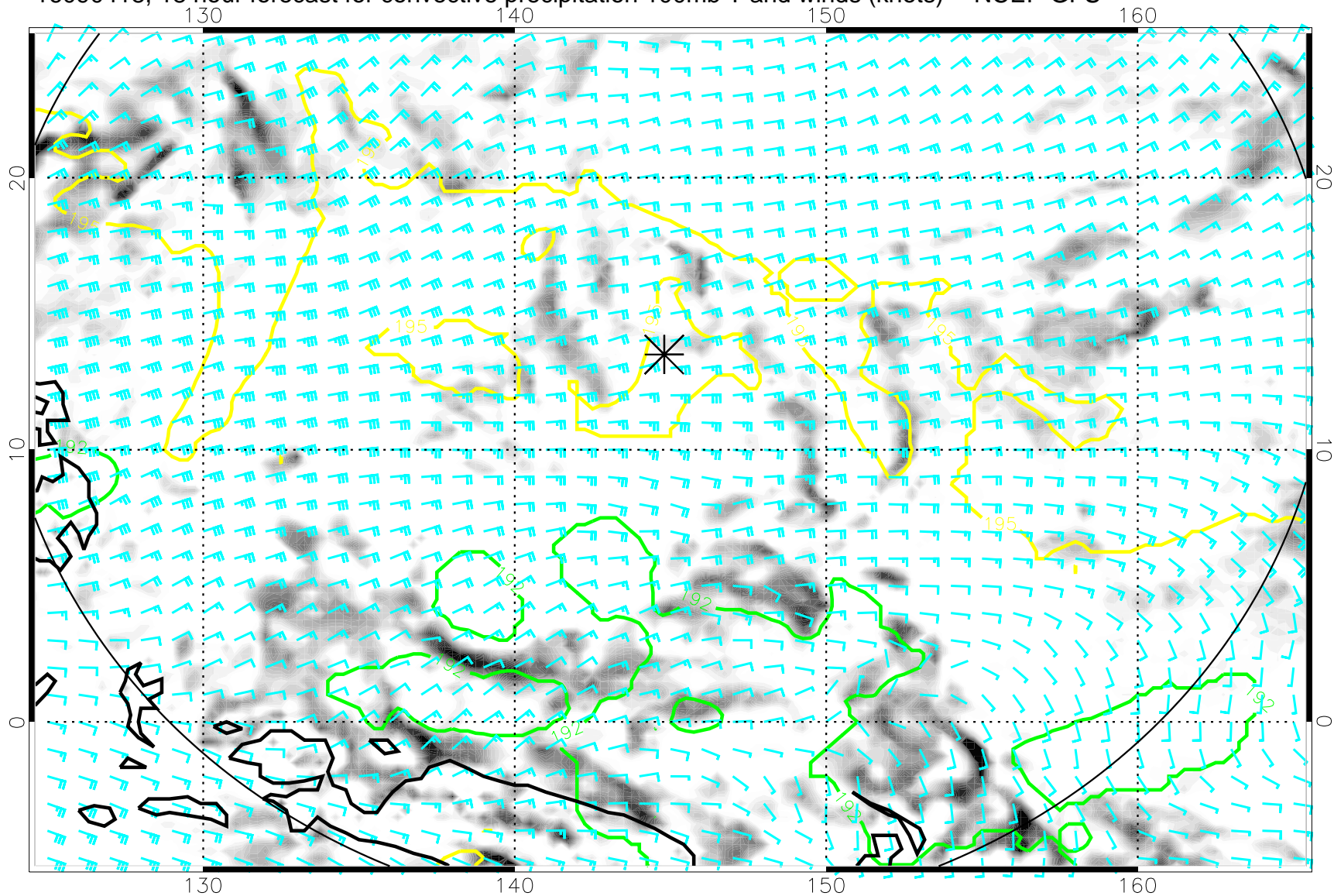
16090418, 18 hour forecast for convective precipitation 100mb T and winds (knots) -- NCEP GFS
