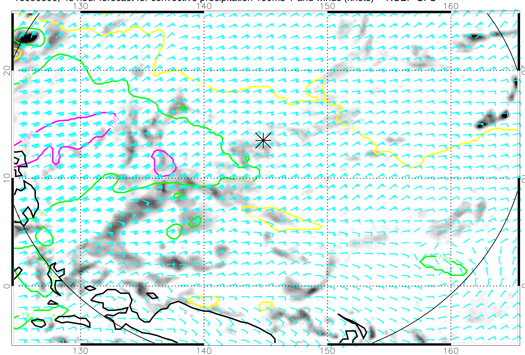
16090600, 48 hour forecast for convective precipitation 100mb T and winds (knots) -- NCEP GFS
