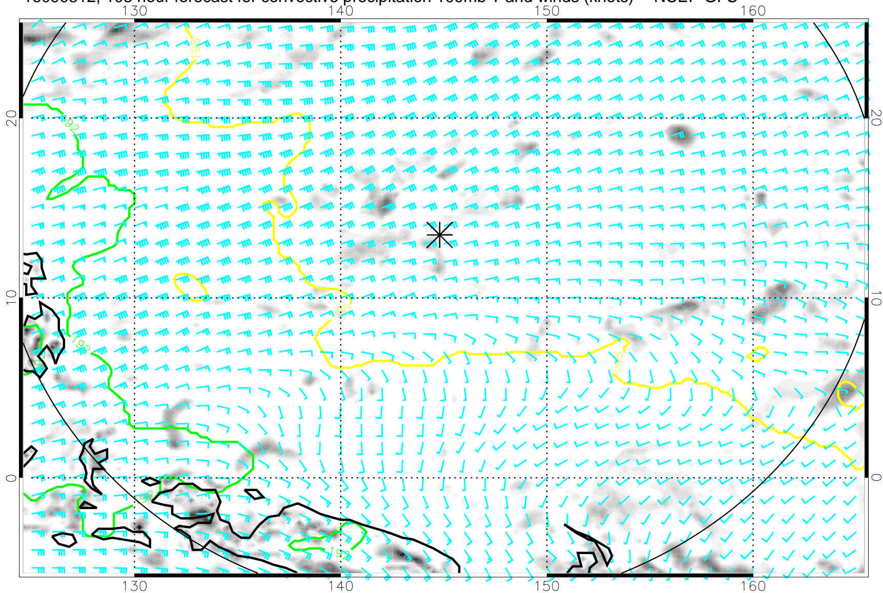
16090812, 108 hour forecast for convective precipitation 100mb T and winds (knots) -- NCEP GFS
