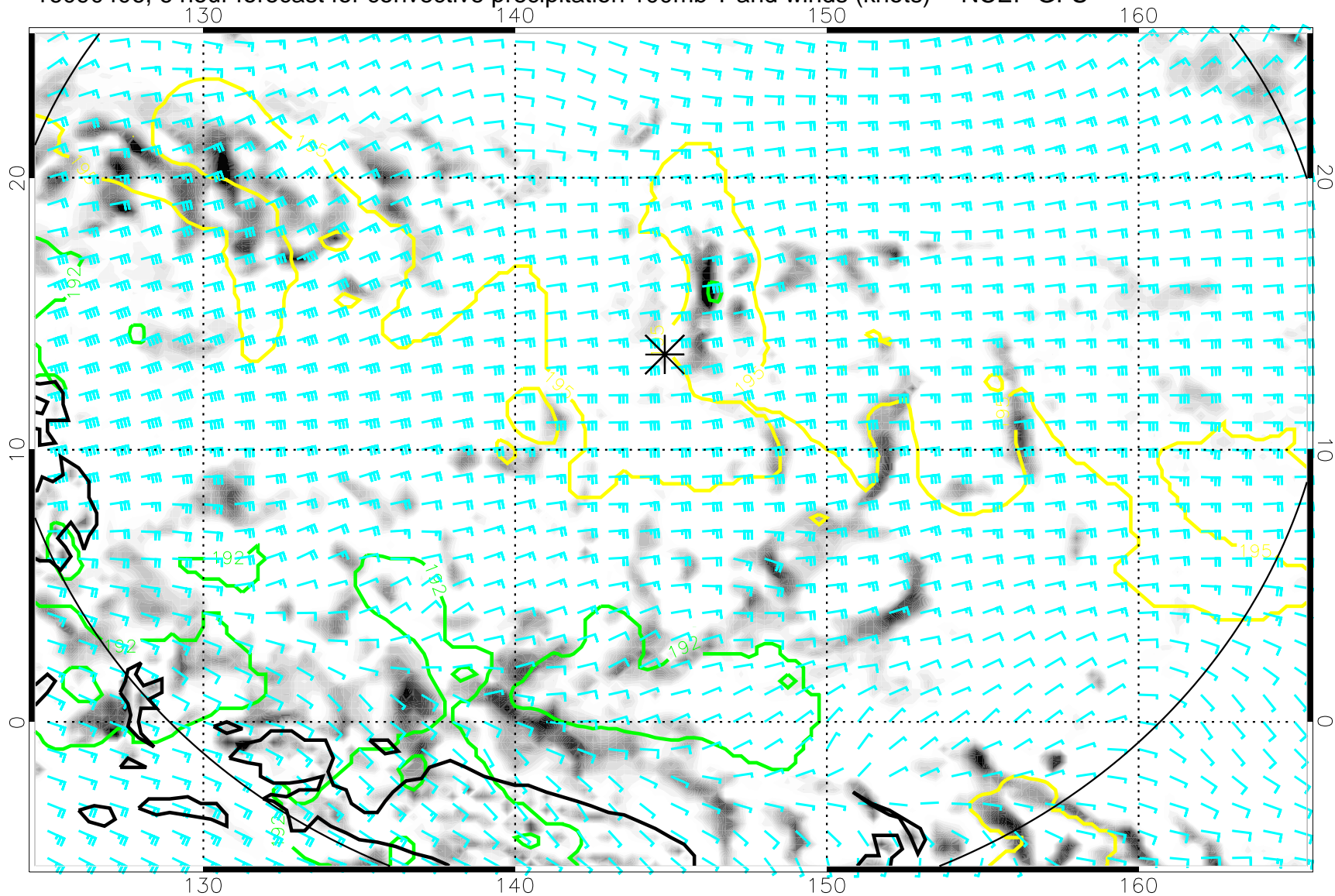
16090406, 6 hour forecast for convective precipitation 100mb T and winds (knots) -- NCEP GFS
