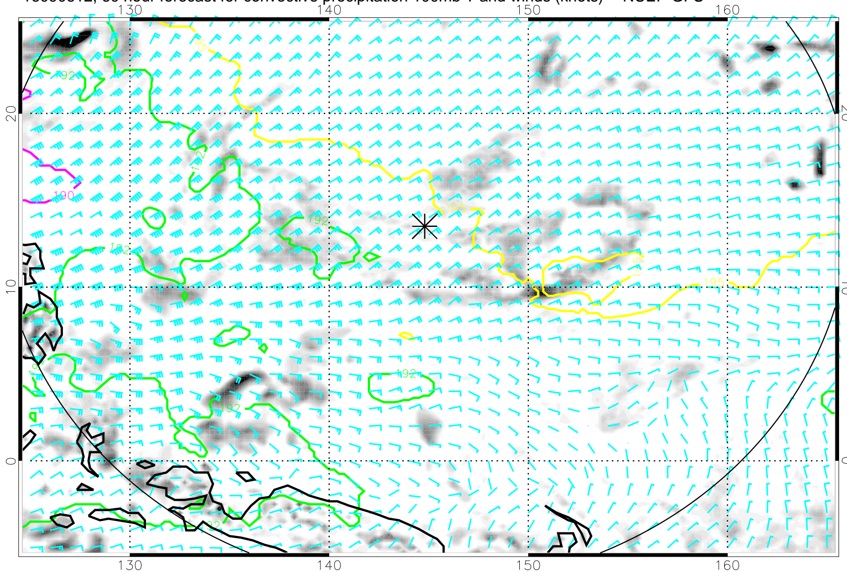
16090612, 60 hour forecast for convective precipitation 100mb T and winds (knots) -- NCEP GFS
