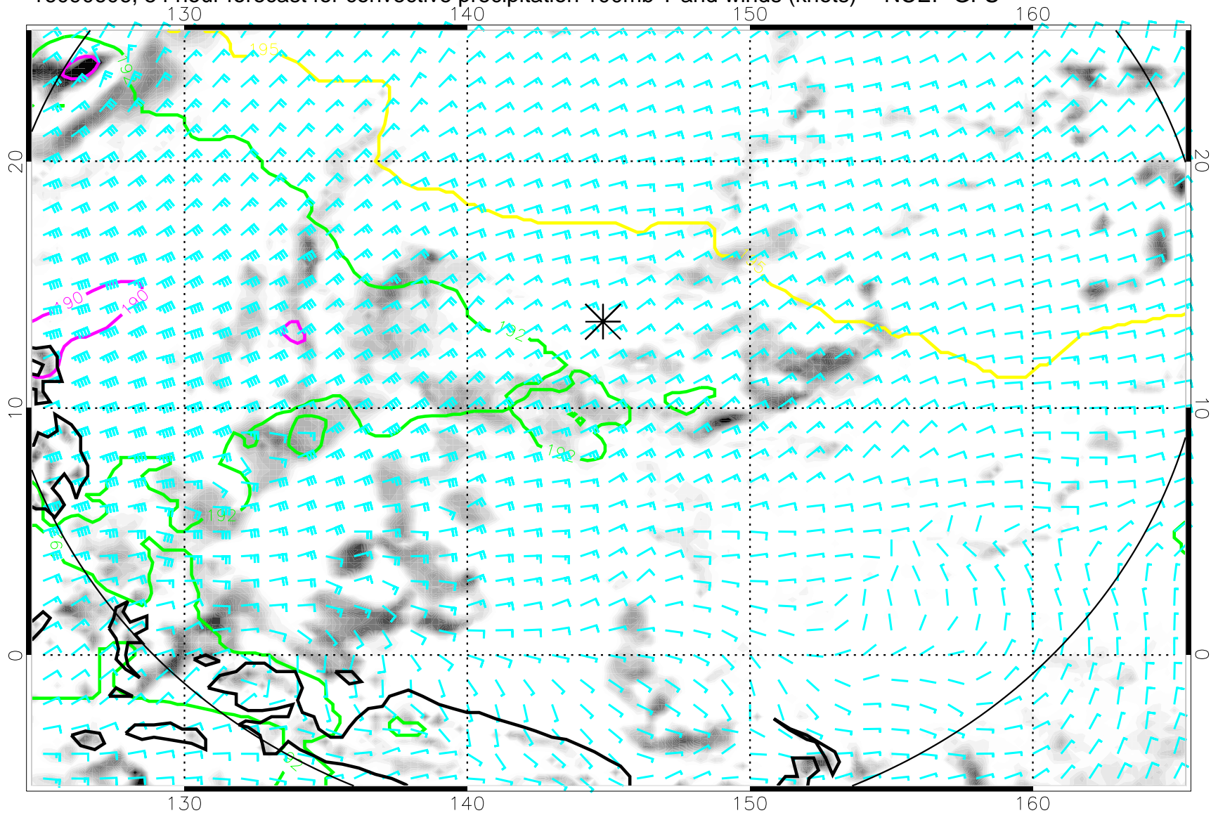
16090606, 54 hour forecast for convective precipitation 100mb T and winds (knots) -- NCEP GFS
