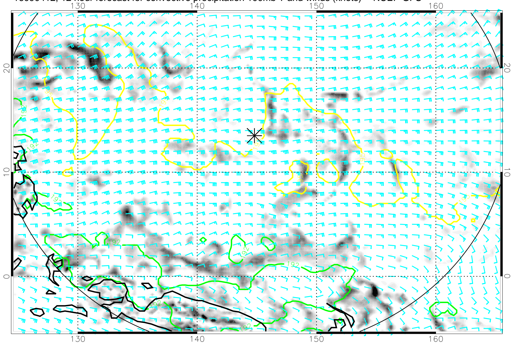
16090412, 12 hour forecast for convective precipitation 100mb T and winds (knots) -- NCEP GFS
