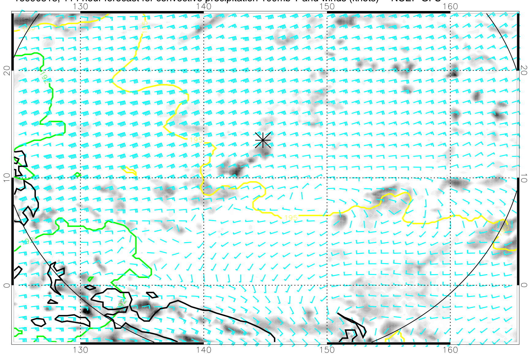
16090818, 114 hour forecast for convective precipitation 100mb T and winds (knots) -- NCEP GFS
