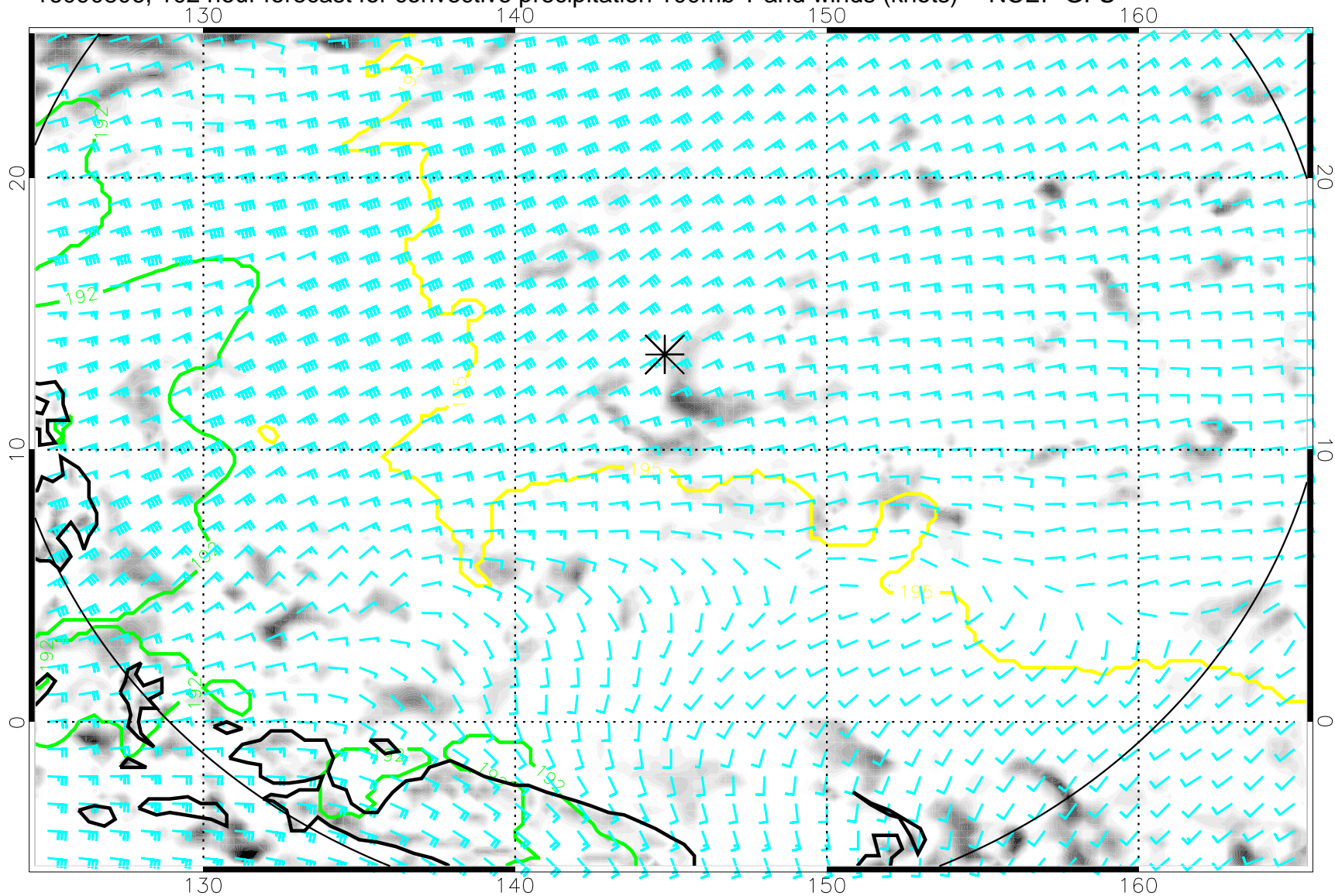
16090806, 102 hour forecast for convective precipitation 100mb T and winds (knots) -- NCEP GFS
