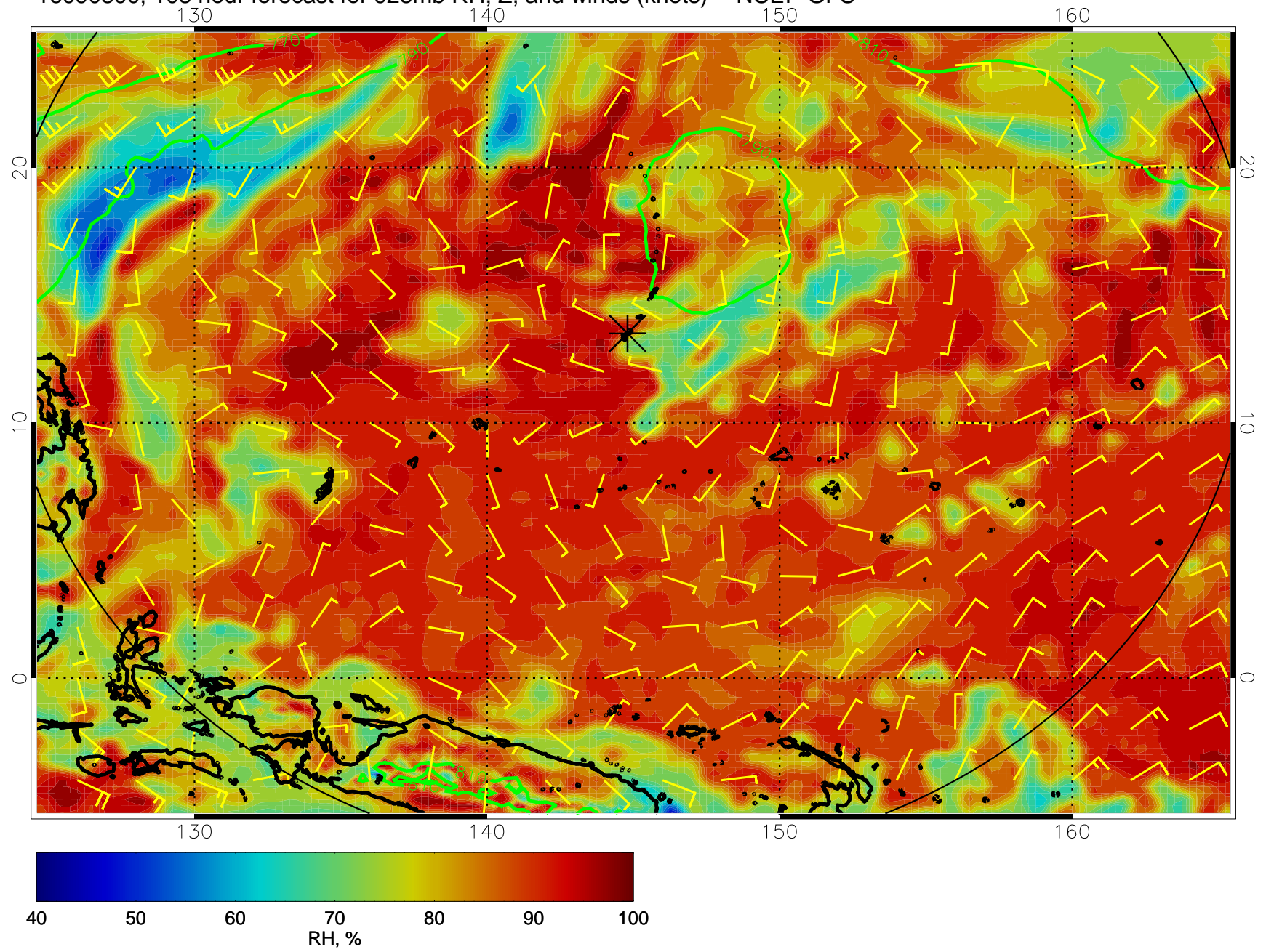
16090800, 108 hour forecast for 925mb RH, Z, and winds (knots) -- NCEP GFS
