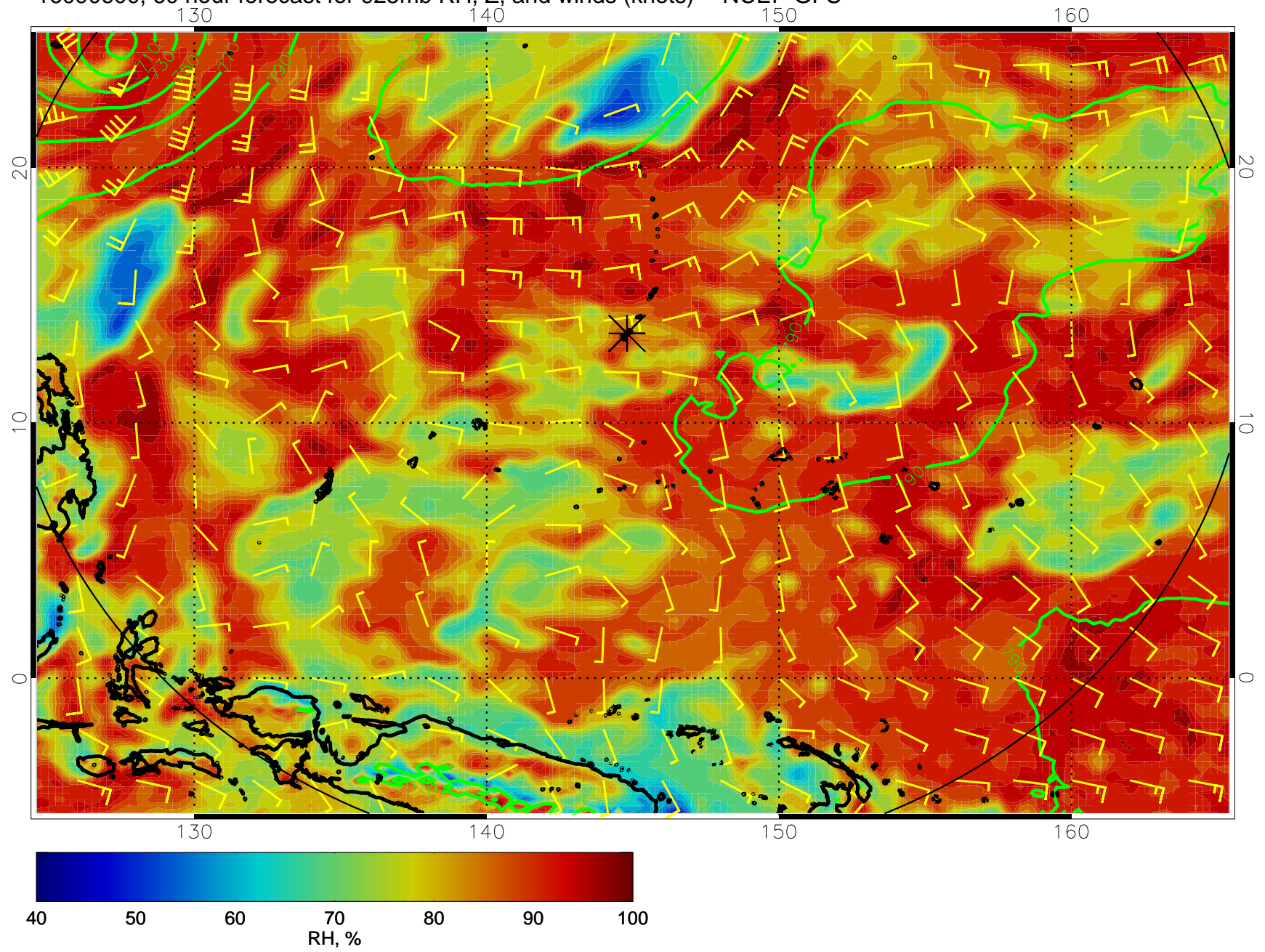
16090600, 60 hour forecast for 925mb RH, Z, and winds (knots) -- NCEP GFS
