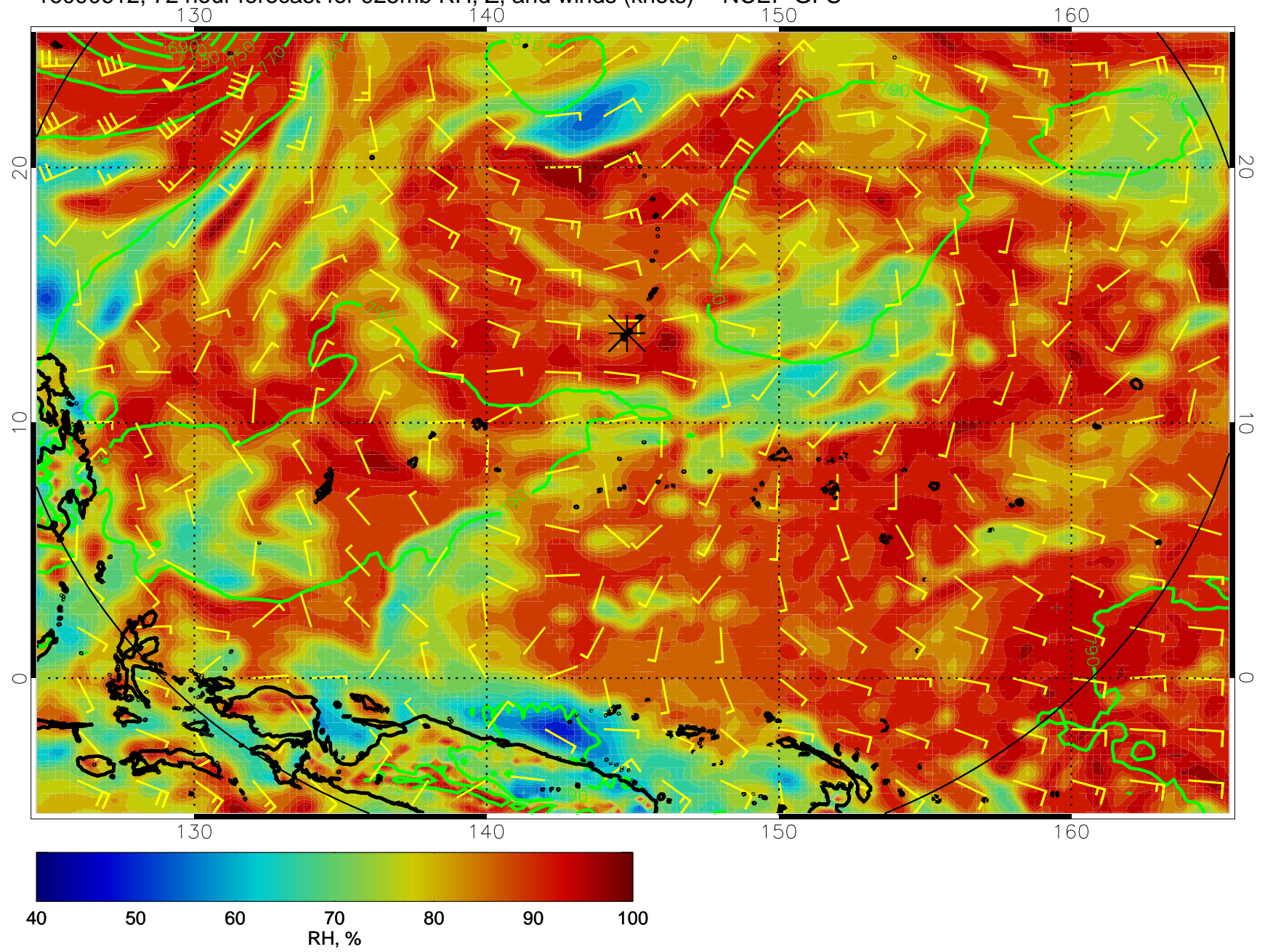
16090612, 72 hour forecast for 925mb RH, Z, and winds (knots) -- NCEP GFS
