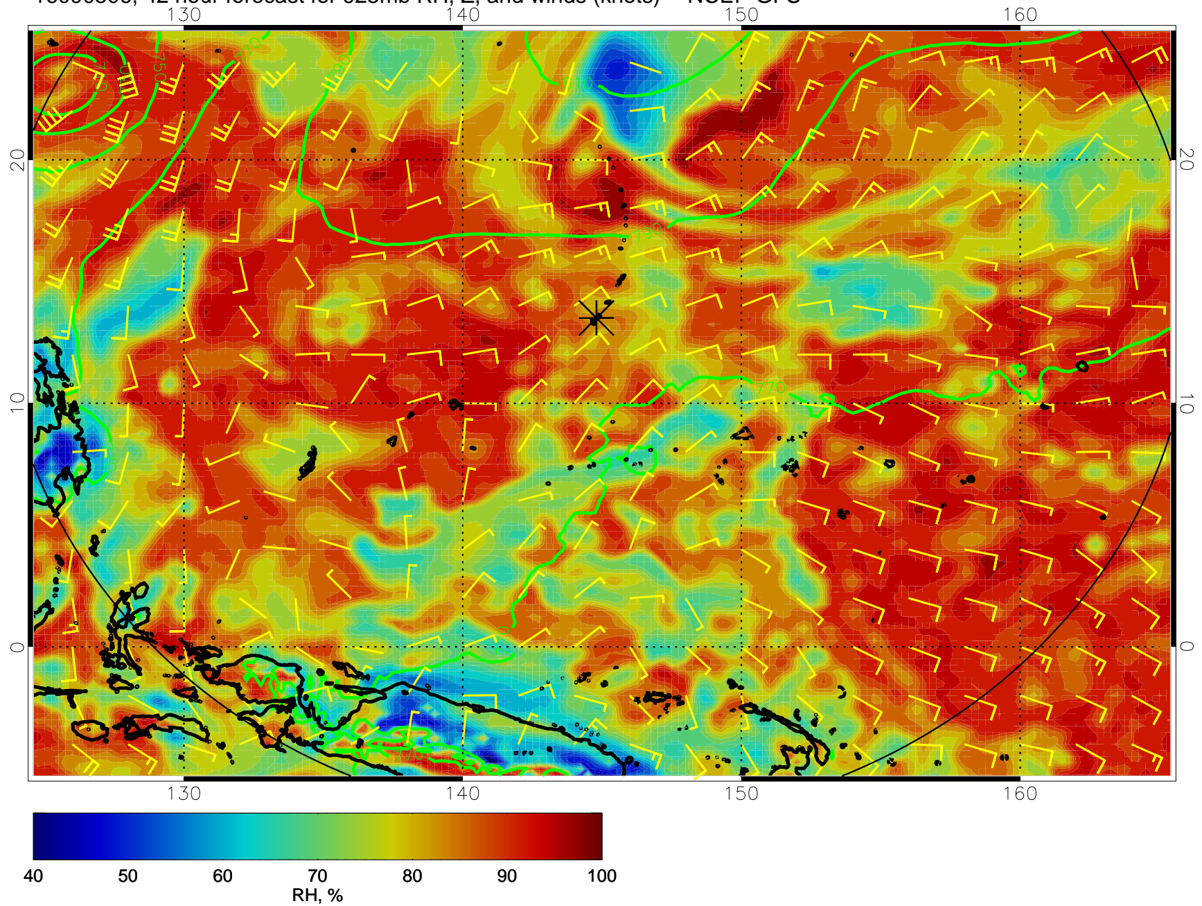
16090506, 42 hour forecast for 925mb RH, Z, and winds (knots) -- NCEP GFS
