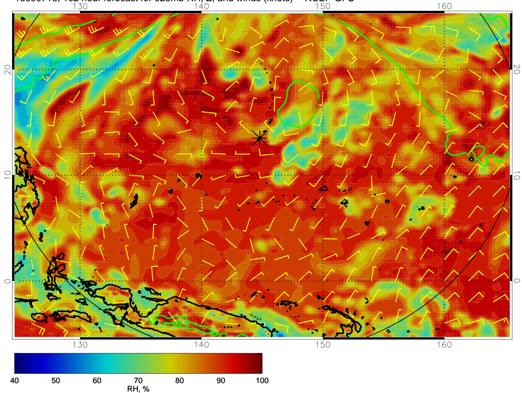
16090718, 102 hour forecast for 925mb RH, Z, and winds (knots) -- NCEP GFS
