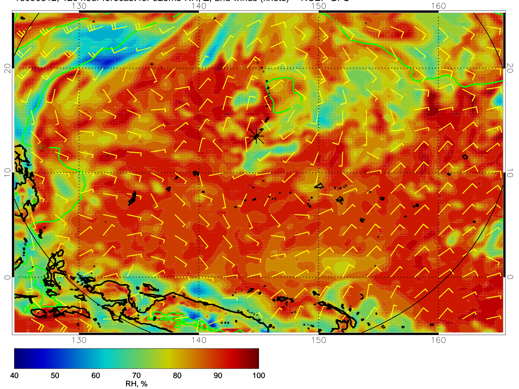
16090812, 120 hour forecast for 925mb RH, Z, and winds (knots) -- NCEP GFS
