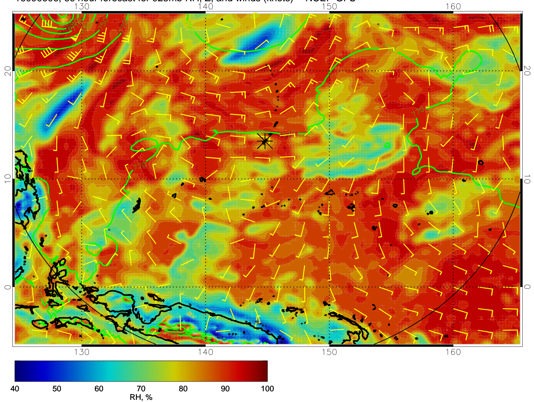
16090606, 66 hour forecast for 925mb RH, Z, and winds (knots) -- NCEP GFS
