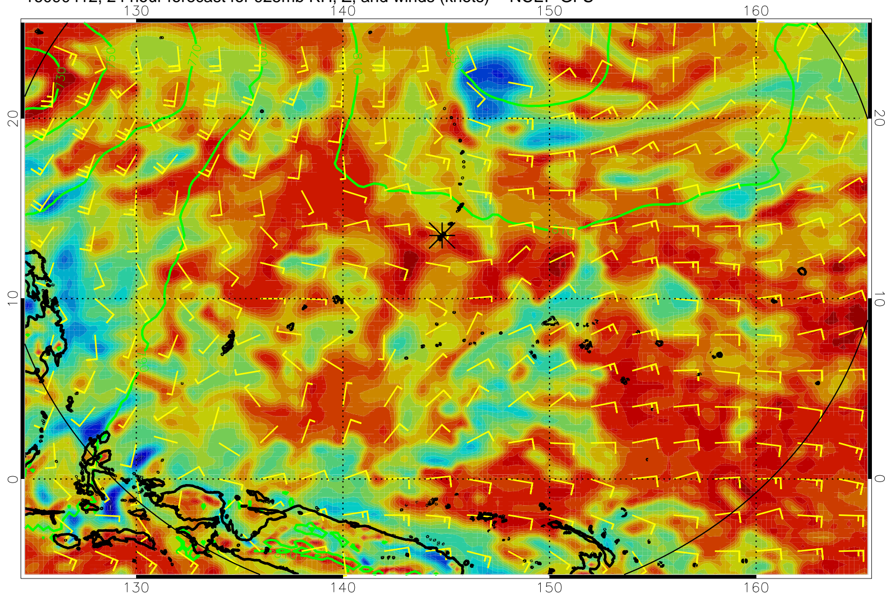
16090412, 24 hour forecast for 925mb RH, Z, and winds (knots) -- NCEP GFS
