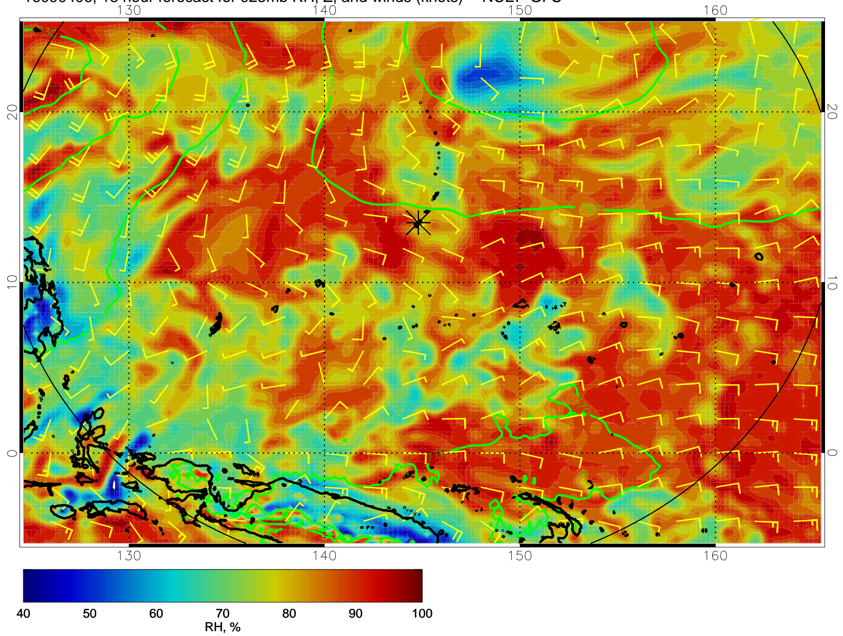
16090406, 18 hour forecast for 925mb RH, Z, and winds (knots) -- NCEP GFS
