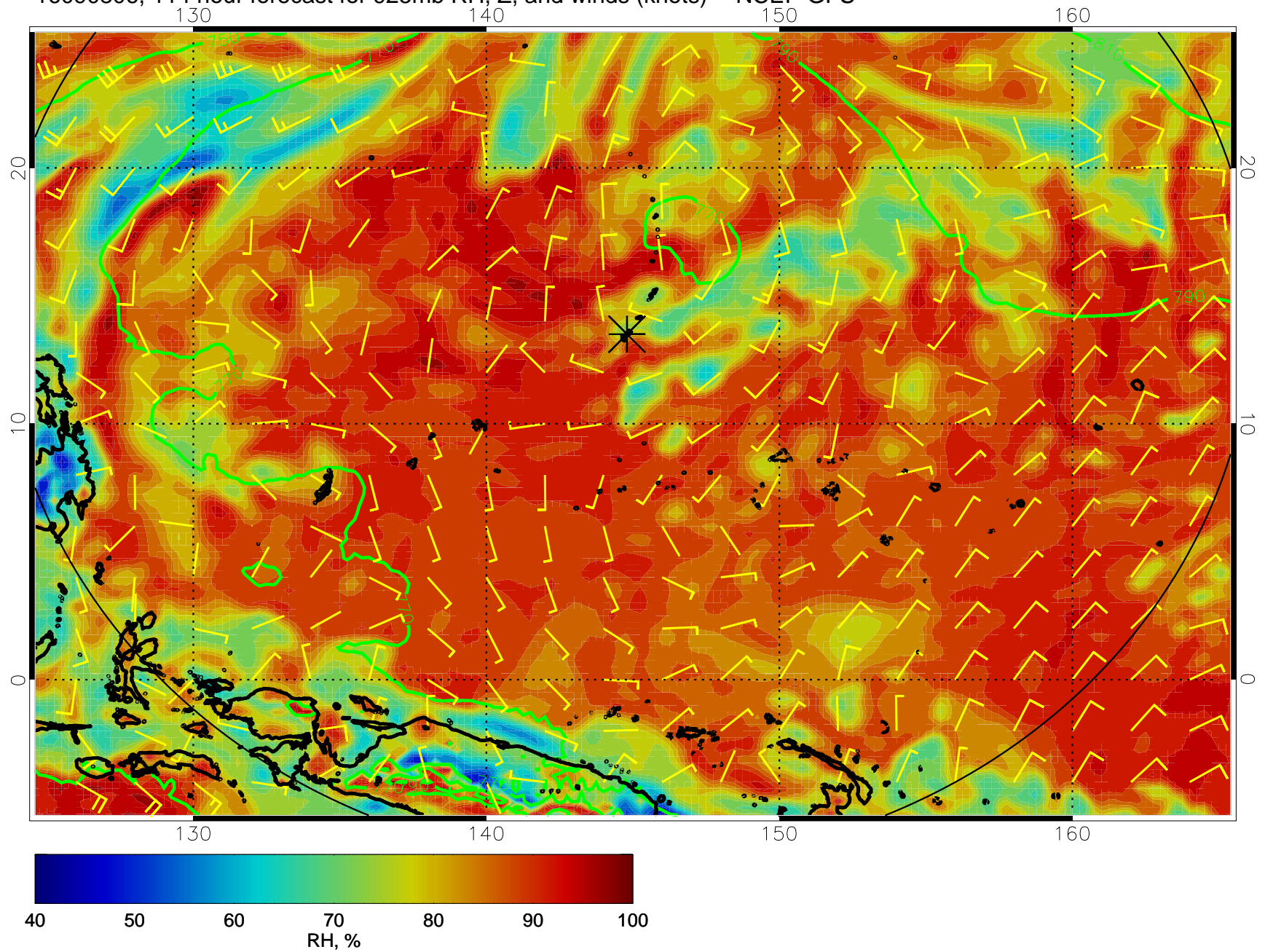
16090806, 114 hour forecast for 925mb RH, Z, and winds (knots) -- NCEP GFS
