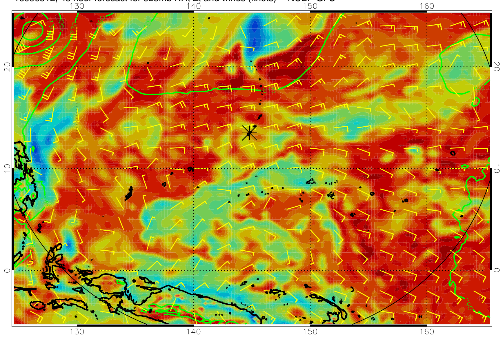
16090512, 48 hour forecast for 925mb RH, Z, and winds (knots) -- NCEP GFS
