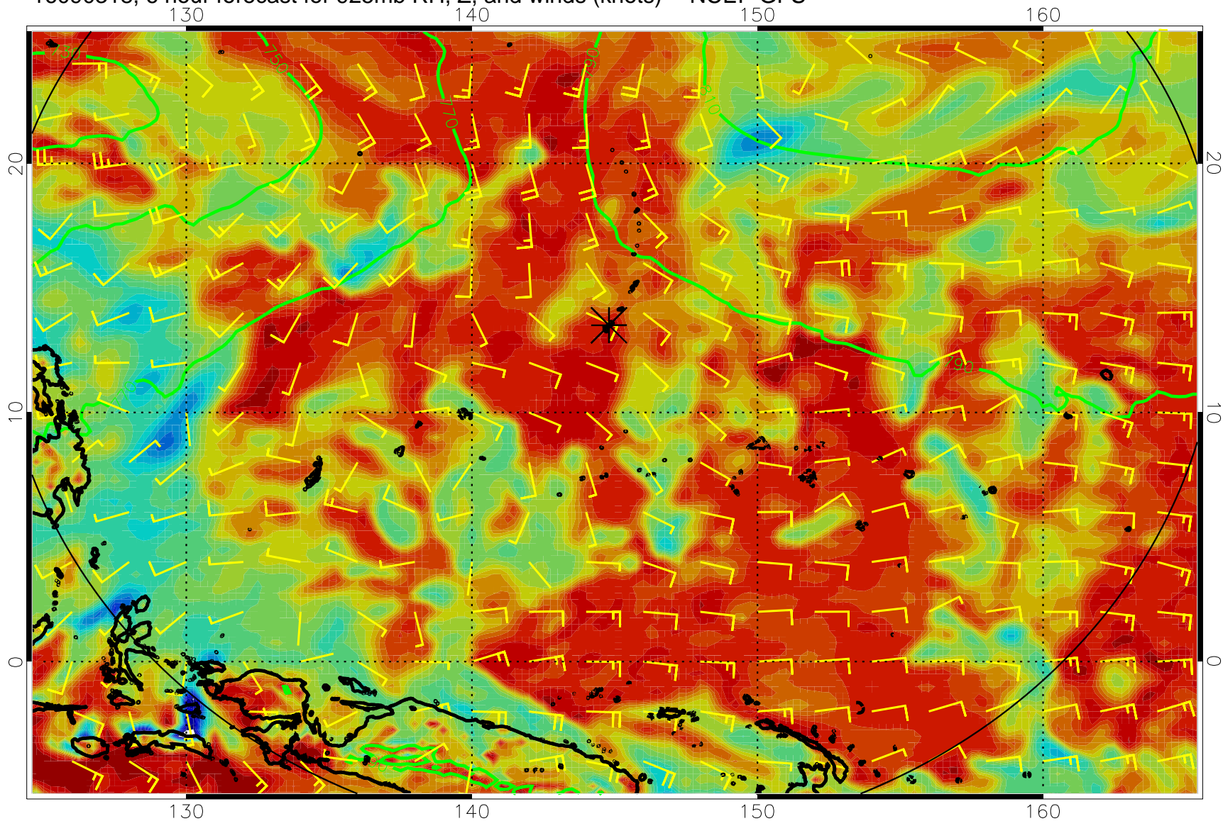
16090318, 6 hour forecast for 925mb RH, Z, and winds (knots) -- NCEP GFS
