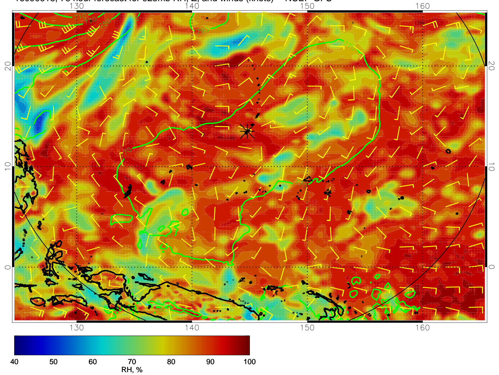
16090618, 78 hour forecast for 925mb RH, Z, and winds (knots) -- NCEP GFS
