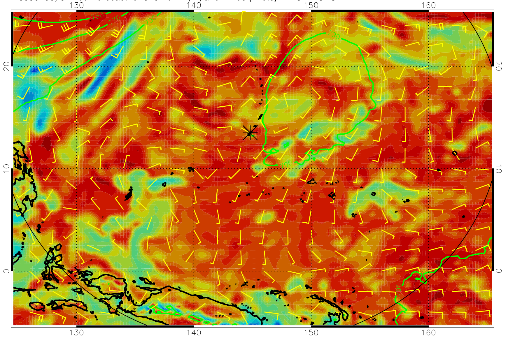
16090700, 84 hour forecast for 925mb RH, Z, and winds (knots) -- NCEP GFS
