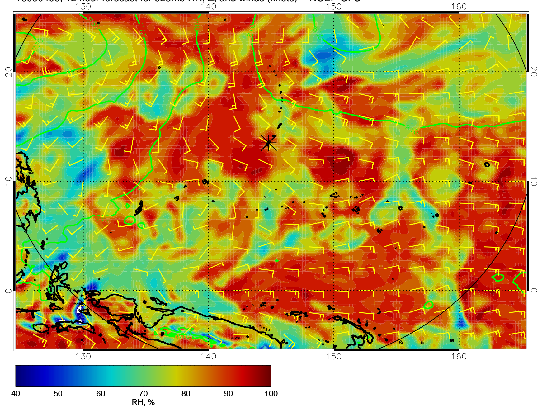
16090400, 12 hour forecast for 925mb RH, Z, and winds (knots) -- NCEP GFS
