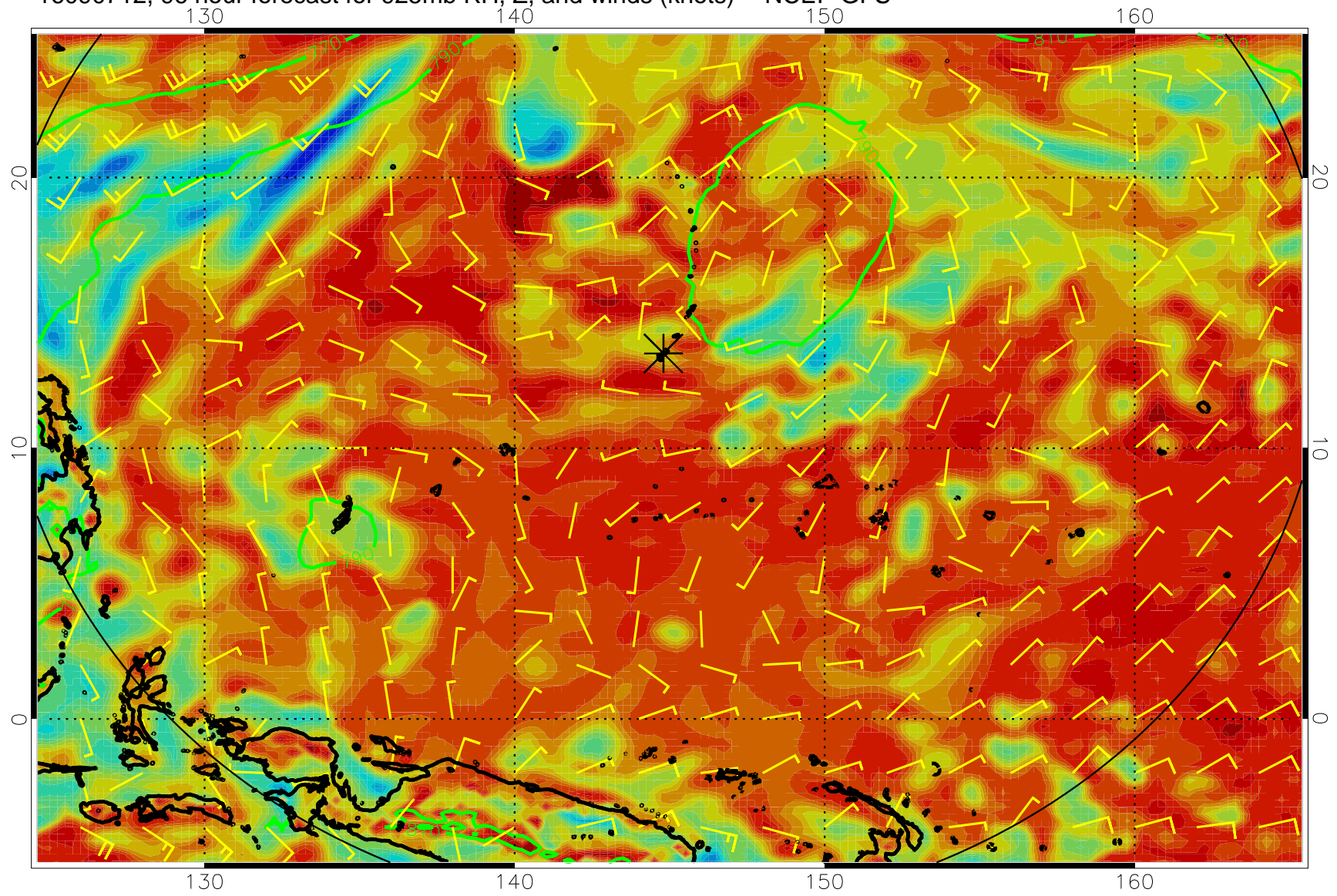
16090712, 96 hour forecast for 925mb RH, Z, and winds (knots) -- NCEP GFS
