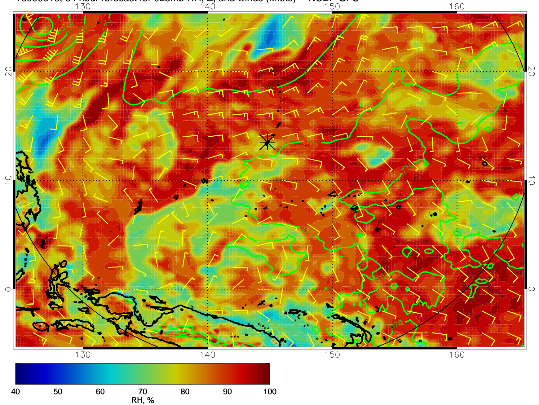
16090518, 54 hour forecast for 925mb RH, Z, and winds (knots) -- NCEP GFS
