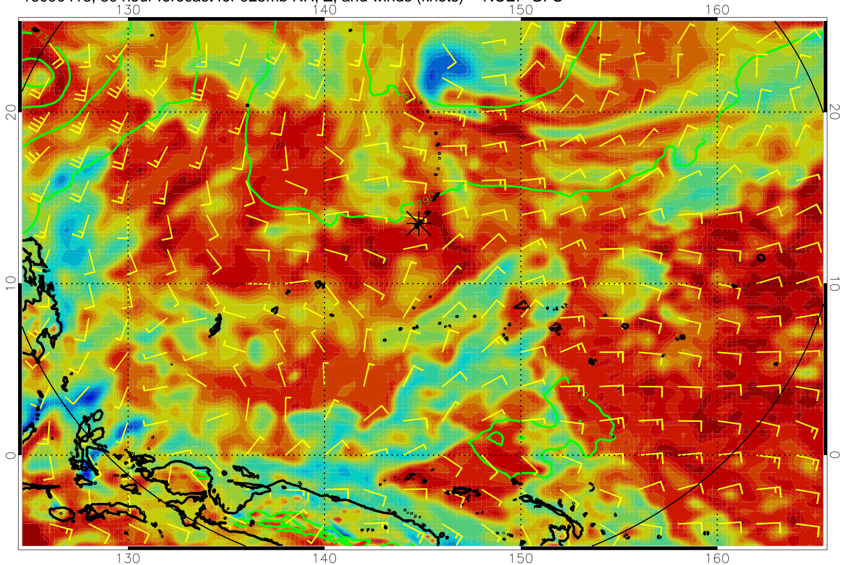
16090418, 30 hour forecast for 925mb RH, Z, and winds (knots) -- NCEP GFS
