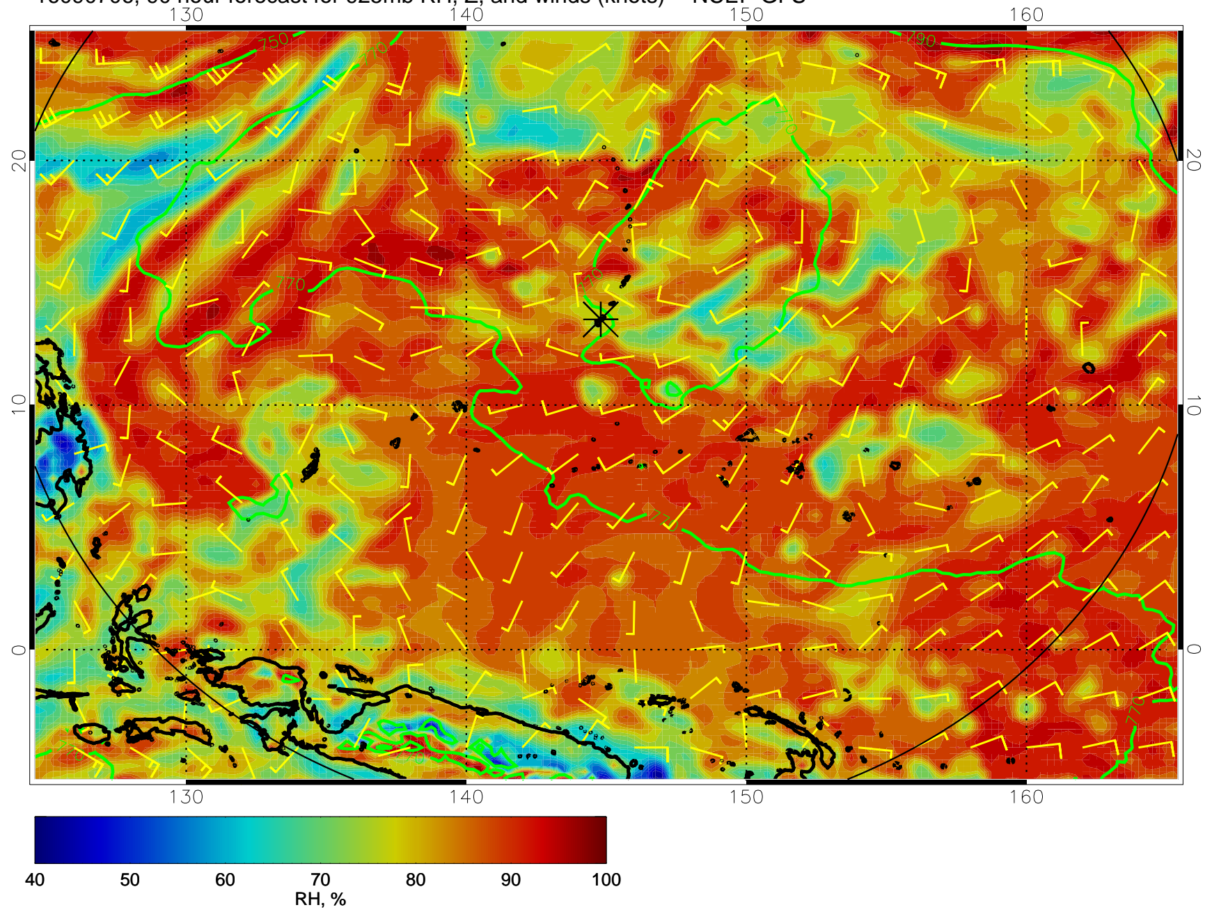
16090706, 90 hour forecast for 925mb RH, Z, and winds (knots) -- NCEP GFS
