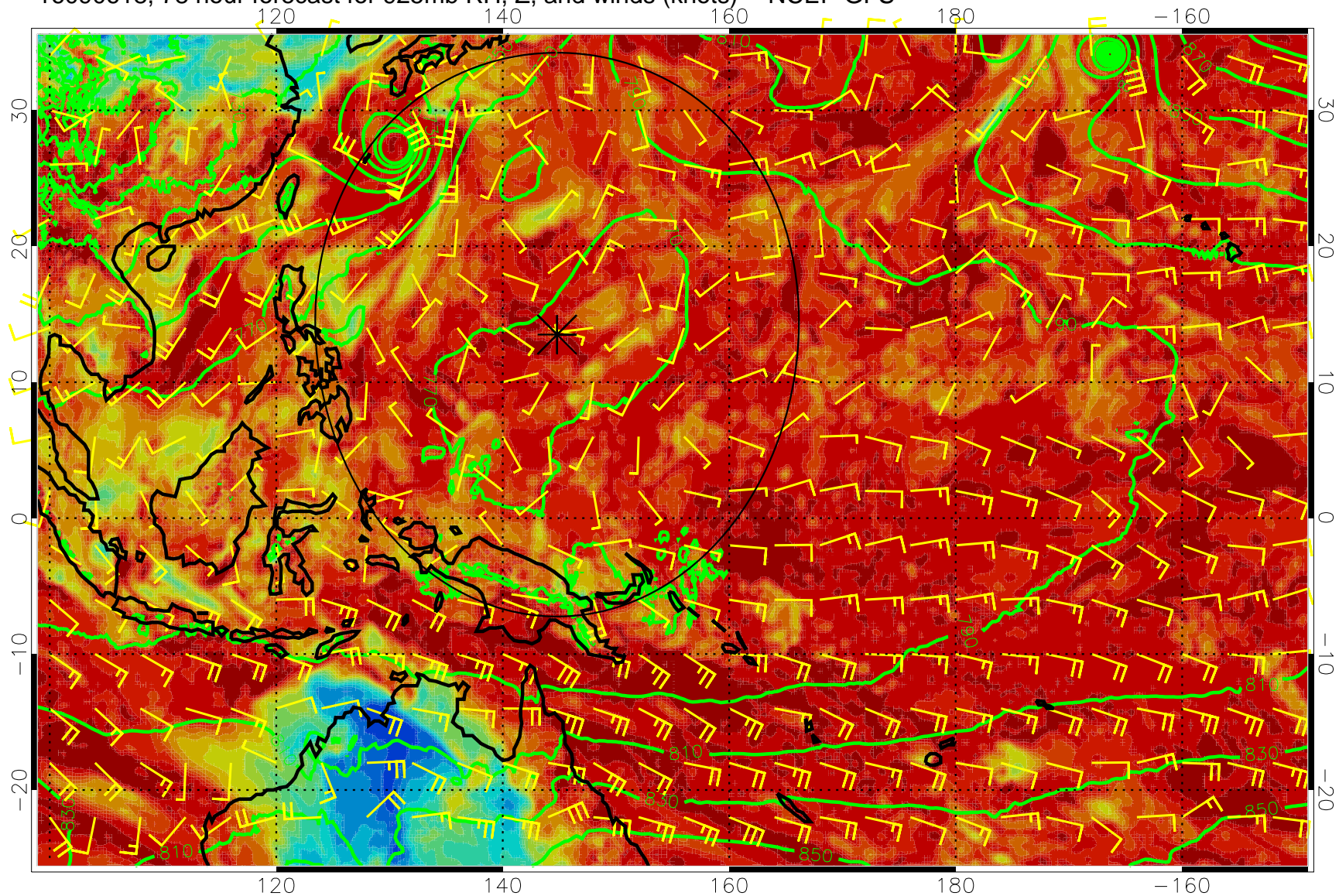
16090618, 78 hour forecast for 925mb RH, Z, and winds (knots) -- NCEP GFS
