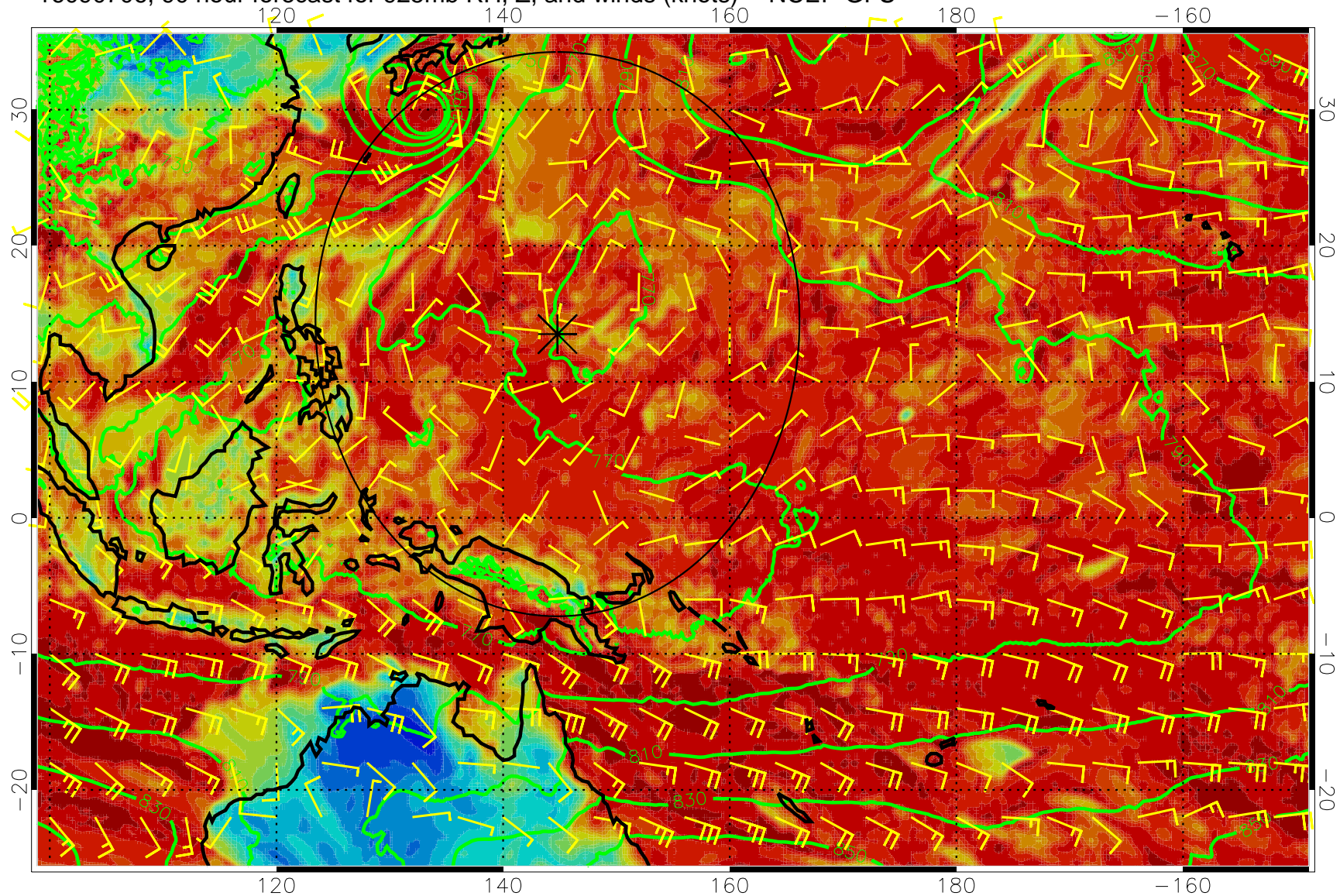
16090706, 90 hour forecast for 925mb RH, Z, and winds (knots) -- NCEP GFS
