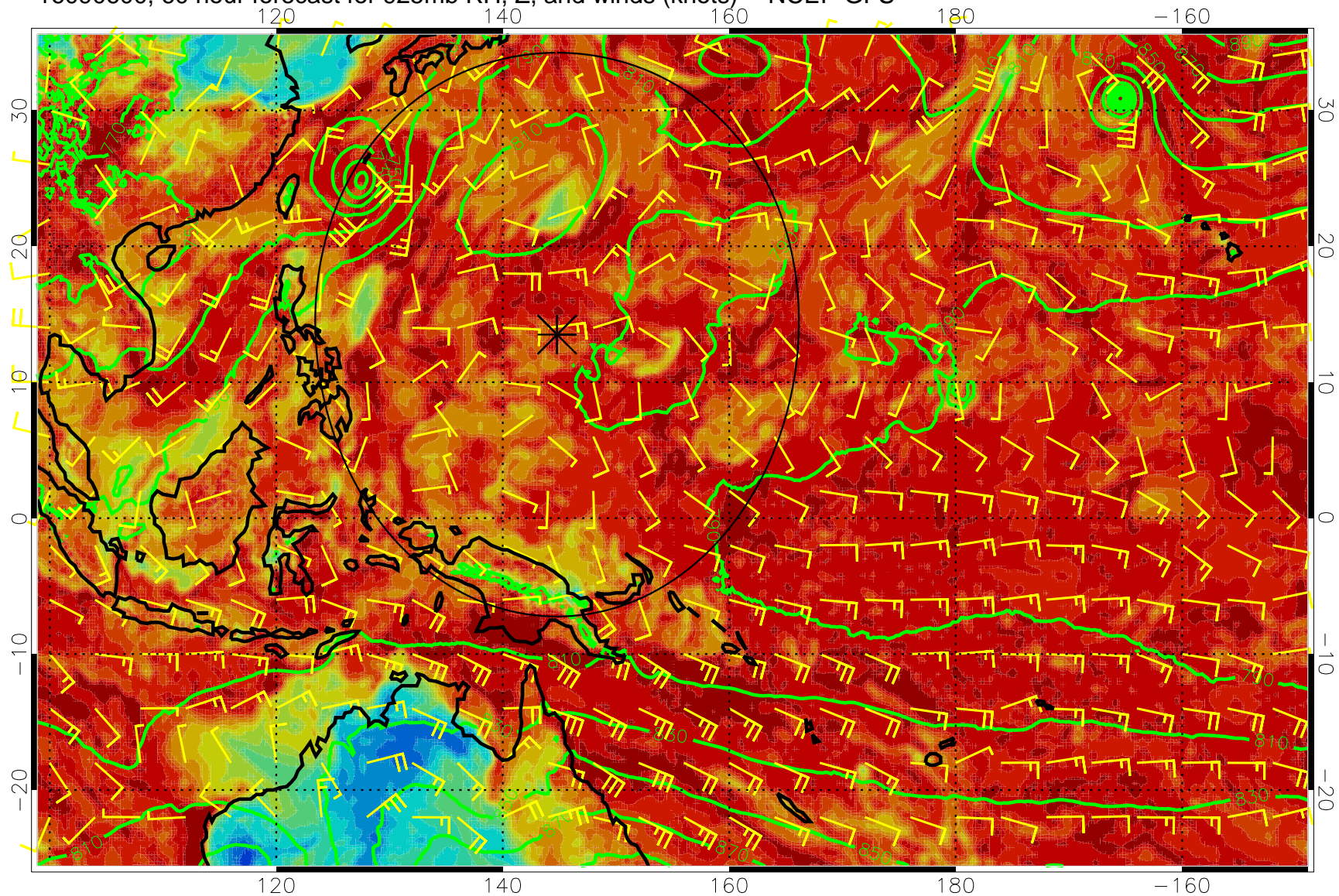
16090600, 60 hour forecast for 925mb RH, Z, and winds (knots) -- NCEP GFS
