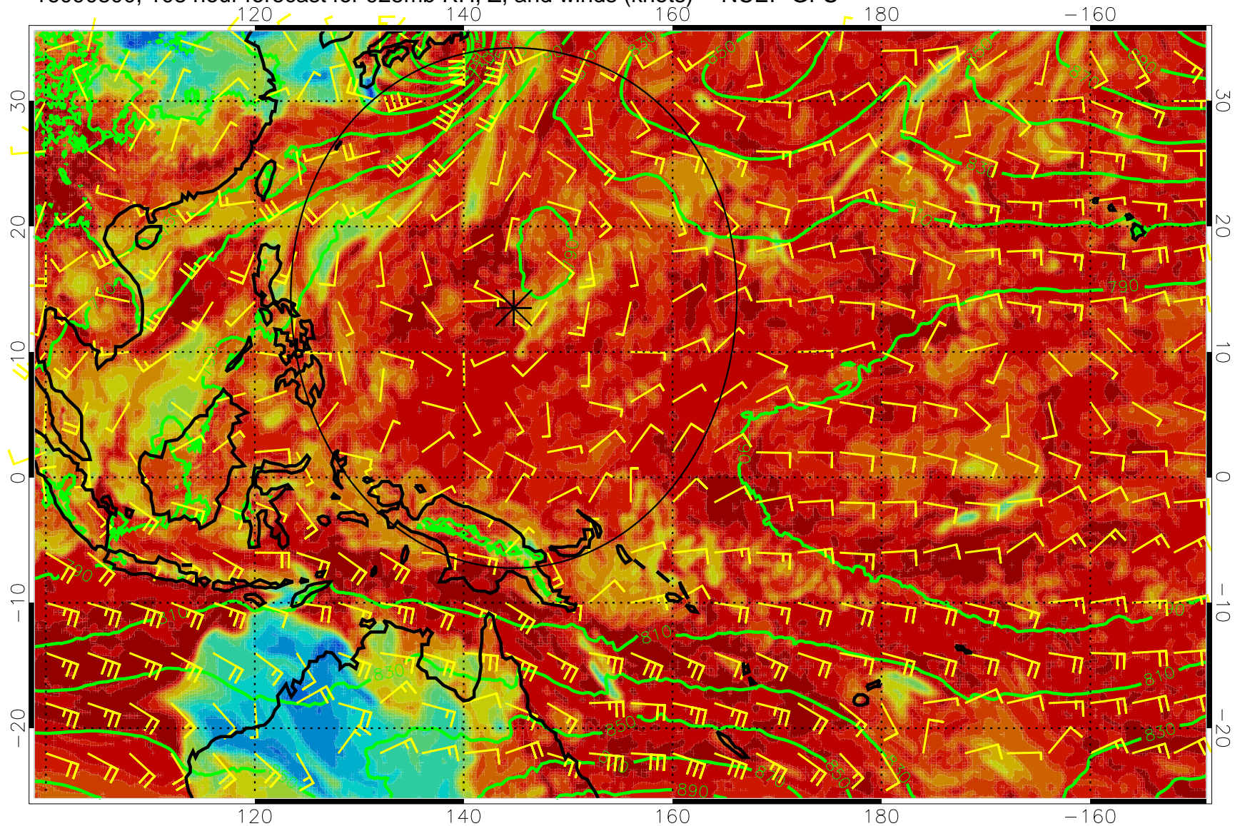
16090800, 108 hour forecast for 925mb RH, Z, and winds (knots) -- NCEP GFS
