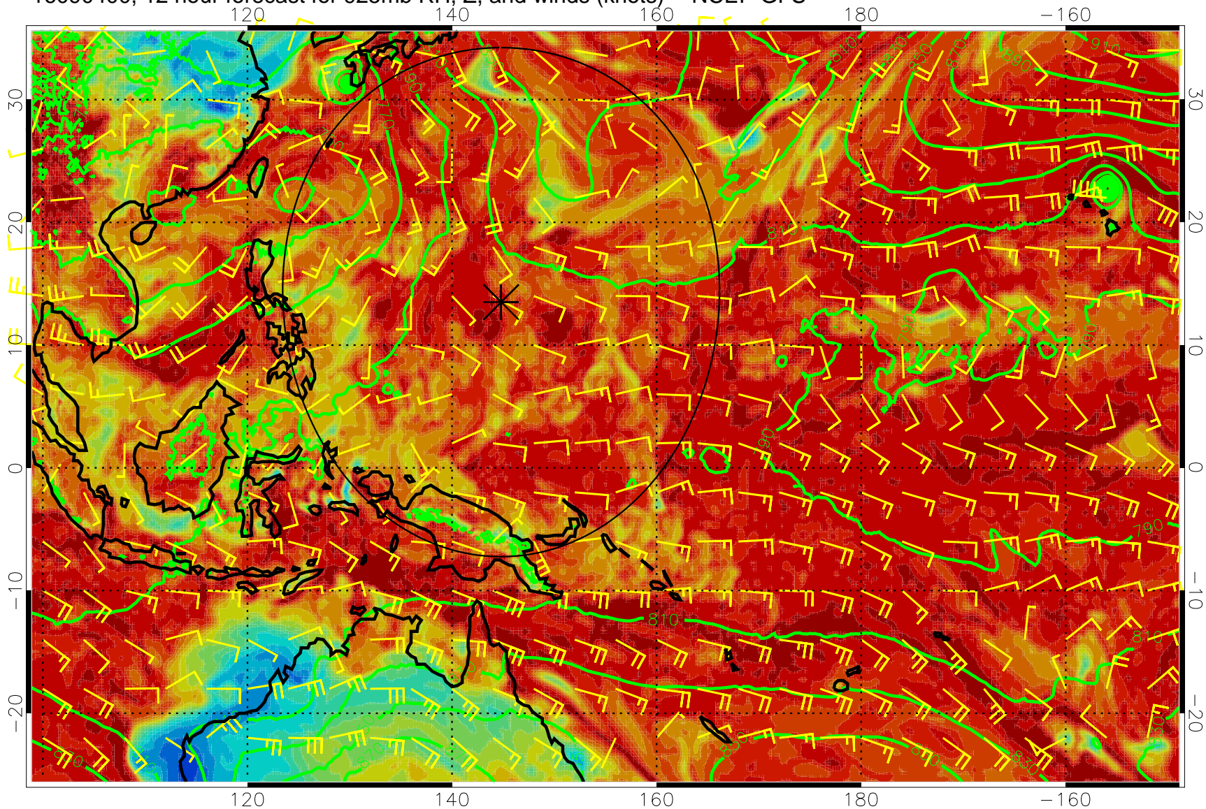
16090400, 12 hour forecast for 925mb RH, Z, and winds (knots) -- NCEP GFS
