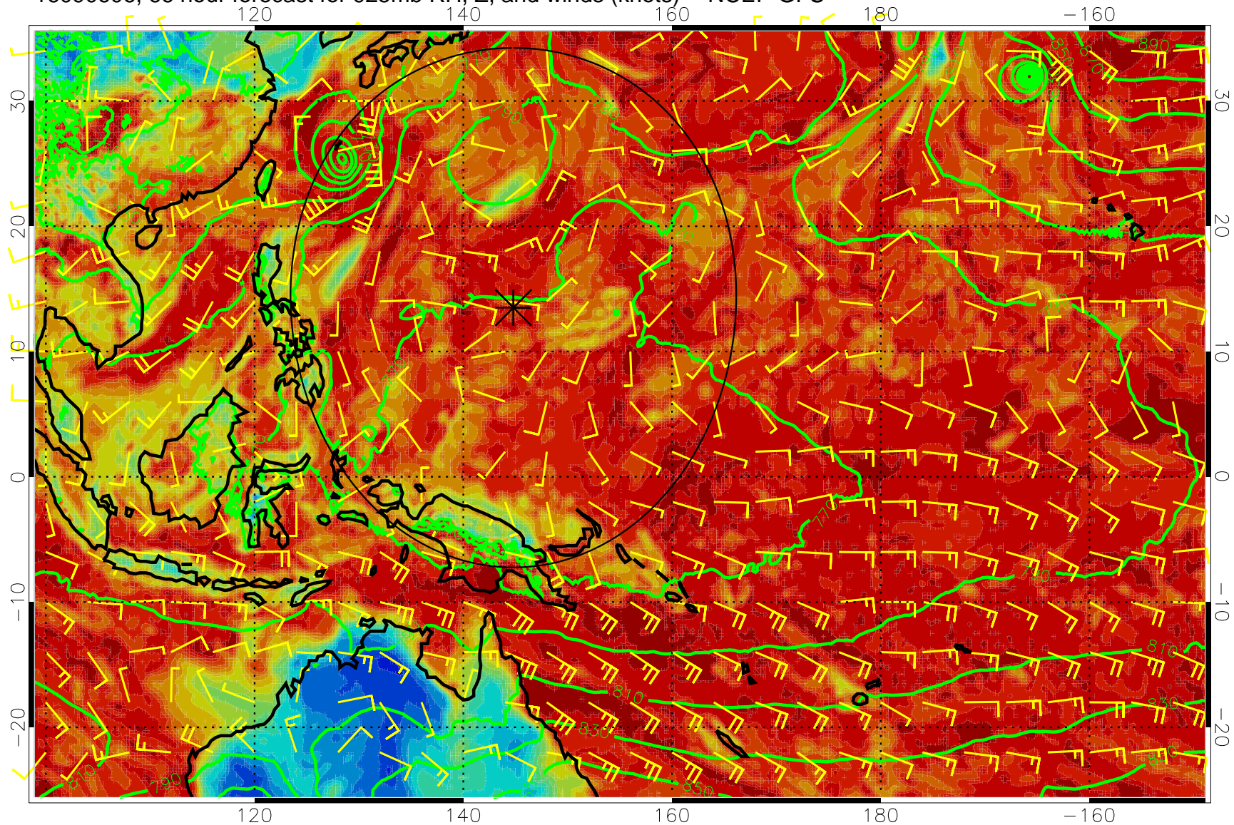
16090606, 66 hour forecast for 925mb RH, Z, and winds (knots) -- NCEP GFS
