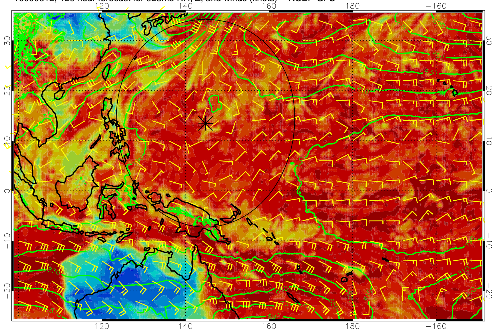
16090812, 120 hour forecast for 925mb RH, Z, and winds (knots) -- NCEP GFS
