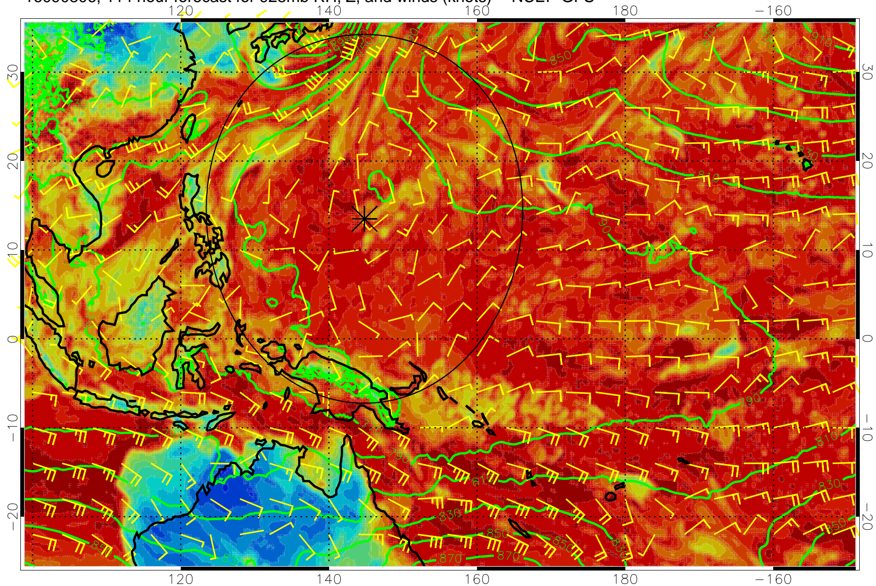
16090806, 114 hour forecast for 925mb RH, Z, and winds (knots) -- NCEP GFS
