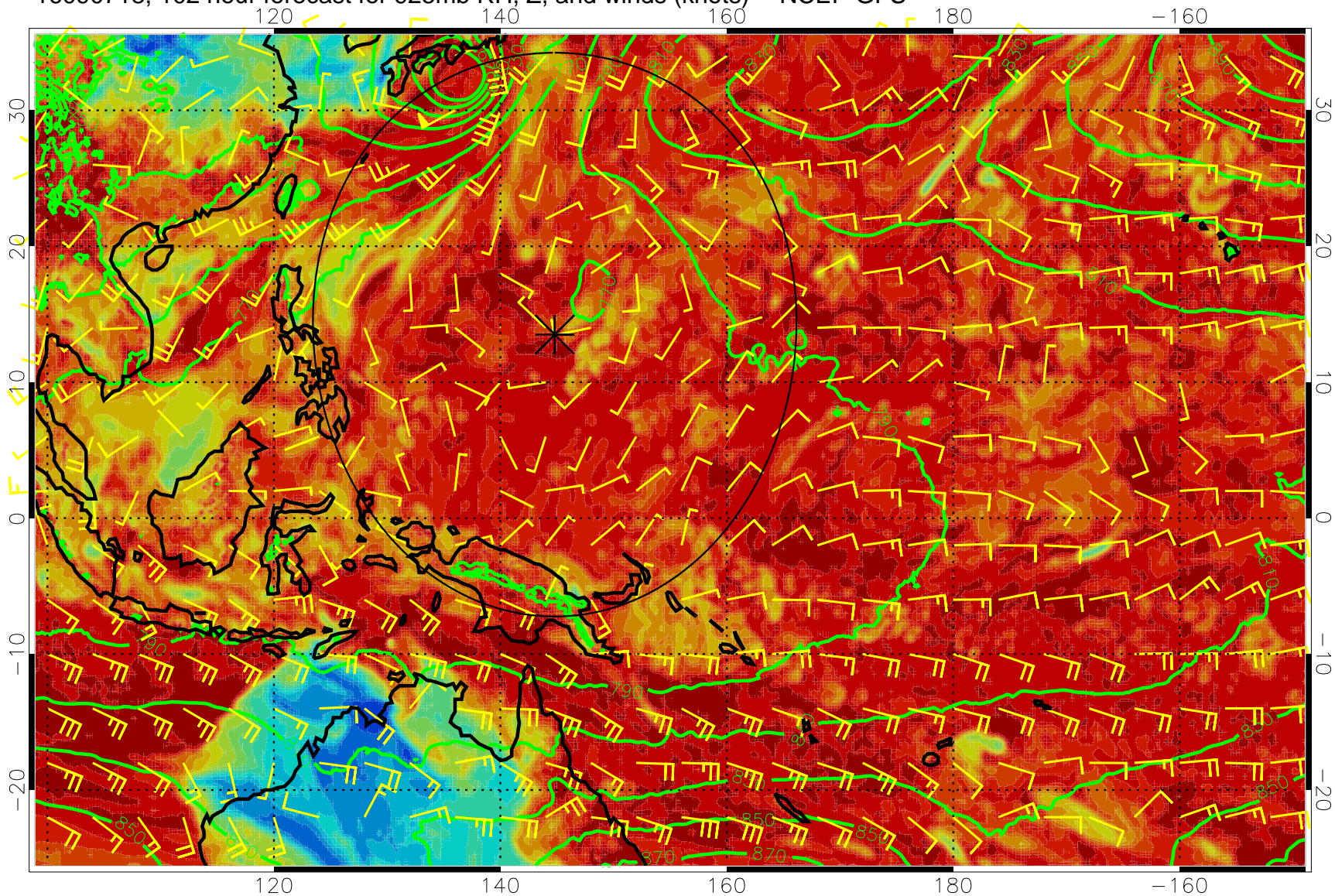
16090718, 102 hour forecast for 925mb RH, Z, and winds (knots) -- NCEP GFS
