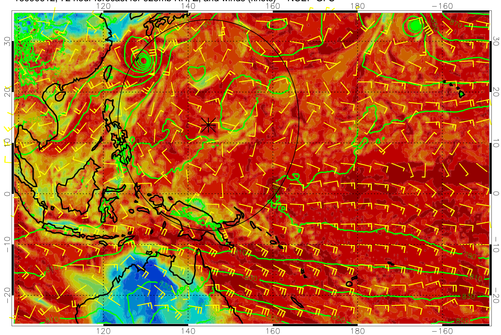
16090612, 72 hour forecast for 925mb RH, Z, and winds (knots) -- NCEP GFS
