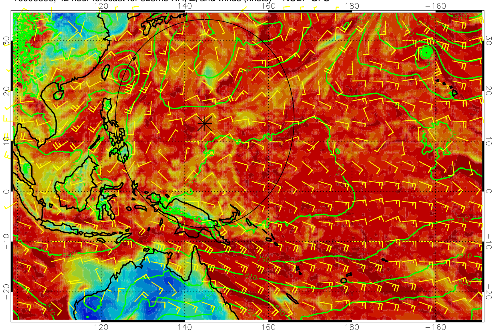
16090506, 42 hour forecast for 925mb RH, Z, and winds (knots) -- NCEP GFS
