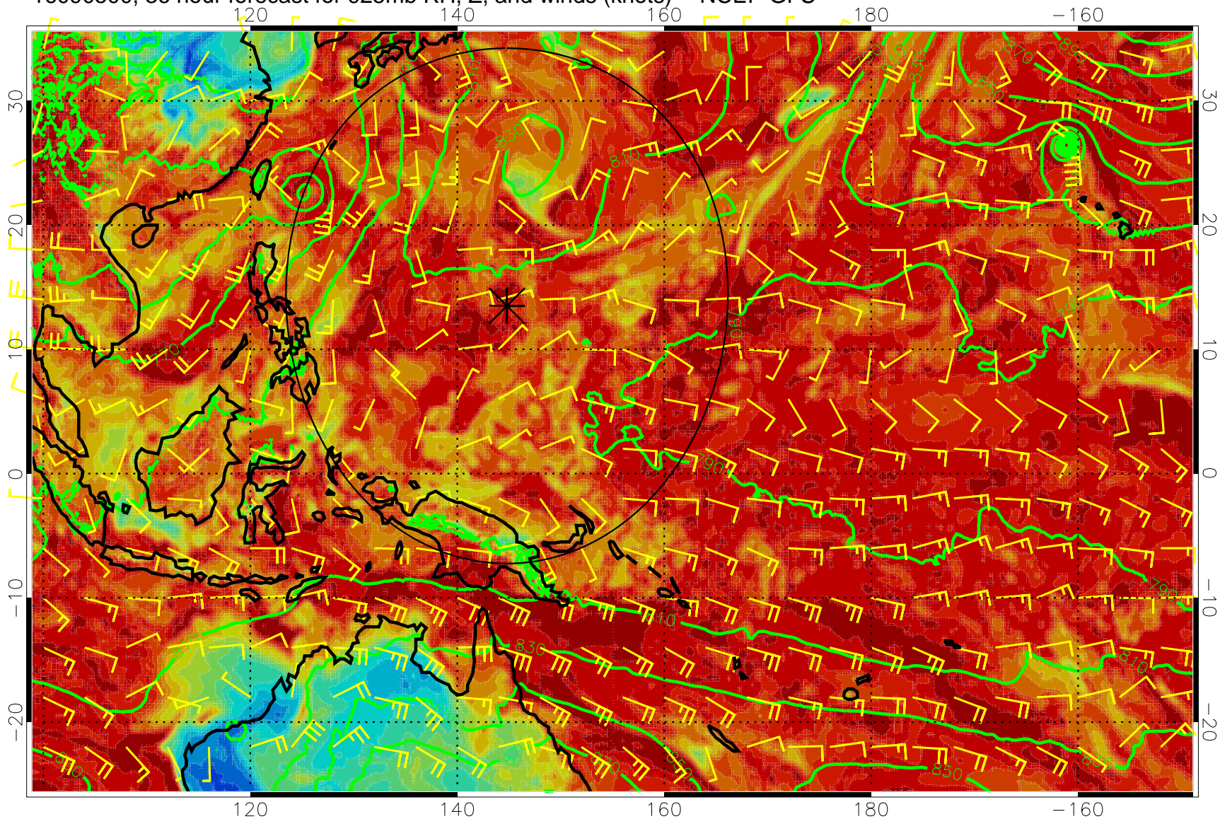
16090500, 36 hour forecast for 925mb RH, Z, and winds (knots) -- NCEP GFS
