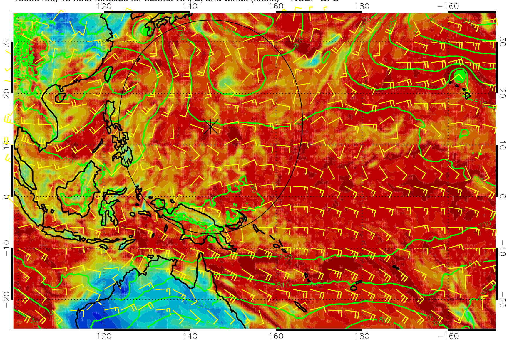
16090406, 18 hour forecast for 925mb RH, Z, and winds (knots) -- NCEP GFS
