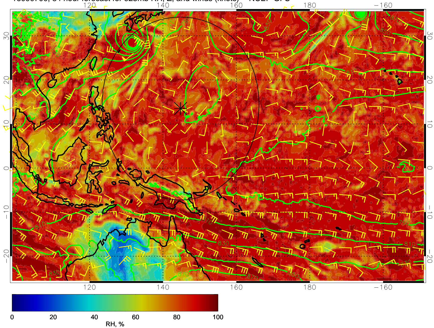
16090700, 84 hour forecast for 925mb RH, Z, and winds (knots) -- NCEP GFS
