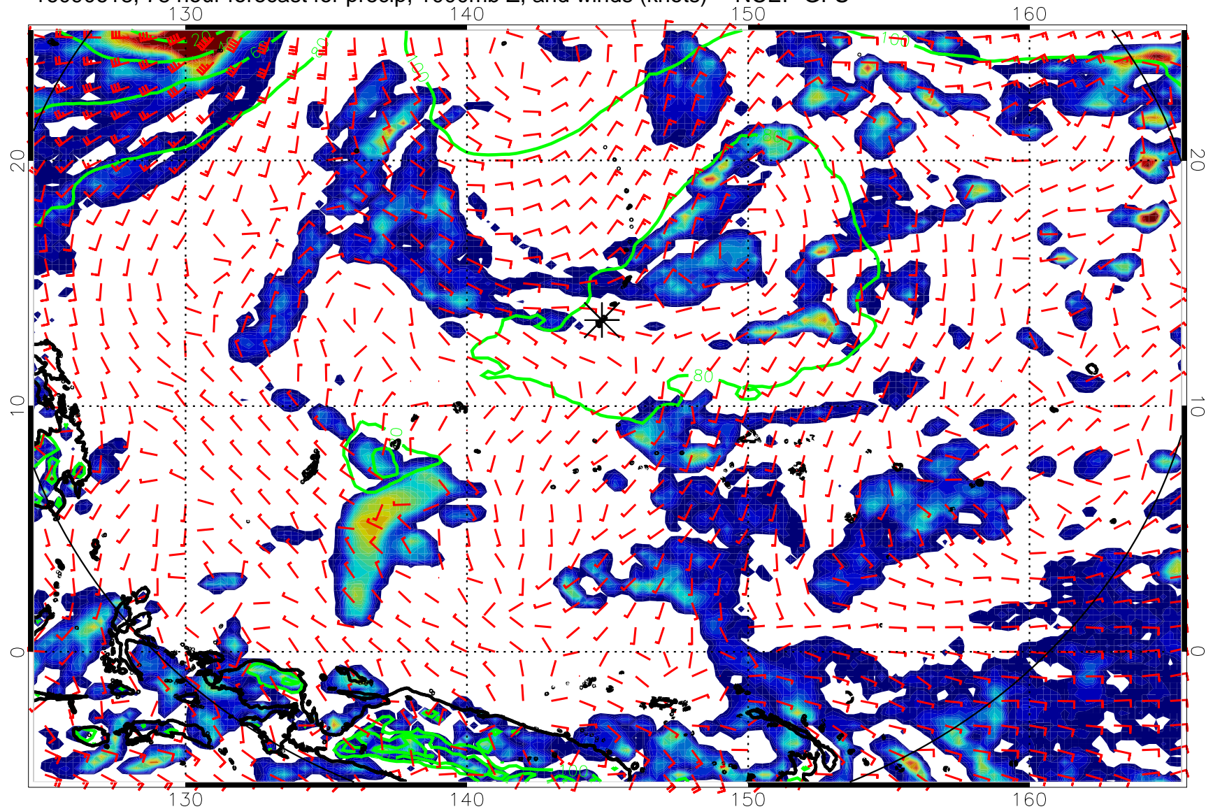
16090618, 78 hour forecast for precip, 1000mb Z, and winds (knots) -- NCEP GFS
