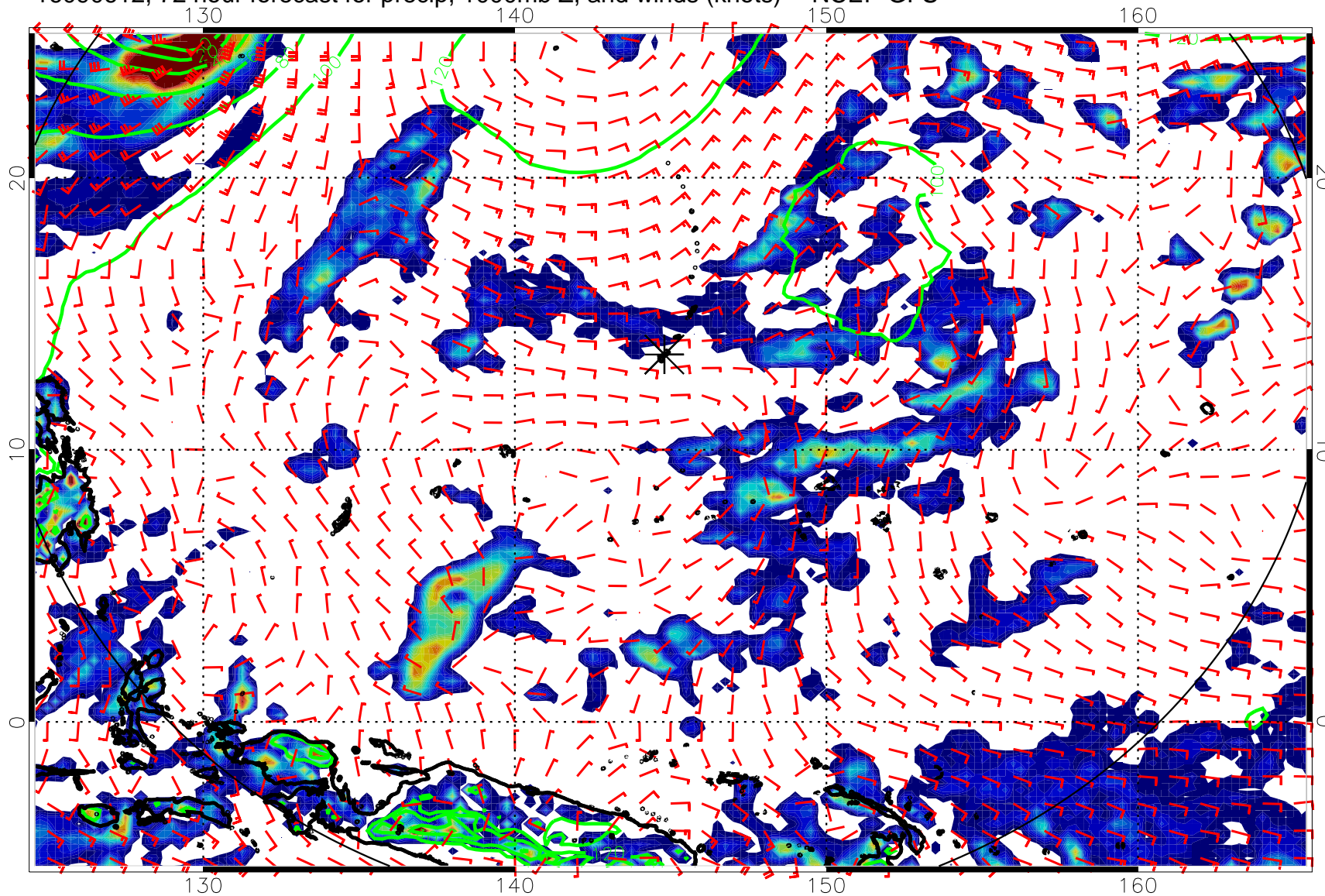
16090612, 72 hour forecast for precip, 1000mb Z, and winds (knots) -- NCEP GFS
