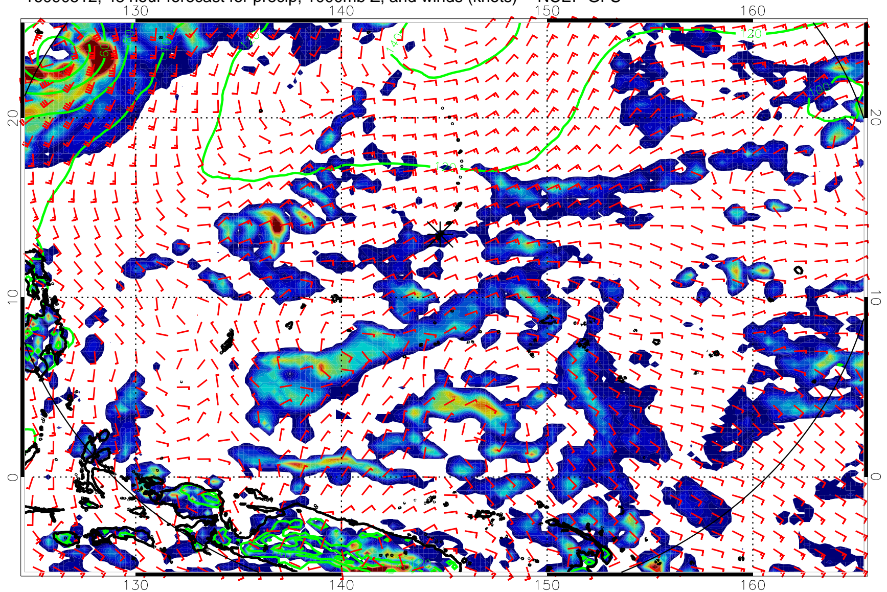
16090512, 48 hour forecast for precip, 1000mb Z, and winds (knots) -- NCEP GFS
