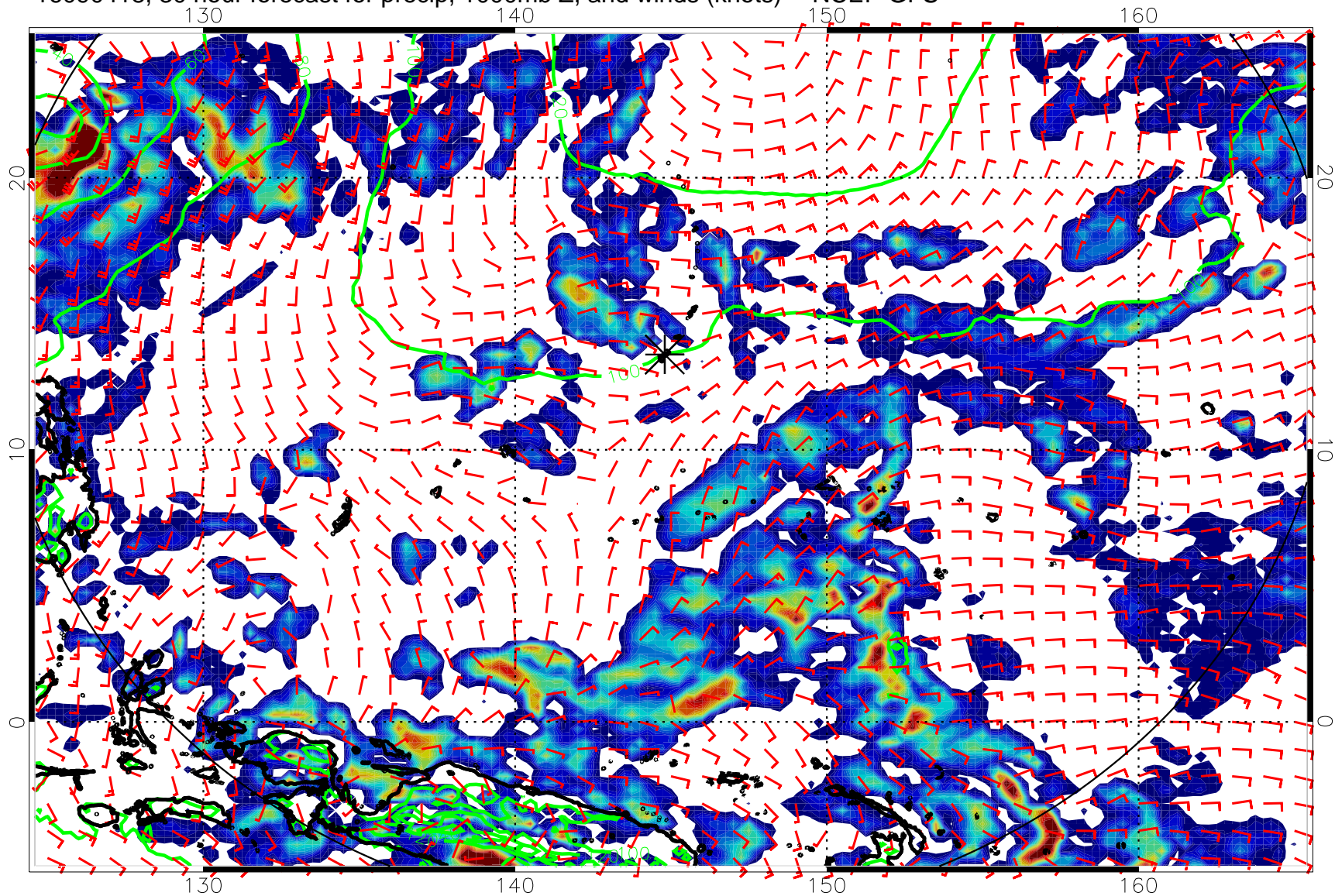
16090418, 30 hour forecast for precip, 1000mb Z, and winds (knots) -- NCEP GFS
