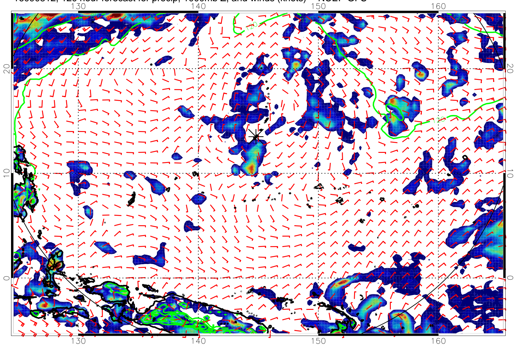
16090812, 120 hour forecast for precip, 1000mb Z, and winds (knots) -- NCEP GFS
