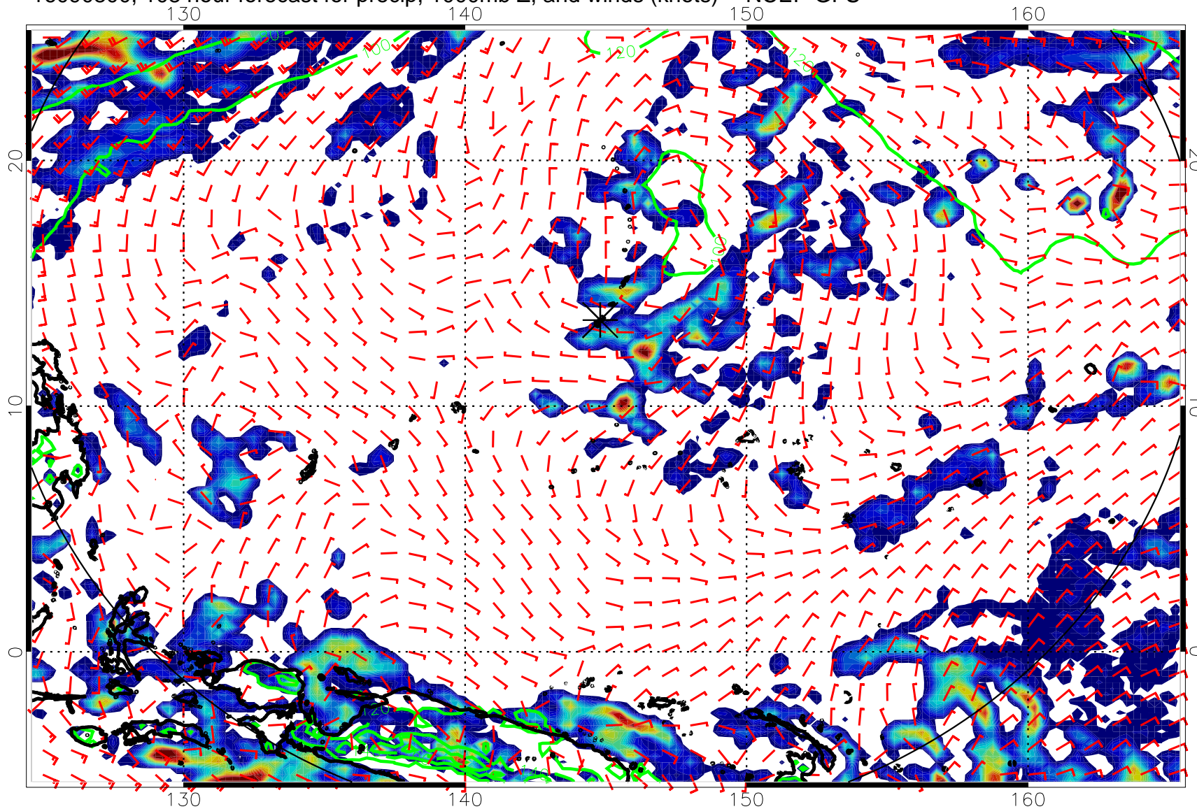
16090800, 108 hour forecast for precip, 1000mb Z, and winds (knots) -- NCEP GFS
