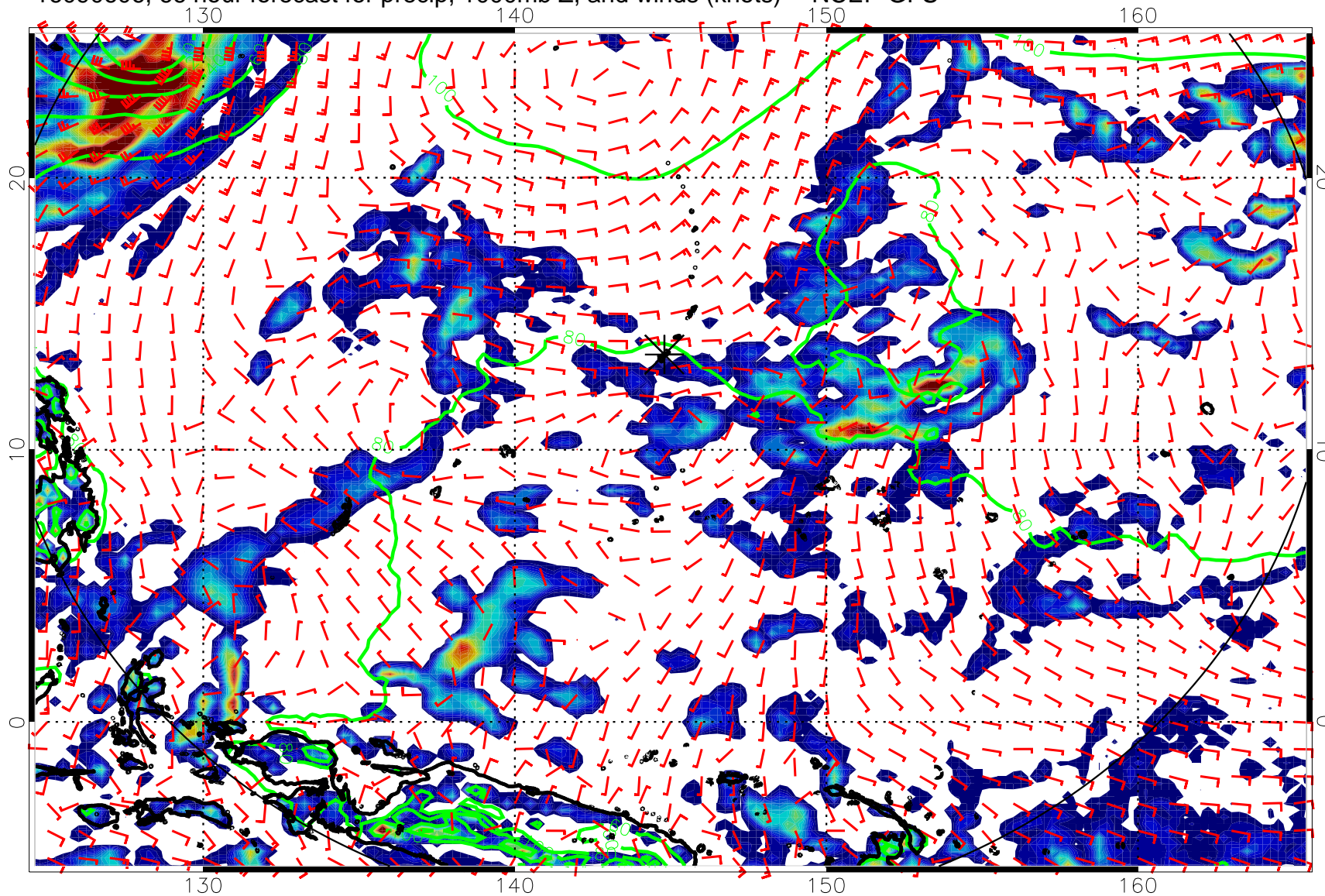
16090606, 66 hour forecast for precip, 1000mb Z, and winds (knots) -- NCEP GFS
