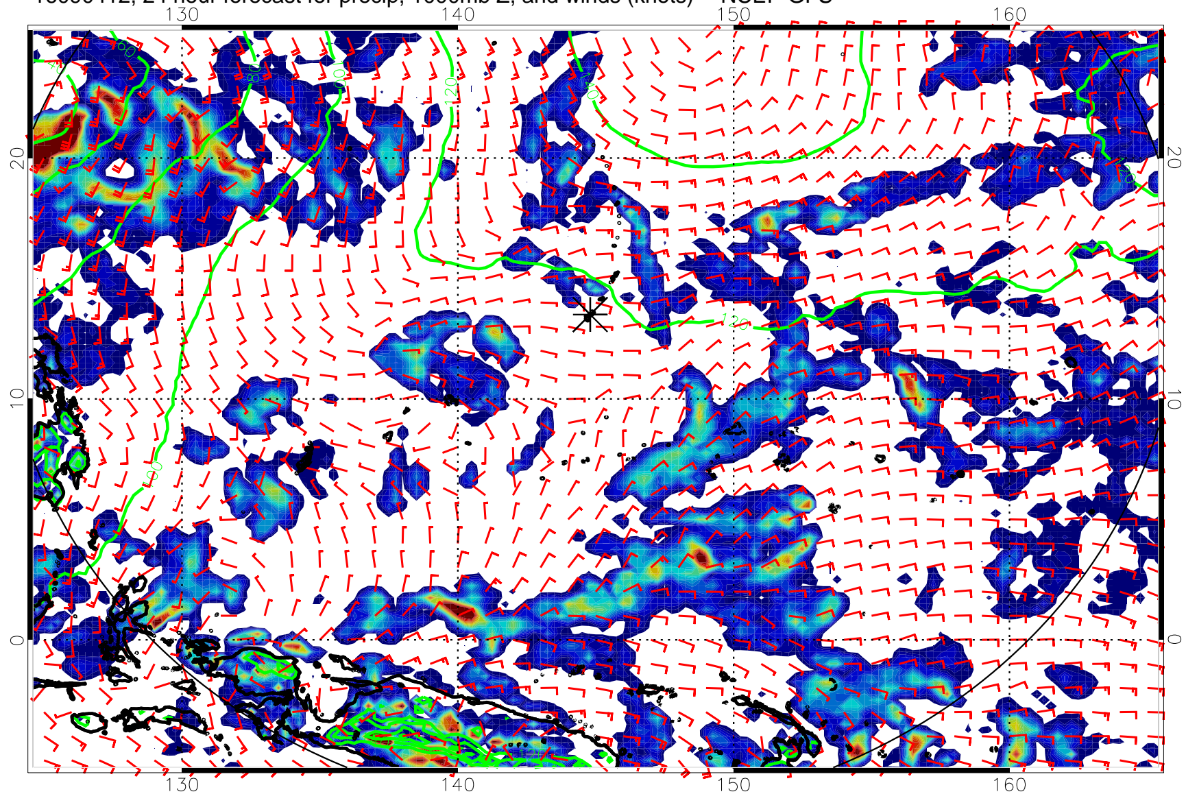
16090412, 24 hour forecast for precip, 1000mb Z, and winds (knots) -- NCEP GFS
