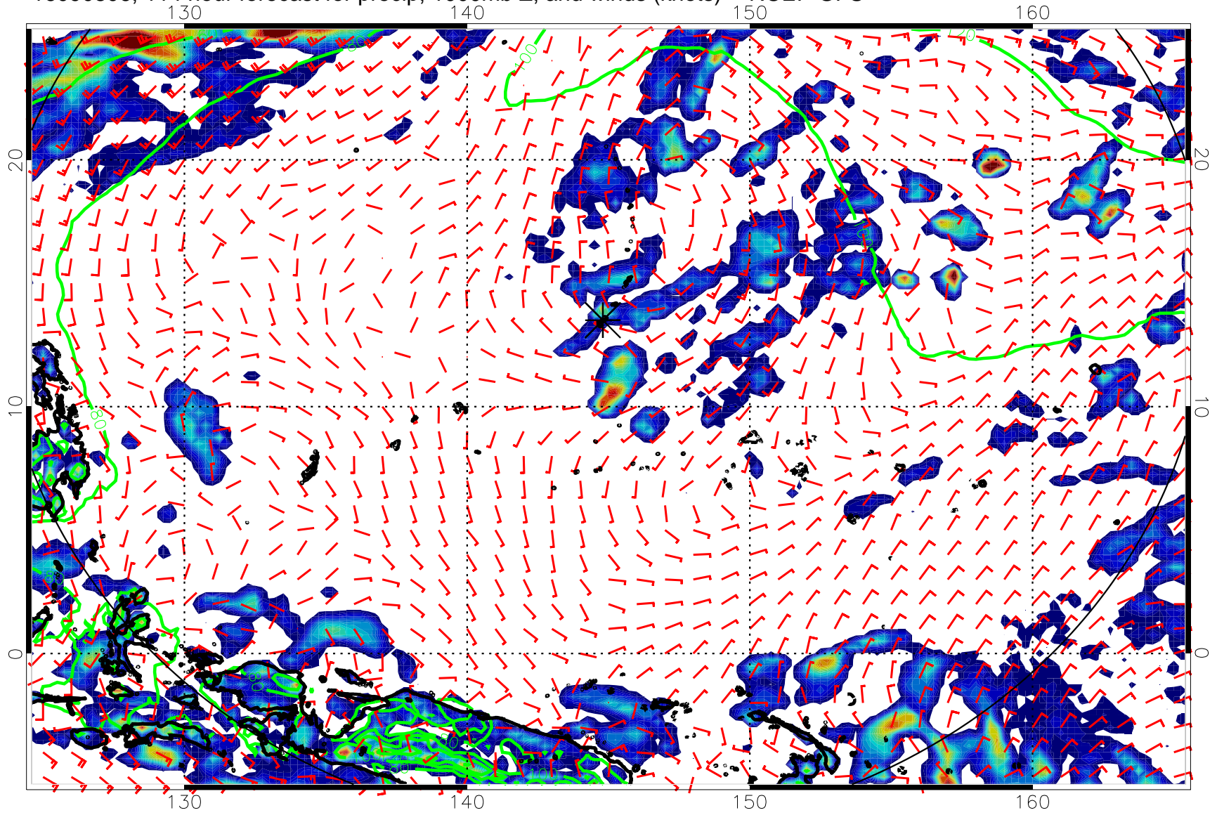
16090806, 114 hour forecast for precip, 1000mb Z, and winds (knots) -- NCEP GFS
