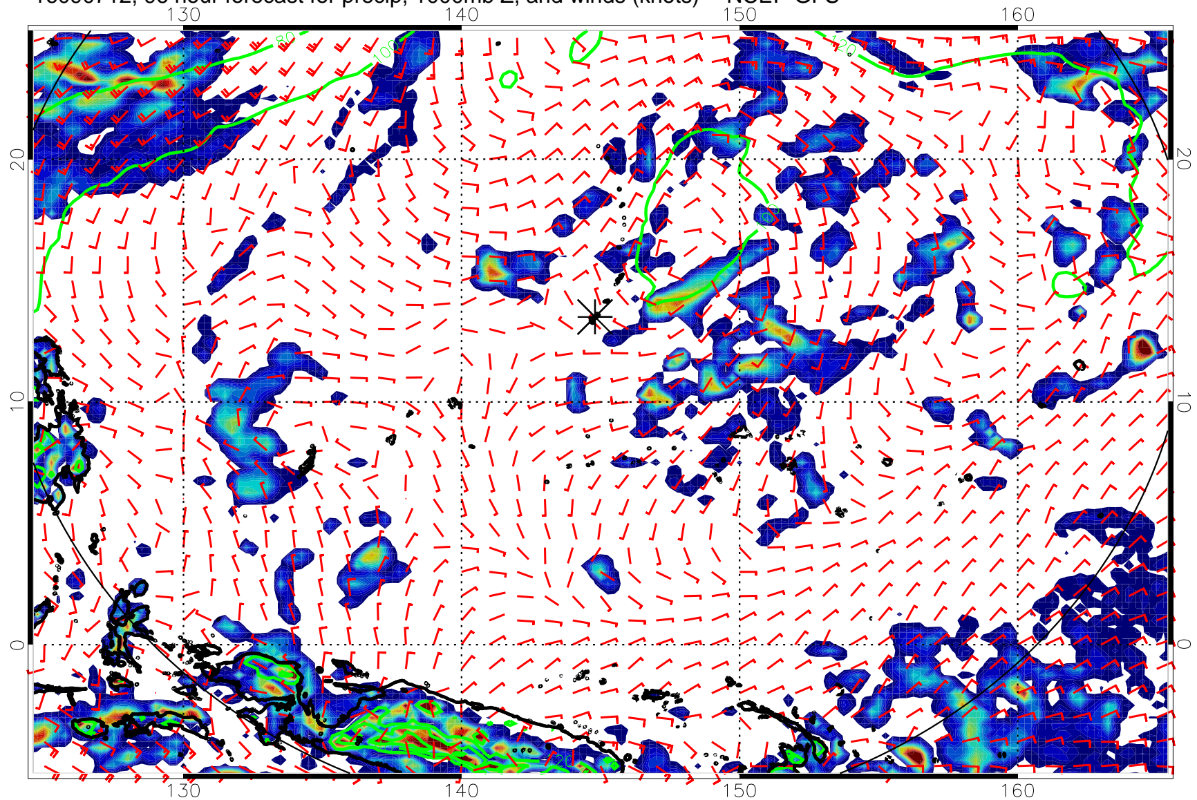
16090712, 96 hour forecast for precip, 1000mb Z, and winds (knots) -- NCEP GFS
