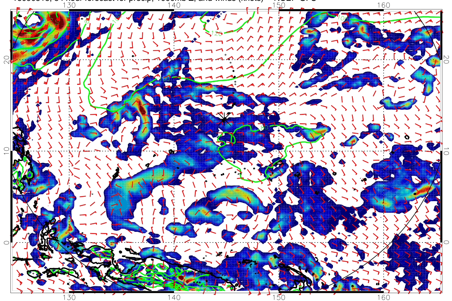
16090518, 54 hour forecast for precip, 1000mb Z, and winds (knots) -- NCEP GFS
