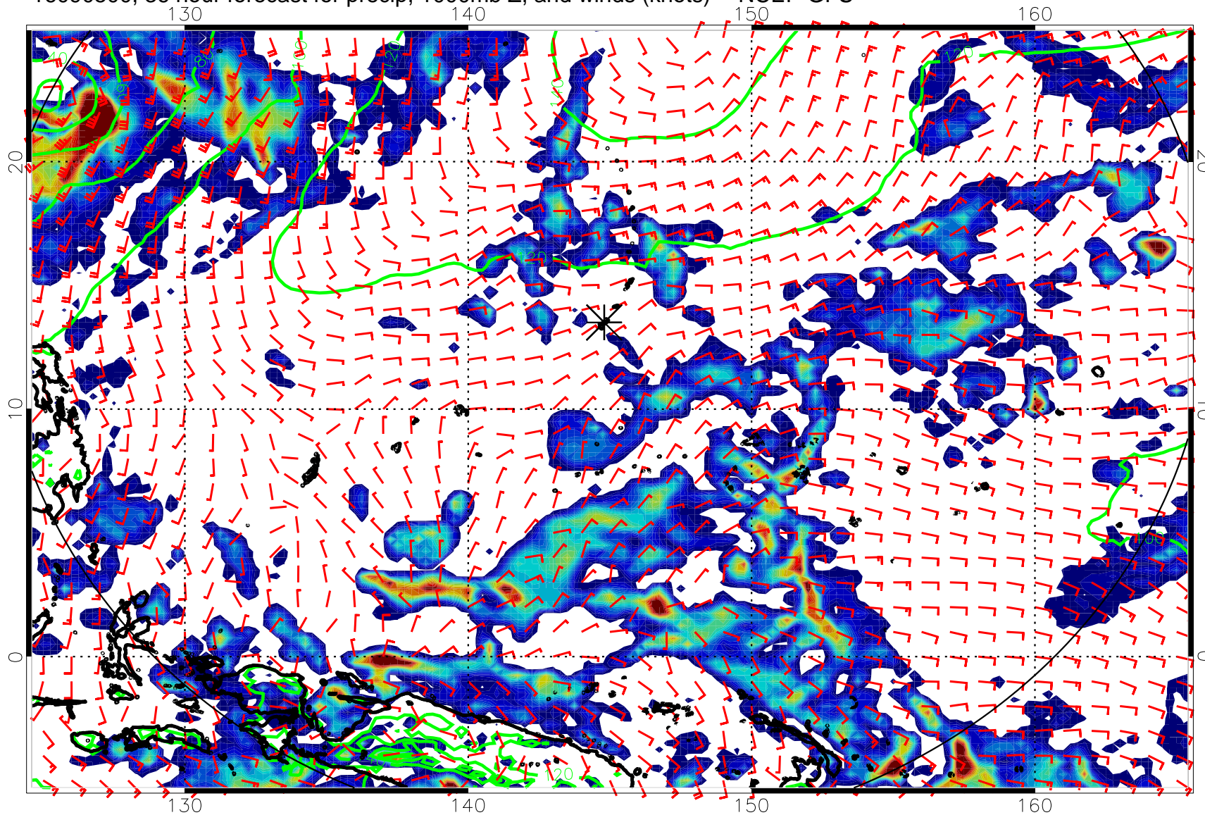
16090500, 36 hour forecast for precip, 1000mb Z, and winds (knots) -- NCEP GFS
