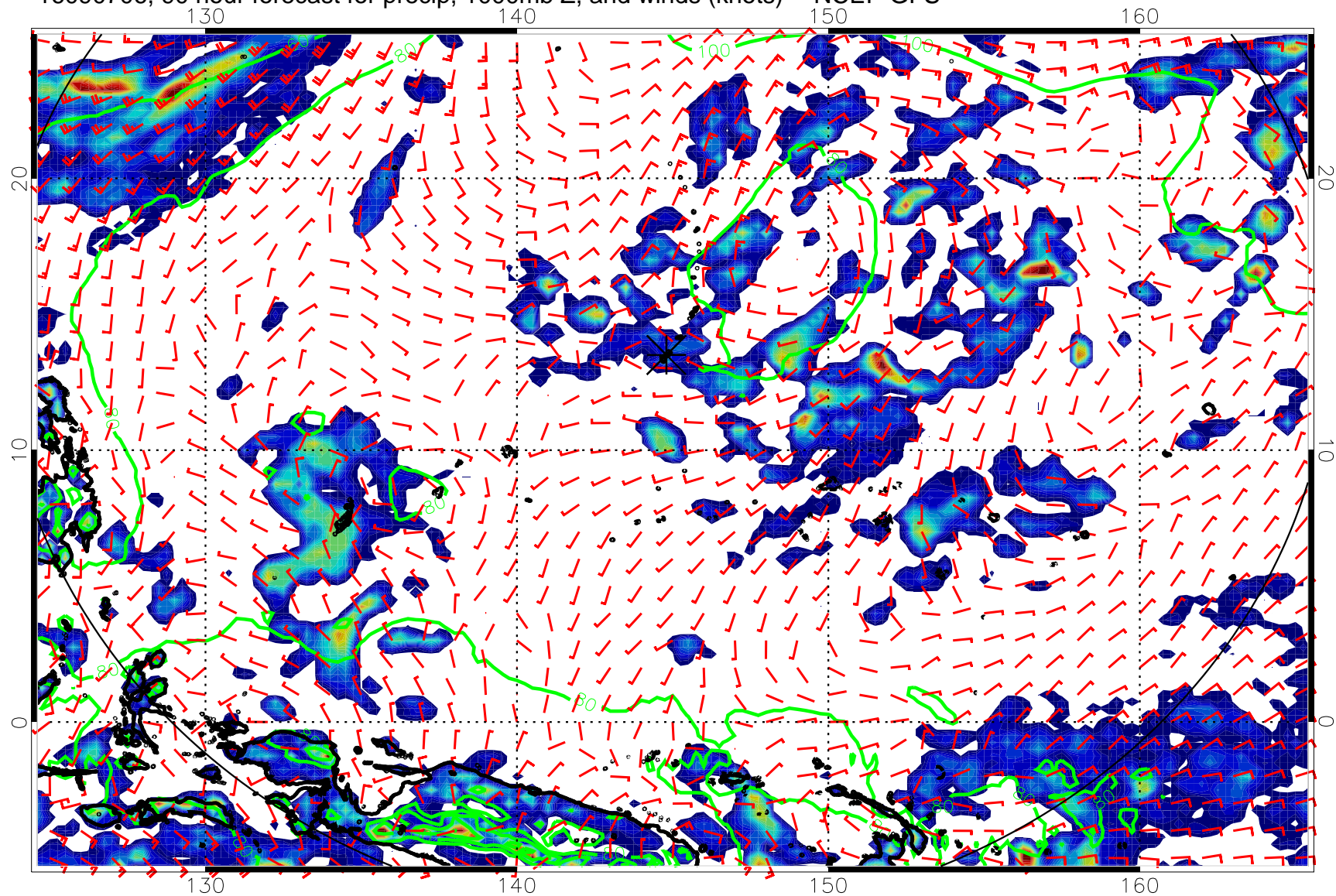
16090706, 90 hour forecast for precip, 1000mb Z, and winds (knots) -- NCEP GFS
