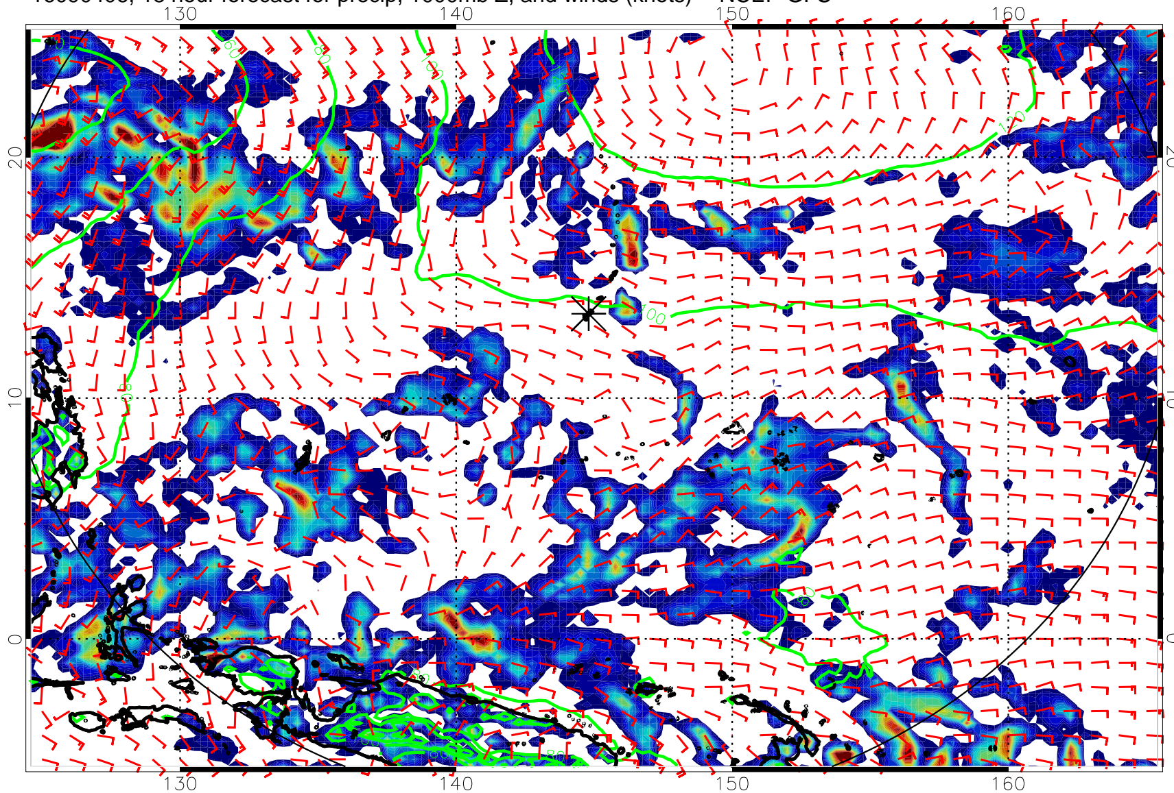
16090406, 18 hour forecast for precip, 1000mb Z, and winds (knots) -- NCEP GFS
