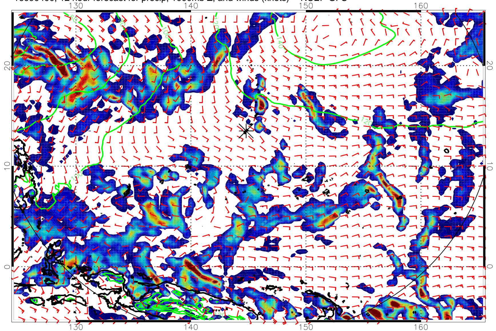
16090400, 12 hour forecast for precip, 1000mb Z, and winds (knots) -- NCEP GFS
