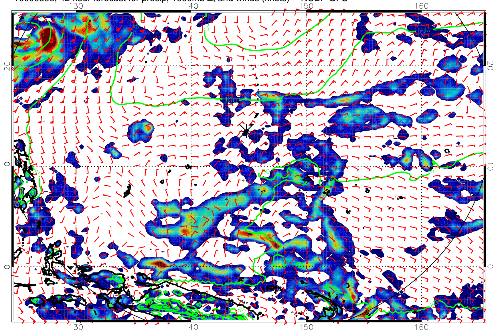
16090506, 42 hour forecast for precip, 1000mb Z, and winds (knots) -- NCEP GFS
