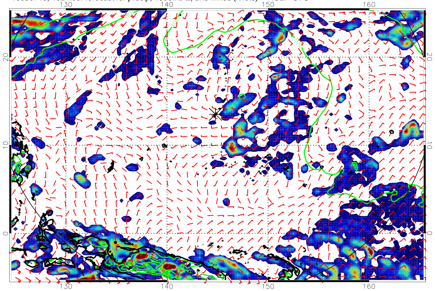
16090718, 102 hour forecast for precip, 1000mb Z, and winds (knots) -- NCEP GFS
