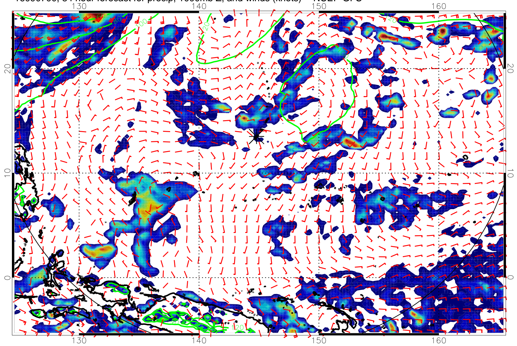
16090700, 84 hour forecast for precip, 1000mb Z, and winds (knots) -- NCEP GFS
