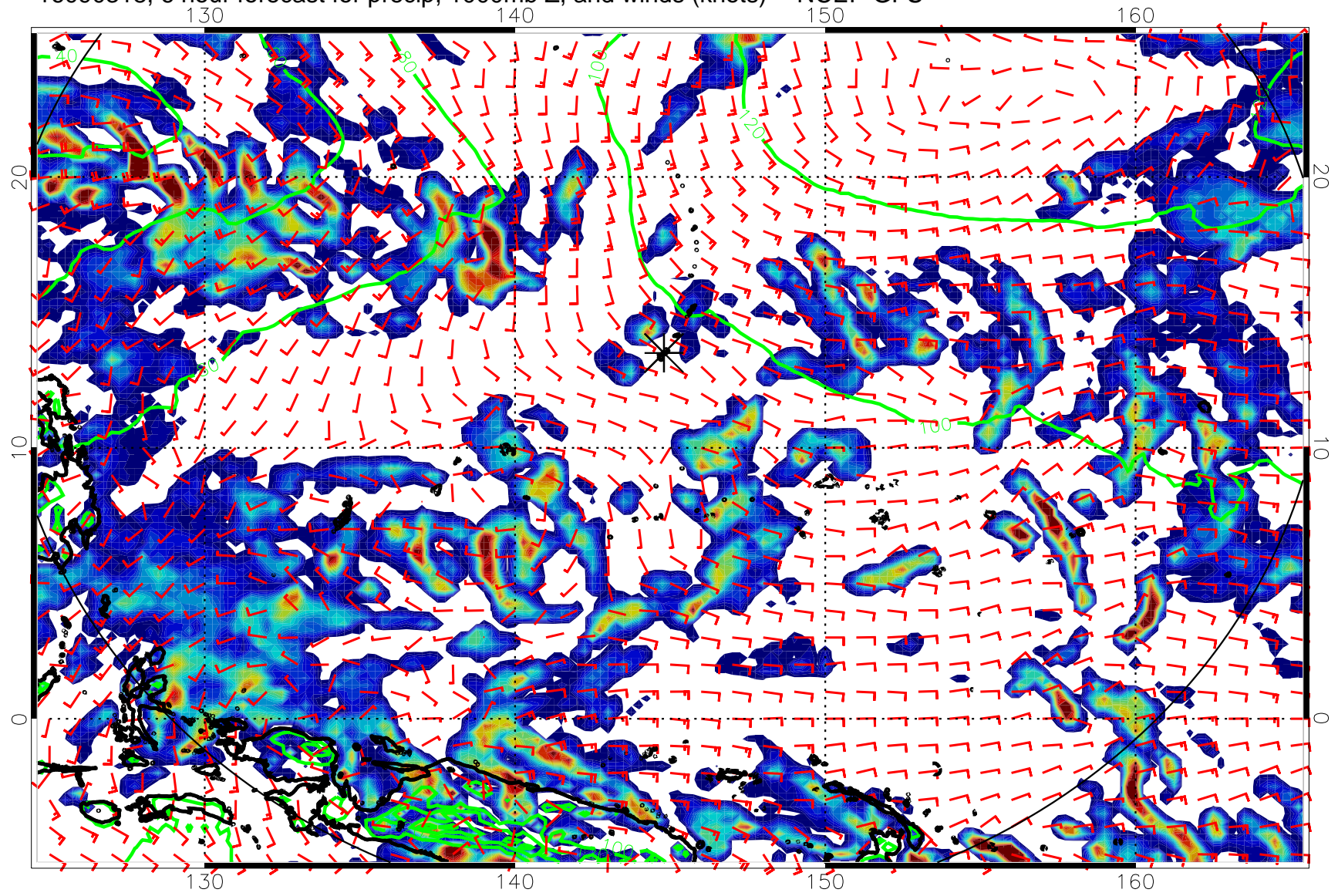
16090318, 6 hour forecast for precip, 1000mb Z, and winds (knots) -- NCEP GFS
