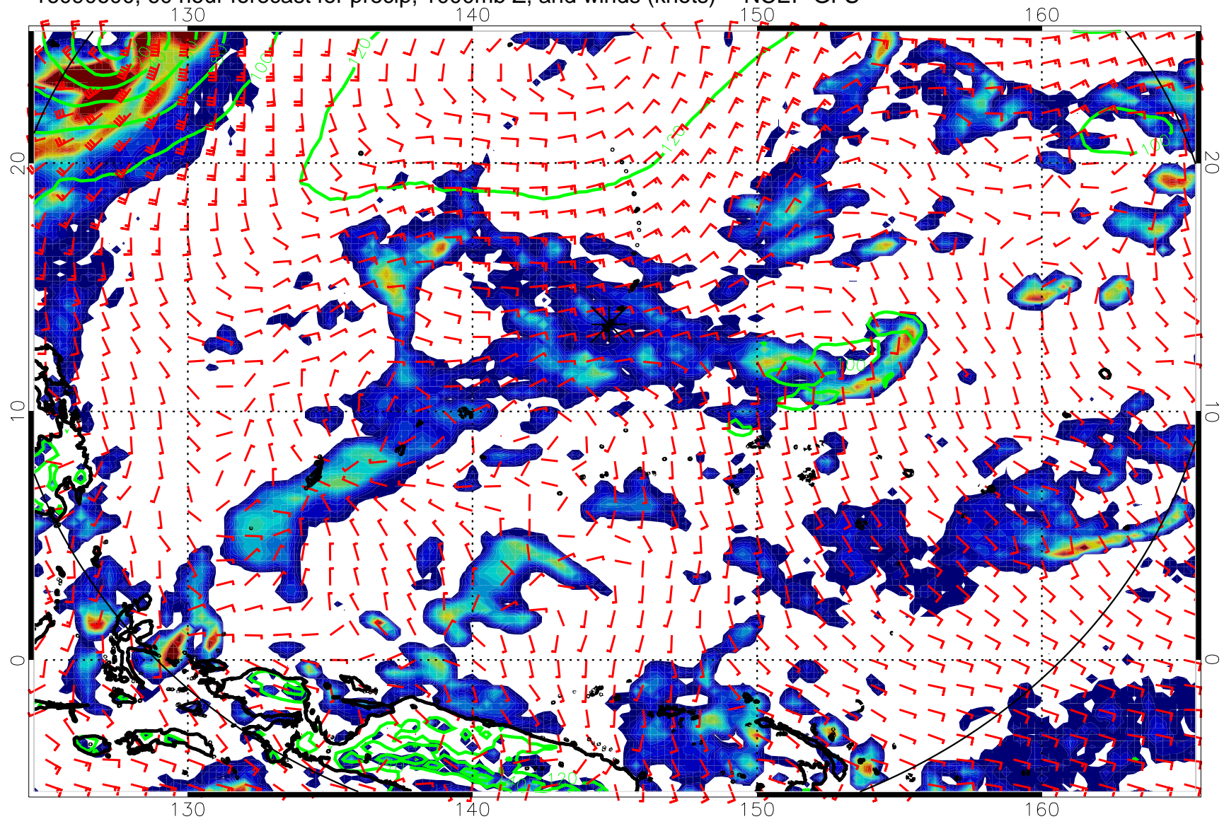
16090600, 60 hour forecast for precip, 1000mb Z, and winds (knots) -- NCEP GFS
