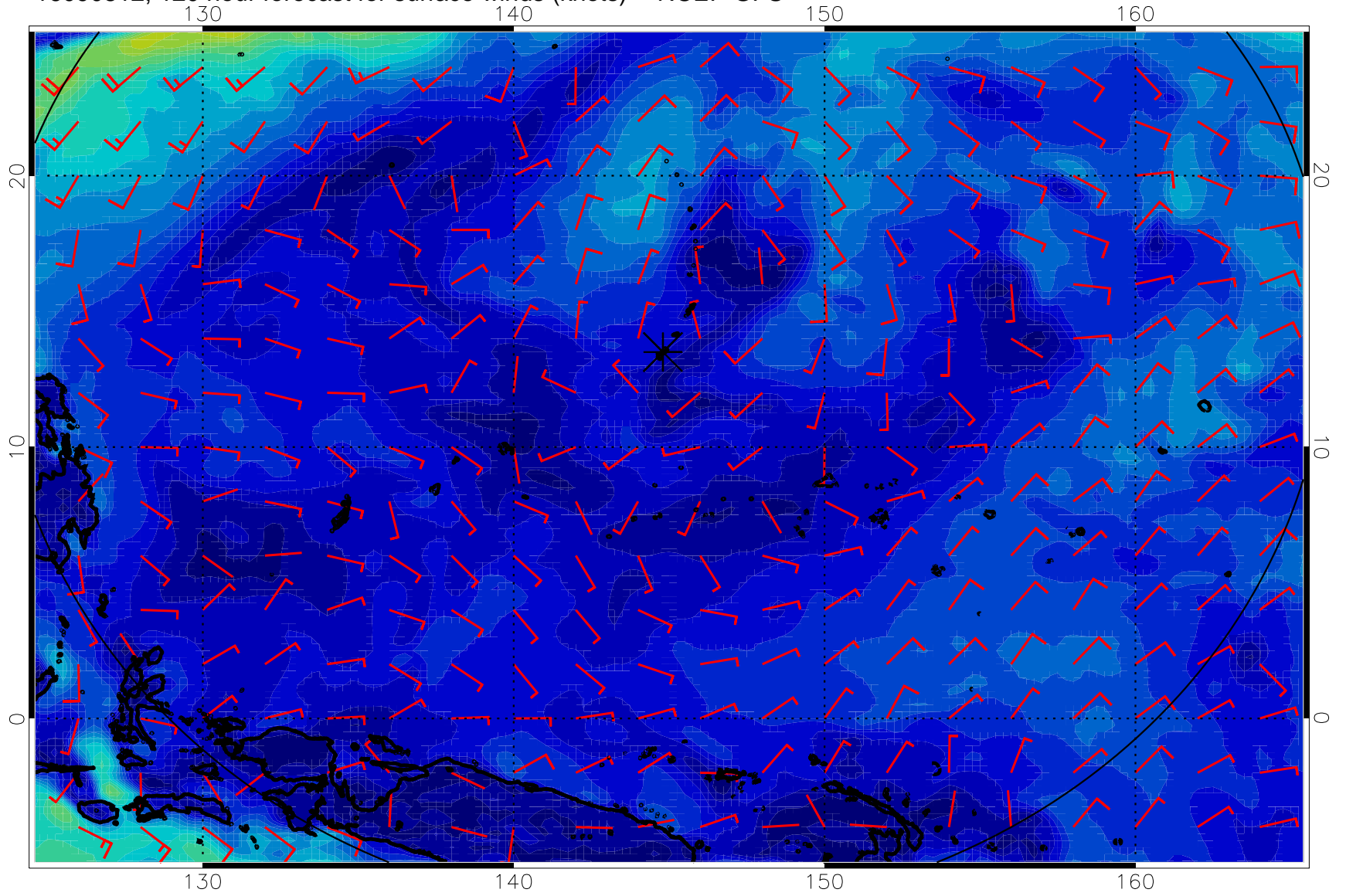
16090812, 120 hour forecast for surface winds (knots) -- NCEP GFS
