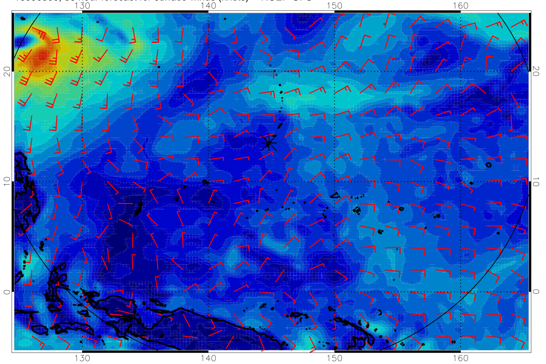
16090500, 36 hour forecast for surface winds (knots) -- NCEP GFS
