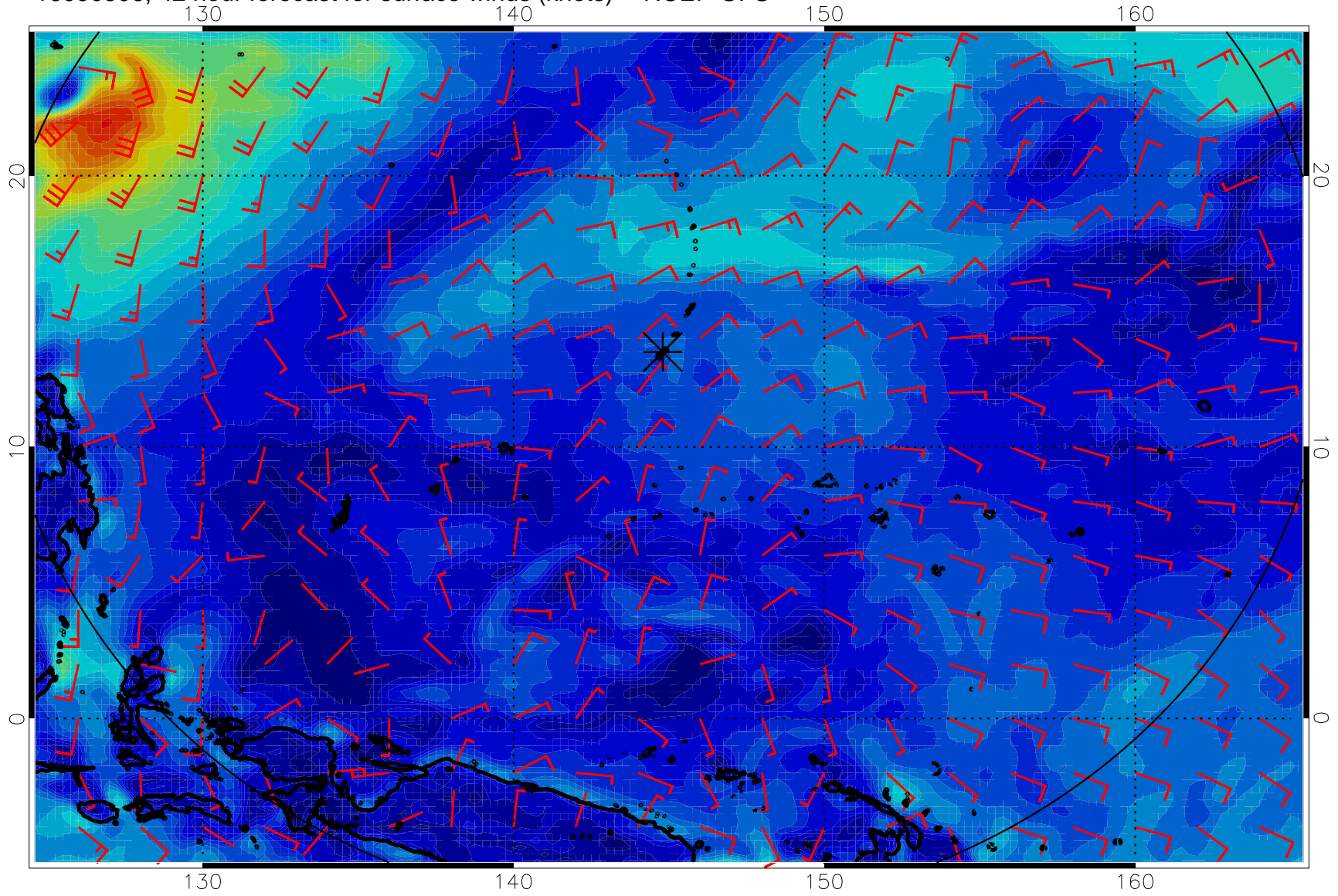
16090506, 42 hour forecast for surface winds (knots) -- NCEP GFS
