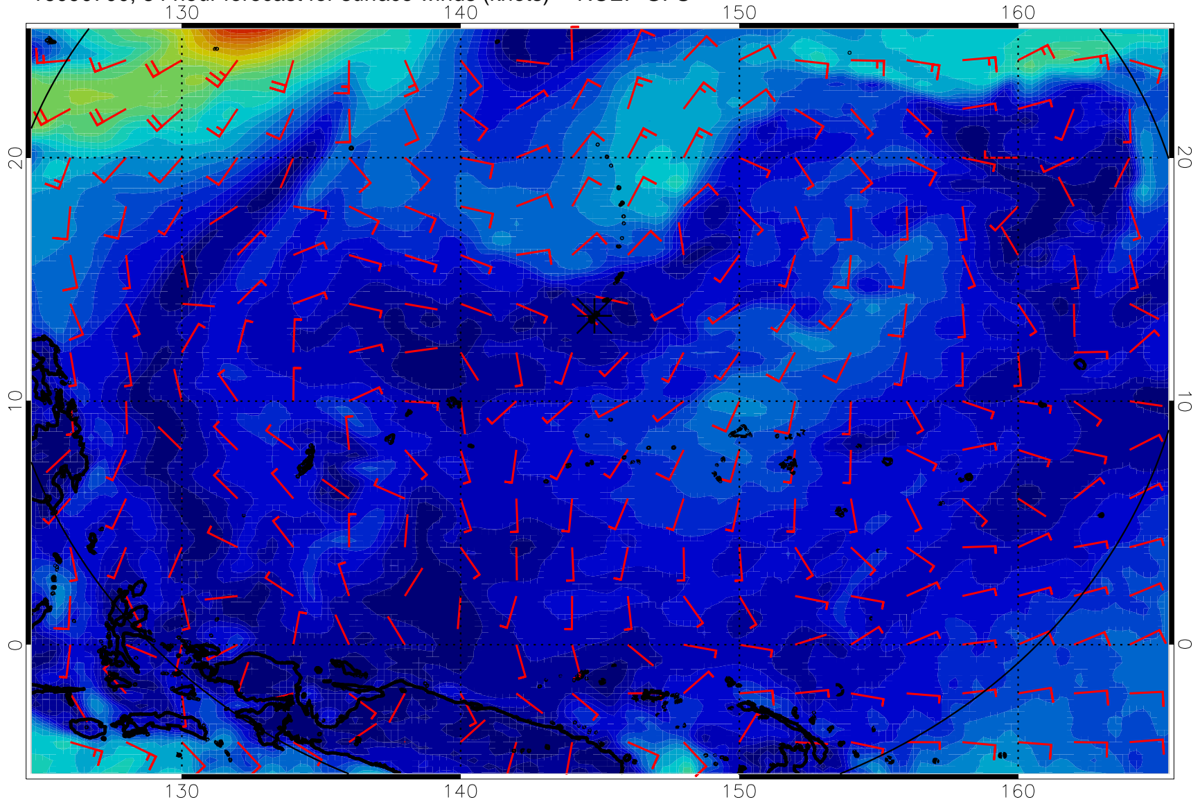
16090700, 84 hour forecast for surface winds (knots) -- NCEP GFS
