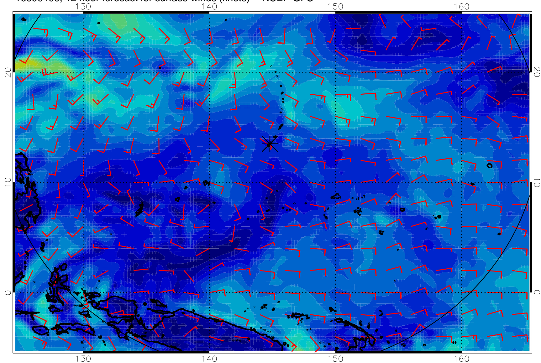
16090400, 12 hour forecast for surface winds (knots) -- NCEP GFS
