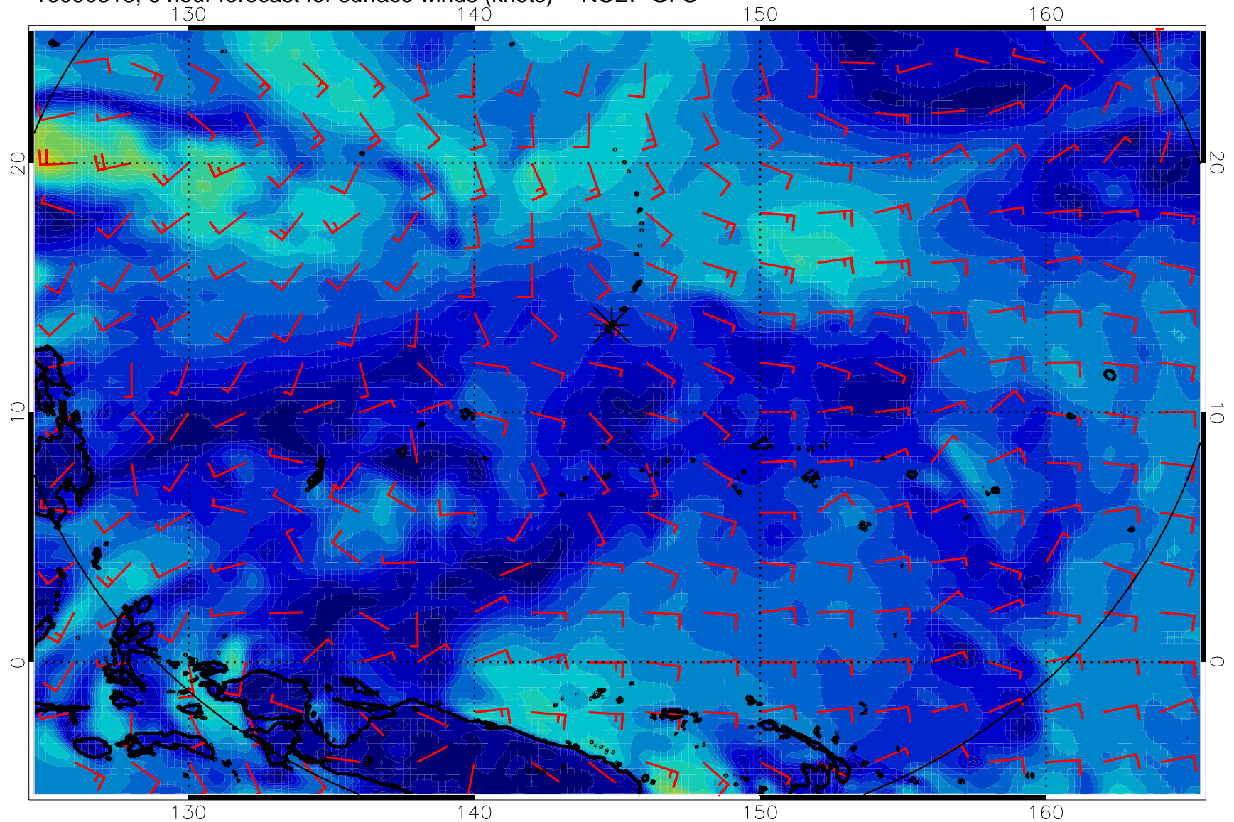
16090318, 6 hour forecast for surface winds (knots) -- NCEP GFS
