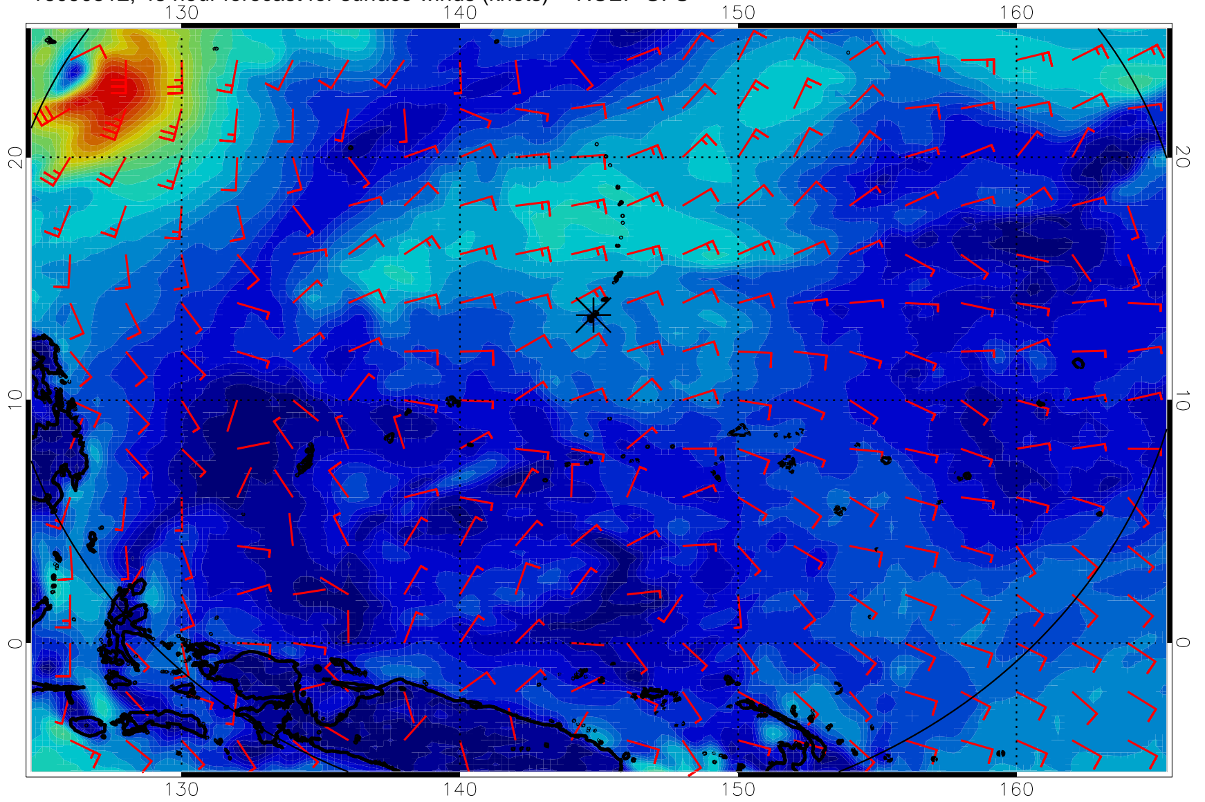
16090512, 48 hour forecast for surface winds (knots) -- NCEP GFS
