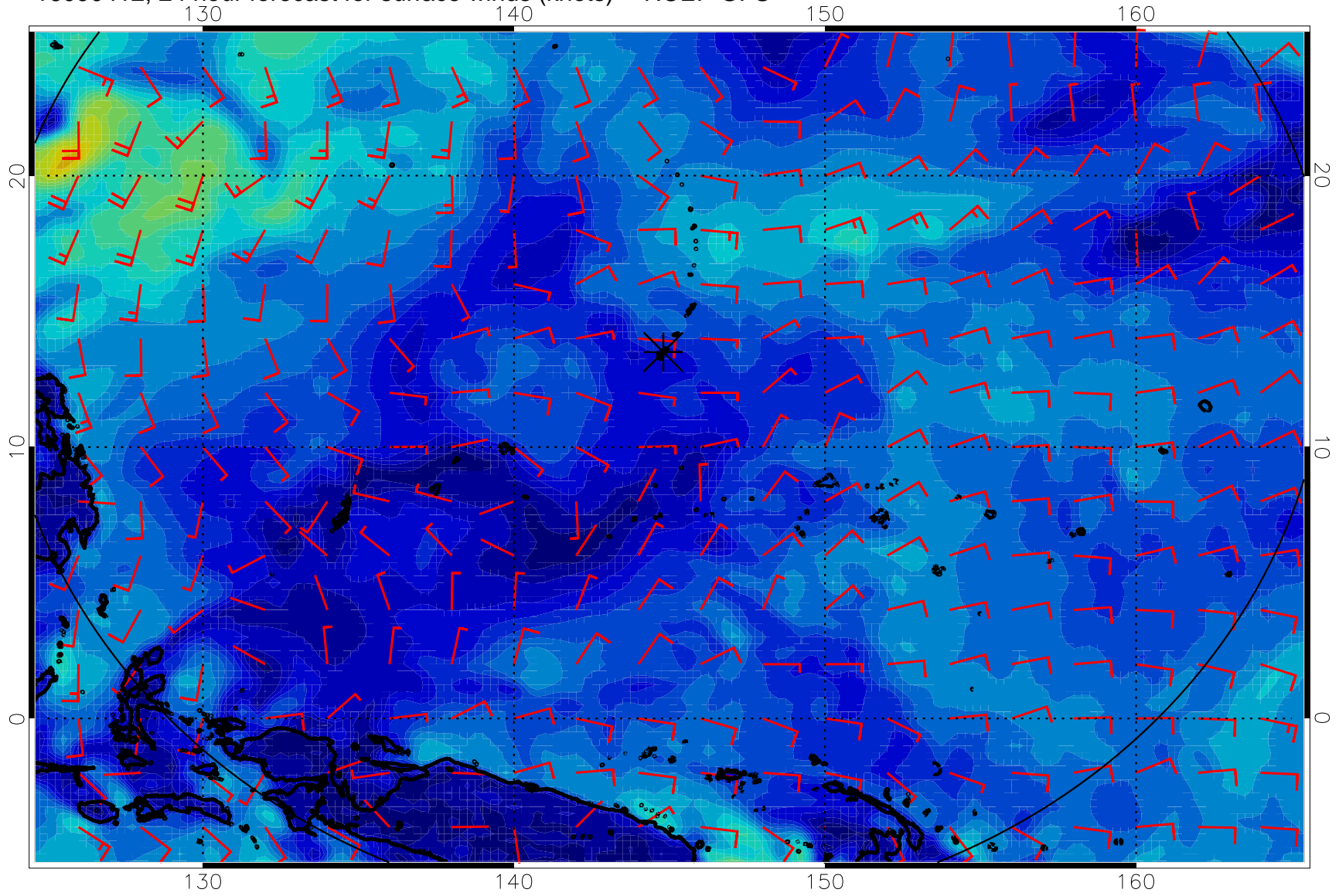
16090412, 24 hour forecast for surface winds (knots) -- NCEP GFS
