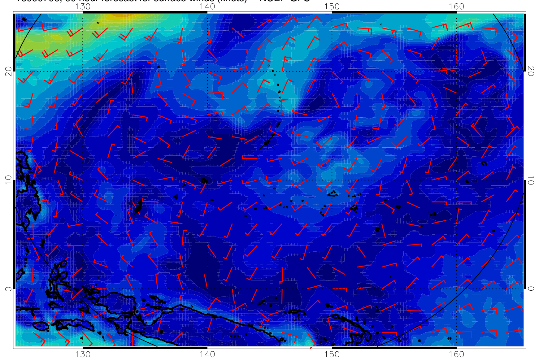
16090706, 90 hour forecast for surface winds (knots) -- NCEP GFS
