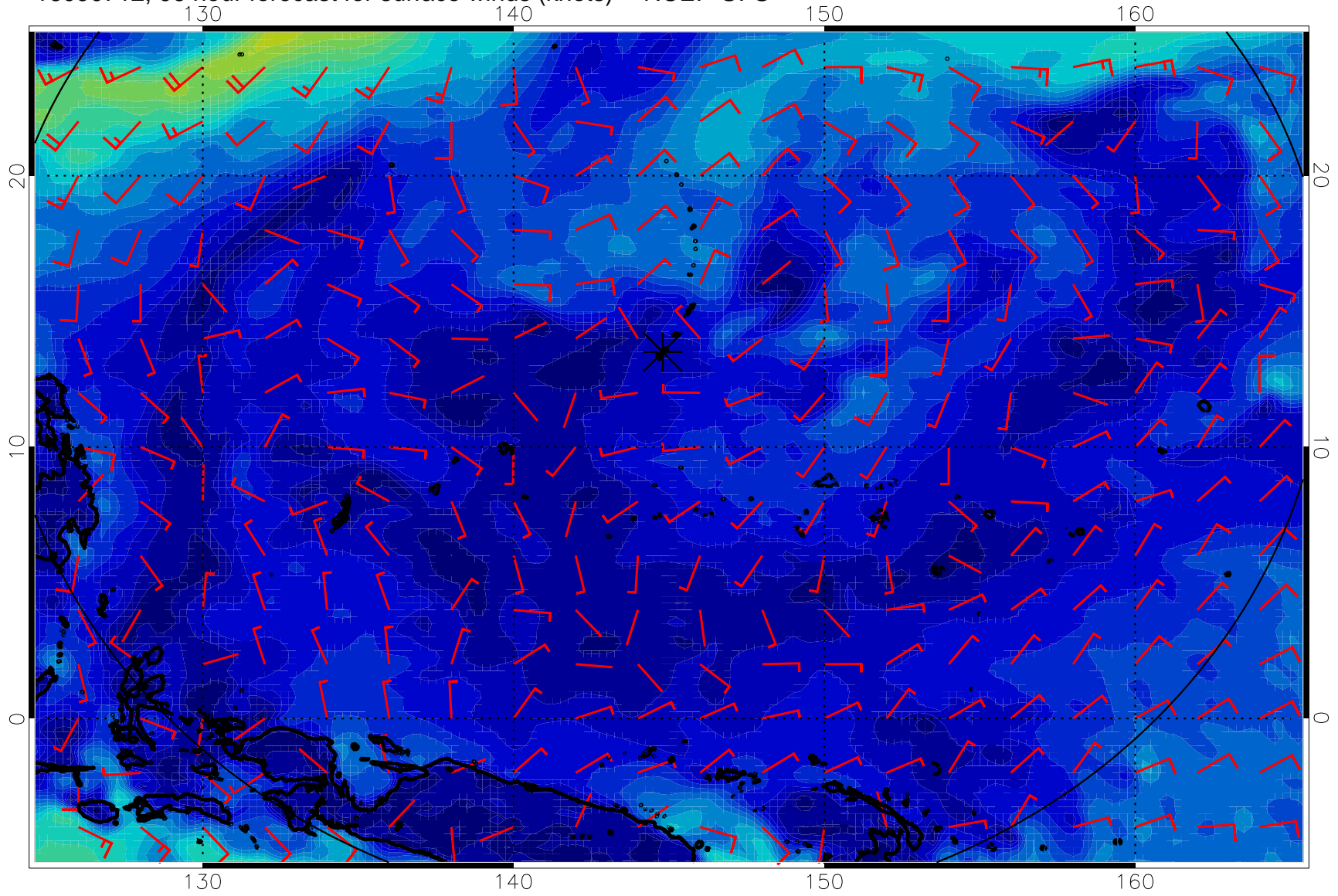
16090712, 96 hour forecast for surface winds (knots) -- NCEP GFS
