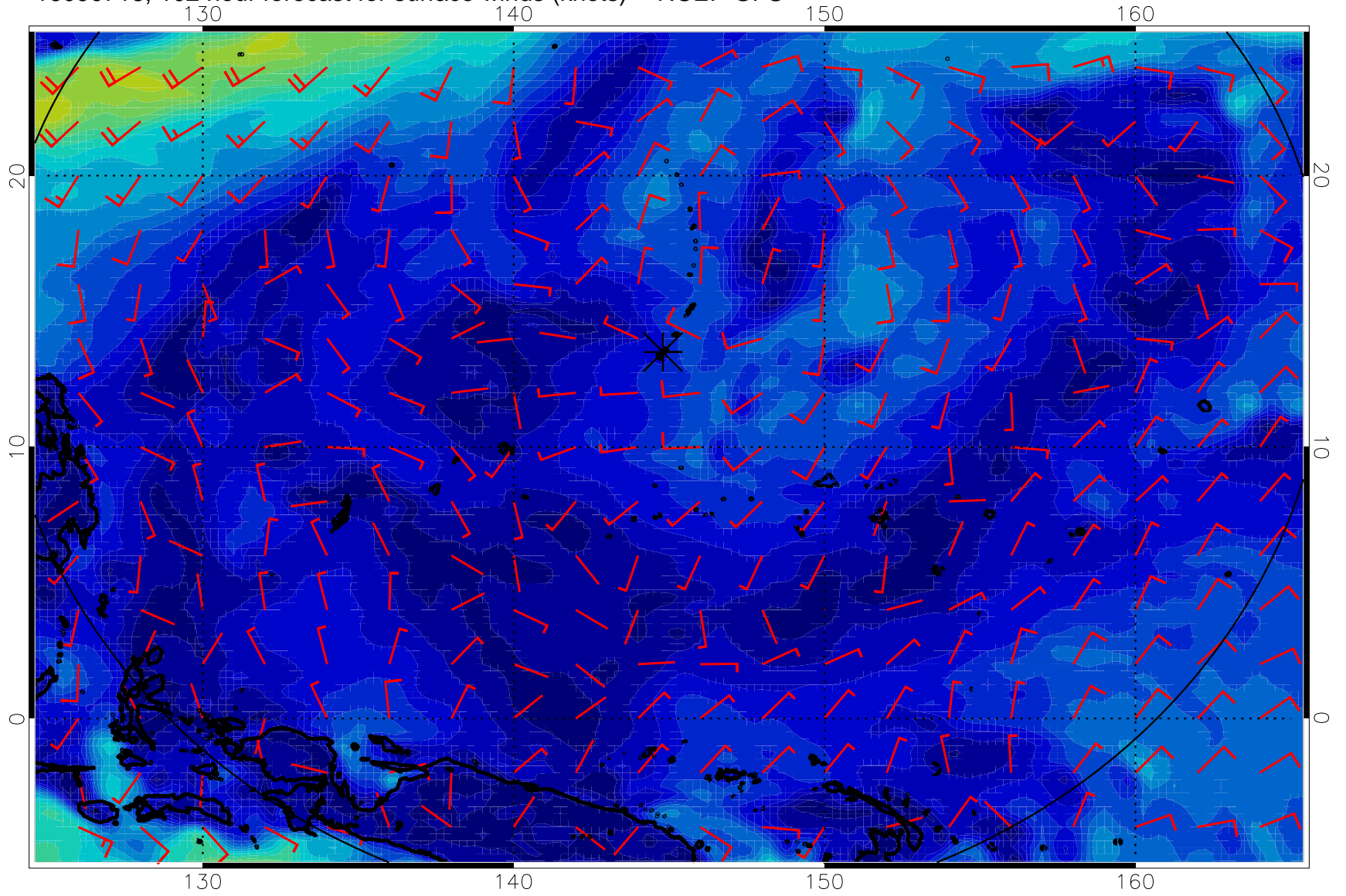
16090718, 102 hour forecast for surface winds (knots) -- NCEP GFS
