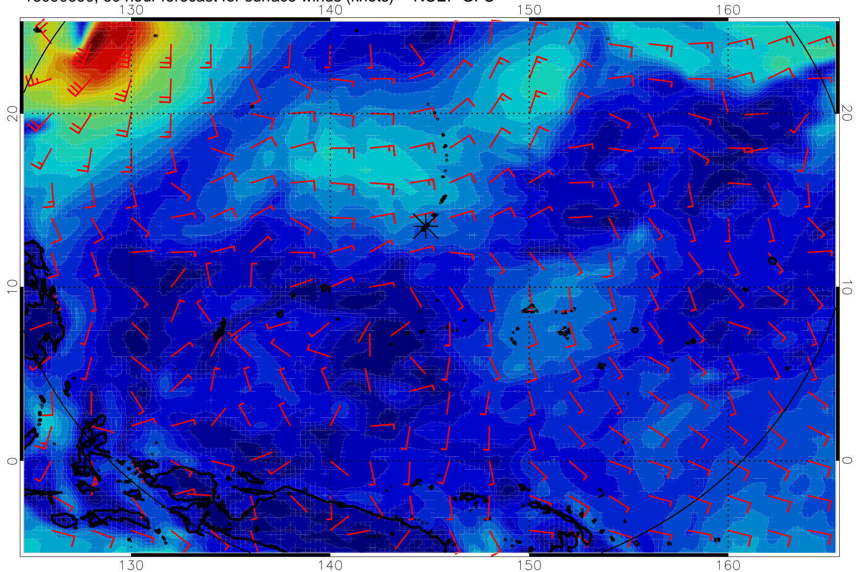
16090600, 60 hour forecast for surface winds (knots) -- NCEP GFS
