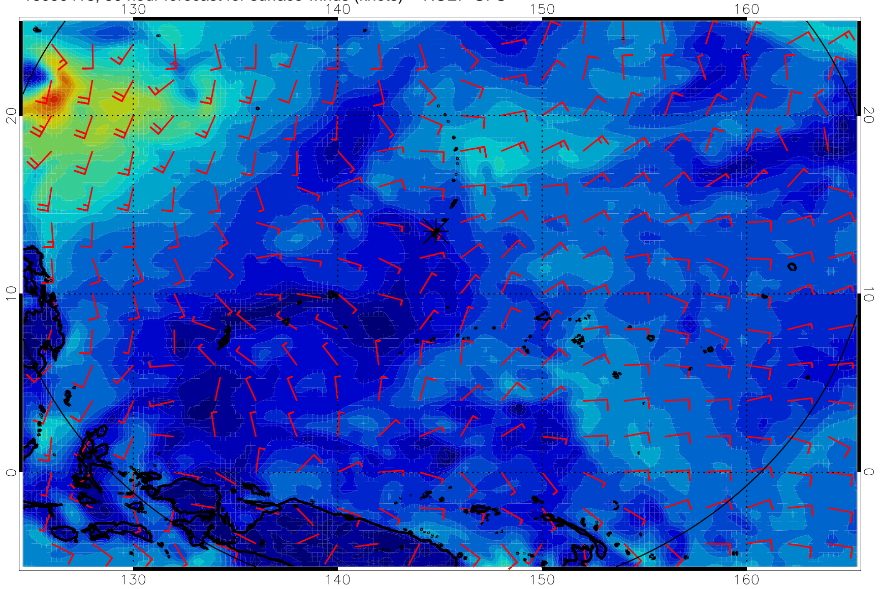
16090418, 30 hour forecast for surface winds (knots) -- NCEP GFS
