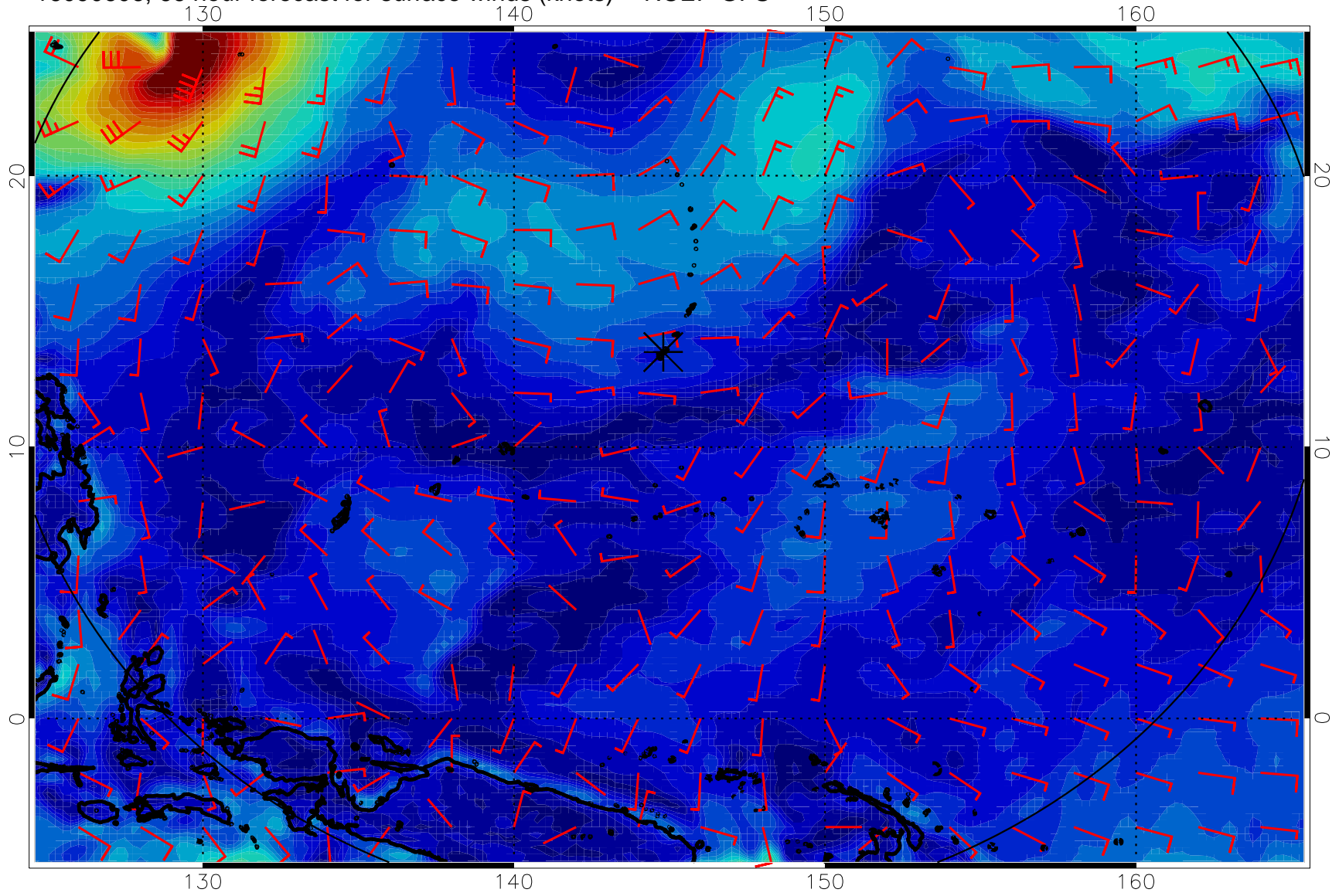
16090606, 66 hour forecast for surface winds (knots) -- NCEP GFS
