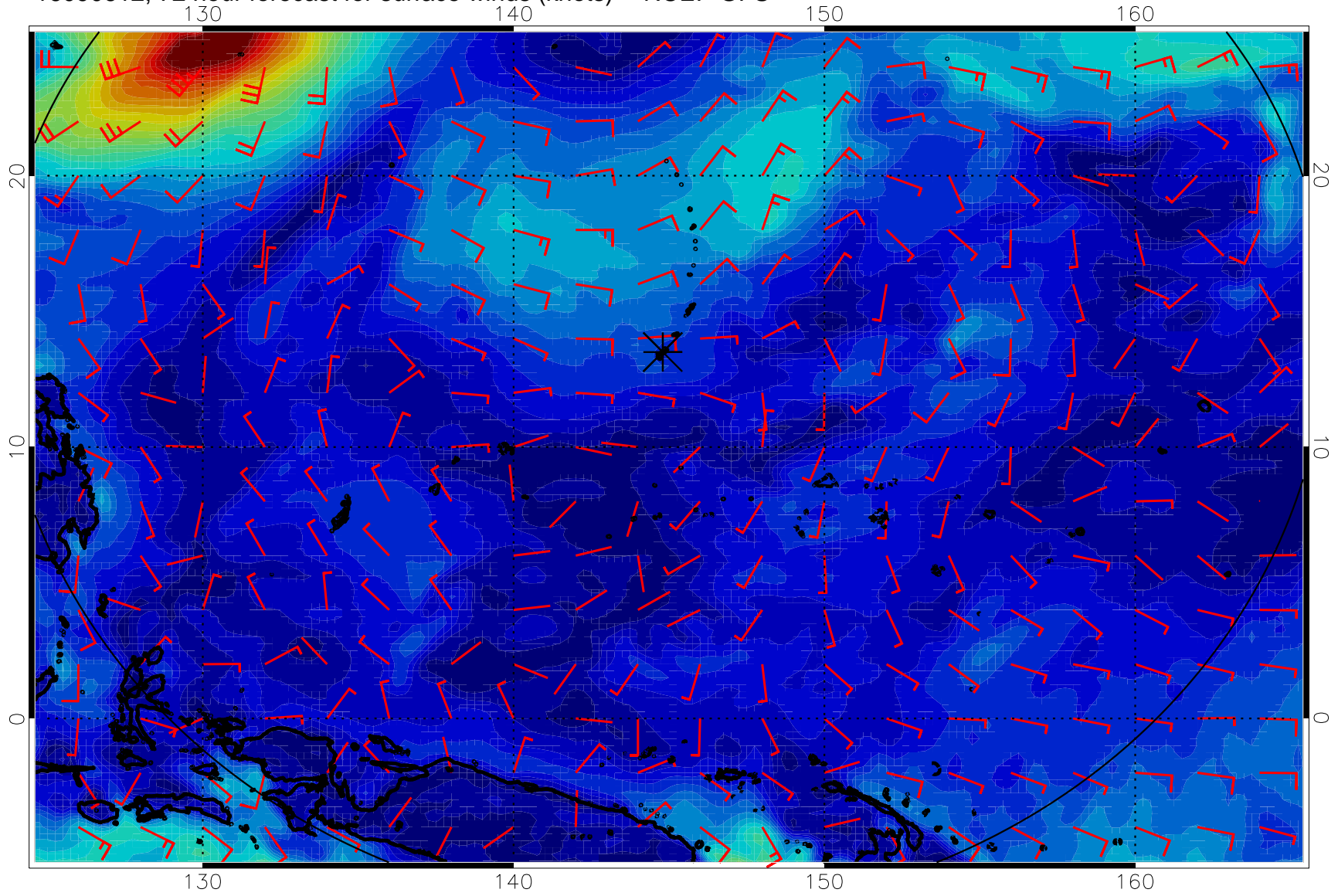
16090612, 72 hour forecast for surface winds (knots) -- NCEP GFS
