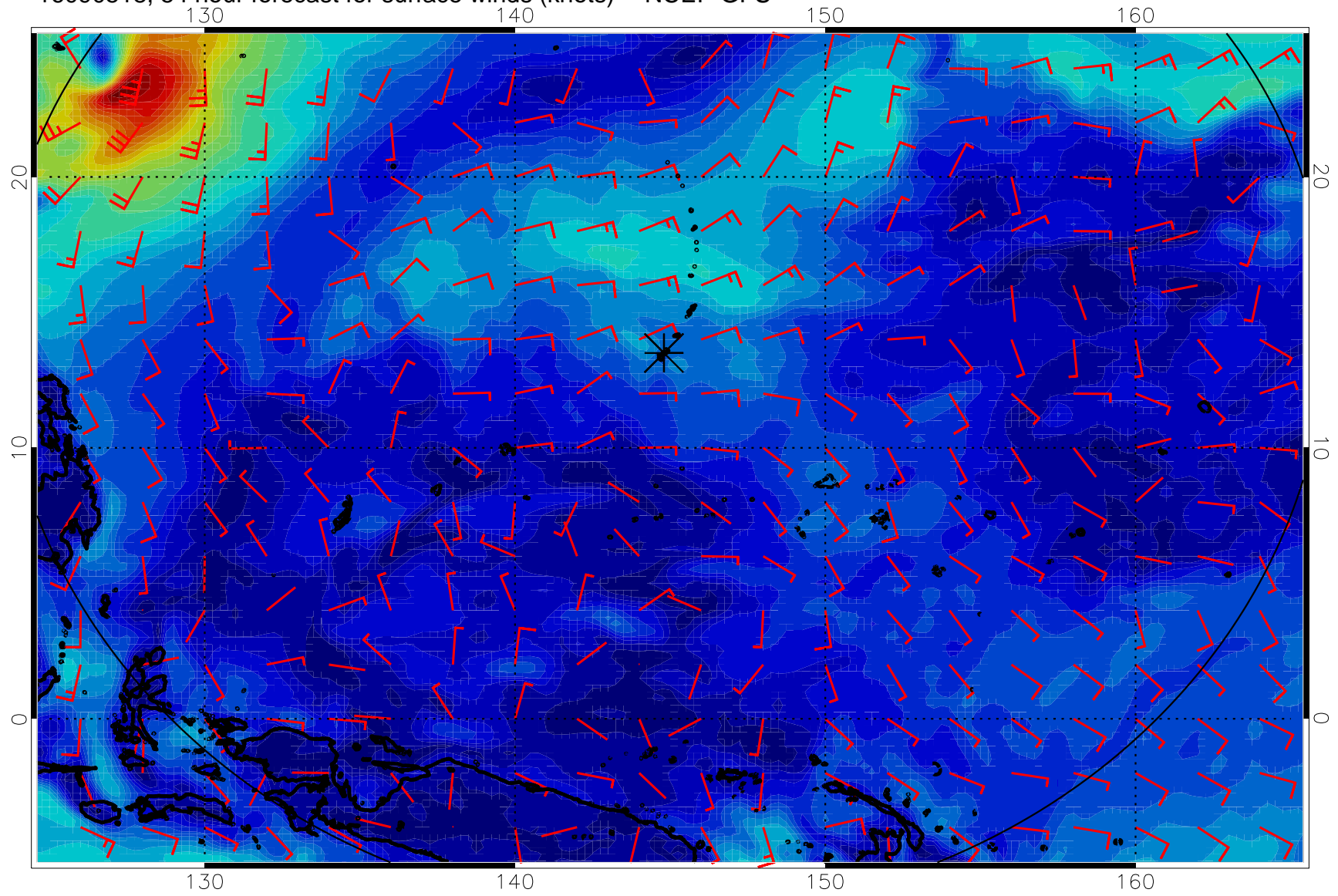
16090518, 54 hour forecast for surface winds (knots) -- NCEP GFS
