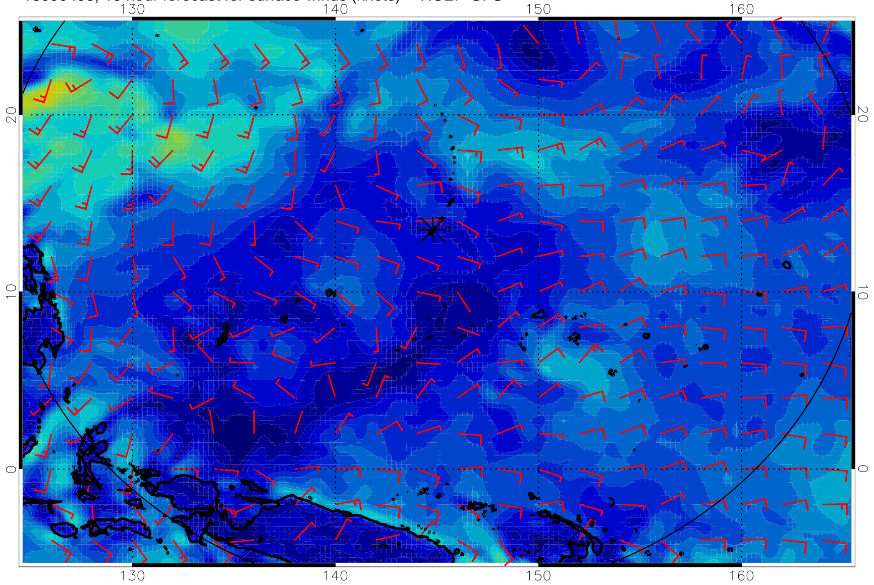
16090406, 18 hour forecast for surface winds (knots) -- NCEP GFS
