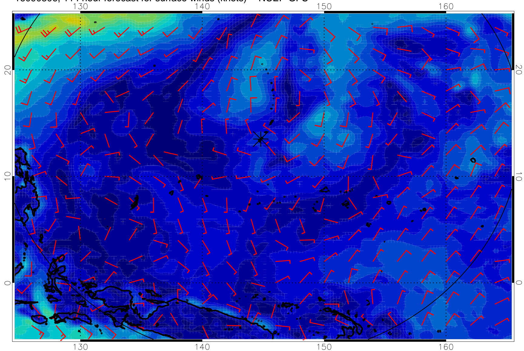
16090806, 114 hour forecast for surface winds (knots) -- NCEP GFS
