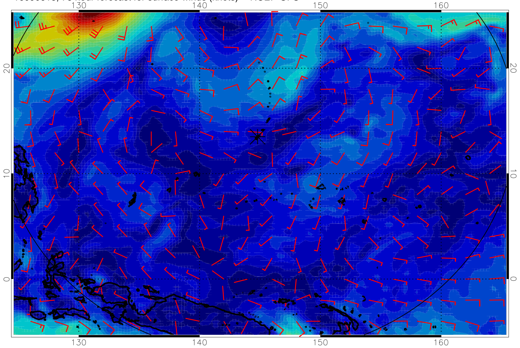
16090618, 78 hour forecast for surface winds (knots) -- NCEP GFS
