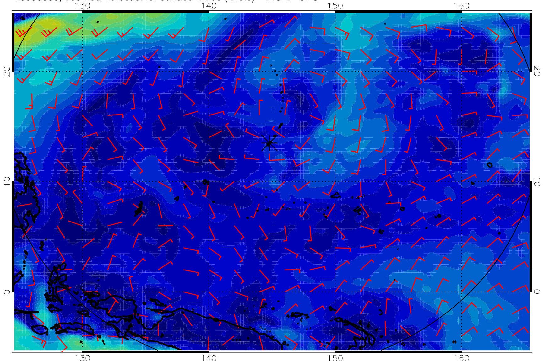
16090800, 108 hour forecast for surface winds (knots) -- NCEP GFS
