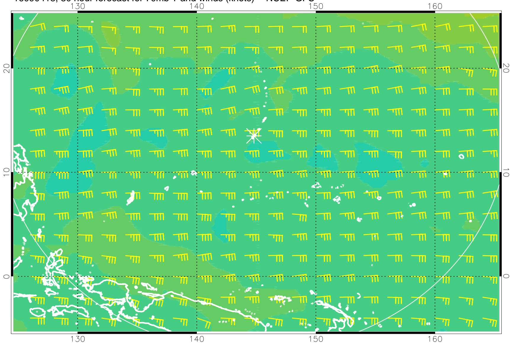
16090418, 30 hour forecast for 70mb T and winds (knots) -- NCEP GFS
