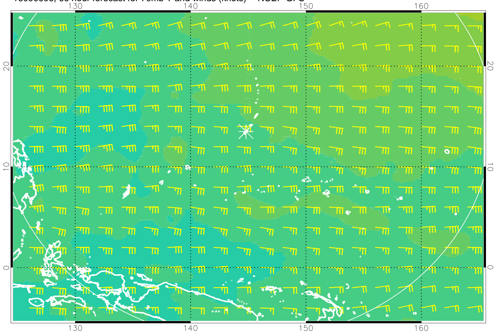
16090606, 66 hour forecast for 70mb T and winds (knots) -- NCEP GFS
