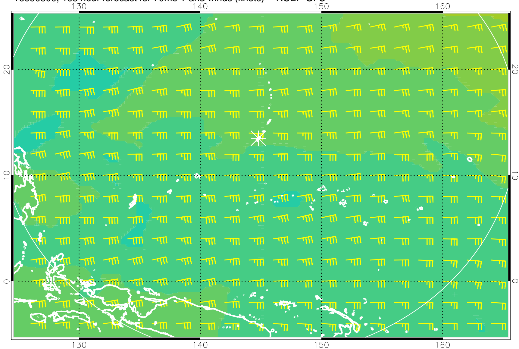
16090800, 108 hour forecast for 70mb T and winds (knots) -- NCEP GFS
