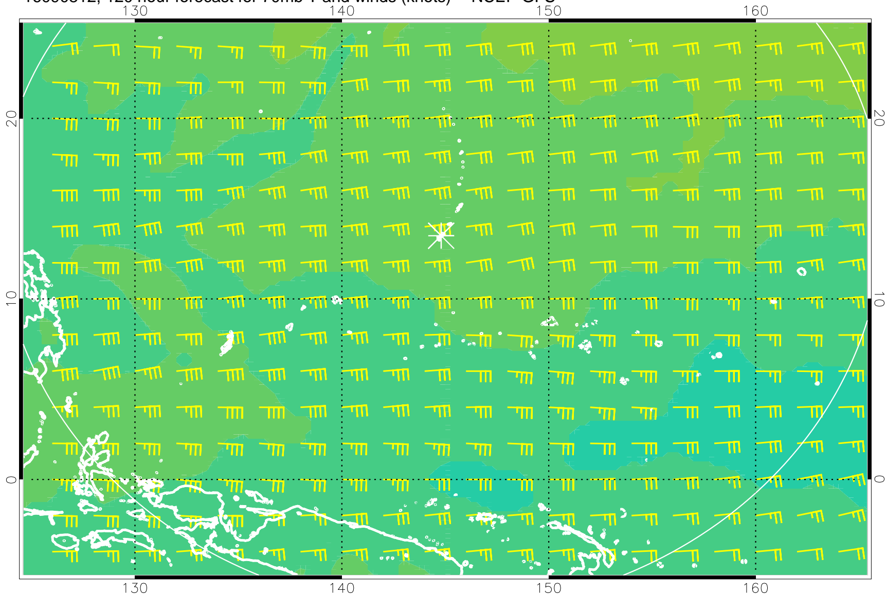
16090812, 120 hour forecast for 70mb T and winds (knots) -- NCEP GFS
