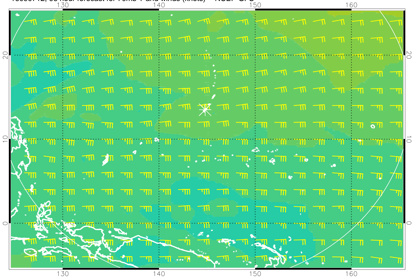
16090712, 96 hour forecast for 70mb T and winds (knots) -- NCEP GFS
