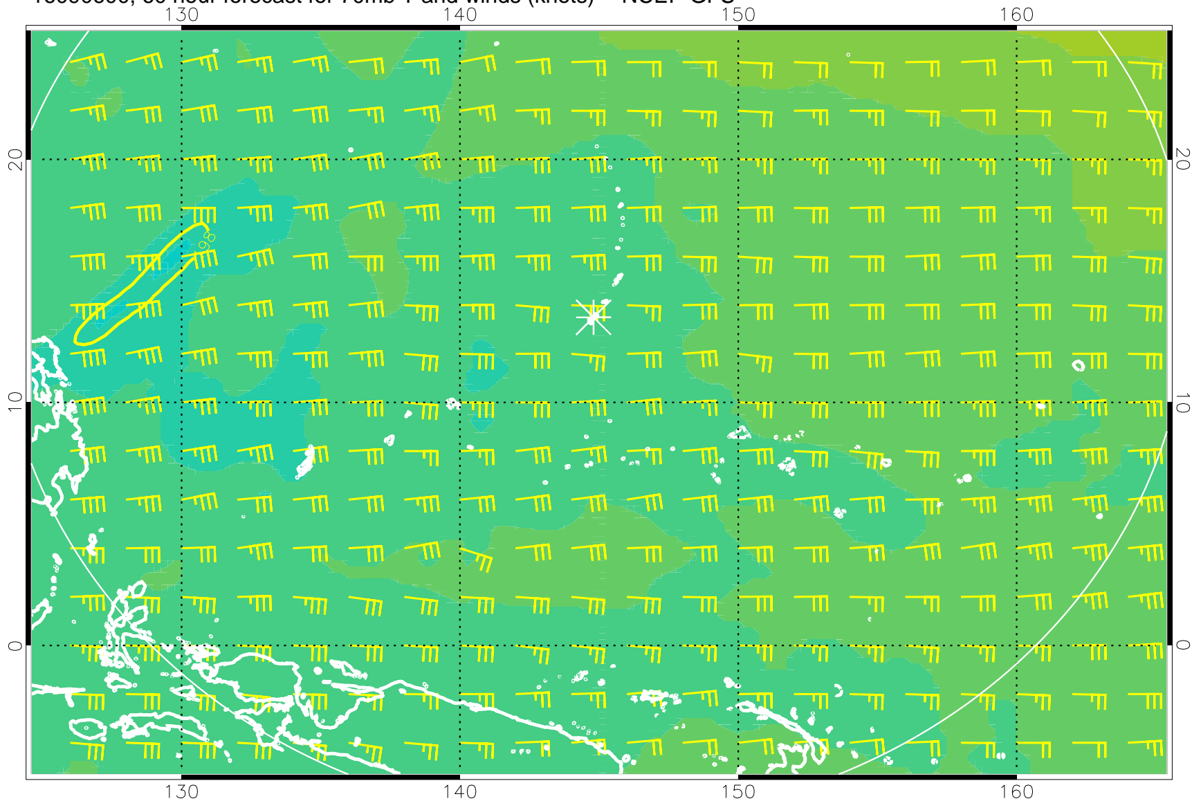
16090600, 60 hour forecast for 70mb T and winds (knots) -- NCEP GFS
