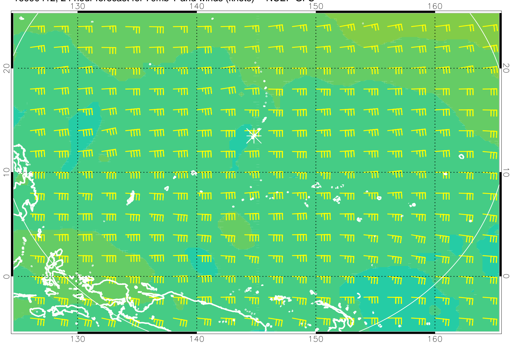
16090412, 24 hour forecast for 70mb T and winds (knots) -- NCEP GFS
