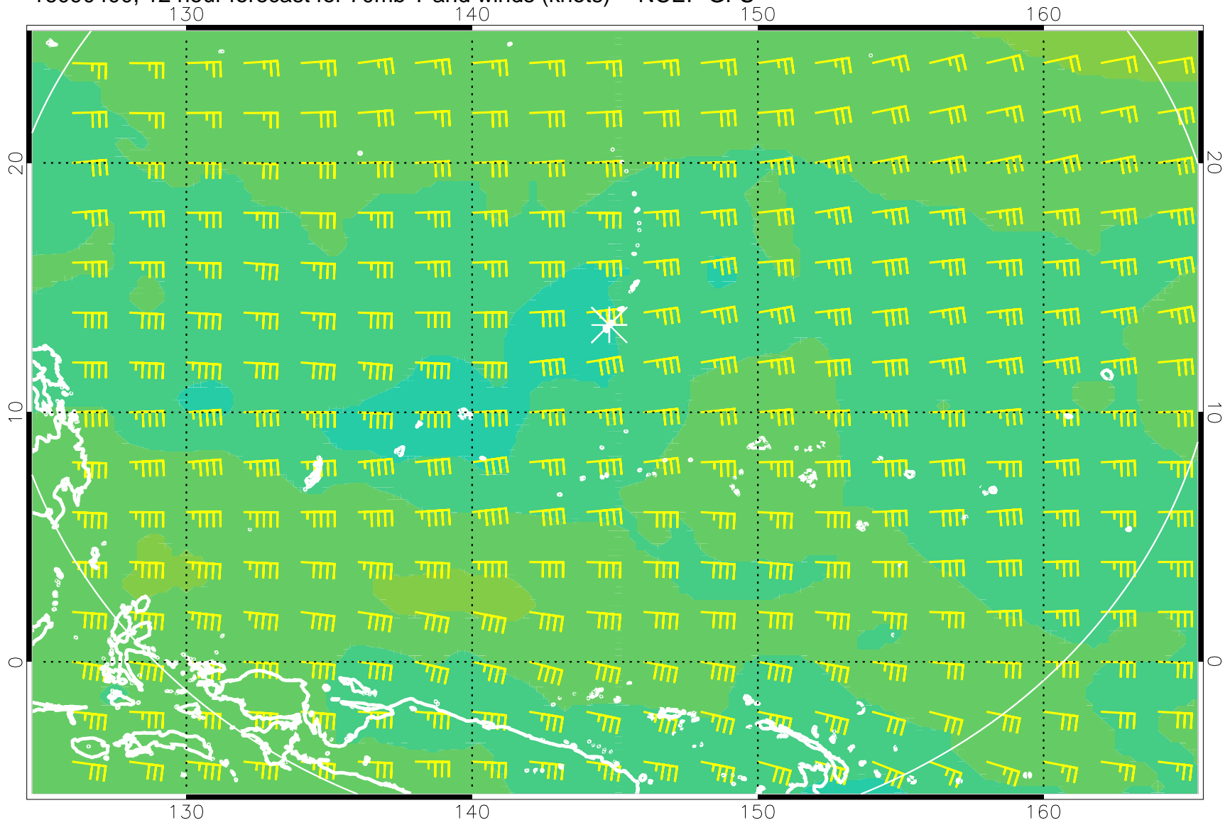
16090400, 12 hour forecast for 70mb T and winds (knots) -- NCEP GFS
