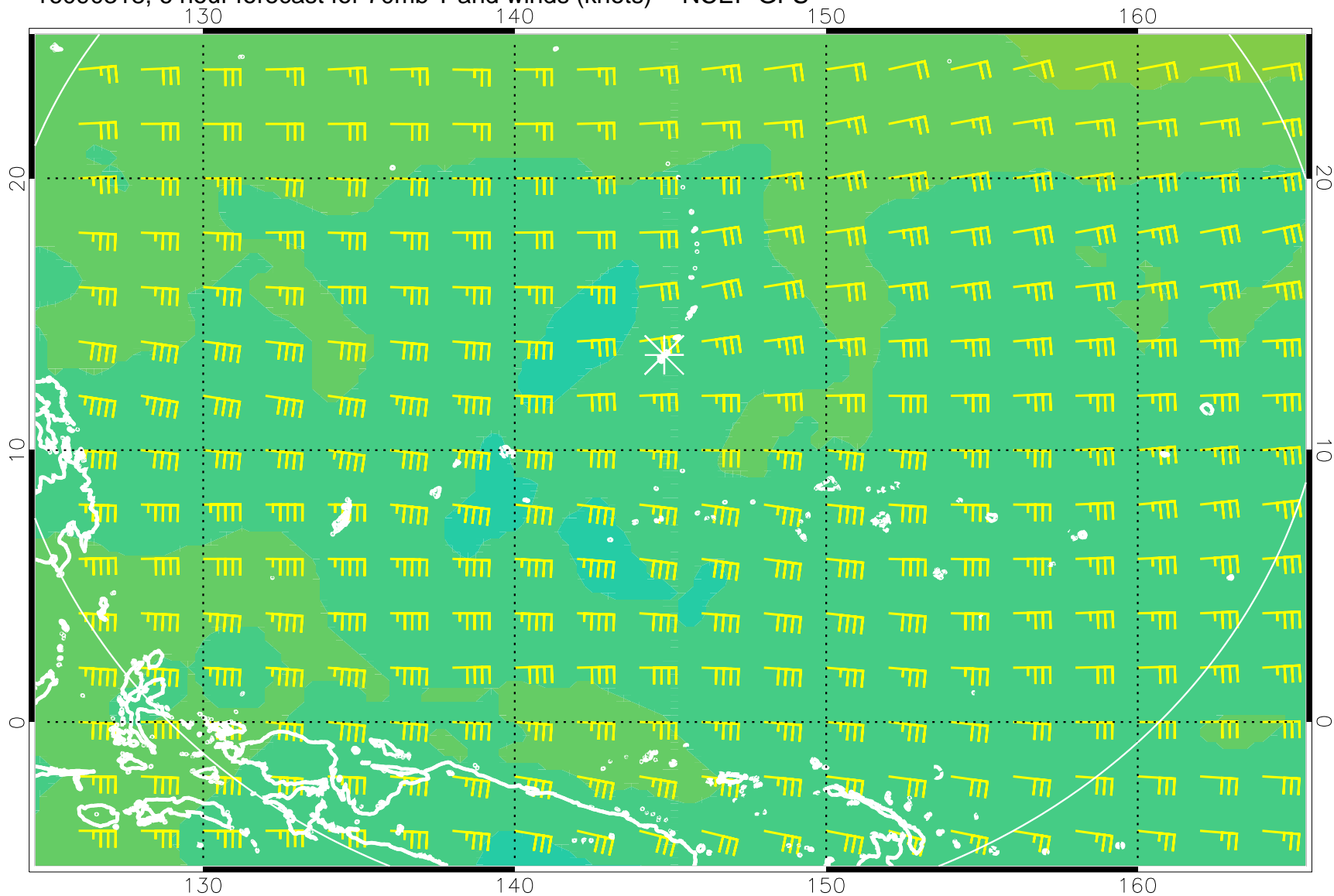
16090318, 6 hour forecast for 70mb T and winds (knots) -- NCEP GFS
