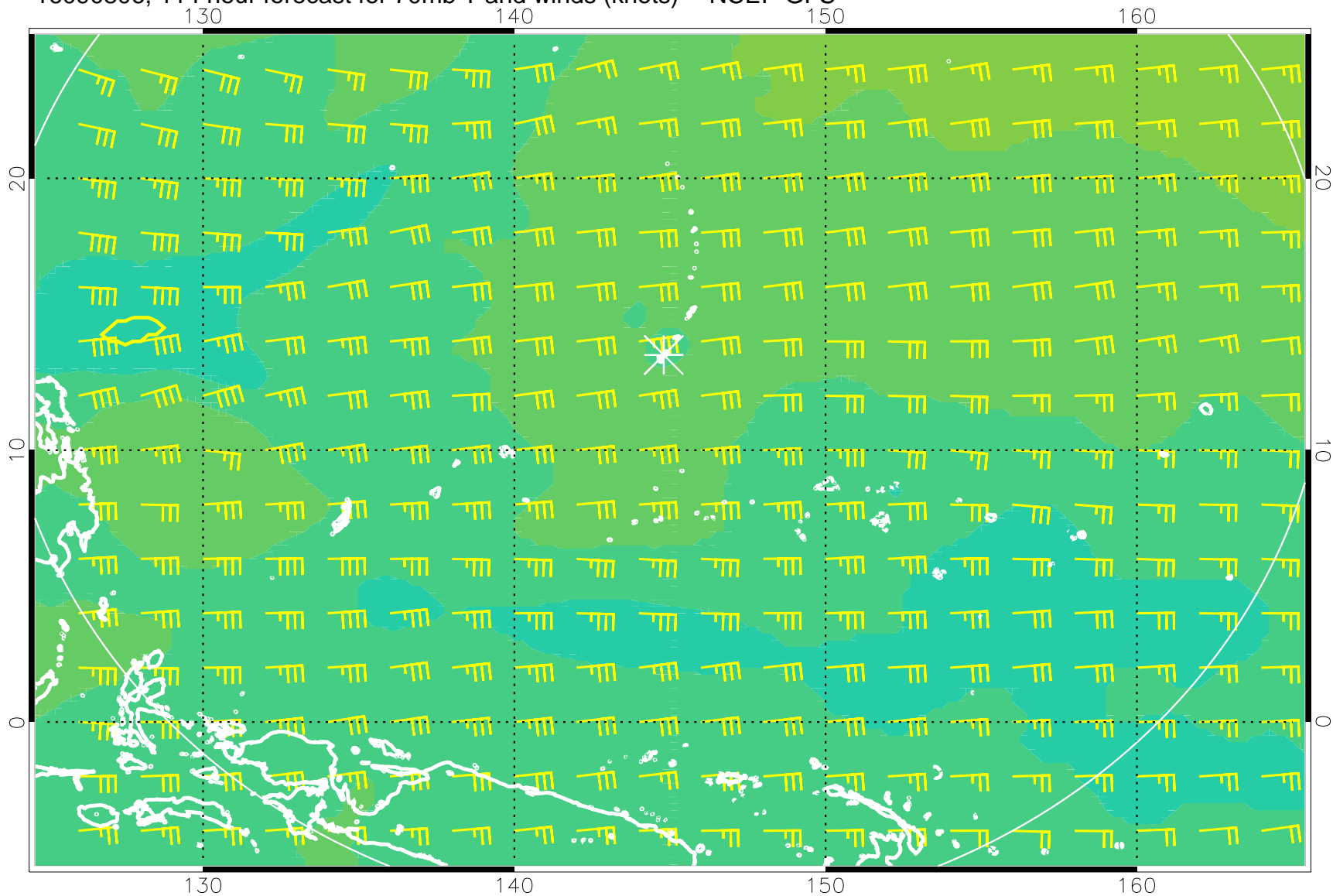
16090806, 114 hour forecast for 70mb T and winds (knots) -- NCEP GFS
