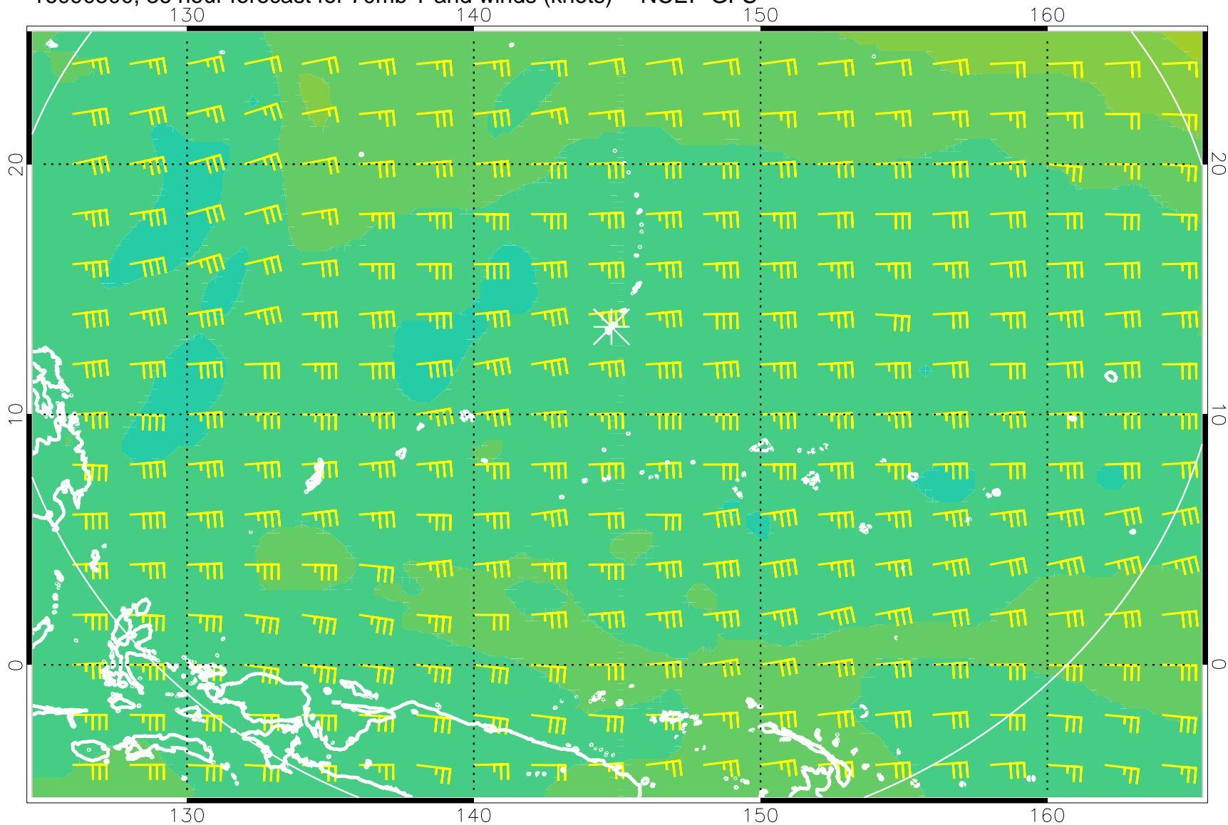
16090500, 36 hour forecast for 70mb T and winds (knots) -- NCEP GFS
