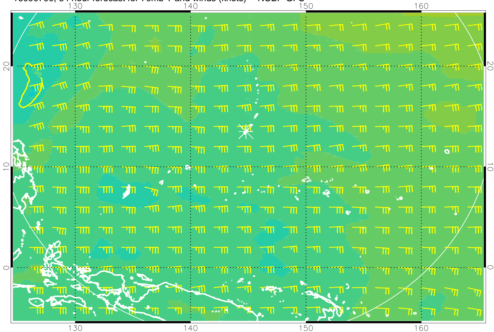
16090700, 84 hour forecast for 70mb T and winds (knots) -- NCEP GFS
