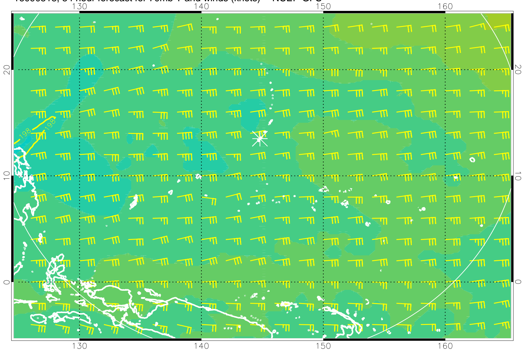
16090518, 54 hour forecast for 70mb T and winds (knots) -- NCEP GFS
