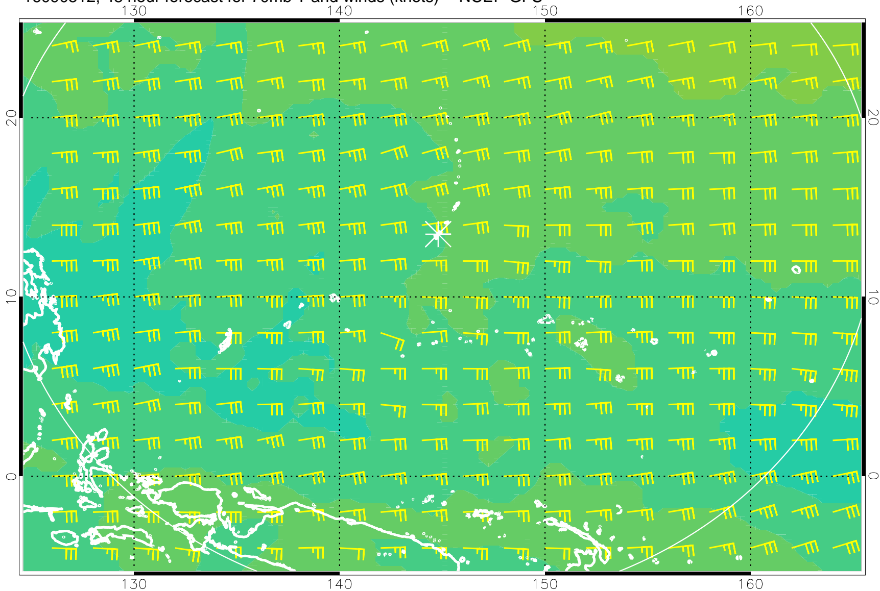
16090512, 48 hour forecast for 70mb T and winds (knots) -- NCEP GFS
