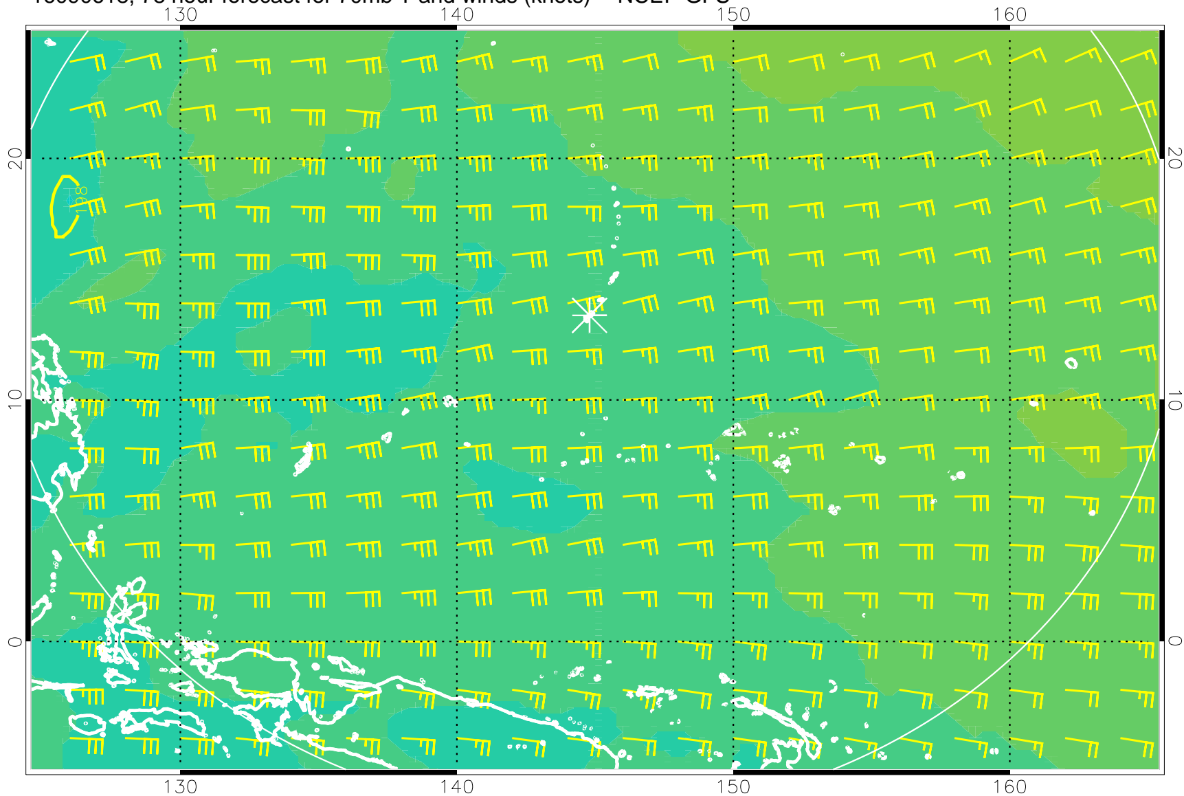
16090618, 78 hour forecast for 70mb T and winds (knots) -- NCEP GFS
