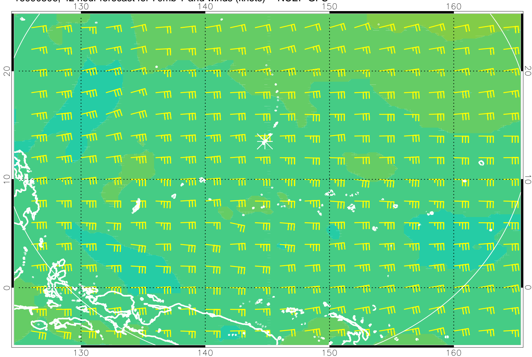
16090506, 42 hour forecast for 70mb T and winds (knots) -- NCEP GFS
