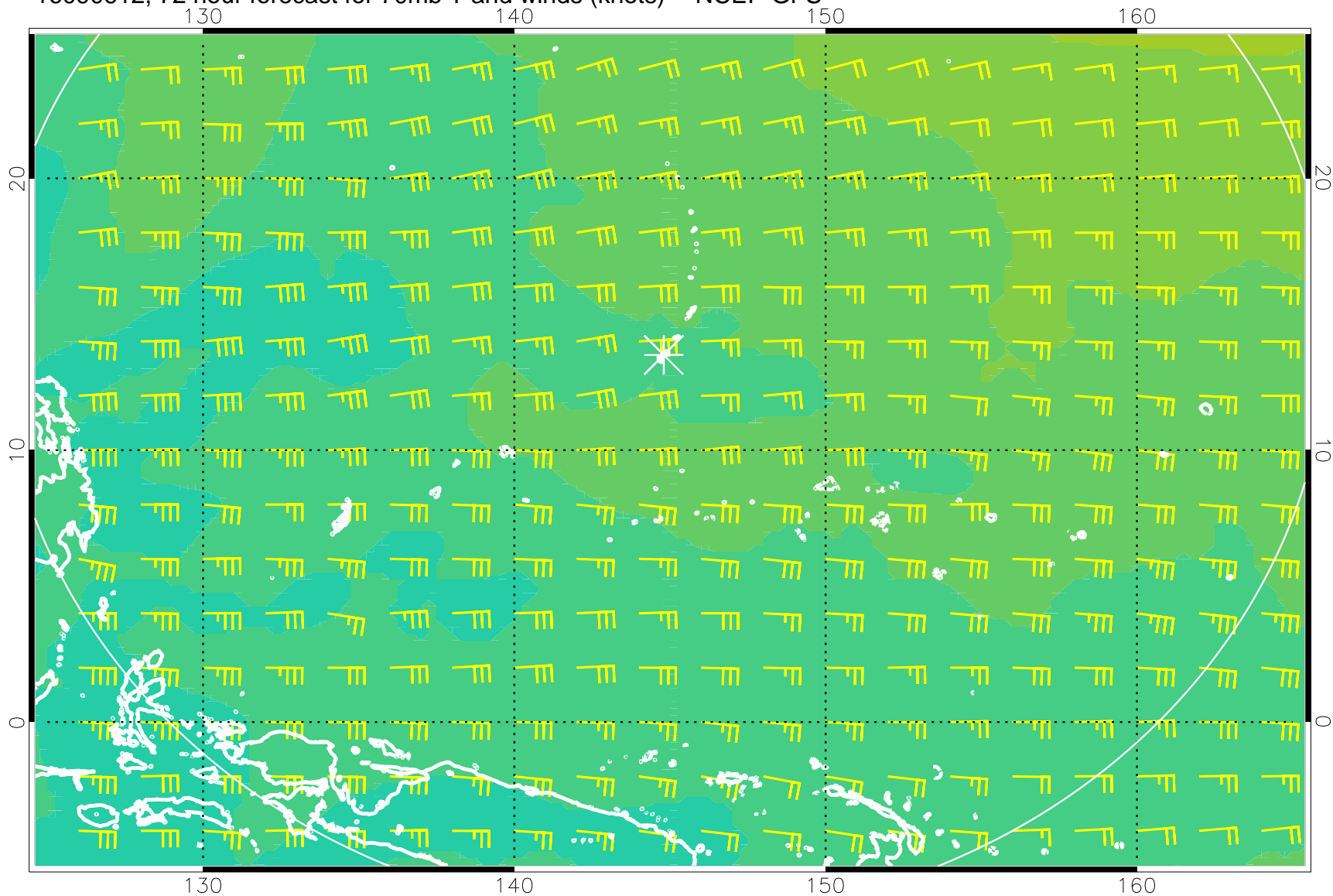
16090612, 72 hour forecast for 70mb T and winds (knots) -- NCEP GFS
