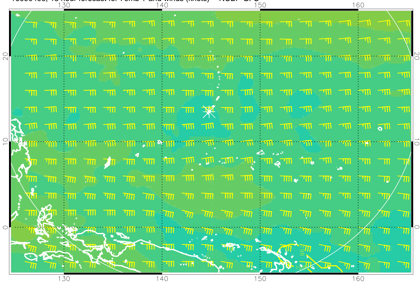
16090406, 18 hour forecast for 70mb T and winds (knots) -- NCEP GFS
