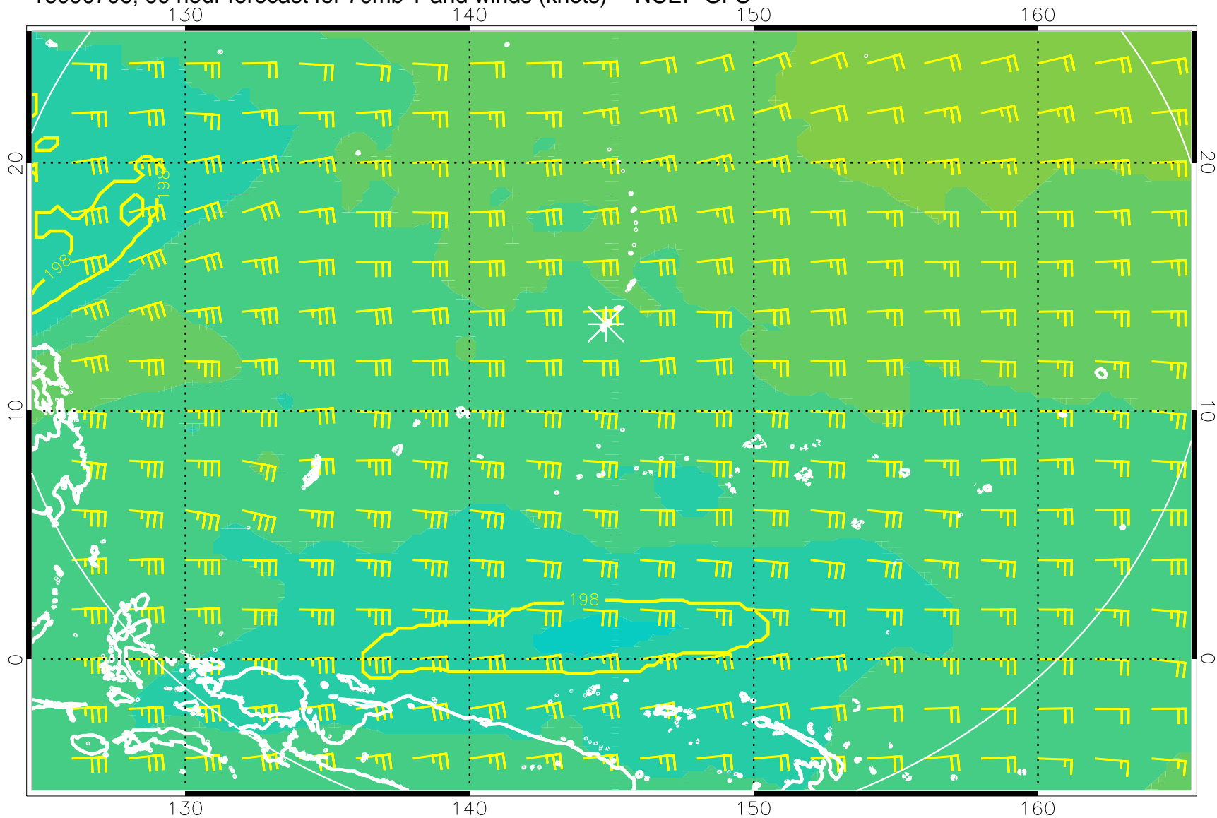
16090706, 90 hour forecast for 70mb T and winds (knots) -- NCEP GFS
