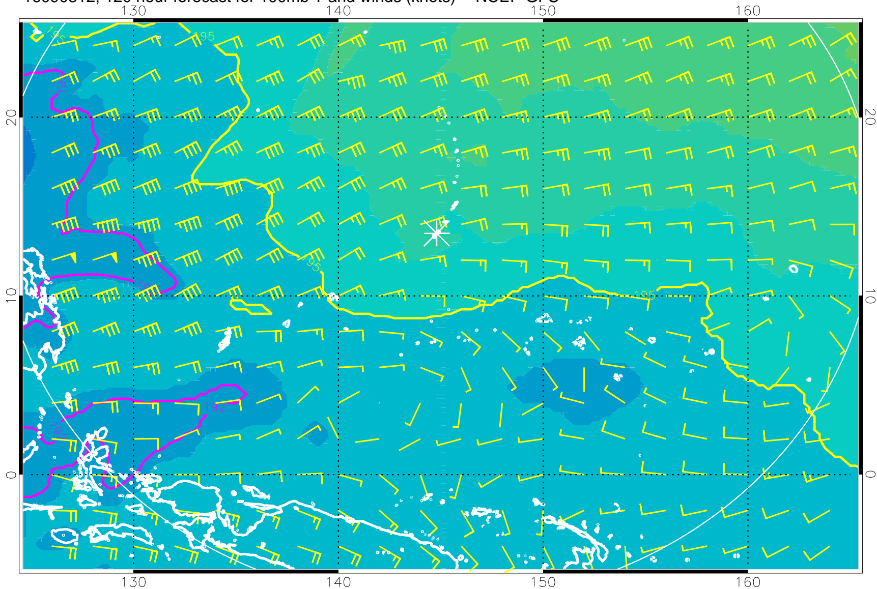
16090812, 120 hour forecast for 100mb T and winds (knots) -- NCEP GFS
