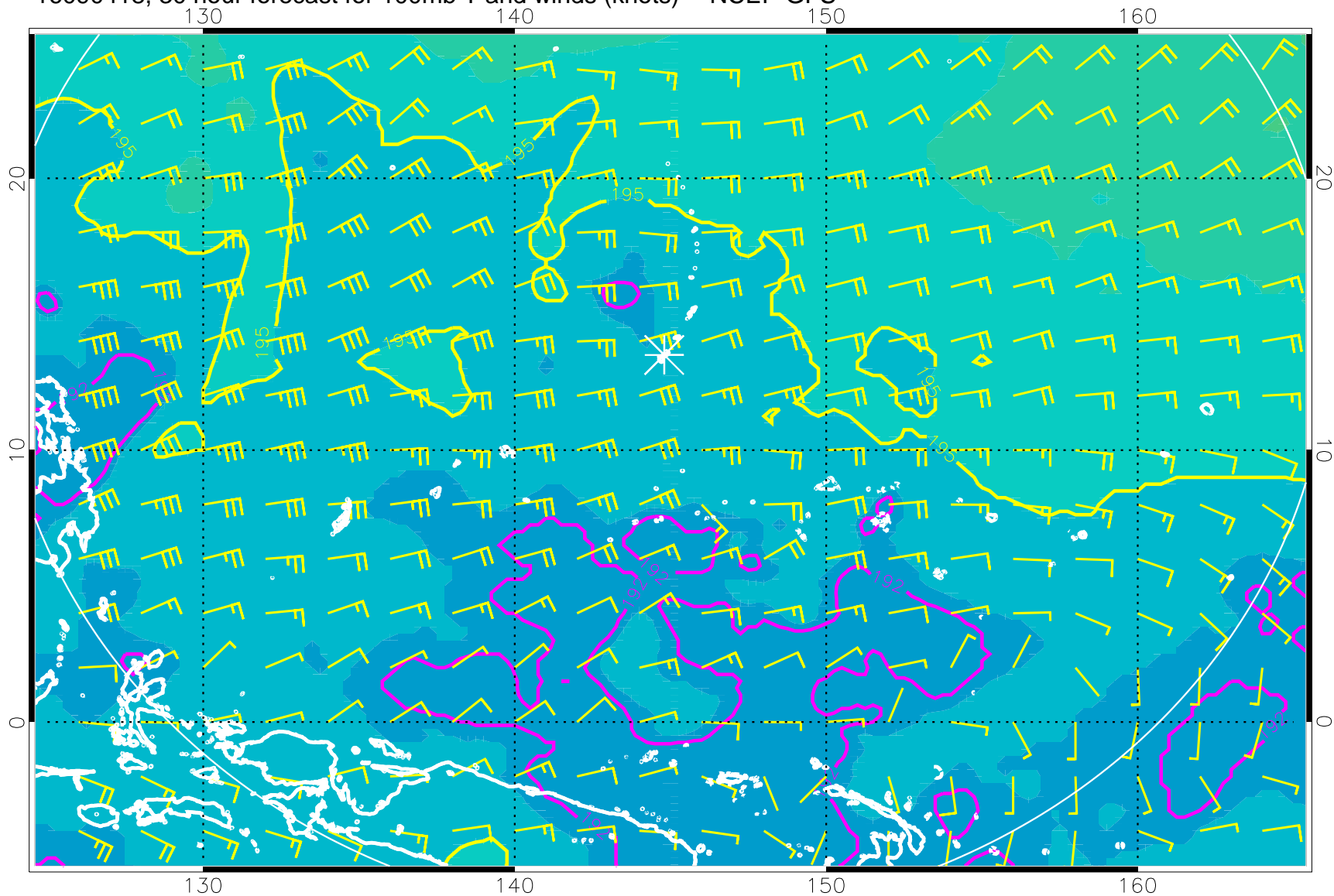
16090418, 30 hour forecast for 100mb T and winds (knots) -- NCEP GFS
