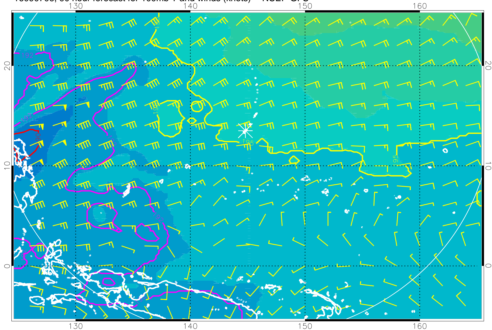
16090706, 90 hour forecast for 100mb T and winds (knots) -- NCEP GFS
