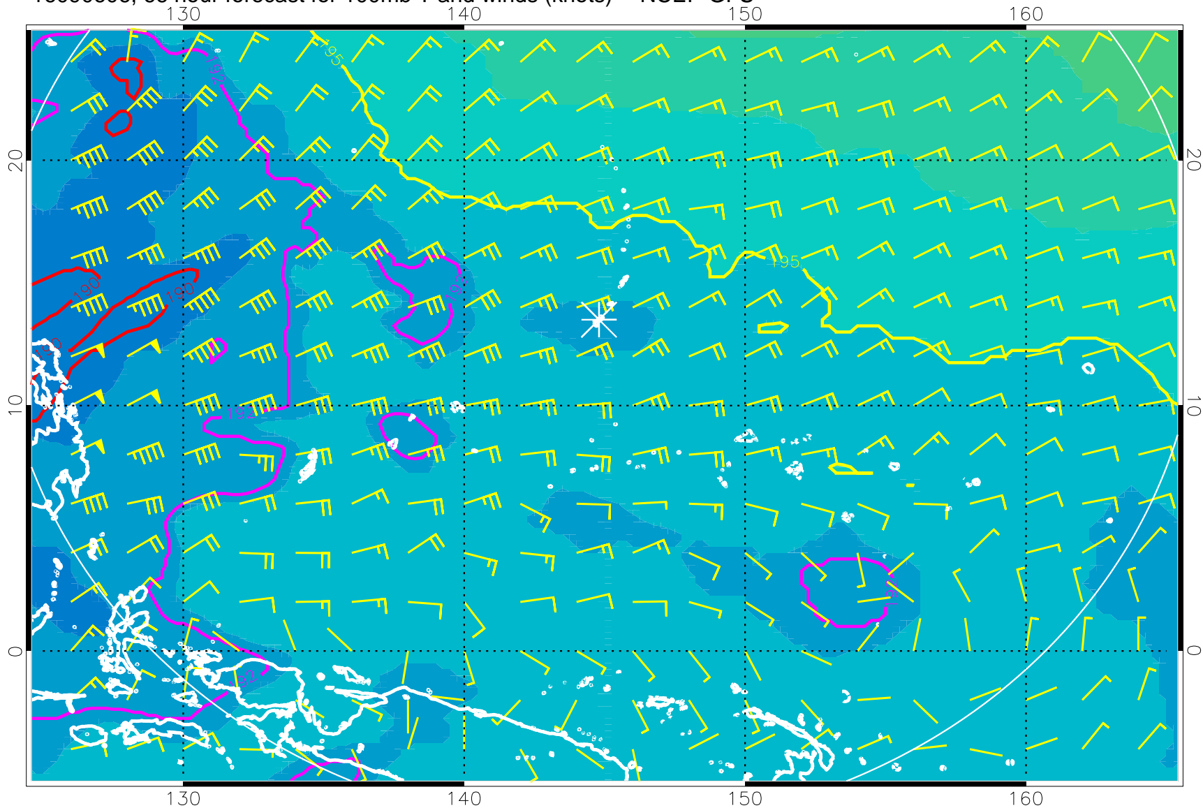
16090606, 66 hour forecast for 100mb T and winds (knots) -- NCEP GFS
