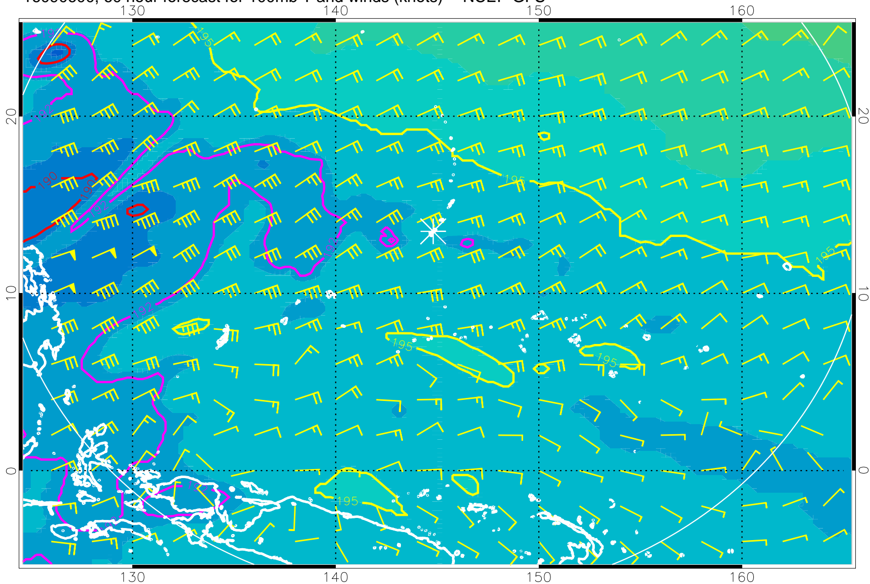
16090600, 60 hour forecast for 100mb T and winds (knots) -- NCEP GFS
