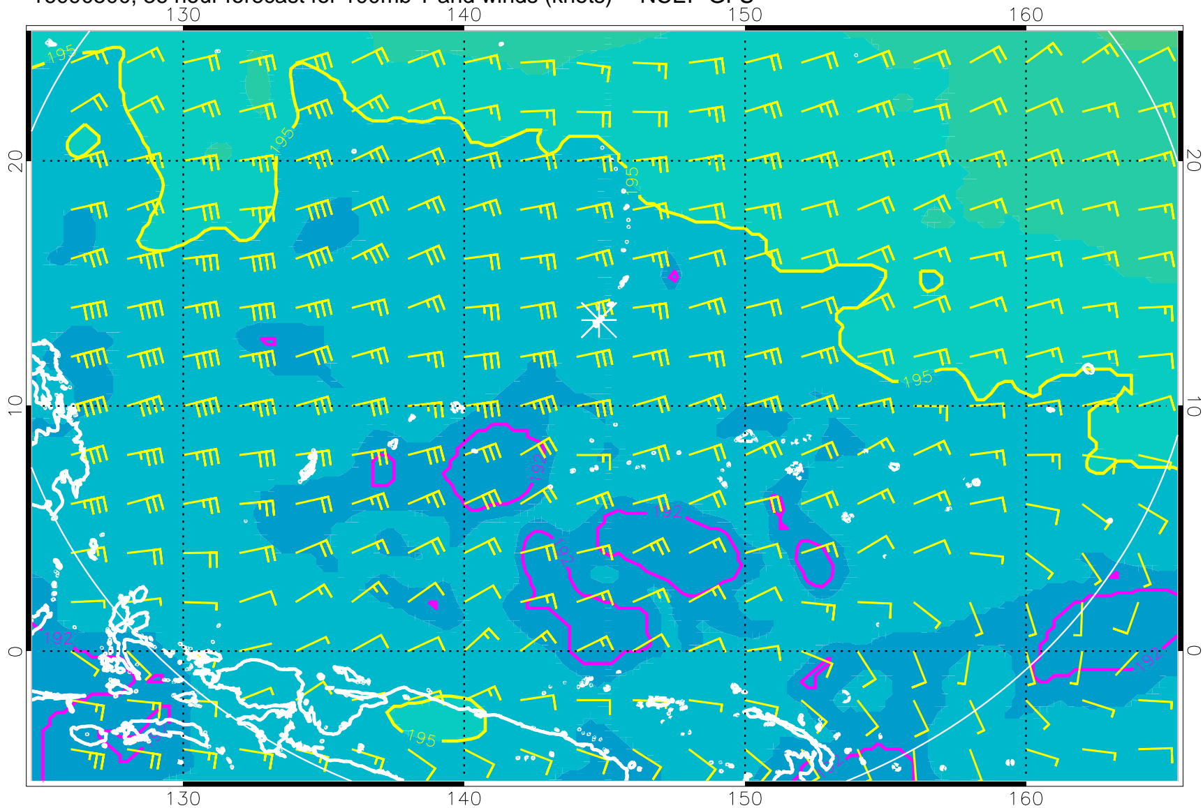
16090500, 36 hour forecast for 100mb T and winds (knots) -- NCEP GFS
