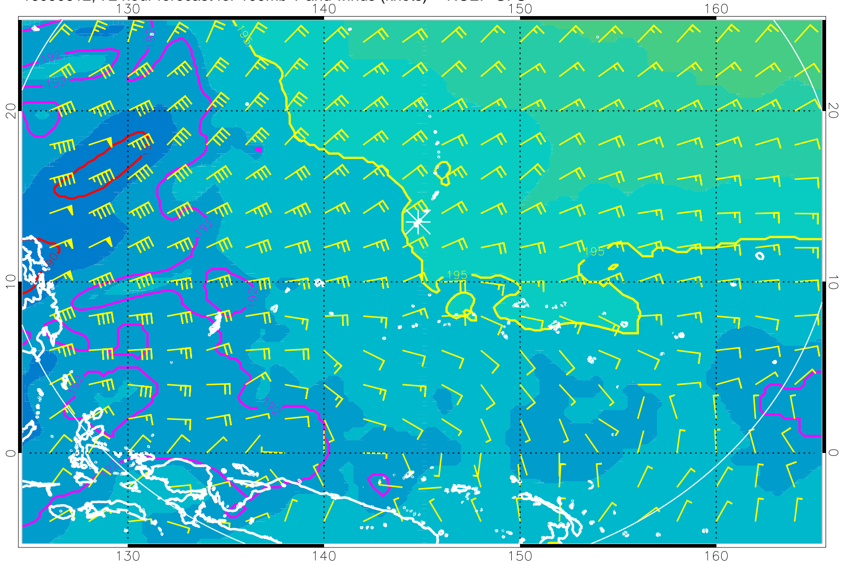
16090612, 72 hour forecast for 100mb T and winds (knots) -- NCEP GFS
