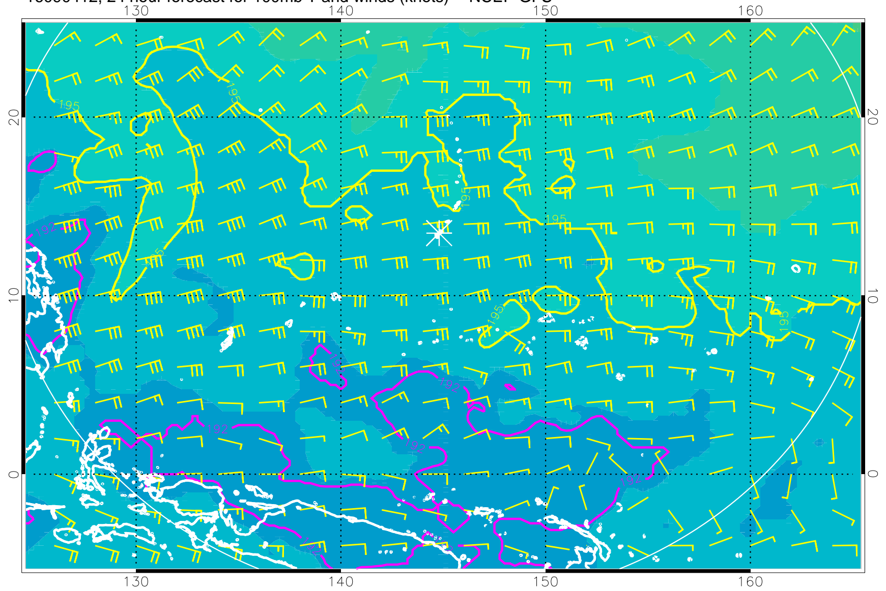
16090412, 24 hour forecast for 100mb T and winds (knots) -- NCEP GFS
