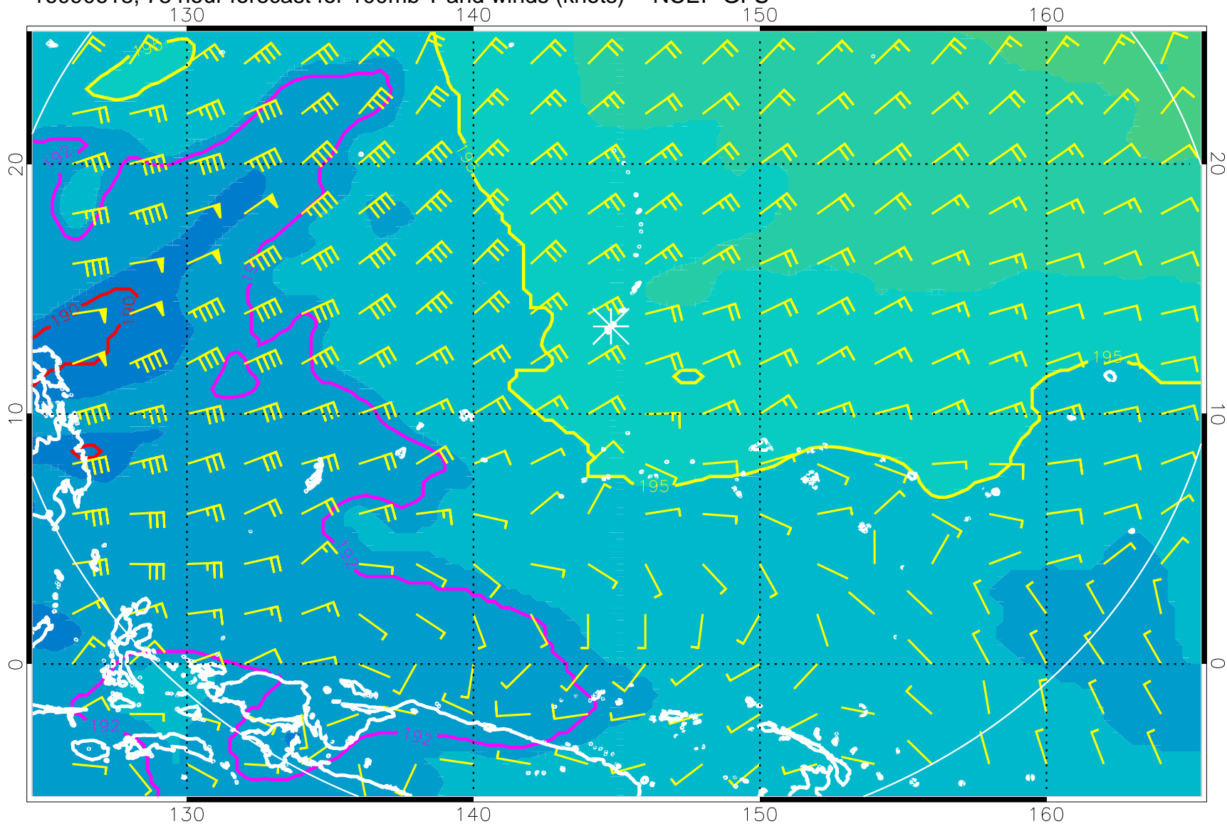
16090618, 78 hour forecast for 100mb T and winds (knots) -- NCEP GFS
