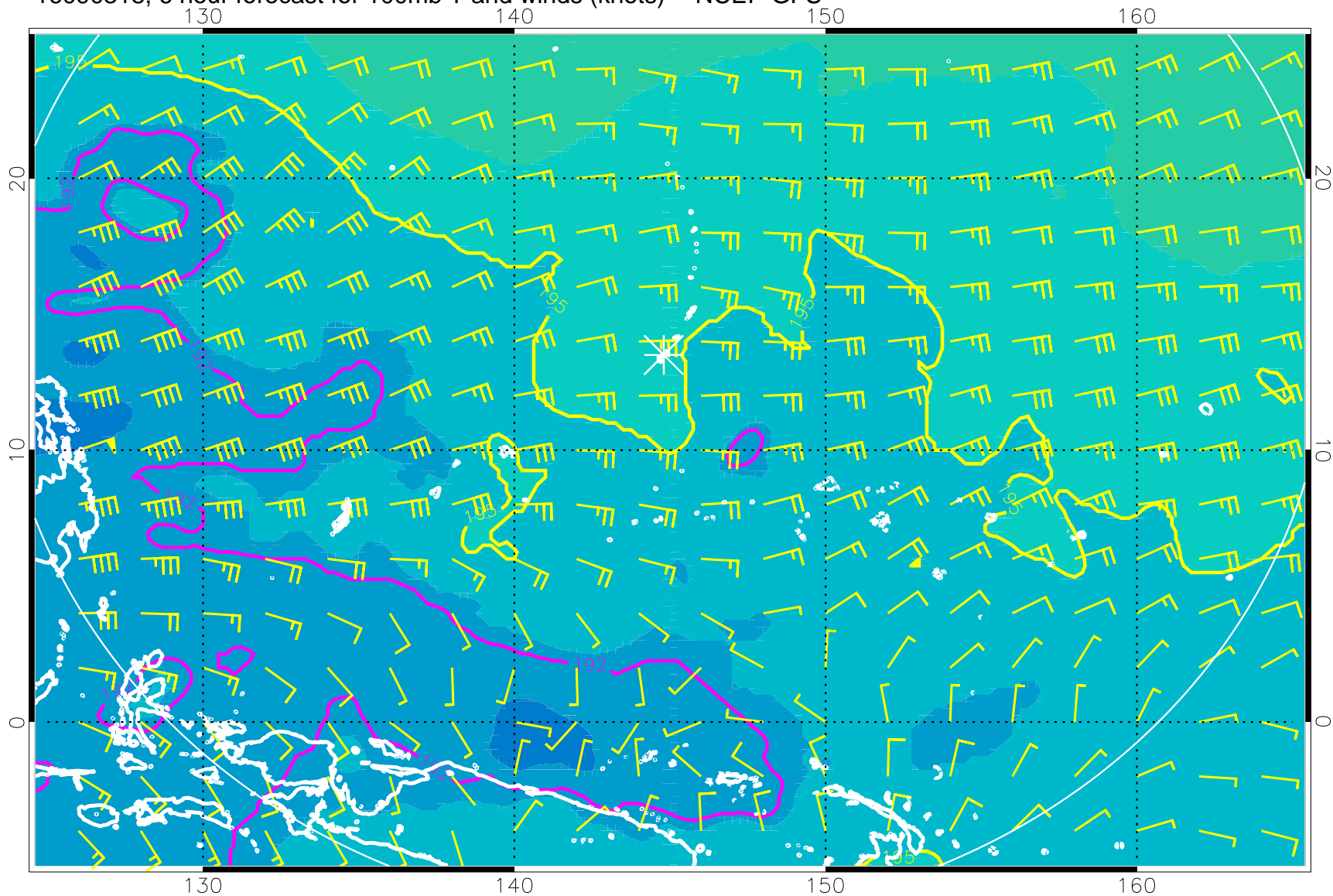
16090318, 6 hour forecast for 100mb T and winds (knots) -- NCEP GFS
