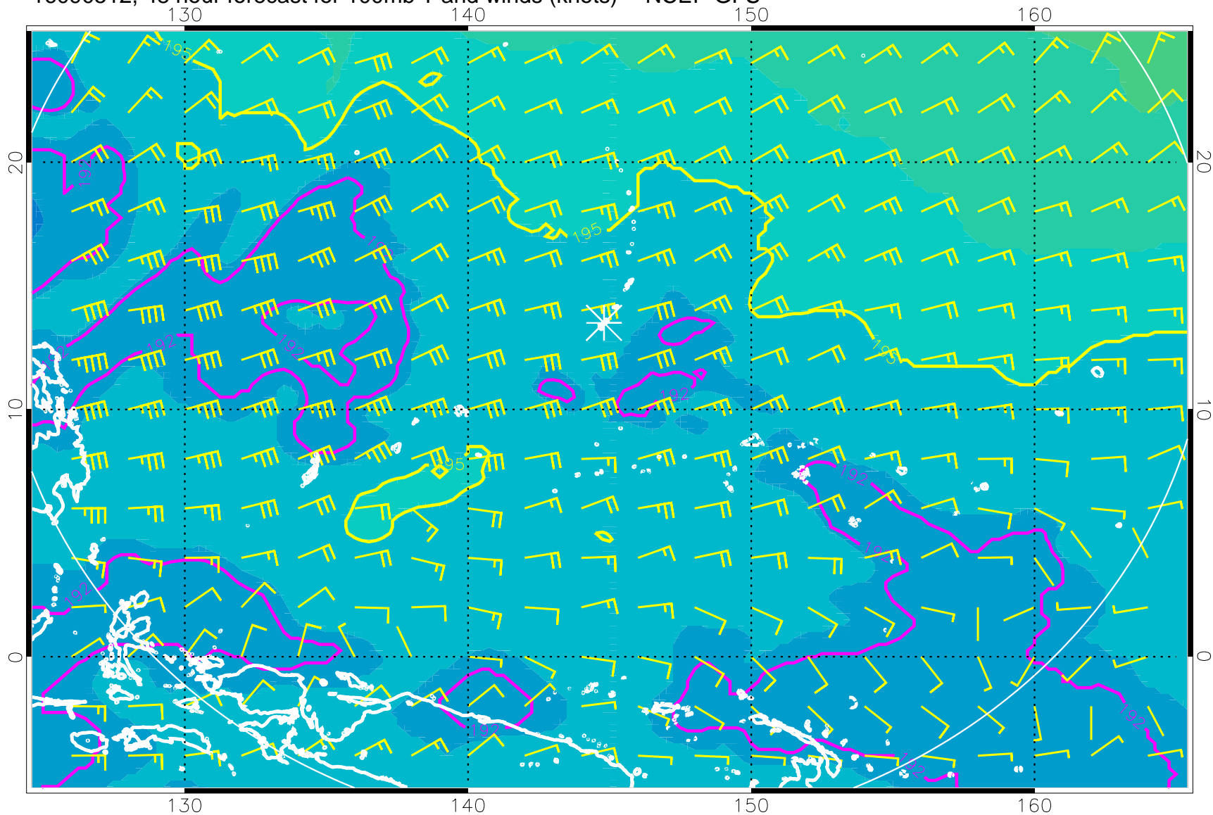
16090512, 48 hour forecast for 100mb T and winds (knots) -- NCEP GFS
