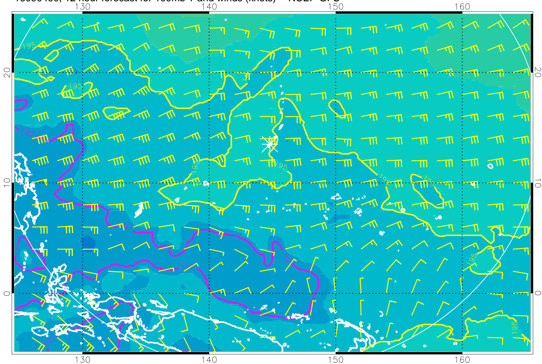
16090400, 12 hour forecast for 100mb T and winds (knots) -- NCEP GFS
