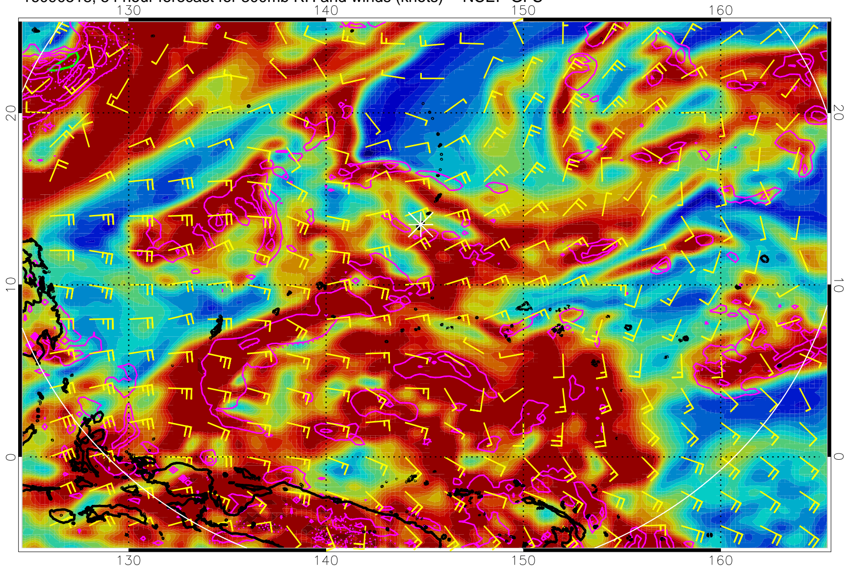
16090518, 54 hour forecast for 300mb RH and winds (knots) -- NCEP GFS
