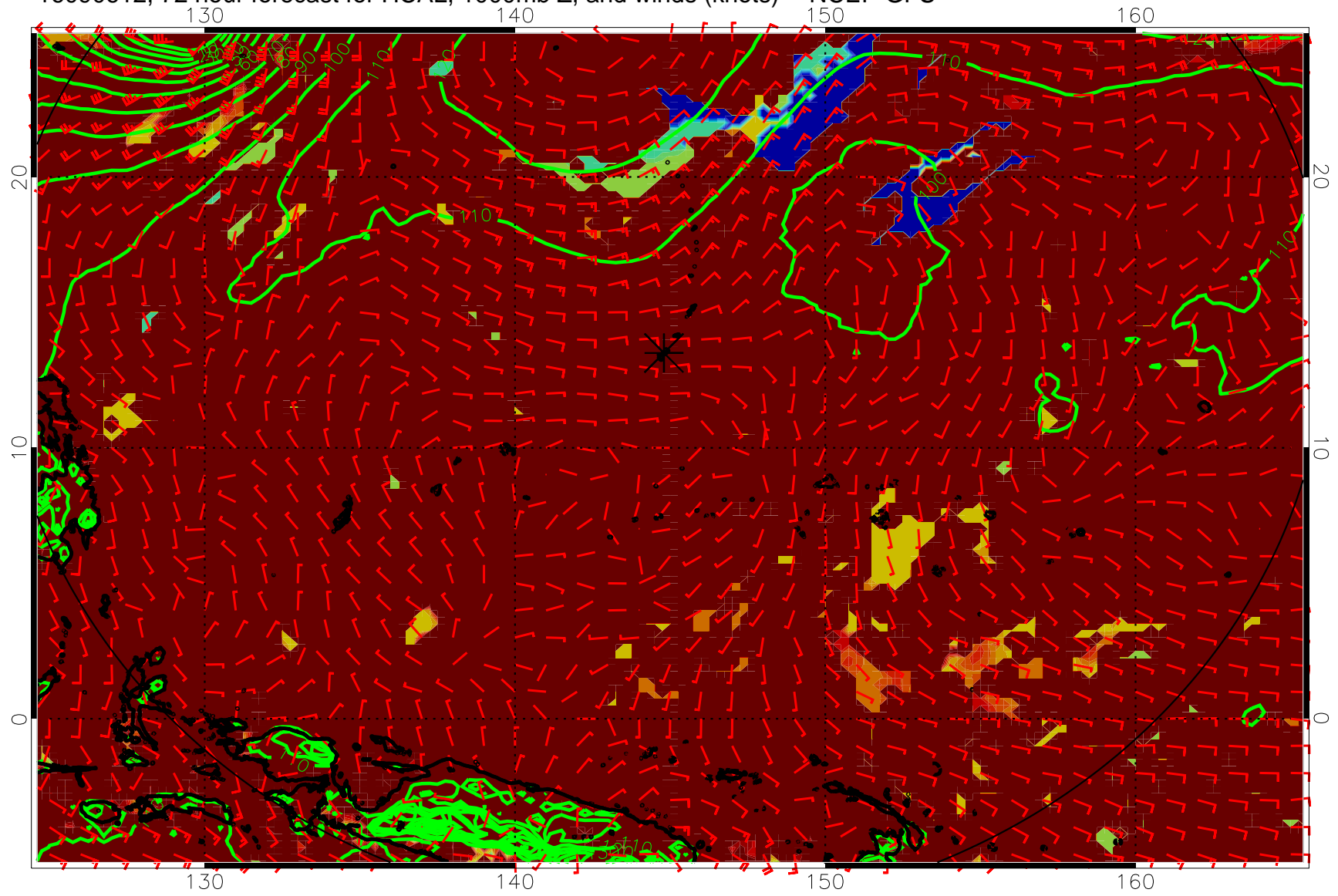
16090612, 72 hour forecast for HCAL, 1000mb Z, and winds (knots) -- NCEP GFS
