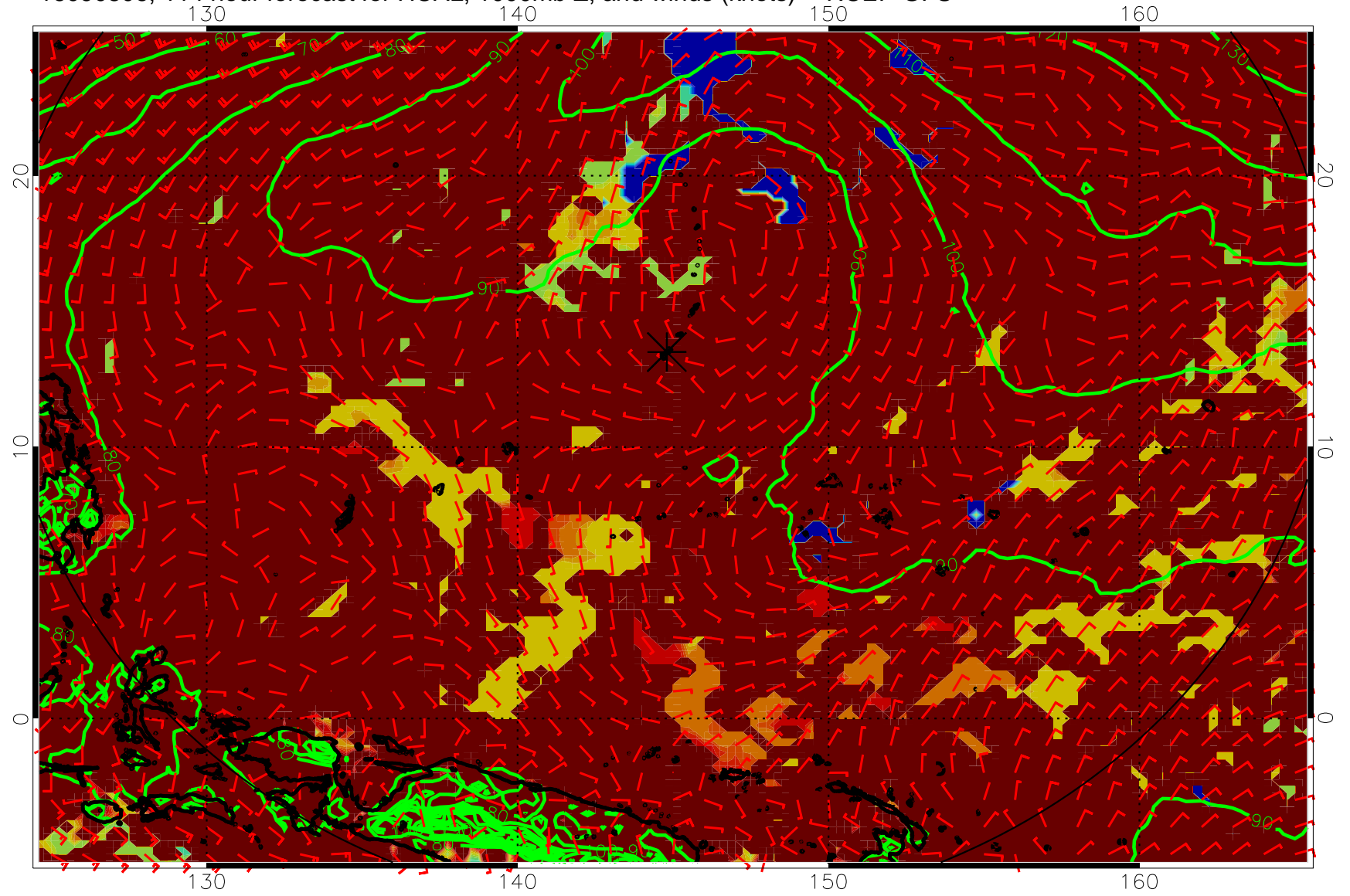
16090806, 114 hour forecast for HCAL, 1000mb Z, and winds (knots) -- NCEP GFS
