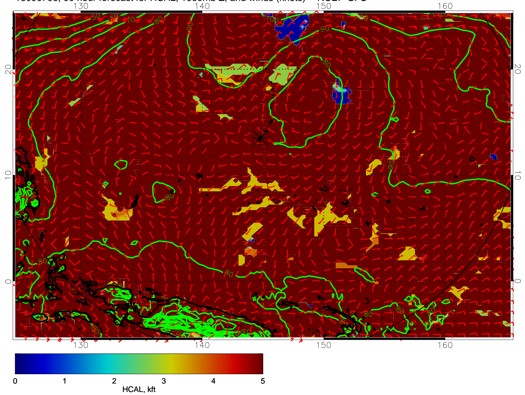
16090706, 90 hour forecast for HCAL, 1000mb Z, and winds (knots) -- NCEP GFS
