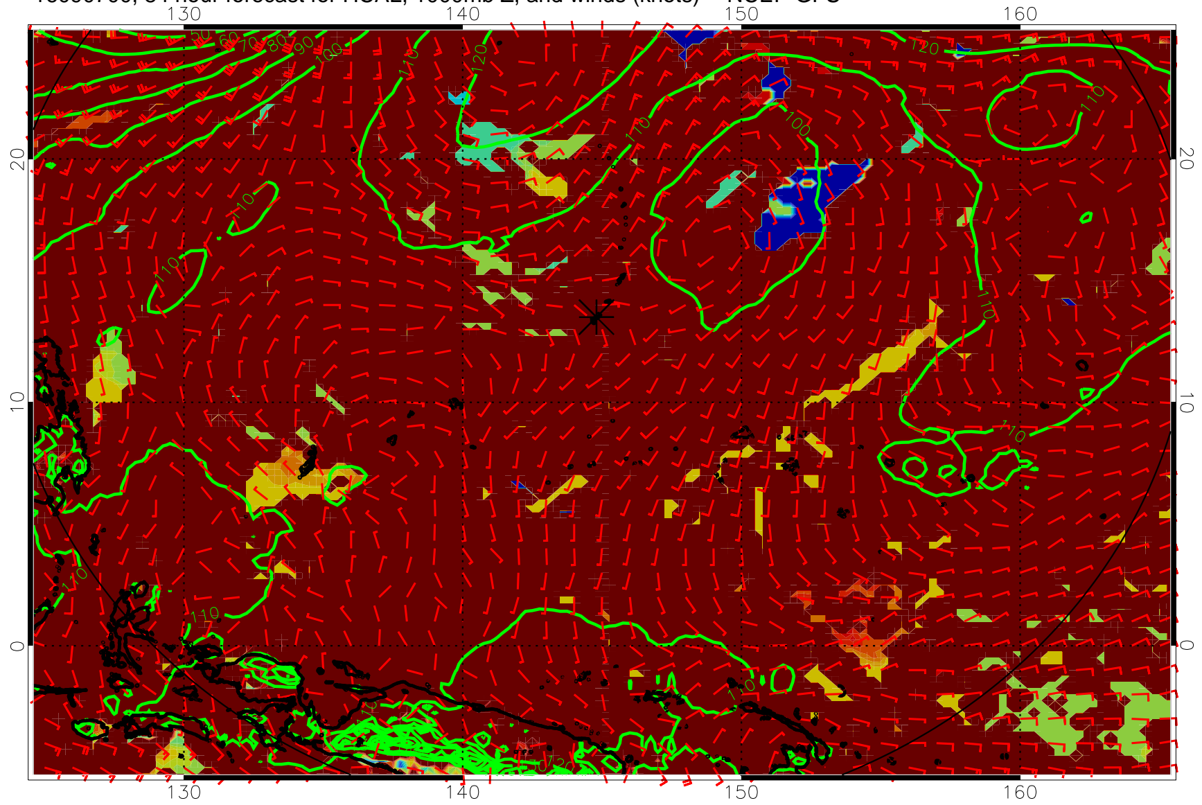
16090700, 84 hour forecast for HCAL, 1000mb Z, and winds (knots) -- NCEP GFS
