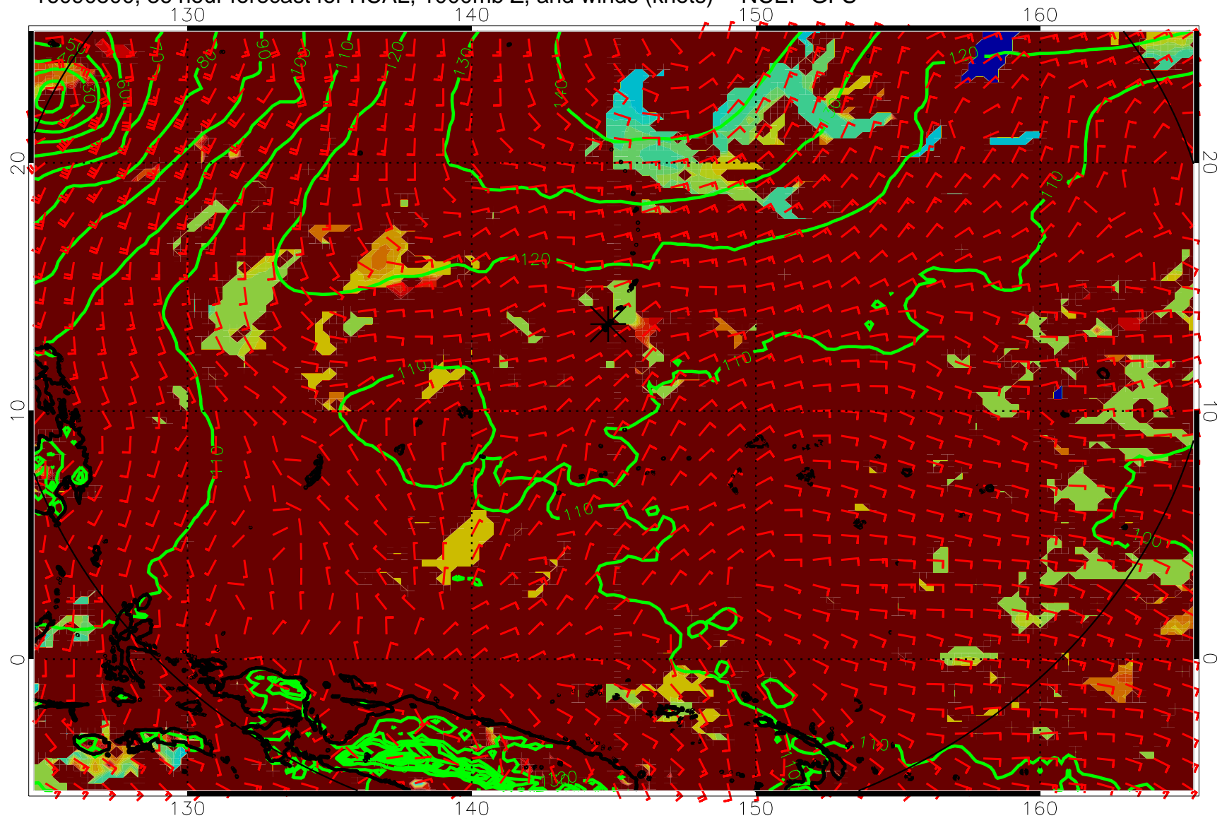
16090500, 36 hour forecast for HCAL, 1000mb Z, and winds (knots) -- NCEP GFS
