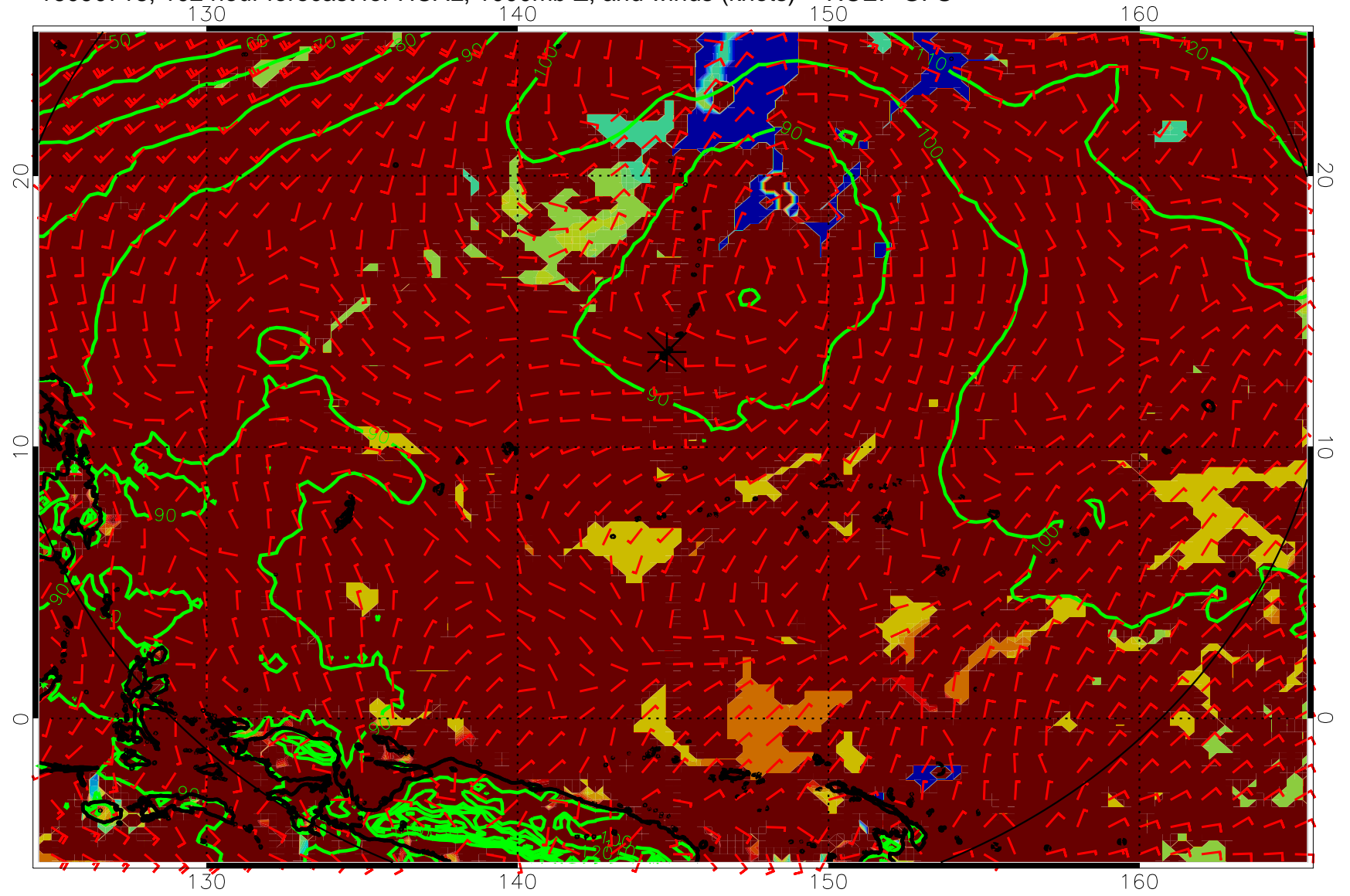
16090718, 102 hour forecast for HCAL, 1000mb Z, and winds (knots) -- NCEP GFS
