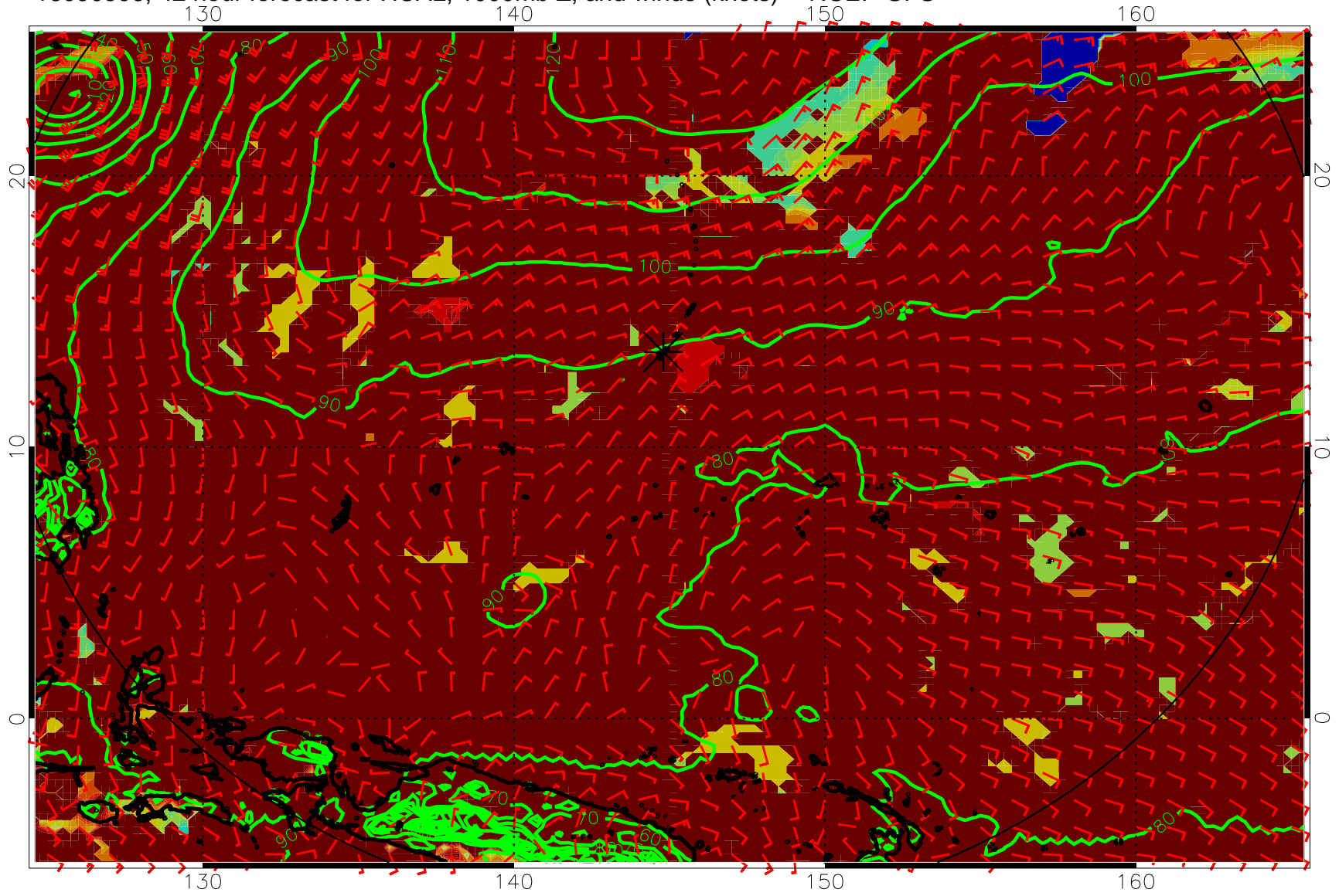
16090506, 42 hour forecast for HCAL, 1000mb Z, and winds (knots) -- NCEP GFS
