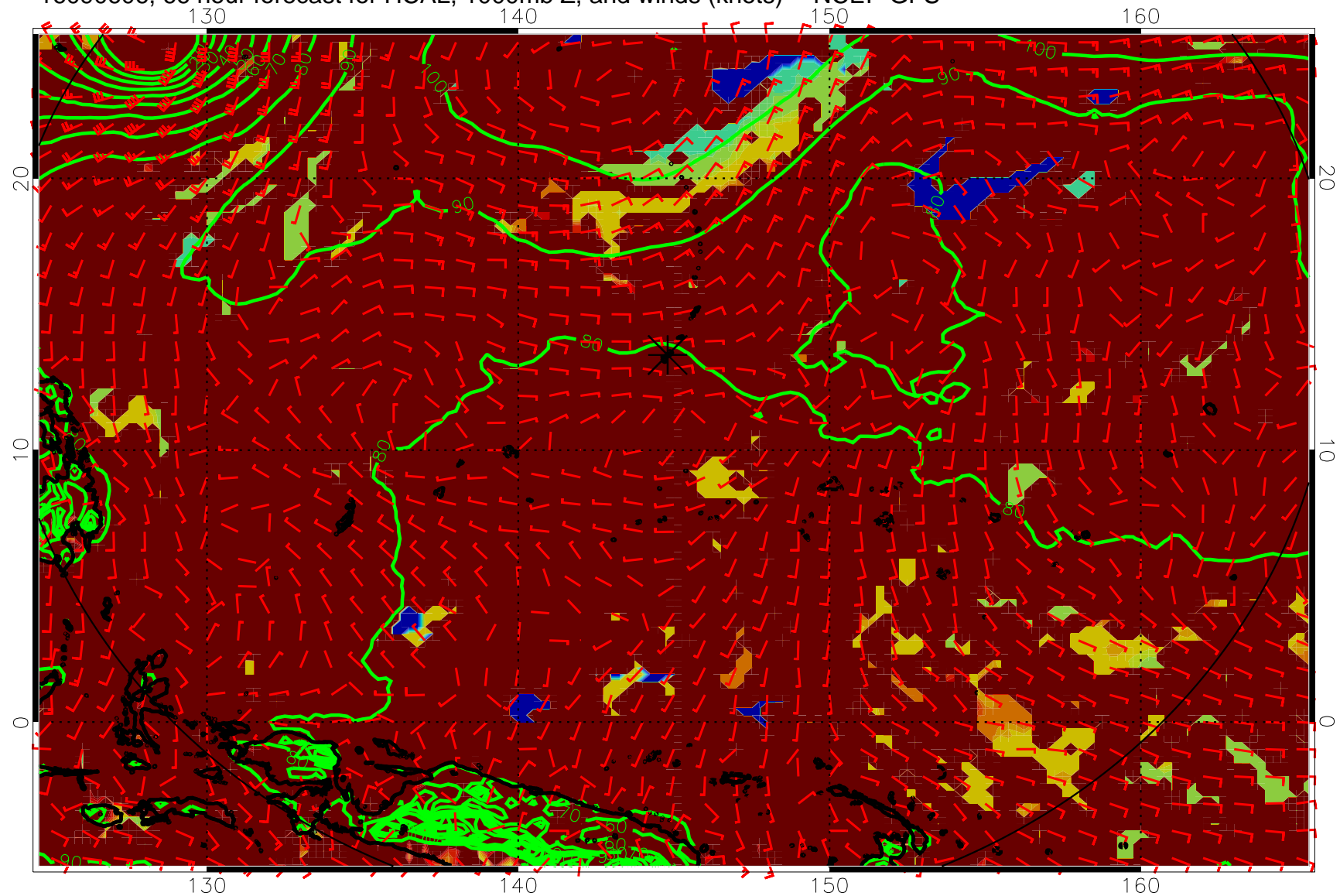
16090606, 66 hour forecast for HCAL, 1000mb Z, and winds (knots) -- NCEP GFS
