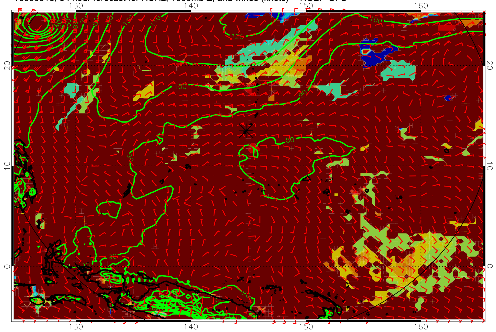
16090518, 54 hour forecast for HCAL, 1000mb Z, and winds (knots) -- NCEP GFS
