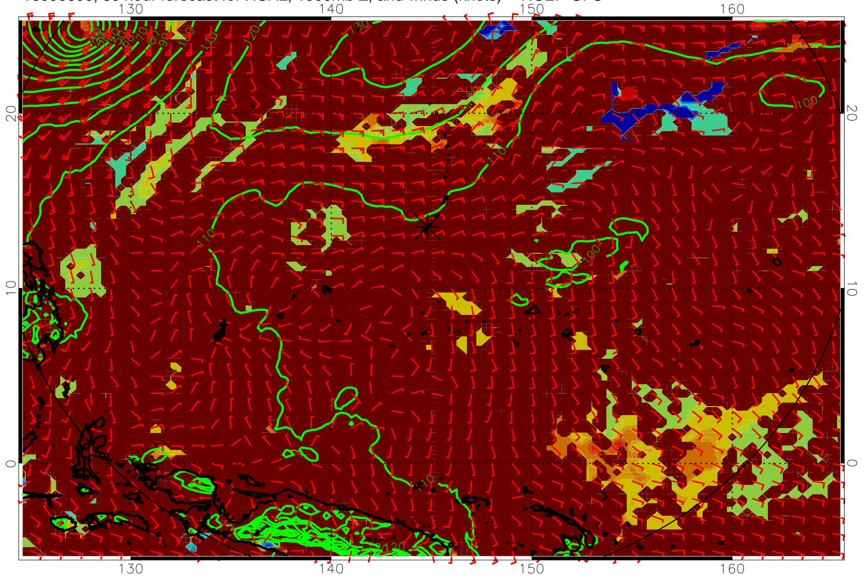
16090600, 60 hour forecast for HCAL, 1000mb Z, and winds (knots) -- NCEP GFS
