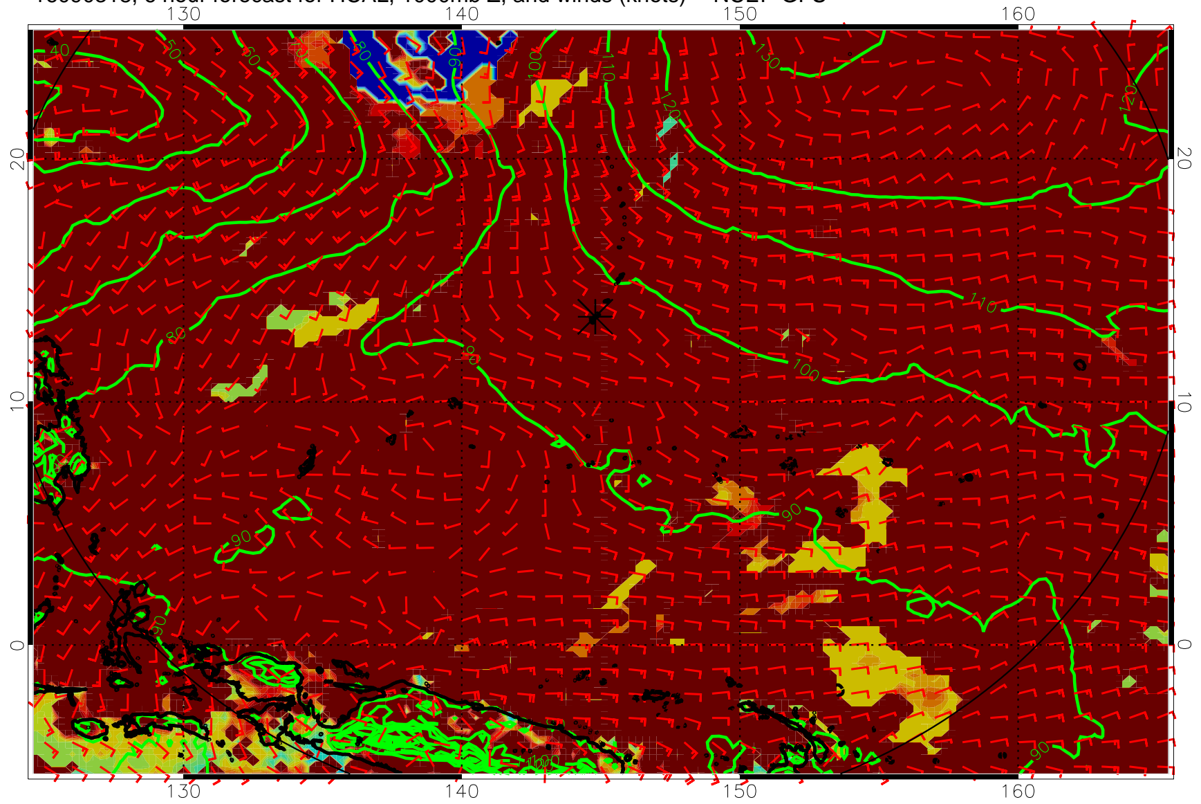
16090318, 6 hour forecast for HCAL, 1000mb Z, and winds (knots) -- NCEP GFS
