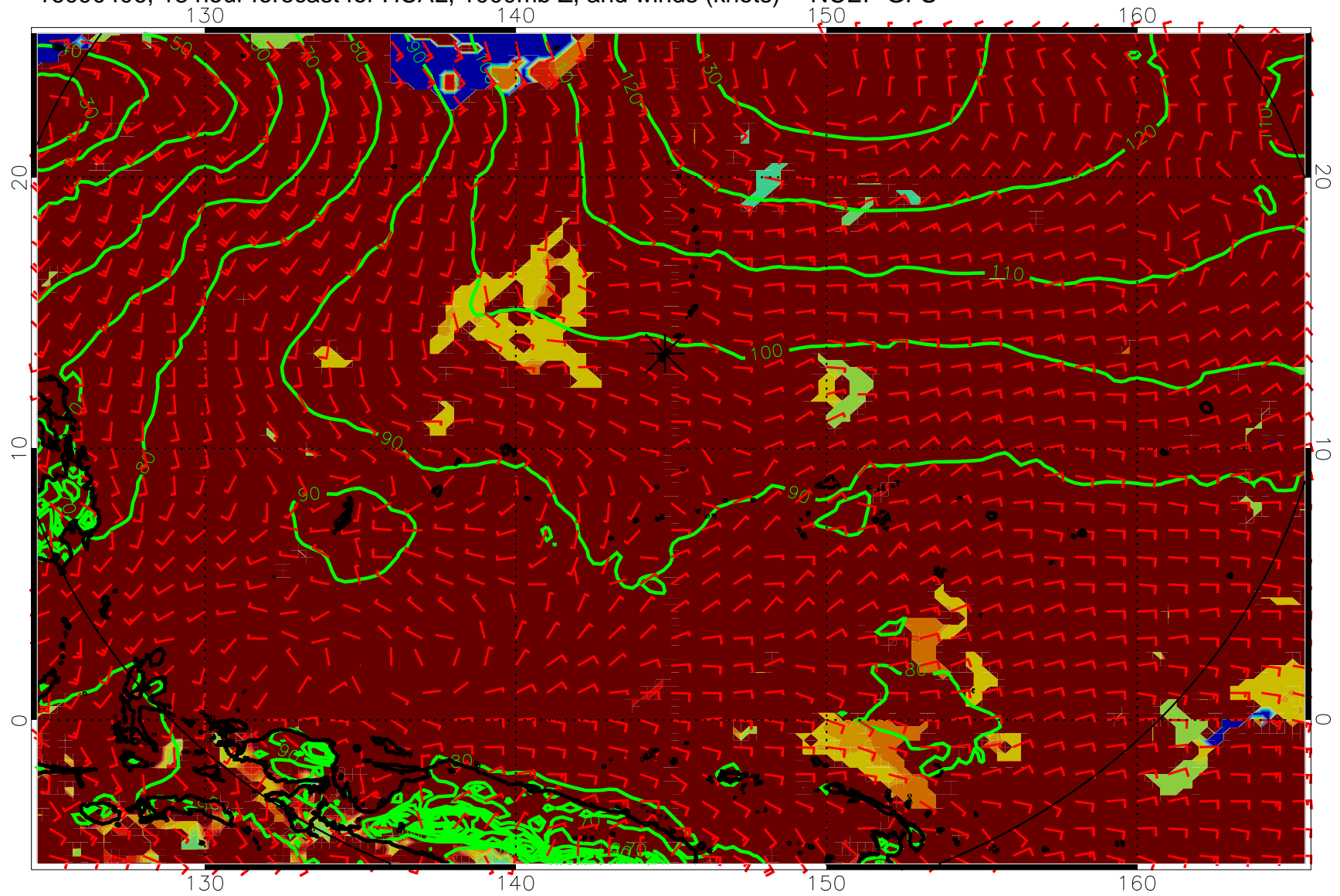
16090406, 18 hour forecast for HCAL, 1000mb Z, and winds (knots) -- NCEP GFS
