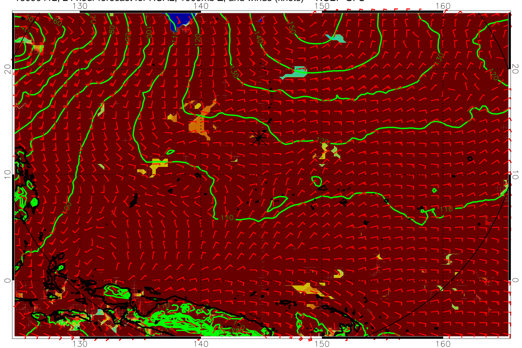
16090412, 24 hour forecast for HCAL, 1000mb Z, and winds (knots) -- NCEP GFS
