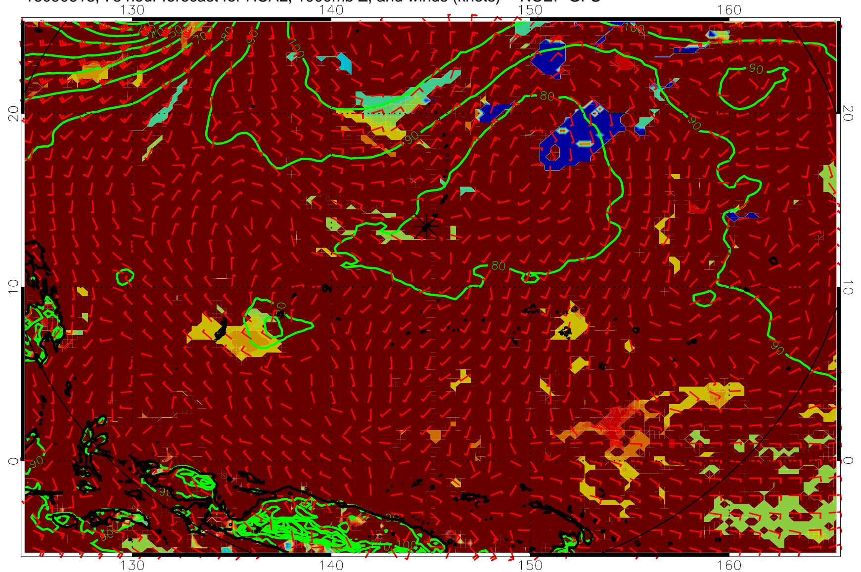
16090618, 78 hour forecast for HCAL, 1000mb Z, and winds (knots) -- NCEP GFS
