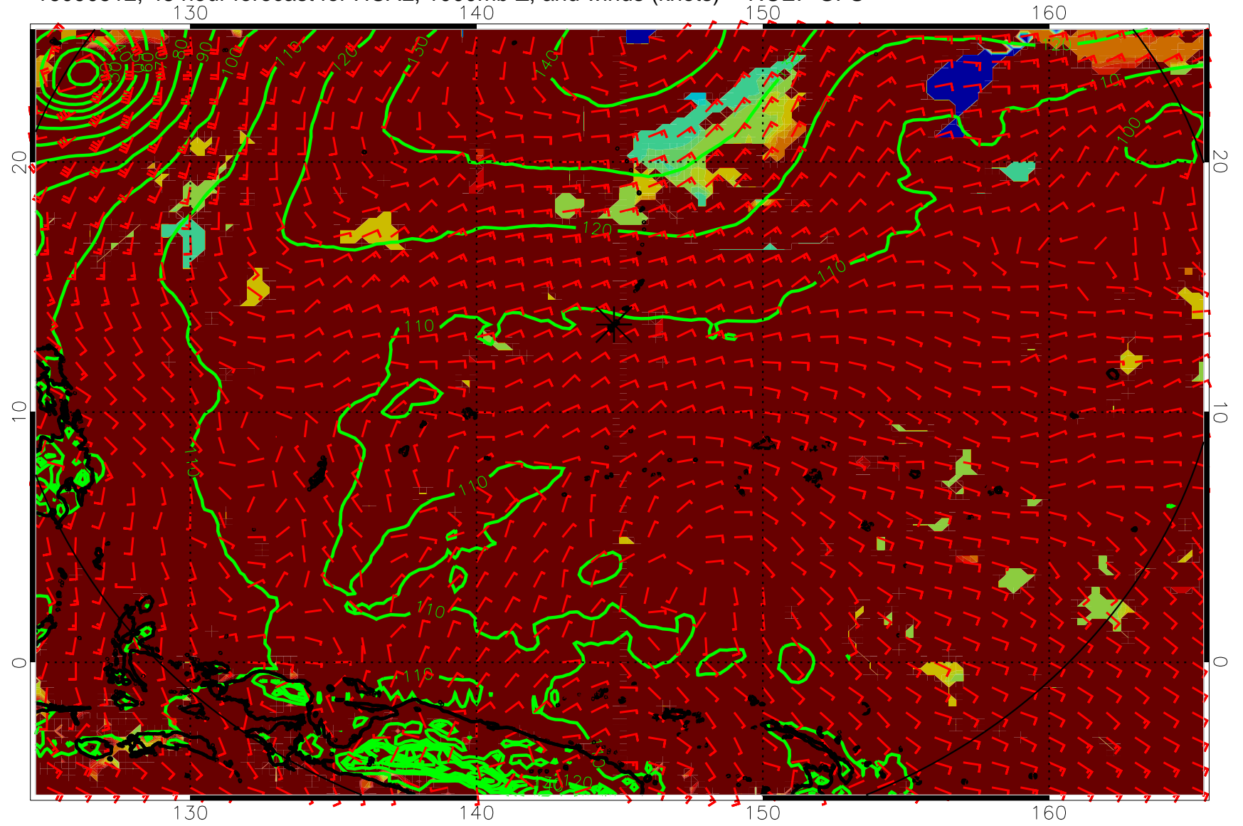
16090512, 48 hour forecast for HCAL, 1000mb Z, and winds (knots) -- NCEP GFS
