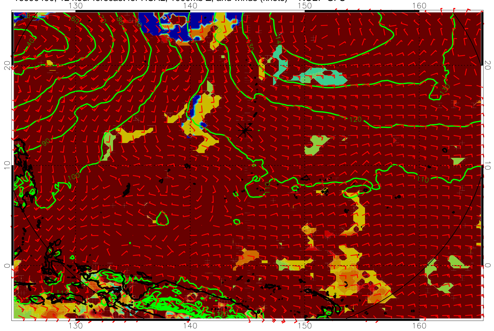
16090400, 12 hour forecast for HCAL, 1000mb Z, and winds (knots) -- NCEP GFS
