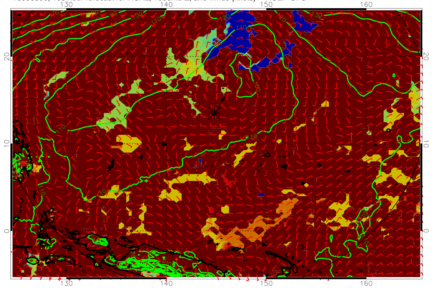
16090800, 108 hour forecast for HCAL, 1000mb Z, and winds (knots) -- NCEP GFS
