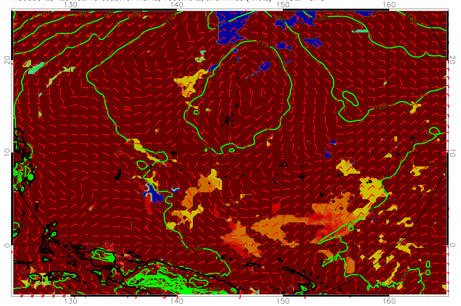
16090812, 120 hour forecast for HCAL, 1000mb Z, and winds (knots) -- NCEP GFS
