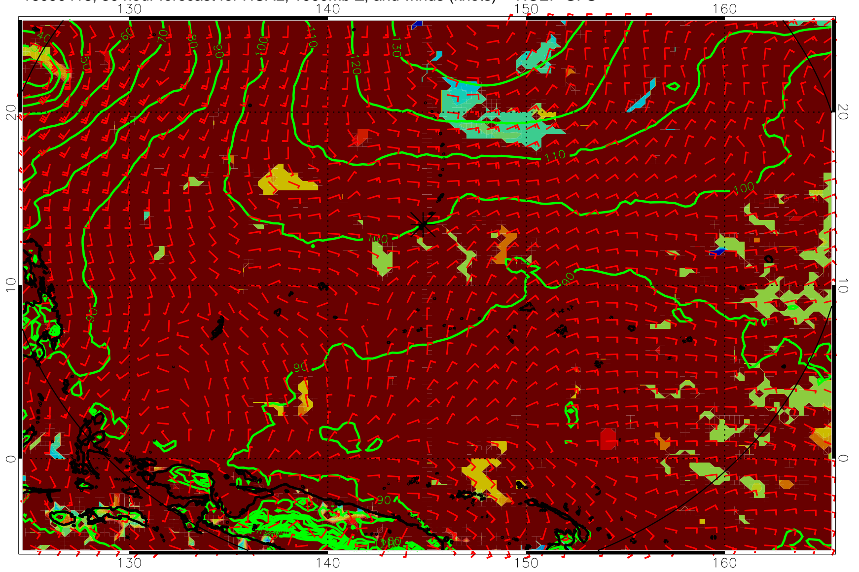
16090418, 30 hour forecast for HCAL, 1000mb Z, and winds (knots) -- NCEP GFS
