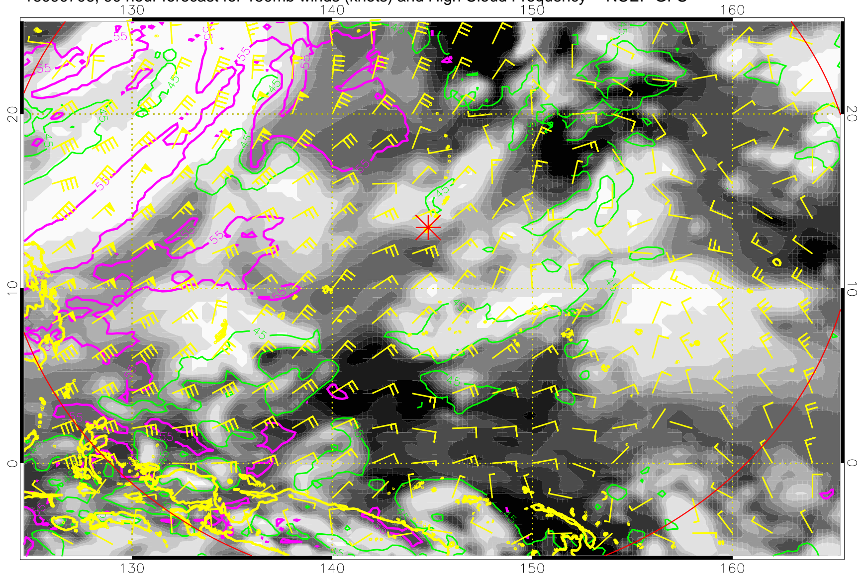
16090706, 90 hour forecast for 150mb winds (knots) and High Cloud Frequency -- NCEP GFS
