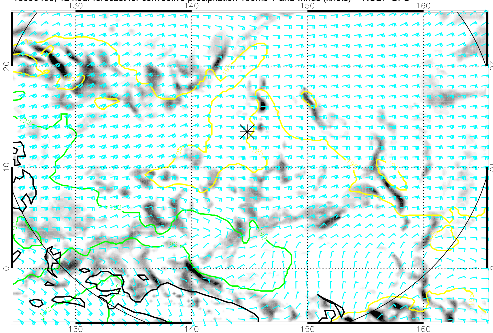
16090400, 12 hour forecast for convective precipitation 100mb T and winds (knots) -- NCEP GFS
