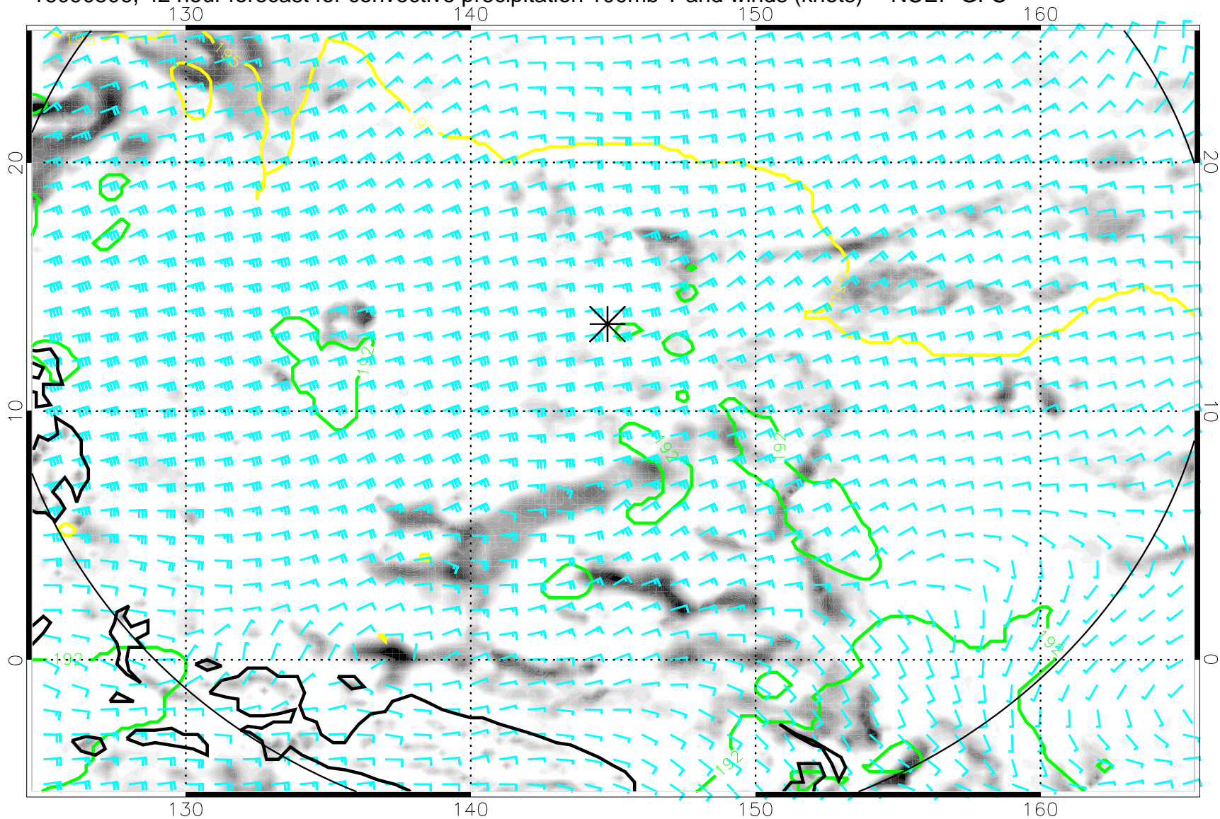
16090506, 42 hour forecast for convective precipitation 100mb T and winds (knots) -- NCEP GFS
