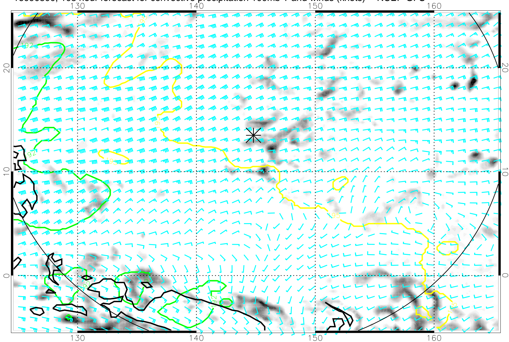
16090800, 108 hour forecast for convective precipitation 100mb T and winds (knots) -- NCEP GFS
