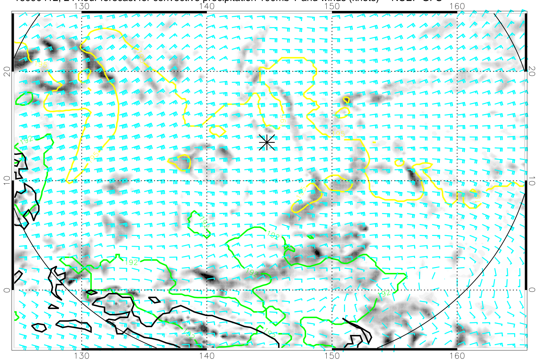
16090412, 24 hour forecast for convective precipitation 100mb T and winds (knots) -- NCEP GFS
