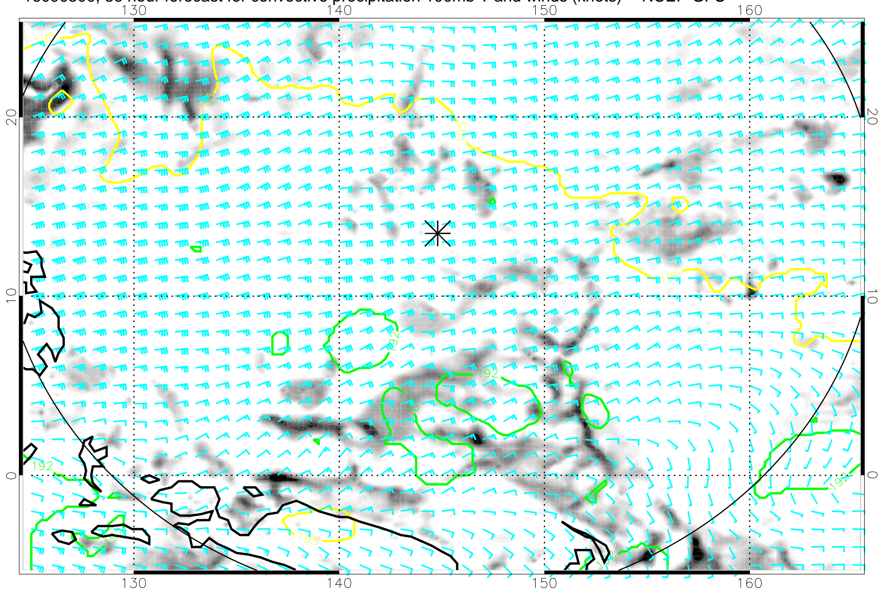
16090500, 36 hour forecast for convective precipitation 100mb T and winds (knots) -- NCEP GFS
