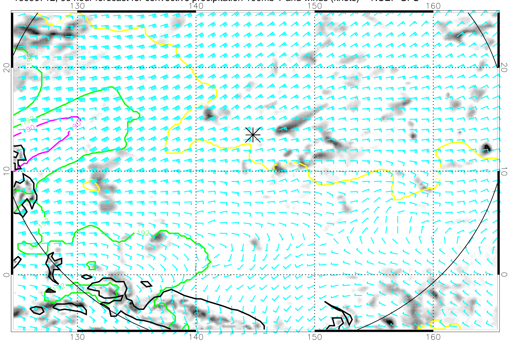
16090712, 96 hour forecast for convective precipitation 100mb T and winds (knots) -- NCEP GFS
