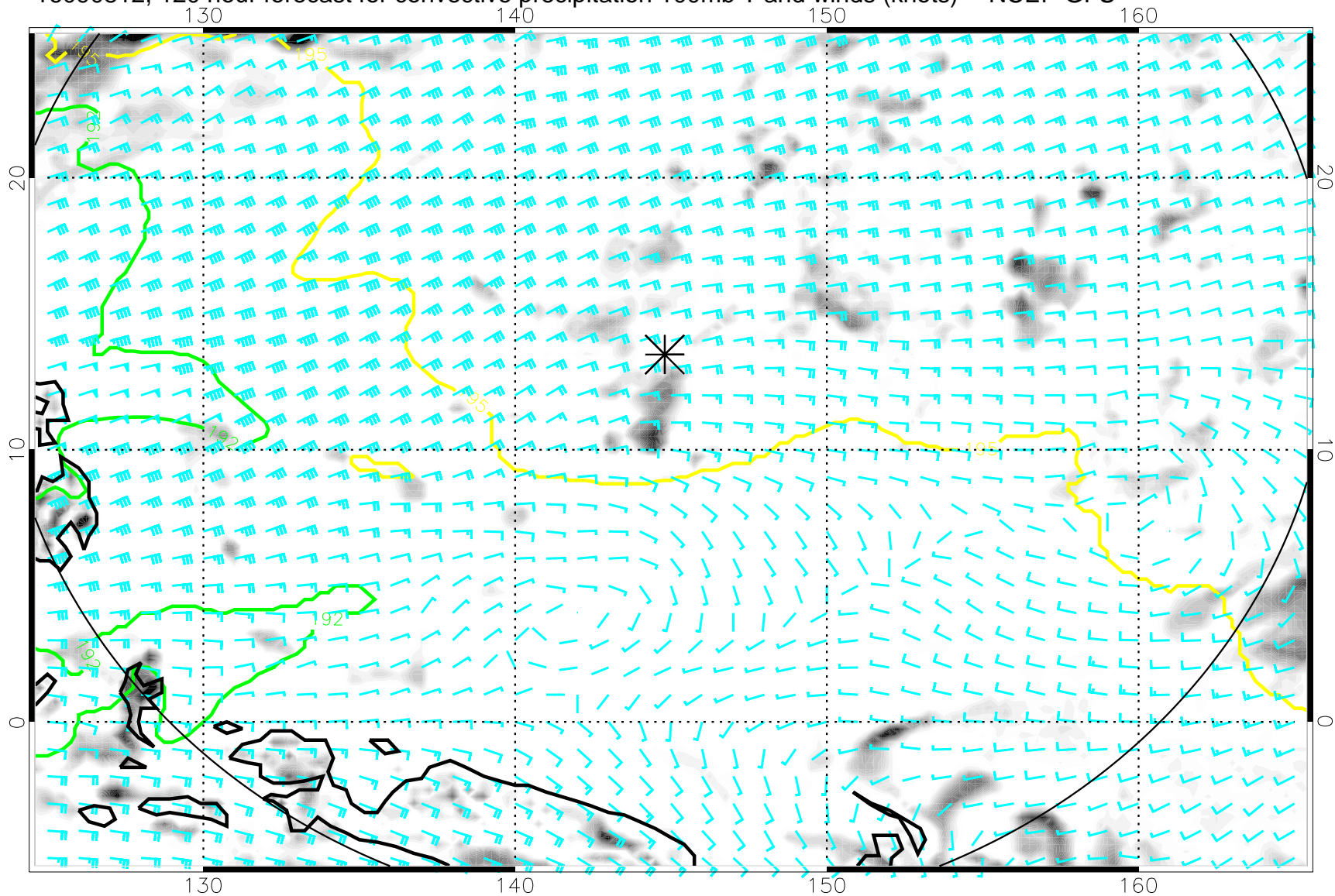
16090812, 120 hour forecast for convective precipitation 100mb T and winds (knots) -- NCEP GFS
