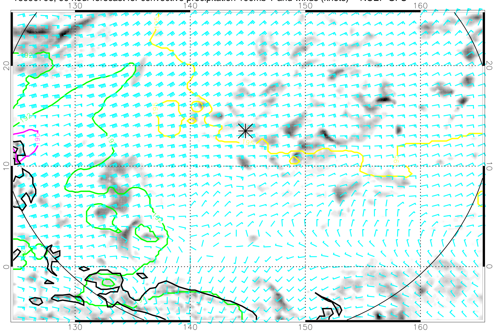
16090706, 90 hour forecast for convective precipitation 100mb T and winds (knots) -- NCEP GFS
