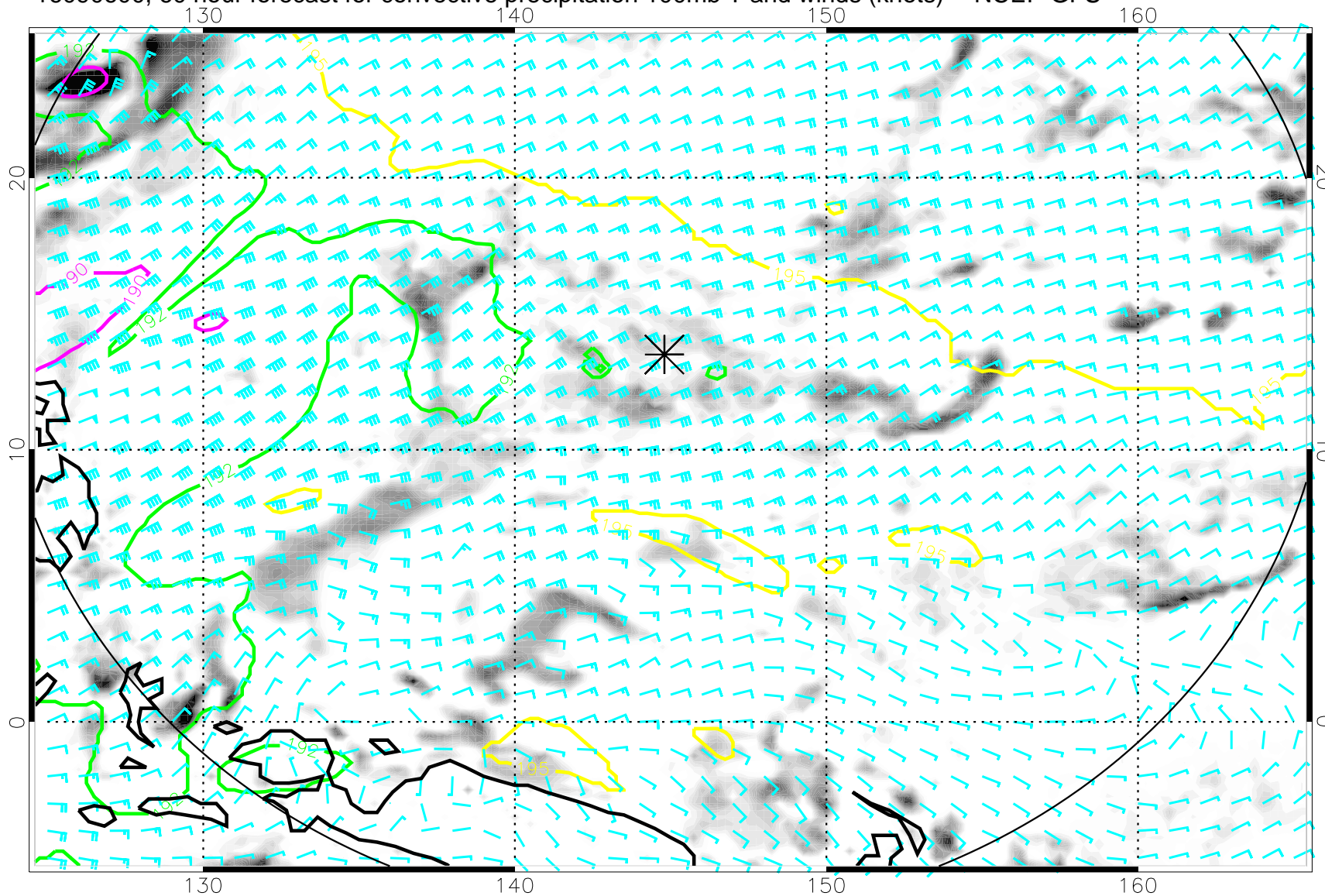
16090600, 60 hour forecast for convective precipitation 100mb T and winds (knots) -- NCEP GFS
