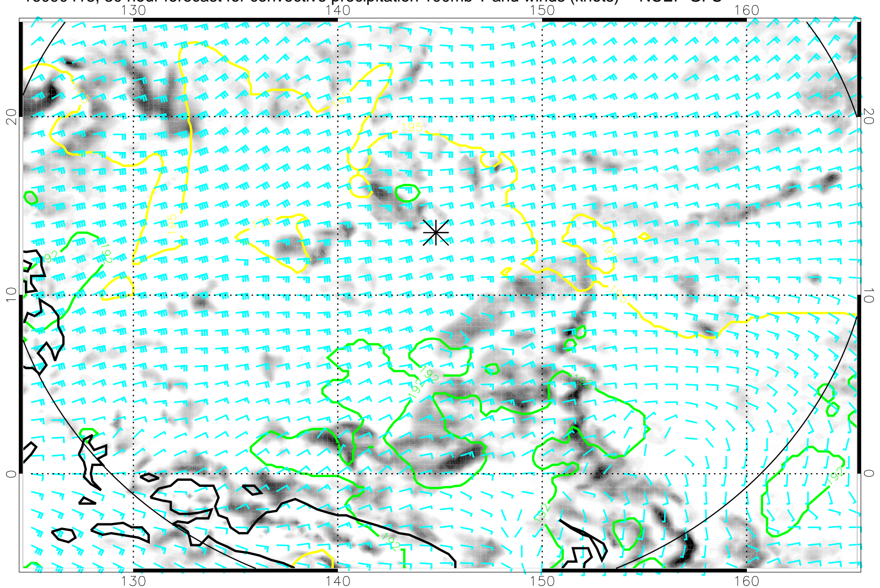
16090418, 30 hour forecast for convective precipitation 100mb T and winds (knots) -- NCEP GFS
