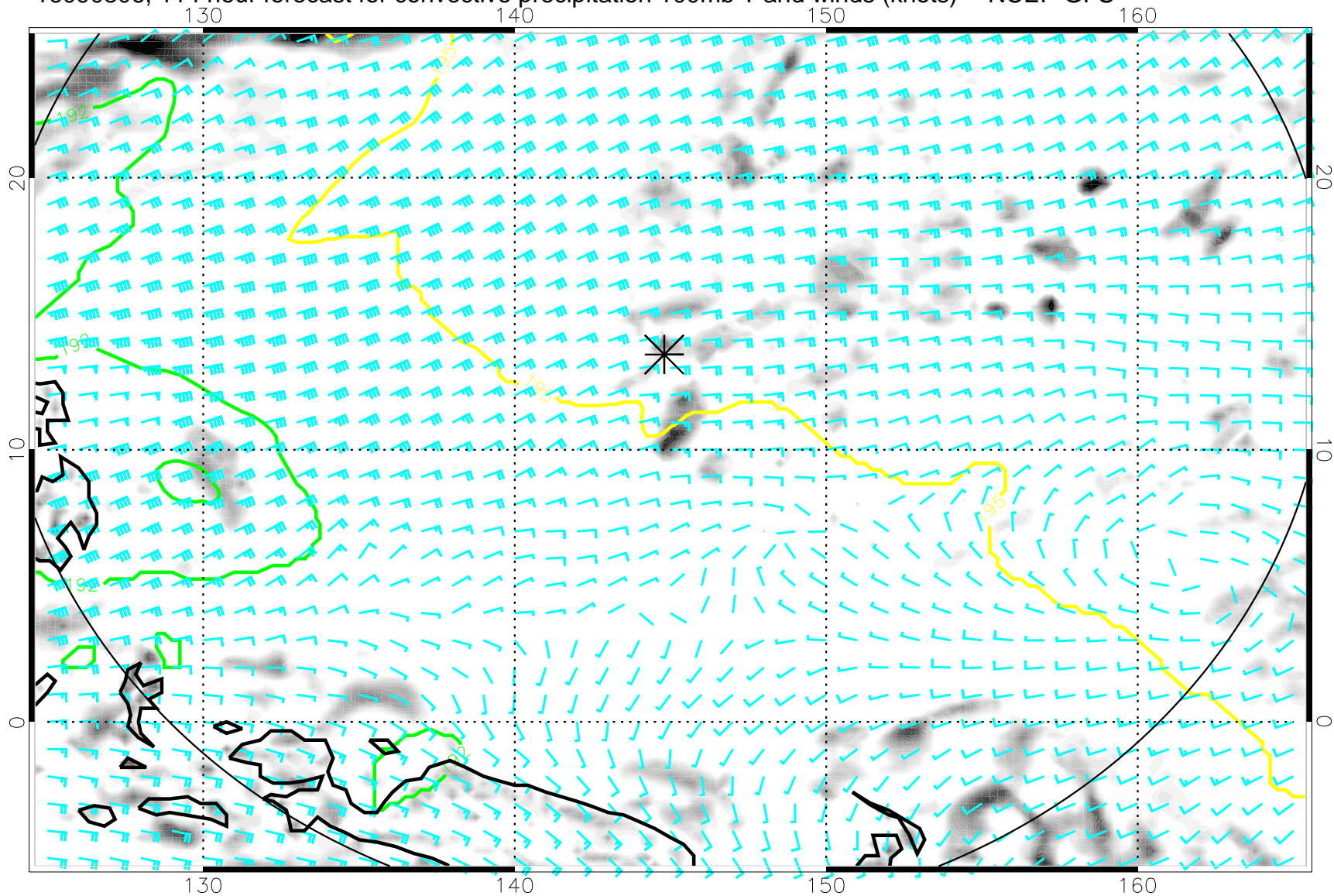
16090806, 114 hour forecast for convective precipitation 100mb T and winds (knots) -- NCEP GFS
