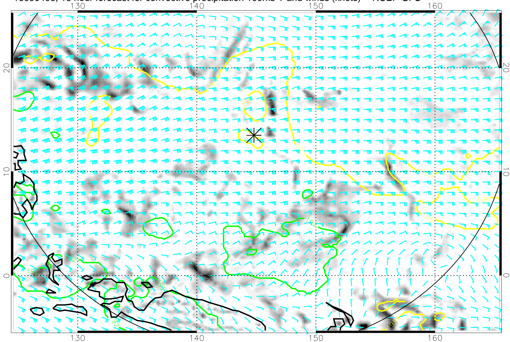
16090406, 18 hour forecast for convective precipitation 100mb T and winds (knots) -- NCEP GFS
