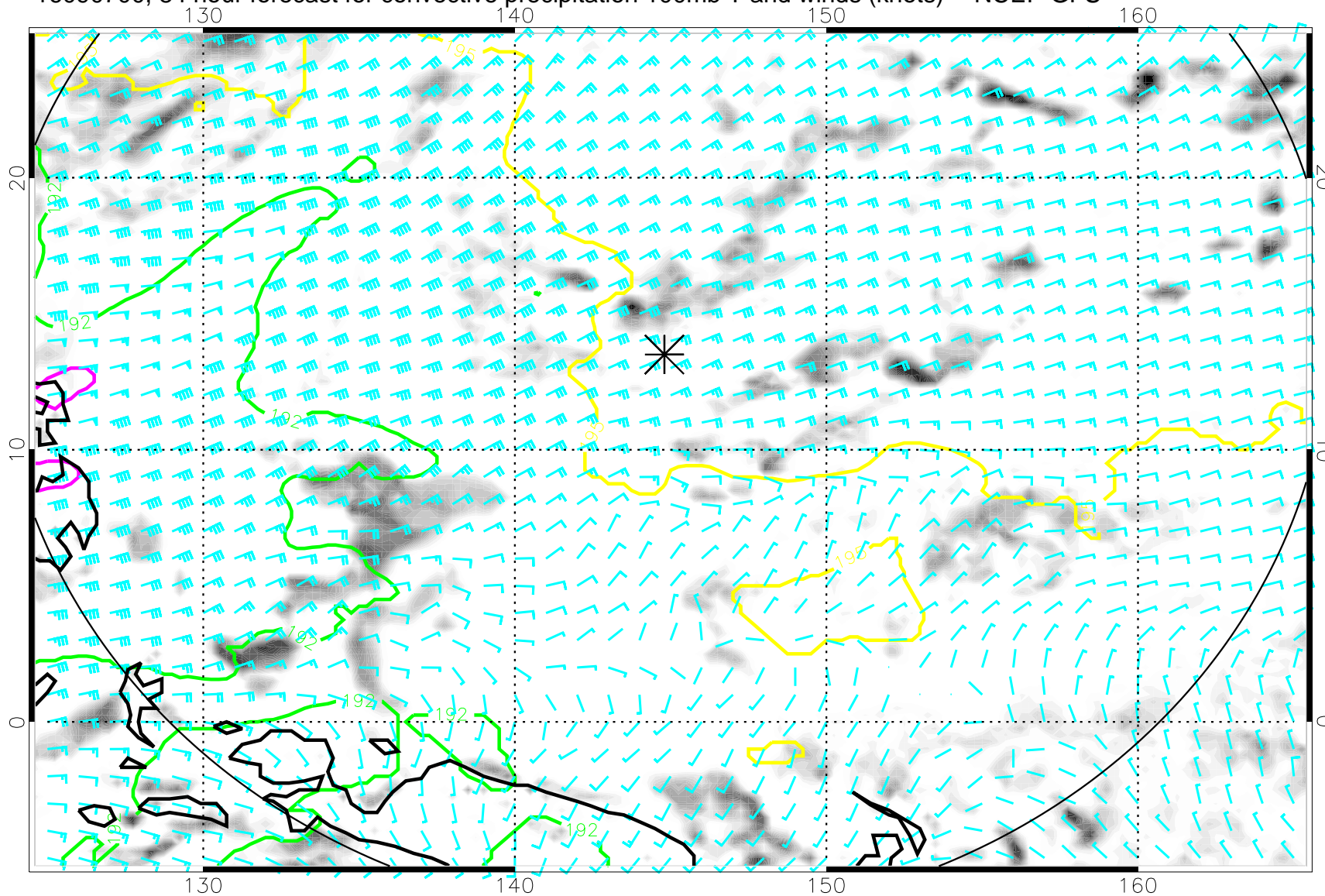
16090700, 84 hour forecast for convective precipitation 100mb T and winds (knots) -- NCEP GFS
