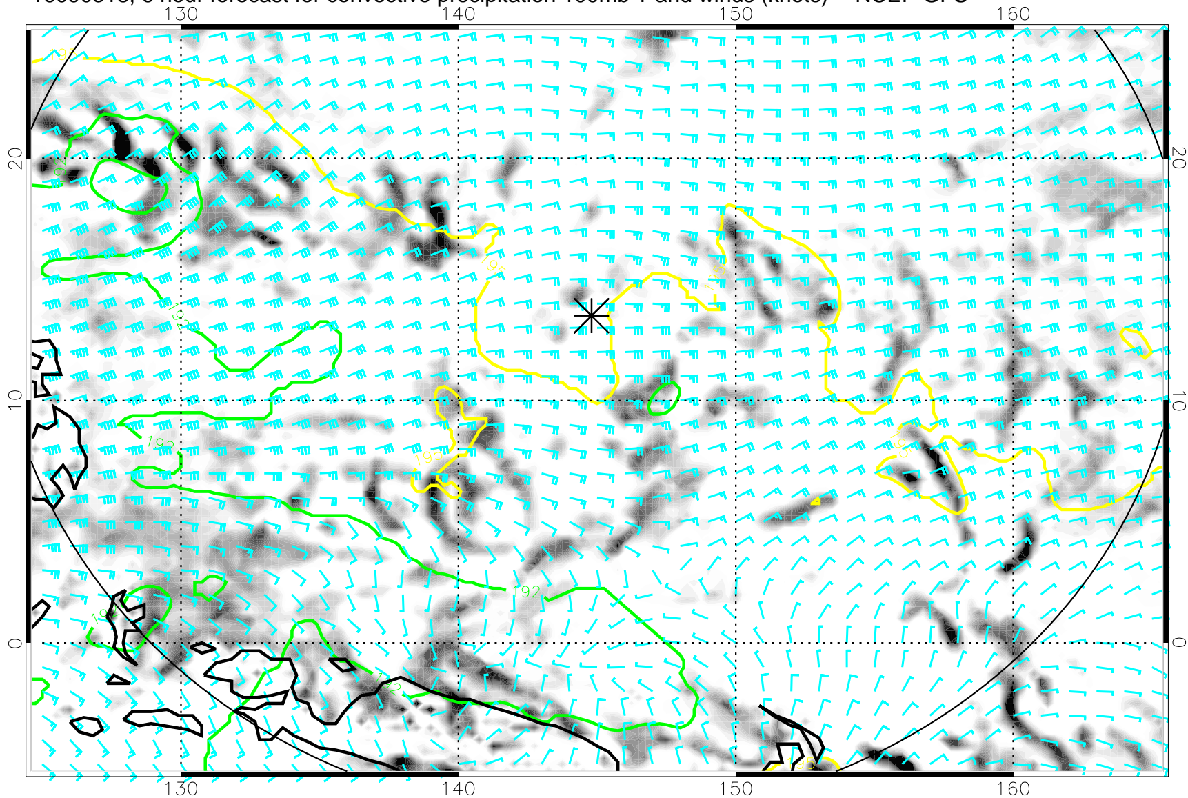
16090318, 6 hour forecast for convective precipitation 100mb T and winds (knots) -- NCEP GFS
