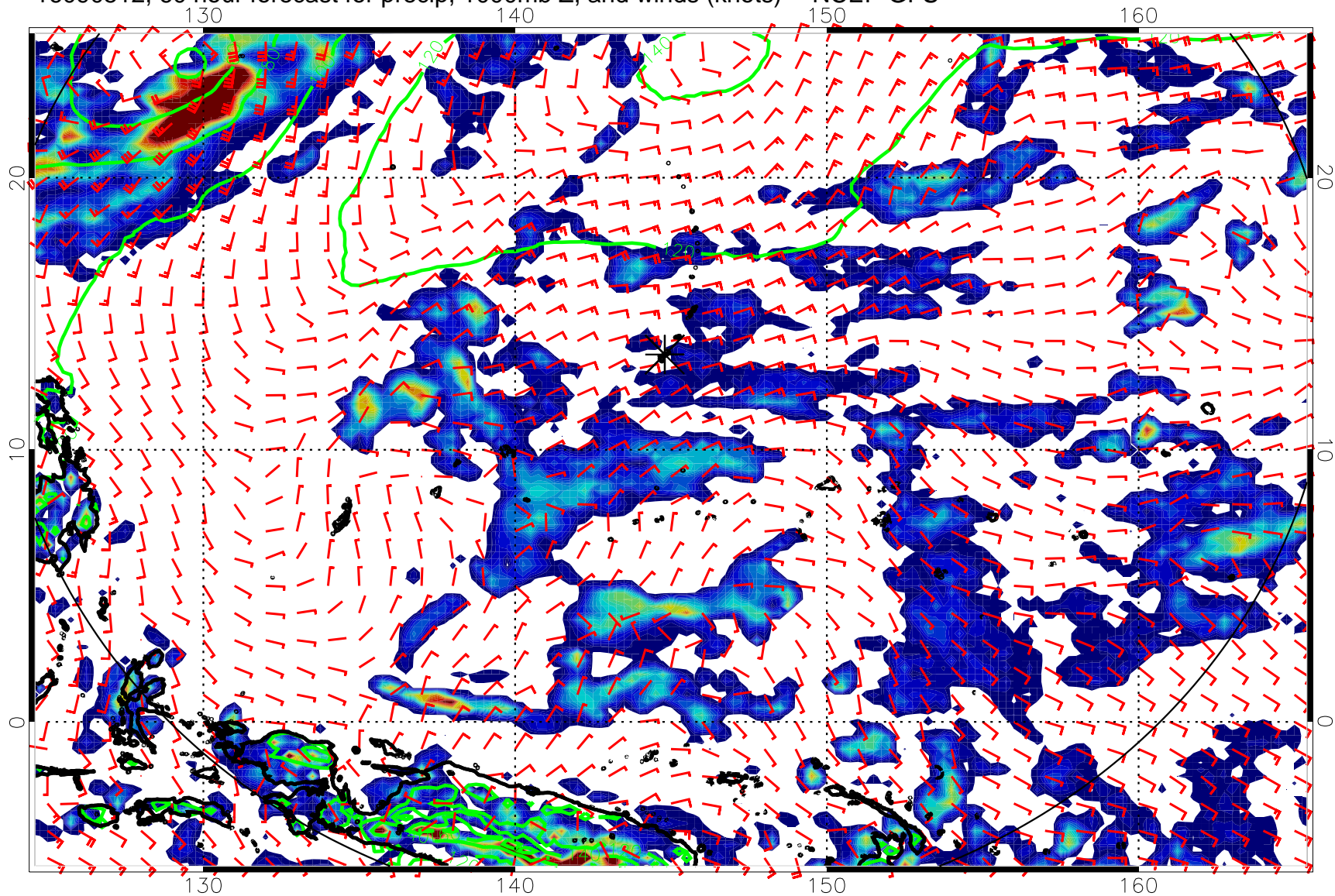
16090512, 60 hour forecast for precip, 1000mb Z, and winds (knots) -- NCEP GFS
