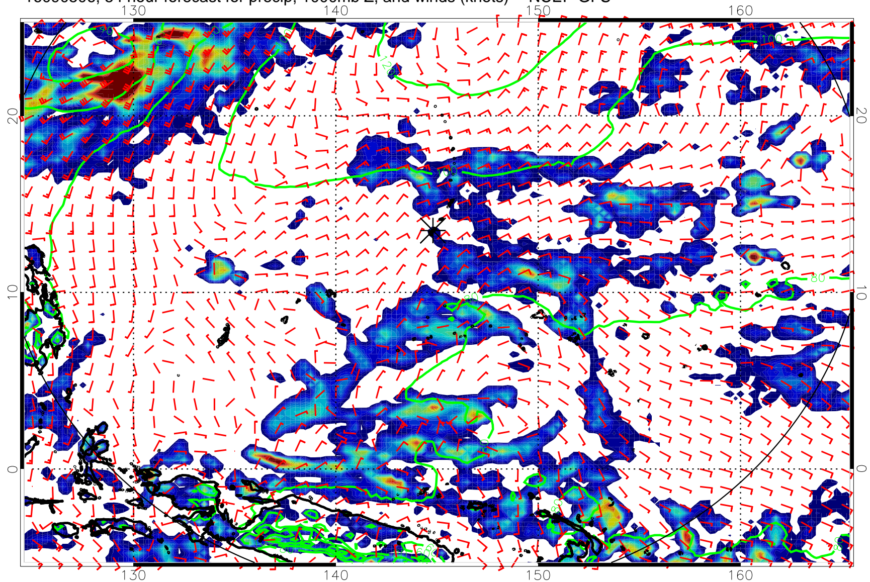
16090506, 54 hour forecast for precip, 1000mb Z, and winds (knots) -- NCEP GFS
