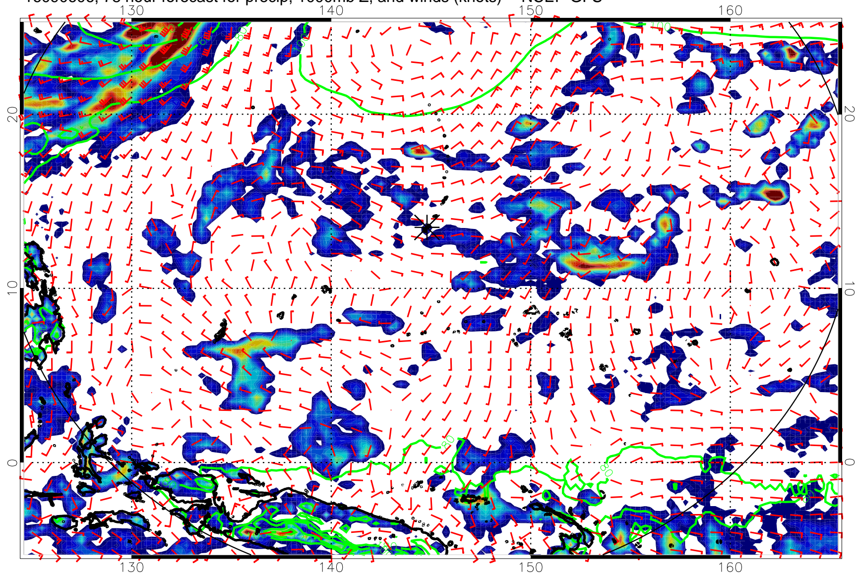
16090606, 78 hour forecast for precip, 1000mb Z, and winds (knots) -- NCEP GFS
