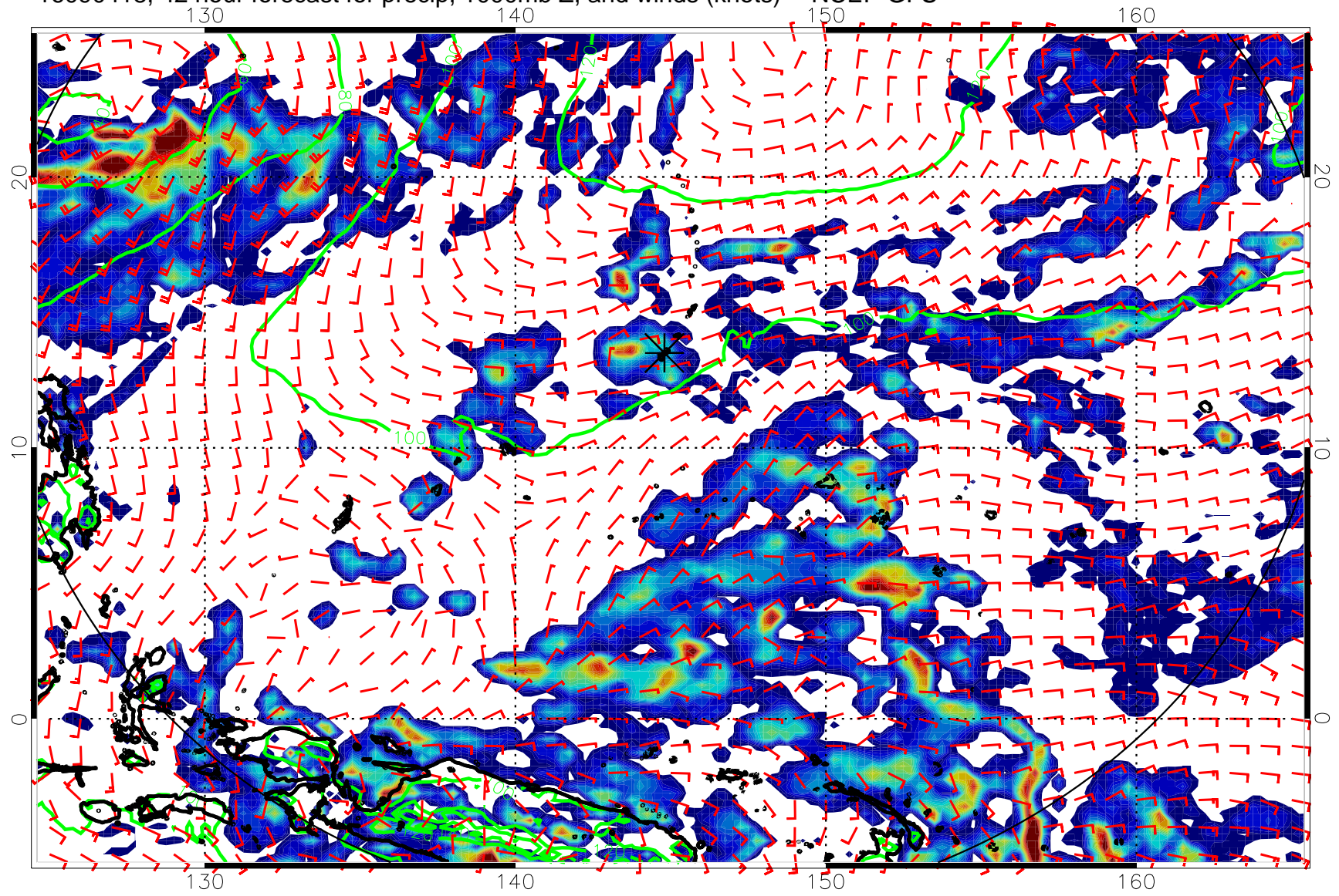
16090418, 42 hour forecast for precip, 1000mb Z, and winds (knots) -- NCEP GFS
