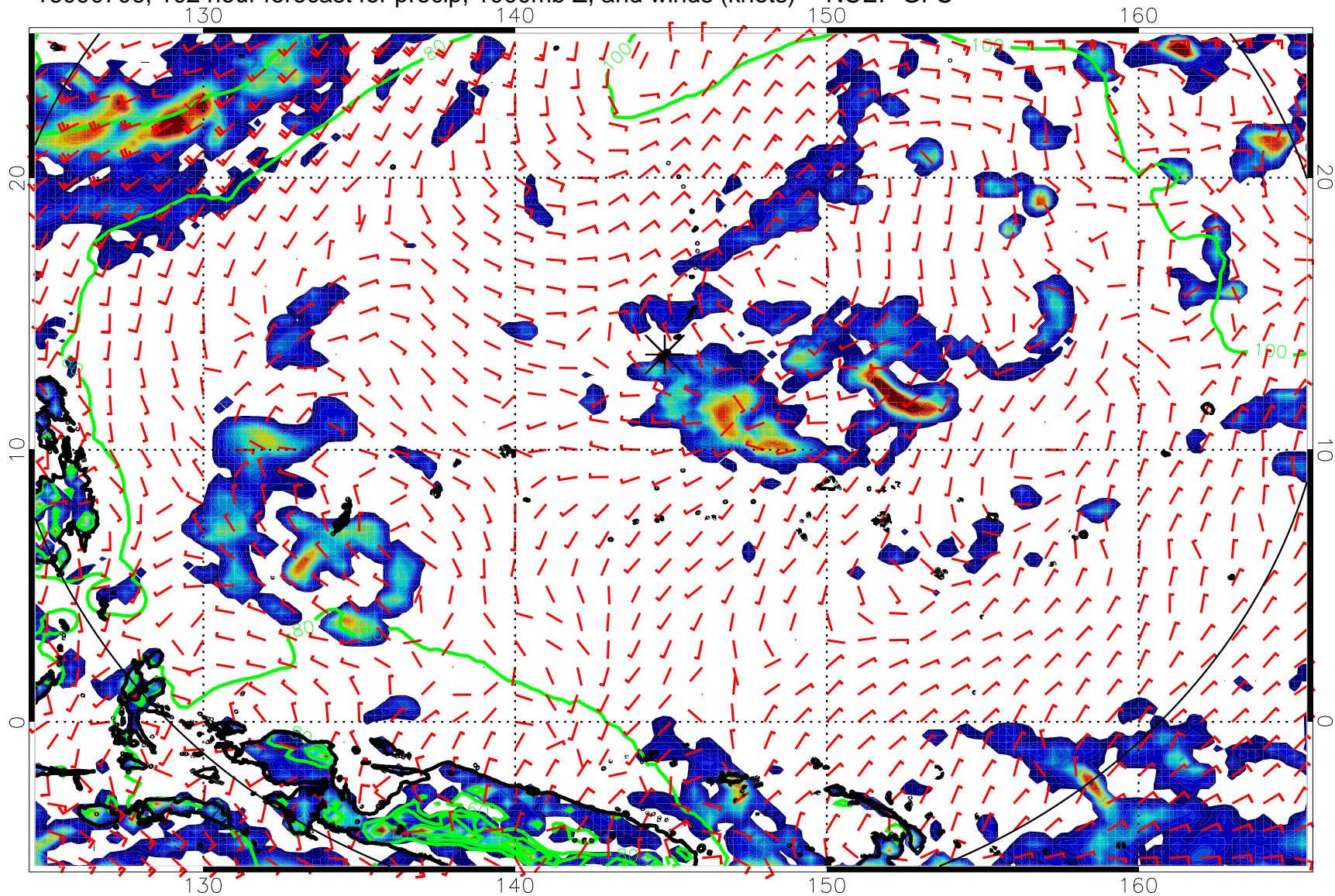
16090706, 102 hour forecast for precip, 1000mb Z, and winds (knots) -- NCEP GFS
