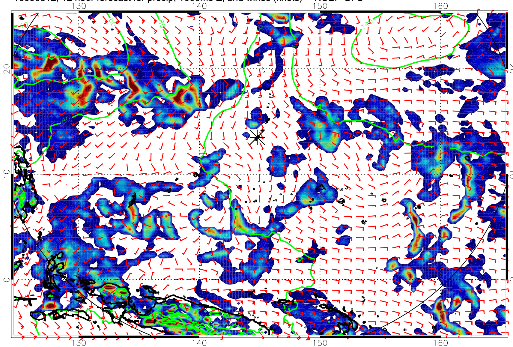
16090312, 12 hour forecast for precip, 1000mb Z, and winds (knots) -- NCEP GFS
