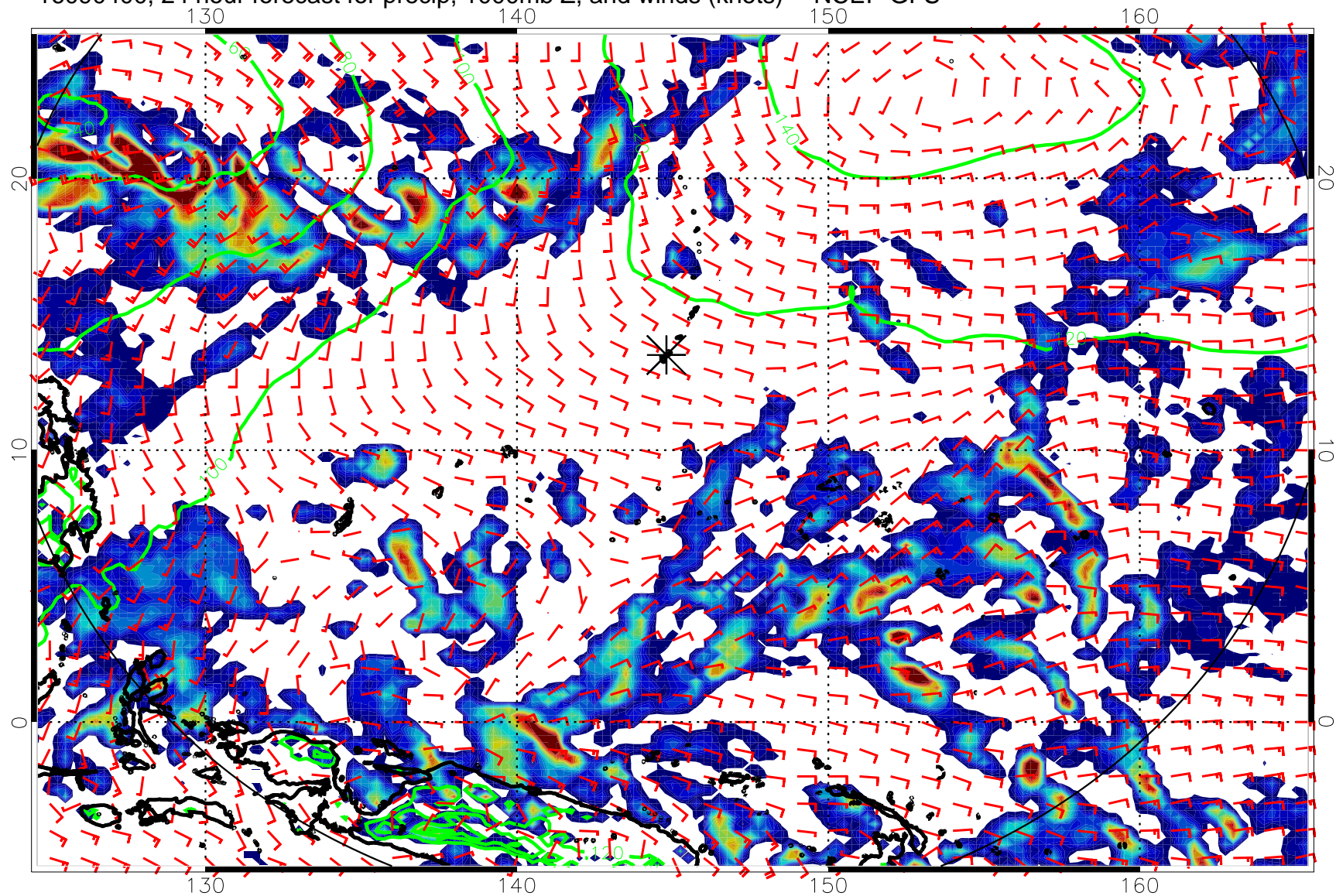
16090400, 24 hour forecast for precip, 1000mb Z, and winds (knots) -- NCEP GFS
