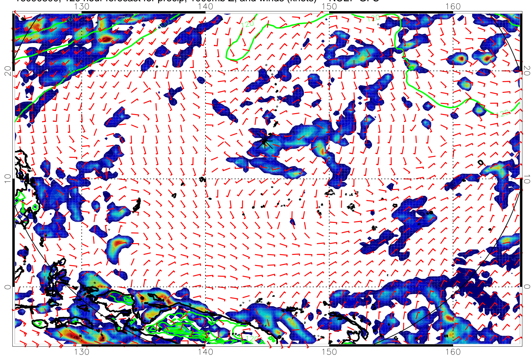
16090800, 120 hour forecast for precip, 1000mb Z, and winds (knots) -- NCEP GFS
