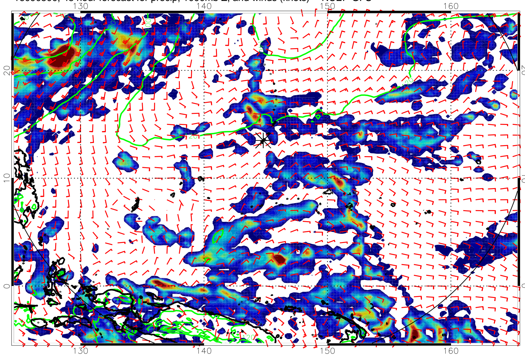
16090500, 48 hour forecast for precip, 1000mb Z, and winds (knots) -- NCEP GFS
