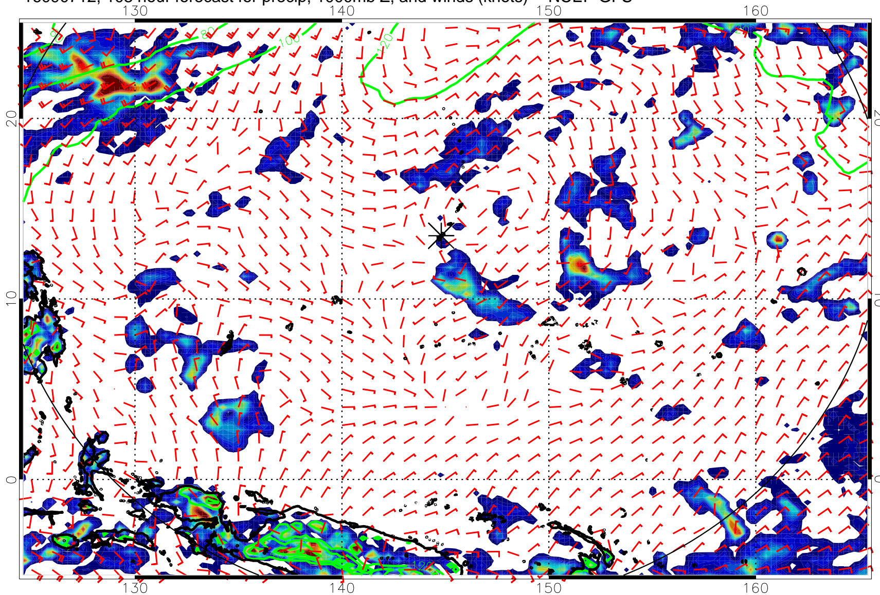
16090712, 108 hour forecast for precip, 1000mb Z, and winds (knots) -- NCEP GFS
