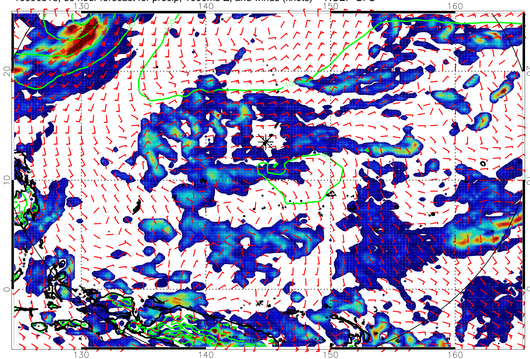
16090518, 66 hour forecast for precip, 1000mb Z, and winds (knots) -- NCEP GFS
