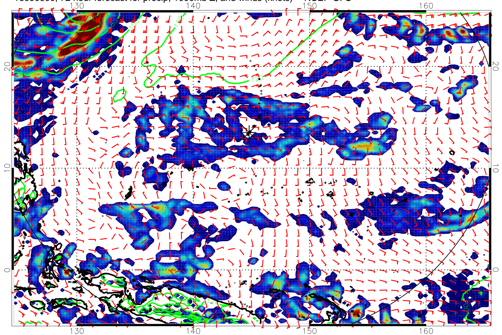
16090600, 72 hour forecast for precip, 1000mb Z, and winds (knots) -- NCEP GFS
