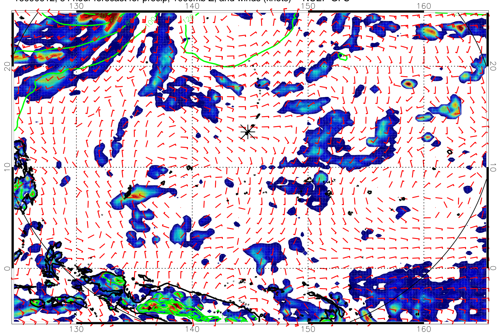
16090612, 84 hour forecast for precip, 1000mb Z, and winds (knots) -- NCEP GFS
