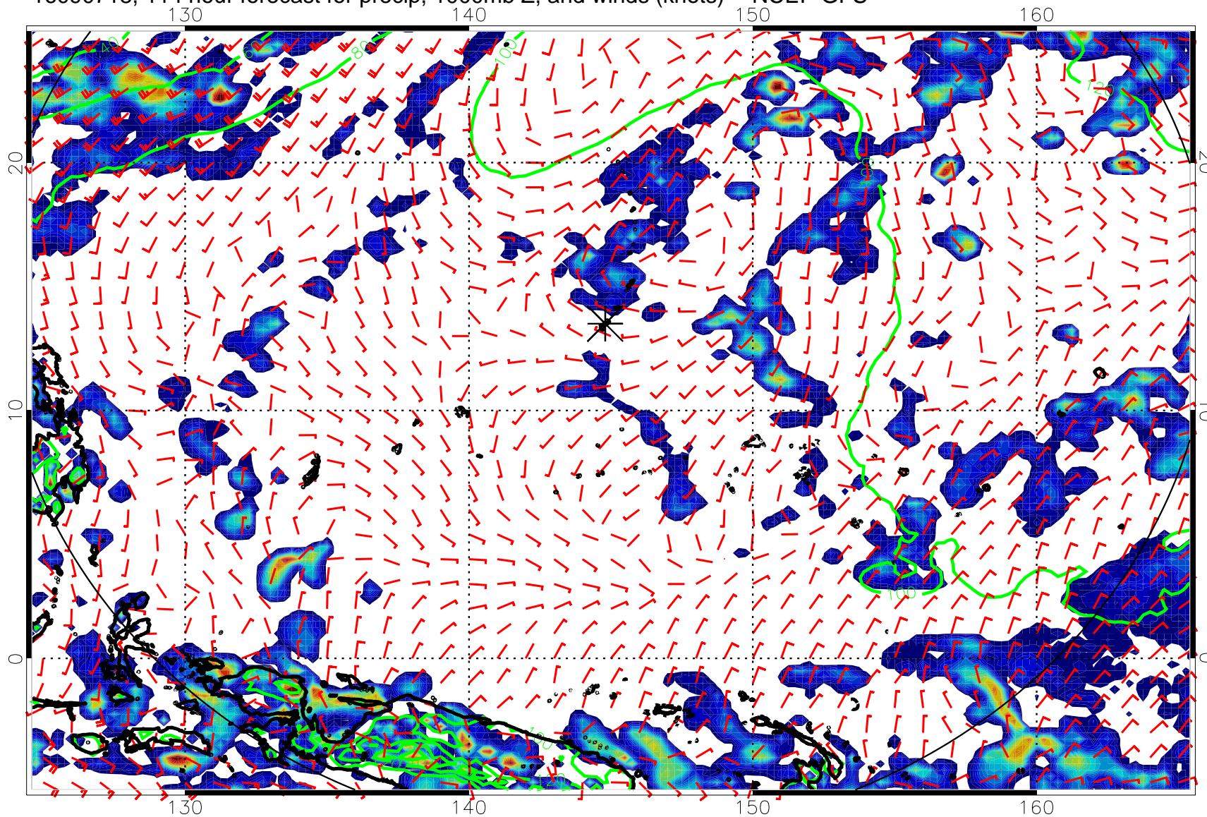
16090718, 114 hour forecast for precip, 1000mb Z, and winds (knots) -- NCEP GFS
