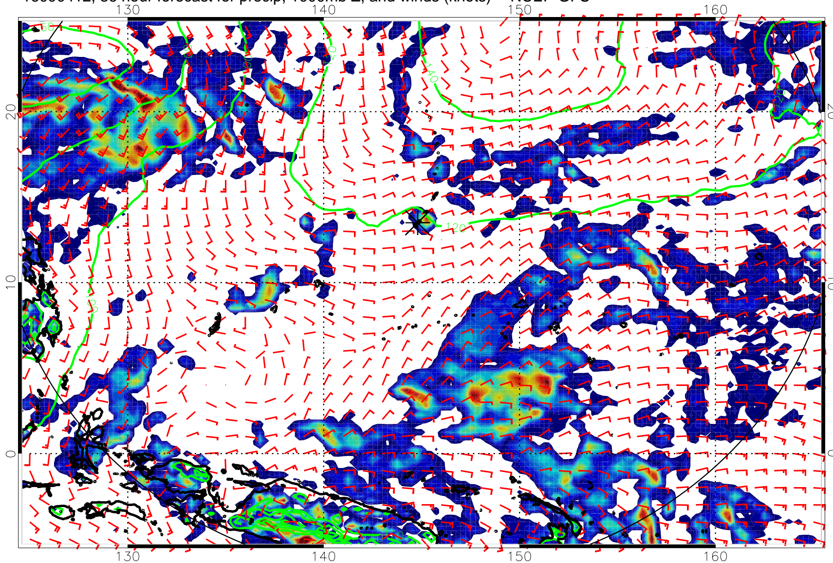
16090412, 36 hour forecast for precip, 1000mb Z, and winds (knots) -- NCEP GFS
