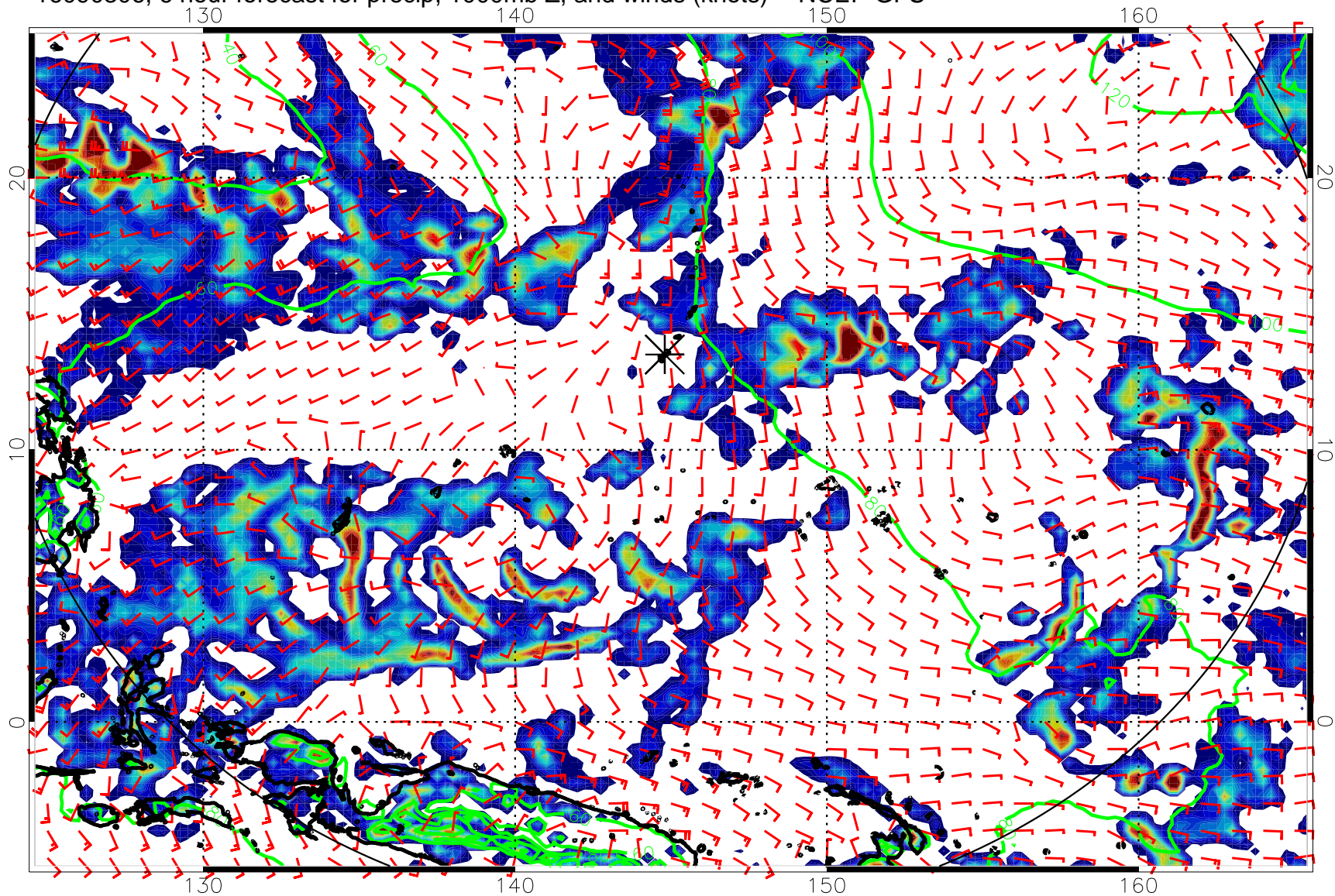
16090306, 6 hour forecast for precip, 1000mb Z, and winds (knots) -- NCEP GFS
