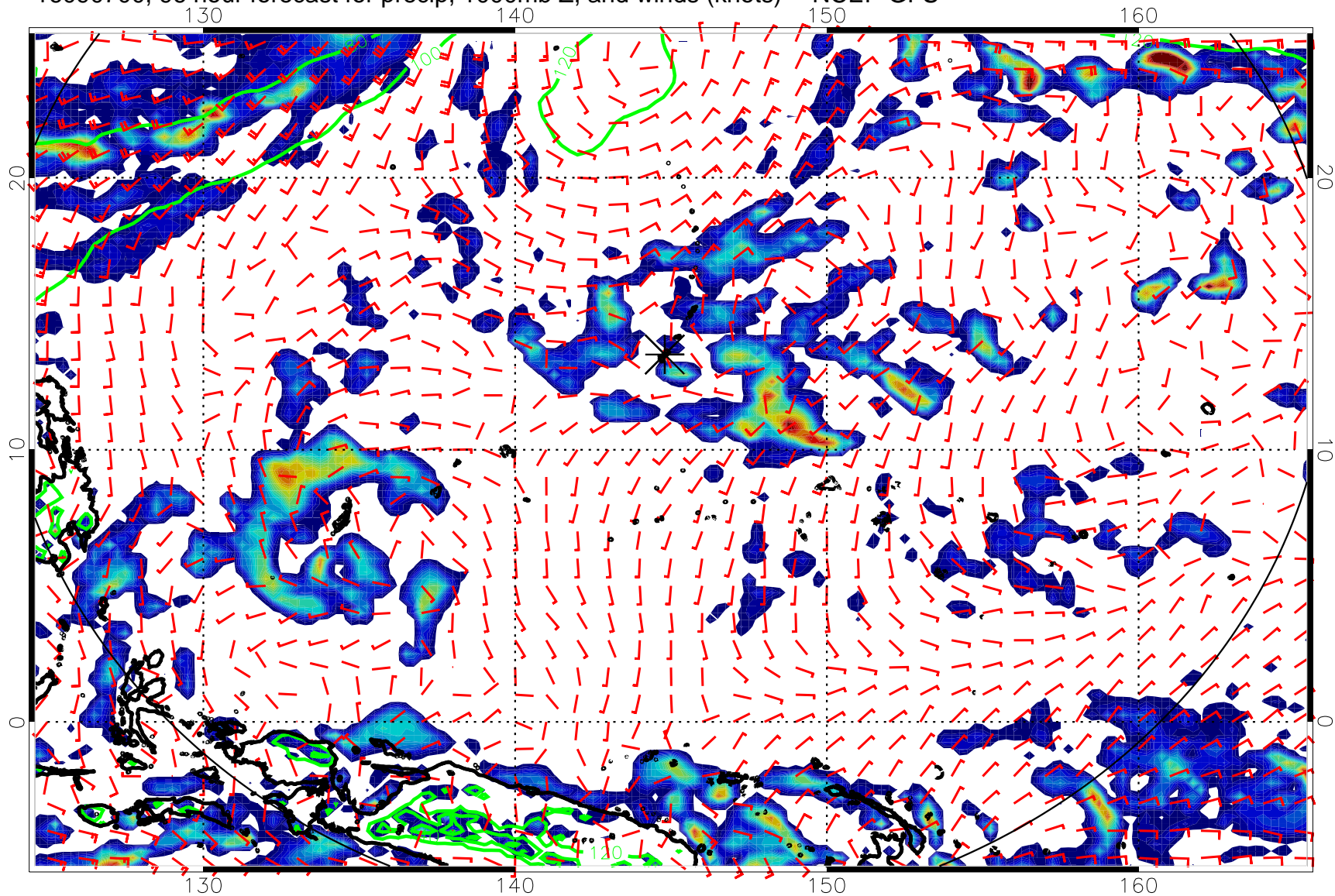
16090700, 96 hour forecast for precip, 1000mb Z, and winds (knots) -- NCEP GFS
