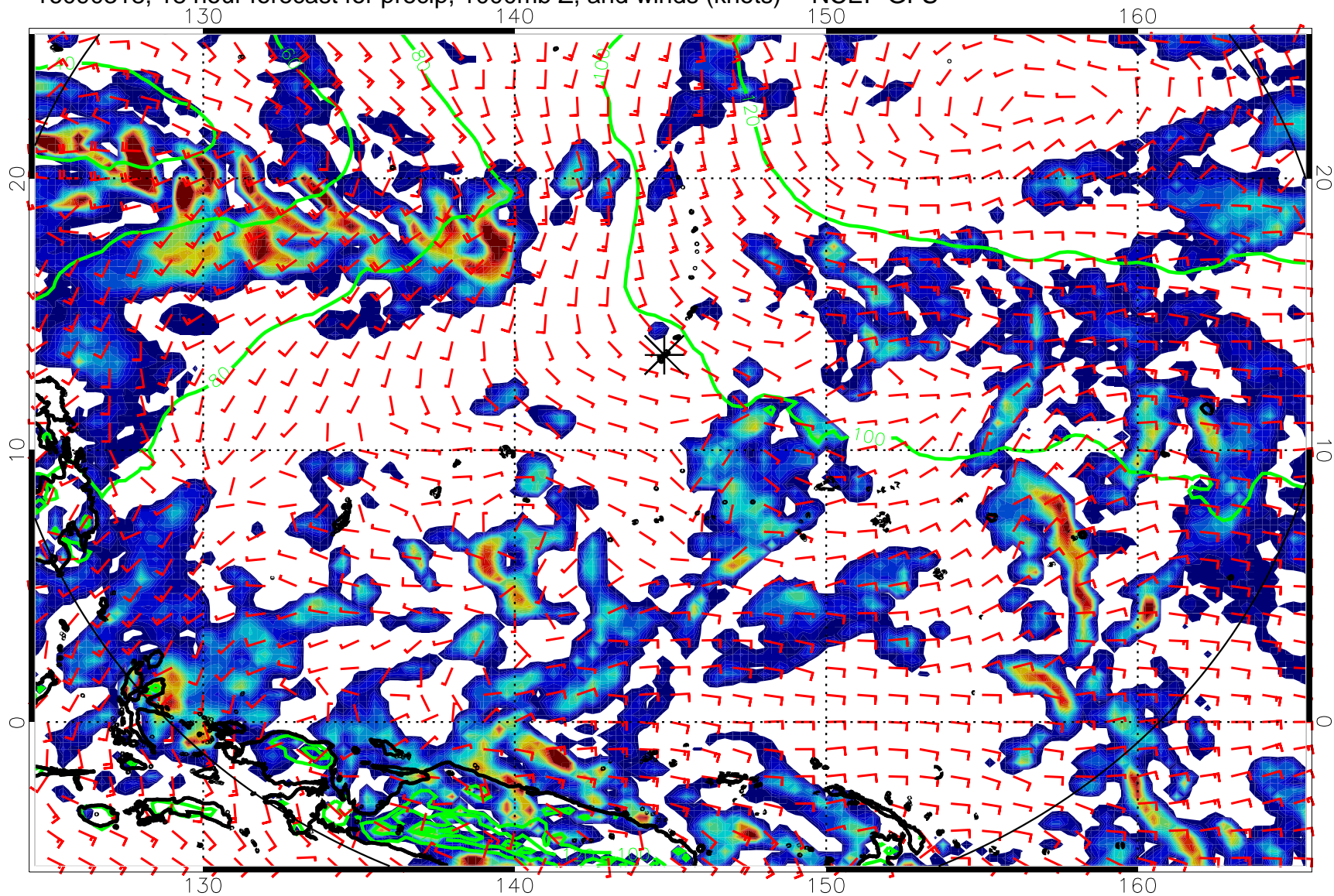
16090318, 18 hour forecast for precip, 1000mb Z, and winds (knots) -- NCEP GFS
