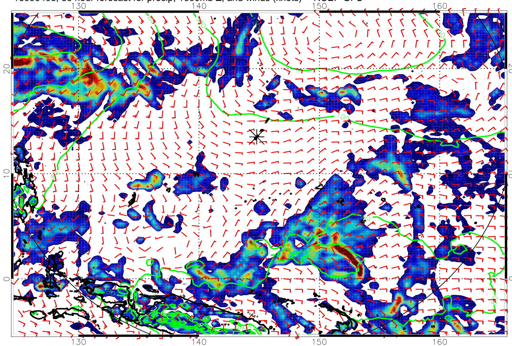
16090406, 30 hour forecast for precip, 1000mb Z, and winds (knots) -- NCEP GFS
