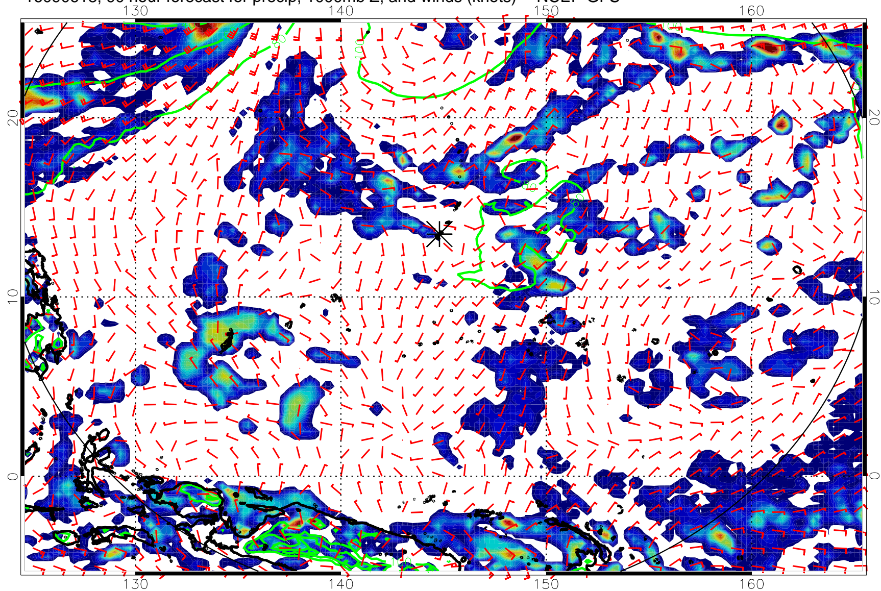
16090618, 90 hour forecast for precip, 1000mb Z, and winds (knots) -- NCEP GFS
