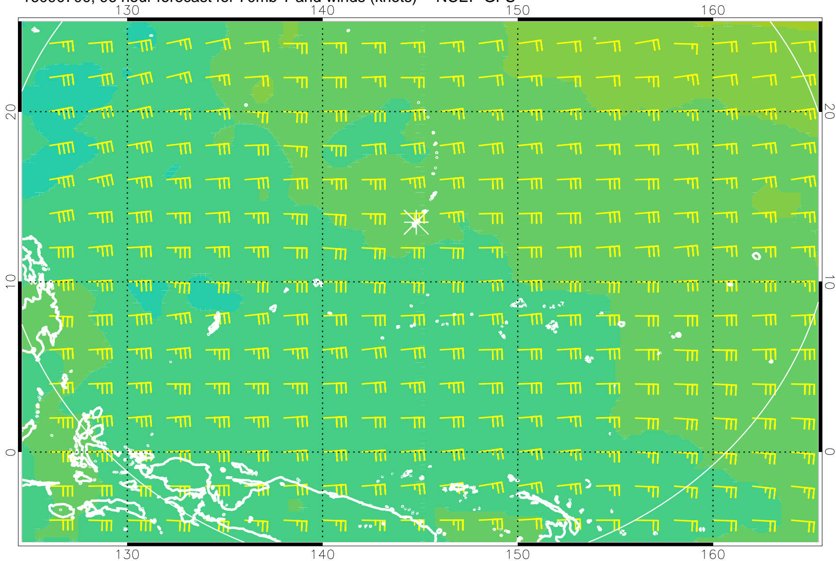
16090700, 96 hour forecast for 70mb T and winds (knots) -- NCEP GFS
