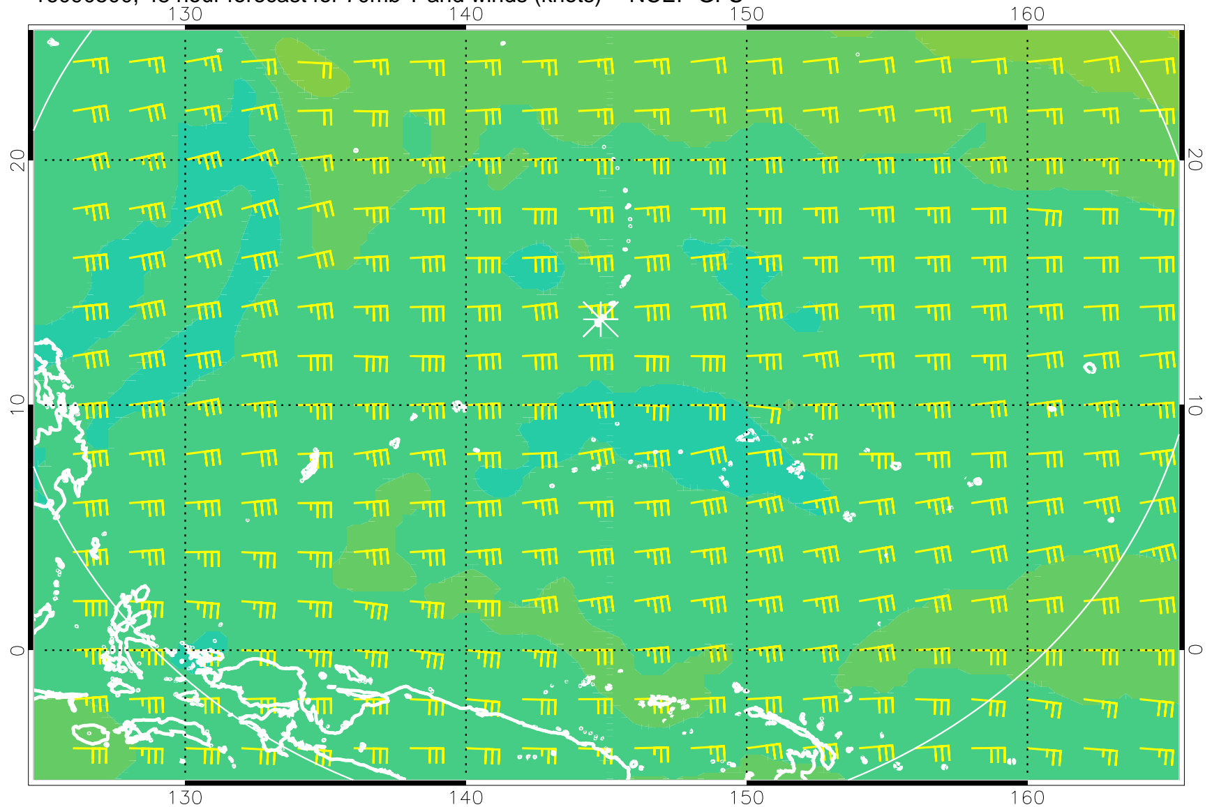
16090500, 48 hour forecast for 70mb T and winds (knots) -- NCEP GFS
