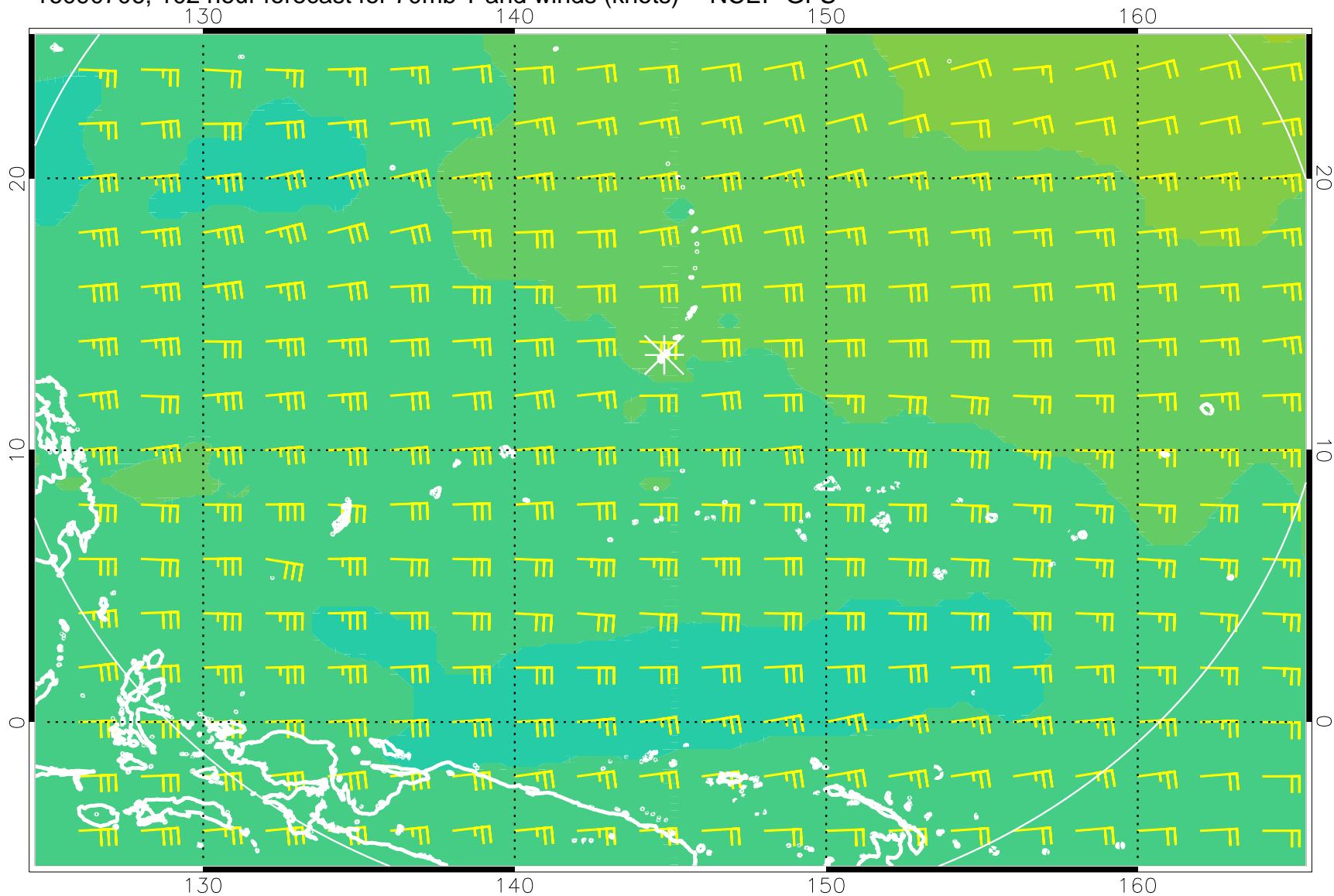
16090706, 102 hour forecast for 70mb T and winds (knots) -- NCEP GFS
