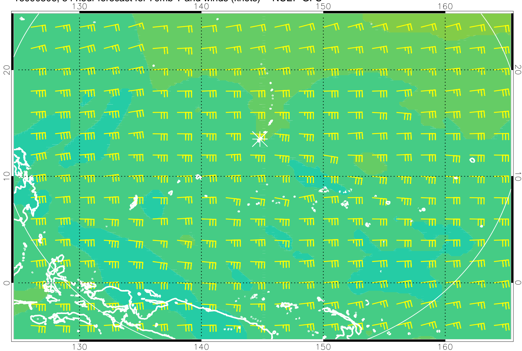
16090506, 54 hour forecast for 70mb T and winds (knots) -- NCEP GFS
