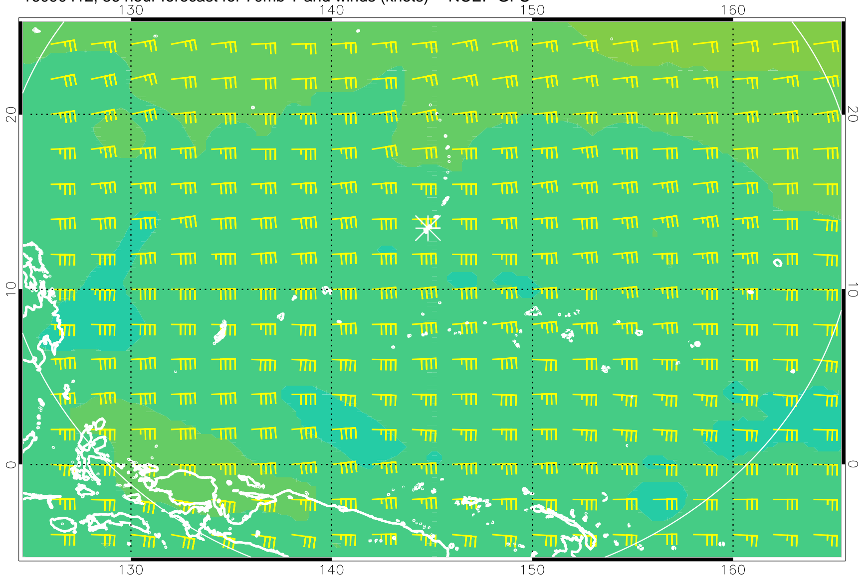
16090412, 36 hour forecast for 70mb T and winds (knots) -- NCEP GFS
