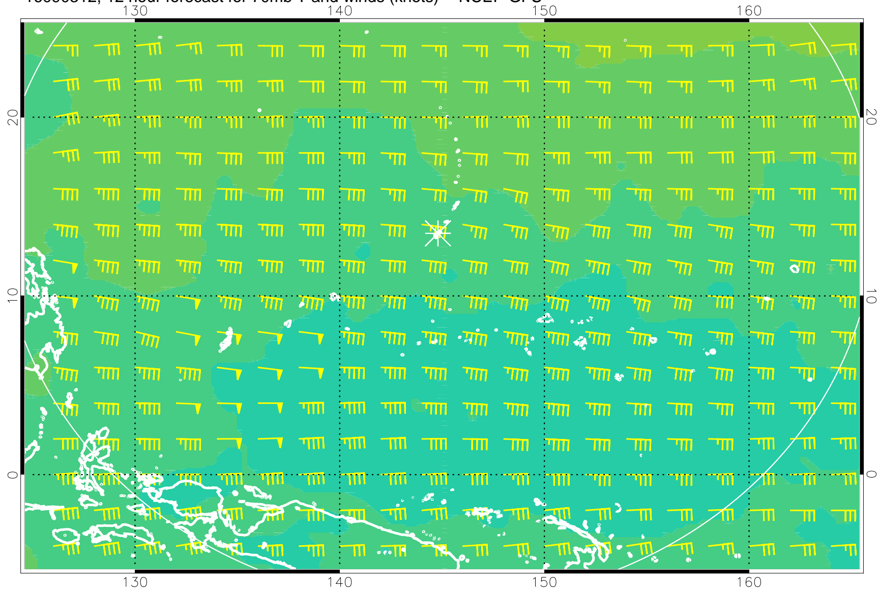
16090312, 12 hour forecast for 70mb T and winds (knots) -- NCEP GFS
