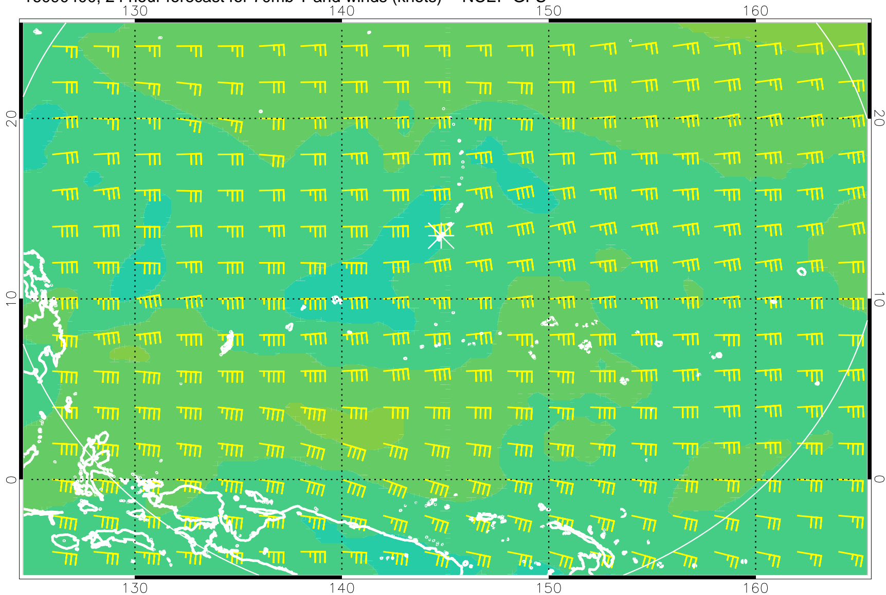
16090400, 24 hour forecast for 70mb T and winds (knots) -- NCEP GFS
