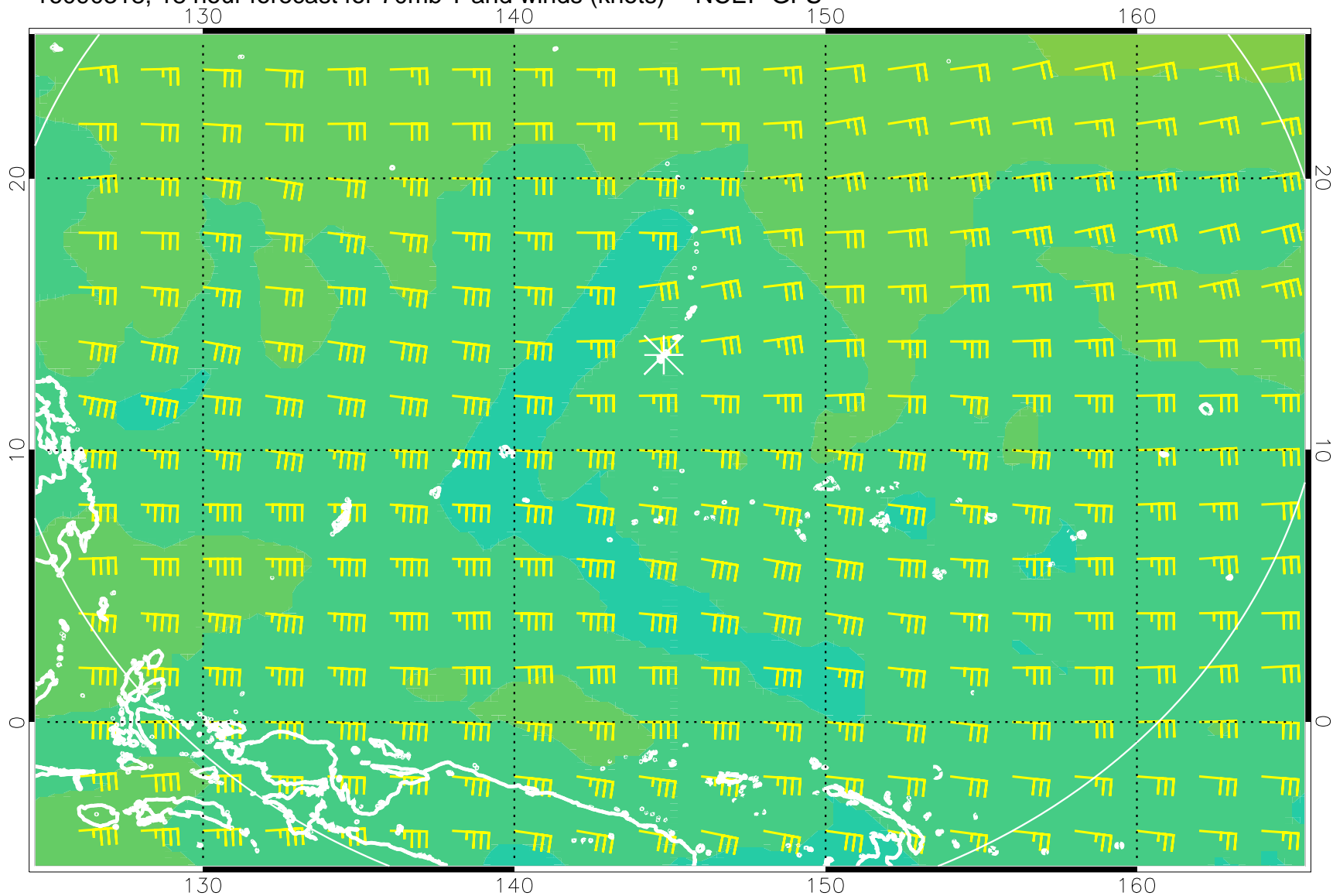
16090318, 18 hour forecast for 70mb T and winds (knots) -- NCEP GFS
