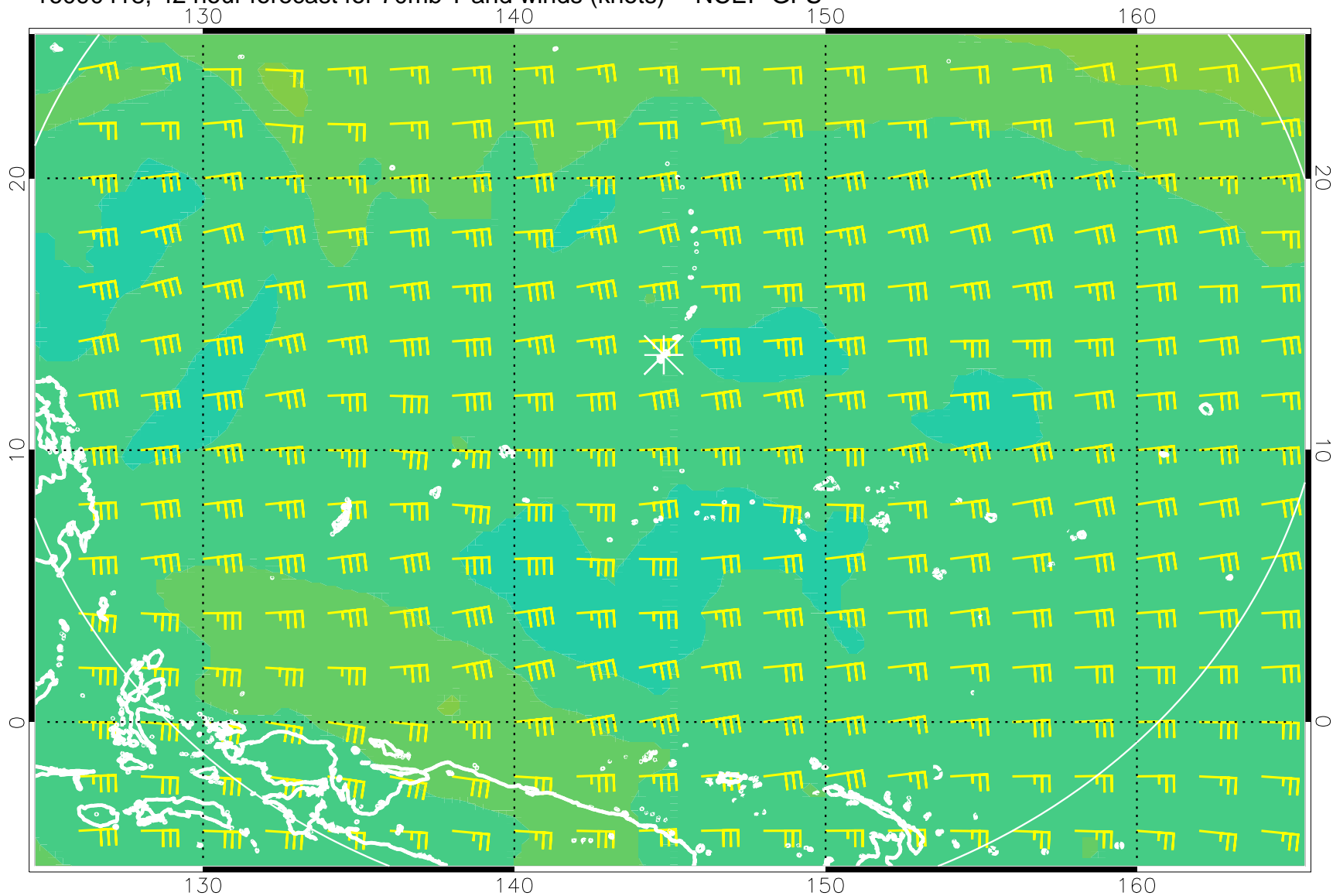
16090418, 42 hour forecast for 70mb T and winds (knots) -- NCEP GFS
