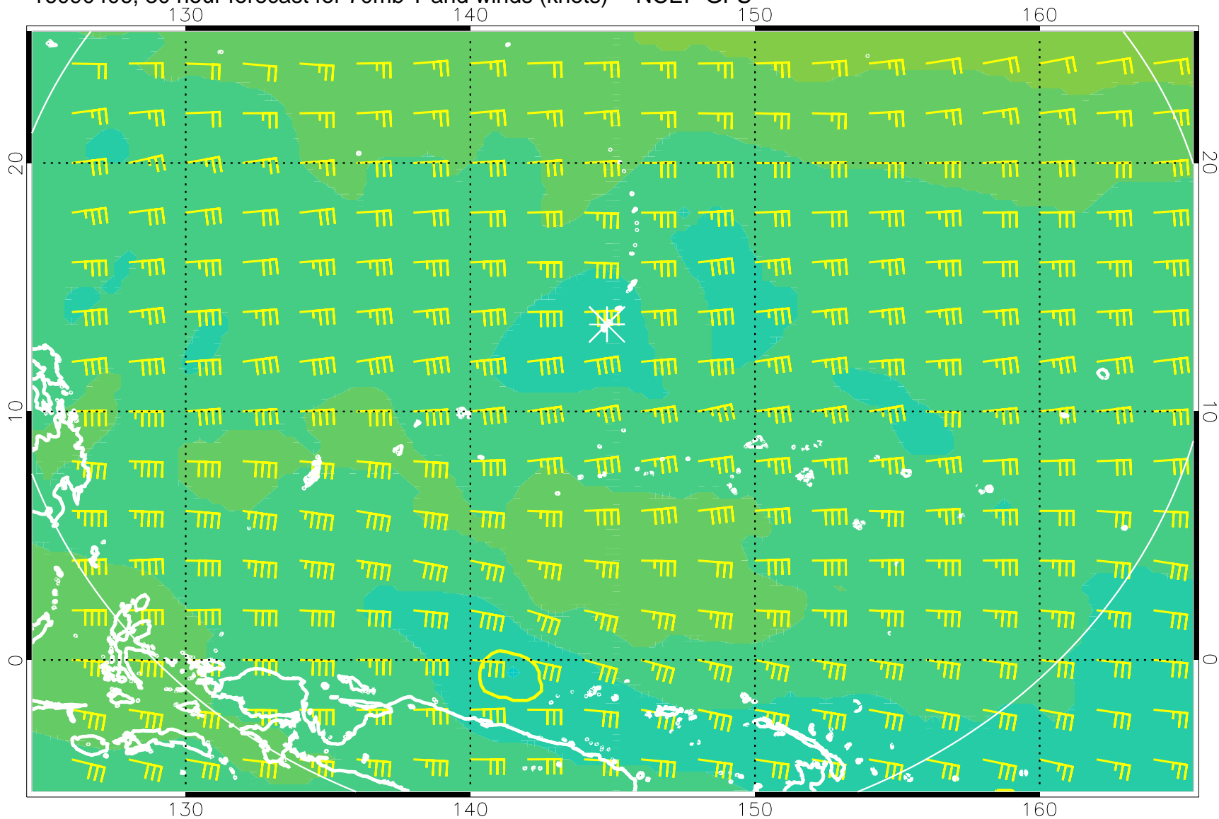
16090406, 30 hour forecast for 70mb T and winds (knots) -- NCEP GFS
