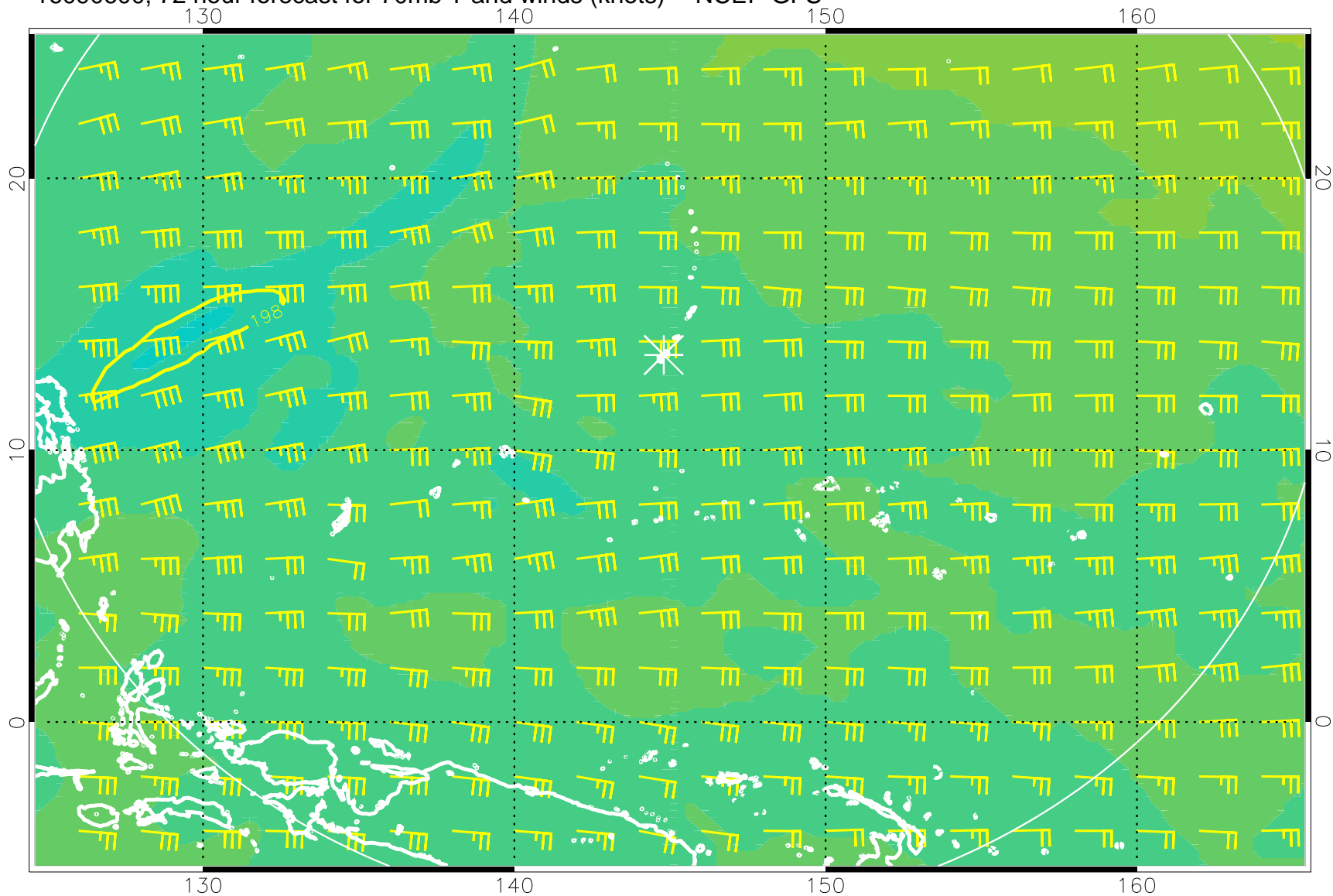
16090600, 72 hour forecast for 70mb T and winds (knots) -- NCEP GFS
