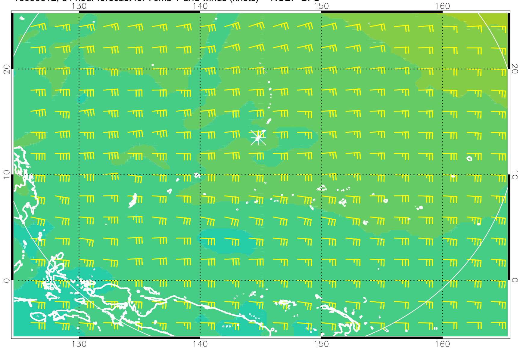
16090612, 84 hour forecast for 70mb T and winds (knots) -- NCEP GFS
