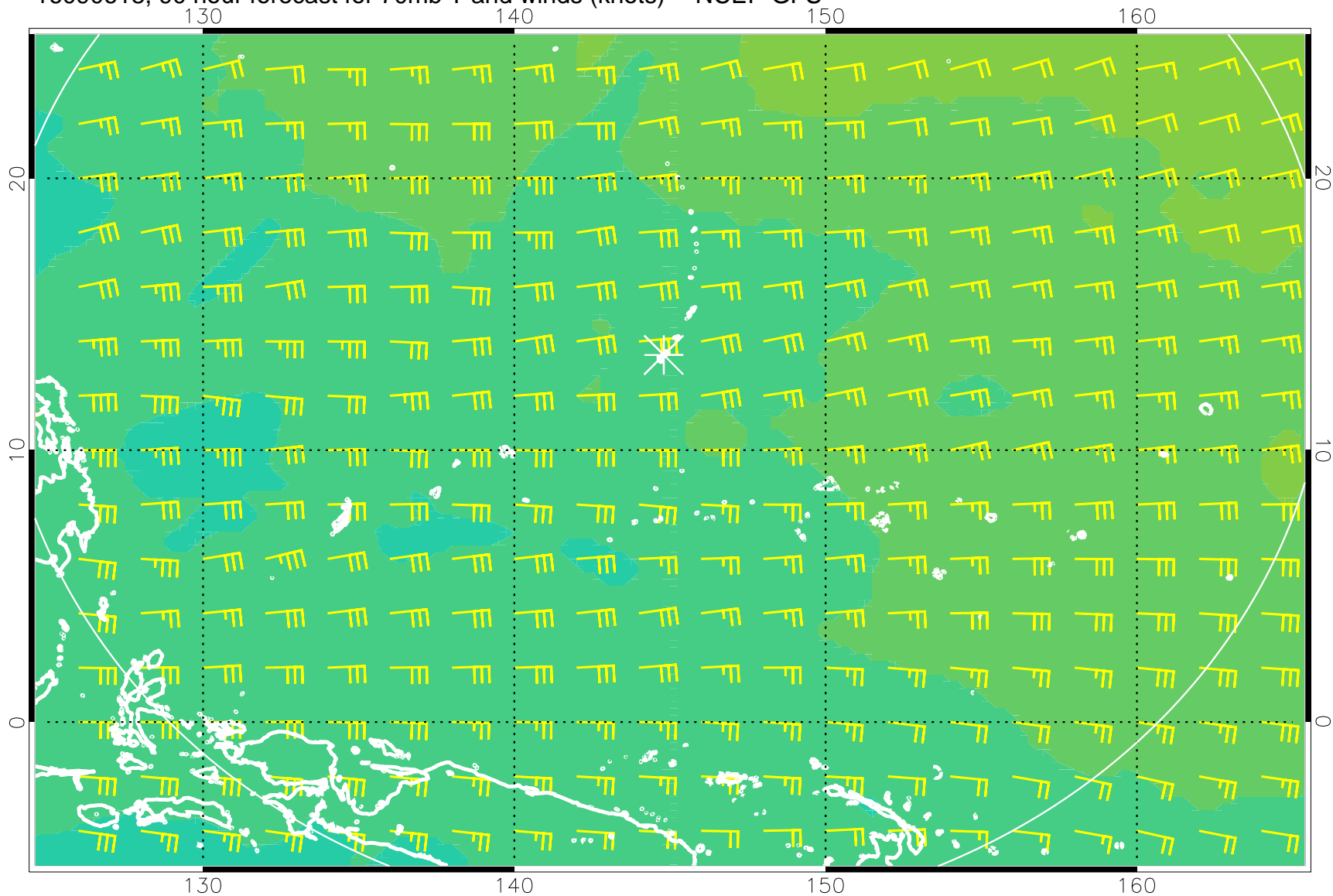
16090618, 90 hour forecast for 70mb T and winds (knots) -- NCEP GFS
