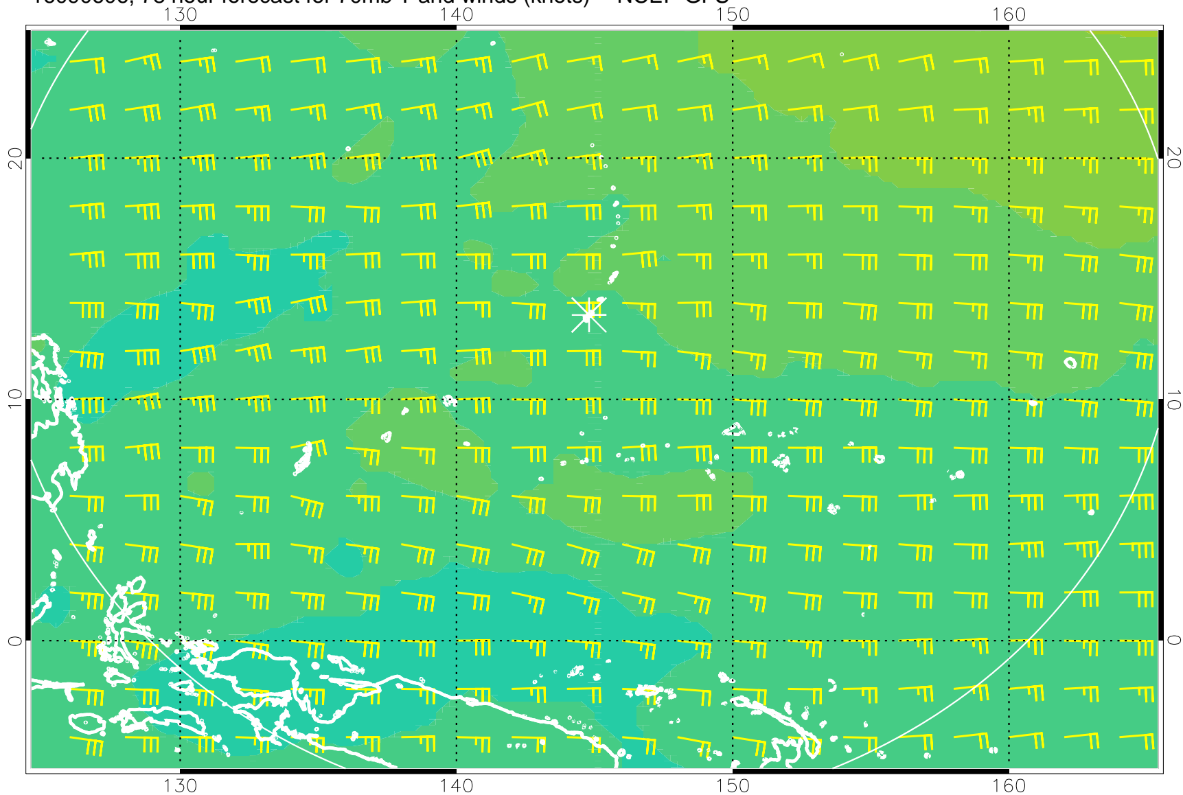
16090606, 78 hour forecast for 70mb T and winds (knots) -- NCEP GFS
