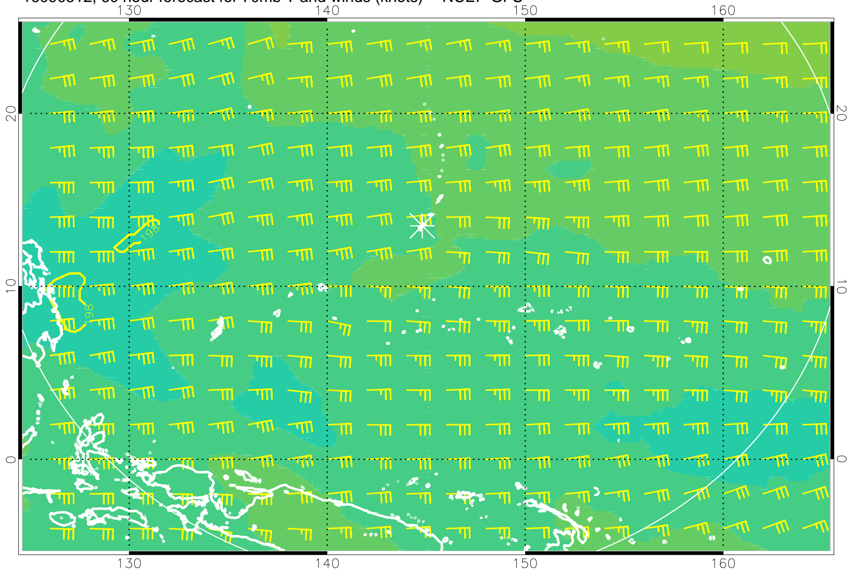
16090512, 60 hour forecast for 70mb T and winds (knots) -- NCEP GFS
