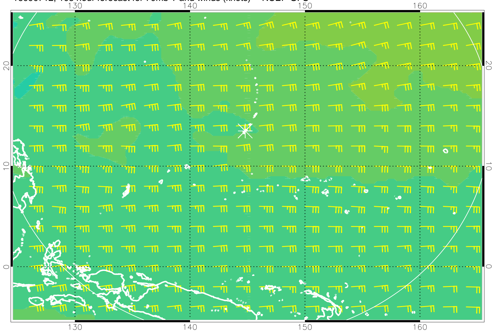
16090712, 108 hour forecast for 70mb T and winds (knots) -- NCEP GFS
