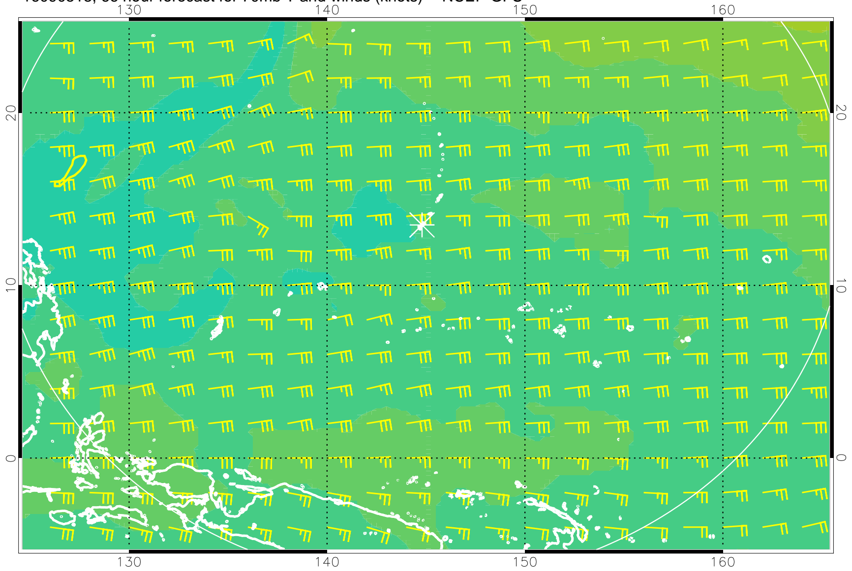
16090518, 66 hour forecast for 70mb T and winds (knots) -- NCEP GFS
