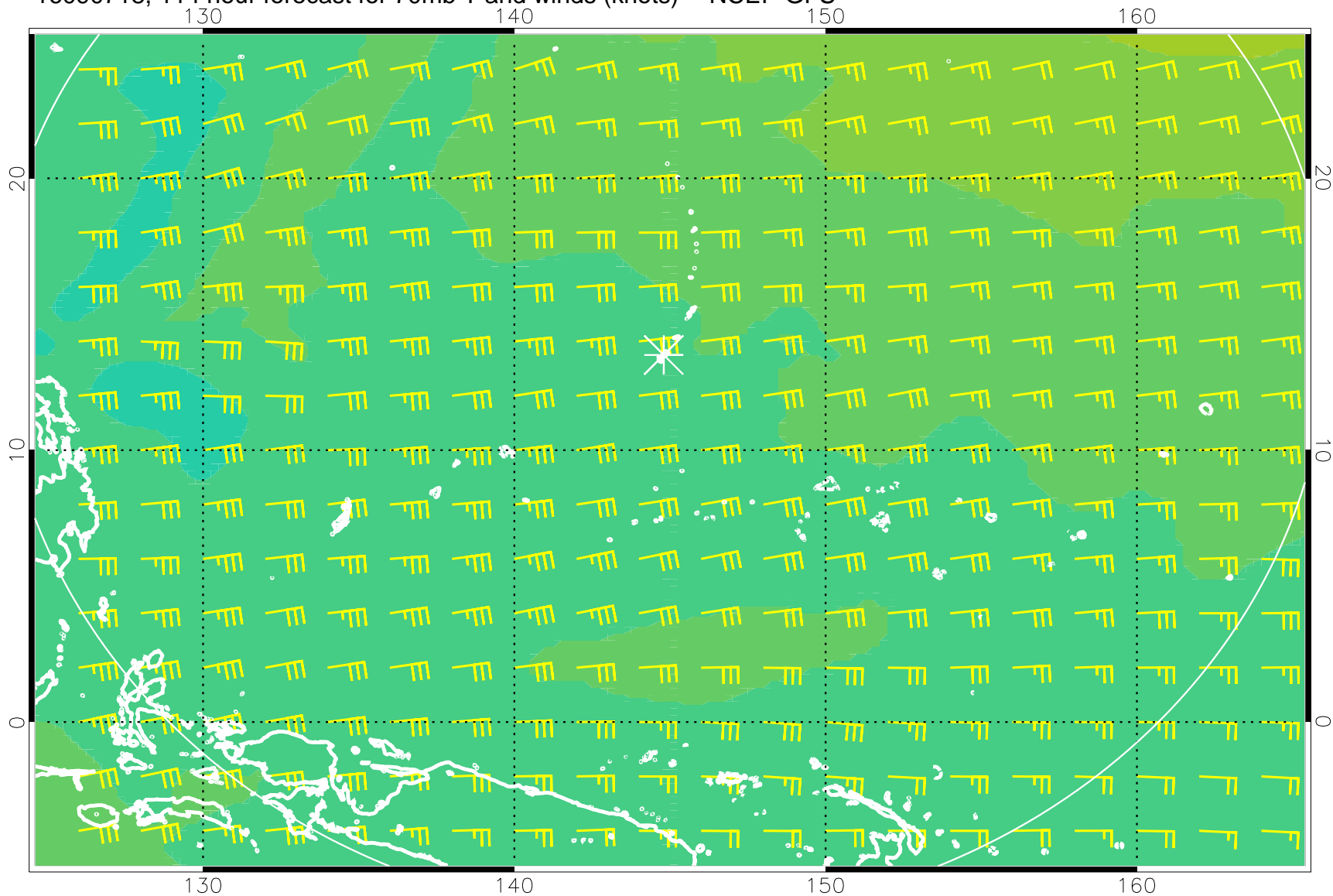
16090718, 114 hour forecast for 70mb T and winds (knots) -- NCEP GFS
