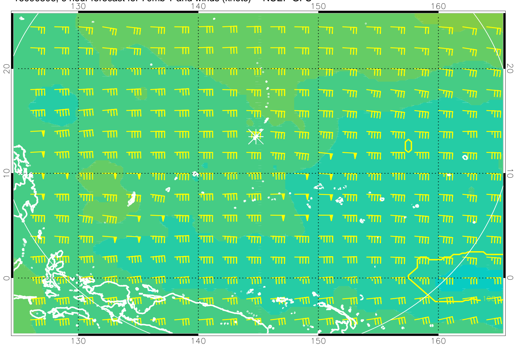
16090306, 6 hour forecast for 70mb T and winds (knots) -- NCEP GFS
