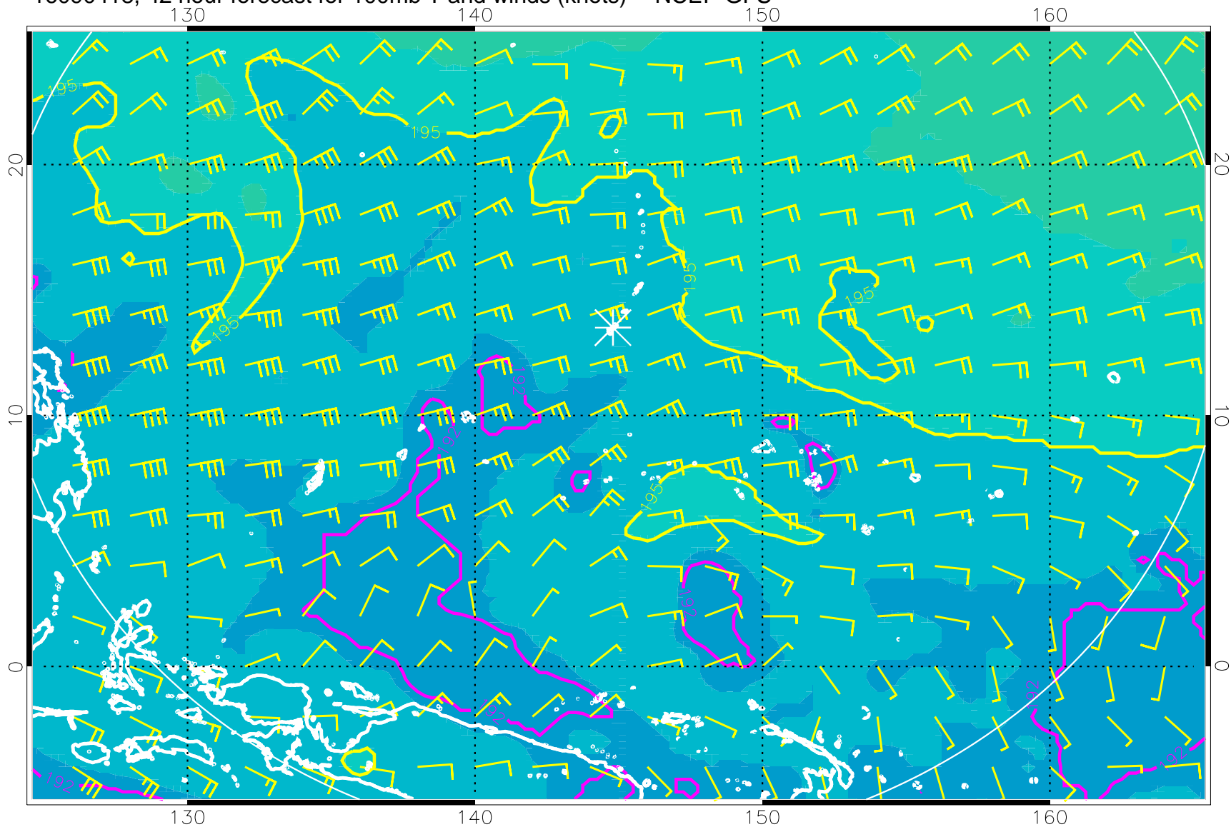
16090418, 42 hour forecast for 100mb T and winds (knots) -- NCEP GFS
