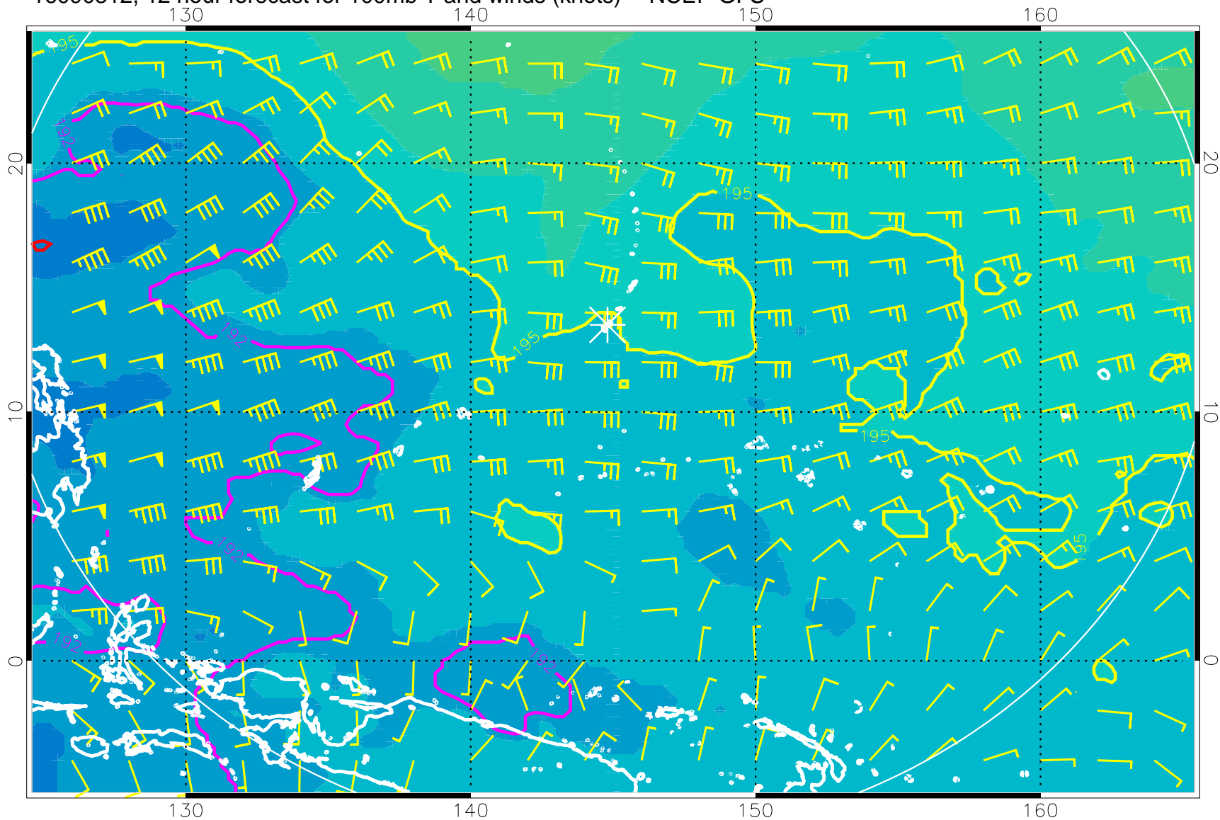
16090312, 12 hour forecast for 100mb T and winds (knots) -- NCEP GFS
