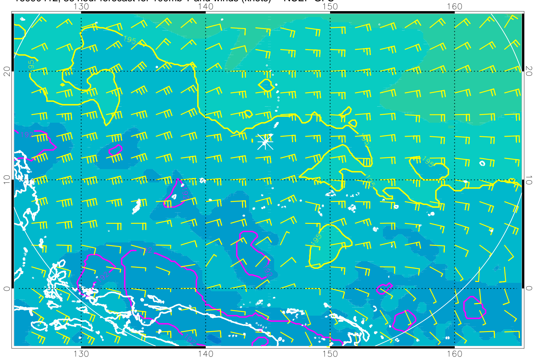
16090412, 36 hour forecast for 100mb T and winds (knots) -- NCEP GFS
