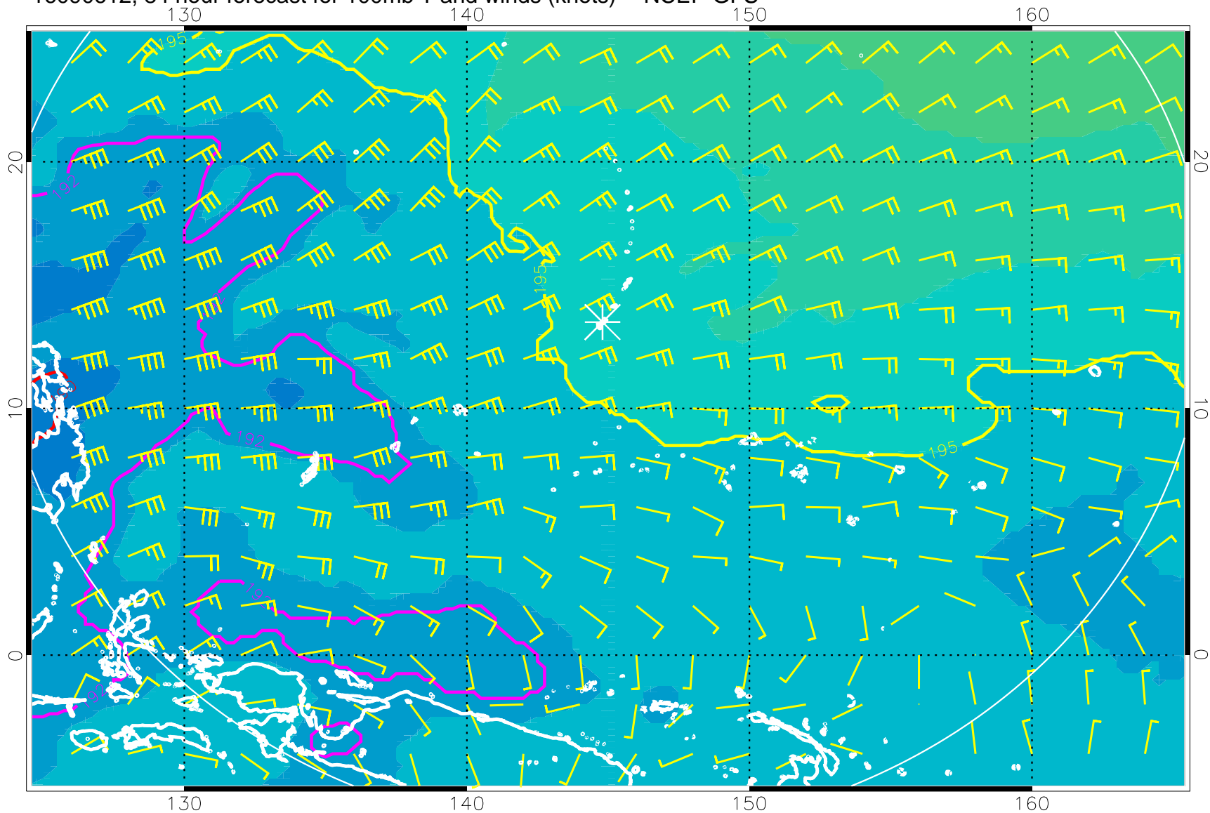
16090612, 84 hour forecast for 100mb T and winds (knots) -- NCEP GFS
