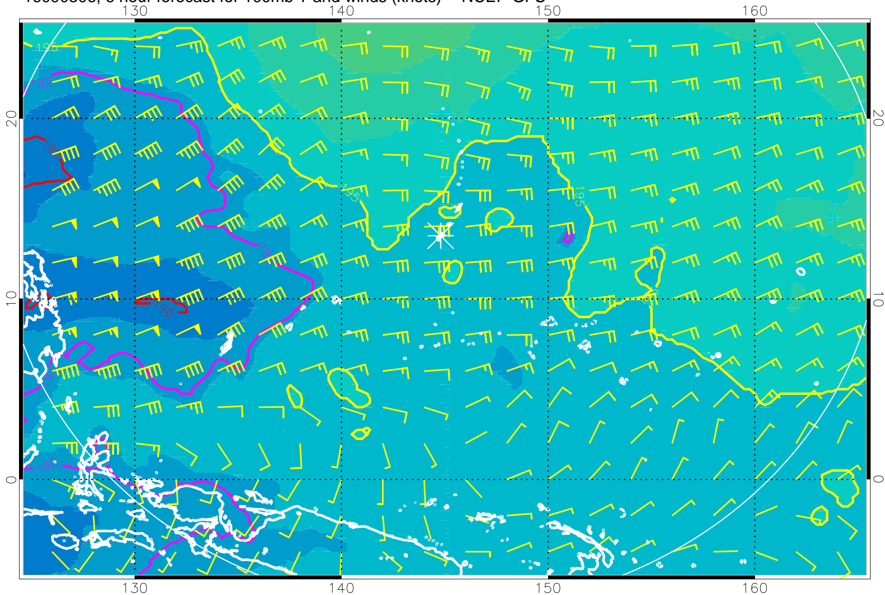
16090306, 6 hour forecast for 100mb T and winds (knots) -- NCEP GFS
