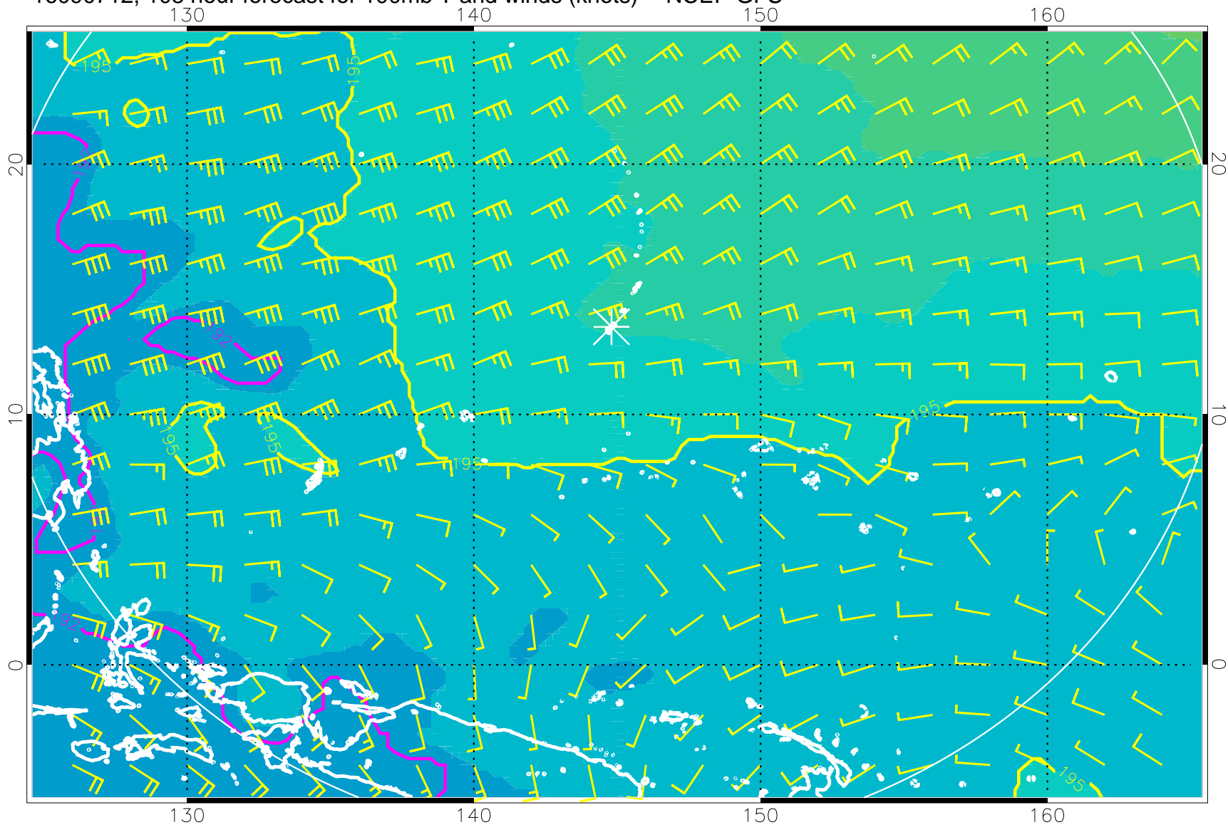
16090712, 108 hour forecast for 100mb T and winds (knots) -- NCEP GFS
