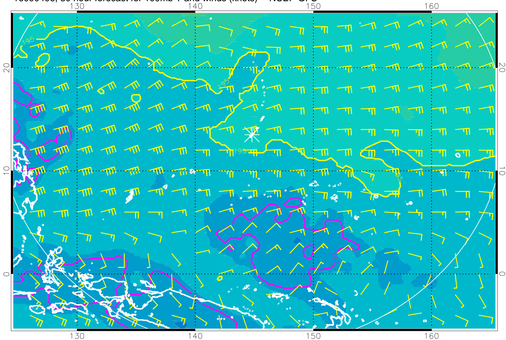
16090406, 30 hour forecast for 100mb T and winds (knots) -- NCEP GFS
