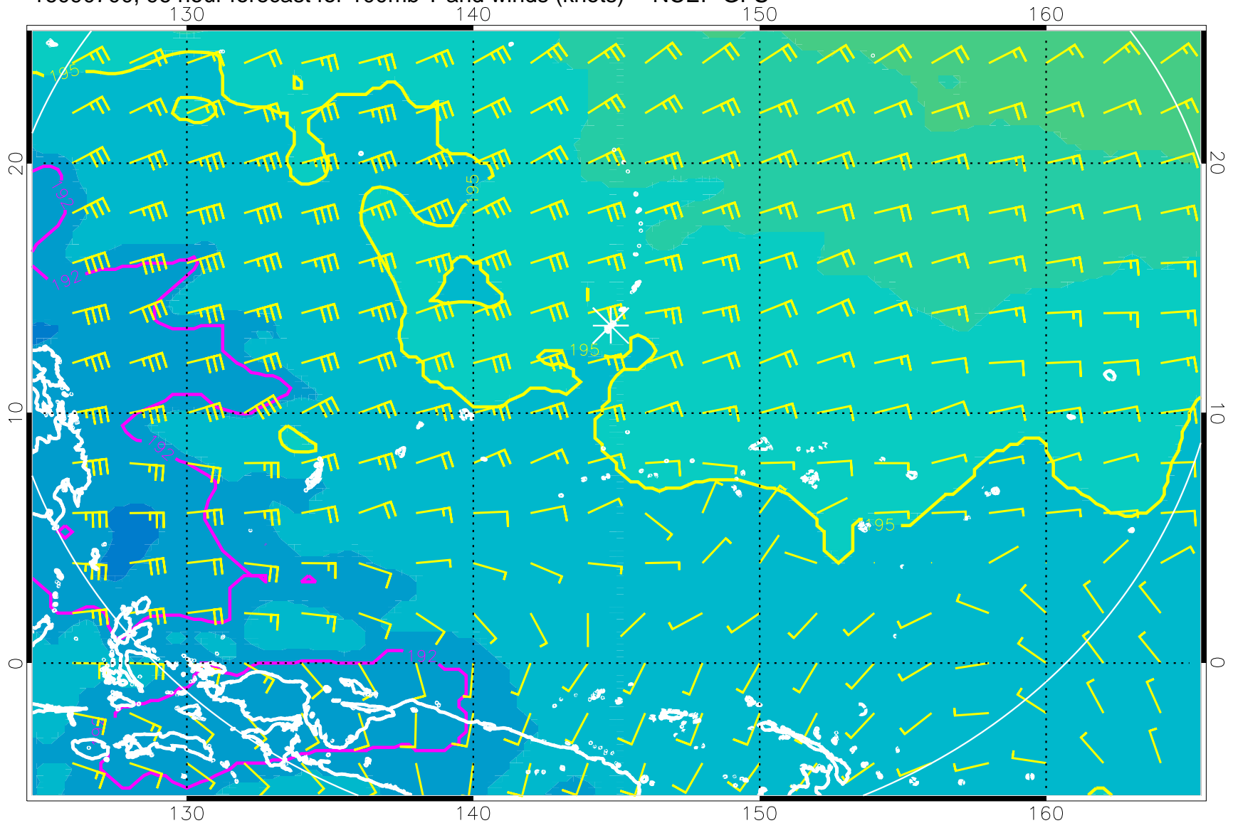
16090700, 96 hour forecast for 100mb T and winds (knots) -- NCEP GFS
