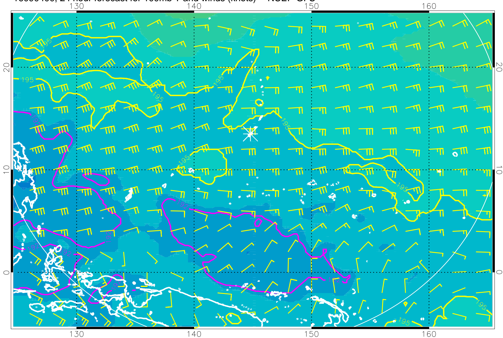
16090400, 24 hour forecast for 100mb T and winds (knots) -- NCEP GFS
