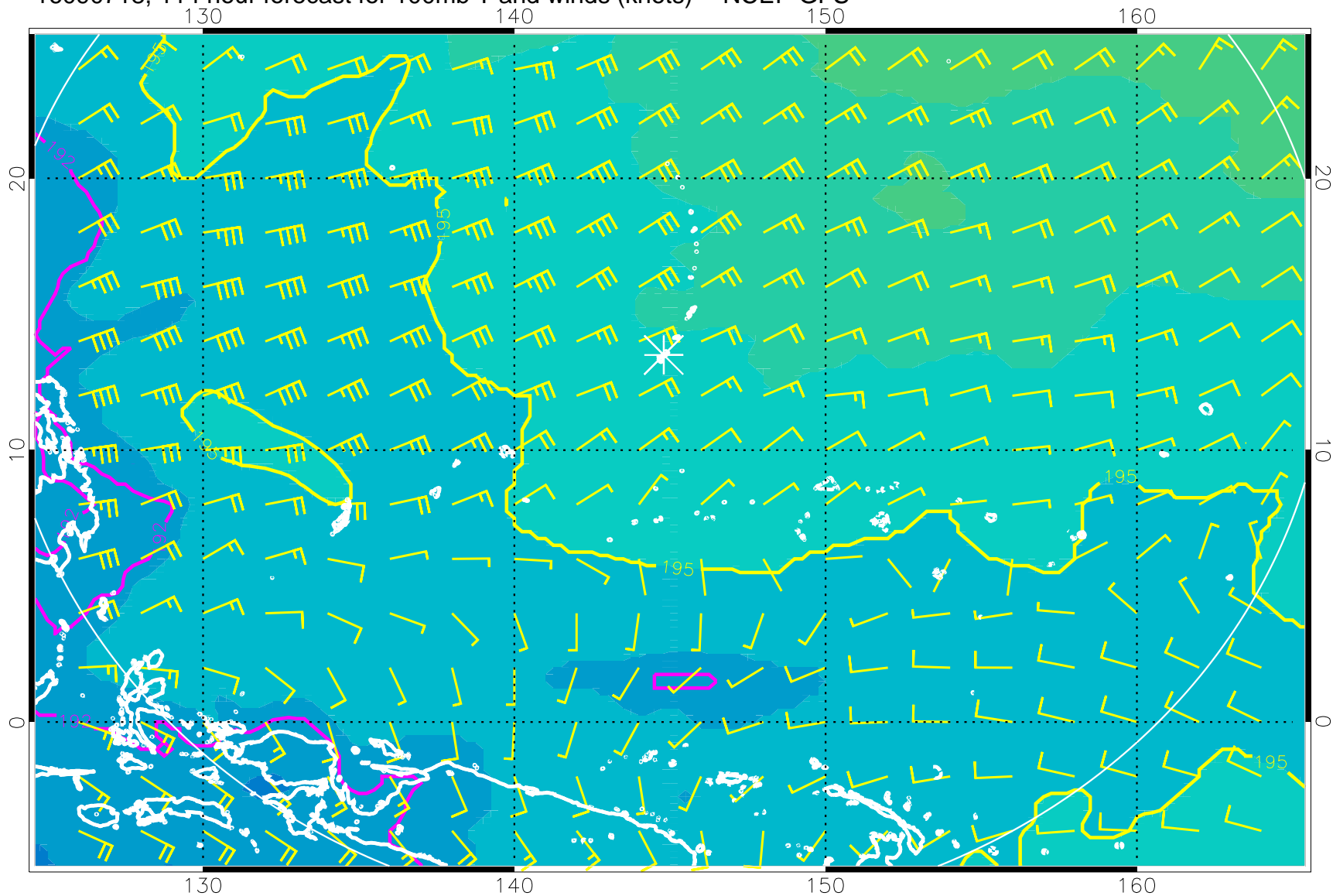
16090718, 114 hour forecast for 100mb T and winds (knots) -- NCEP GFS
