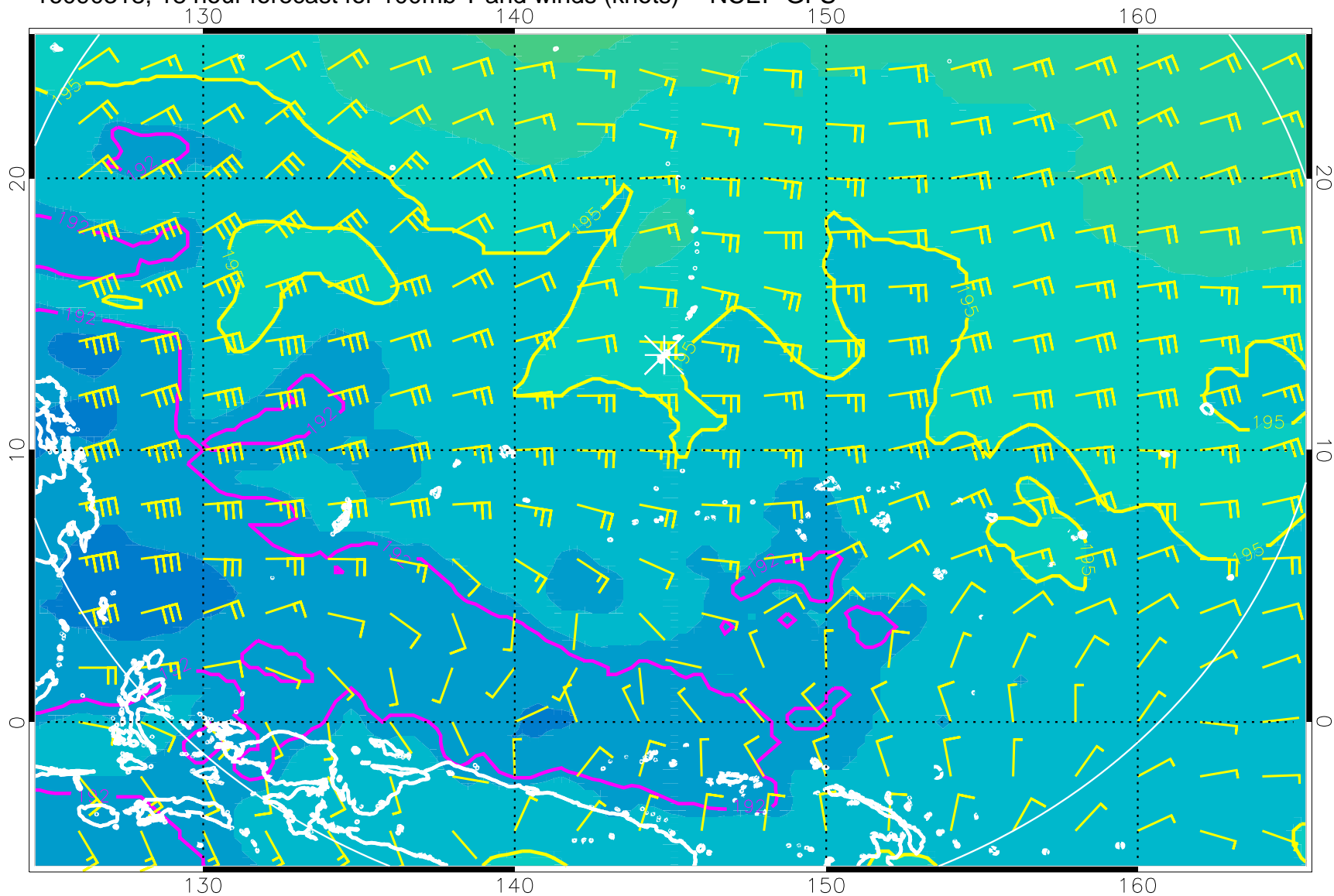
16090318, 18 hour forecast for 100mb T and winds (knots) -- NCEP GFS
