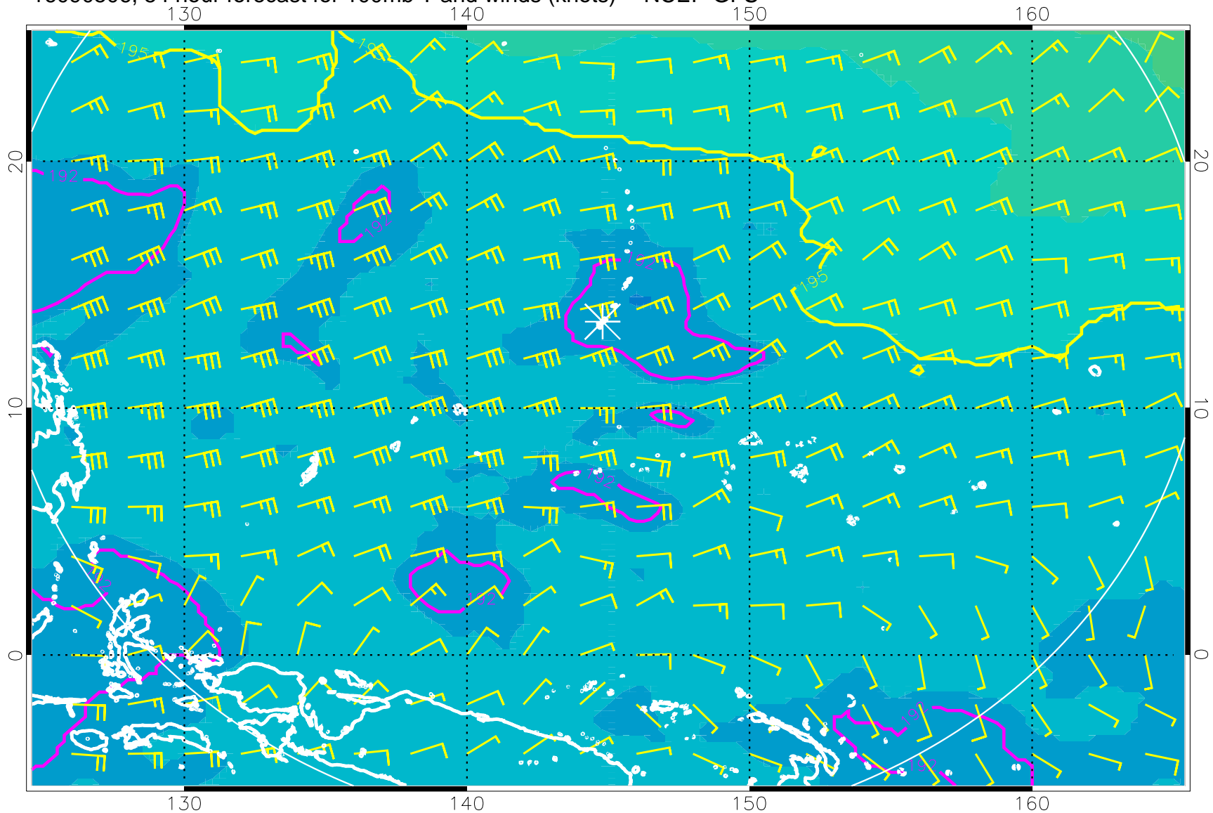
16090506, 54 hour forecast for 100mb T and winds (knots) -- NCEP GFS
