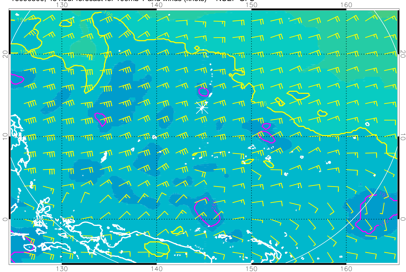
16090500, 48 hour forecast for 100mb T and winds (knots) -- NCEP GFS
