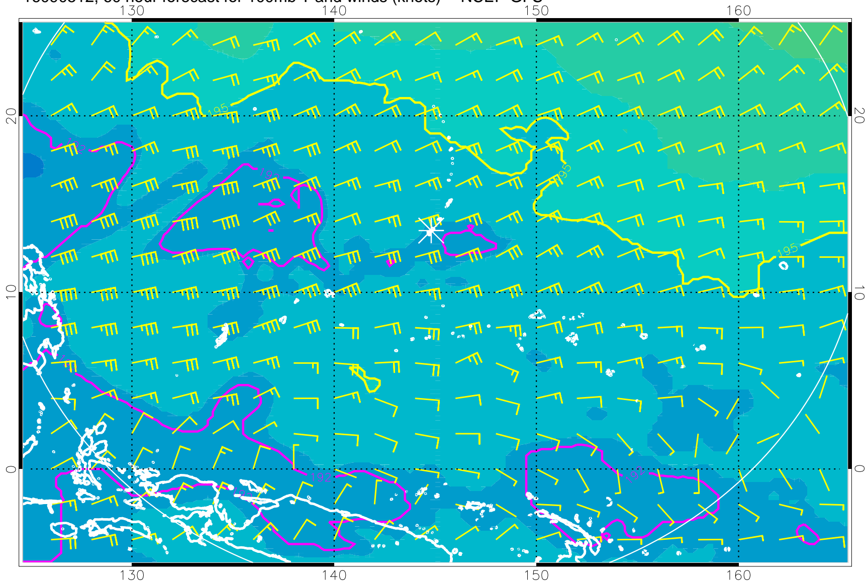
16090512, 60 hour forecast for 100mb T and winds (knots) -- NCEP GFS
