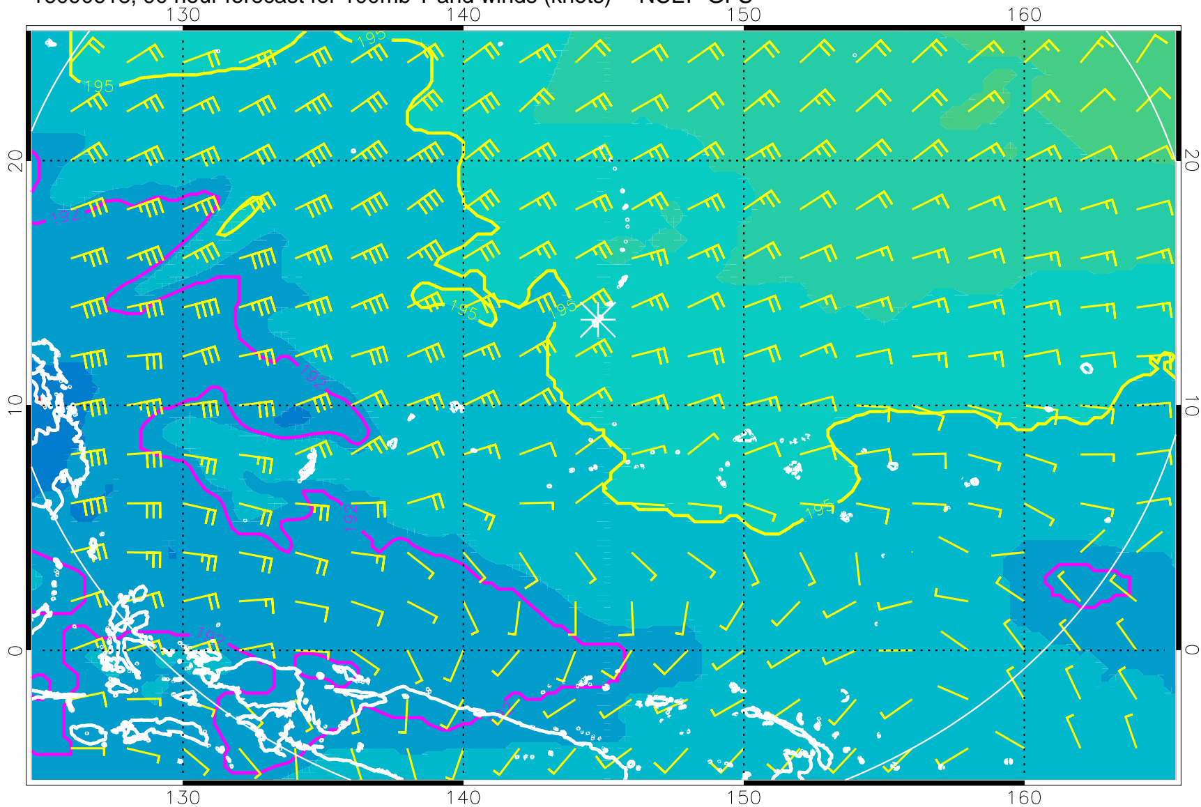
16090618, 90 hour forecast for 100mb T and winds (knots) -- NCEP GFS
