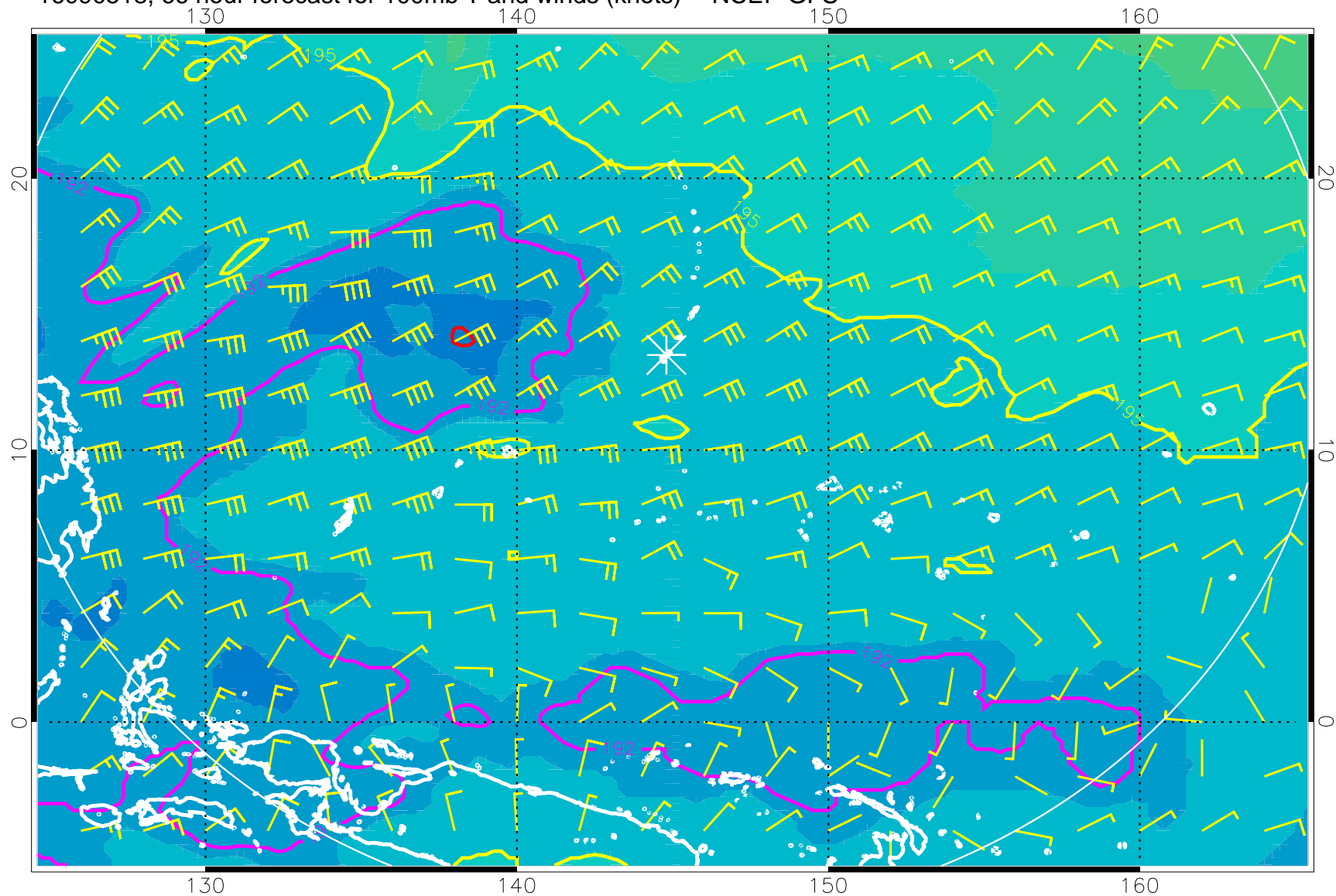
16090518, 66 hour forecast for 100mb T and winds (knots) -- NCEP GFS
