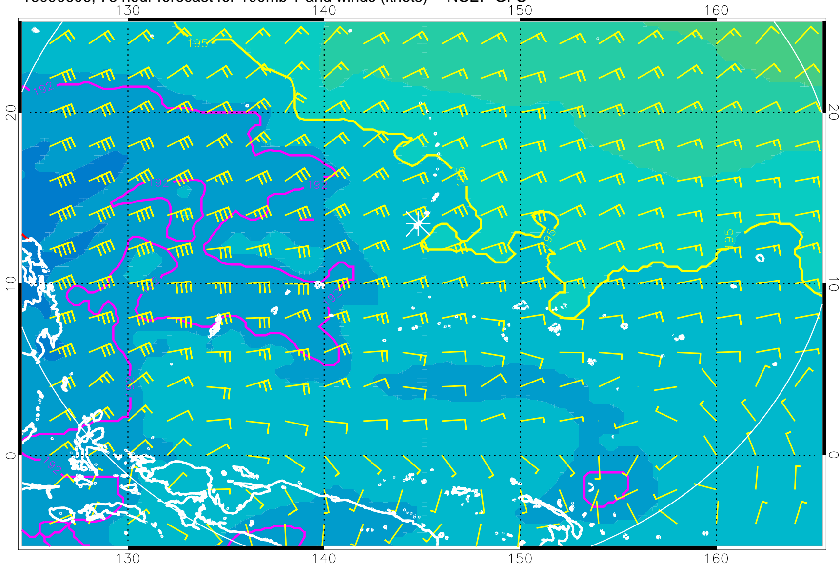
16090606, 78 hour forecast for 100mb T and winds (knots) -- NCEP GFS
