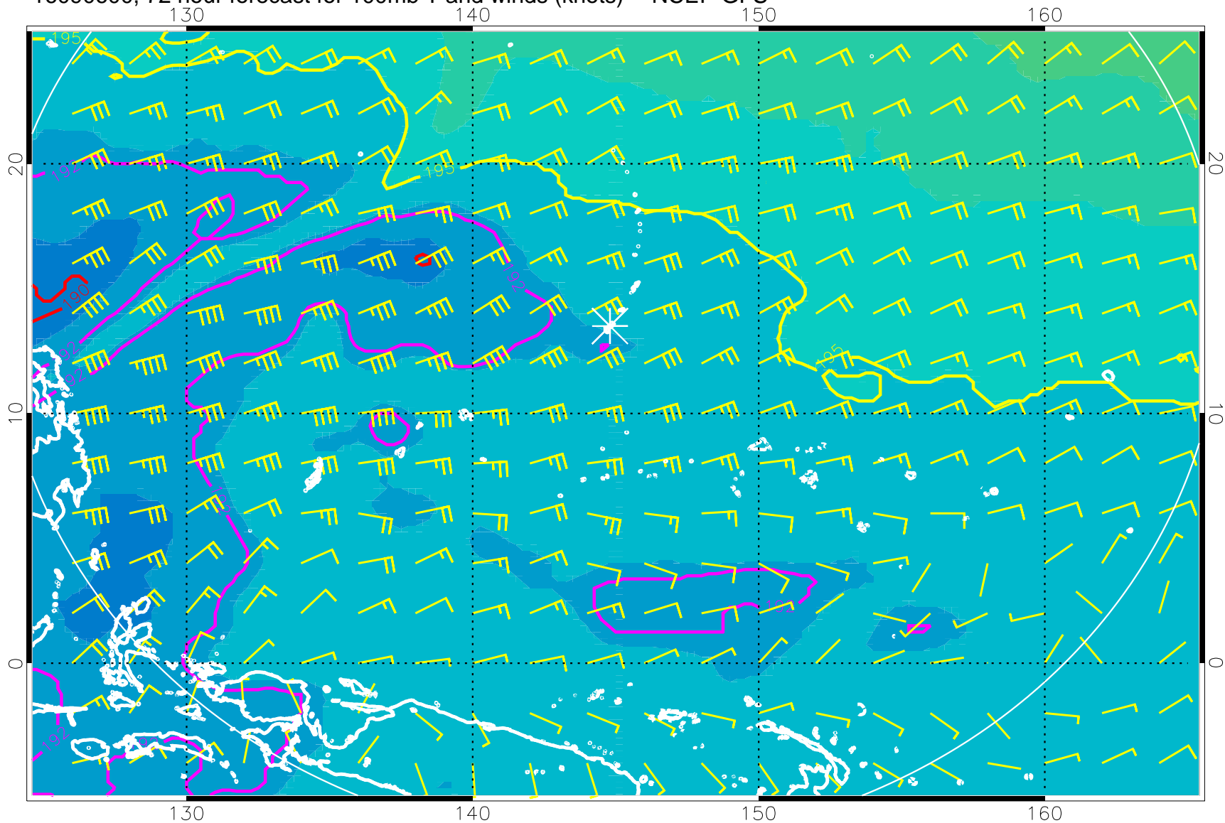
16090600, 72 hour forecast for 100mb T and winds (knots) -- NCEP GFS
