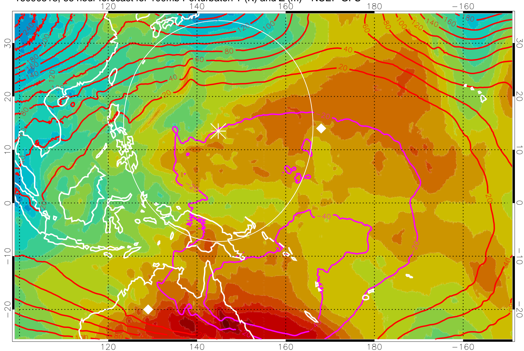
16090518, 66 hour forecast for 100mb Perturbaton T (K) and Z (m)-- NCEP GFS
