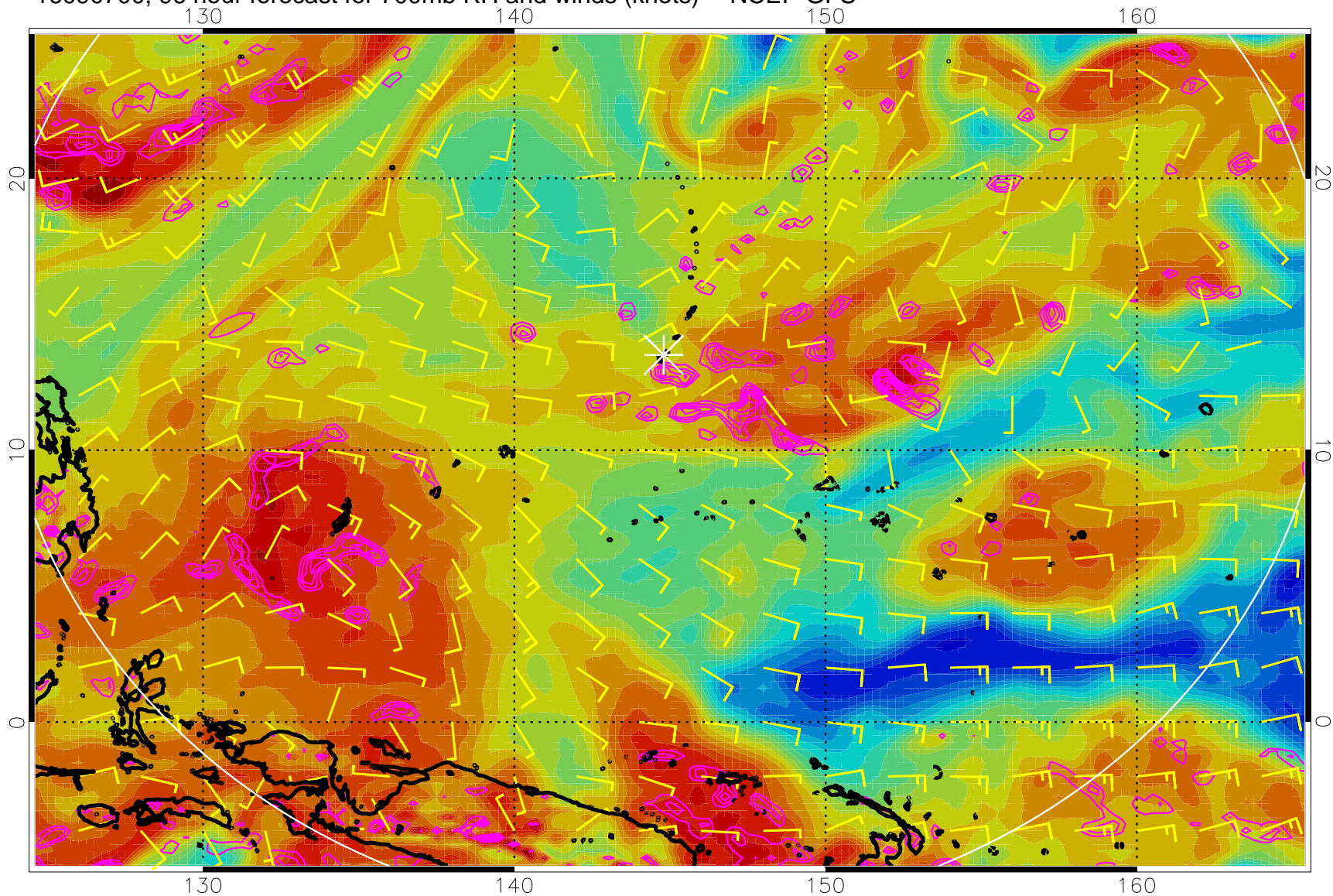
16090700, 96 hour forecast for 700mb RH and winds (knots) -- NCEP GFS
