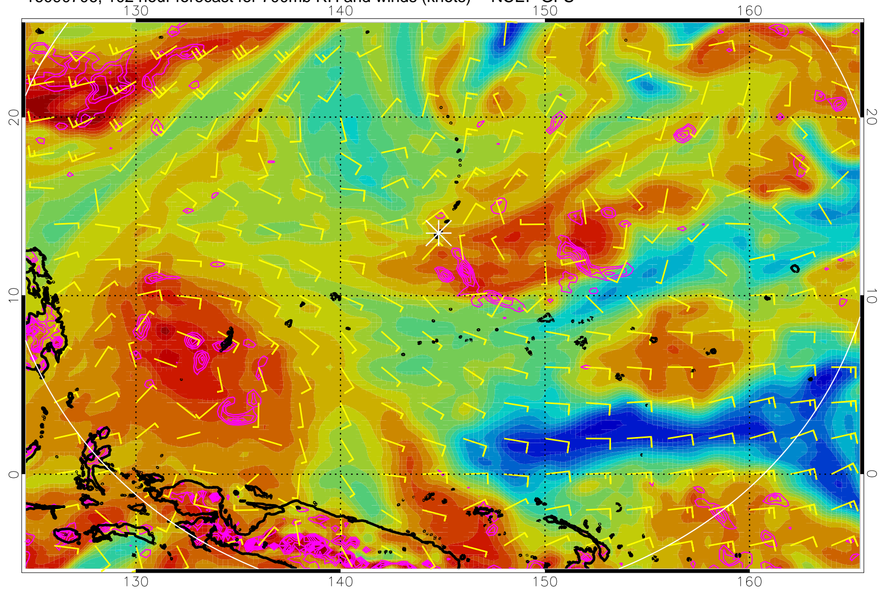
16090706, 102 hour forecast for 700mb RH and winds (knots) -- NCEP GFS
