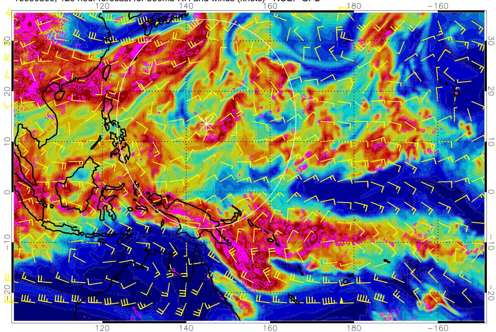
16090800, 120 hour forecast for 500mb RH and winds (knots) - NCEP GFS
