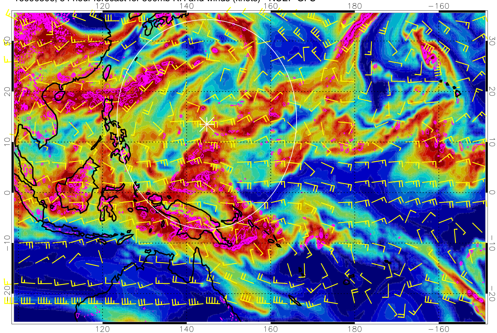
16090506, 54 hour forecast for 500mb RH and winds (knots) - NCEP GFS
