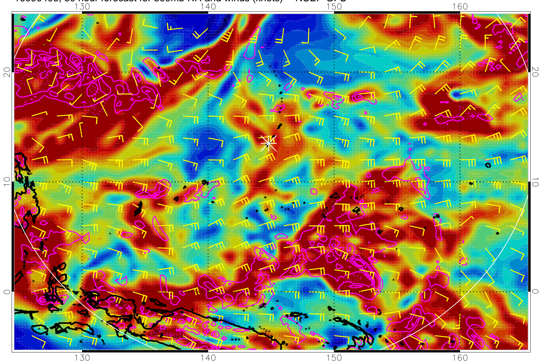
16090406, 30 hour forecast for 300mb RH and winds (knots) -- NCEP GFS
