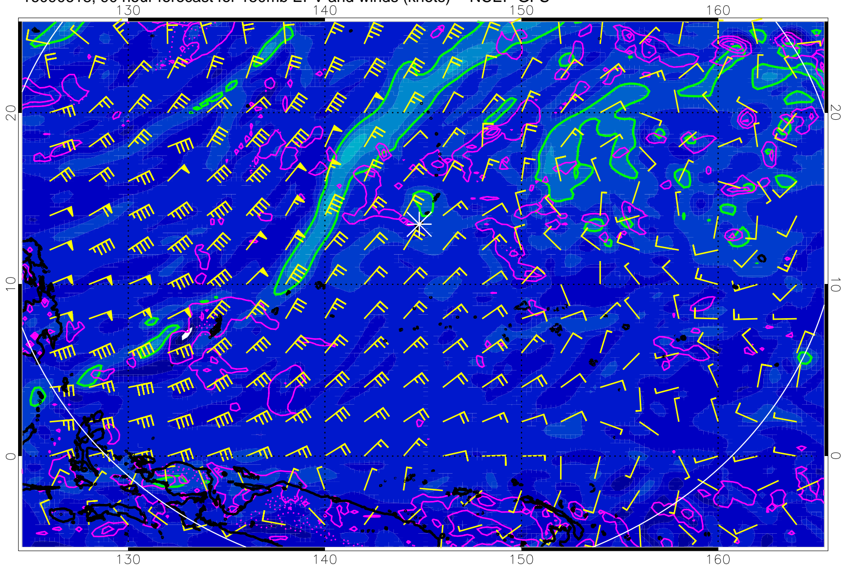
16090618, 90 hour forecast for 150mb EPV and winds (knots) -- NCEP GFS
