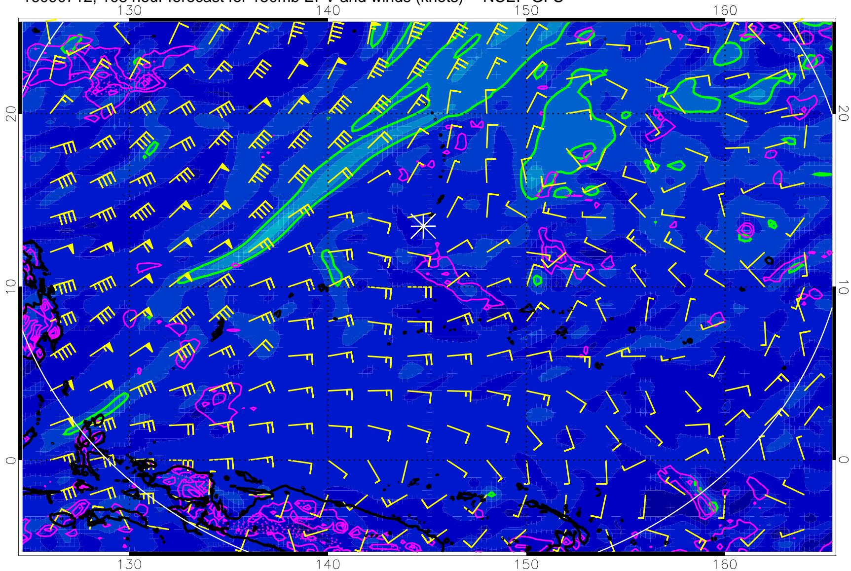
16090712, 108 hour forecast for 150mb EPV and winds (knots) -- NCEP GFS
