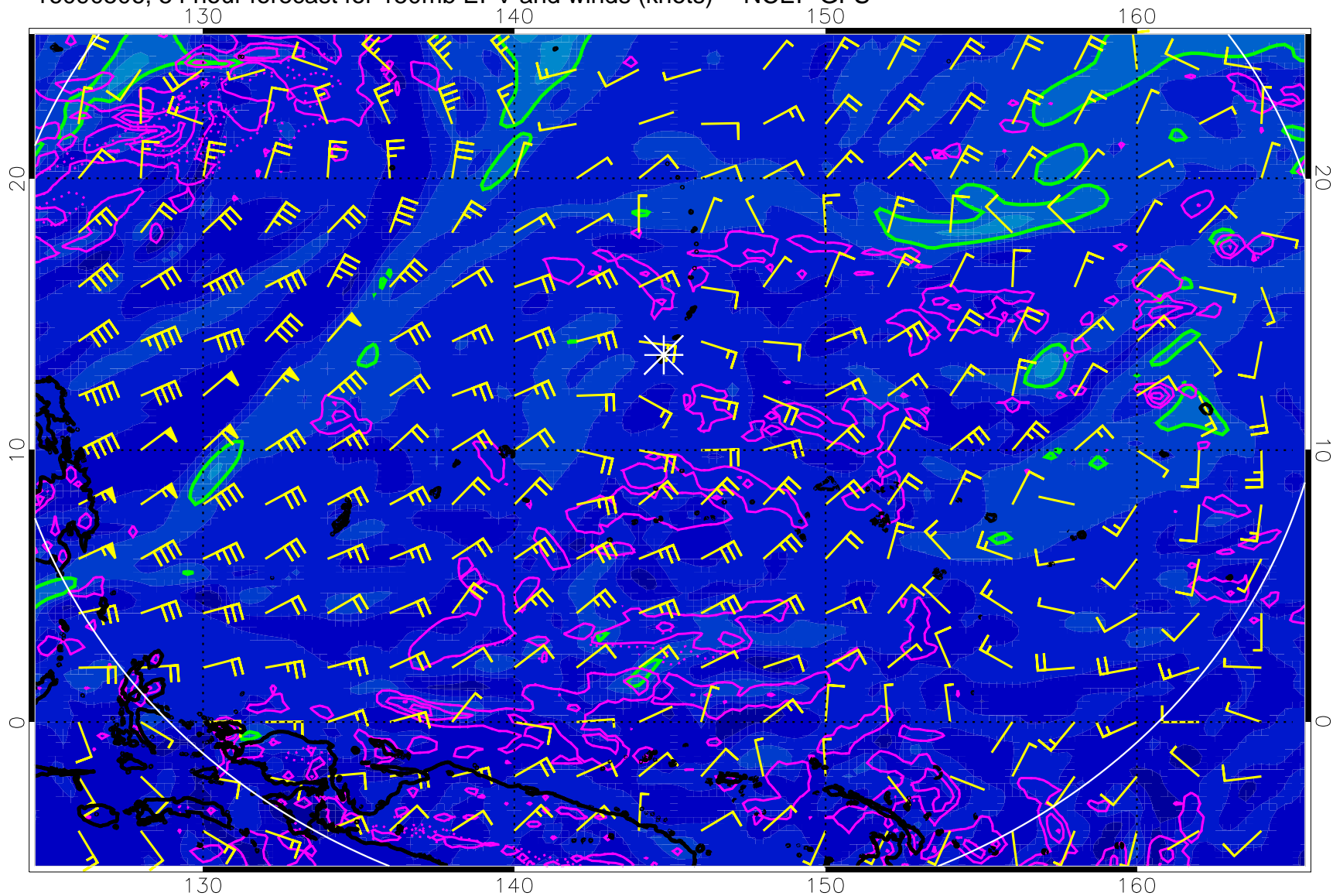
16090506, 54 hour forecast for 150mb EPV and winds (knots) -- NCEP GFS
