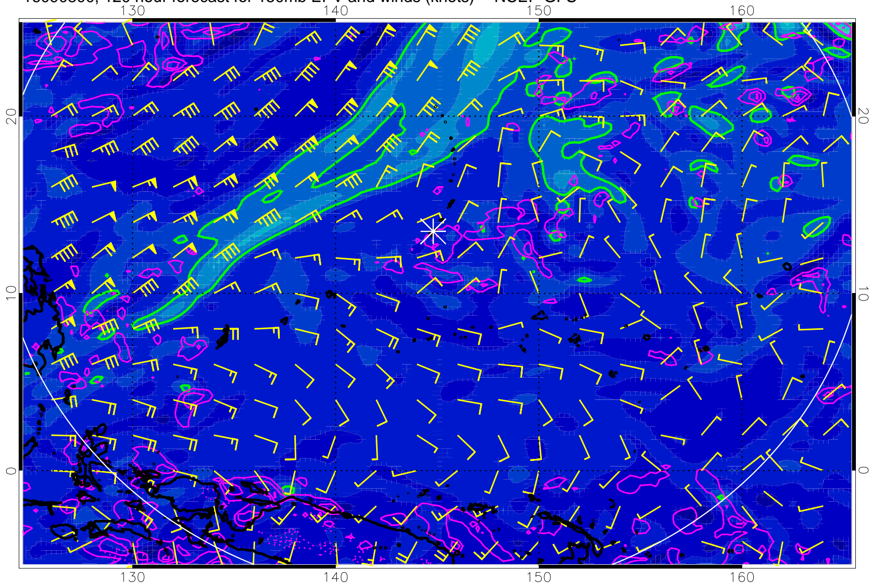
16090800, 120 hour forecast for 150mb EPV and winds (knots) -- NCEP GFS
