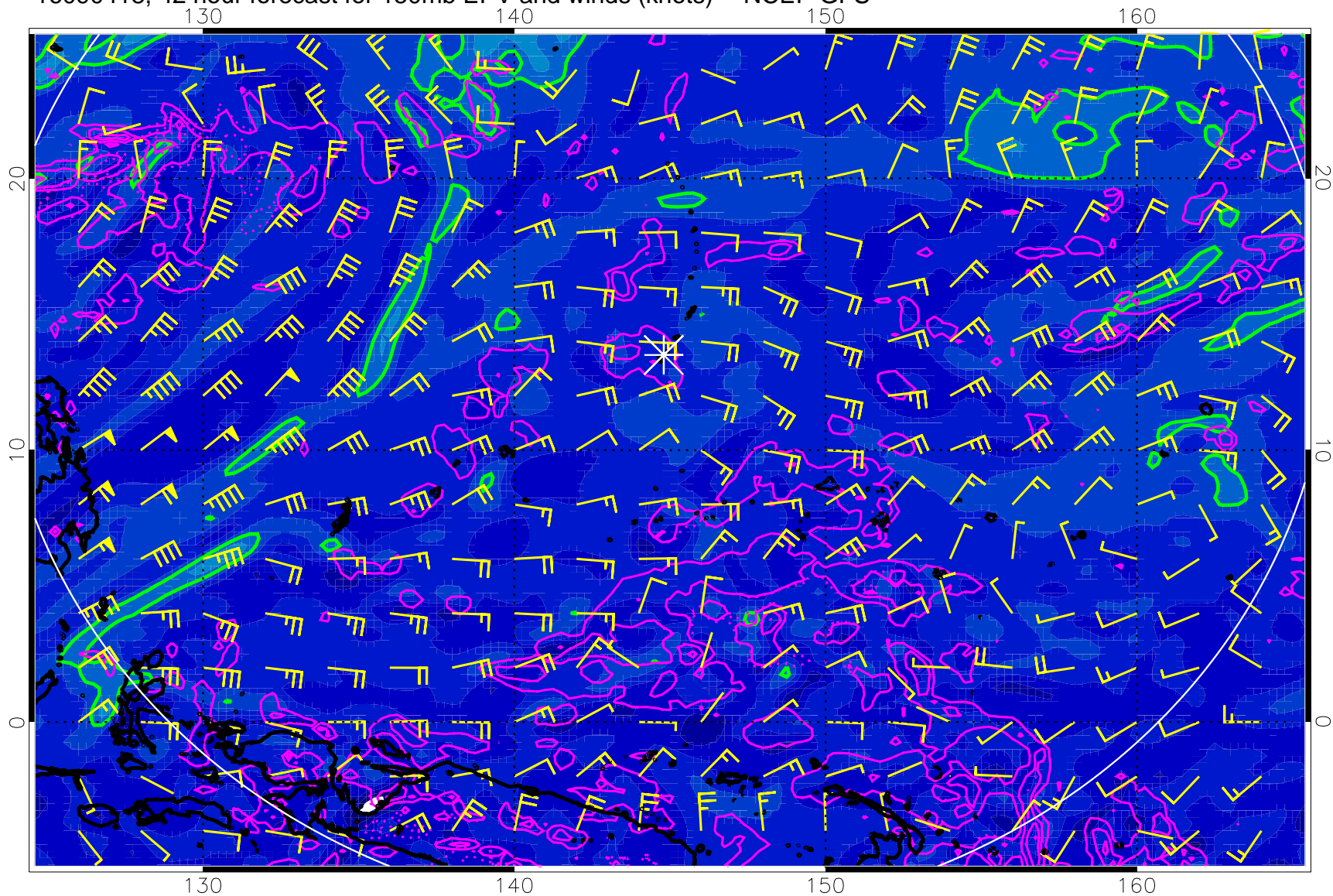
16090418, 42 hour forecast for 150mb EPV and winds (knots) -- NCEP GFS
