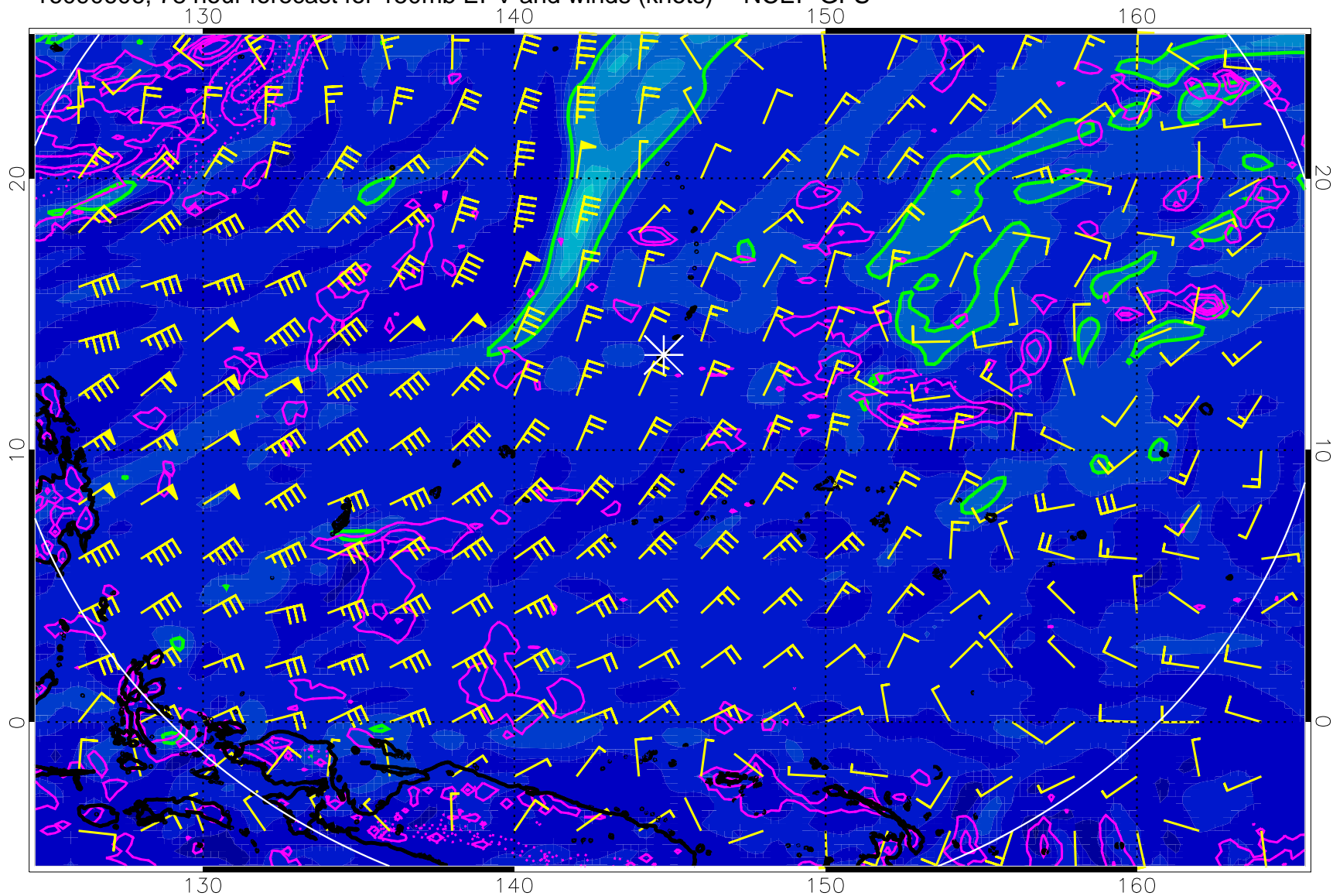
16090606, 78 hour forecast for 150mb EPV and winds (knots) -- NCEP GFS
