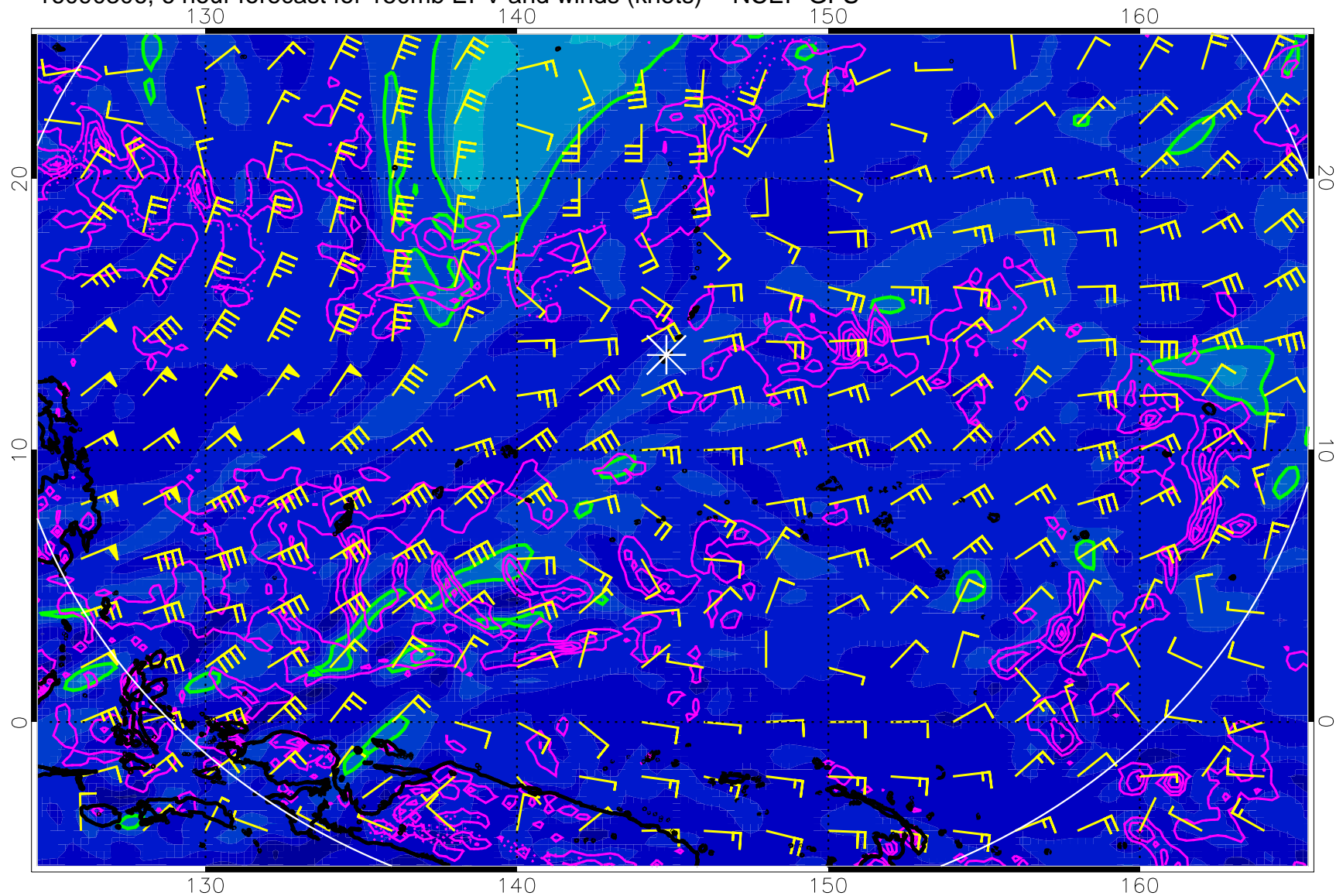
16090306, 6 hour forecast for 150mb EPV and winds (knots) -- NCEP GFS
