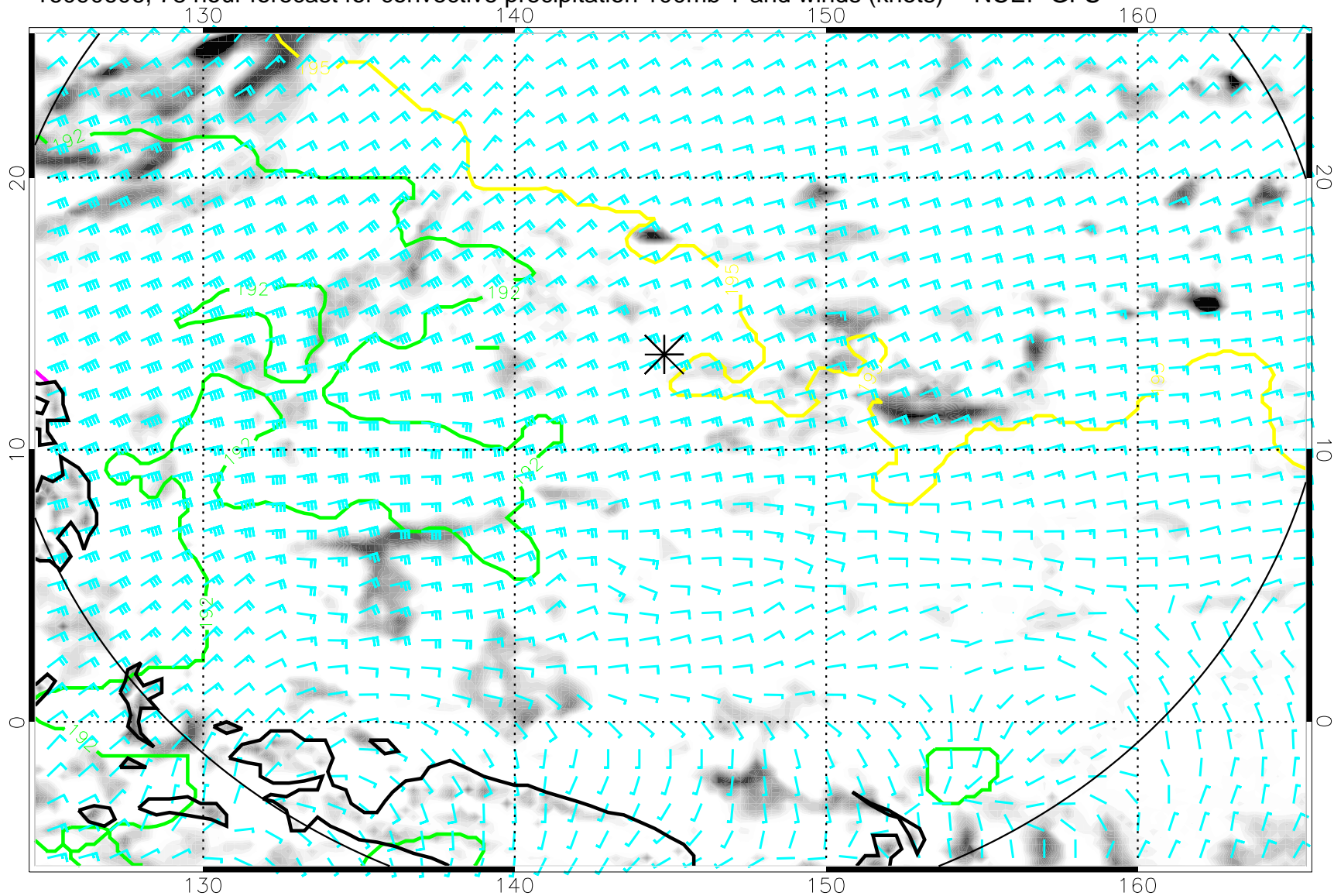
16090606, 78 hour forecast for convective precipitation 100mb T and winds (knots) -- NCEP GFS
