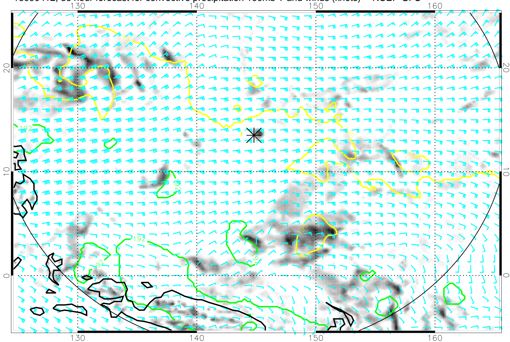
16090412, 36 hour forecast for convective precipitation 100mb T and winds (knots) -- NCEP GFS
