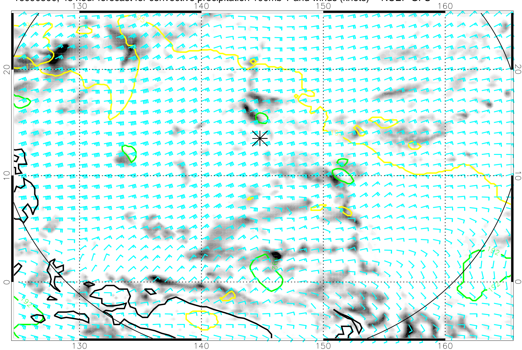
16090500, 48 hour forecast for convective precipitation 100mb T and winds (knots) -- NCEP GFS
