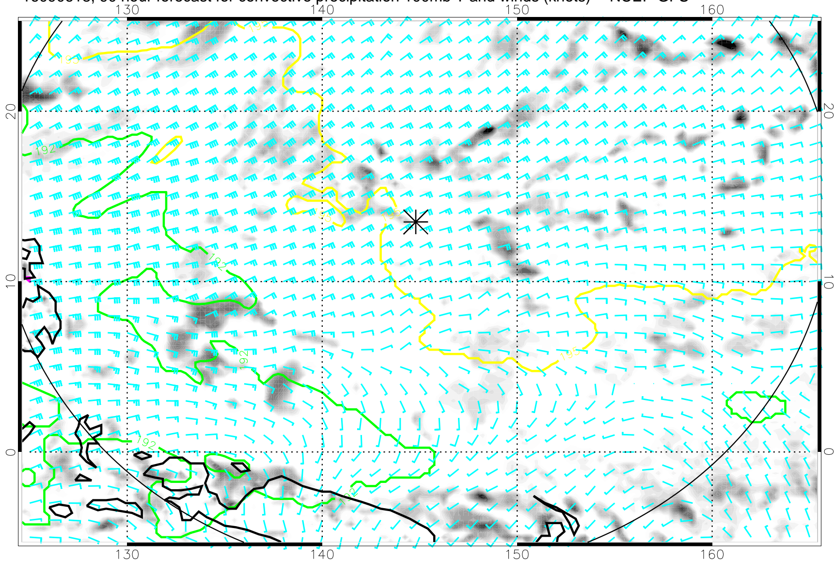
16090618, 90 hour forecast for convective precipitation 100mb T and winds (knots) -- NCEP GFS
