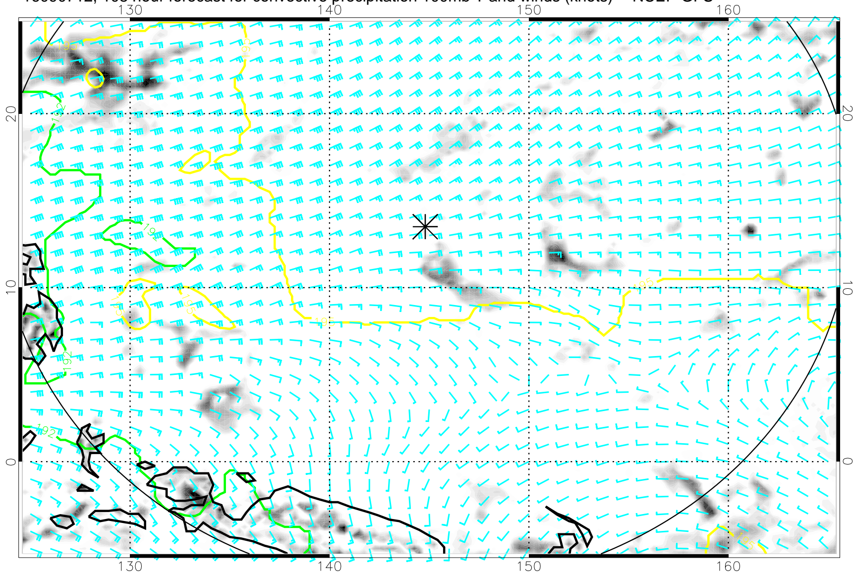
16090712, 108 hour forecast for convective precipitation 100mb T and winds (knots) -- NCEP GFS
