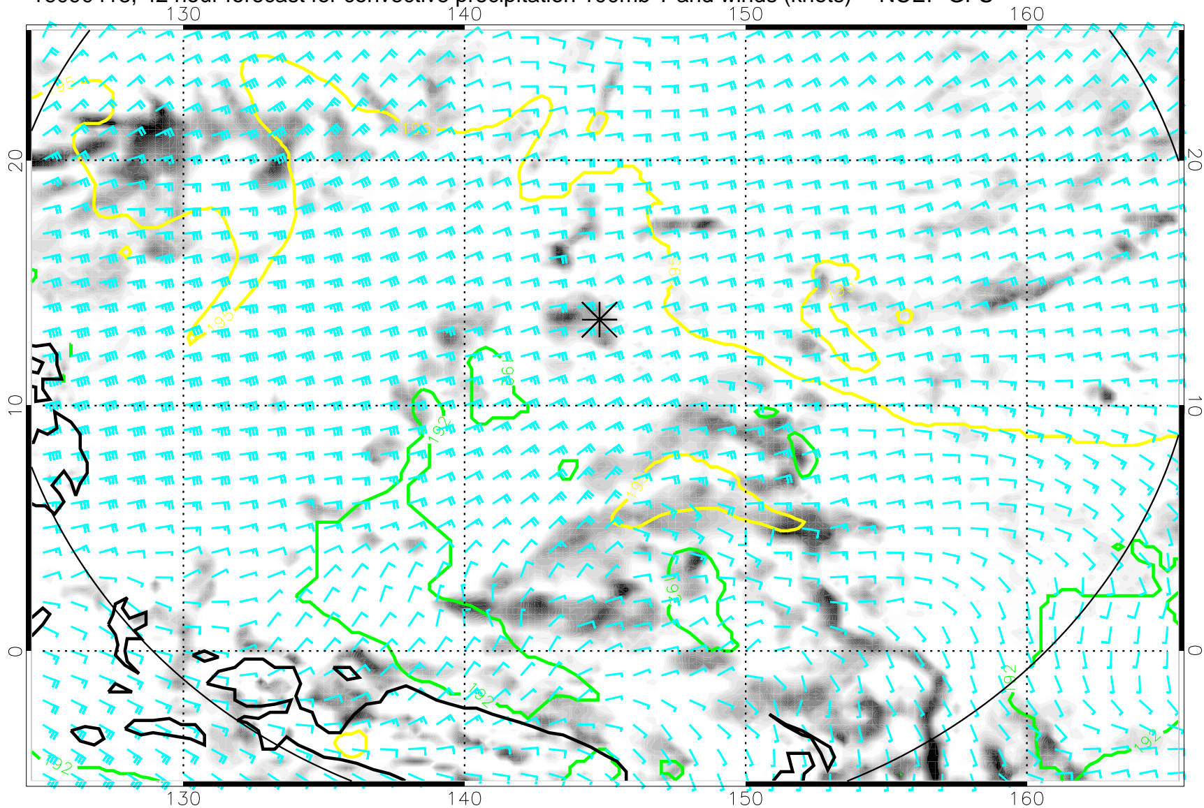
16090418, 42 hour forecast for convective precipitation 100mb T and winds (knots) -- NCEP GFS
