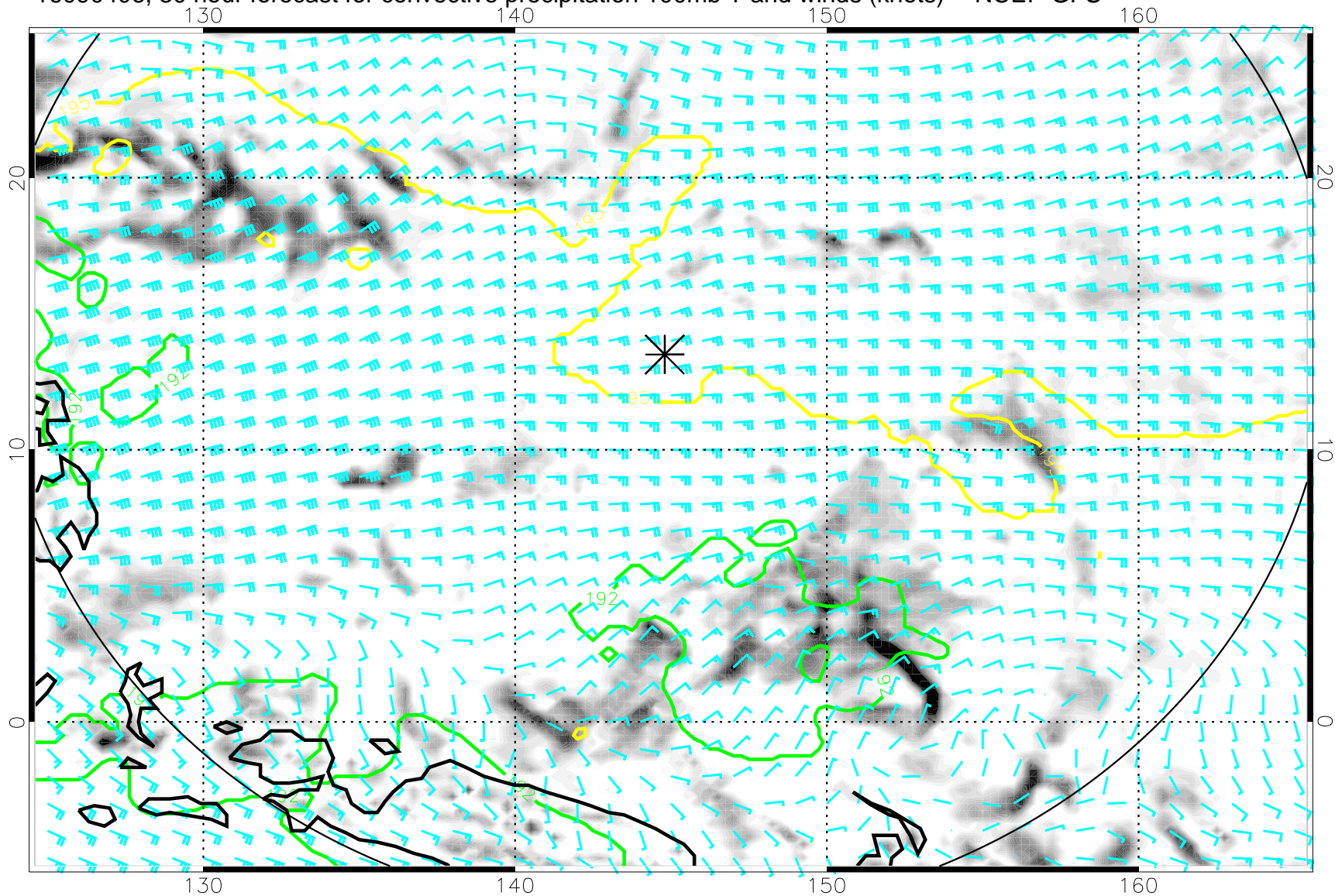
16090406, 30 hour forecast for convective precipitation 100mb T and winds (knots) -- NCEP GFS
