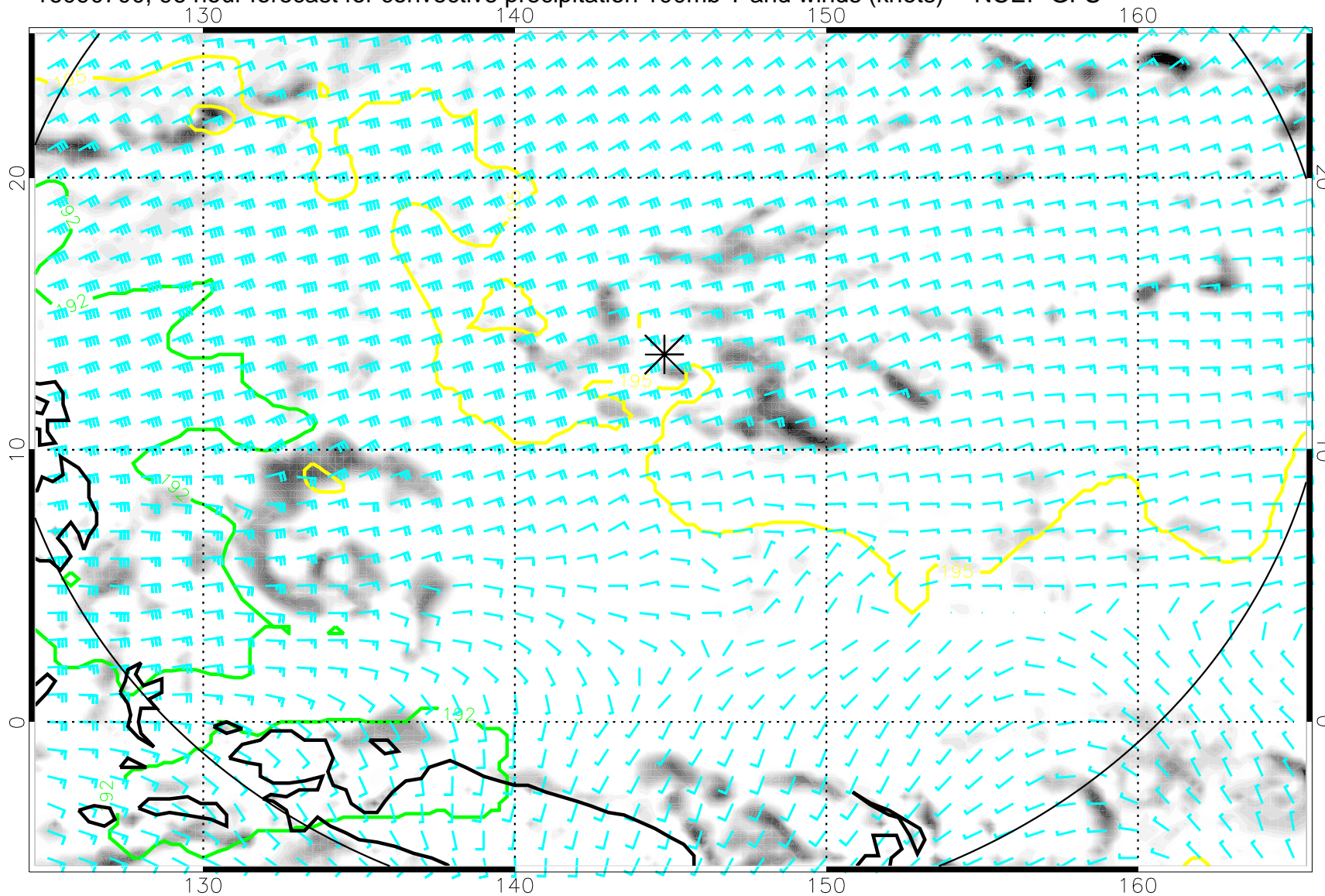
16090700, 96 hour forecast for convective precipitation 100mb T and winds (knots) -- NCEP GFS
