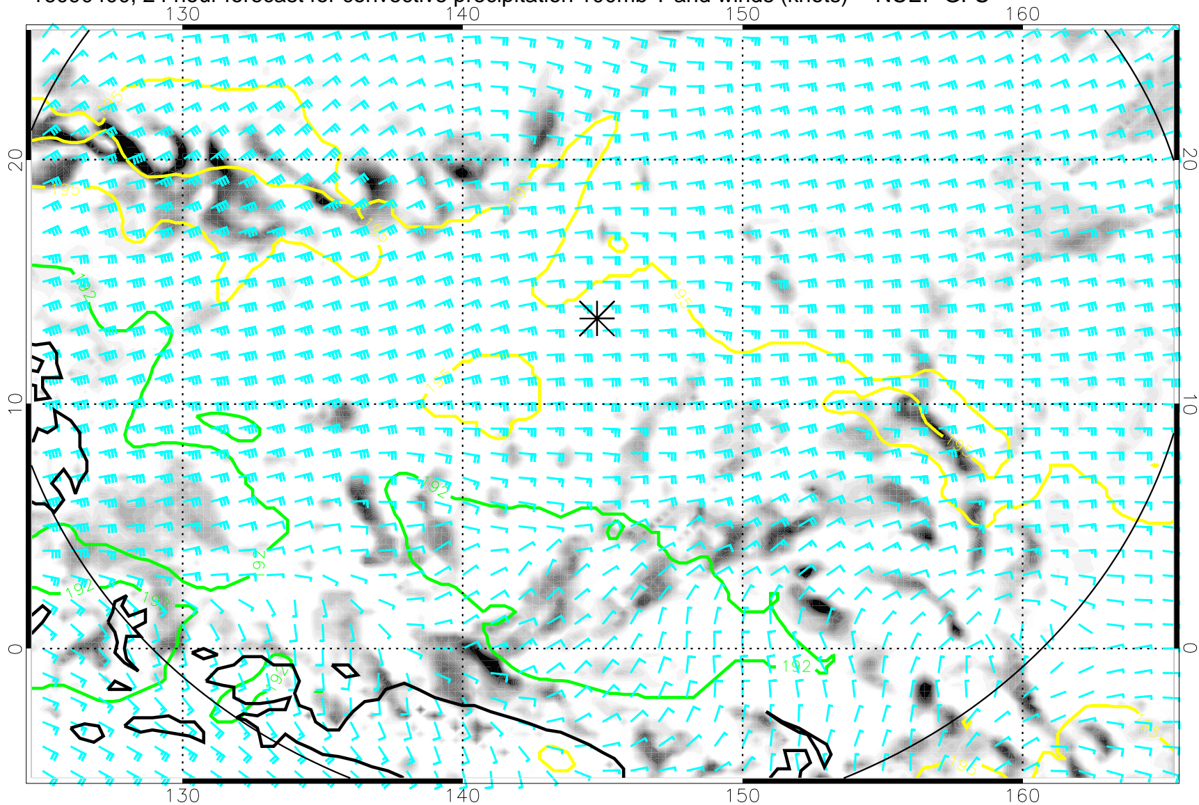
16090400, 24 hour forecast for convective precipitation 100mb T and winds (knots) -- NCEP GFS
