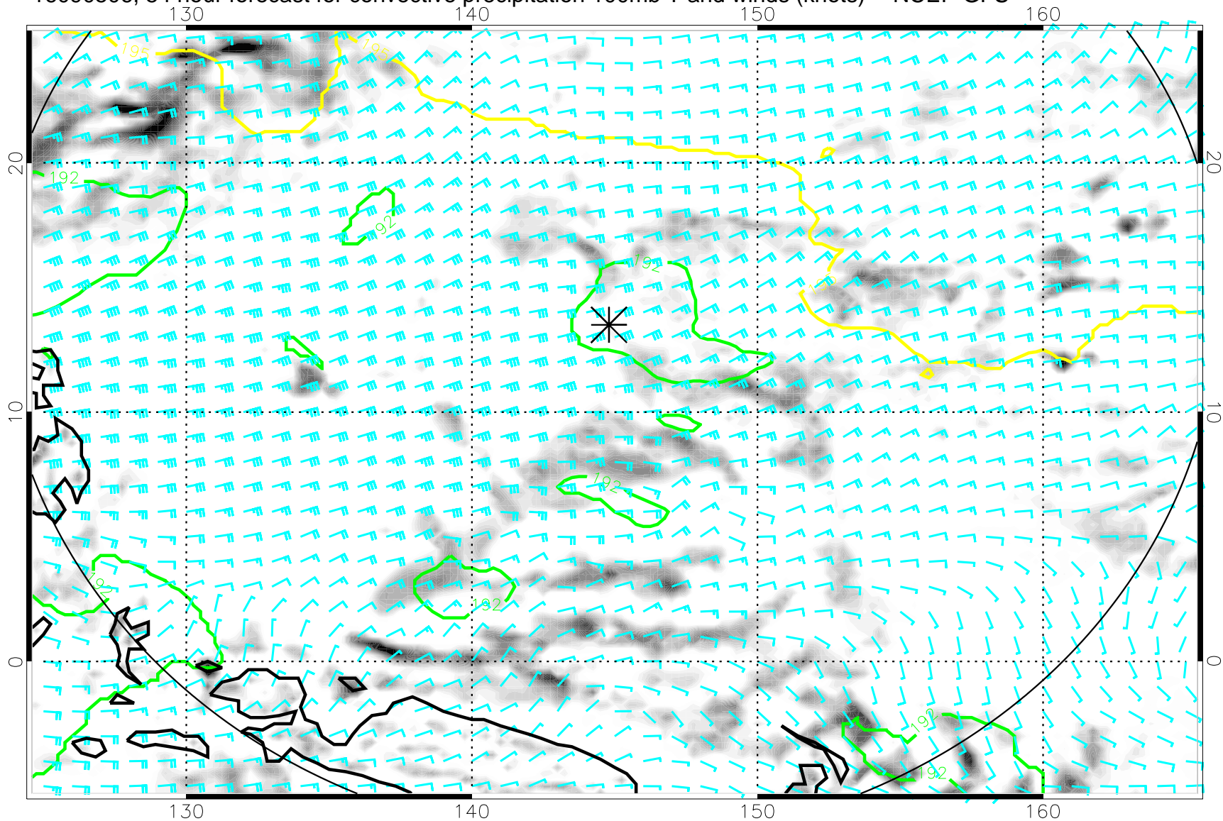
16090506, 54 hour forecast for convective precipitation 100mb T and winds (knots) -- NCEP GFS
