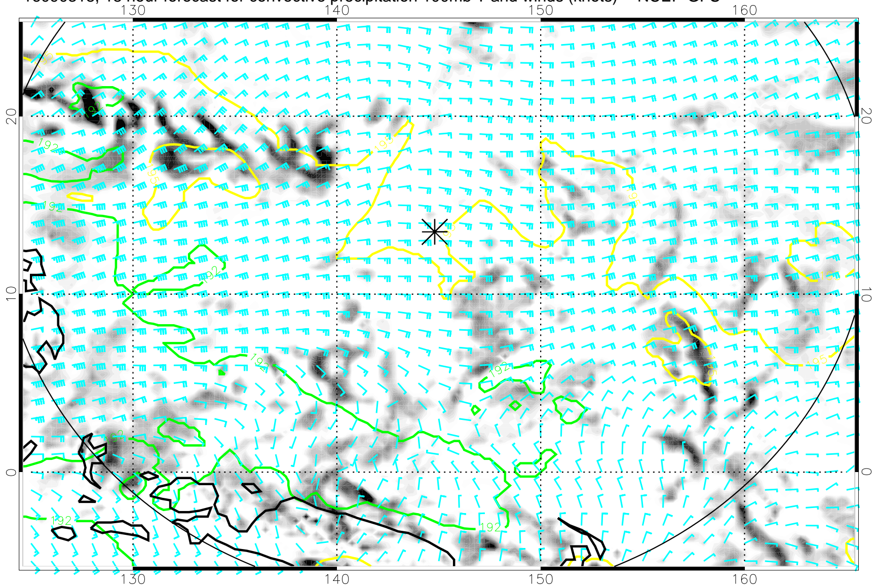
16090318, 18 hour forecast for convective precipitation 100mb T and winds (knots) -- NCEP GFS
