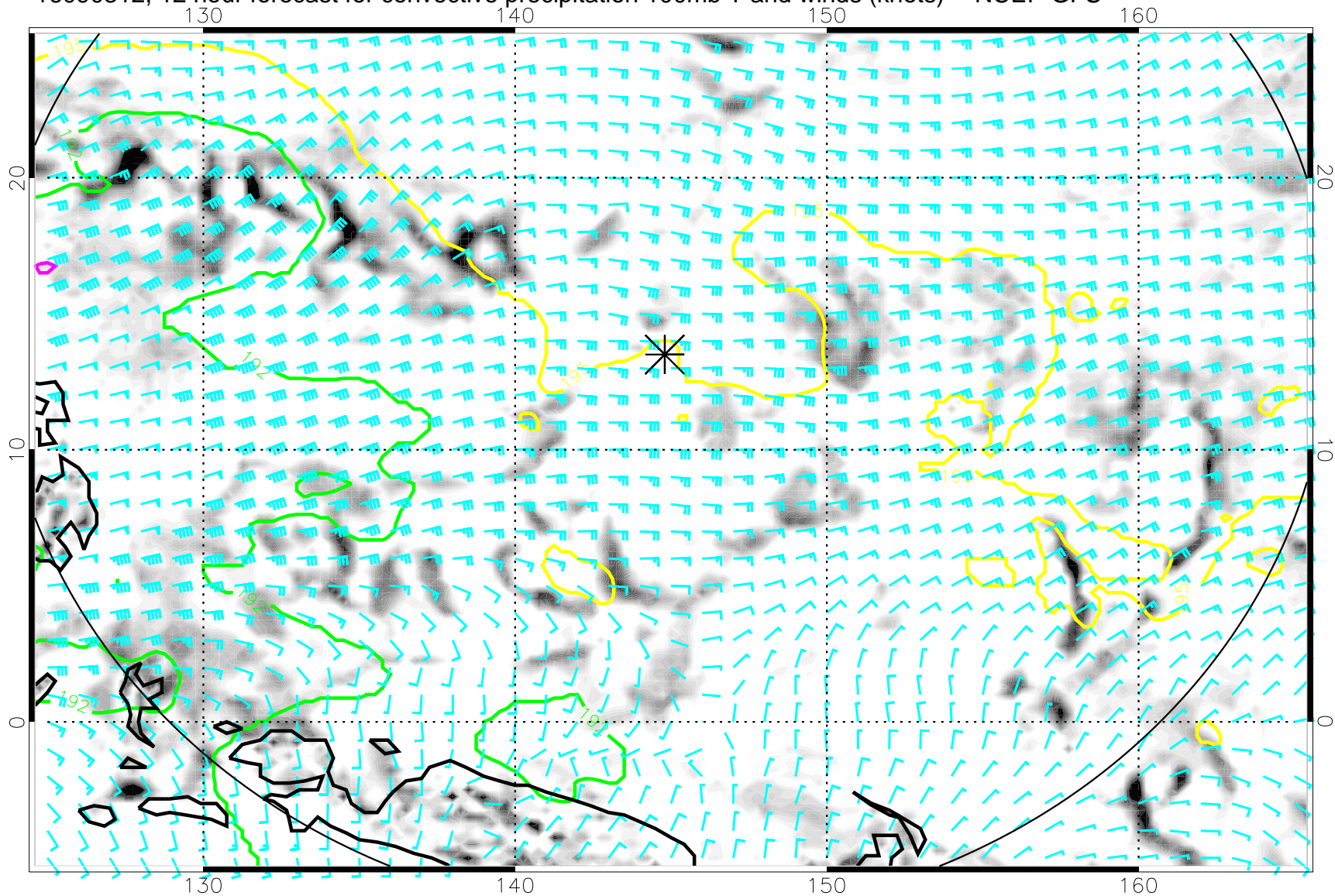
16090312, 12 hour forecast for convective precipitation 100mb T and winds (knots) -- NCEP GFS
