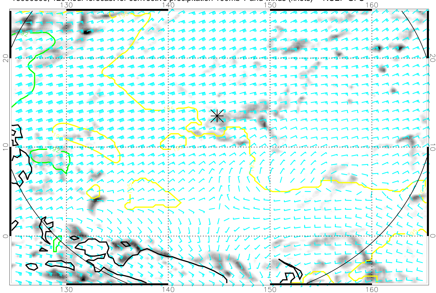
16090800, 120 hour forecast for convective precipitation 100mb T and winds (knots) -- NCEP GFS
