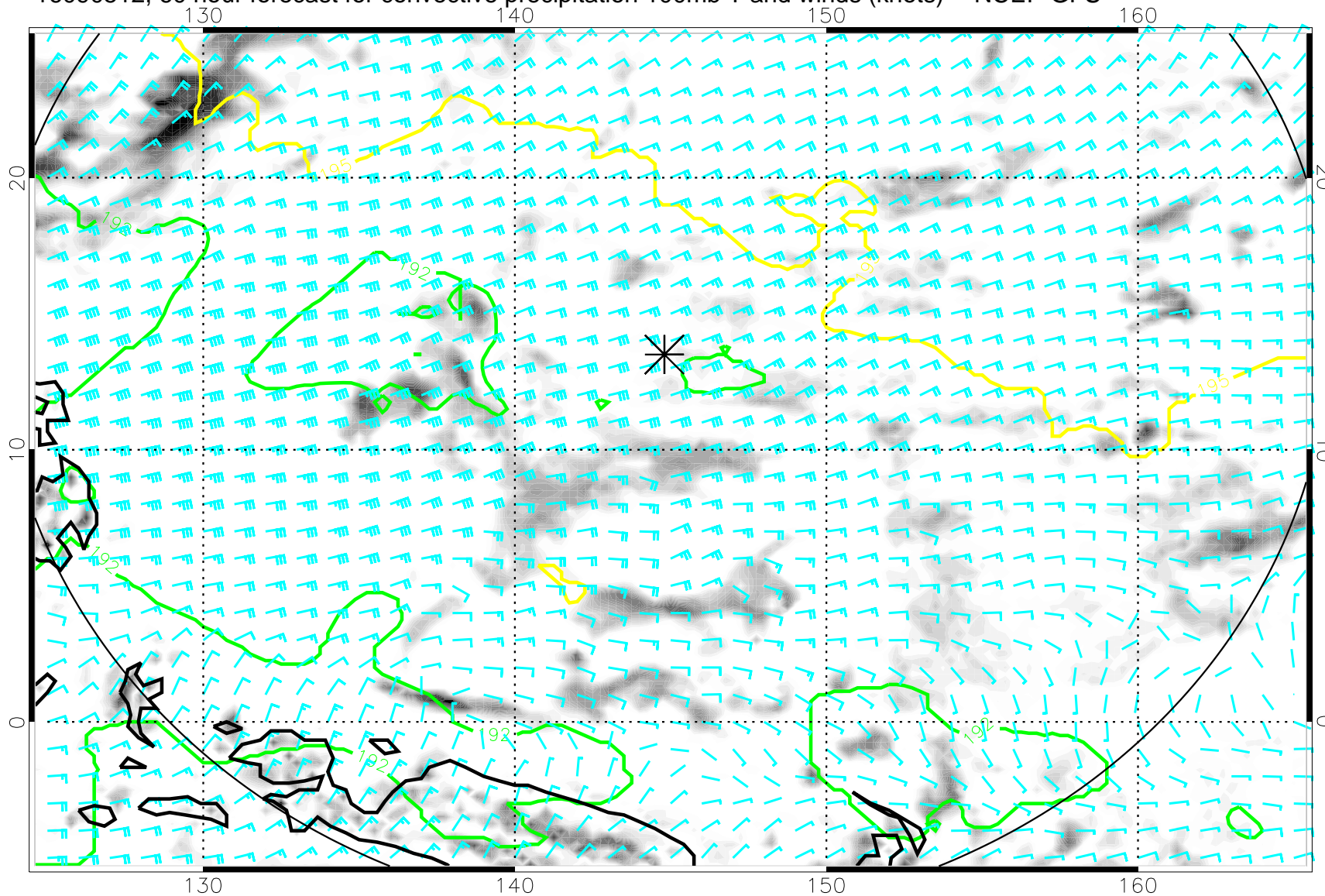
16090512, 60 hour forecast for convective precipitation 100mb T and winds (knots) -- NCEP GFS
