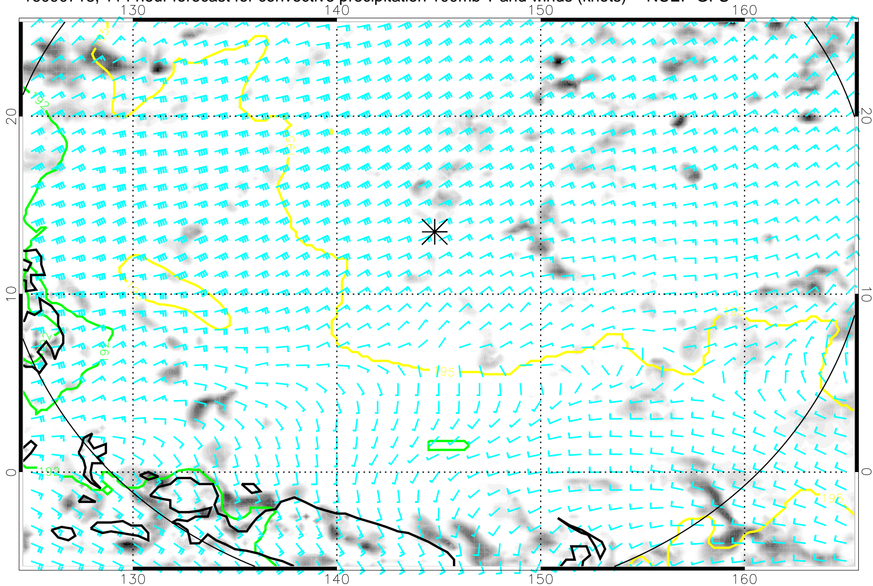
16090718, 114 hour forecast for convective precipitation 100mb T and winds (knots) -- NCEP GFS
