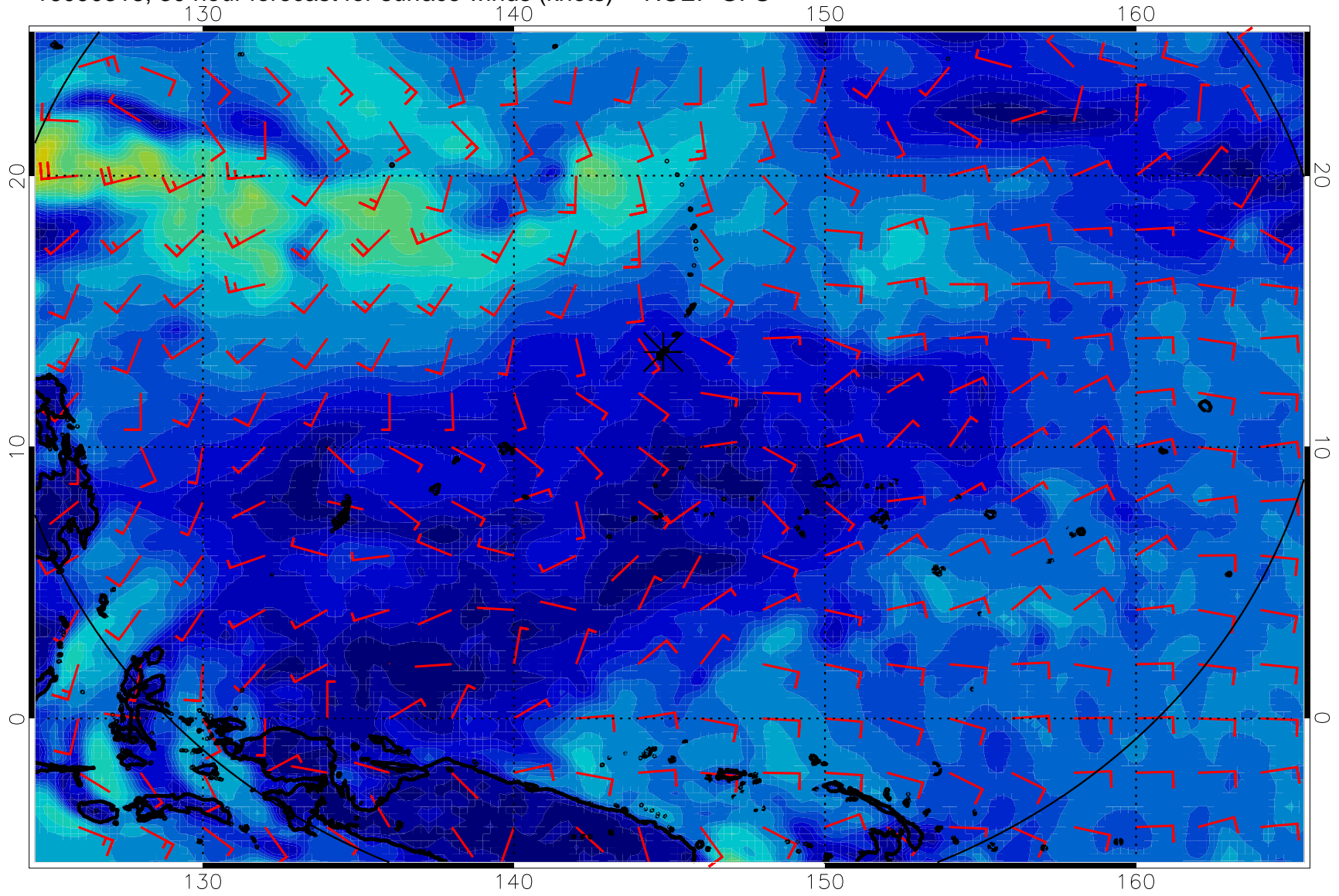
16090318, 30 hour forecast for surface winds (knots) -- NCEP GFS
