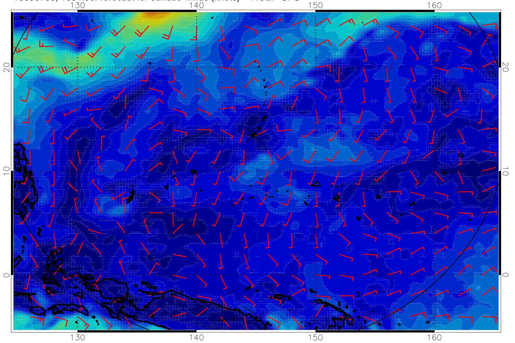
16090700, 108 hour forecast for surface winds (knots) -- NCEP GFS
