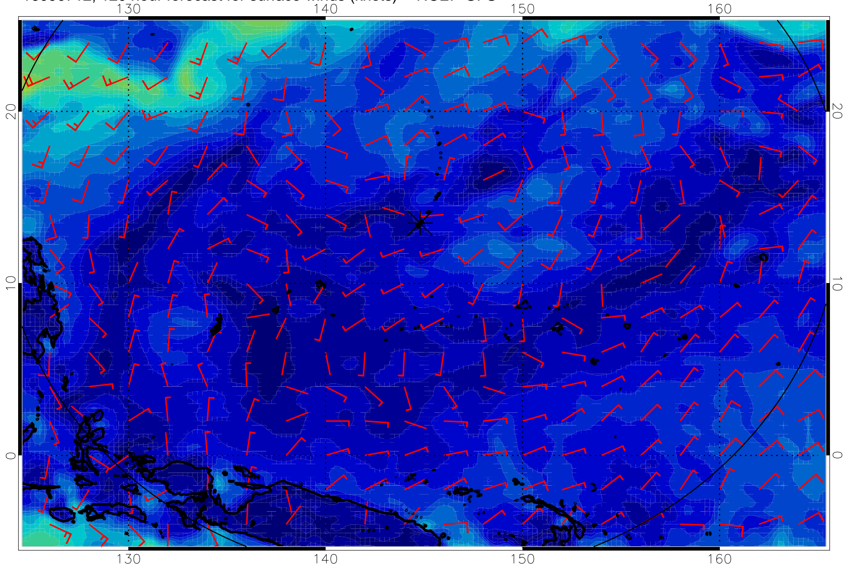
16090712, 120 hour forecast for surface winds (knots) -- NCEP GFS
