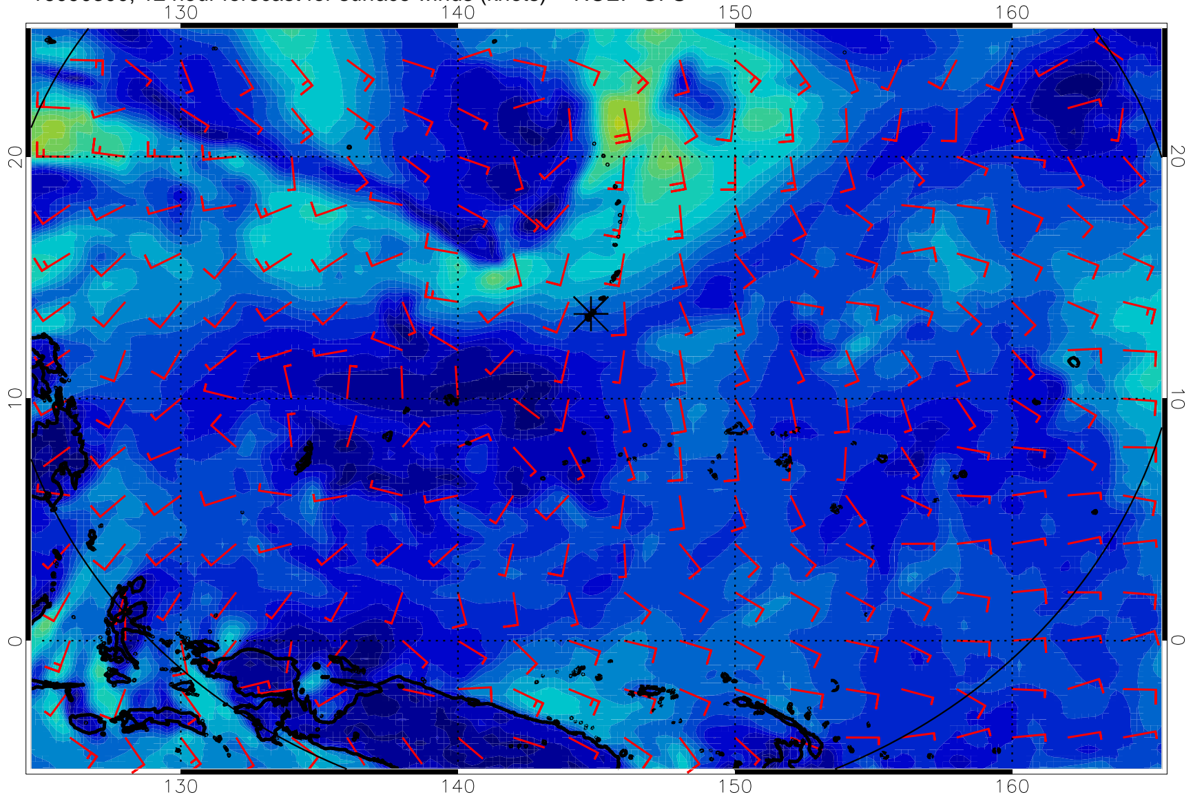
16090300, 12 hour forecast for surface winds (knots) -- NCEP GFS
