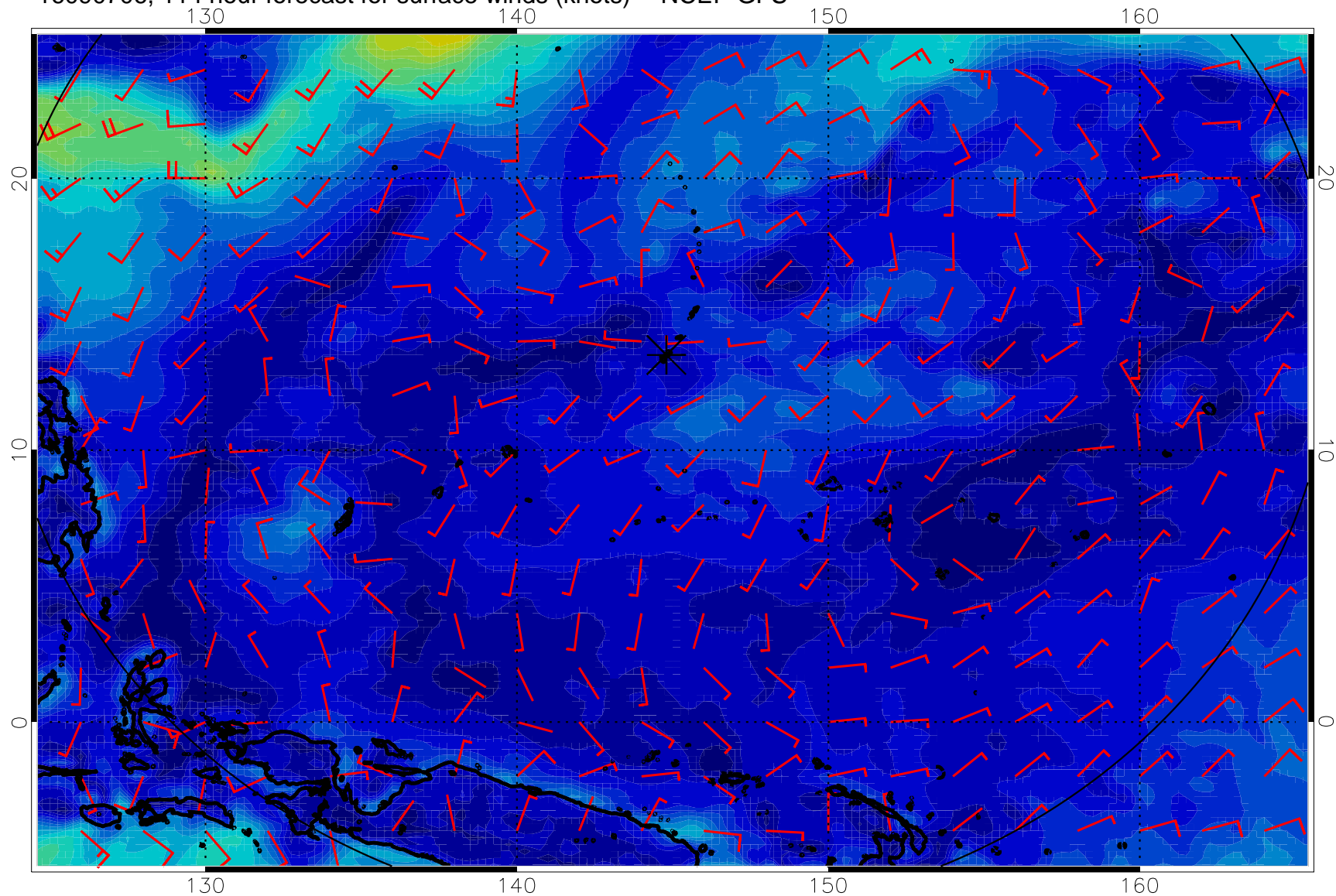
16090706, 114 hour forecast for surface winds (knots) -- NCEP GFS
