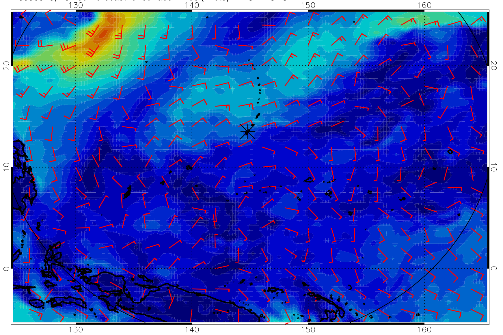
16090518, 78 hour forecast for surface winds (knots) -- NCEP GFS
