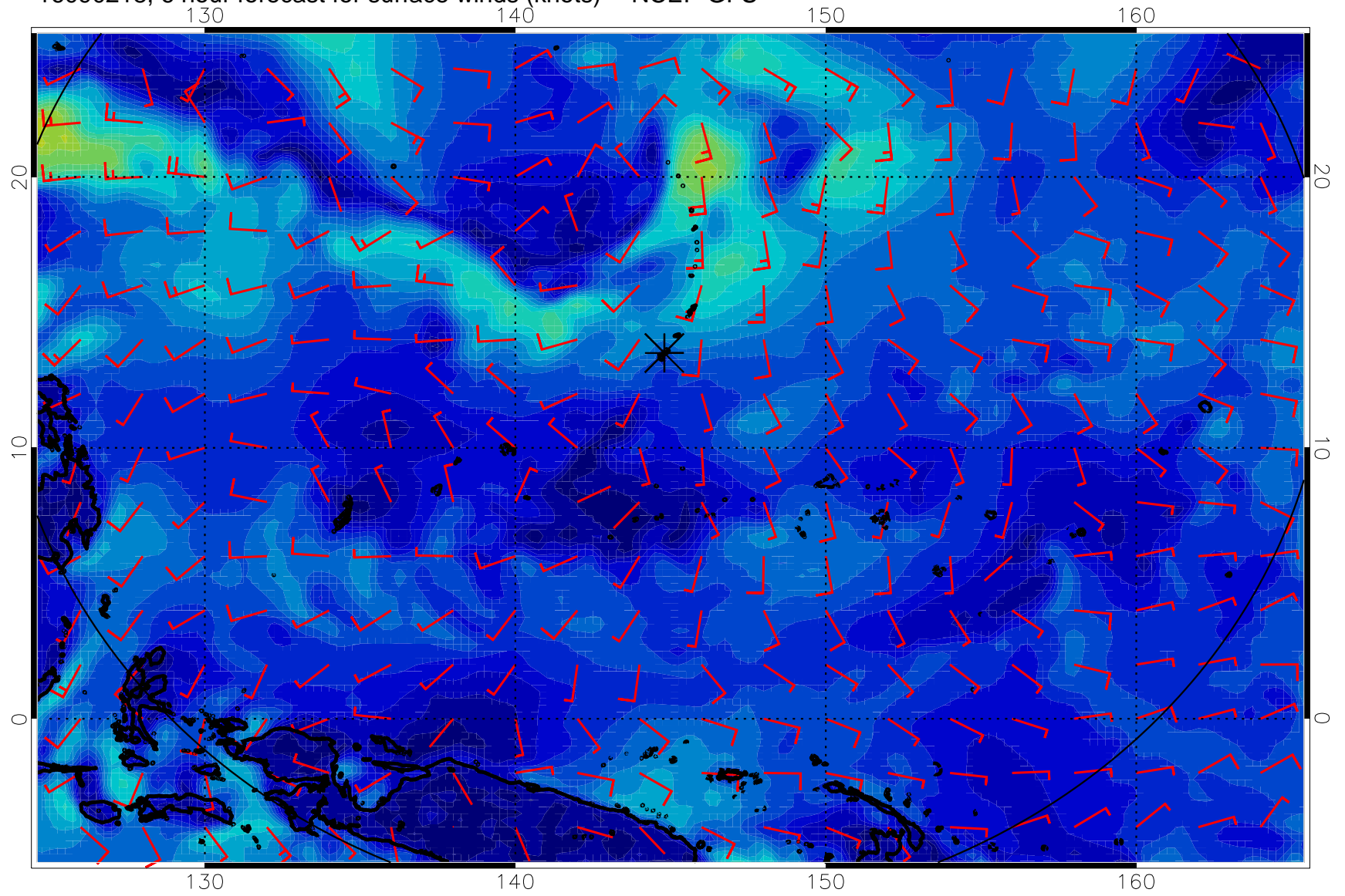
16090218, 6 hour forecast for surface winds (knots) -- NCEP GFS
