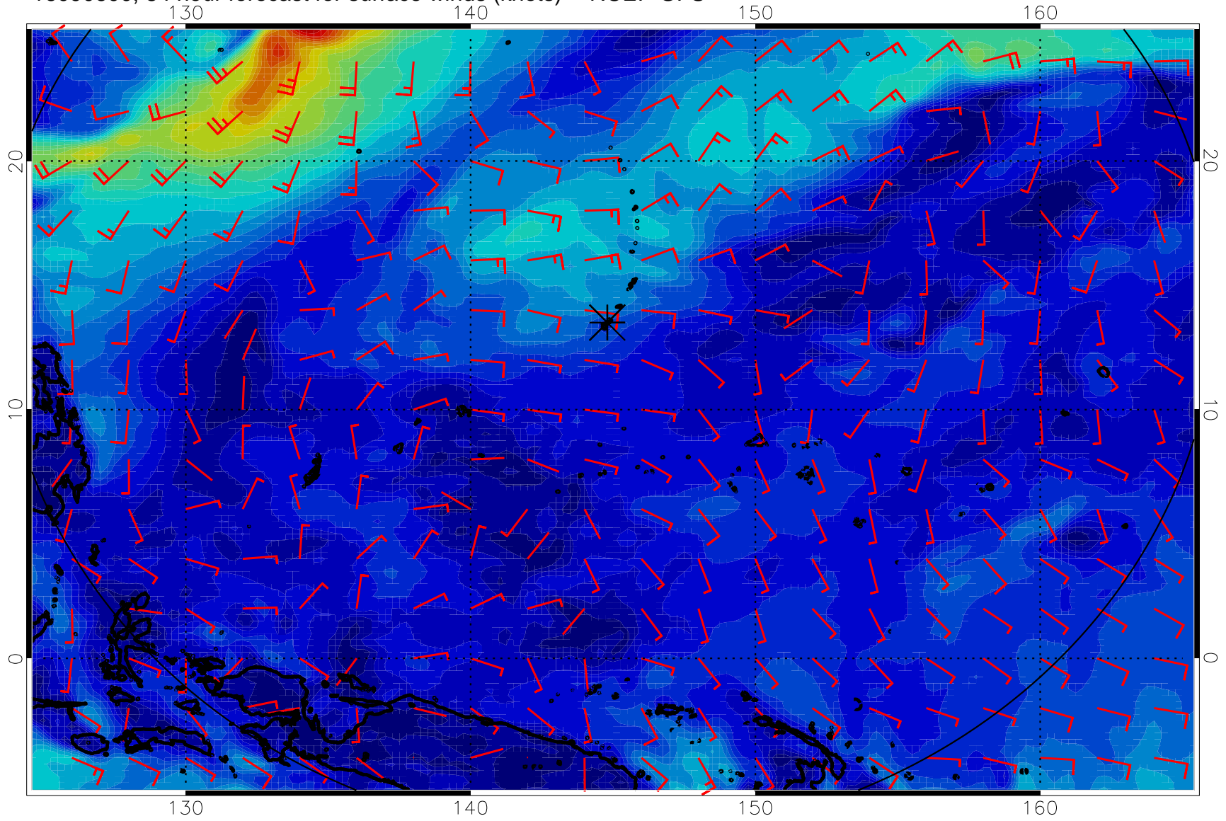
16090600, 84 hour forecast for surface winds (knots) -- NCEP GFS
