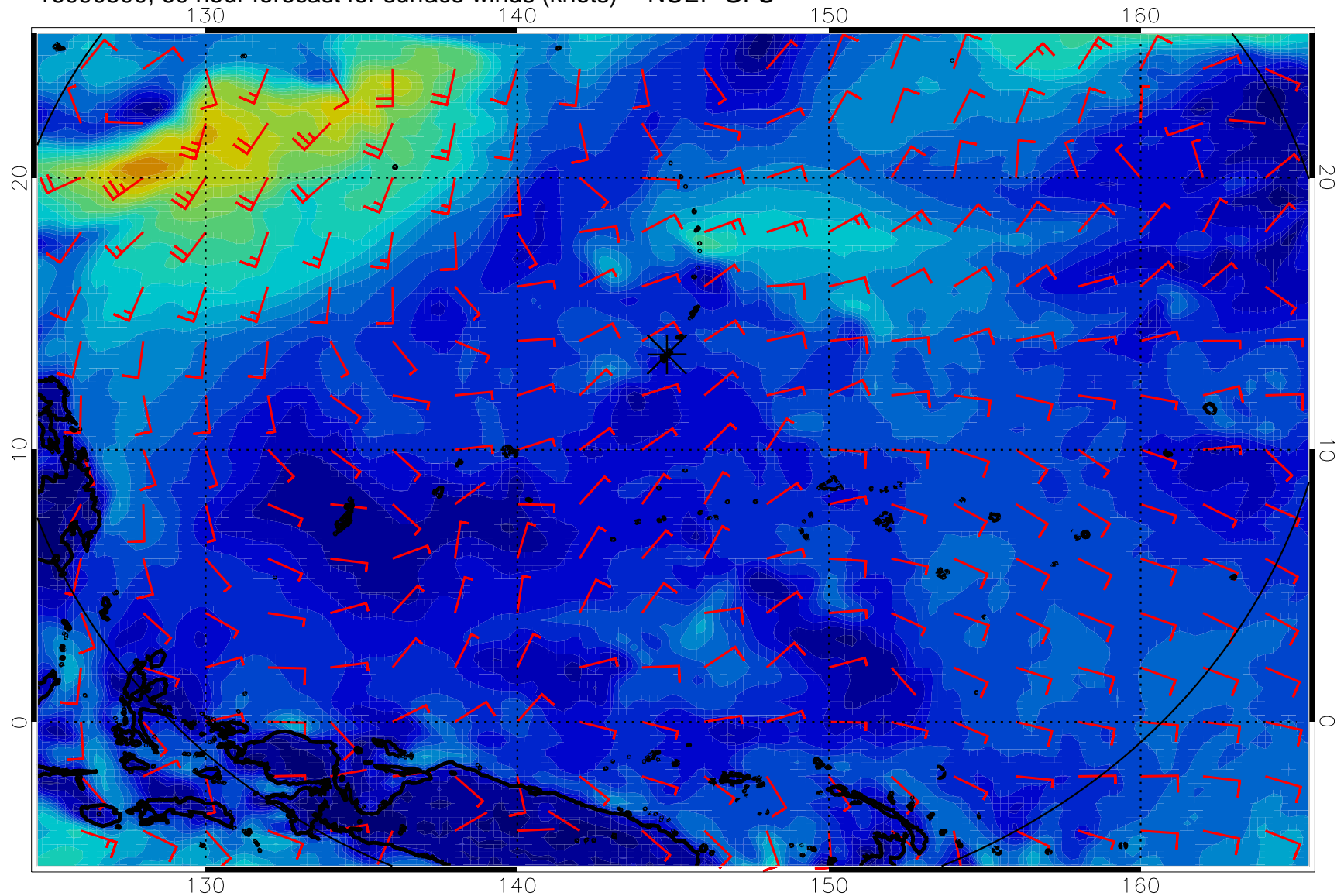
16090500, 60 hour forecast for surface winds (knots) -- NCEP GFS
