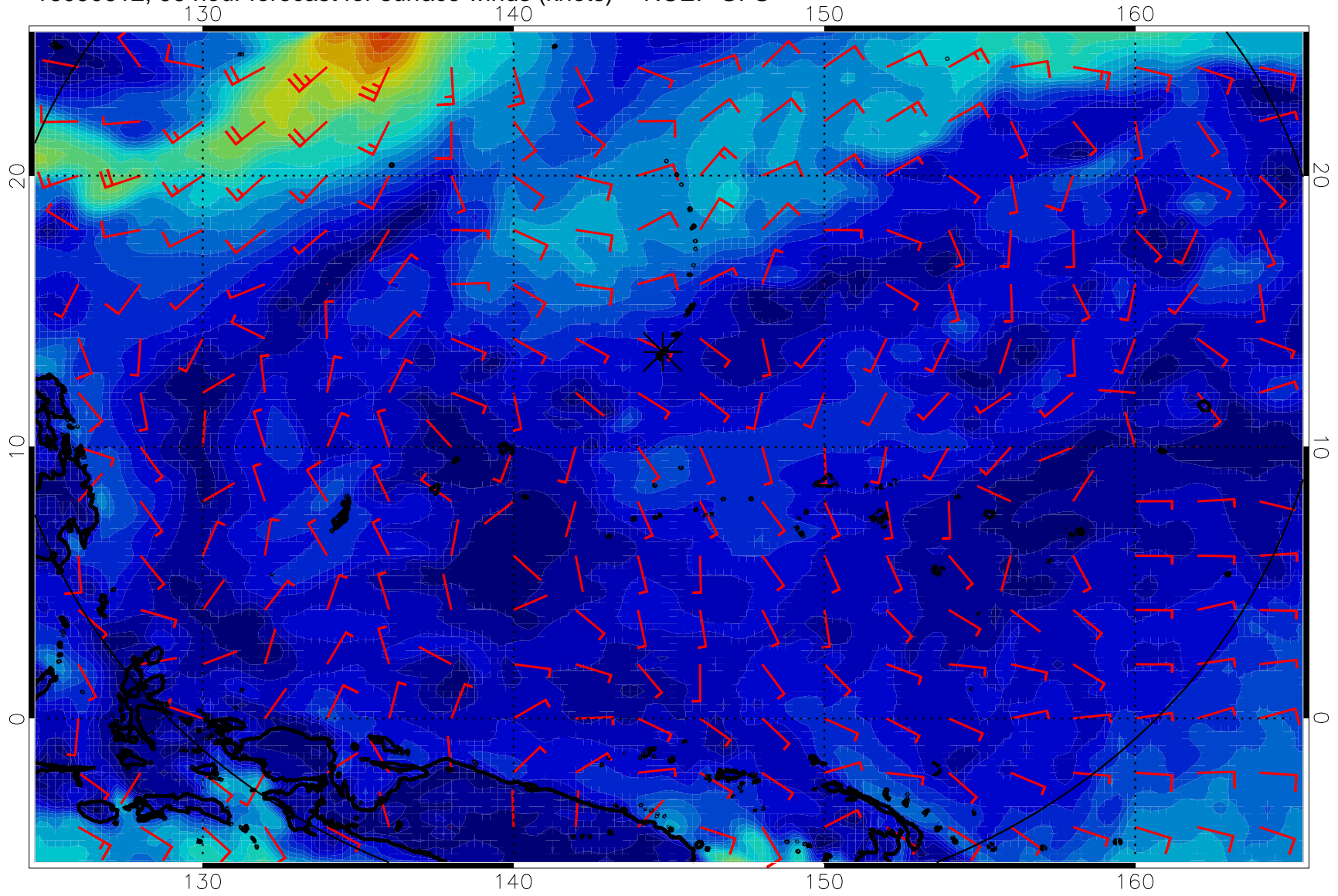
16090612, 96 hour forecast for surface winds (knots) -- NCEP GFS
