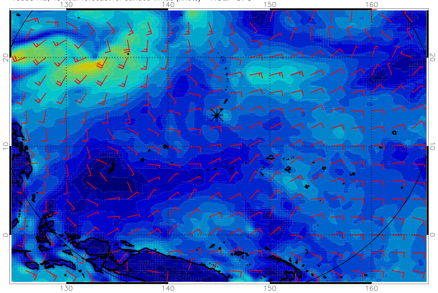
16090412, 48 hour forecast for surface winds (knots) -- NCEP GFS
