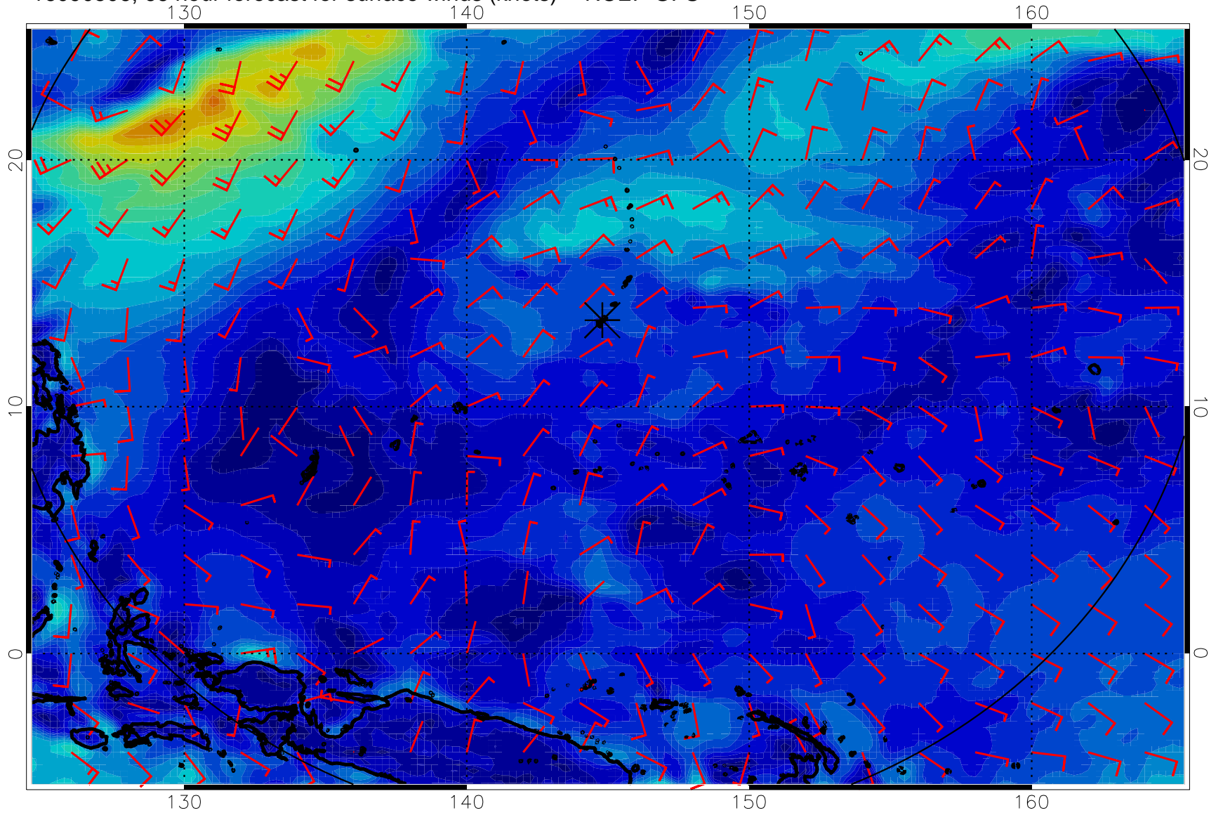
16090506, 66 hour forecast for surface winds (knots) -- NCEP GFS
