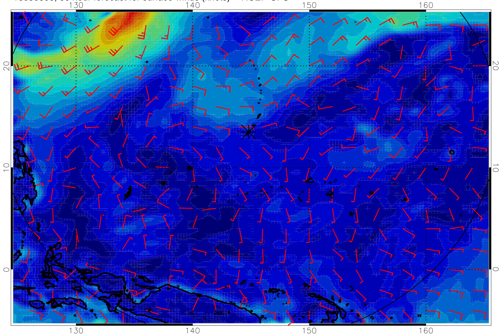
16090606, 90 hour forecast for surface winds (knots) -- NCEP GFS
