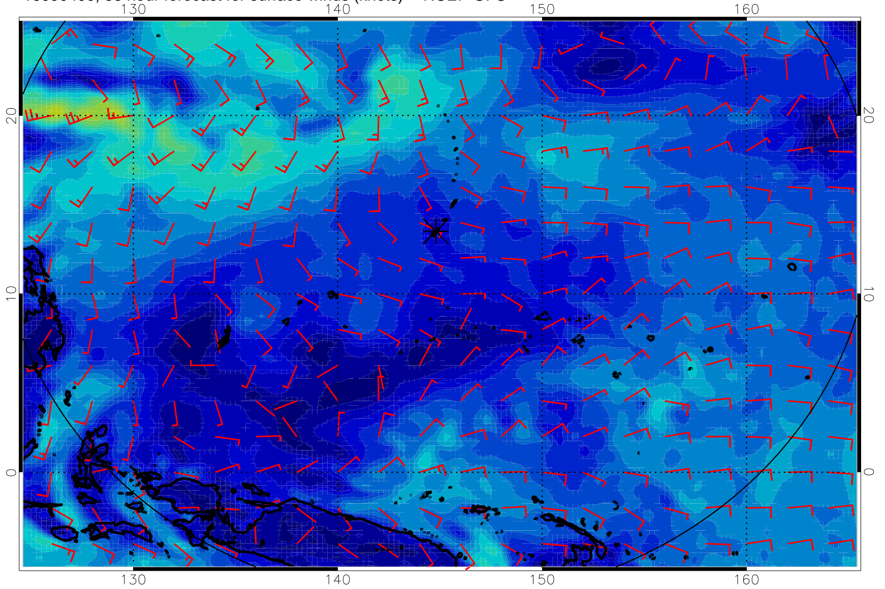
16090400, 36 hour forecast for surface winds (knots) -- NCEP GFS
