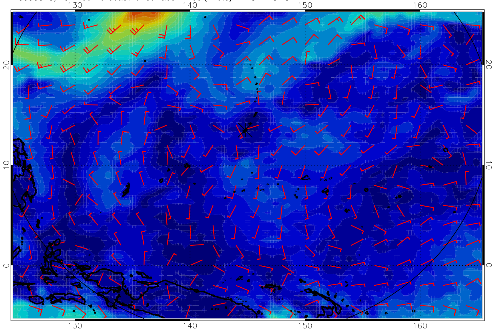
16090618, 102 hour forecast for surface winds (knots) -- NCEP GFS
