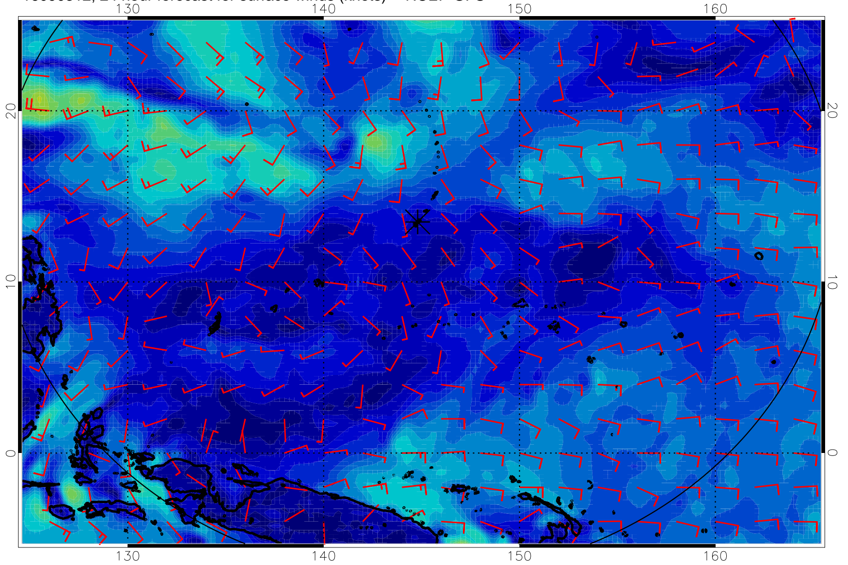
16090312, 24 hour forecast for surface winds (knots) -- NCEP GFS
