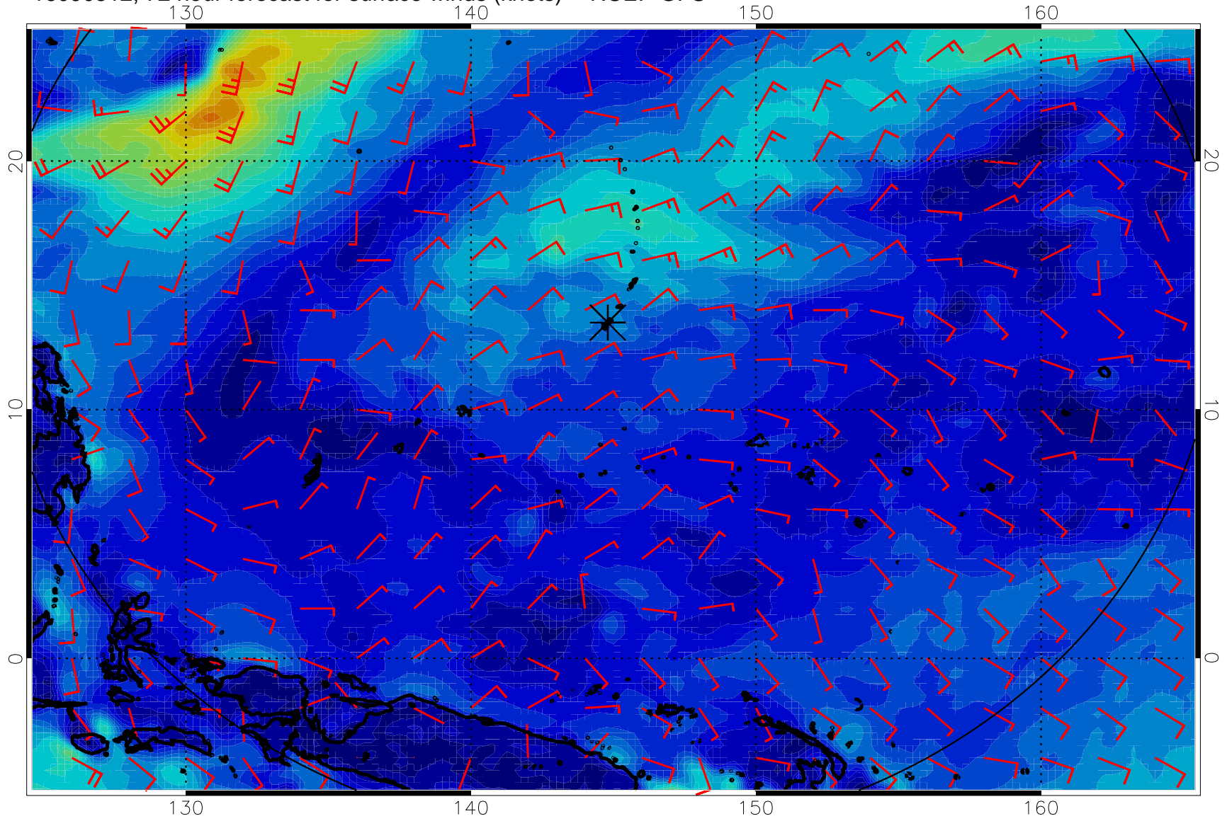
16090512, 72 hour forecast for surface winds (knots) -- NCEP GFS
