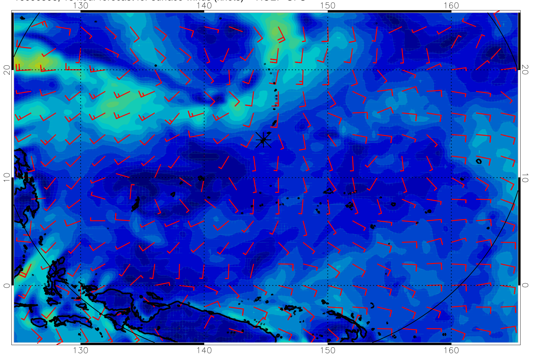
16090306, 18 hour forecast for surface winds (knots) -- NCEP GFS
