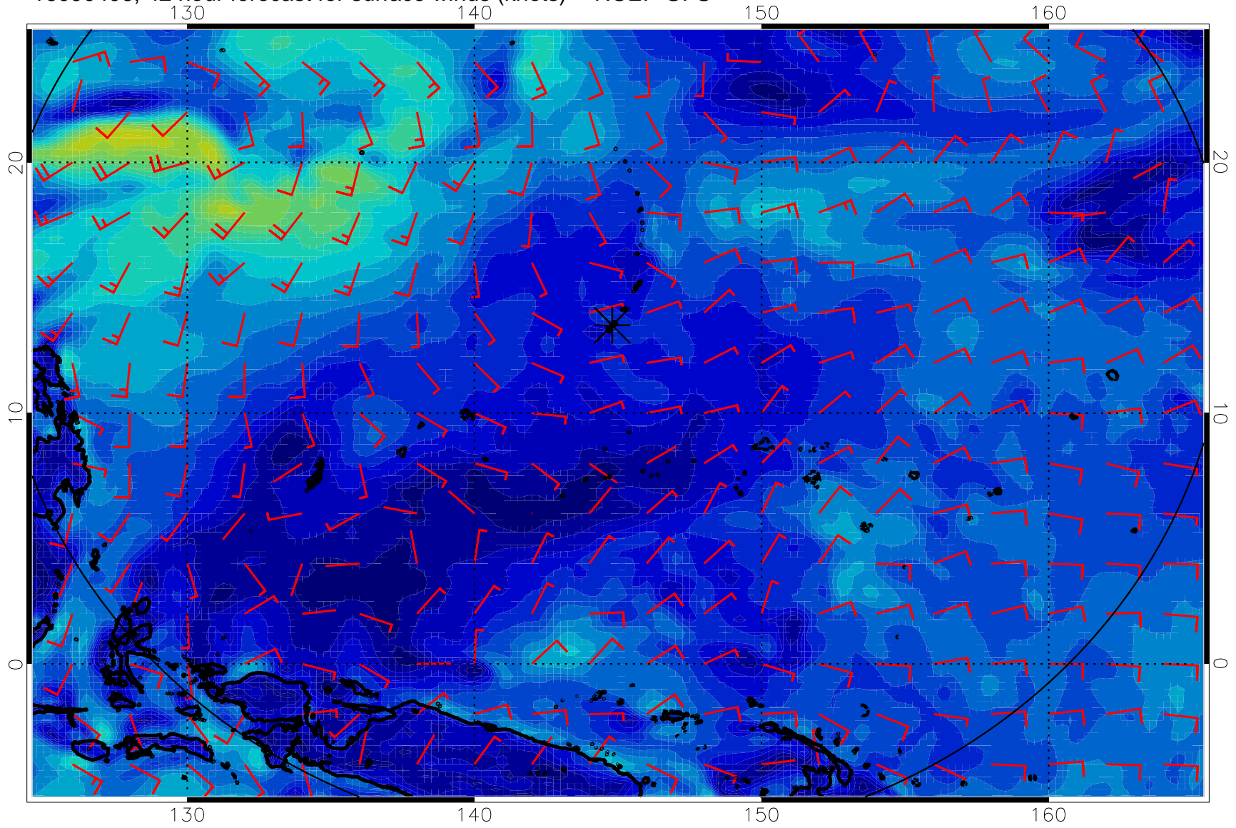
16090406, 42 hour forecast for surface winds (knots) -- NCEP GFS
