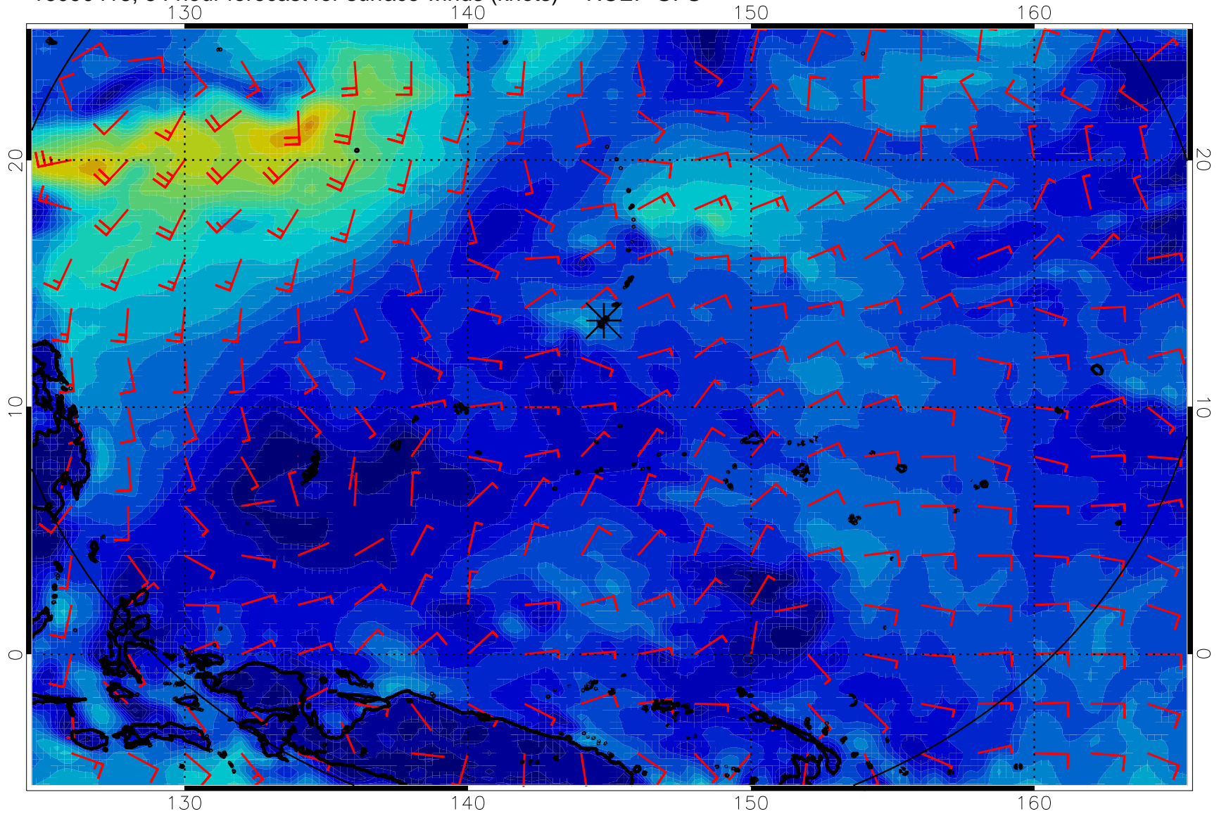
16090418, 54 hour forecast for surface winds (knots) -- NCEP GFS
