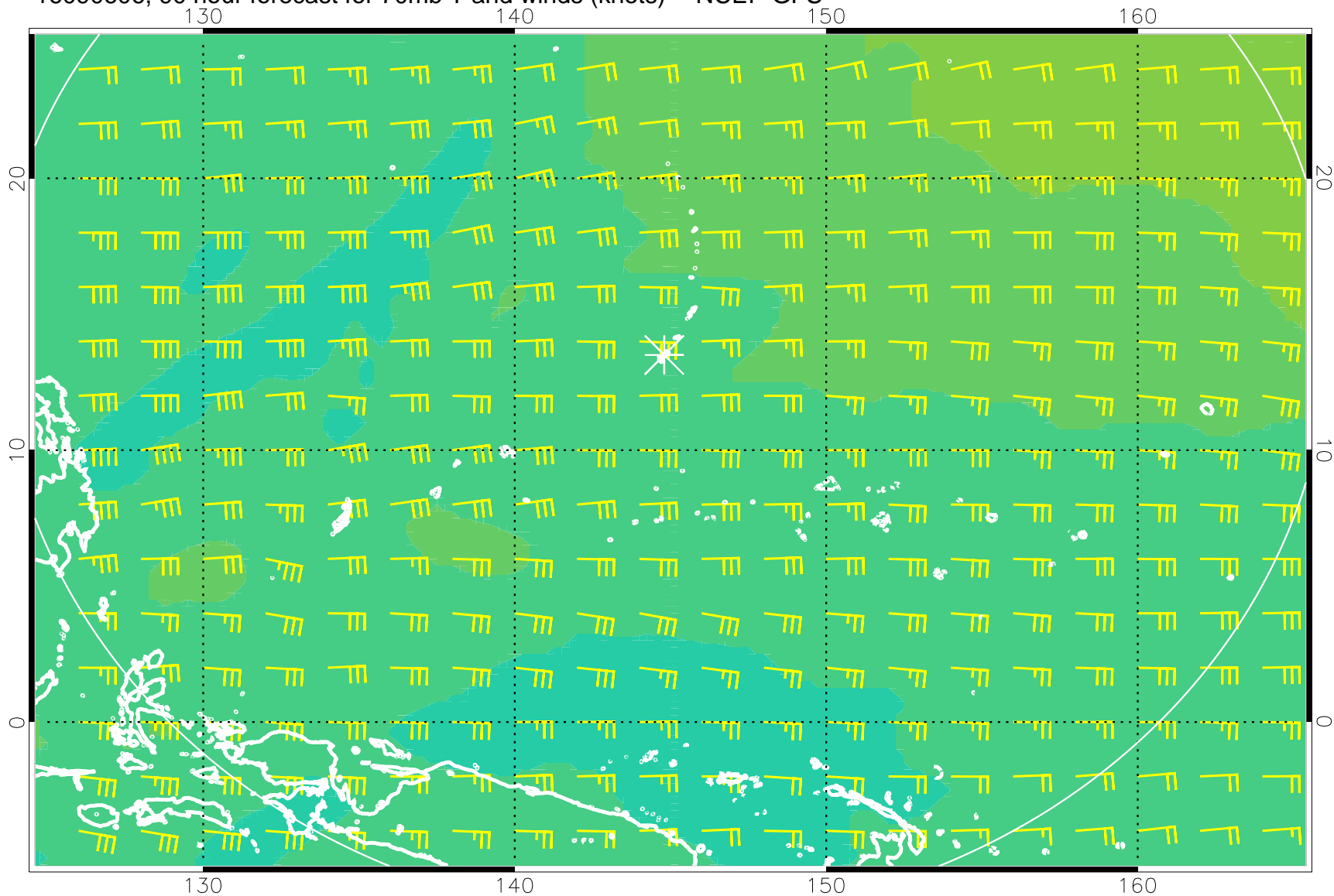
16090606, 90 hour forecast for 70mb T and winds (knots) -- NCEP GFS
