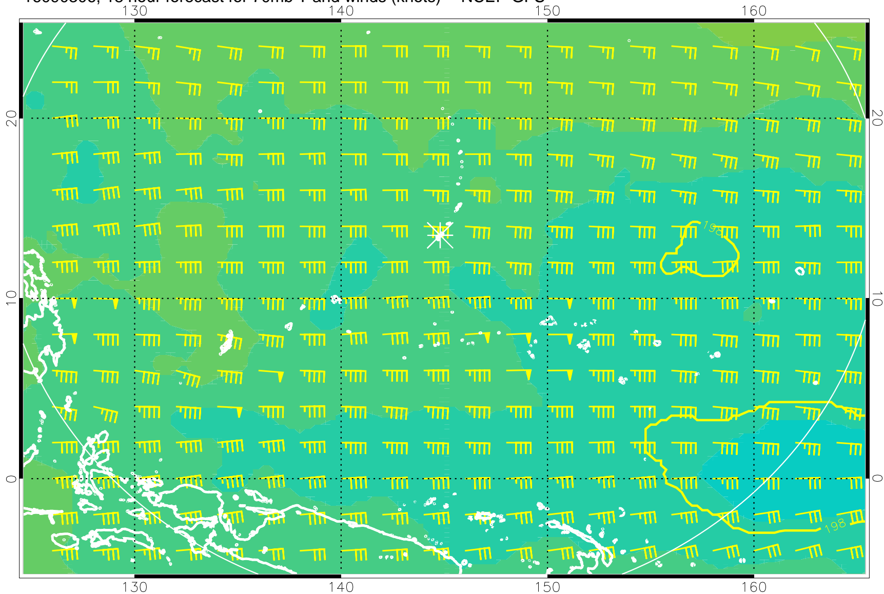
16090306, 18 hour forecast for 70mb T and winds (knots) -- NCEP GFS
