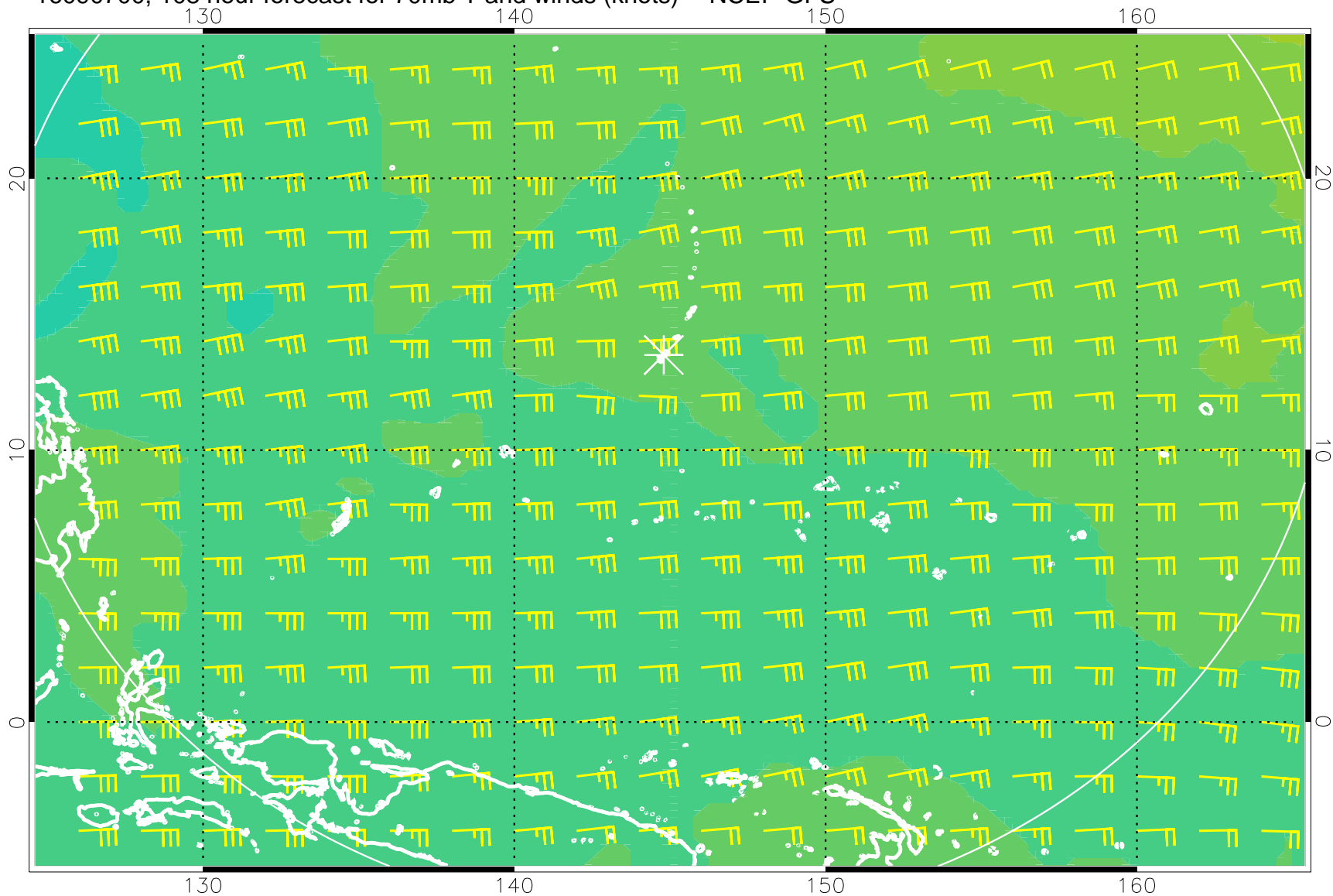
16090700, 108 hour forecast for 70mb T and winds (knots) -- NCEP GFS
