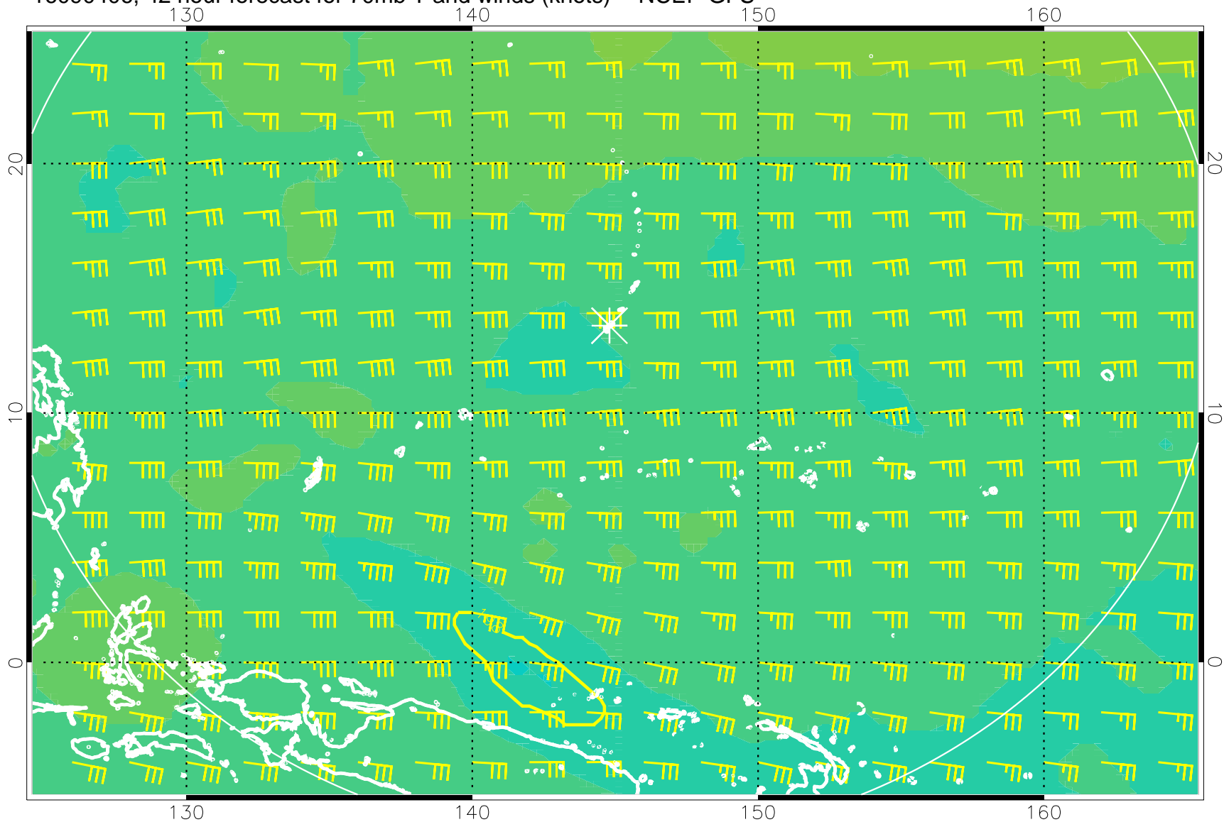
16090406, 42 hour forecast for 70mb T and winds (knots) -- NCEP GFS
