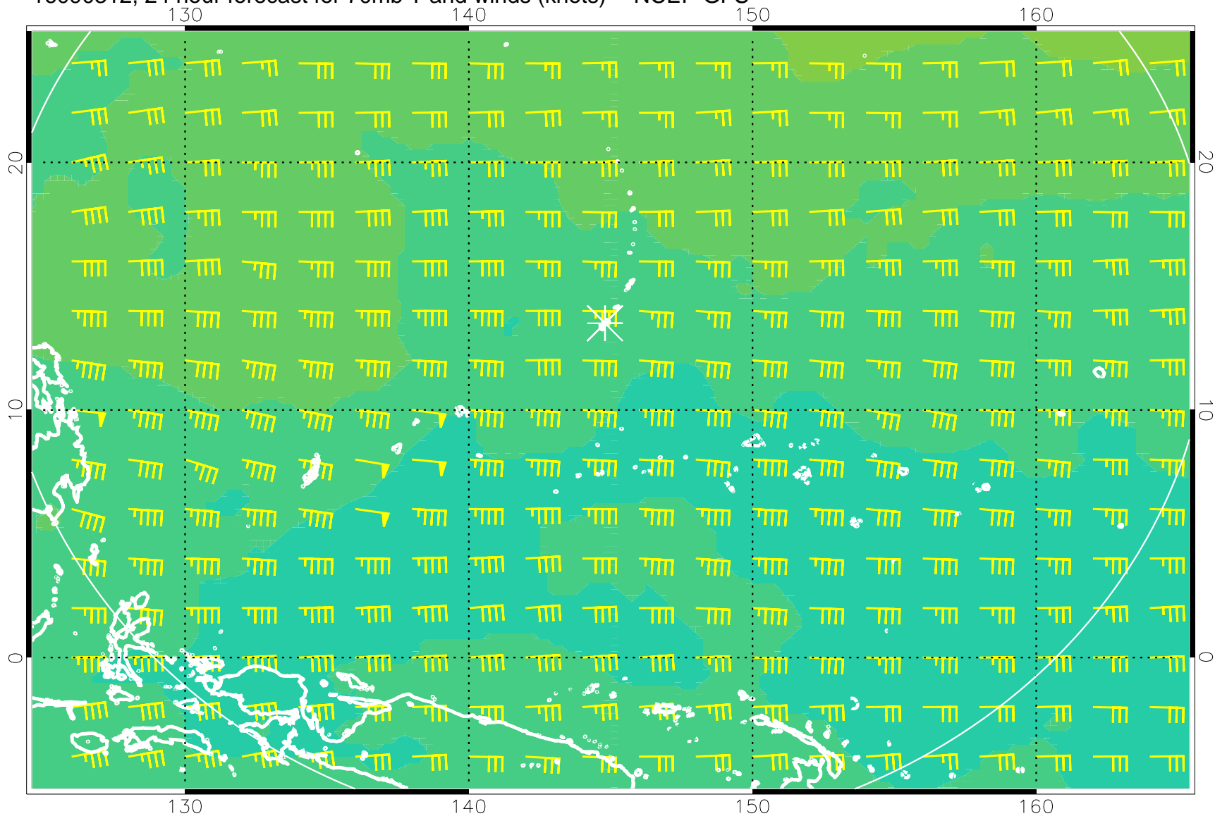
16090312, 24 hour forecast for 70mb T and winds (knots) -- NCEP GFS
