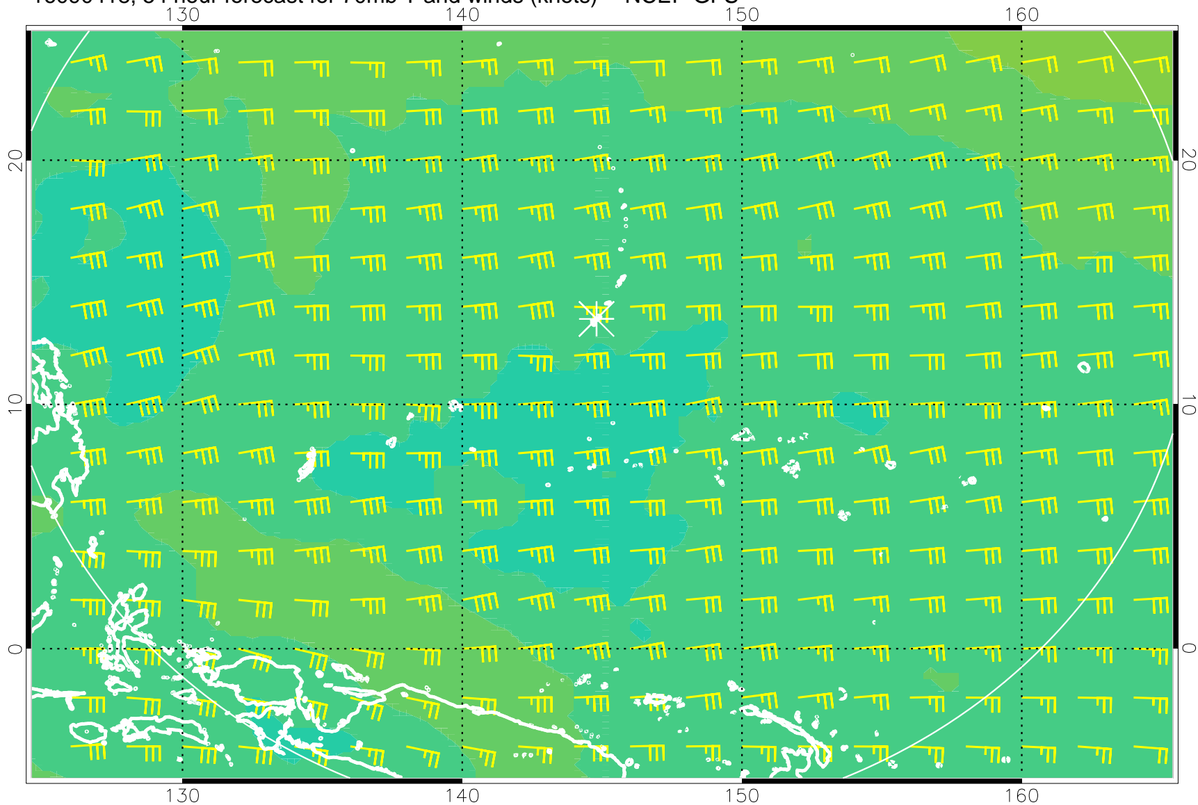
16090418, 54 hour forecast for 70mb T and winds (knots) -- NCEP GFS
