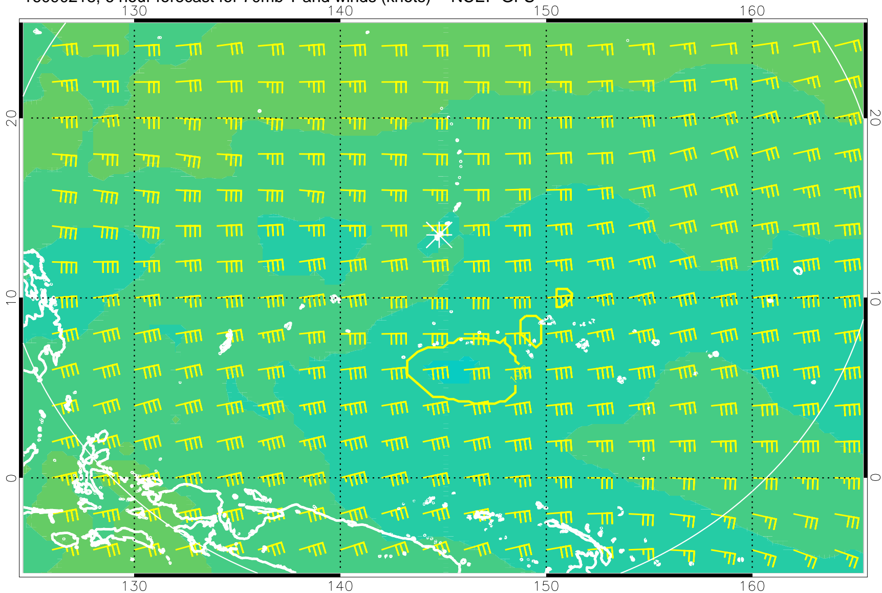
16090218, 6 hour forecast for 70mb T and winds (knots) -- NCEP GFS
