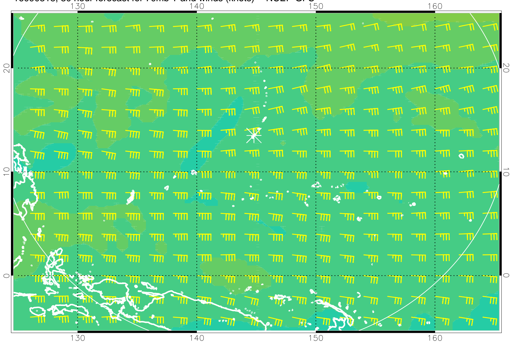
16090318, 30 hour forecast for 70mb T and winds (knots) -- NCEP GFS
