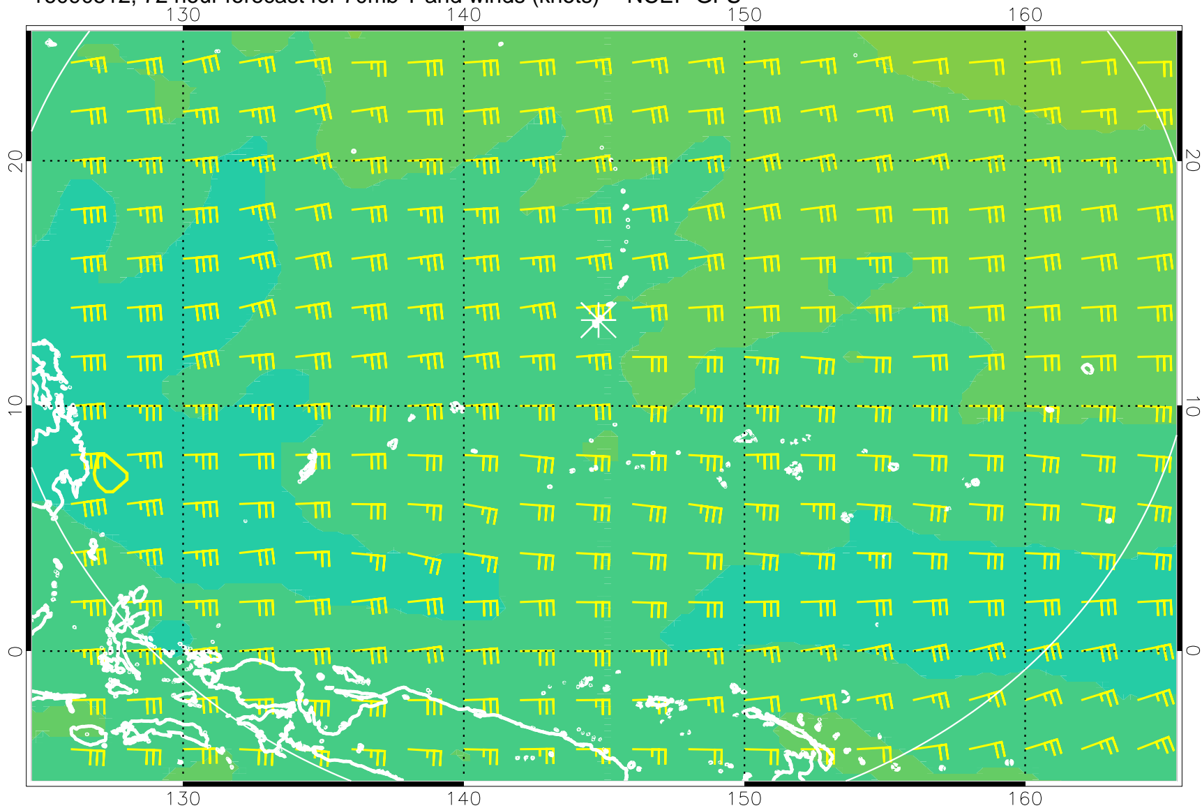
16090512, 72 hour forecast for 70mb T and winds (knots) -- NCEP GFS
