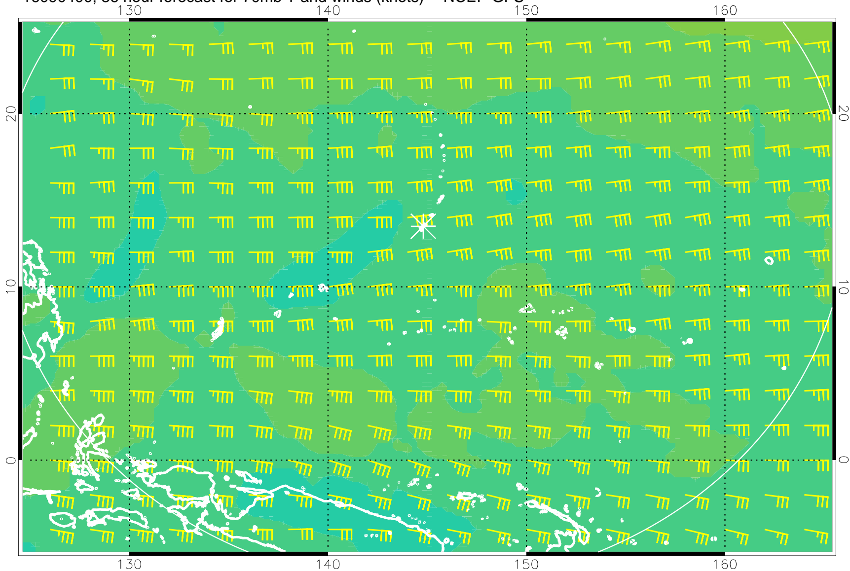
16090400, 36 hour forecast for 70mb T and winds (knots) -- NCEP GFS
