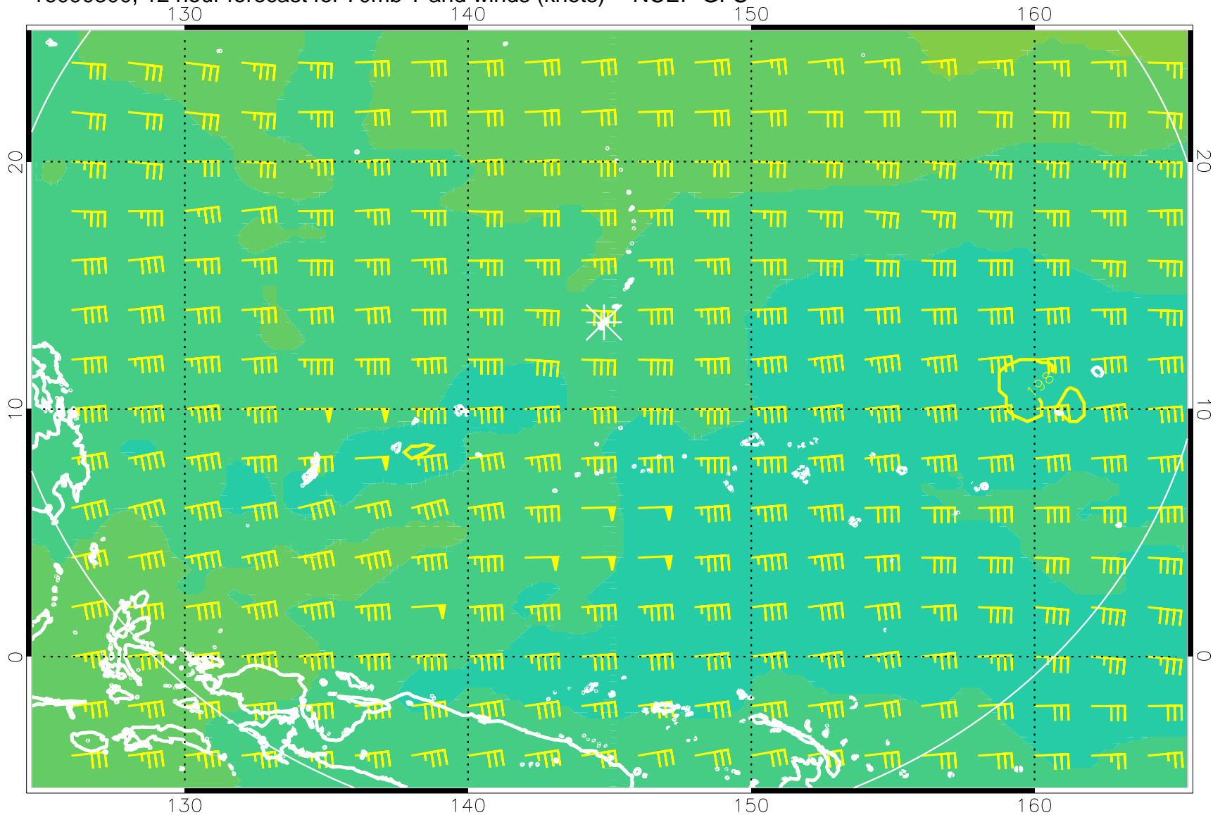
16090300, 12 hour forecast for 70mb T and winds (knots) -- NCEP GFS
