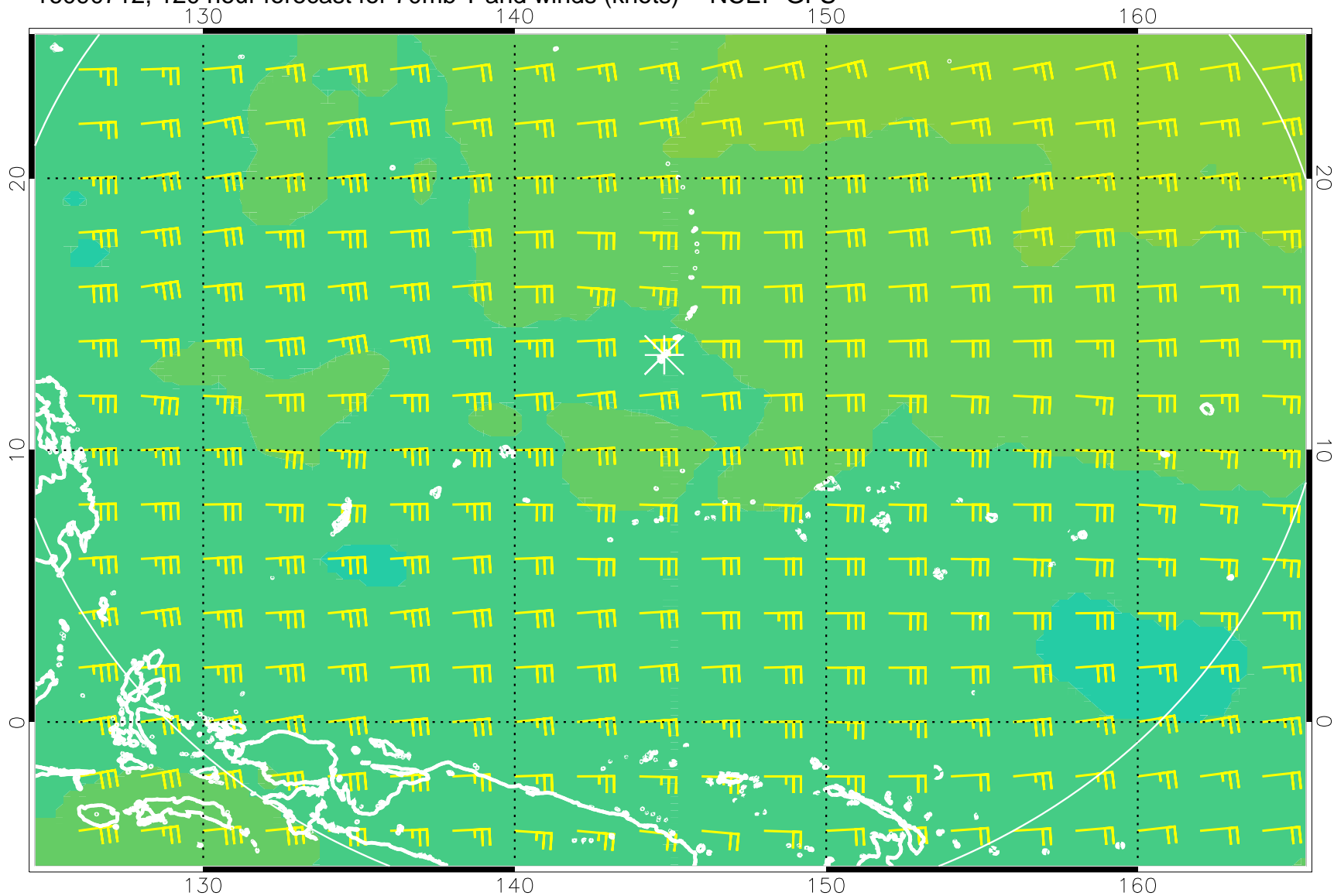
16090712, 120 hour forecast for 70mb T and winds (knots) -- NCEP GFS
