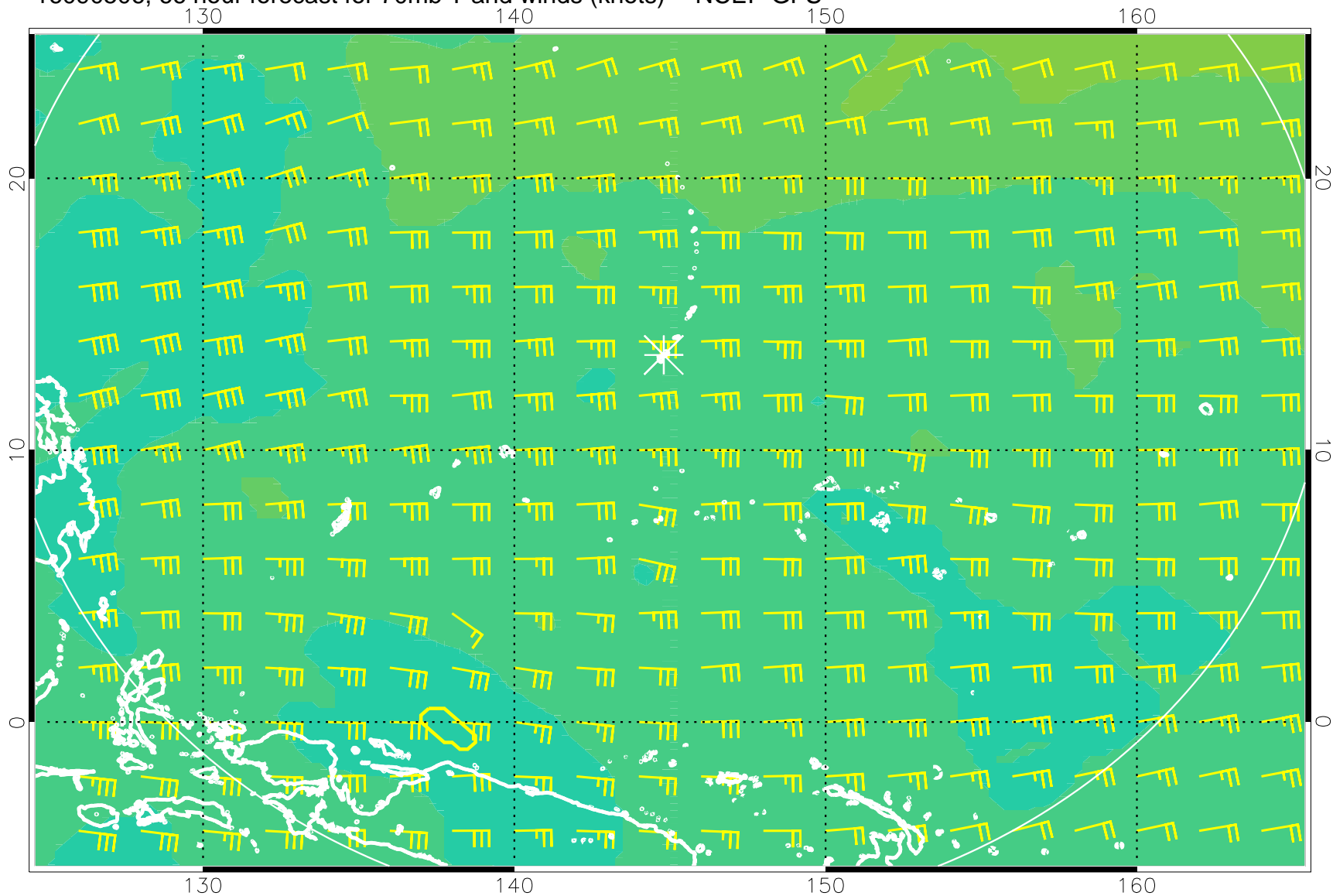
16090506, 66 hour forecast for 70mb T and winds (knots) -- NCEP GFS
