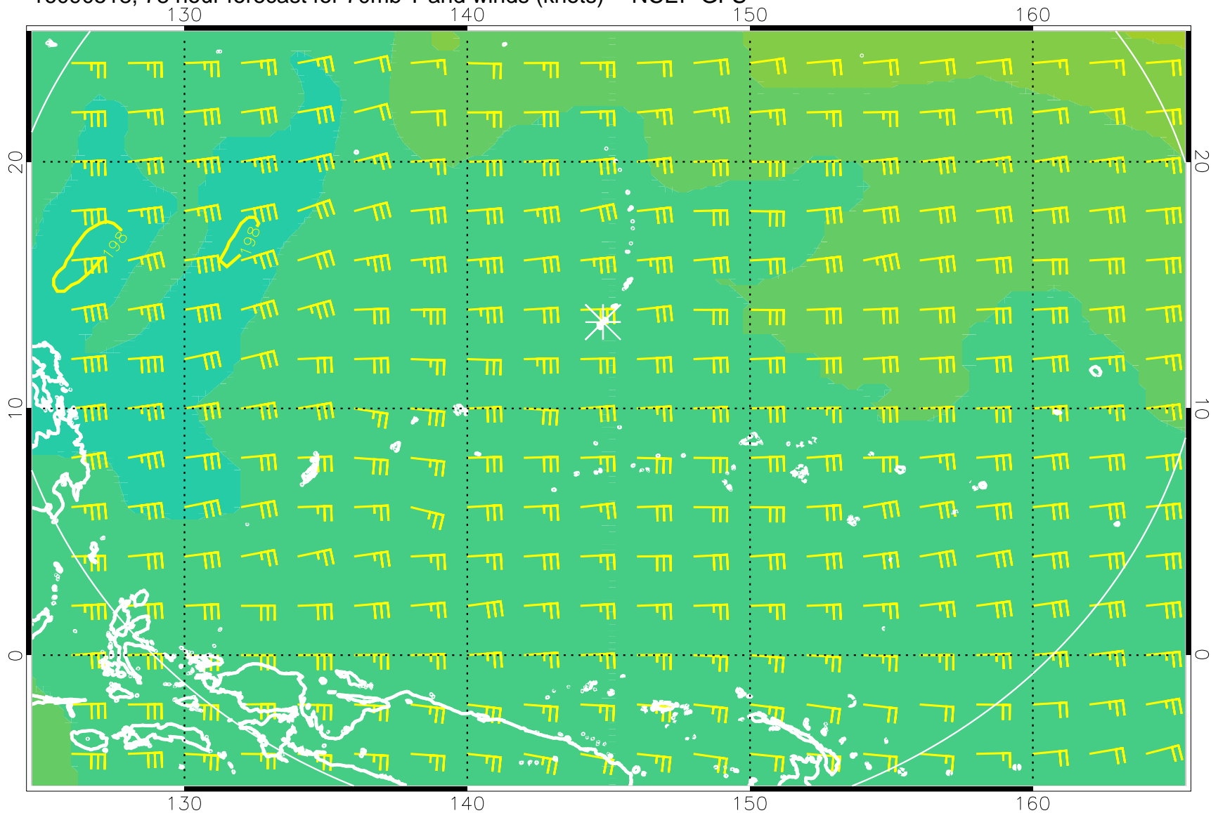
16090518, 78 hour forecast for 70mb T and winds (knots) -- NCEP GFS
