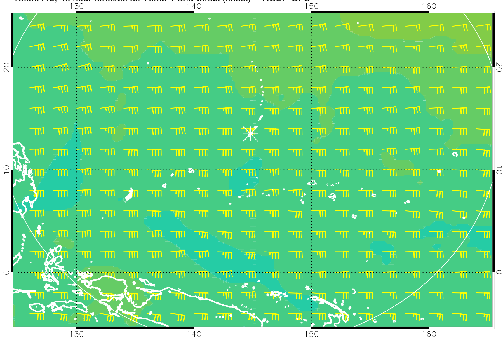
16090412, 48 hour forecast for 70mb T and winds (knots) -- NCEP GFS
