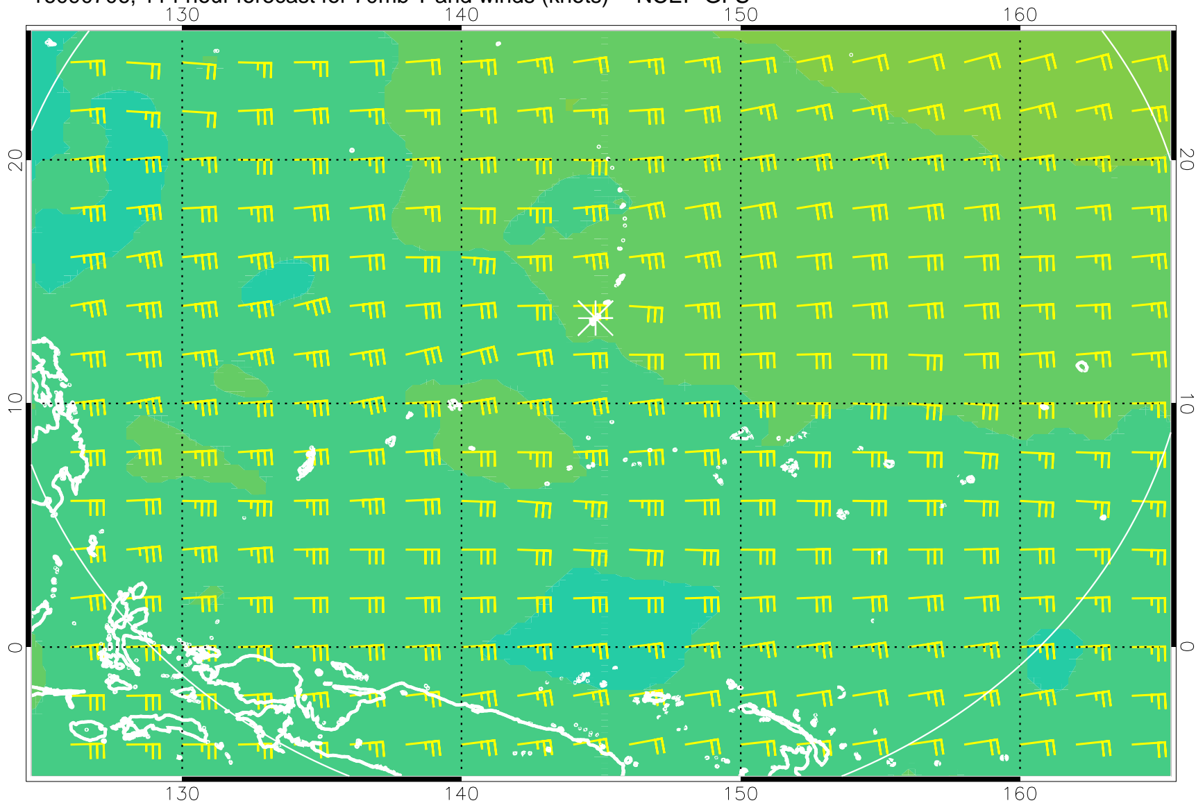
16090706, 114 hour forecast for 70mb T and winds (knots) -- NCEP GFS
