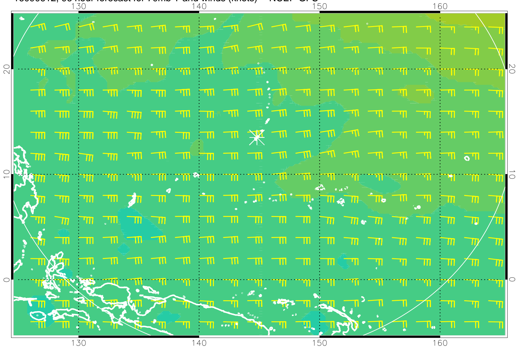
16090612, 96 hour forecast for 70mb T and winds (knots) -- NCEP GFS
