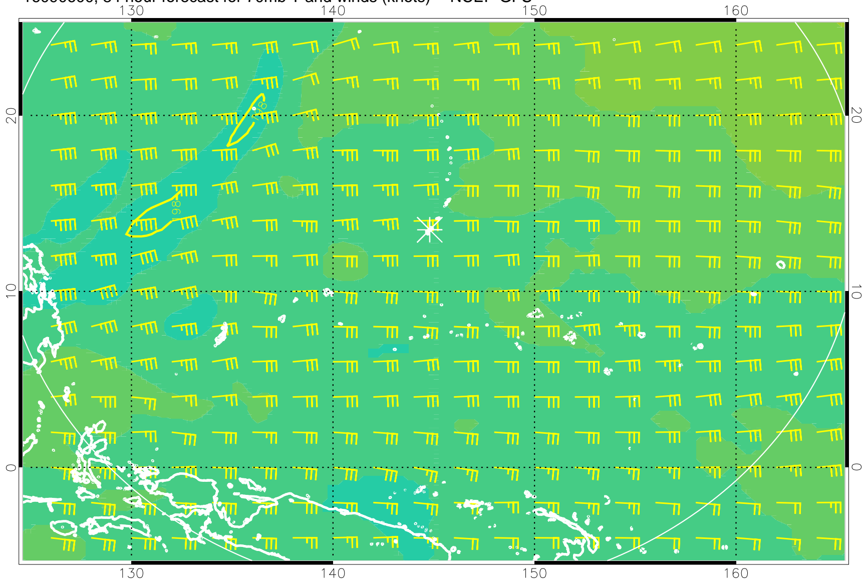
16090600, 84 hour forecast for 70mb T and winds (knots) -- NCEP GFS
