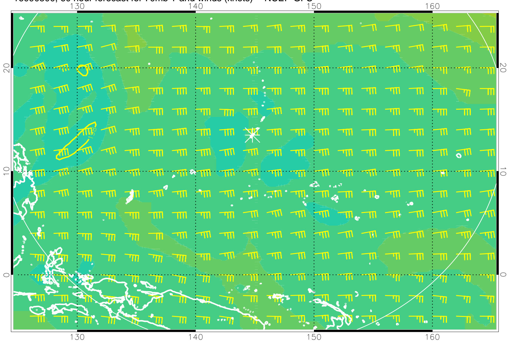
16090500, 60 hour forecast for 70mb T and winds (knots) -- NCEP GFS
