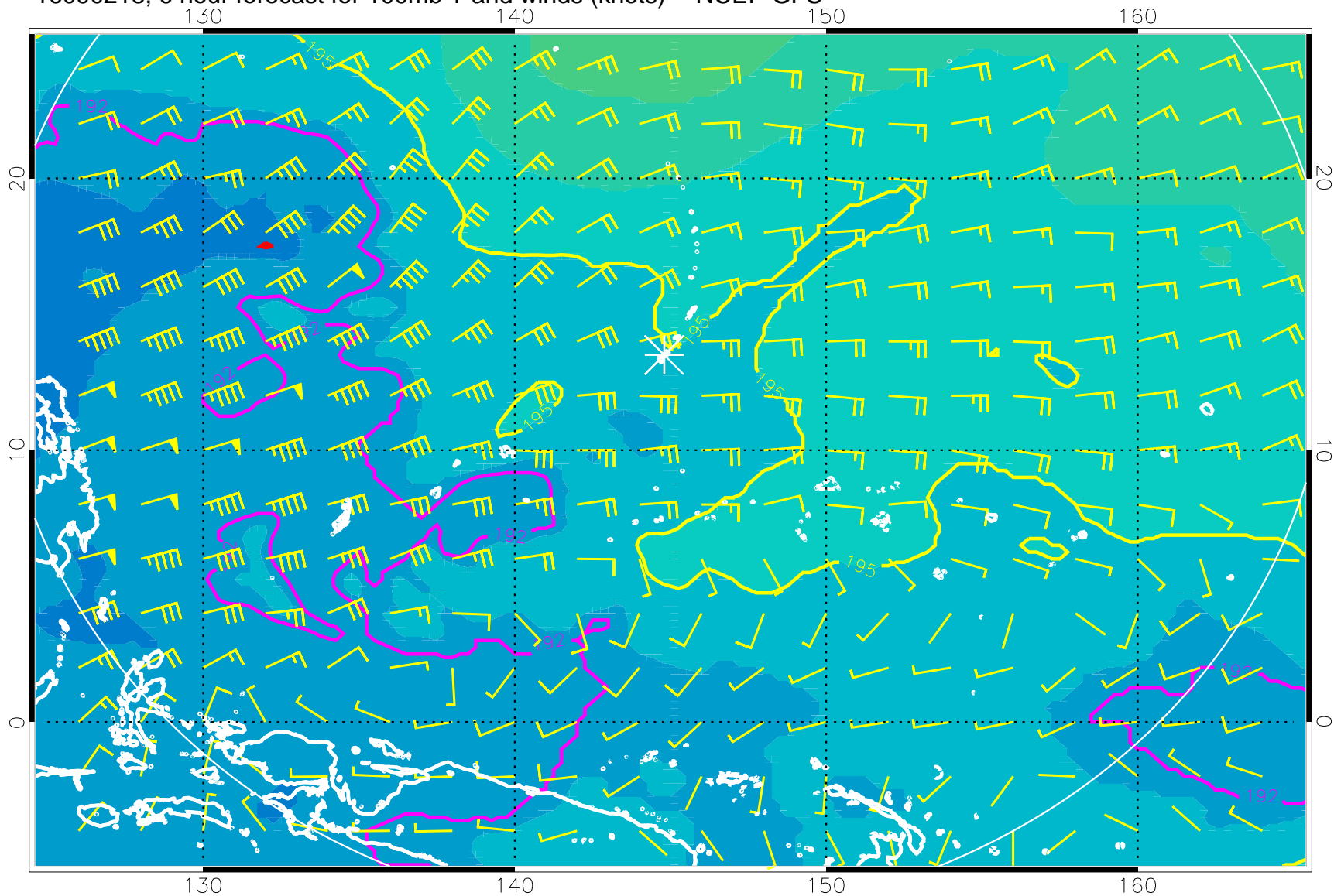
16090218, 6 hour forecast for 100mb T and winds (knots) -- NCEP GFS
