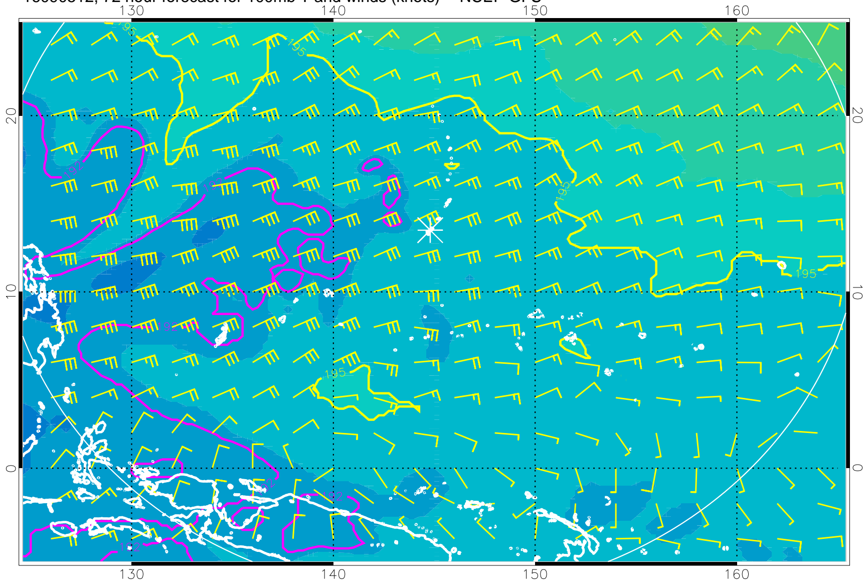
16090512, 72 hour forecast for 100mb T and winds (knots) -- NCEP GFS
