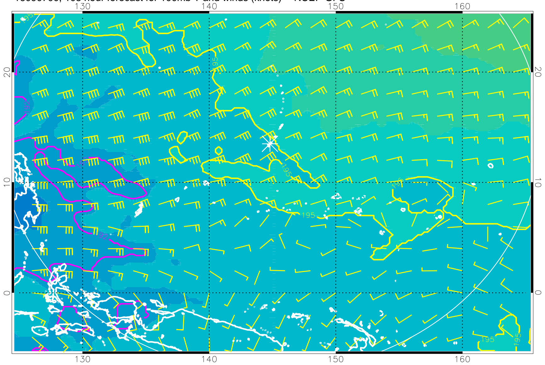
16090700, 108 hour forecast for 100mb T and winds (knots) -- NCEP GFS
