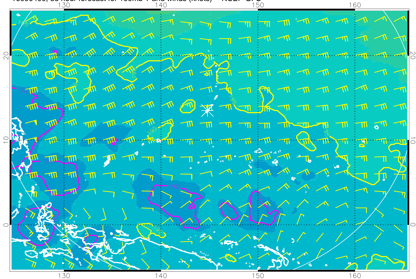
16090400, 36 hour forecast for 100mb T and winds (knots) -- NCEP GFS
