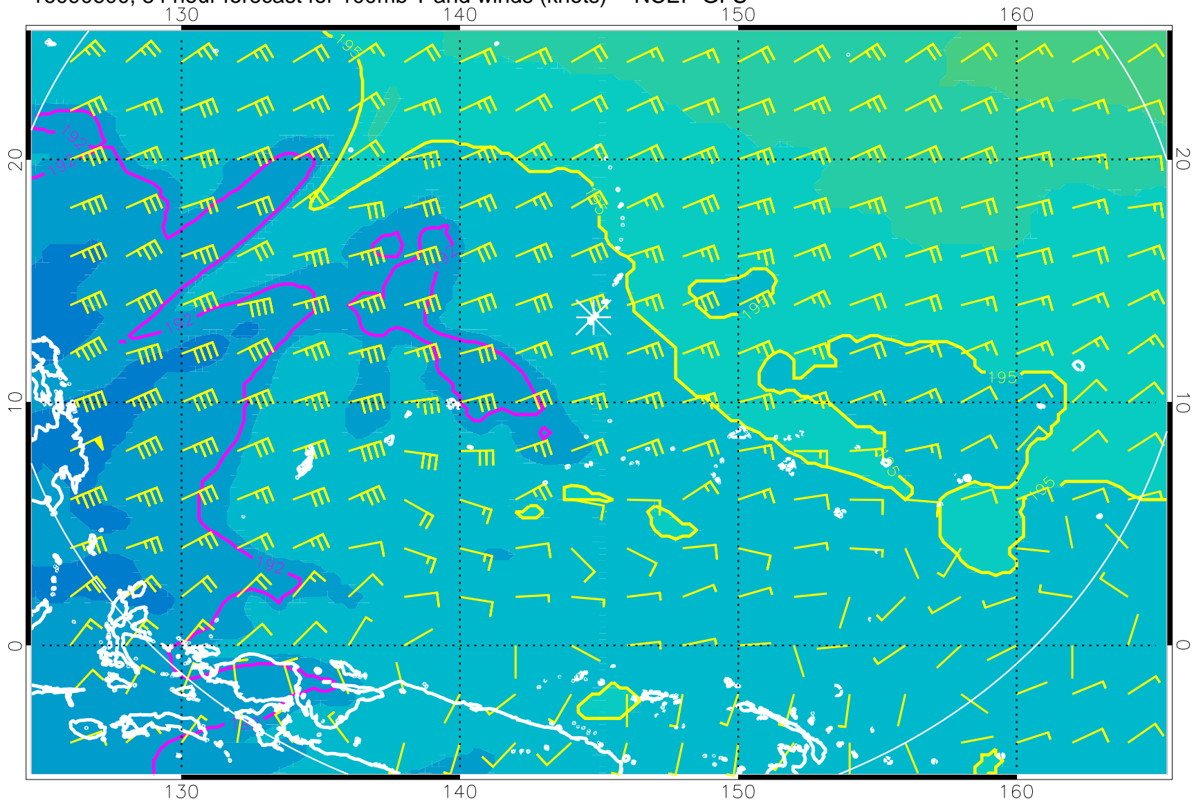
16090600, 84 hour forecast for 100mb T and winds (knots) -- NCEP GFS
