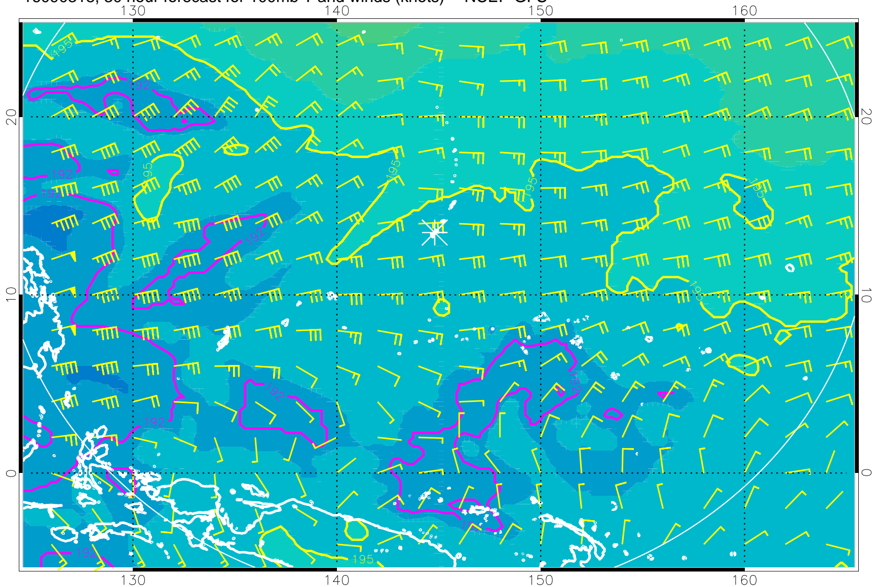
16090318, 30 hour forecast for 100mb T and winds (knots) -- NCEP GFS
