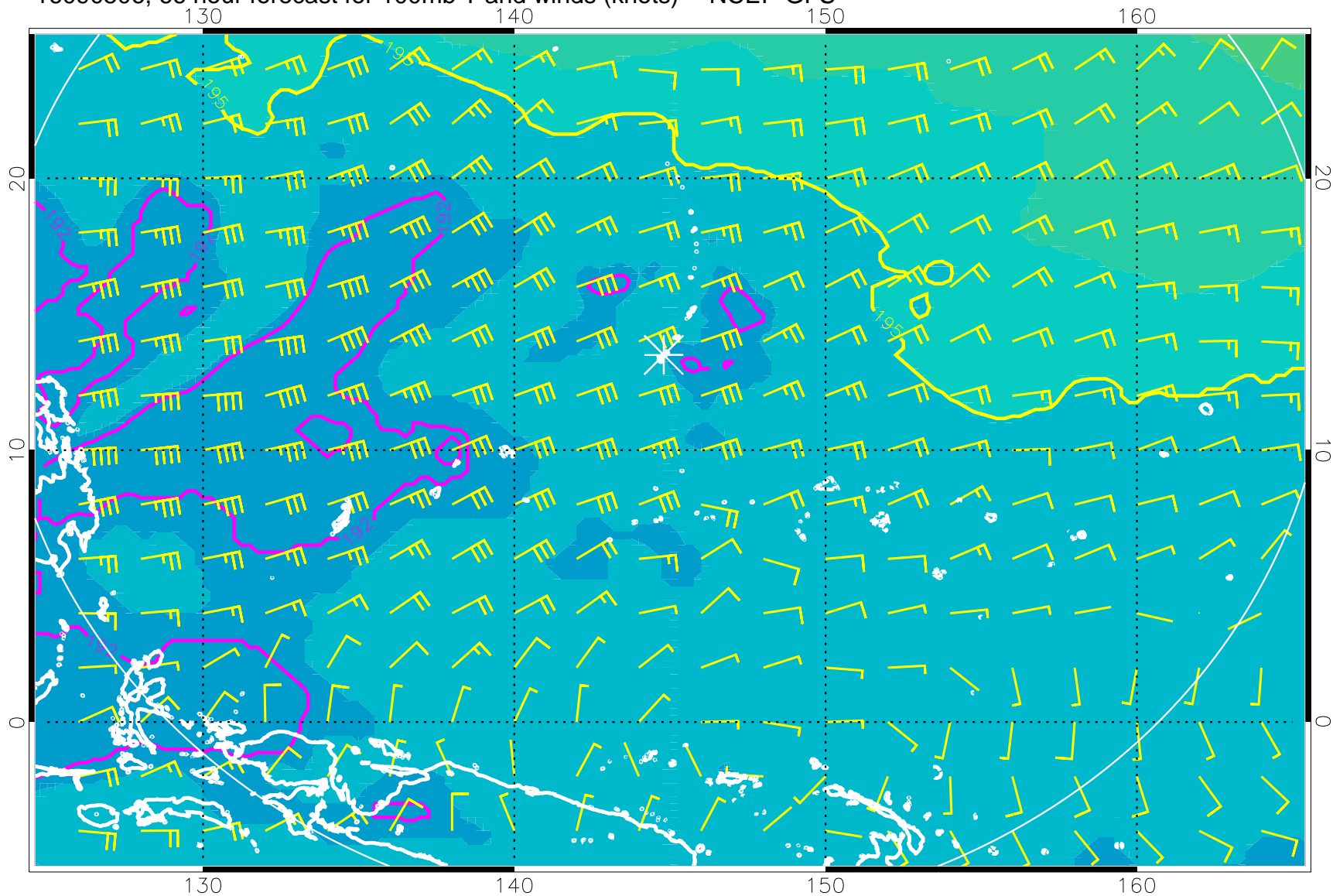
16090506, 66 hour forecast for 100mb T and winds (knots) -- NCEP GFS
