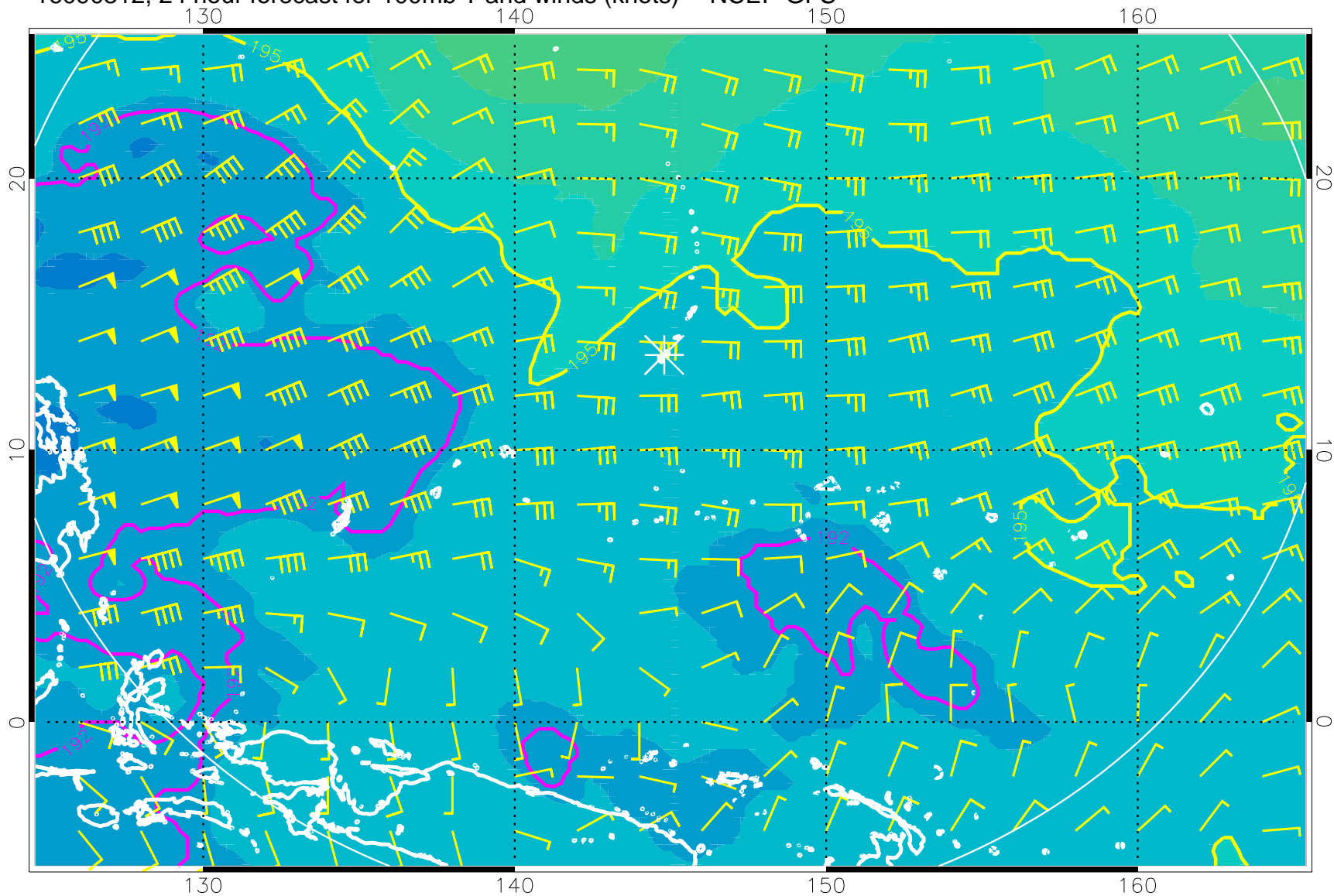
16090312, 24 hour forecast for 100mb T and winds (knots) -- NCEP GFS
