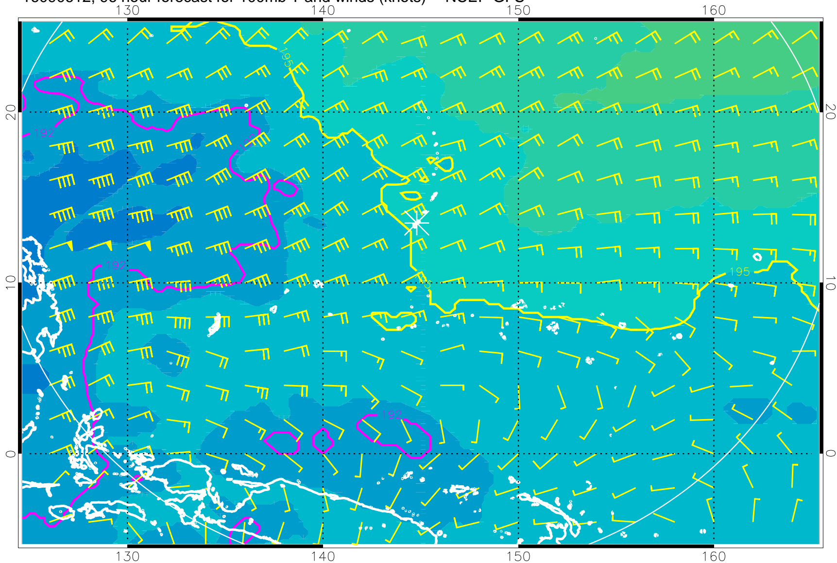
16090612, 96 hour forecast for 100mb T and winds (knots) -- NCEP GFS
