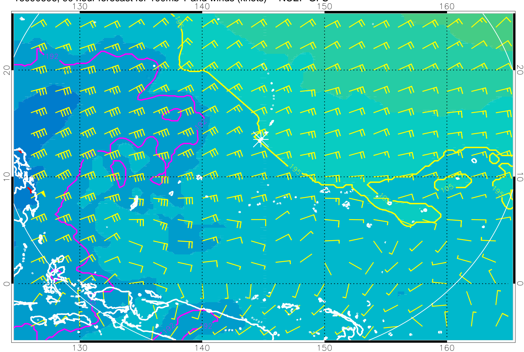
16090606, 90 hour forecast for 100mb T and winds (knots) -- NCEP GFS
