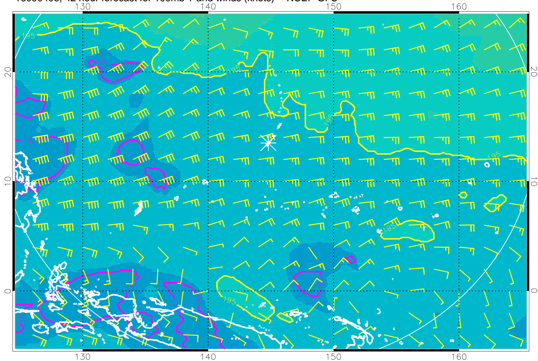
16090406, 42 hour forecast for 100mb T and winds (knots) -- NCEP GFS
