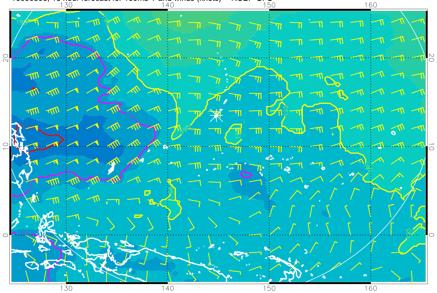
16090306, 18 hour forecast for 100mb T and winds (knots) -- NCEP GFS
