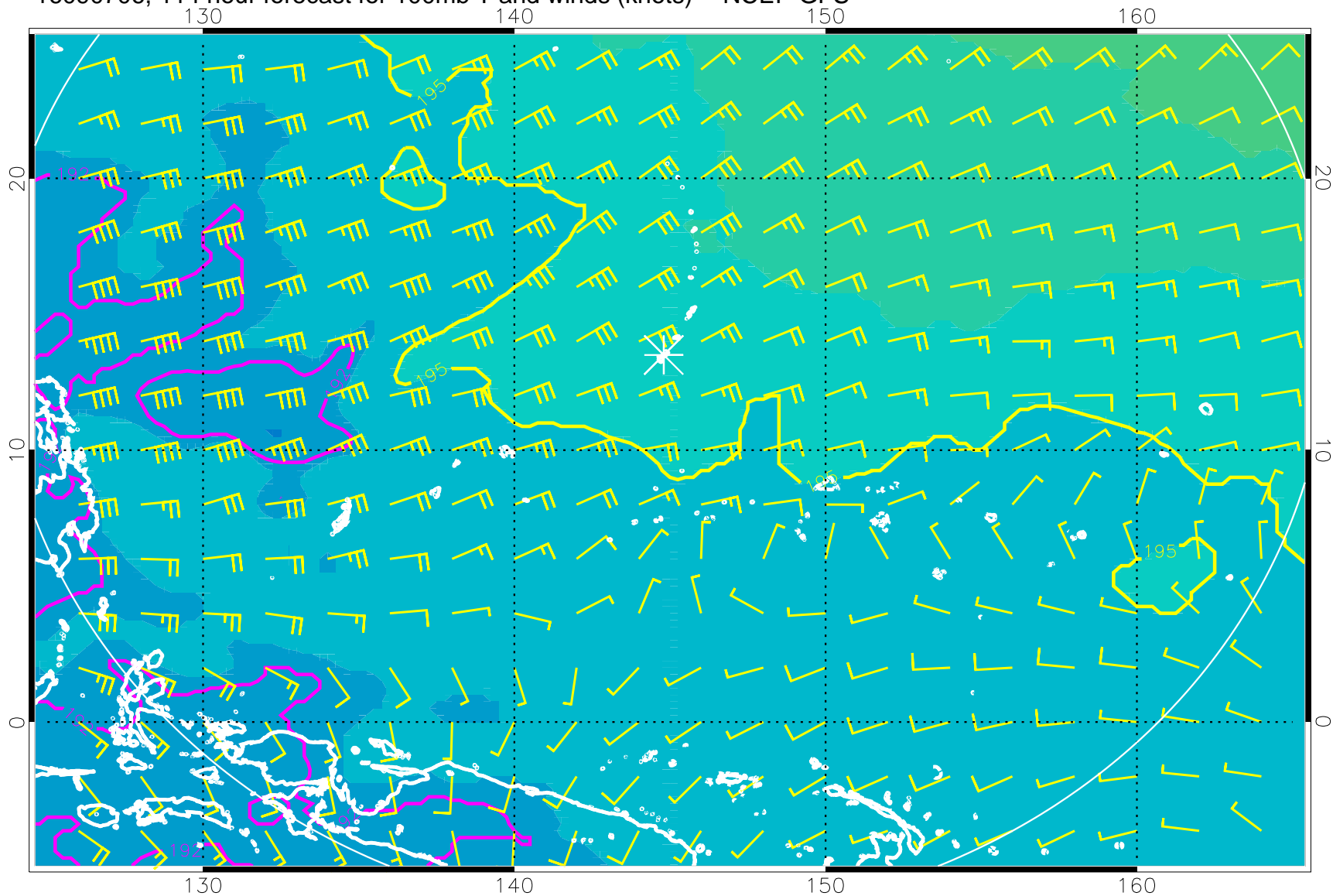
16090706, 114 hour forecast for 100mb T and winds (knots) -- NCEP GFS
