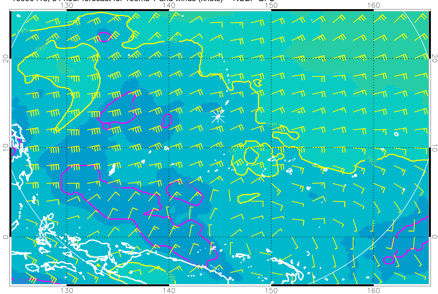
16090418, 54 hour forecast for 100mb T and winds (knots) -- NCEP GFS
