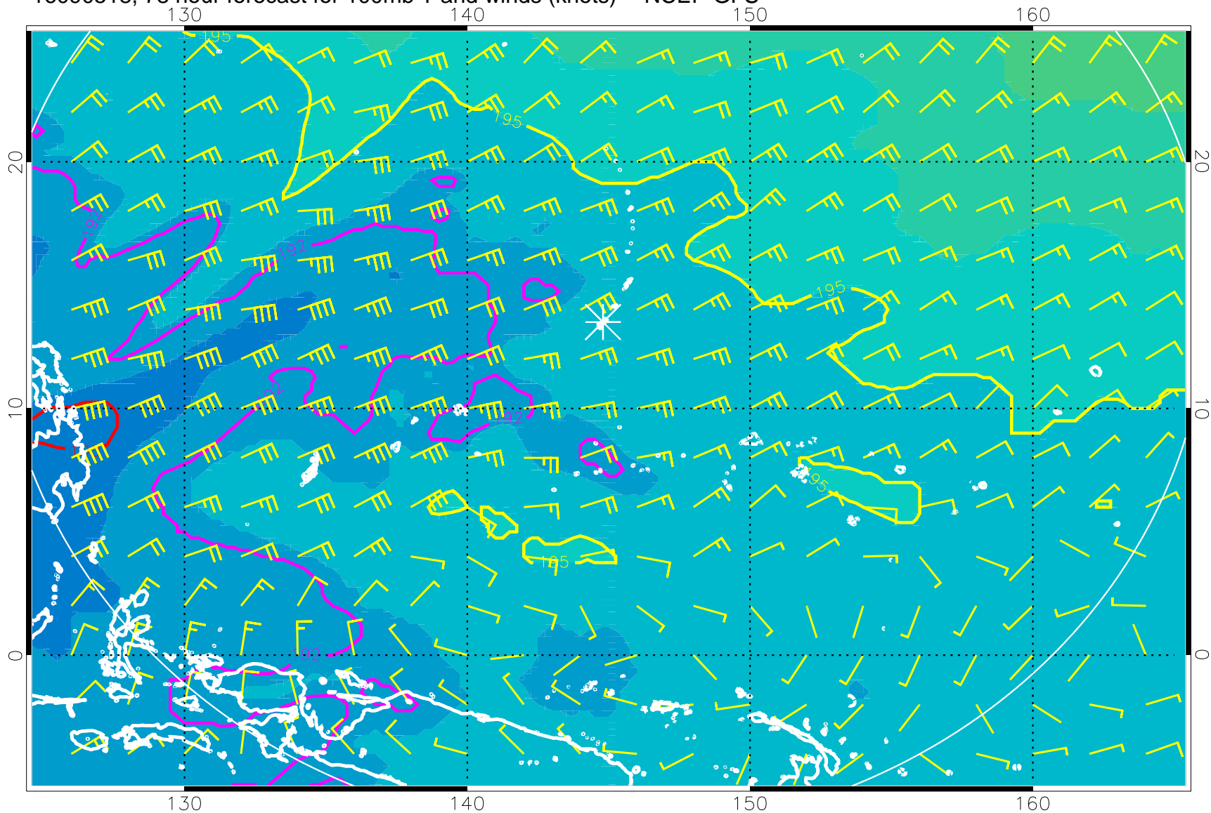
16090518, 78 hour forecast for 100mb T and winds (knots) -- NCEP GFS
