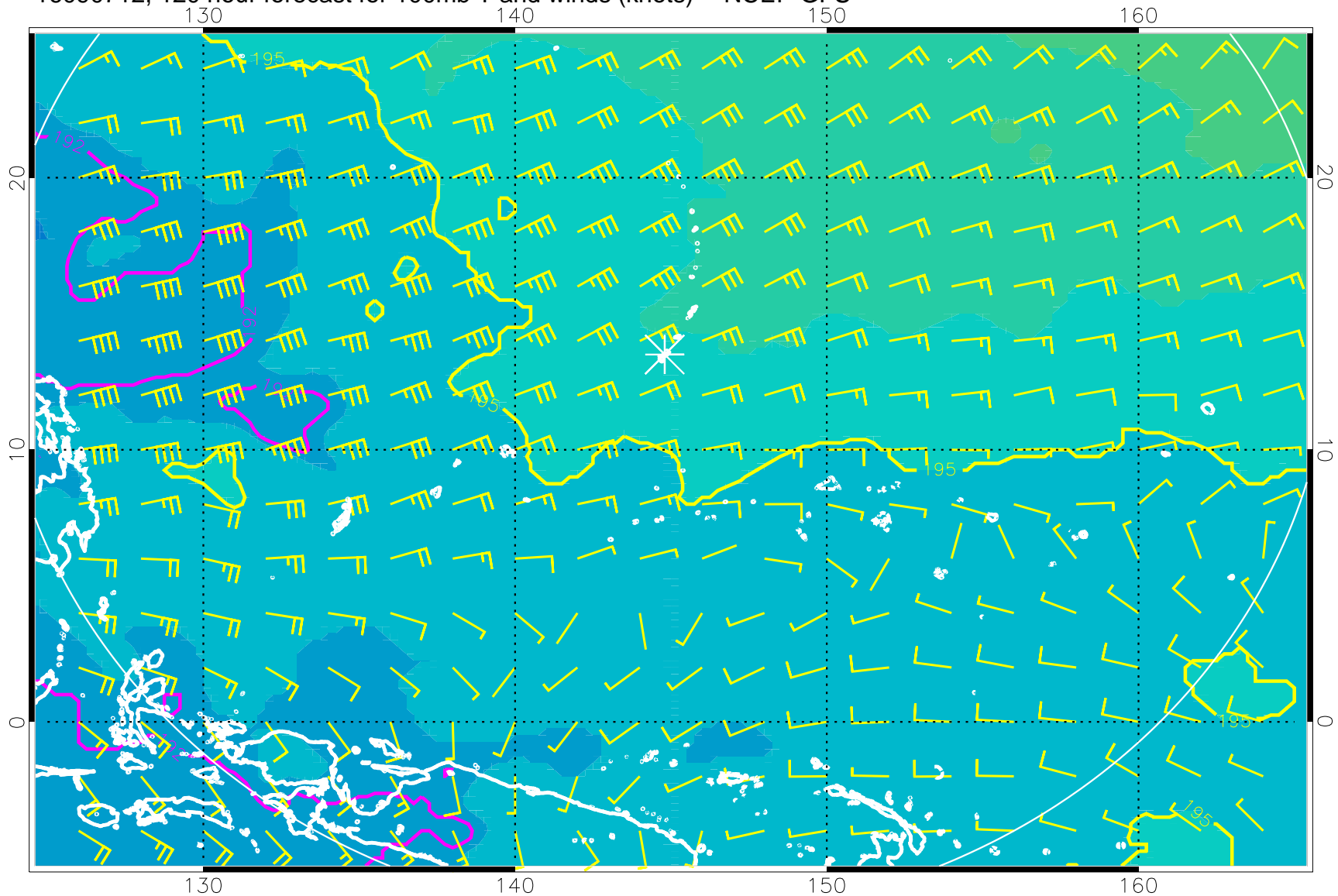
16090712, 120 hour forecast for 100mb T and winds (knots) -- NCEP GFS
