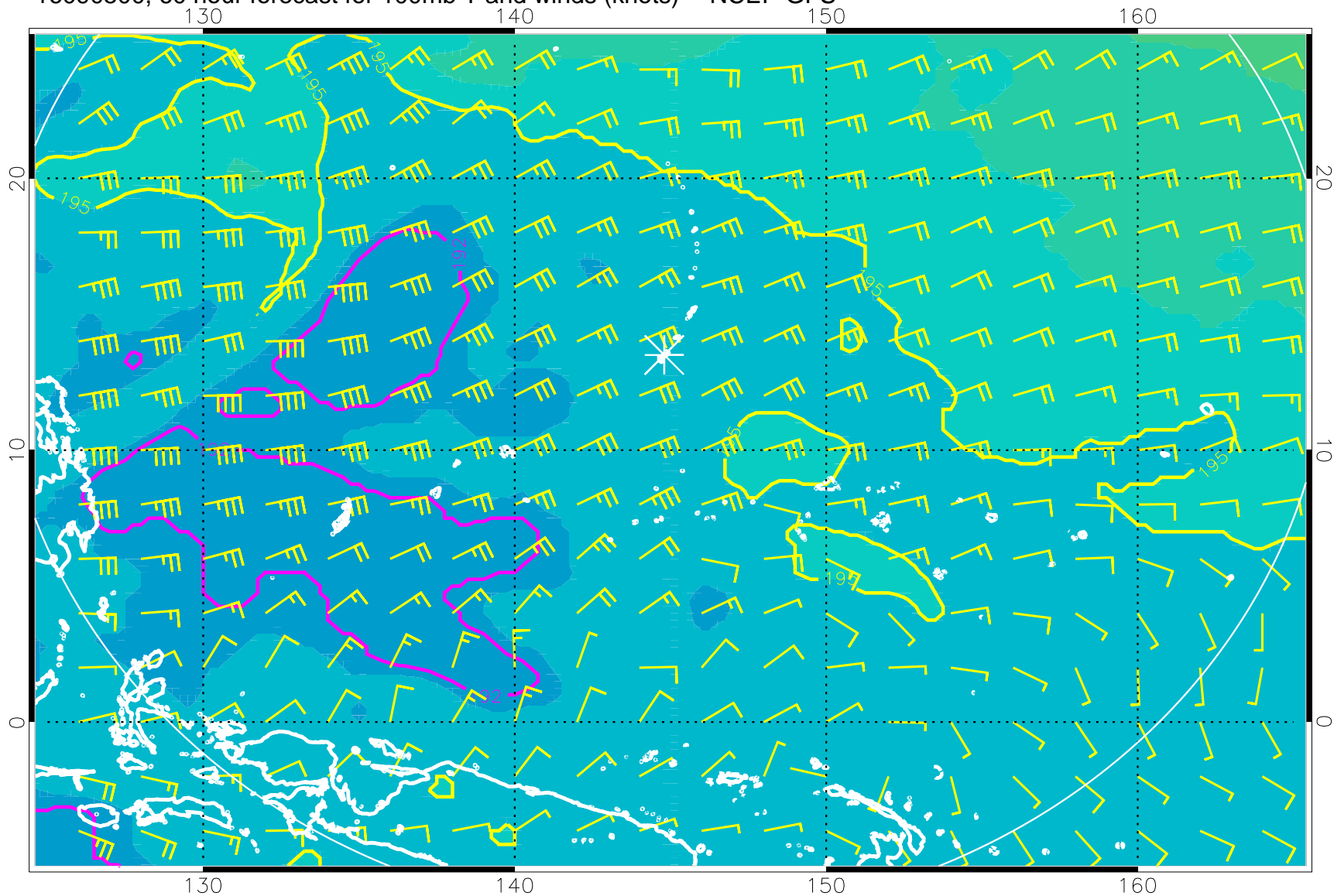
16090500, 60 hour forecast for 100mb T and winds (knots) -- NCEP GFS
