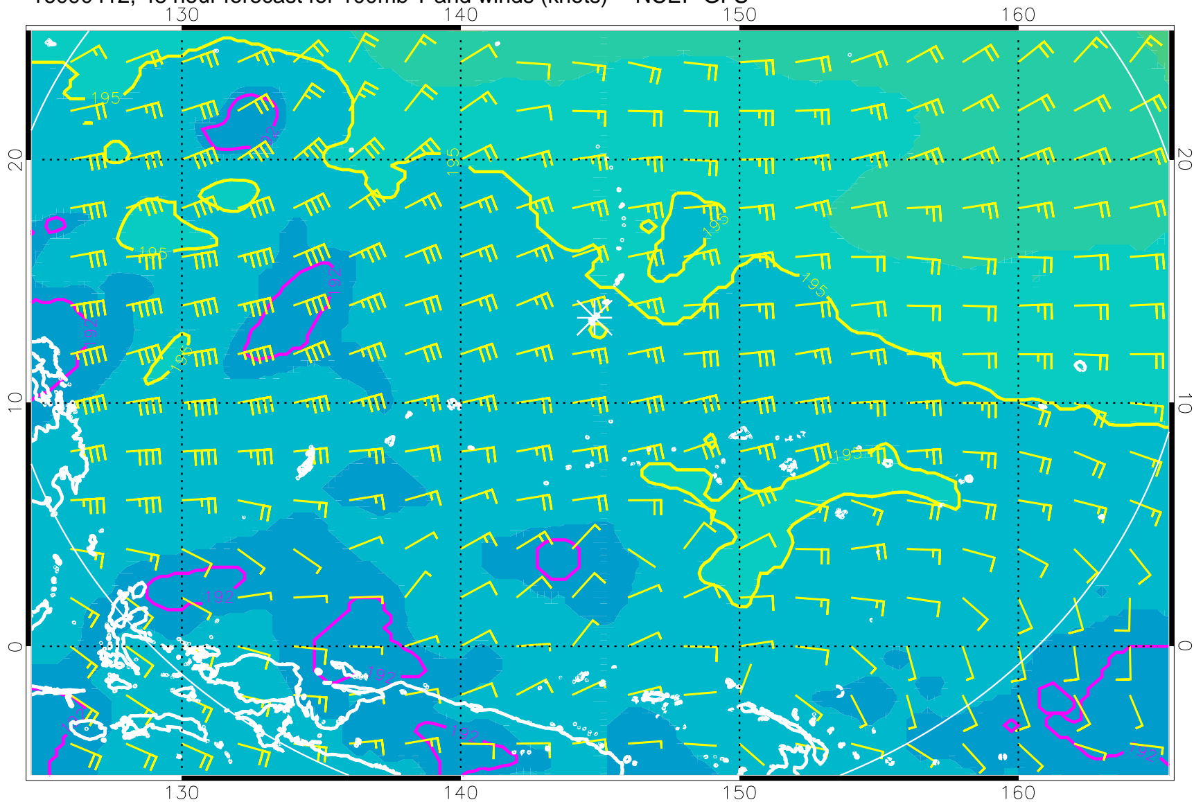
16090412, 48 hour forecast for 100mb T and winds (knots) -- NCEP GFS
