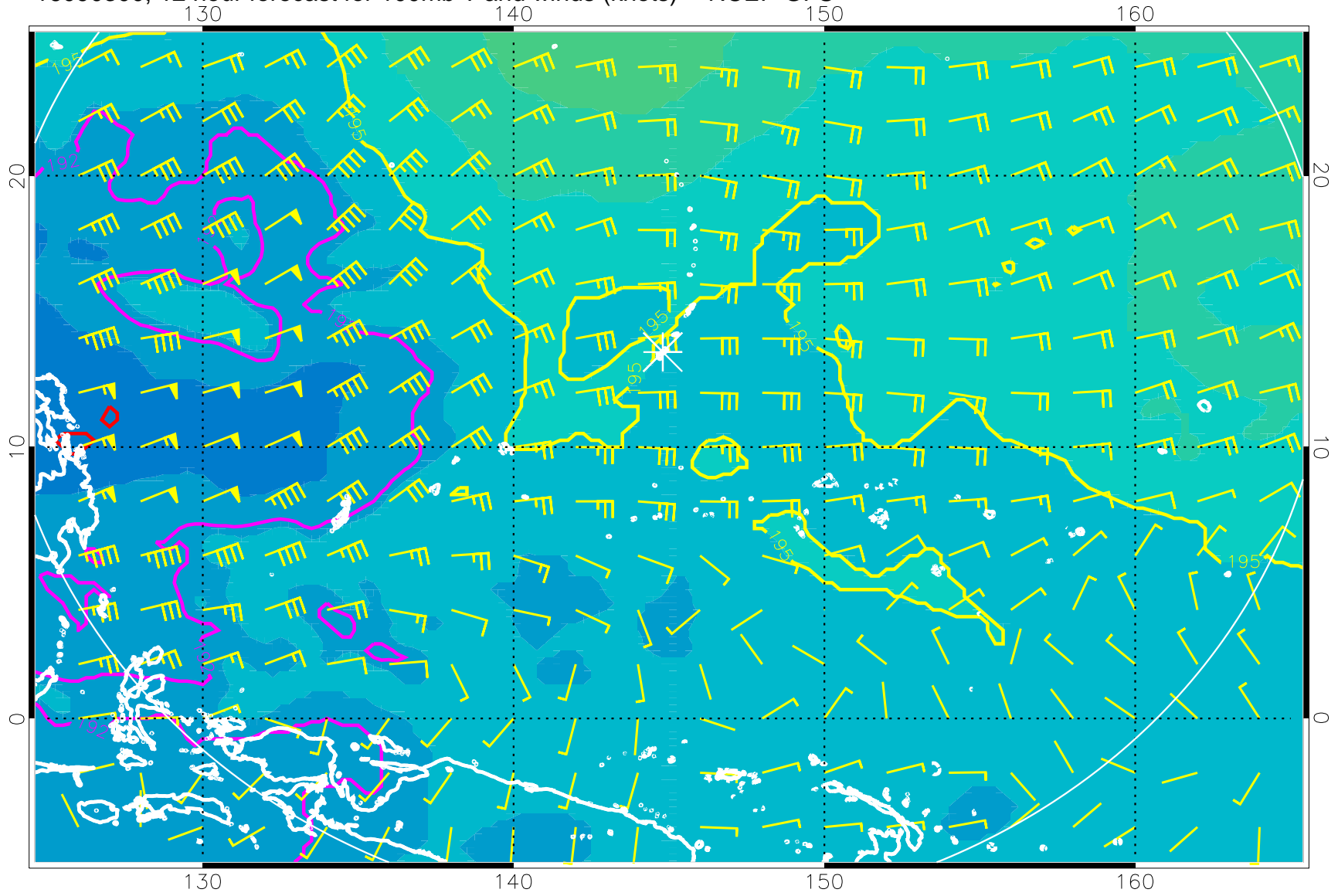
16090300, 12 hour forecast for 100mb T and winds (knots) -- NCEP GFS
