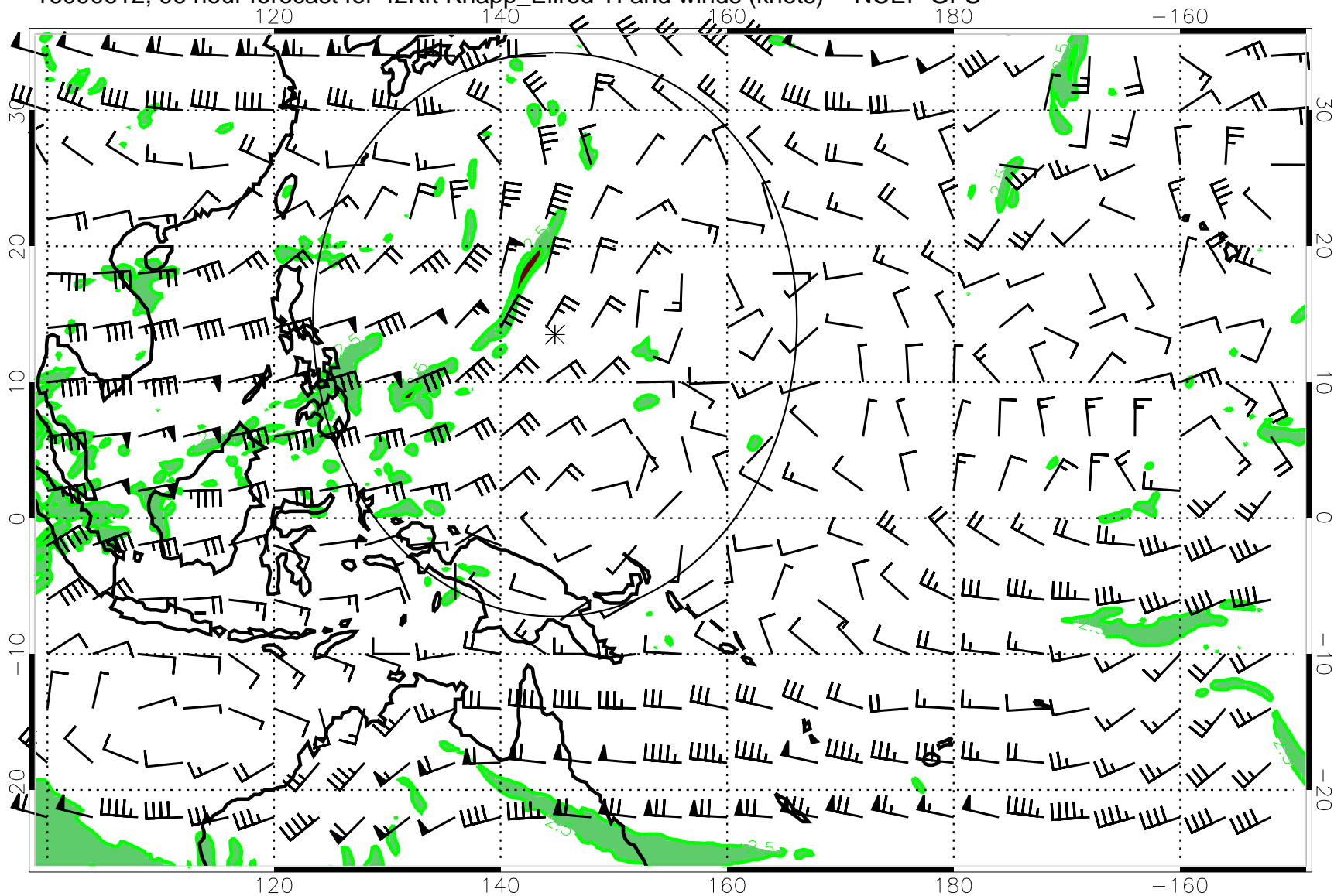
16090612, 96 hour forecast for 42Kft Knapp_Ellrod TI and winds (knots) -- NCEP GFS
